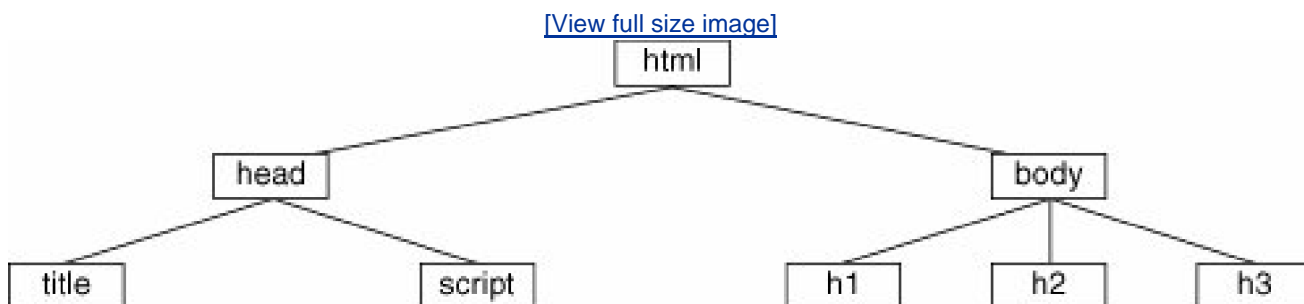
Figure 15-1. Graphic depiction of HTML document in Listing 15-1
