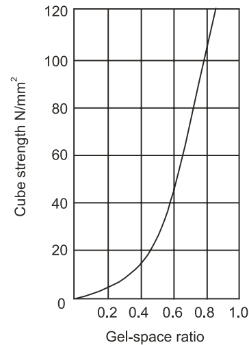
Fig. 10.16 Relation between Compressive Strength of the Mortar and Gel-Space Ratio
