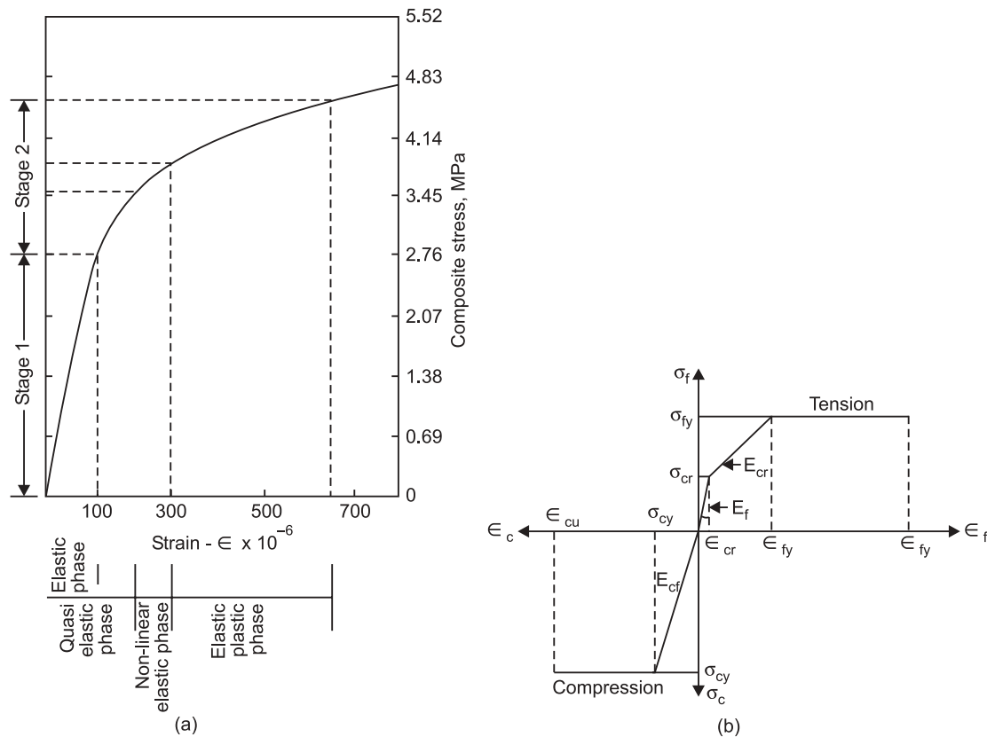
Figure 20.4 Stress-strain Curves of Ferrocement in Tension and Compression
