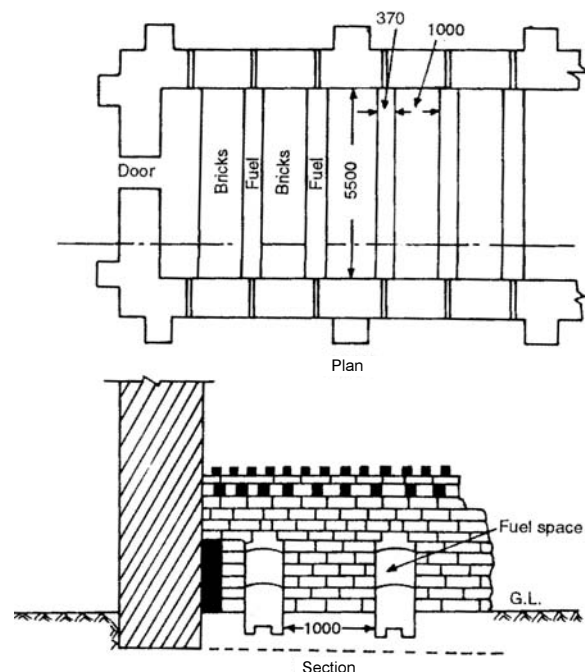
Fig. 2.10 Intermittent Kiln
