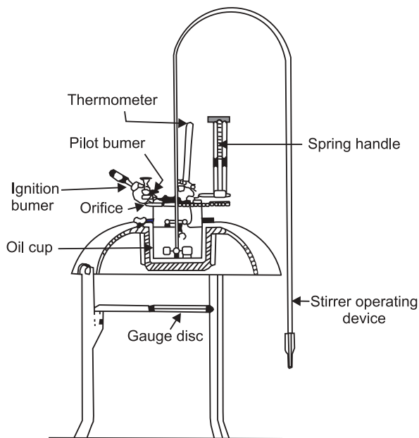
Fig. 18.6 Pensky-Marten test
