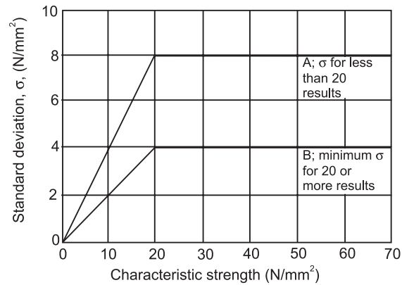
Fig. 11.6 Standard Deviation Vs Characteristic Specified Strength
