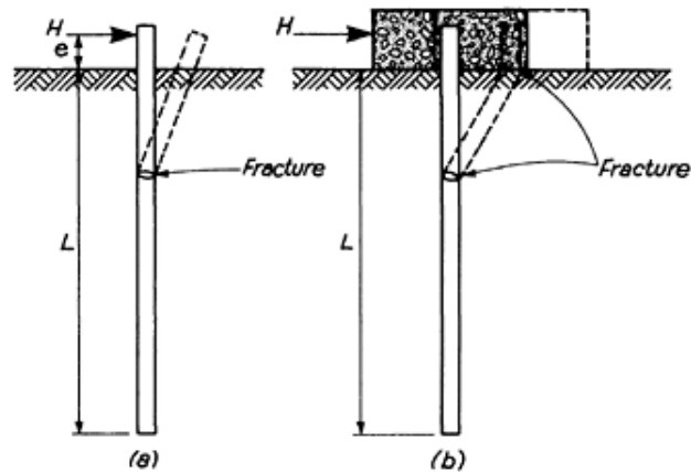
Fig. 6.19 Long vertical pile under horizontal load
