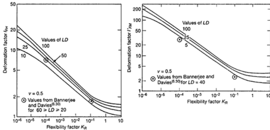
Fig. 6.53 Deformation factors for fixed-head piles (after Poulos (6.27) )
