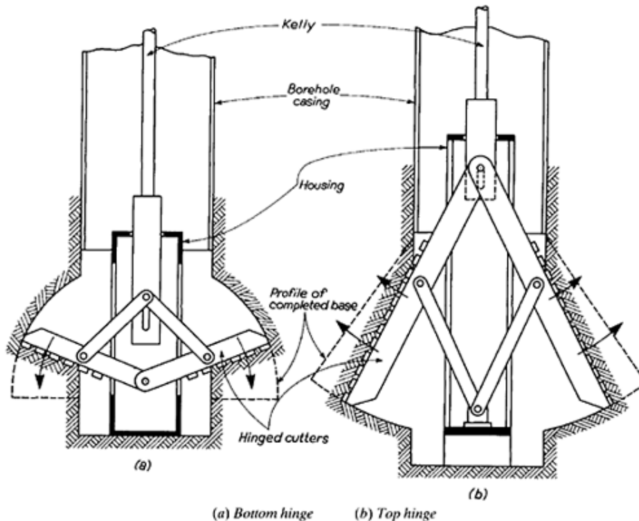
Fig. 3.29 Under-reaming tools
