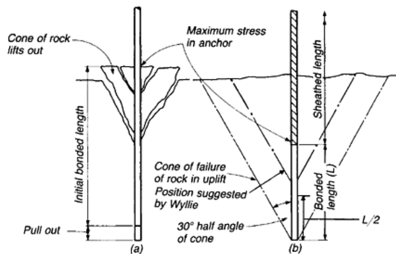
Fig. 6.12 Pull-out of cone of rock
