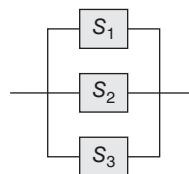
Figure 13.24 RBD for Exercise 13.8.
