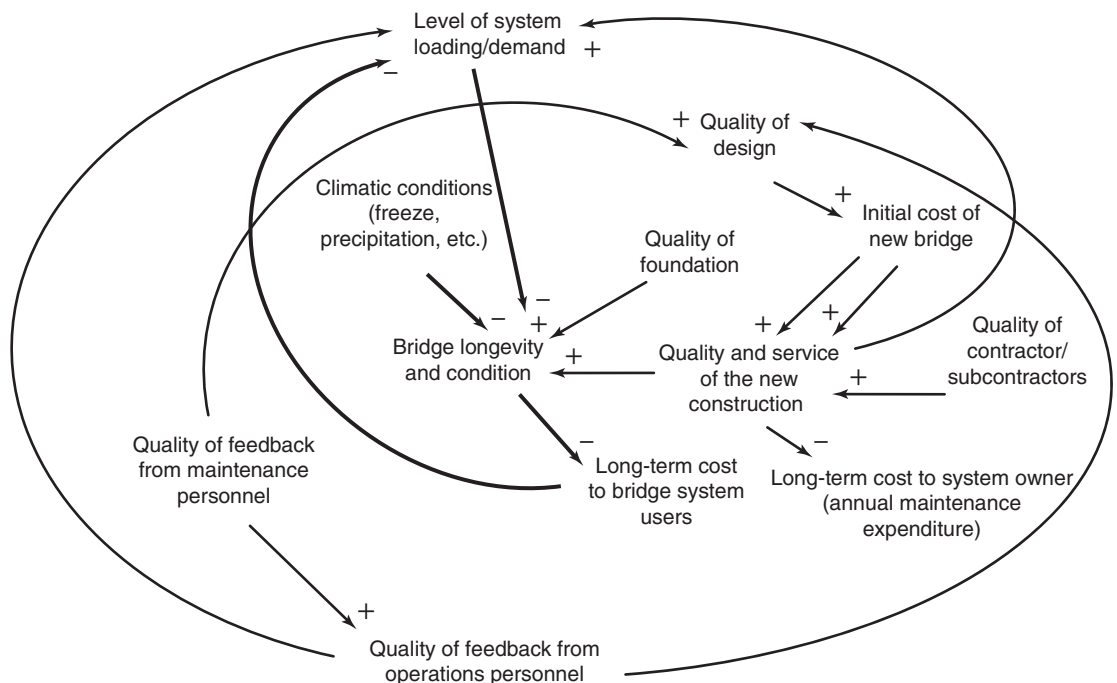
Figure 14.5 Causal loop diagram of a systems dynamics model predicting the longevity of a highway bridge deck.
