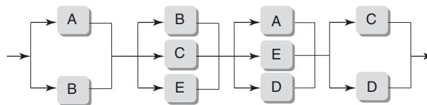
Figure 13.21 RBD for Example 13.8.
