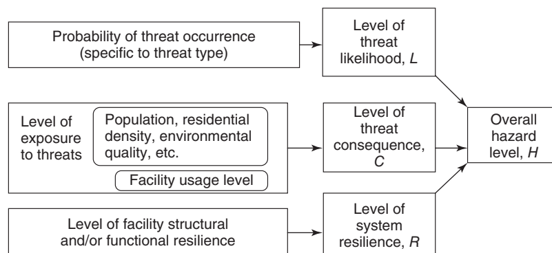
Figure 27.13 Procedure for rating the hazard associated with a civil engineering system.
