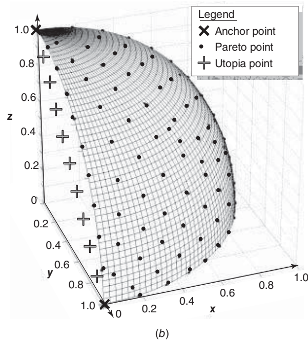
Figure 12.2 Illustration of Pareto solutions and the Pareto frontier (adapted from Bai, 2012; adapted from Utyuzhnikov et al., 2009): (a) Convex frontier shown with two decision criteria and (b) concave frontier shown with three decision criteria.
