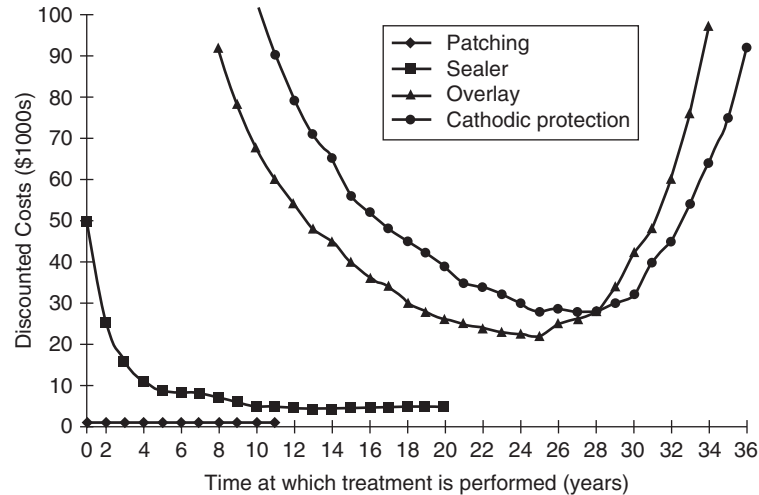
Figure 25.12 Plot of the discounted costs versus the treatment times.
