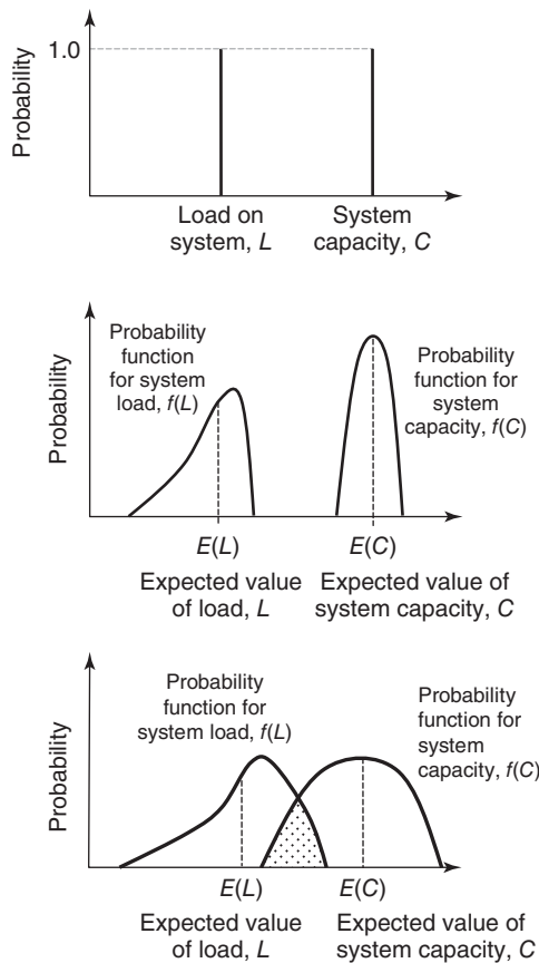
Figure 13.13 Loading and capacity functions.
