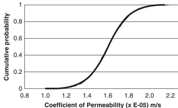
Figure 21.11 Probability distribution for permeability coefficient.
