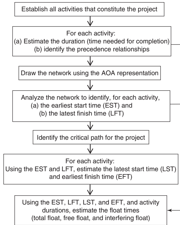
Figure 17.28 Steps for critical path method.
