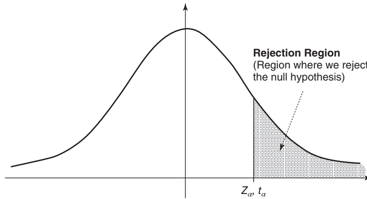
Figure 6.15 Figure for upper-tailed test.
