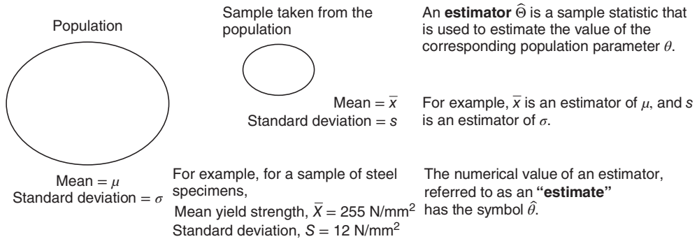
Figure 6.8 What is an estimator?
