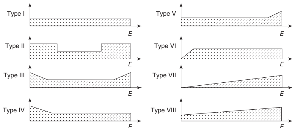
Figure 13.9 A few failure rate plots.
