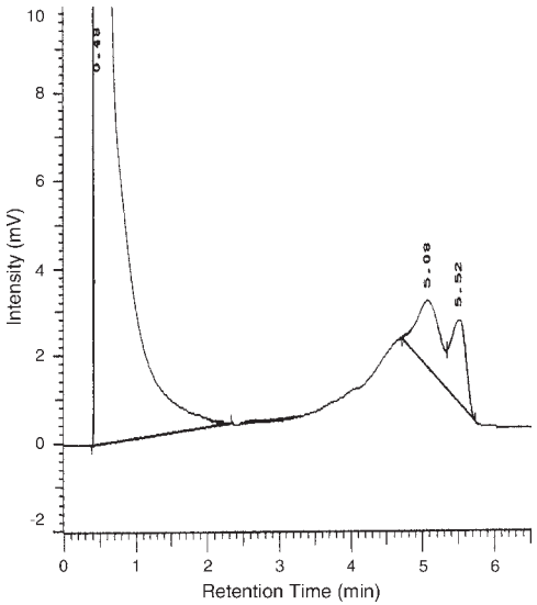
Fig. 5. Chromatogram of a mixture of polymerase chain reaction products amplified from the fetal DNA and the wild-type DNA. (Reproduced from ref. 2 , with the permission of John Wiley and Sons Ltd.)
