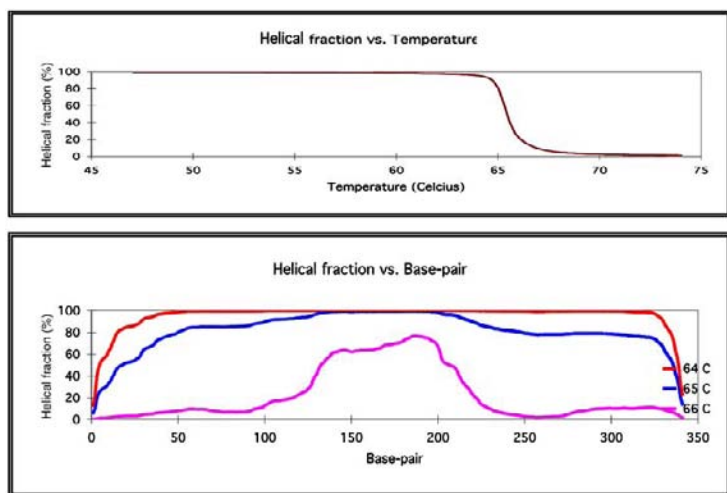
Fig. 2. The melting profile of exon 3 of the G6PT1 gene. The DNA sequence of the amplicon is: CTGCCCCATCTGACCCCACCCTCAacatgggcagtaggctggacacctacgtgtcgccctctgcccacagtggtttgagccatctcagtttggcacttgggtgggccatctgtcaaccagcatgaacctggctggagggctgggccctatcctggcaaccatcctgcccagagctacagctggcgcgagcacgctggccctatctgggcaactgtggtgtggtgtgtctctcctctgtctcctgctcatccacaatgaacctgctgatgttggaactccgcaacctggaccccatgcctctgagggaagaaggtGAGCCCCCACCAGACCGACCACT. The uppercase letters are primer sequences. The letter in bold type is the nucleotide position of the mutation in the wild-type sequence, i.e., 1563G>A. The mutation is located at nucleotide position 136 of the amplicon. The sequence is shown in the sense of direction.
