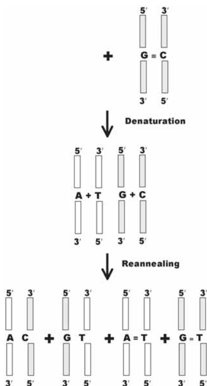
Fig. 1. Schematic presentation of heteroduplex formation through hybridization.
