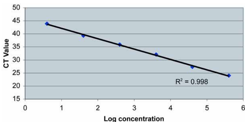
Fig. 2. An example of a standard curve for the real-time polymerase chain reaction assay of the small sub-unit rRNA ( ssrRNA ) gene of Plasmodium falciparum . Standard curves constructed by plotting the threshold cycle value (y-axis) against the input concentration of each dilution (x-axis) from 400,000 to 4 genome equivalents in logarithmic scale.
