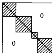
Figure 20.12 Structure of a block-diagonal matrix.
