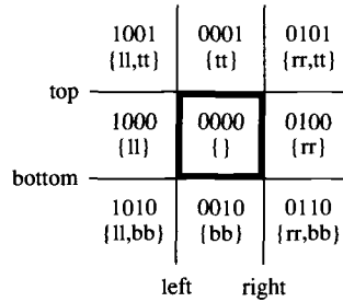
Figure 14.4 The clipping window partitions the plane into nine regions.
