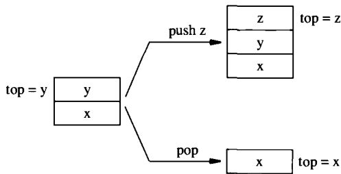
Figure 19.1 Elements are inserted at and removed from the top of the stack.
