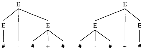
Figure 6.5 Two incompatible structures for the expression # · # + #.
