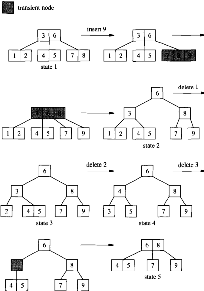
Figure 21.32 Tracing insertions and deletions in a (2,3)-tree.
