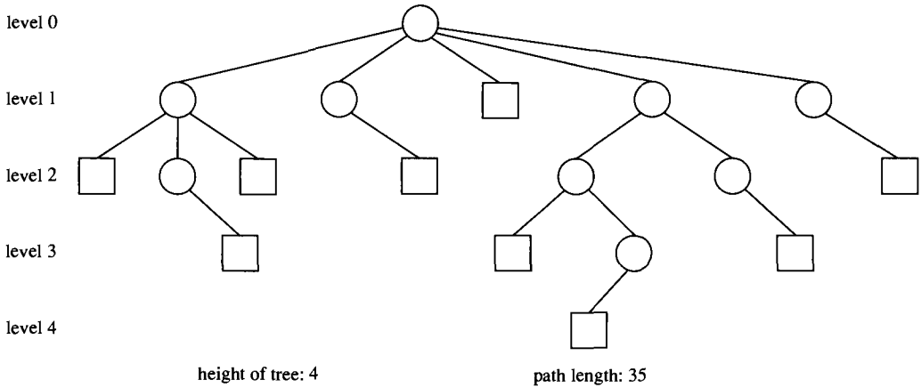
Figure 16.3 A tree of height = 4 and path length = 35.
