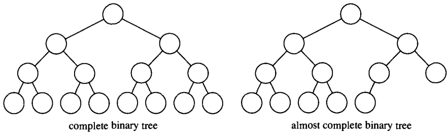
Figure 16.4 Examples of well-balanced binary trees.
