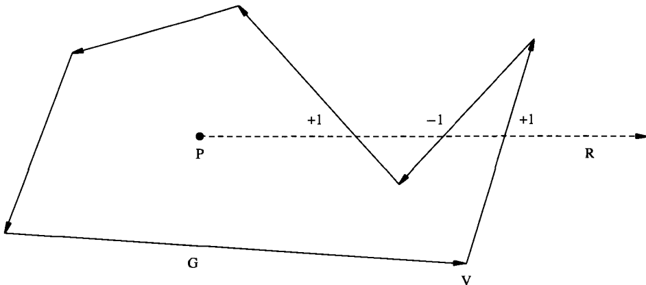
Figure 24.8 Point-in polygon test by adding up crossing numbers.
