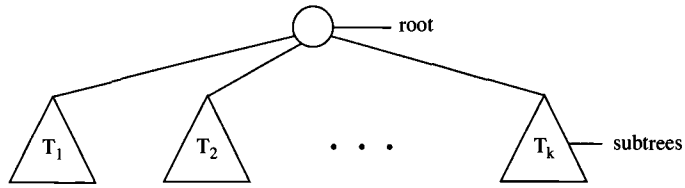
Figure 16.2 Recursive definition of a rooted, ordered tree.
