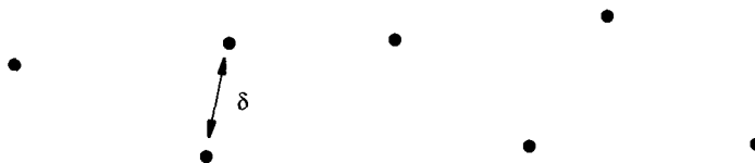
Figure 26.1 Identify a closest pair among n points in the plane.
