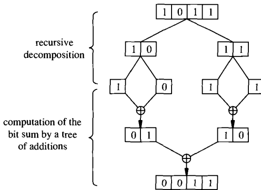
Figure 8.3 Logarithmic bit sum algorithm as a result of divide-and-conquer.
