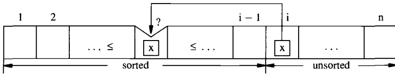
Figure 17.1 Insertion sorts move an easily accessed element to its correct place.
