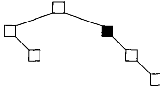
Figure 21.22 Example of a tree not height-balanced; the marked node violates the balance condition.
