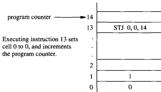
Figure 15.2 Stored program computer: Data and instructions share the memory.
