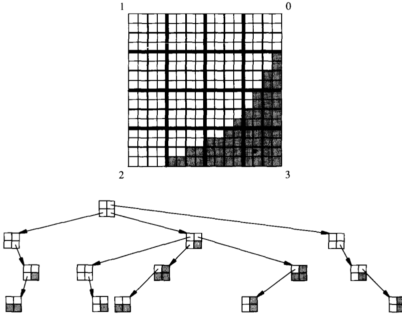
Figure 23.2 A quarter circle digitized on a 16 \cdot 16 grid, and its representation as a 4-level quadtree.
