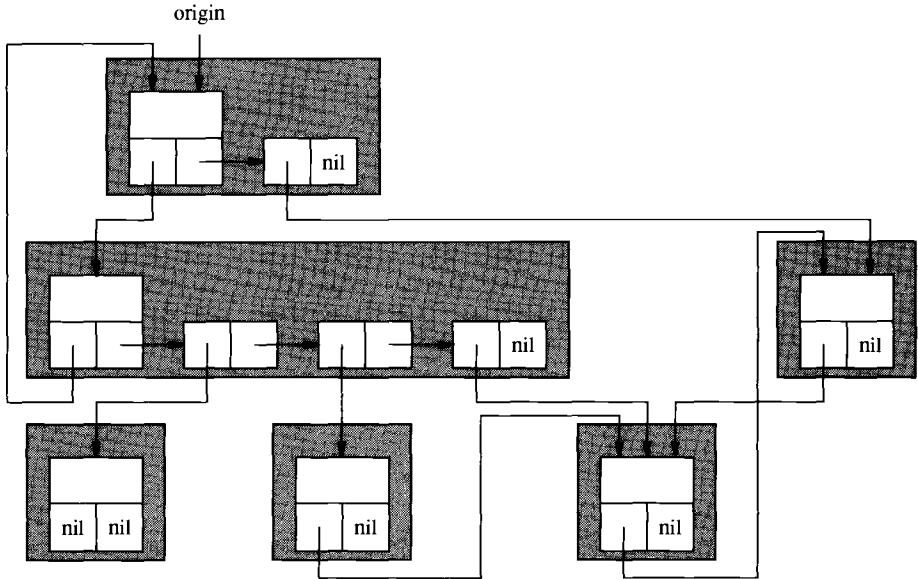
Figure 21.16 A possible implementation as a list structure.
