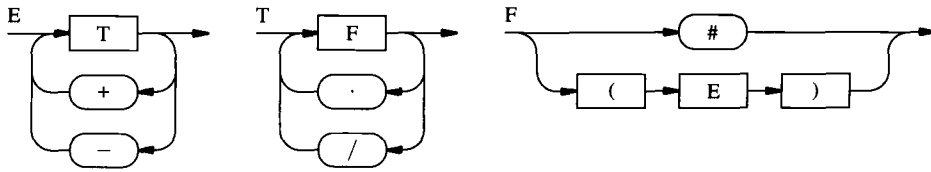
Figure 6.1 Syntax diagrams for simple arithmetic expressions.
