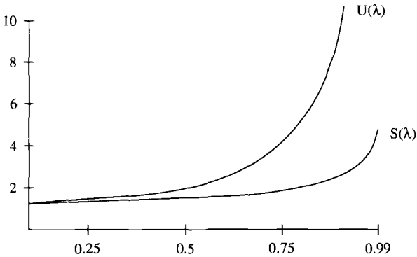
Figure 22.5 The average number of probes per search grows rapidly as the load factor approaches 1.
