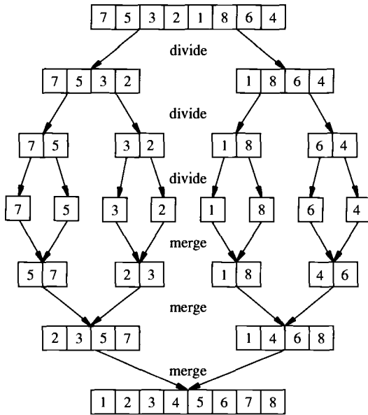
Figure 17.12 Sorting an array by using a divide-and-conquer scheme.
