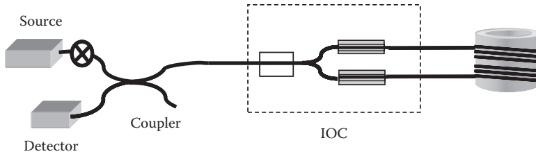
FIGURE 8.12 Schematic of integrated optics gyroscope configuration.
