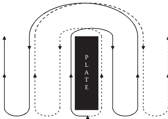
FIGURE 8.22 Thermally symmetric, crossover-free winding pattern for 10 spiral layers.
