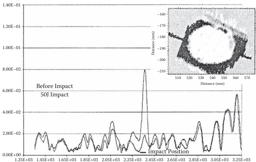
FIGURE 3.13 Impact detection using bow-tie fiber.
