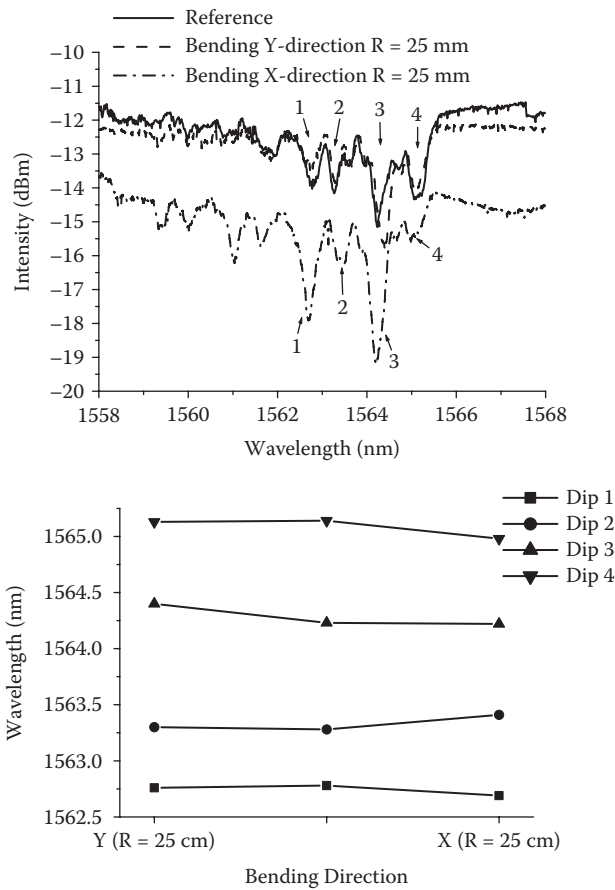
FIGURE 5.10 (a) Measured spectra of FBG in multimode fiber inscribed by IR femtosecond laser at different bending conditions: (i) without bending; (ii) bending in x-direction; and (iii) bending in y-direction; (b) the MM FBG spectra of dip locations as a function of bending direction for different dips.
