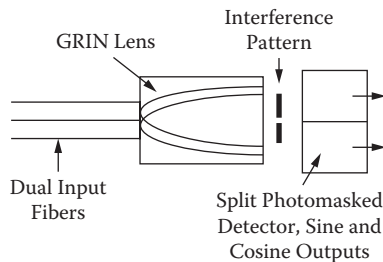
FIGURE 1.34 Quadrature demodulation avoids signal fading problems. The method shown here expands the two beams into an interference pattern that is imaged onto a split detector.
