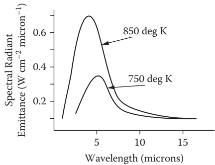
FIGURE 1.18 Blackbody radiation curves provide unique signatures for each temperature.
