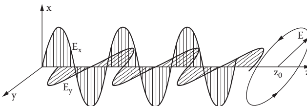
FIGURE 3.1 Polarization components of E wave.
