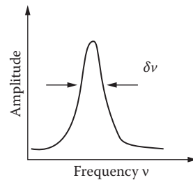
FIGURE 3.7 Spectral spread of laser emission.
