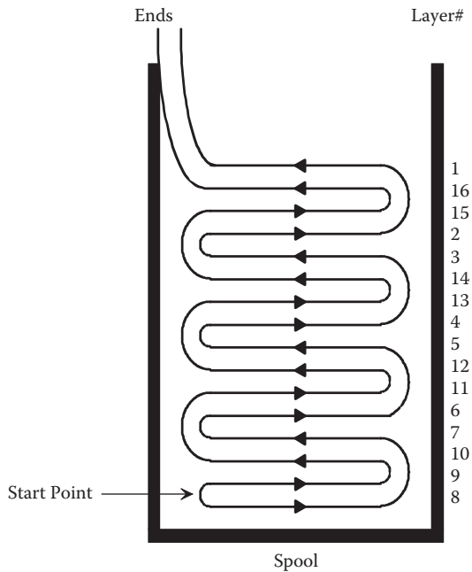
FIGURE 8.21 Quadrupolar-winding pattern for 16 fiber layers.
