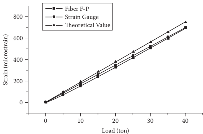
FIGURE 10.13 Comparison of theoretical values and experimental results obtained with the strain gauge and the fiber F-P strain sensor.
