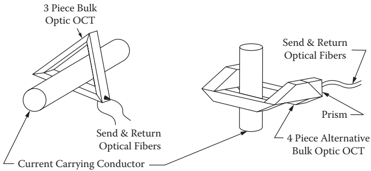
FIGURE 3.19 Revised bulk-optic structures.
