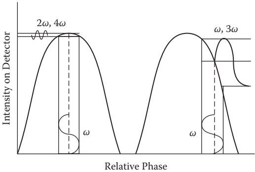
FIGURE 1.27 An open-loop fiber optic gyro has predominantly even-order harmonics in the absence of rotation. Upon rotation, the open-loop fiber optic gyro has an odd harmonic output whose amplitude indicates the magnitude of the rotation rate and whose phase indicates direction.
