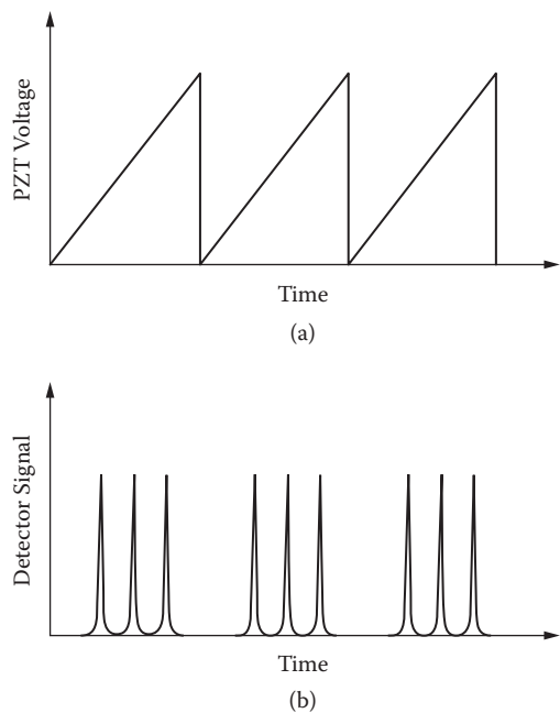
FIGURE 7.13 Typical scanning of the Fabry-Perot filter for wavelength-multiplexed sensors: (a) PZT driving signal; (b) detector signal for three wavelength-multiplexed sensors.
