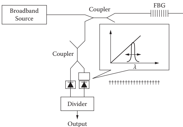
FIGURE 4.5 Schematic of edge filter-based FBG sensor interrogation.
