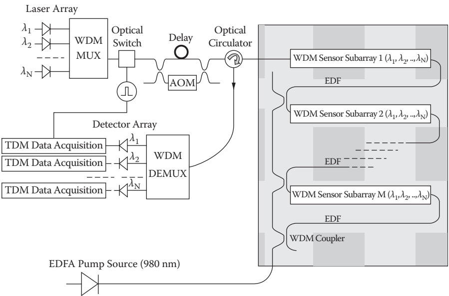
FIGURE 9.14 Schematic arrangement using EDFA in a sensor array.
