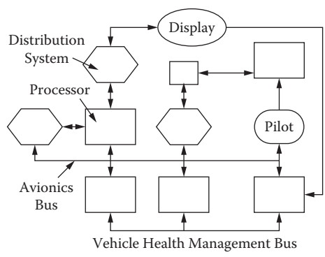
FIGURE 1.51 A typical vehicle health management bus for an avionics system would be the interface point for the fiber optic smart structure modules of Figure 1.50.
