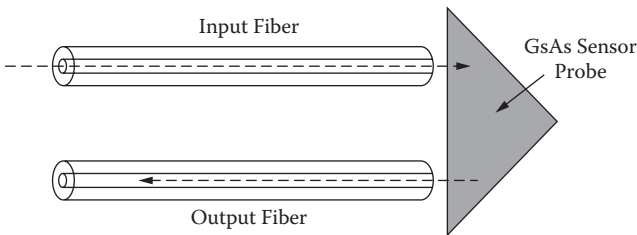
FIGURE 1.19 Fiber optic sensor based on variable absorption of materials such as GaAs allows the measurement of temperature and pressure.
