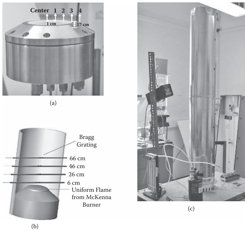
FIGURE 5.18 (a) Horizontal direction along burner; (b) vertical direction along burner; (c) hole distributions in the chimney along vertical direction.
