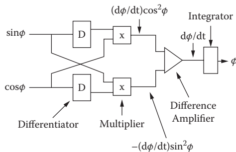
FIGURE 1.35 Quadrature demodulation electronics take the sinusoidal outputs from the split detector and convert them via cross-multiplication and differentiation into an output that can be integrated to form the direct phase difference.
