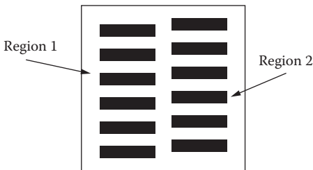
FIGURE 1.15 Dual grating mask with regions 90° out of phase to support quadrature detection, which allows grating-based sensors to track through multiple lines.
