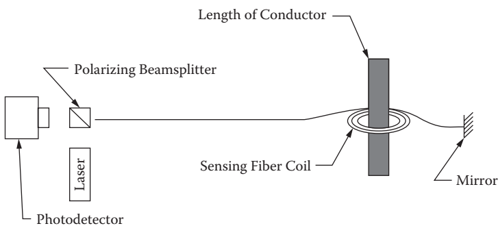
FIGURE 3.16 Reflective-type wound-fiber OCT.
