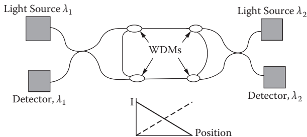
FIGURE 1.30 A distributed fiber optic acoustic sensor based on interlaced Sagnac loops allows the detection of the location and the measurement of the amplitude along a length of optical fiber that may be many kilometers long.
