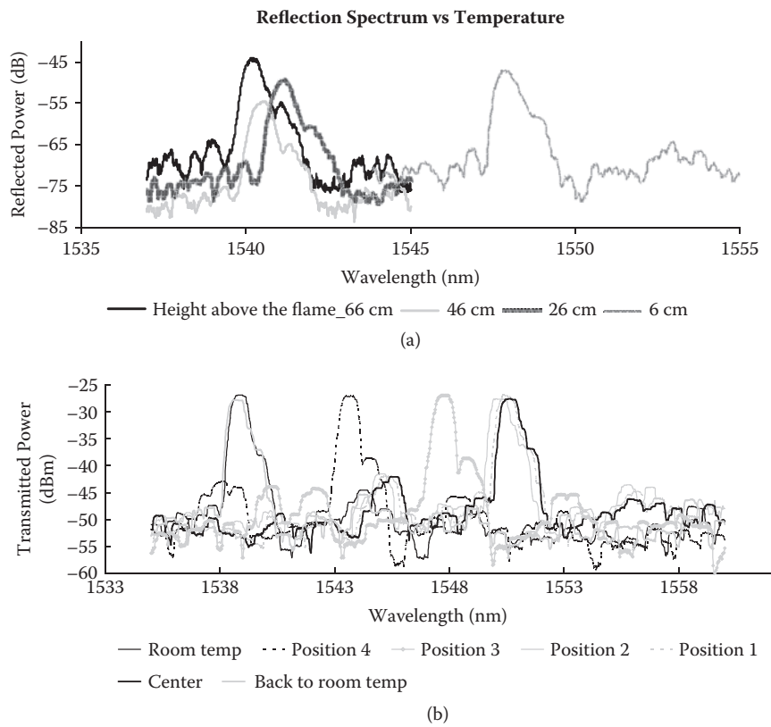
FIGURE 5.19 (a) Grating spectrum measured with different locations along the vertical direction; (b) grating spectrum measured with different locations along the horizontal direction.
