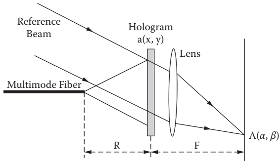
FIGURE 6.1 Fiber specklegram formation.
