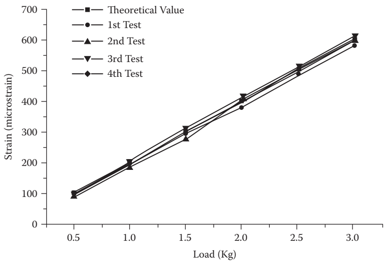
FIGURE 10.14 Repeatability test results for the fiber F-P strain sensor based on a standard cantilever setup.
