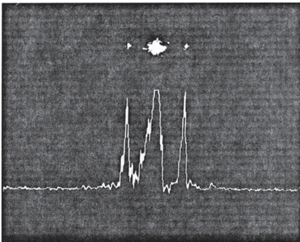
FIGURE 6.32 Output correlation distribution.
