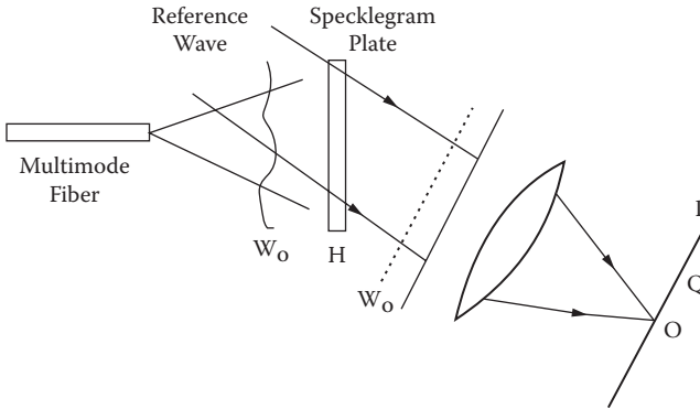
FIGURE 6.21 Specklegram reconstruction process.
