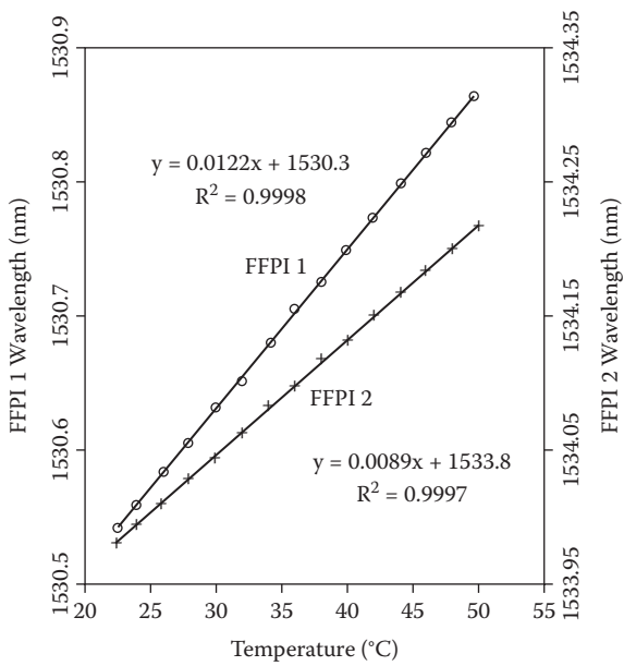
FIGURE 10.5 Variation of FFPI wavelength with temperature.
