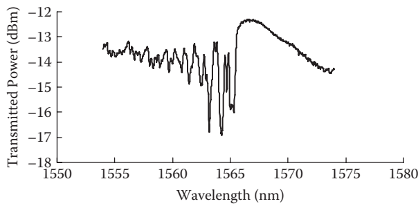
FIGURE 5.3 The measured transmission spectrum of MM FBG obtained by the single mode excitation condition: tunable laser with an SMF pigtail.
