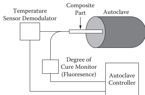
FIGURE 1.49 Smart manufacturing systems offer the prospect of monitoring key parameters of parts as they are being made, which increases yield and lowers overall costs.
