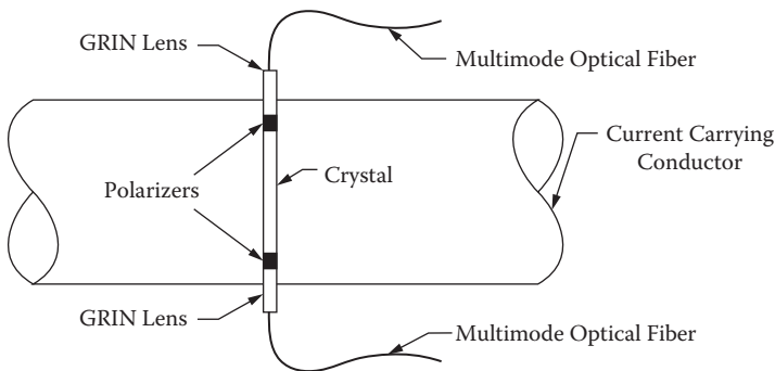
FIGURE 3.21 Single-pass, crystal-based OCT.
