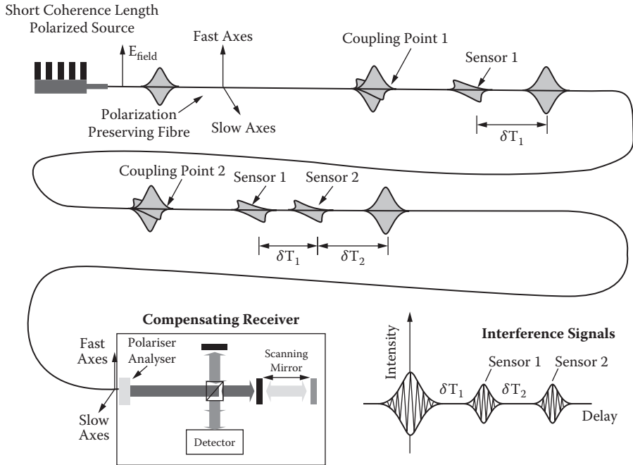
FIGURE 3.9 Quasi-distributed polarimetric sensor.
