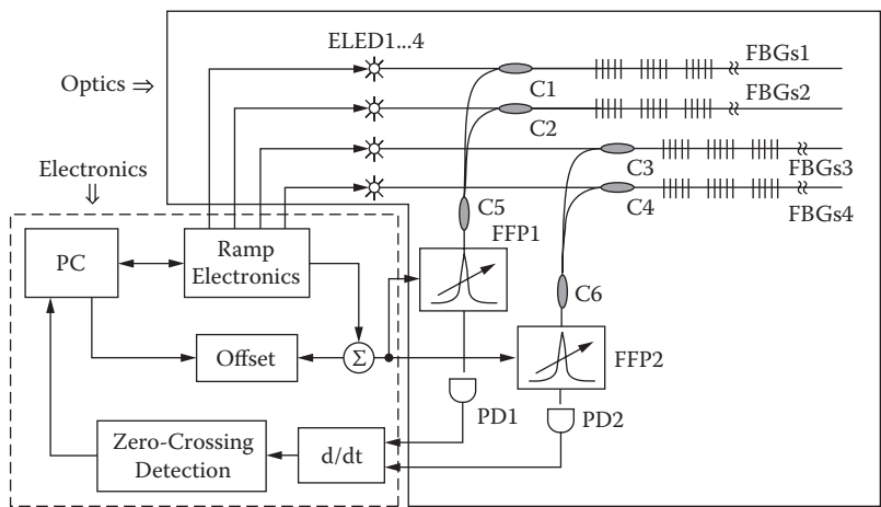
FIGURE 7.14 Schematic diagram of a 64-channel sensor fiber Bragg grating sensor system adopting Fabry-Perot filters. (From S. T. Vohra et al., Proc. 13th Int. Conf. Optical Fiber Sensors (OFS-13) , Kyongju, Korea, SPIE, 3746, pp. 32–37, 1999.)
