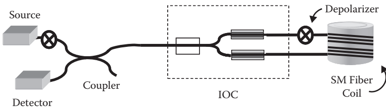
FIGURE 8.13 Schematic of depolarized/single mode fiber optic gyroscope configuration.
