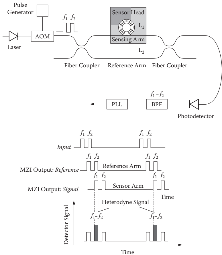
FIGURE 9.8 An MZI-based fiber hydrophone using the differential delayed heterodyne technique.
