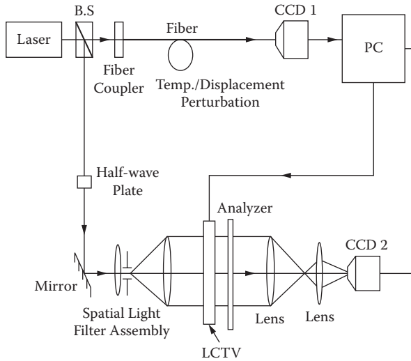
FIGURE 6.31 JTC-FSS sensing system.
