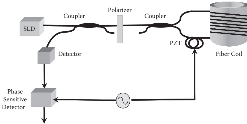
FIGURE 8.5 Schematic of IFOG with biasing phase modulator.
