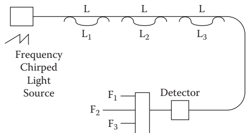
FIGURE 1.42 Frequency division multiplexing can be used to tag a series of fiber sensors. In this case the Mach-Zehnder interferometers are shown with a carrier frequency on which the output signal rides.
