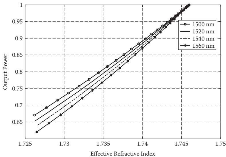
FIGURE 5.29 Calculated bend loss curves of the sapphire fiber as a function of effective refractive index for different wavelengths.
