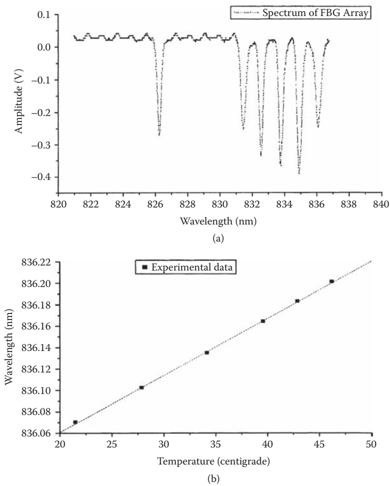
FIGURE 10.31 Results of the FBG temperature sensor system based on a CCD spectrometer. (a) Spectrum of sensing and reference FBGs; (b) experimental results.
