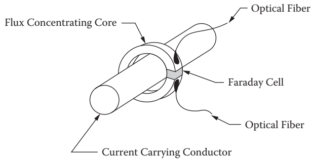
FIGURE 3.20 Hybrid or flux concentrator OCT.
