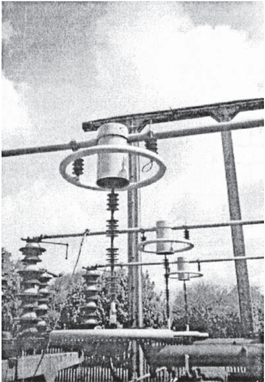
FIGURE 3.33 Field installation of three-phase optical voltage and current sensors showing the capacitive divider implementation.
