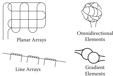
FIGURE 1.31 Flexible geometries of interferometric fiber optic sensors' transducers are one of the features of fiber sensors attractive to designers configuring special-purpose sensors.
