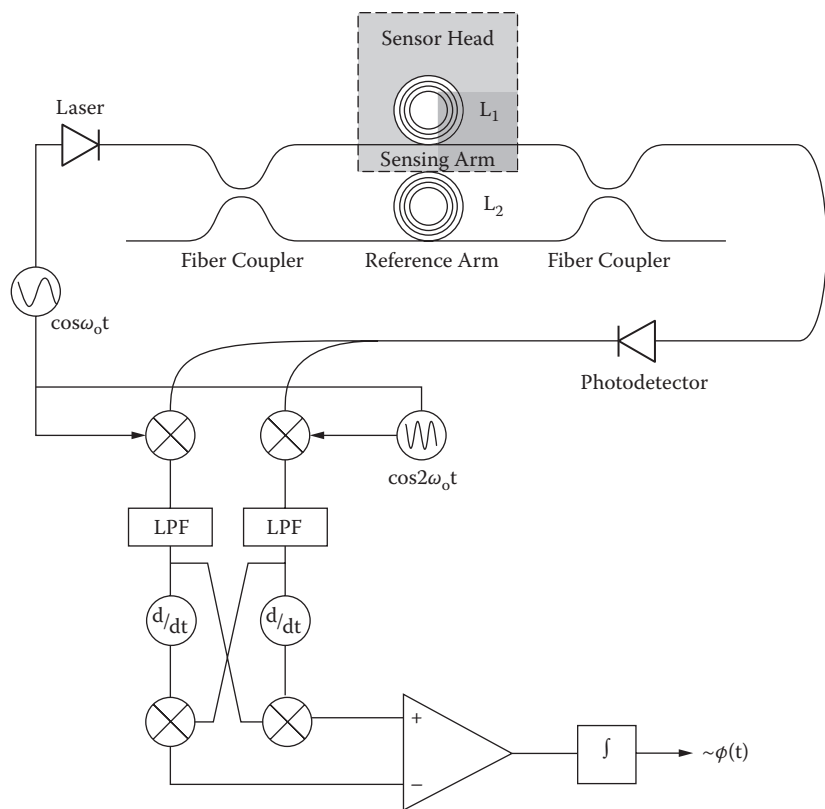
FIGURE 9.5 A fiber hydrophone using the phase-generated carrier homodyne technique.
