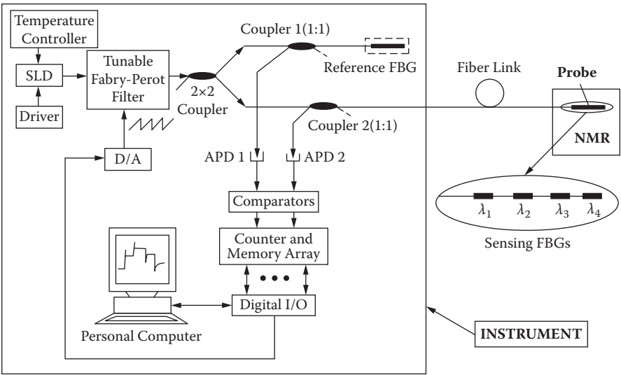
FIGURE 10.27 Schematic diagram of FBG temperature sensor system with a tunable FP filter.
