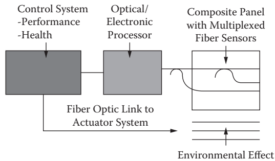
FIGURE 1.48 Fiber optic smart structure systems consist of optical fiber sensors embedded or attached to parts sensing environmental effects that are multiplexed and directed down. The effects are then sent through an optical/electronic signal processor that in turn feeds the information to a control system that may or may not act on the information via a fiber link to an actuator.
