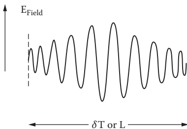
FIGURE 3.6 Wave train representation of a photon.
