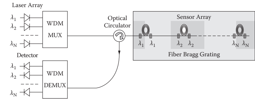
FIGURE 9.12 A schematic diagram of an N -channel WDM hydrophone array.
