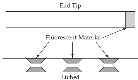
FIGURE 1.20 Fluorescent fiber optic sensor probe configurations can be used to support the measurement of physical parameters as well as the presence or absence of chemical species. These probes may be configured to be single ended or multipoint by using side etch techniques and attaching the fluorescent material to the fiber.
