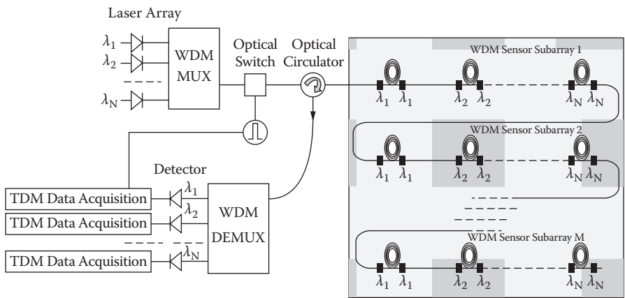
FIGURE 9.13 A schematic diagram of an N \times M channel TDM-WDM hydrophone array.
