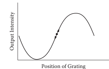
FIGURE 1.14 Dynamic range limitations of the grating-based sensor of Figure 1.13 are due to smaller grating spacing increasing sensitivity at the expense of range.
