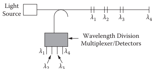
FIGURE 1.43 Wavelength division multiplexing is often very energy efficient. A series of fiber sensors is multiplexed by being arranged to reflect in a particular spectral band that is split via a dispersive element onto separate detectors.
