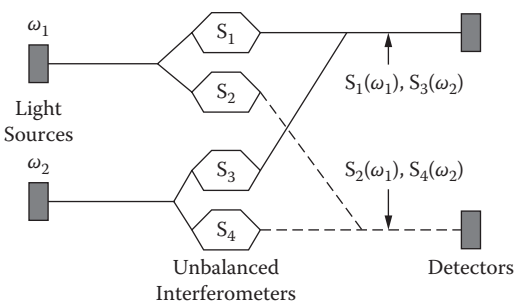
FIGURE 1.46 Spatial multiplexing of four fiber optic sensors may be accomplished by operating two light sources with different carrier frequencies and cross-coupling the sensor outputs onto two output fibers.
