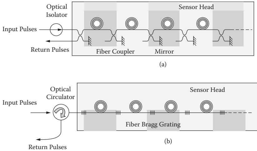
FIGURE 9.10 Schemes of reflective TDM hydrophone arrays.
