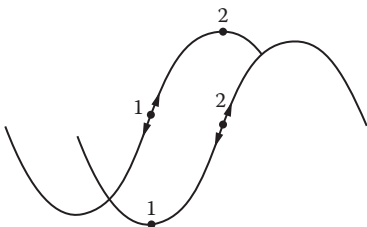
FIGURE 1.16 Diagram of a quadrature detection method that allows one area of maximum sensitivity while the other reaches a minimum, and vice versa, allowing uniform sensitivity over a wide dynamic range.
