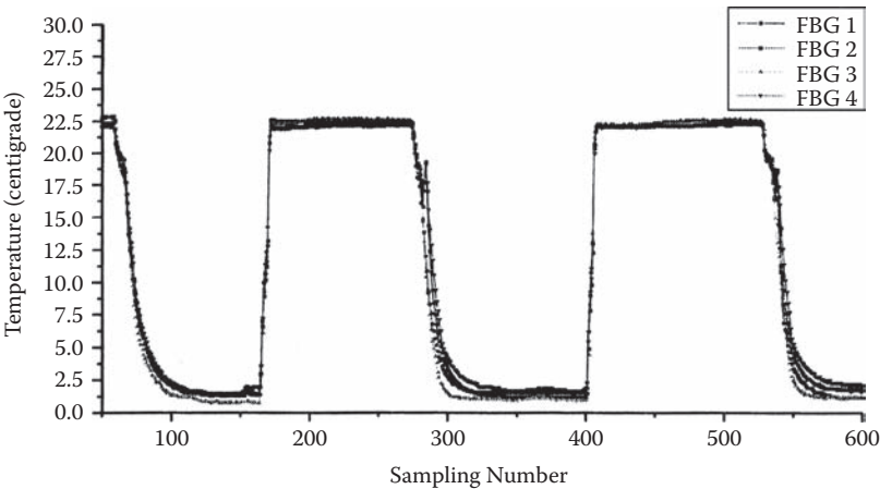
FIGURE 10.28 Results of temperature measurement with FBGs operated in a nuclear magnetic resonance (NMR) machine.
