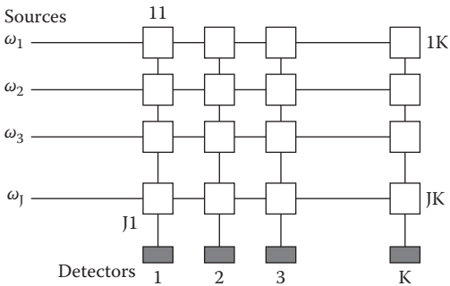
FIGURE 1.47 Extensions of spatial multiplexing the JK sensors can be accomplished by operating J light sources at J different frequencies and cross-coupling to K output fibers.
