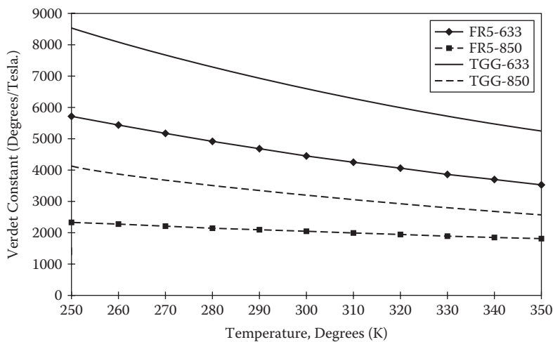
FIGURE 3.26 Variation of Verdet constant with temperature and wavelength.
