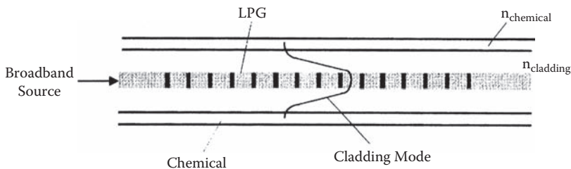
FIGURE 10.34 Schematic diagram of the long-period grating chemical sensor.
