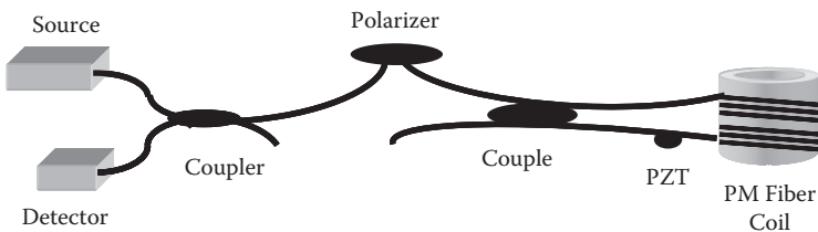
FIGURE 8.11 Schematic of all-fiber IFOG configuration.
