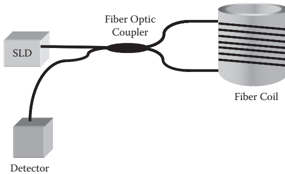
FIGURE 8.2 Schematic of basic IFOG configuration.
