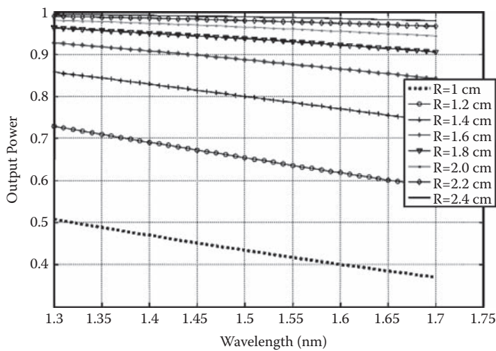
FIGURE 5.30 Calculated bend loss curve as a function of bend radius for different wavelengths.
