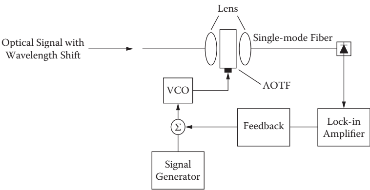
FIGURE 4.8 Interrogation scheme using an acoustic-optic tunable filter.
