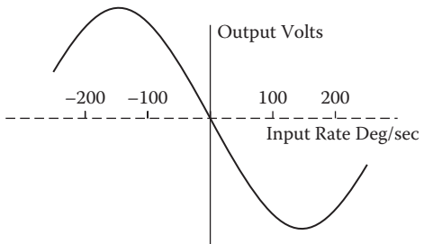
FIGURE 1.28 A typical open-loop fiber optic gyro output, obtained by measuring one of the odd harmonic output components’ amplitude and phase, results in a sinusoidal output that has a region of good linearity centered about the zero rotation point.
