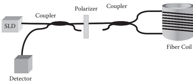
FIGURE 8.3 Schematic of minimum configuration IFOG.
