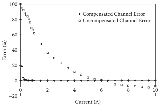
FIGURE 3.25 OCT output errors (vibration: 180 Hz, 8 g, connectors vibrated).
