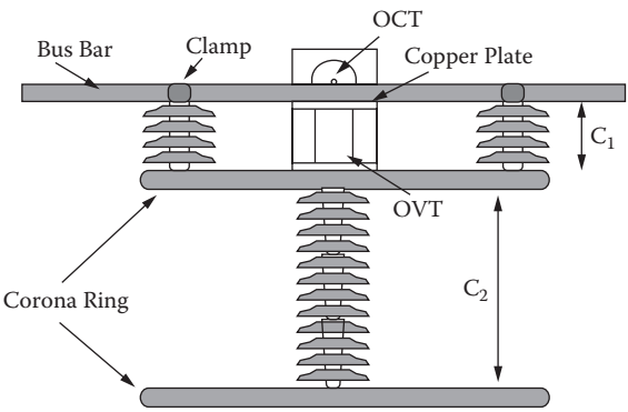
FIGURE 3.32 Implementation of the capacitive voltage divider.
