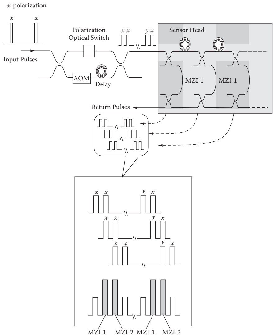
FIGURE 9.16 Mitigation of polarization-induced signal fading in a hydrophone array by polarization-switching approach.
