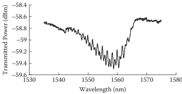
FIGURE 5.4 The measured transmission spectrum of MM FBG obtained by the multimode excitation condition: broadband light source from an optical spectra analyzer.
