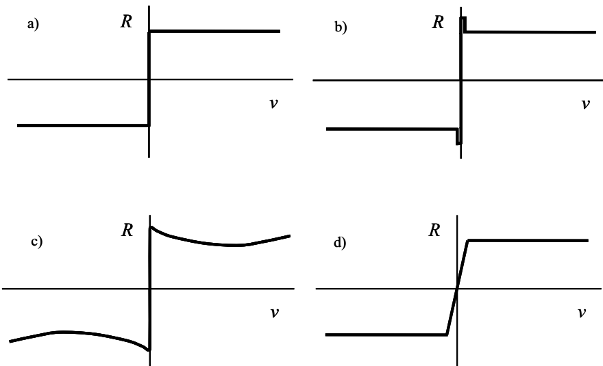
Fig. 1.9. Different idealization for dry friction
