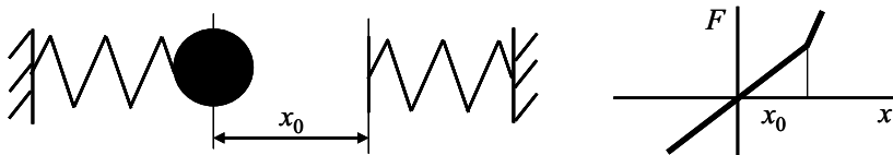
Fig. 1.5. Designed hard nonlinearity
