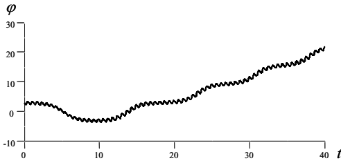
Fig. 7.13. Slow rotation of the pendulum
