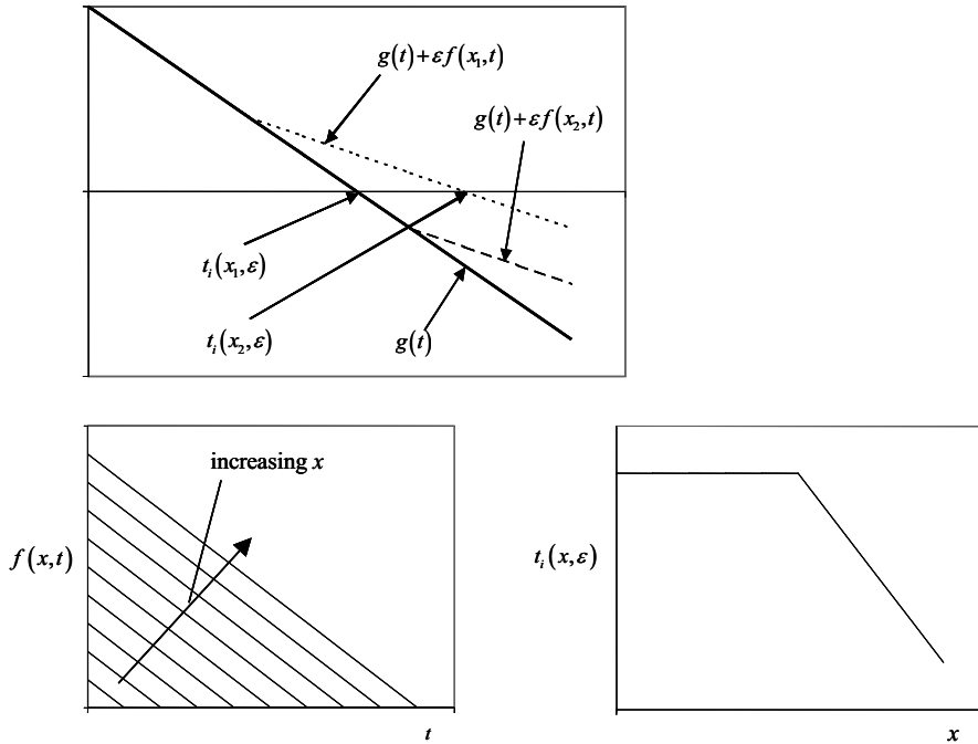
Fig. AIII.2. On the definition and Lipschitz-continuity of the implicit function t_i(x, \varepsilon)
