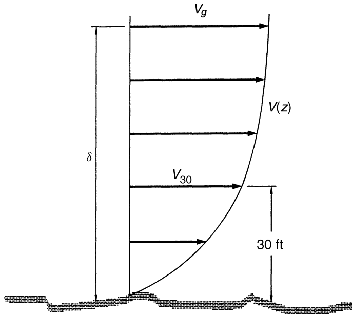
Fig. 4.21 Velocity profile.
