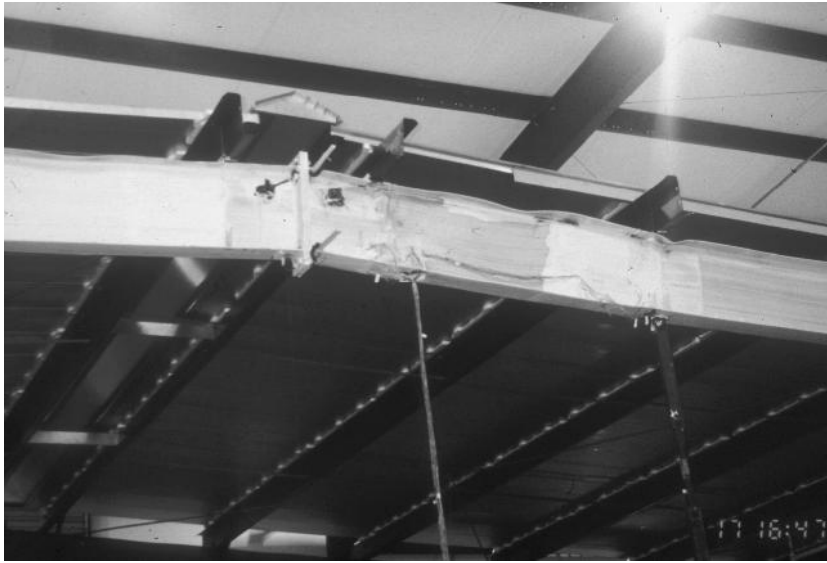
Fig. 8.41 Local buckling of flange. (Courtesy of Structures/Materials Laboratory, Virginia Tech.)
