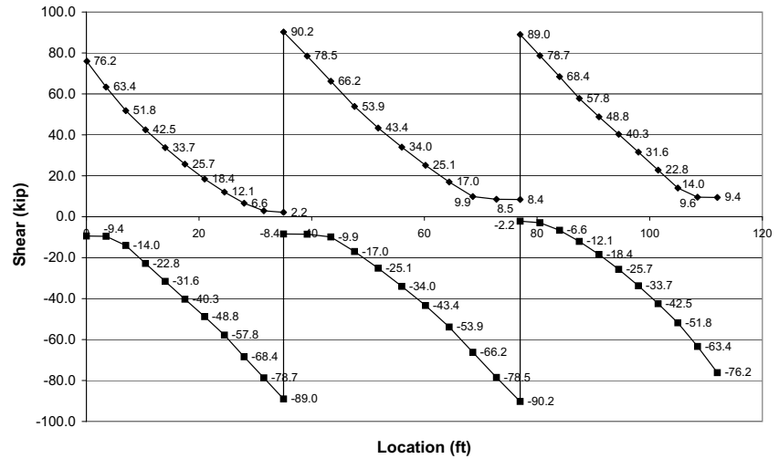
Fig. 5.20 Live-load shear envelope for HL-93 on 35-42-35 ft beam.
