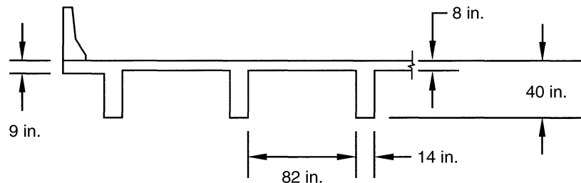
Fig. E7.3-2 Trial section for T-beam bridge.
