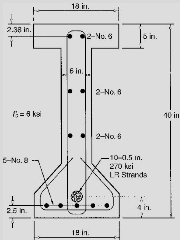
Fig. 7.27 Beam cross section used in Example 7.7.
