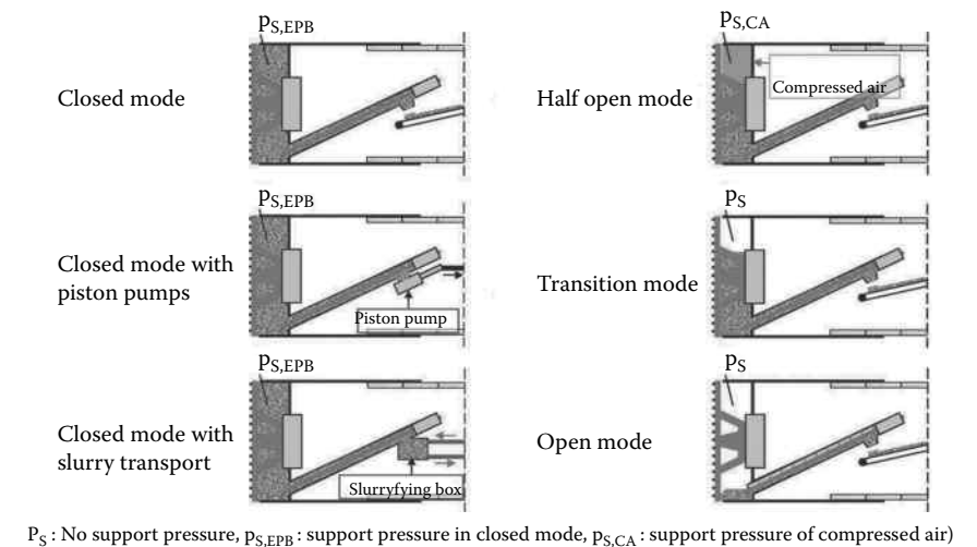
FIGURE 10.5 Working modes of EPB TBMs. (Adapted from Herrenknecht, M., Thewes, M., Budach, C., 2011. Geomechanics and Tunnelling , 4:1:11–35. With permission.)
