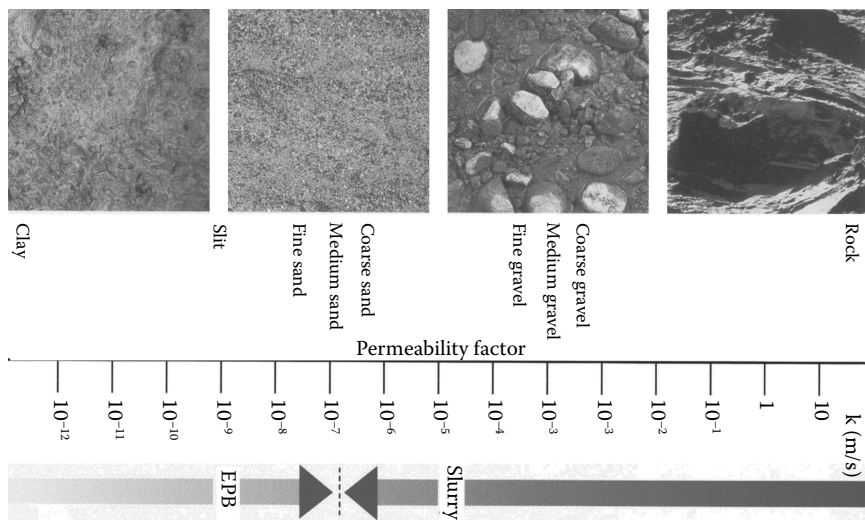
FIGURE 3.17 Selection criteria of permeability factor for earth pressure balance and slurry tunnel boring machines. (Adapted from B  ppler, K., 2007. Tunnelling with Slurry TBMs (Mixshields) , Tunneling Seminar, Herrenknecht AG, Germany, University of Texas at Austin. With permission.)
