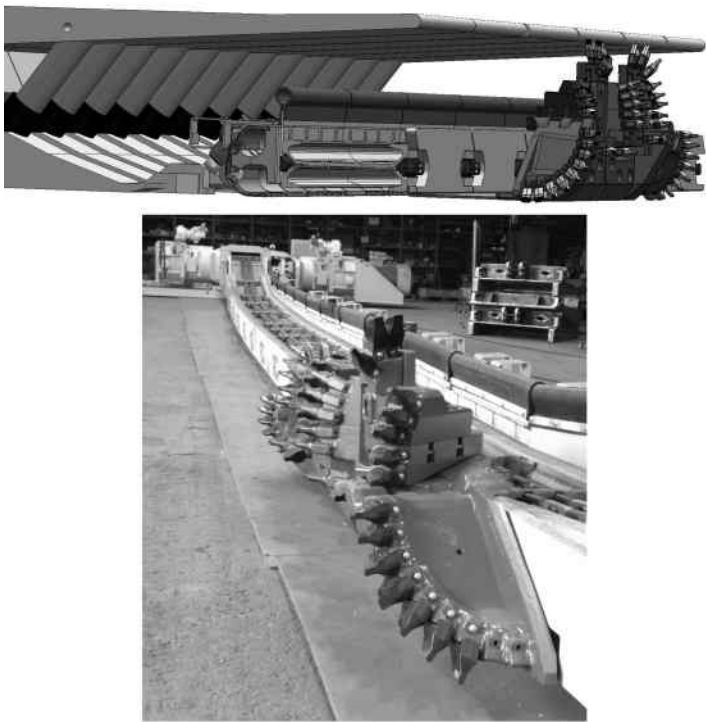
FIGURE 14.4 A drawing (upper) and view (lower) of a plough. (Courtesy of Halbach and Braun.)
