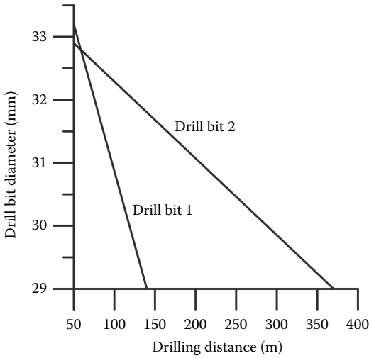
FIGURE 6.10 The variation of decrease in drill bit diameter with drilling distance due to wear characteristics of the drilled rock formations.
