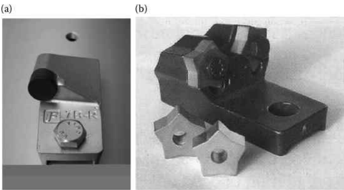
FIGURE 15.3 Circular (a) and star-shaped (b) tool geometries. (Courtesy of Fantini.)
