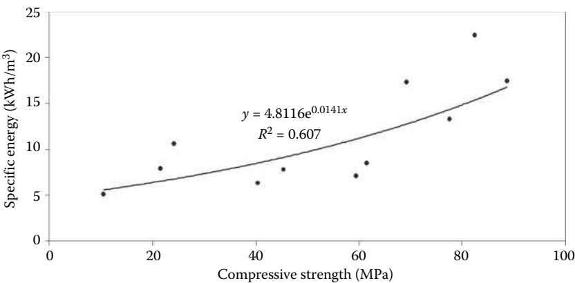
FIGURE 13.8 The relationship between drilling specific energy and rock compressive strength.
