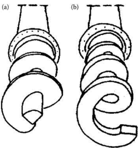
FIGURE 10.6 Shaft-type (a) and ribbon-type (b) screws. (Adapted from Maidl, B., Herrenknecht, M., Anheuser, L., 1996. Mechanized Shield Tunnelling . Ernst and Sohn, ISBN: 3-433-01292-X, 427 p. With permission.)
