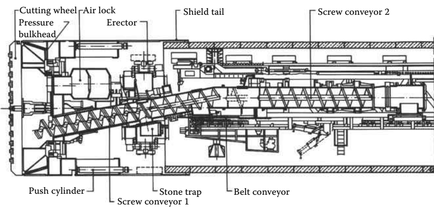
FIGURE 10.7 Extended screw conveyor of EPB TBMs. (Adapted from Herrenknecht, M., Thewes, M., Budach, C., 2011. Geomechanics and Tunnelling , 4:1:11–35. With permission.)
