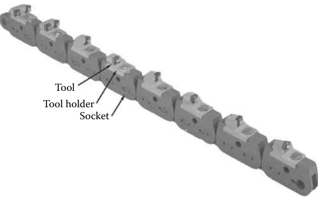
FIGURE 15.2 A picture of a sequence of cutting tools. (Courtesy of Garrone, Product Catalogues. With permission.)
