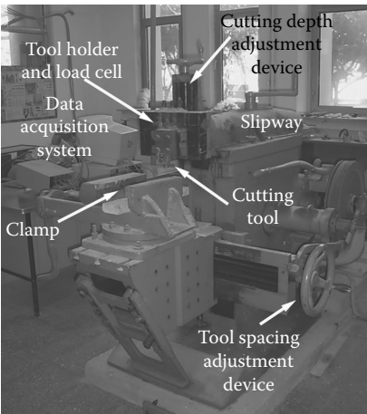
FIGURE 5.2 Small-scale linear cutting machine in ITU Laboratories.
