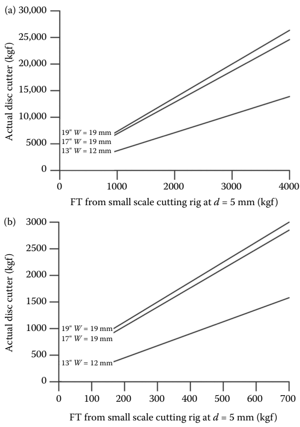
FIGURE 5.11 Relationships between the tool forces ((a) normal force and (b) rolling force) of the portable linear cutting tests and full-scale linear cutting tests for constant cross-section disk cutters with different tip width and diameters. (Adapted from Bilgin, N. et al. 2010a. Development of a portable rock cutting rig for rock cuttability determination. Proceedings of the European Rock Mechanics Symposium (EUROCK 2010) , eds. J. Zhao, V. Labiouse, J.P. Duth, J.F. Mathier, ISBN: 978-0-415-58654-2, June 15–18, Lausanne-Switzerland, CRC Press/Balkema, Taylor & Francis Group, pp. 405–408.)
