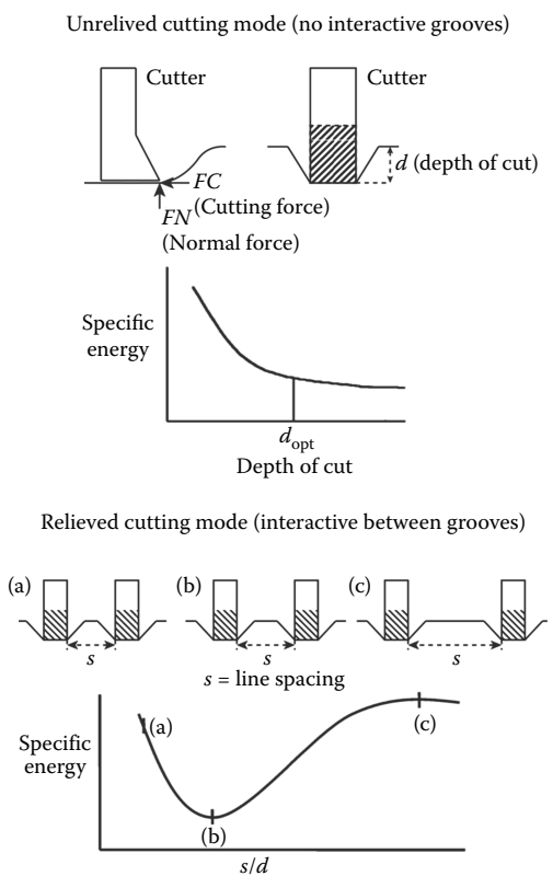
FIGURE 4.10 Relieved and unrelieved cutting mode with chisel cutters. (a) Too small spacing (overcrushing), (b) optimum spacing (chipping), and (c) too large spacing (ridge occurrence-coring).
