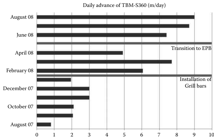
FIGURE 9.21 Daily advance rates of TBM S-360 in line 1. (From archive of N. Bilgin.)
