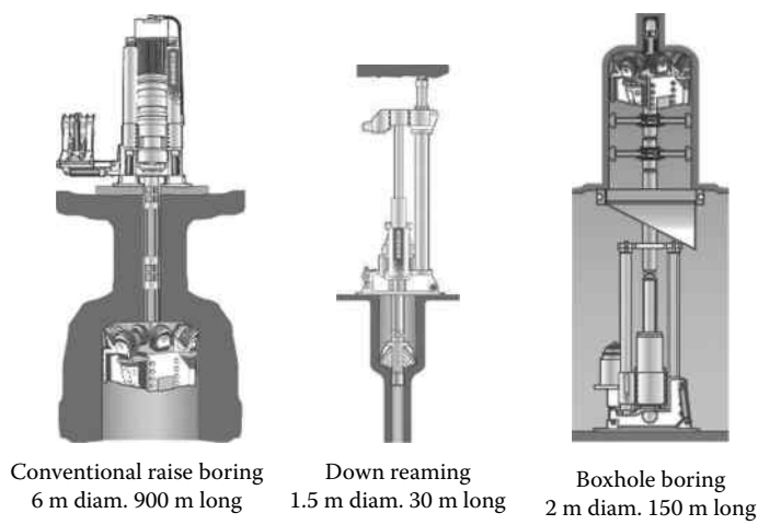
FIGURE 12.3 Conventional raise boring, down reaming, and boxhole boring. (Courtesy of Atlas Copco.)
