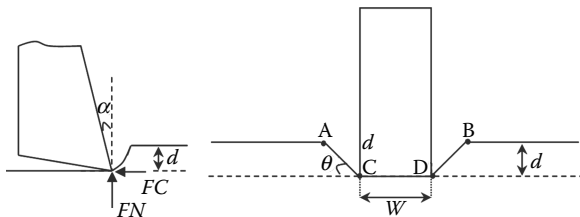
FIGURE 4.20 Basic tool parameters of calculation of specific energy.
