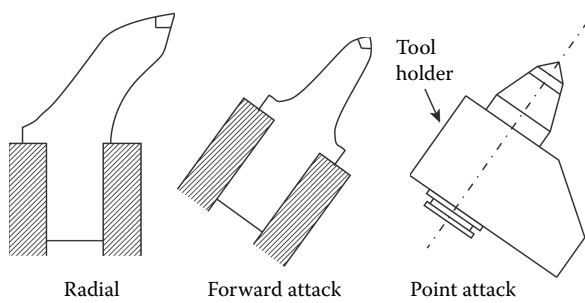
FIGURE 4.7 Radial, forward attack, and point attack tools.
