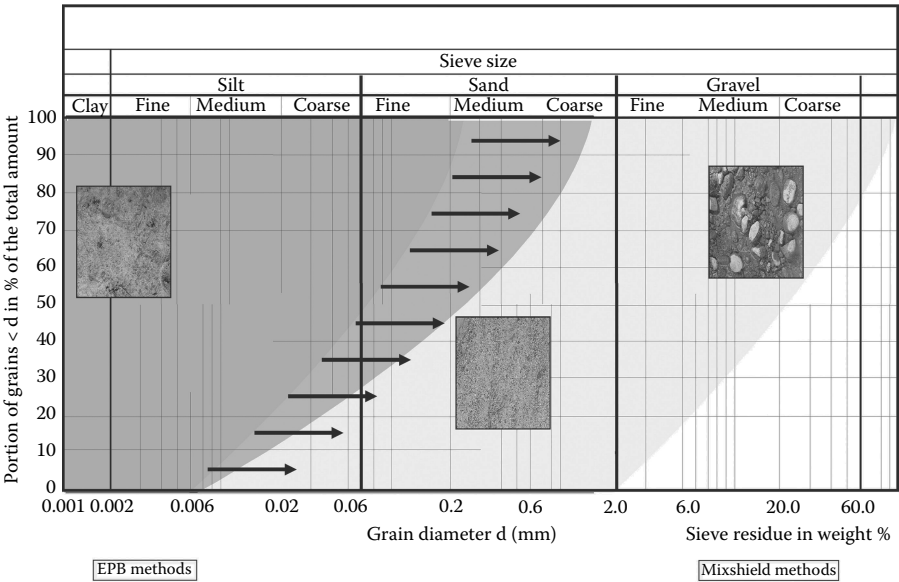
FIGURE 3.15 Selection criteria of grain size for earth pressure balance and slurry tunnel boring. (Adapted from B  ppler, K., 2007. Tunnelling with Slurry TBMs (Mixshields) , Tunneling Seminar, Herrenknecht AG, Germany, University of Texas at Austin. With permission.)
