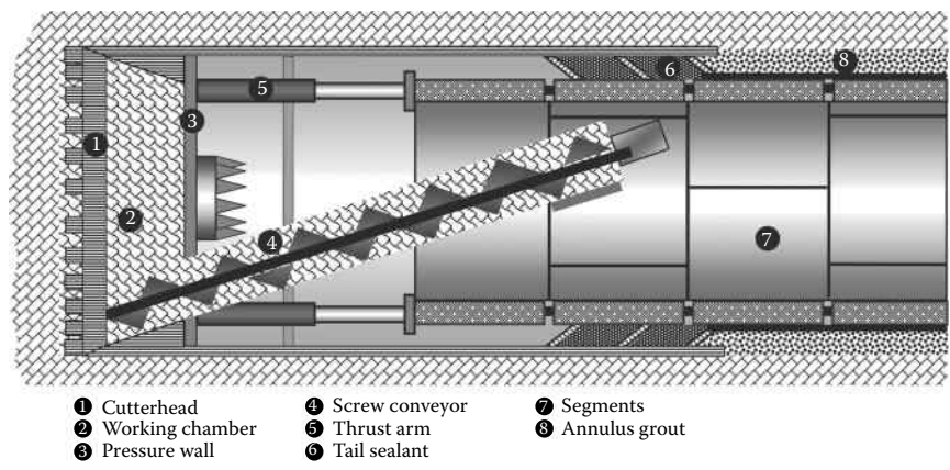
FIGURE 10.4 Schematic of an EPB TBM System. (Adapted from Efnarc, 2005. Specification and guidelines for the use of specialist products for mechanized tunnelling (TBM) in soft ground and hard rock. European Federation Dedicated to Specialist Construction Chemicals and Concrete Systems.)
