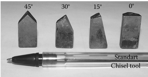
FIGURE 5.3 Cutting tools used with small-scale linear cutting machine.
