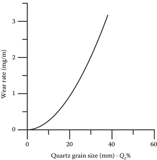
FIGURE 6.9 The variation of cutter wear rate with the product of quartz content and quartz grain size.
