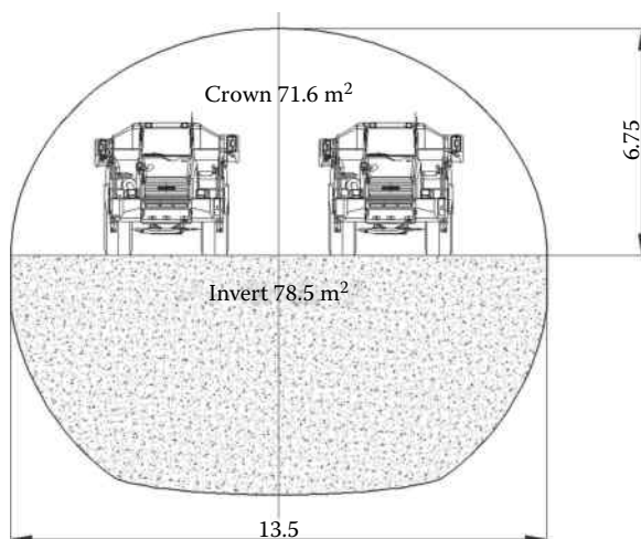
FIGURE 8.5 Cross section of the power tunnel.
