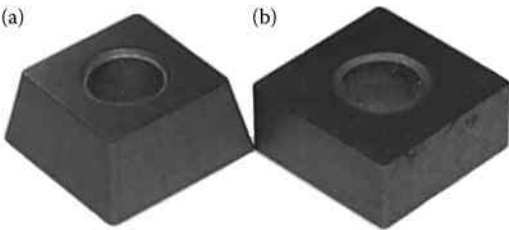
FIGURE 15.4 Rectangular prism tools: four-edge tool (a) and eight-edge tool (b).
