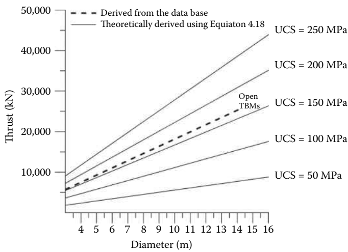
FIGURE 9.6 Relationship between diameter and thrust for open-type TBMs for different rock compressive strength.
