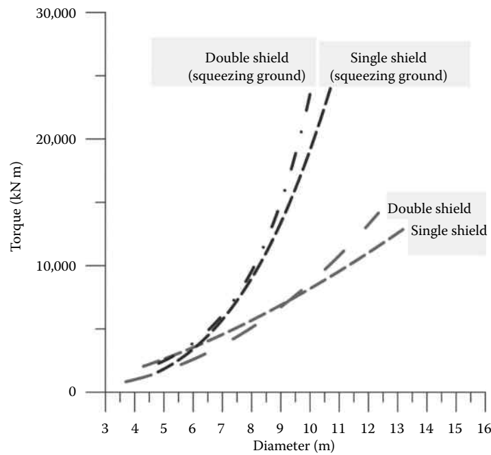
FIGURE 9.10 Relationship between TBM diameter and torque for single- and double-type TBMs.
