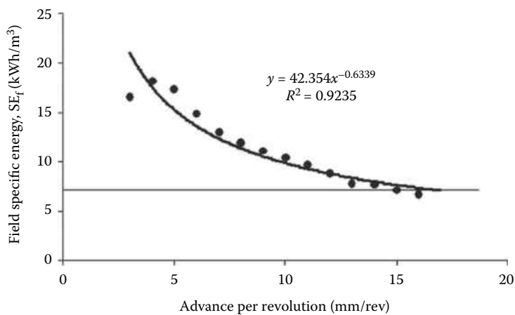
FIGURE 9.16 Relationship between advance per revolution and field SE in Kadikoy–Kartal Metro Tunnel for Kartal Dolayoba limestone, siltstone, and carbonated shale with mean compressive strength of 50 MPa. (Adapted from Bilgin, N. et al., 2012b. Rock mechanics aspects related to cutting efficiency of mechanical excavators, 25 years of experience in Istanbul, EUROCK 2012 , Stockholm.)
