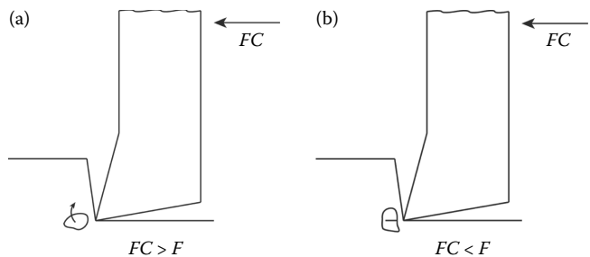
FIGURE 6.3 Theoretical consideration of cutting a quartz grain. (a) Quartz grain is broken from the rock matrix and (b) quartz grain is cut.
