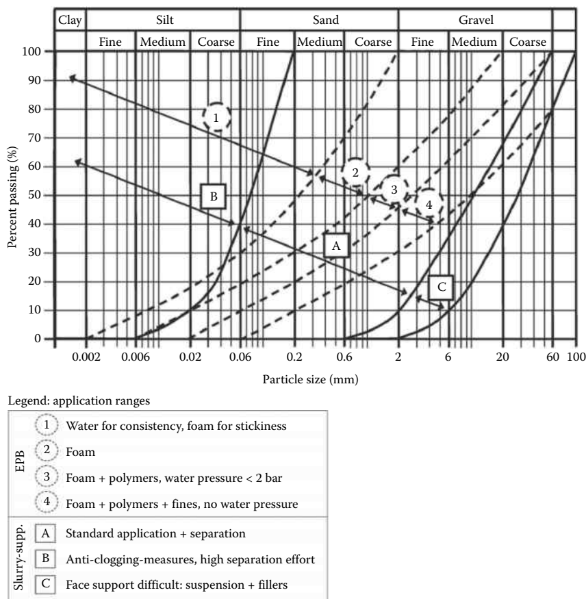
FIGURE 10.2 Applicable soil ranges for SPB and EPB TBMs. (Adapted from Thewes, M., 2007. Proc. the 2nd Symposium on Underground Excavation for Transportation , November 15–17, Istanbul, pp. 49–56; Thewes, M., Budach, C., 2010. Geomechanics and Tunnelling , 3(3):256–267)
