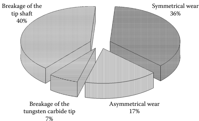
FIGURE 6.15 Classification of cutter wear in Kucuksu tunnel.
