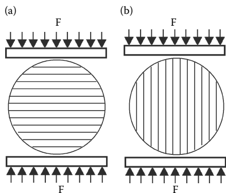
FIGURE 3.7 Foliation effects of the loading direction. (a) Parallel to bedding and (b) perpendicular to bedding.
