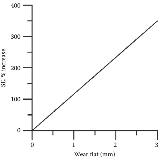
FIGURE 6.8 The relationship between wear flat and specific energy increase in percent.
