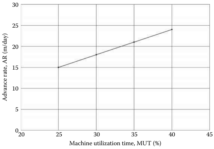
FIGURE 7.15 Variation of daily AR with MUT for 14\text{ m}^2 of cross-section area.
