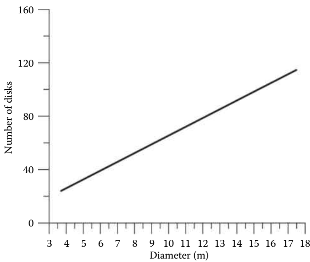
FIGURE 9.13 Relationship between TBM diameter and number of disks for all types of TBMs.
