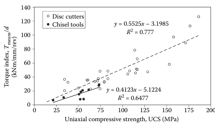
FIGURE 4.15 Relationship between uniaxial compressive strength of rocks and torque index (torque of TBM per unit depth of cut per revolution) of TBM for chisel tools and disk cutters. (Adapted from Bilgin, N., Copur, H., Balci, C., 2012. Tunnelling and Underground Space Technology , 27, 41–51.)
