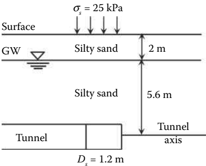
FIGURE 11.6 Geometry for Numerical Example 11.5.7.
