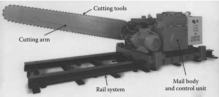
FIGURE 15.1 Basic modules of a chain saw machine. (Courtesy of Garrone, Product Catalogues. With permission.)
