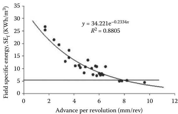
FIGURE 9.17 Relationship between advance per revolution and field SE in Beykoz Tunnel for limestone, sandstone, and carbonated shale with mean compressive strength of 100 MP. (Adapted from Bilgin, N., Copur, H., Balci, C., 2012a. Tunnelling and Underground Space Technology , 27, 41–51.)
