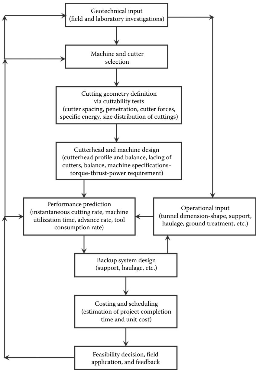
FIGURE 5.1 Generalized mechanical excavation system. (Modified after Copur, H., 1999. Theoretical and experimental studies of rock cutting with drag bits toward the development of a performance prediction model for roadheaders. PhD thesis, Colorado School of Mines, 361 p.)
