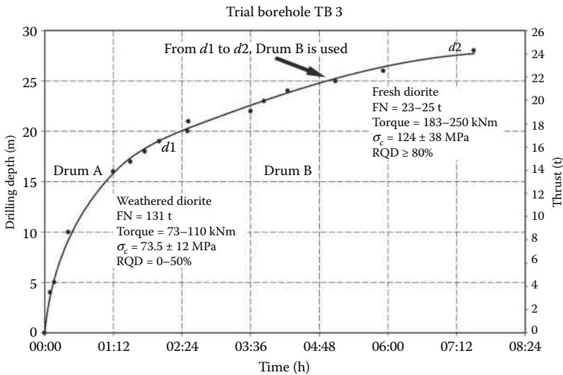
FIGURE 13.6 The relationships between drilling depth and drilling time for trial borehole TB3. (Adapted from the archive of Bilgin, N., 2006. A large-diameter drill rig study in Cifteler construction site in Istanbul. Istanbul Technical University, p. 30.)
