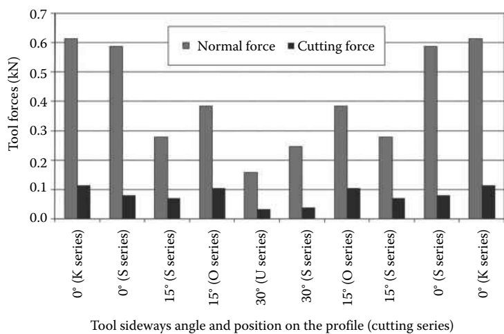
FIGURE 15.9 Variation of tool forces on a sequence of tools.
