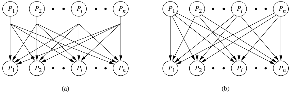
Figure 5.4 Two all-to-all communication patterns: (a) all-broadcast communication and (b) all-scatter communication.
