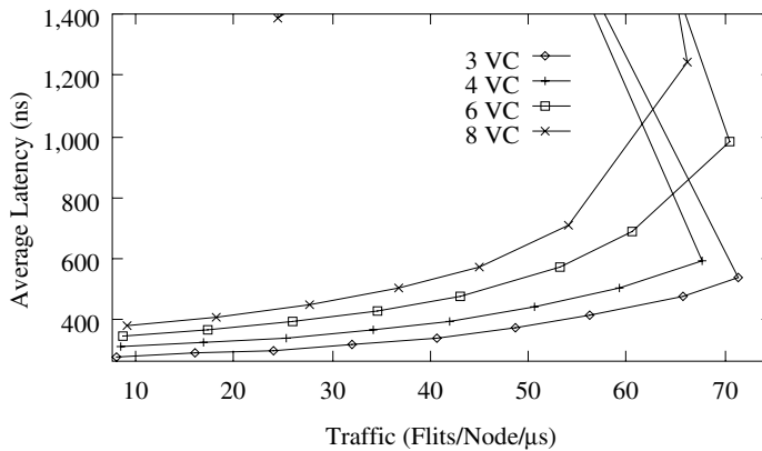
Figure 9.41 Average message latency versus accepted traffic as a function of the number of virtual channels for the fully adaptive routing algorithm.
