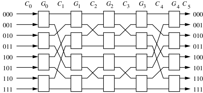
Figure 1.17 An 8 \times 8 Beneš network.
