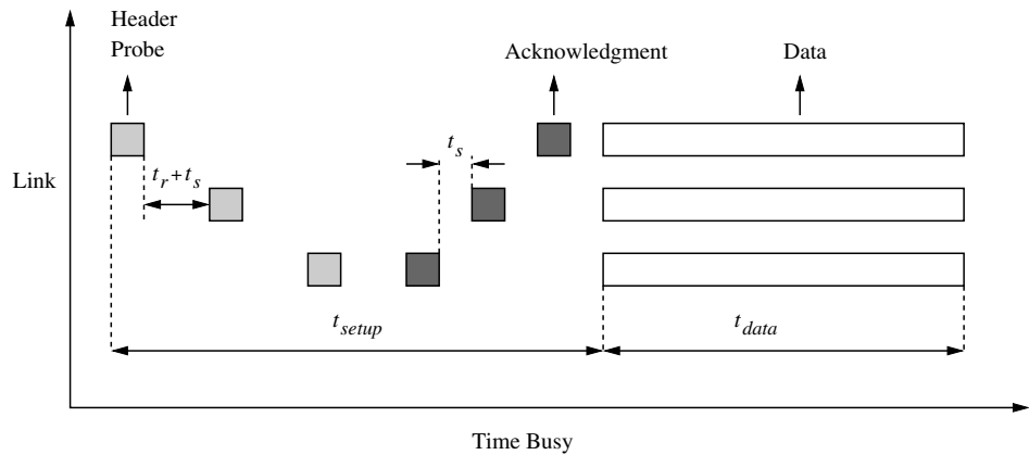
Figure 2.6 Time-space diagram of a circuit-switched message.
