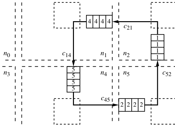
Figure 3.2 Deadlocked configuration for R .
