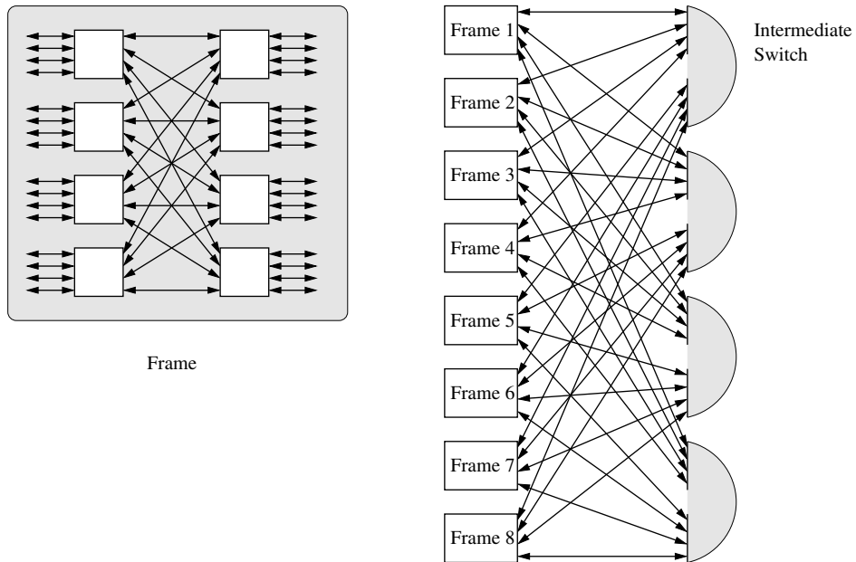
Figure 7.46 System interconnect using an SP2 frame.
