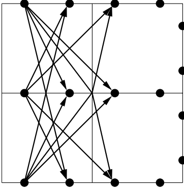
Figure 3.26 Indirect dependencies of the extended channel dependency graph for R_1 .
