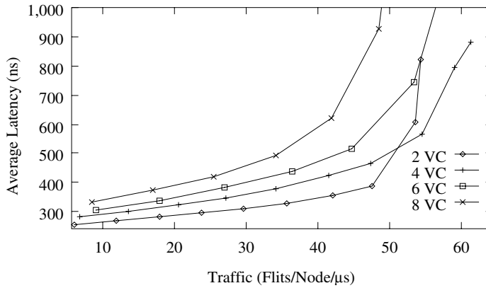
Figure 9.40 Average message latency versus accepted traffic as a function of the number of virtual channels for the partially adaptive routing algorithm.
