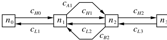
Figure 3.27 Channel labeling for the linear array.
