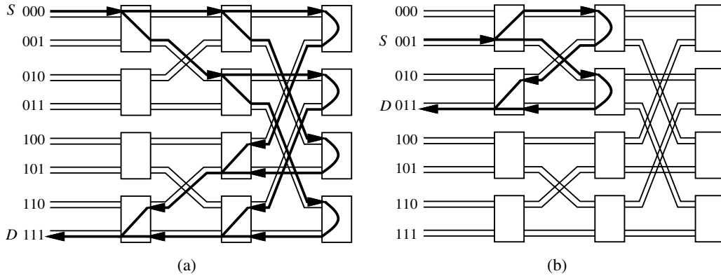
Figure 4.33 Paths available in an eight-node butterfly BMIN: (a) \text{FirstDifference}(S, D) = 2 ; (b) \text{FirstDifference}(S, D) = 1 .
