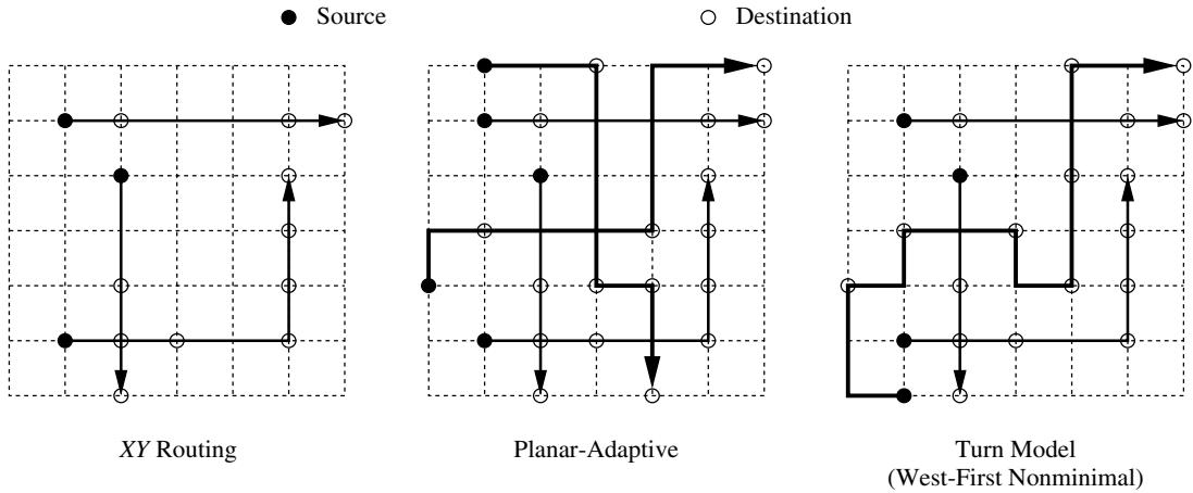
Figure 5.36 Examples of multideestination messages on a 2-D mesh under the BRCP model.
