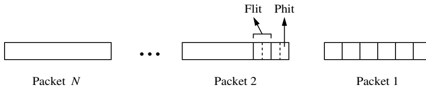
Figure 2.2 Alternative flow control units in a message.
