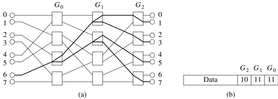
Figure 5.23 Multicast on multistage networks using multiport encoding: (a) path followed by a multideestination message; (b) message format using multiport encoding.
