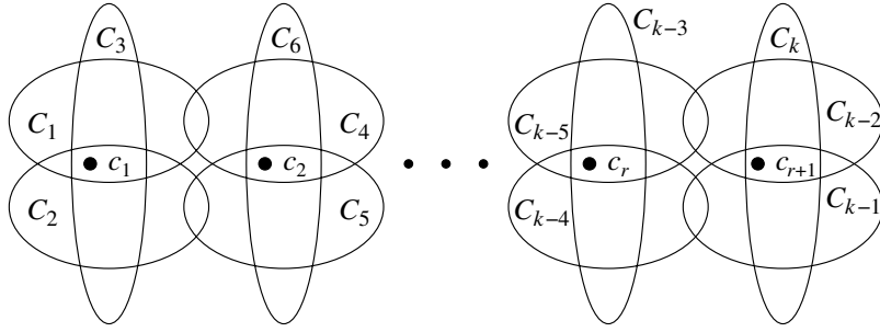
Figure 6.2 Channel sets supplied by all the minimally connected routing subfunctions of R and the corresponding elements in C_m .
