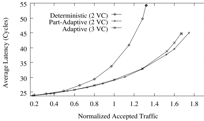
Figure 9.10 Average message latency versus normalized accepted traffic for local traffic (side = 2).
