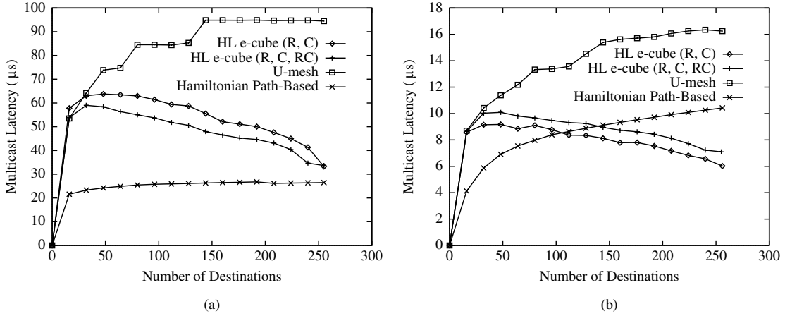
Figure 9.46 Comparison of single-source multicast latency on 16 \times 16 meshes with two different communication start-up ( t_s ) values: (a) t_s = 10\mu s and (b) t_s = 1\mu s (from [268]).
