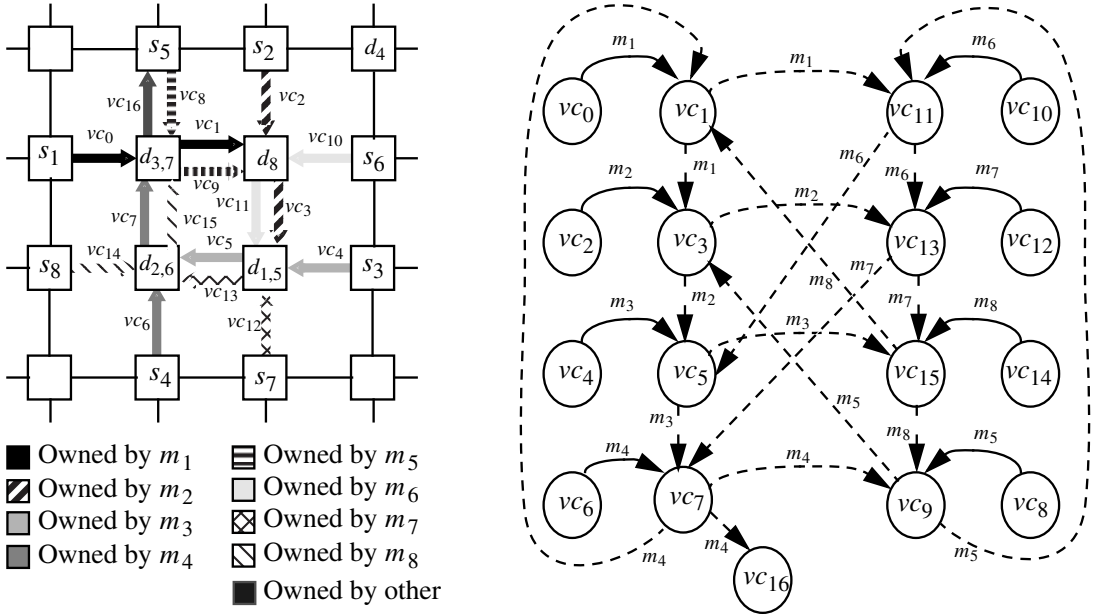
Figure 3.15 A cyclic nondeadlocked network state under minimal adaptive routing with two virtual channels per physical channel (from [283]).
