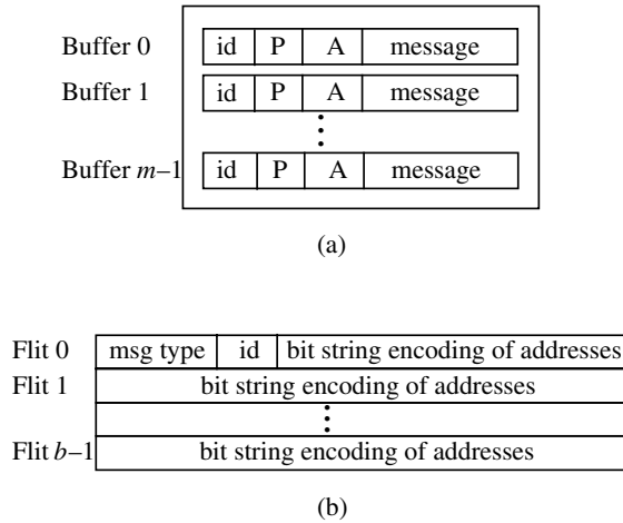
Figure 5.43 Architectural supports for implementing multidestination gather/broadcasting messages: (a) synchronization buffers at a router interface; (b) message format (from [265]). (A = arrived/not arrived; id = synchronization id; P = participate/not participate.)
