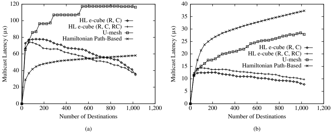
Figure 9.47 Comparison of single-source multicast latency on 32 \times 32 meshes with two different communication start-up ( t_s ) values: (a) t_s = 10\mu s and (b) t_s = 1\mu s (from [268]).
