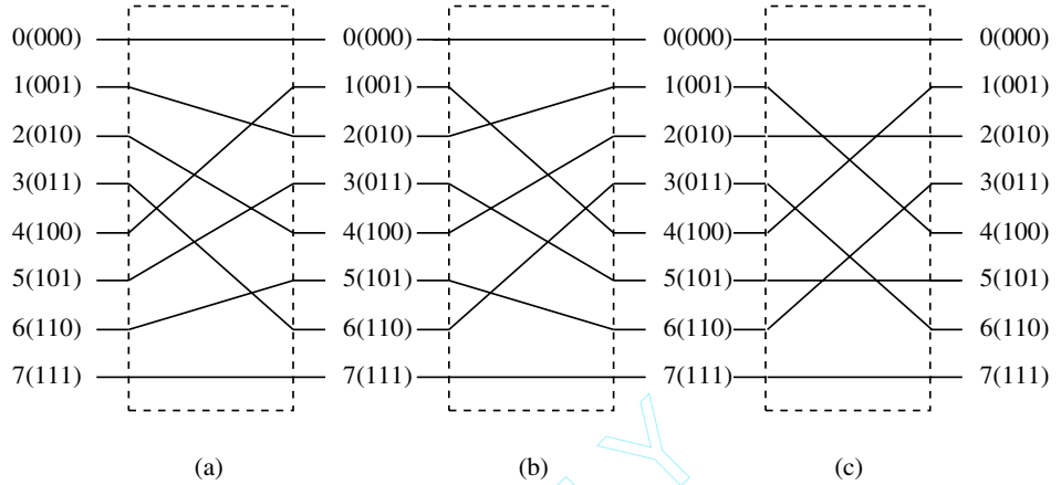
Figure 1.13 (a) The perfect shuffle, (b) inverse perfect shuffle, and (c) bit reversal permutations for N = 8 .
