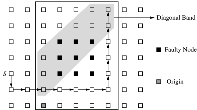
Figure 6.25 Fault-tolerant routing using origin-based routing.
