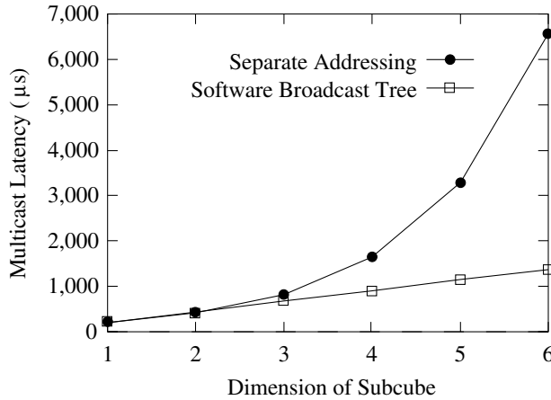
Figure 9.42 Comparison of 100-byte broadcasts on a 64-node nCUBE-2.
