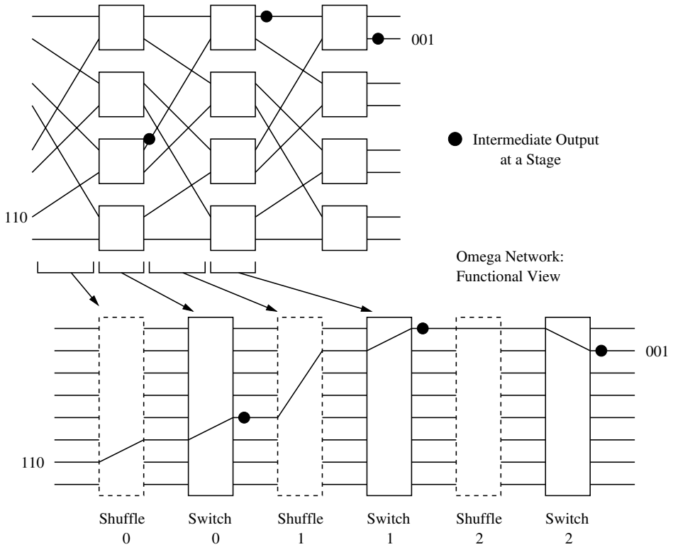
Figure 4.31 Functional view of the structure of a multistage Omega network.
