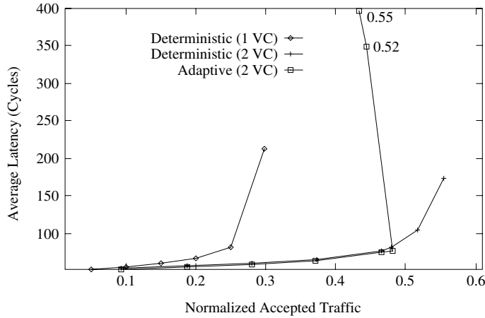
Figure 9.2 Average message latency versus normalized accepted traffic on a 16 \times 16 mesh for a uniform distribution of message destinations.
