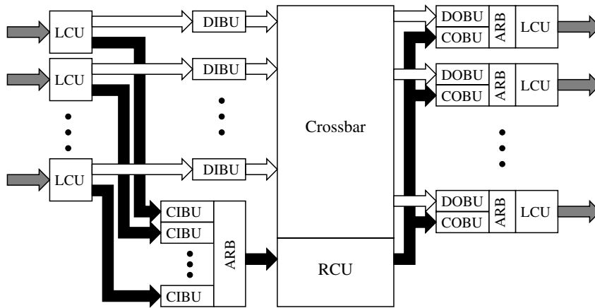
Figure 7.42 Block diagram of Ariadne: a PCS router.
