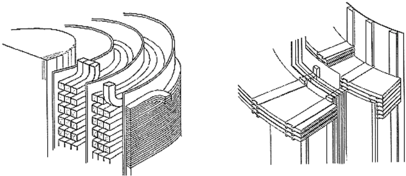
A helical winding closest to the core followed by a disc winding and a layer winding for voltage regulation.
