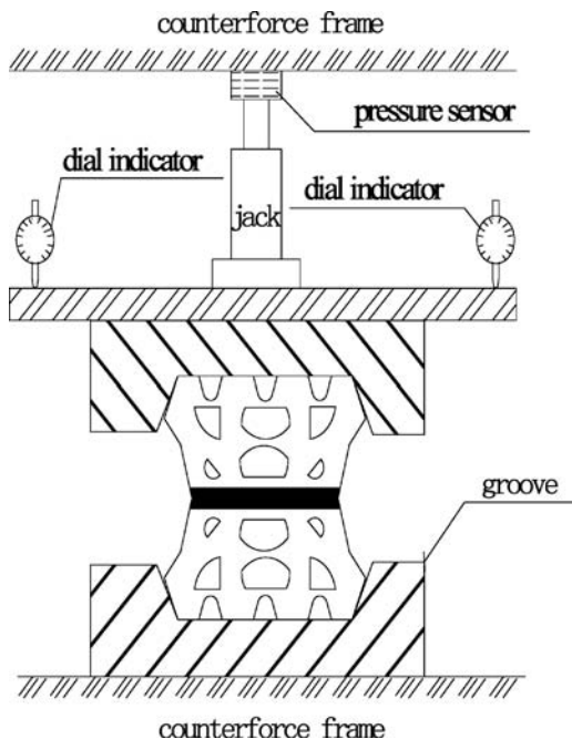
Figure 3. Compression deformation test of bar sample.
