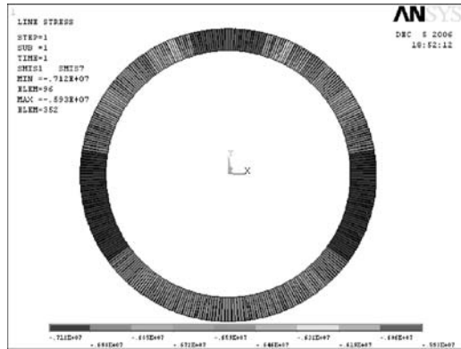
Figure 12. Axial forces.
