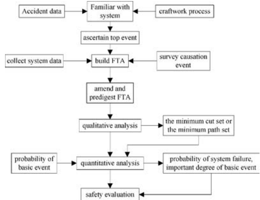
Figure 5. Flowchart of FTA.
