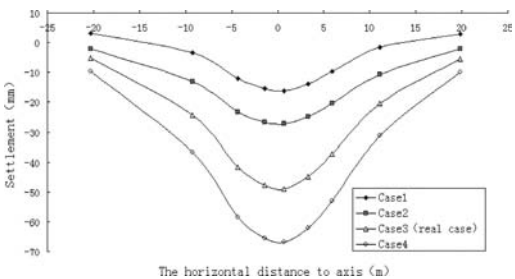
Figure 4. Surface settlement comparison between different construction conditions.
