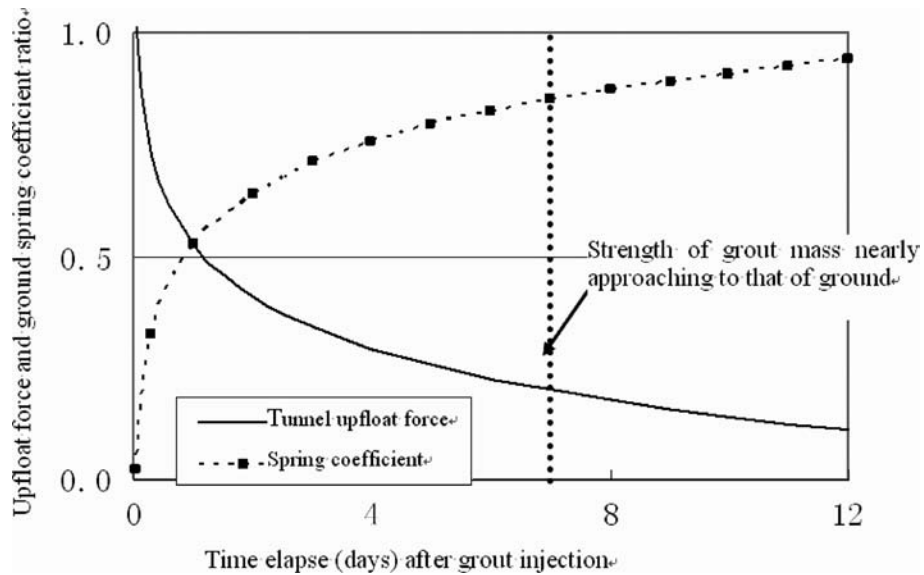
Figure 7. Schematic calculation modeling simulated on uplift longitudinal upon tunnel segments.
