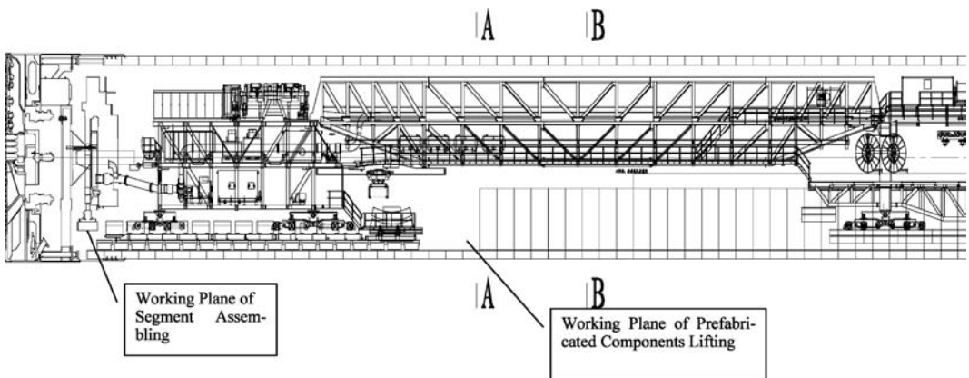
Figure 2. Shield machinery and backup system layout.
