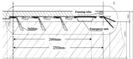
Figure 10. Tailskin structure.
