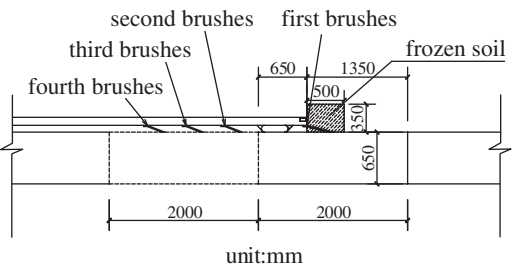
Figure 8. Schematic plan of frozen reinforced zone.
