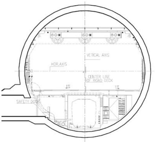
Figure 5. LRT only cross passage.
