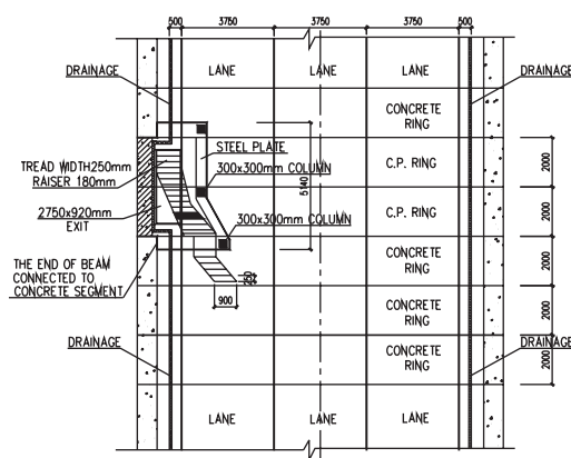
Figure 10. Plan on escape stairs.
