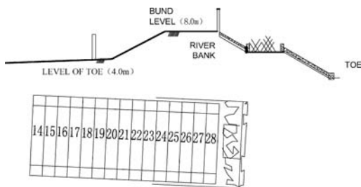
Figure 13. TBM advancing under the bank of Yangtze River.
