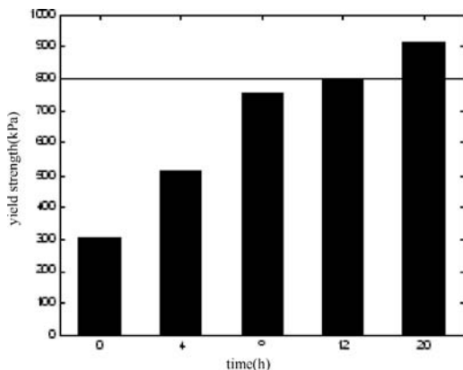
Figure 3. Yield strength variation of grout.
