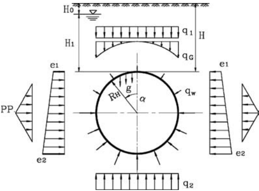
Figure 3. Calculation diagram of modified routine method. *In the figure, H 0 -Depth of underground water (m); H 1 -Height of hydrostatic head; H- Embedment depth (m); q 1 -Top vertical earth pressure (kPa); q 2 -Vercial reaction of bottom foundation (kPa); q G -Earth pressure of extrados (kPa); q W -Hydrostatic pressure (kPa); e 1 -Top horizontal earth pressure (kPa); e 2 -Bottom horizontal earth pressure (kPa); PP-Earth pressure of lateral triangle (kPa); R H -Calculated radius (m);g-Self-weight of lining (kPa); \alpha -Angel between calculated section and vertical axle ( ^{\circ} ), counterclockwise direction is considered as positive.
