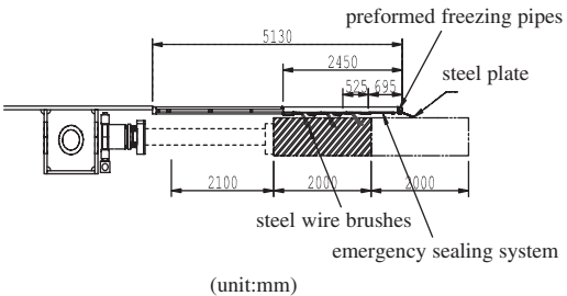
Figure 1. Inflatable sealing system at shield tail.
