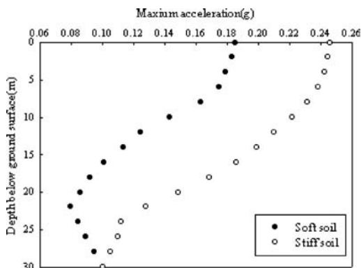
Figure 3. Calculated maximum accelerations for two types of soil.
