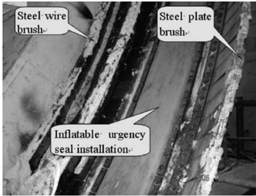
Figure 2. Picture of shield tail seal structure.
