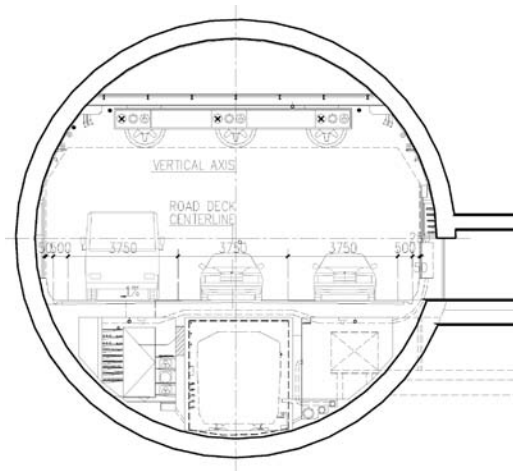
Figure 4. Road deck only cross passage.
