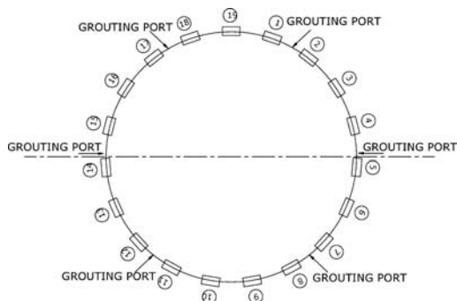
Figure 21. Location of grout ports for Yangtze Tunnel drive.
