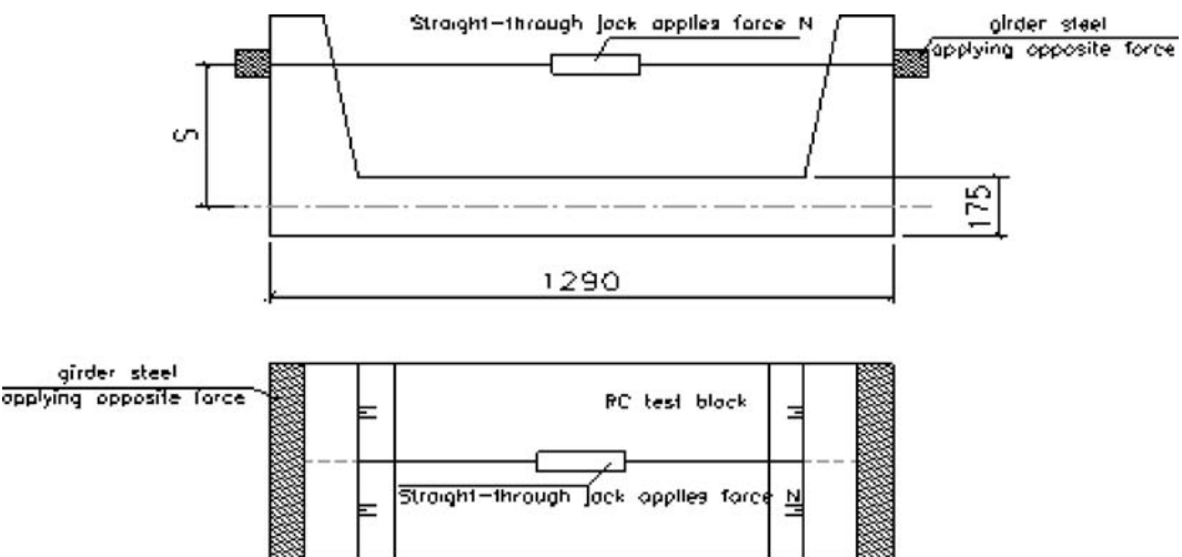
Figure 3. Specimen loading.
