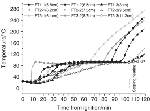
Figure 4. Temperature-time curves of the specimens of FT1, FT2 and FT3.
