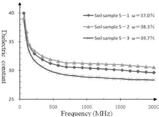
Figure 12. The curve of dielectric constant of the soil samples in the fifth soil layer (5-1, 5-2, 5-3) changing in frequency.
