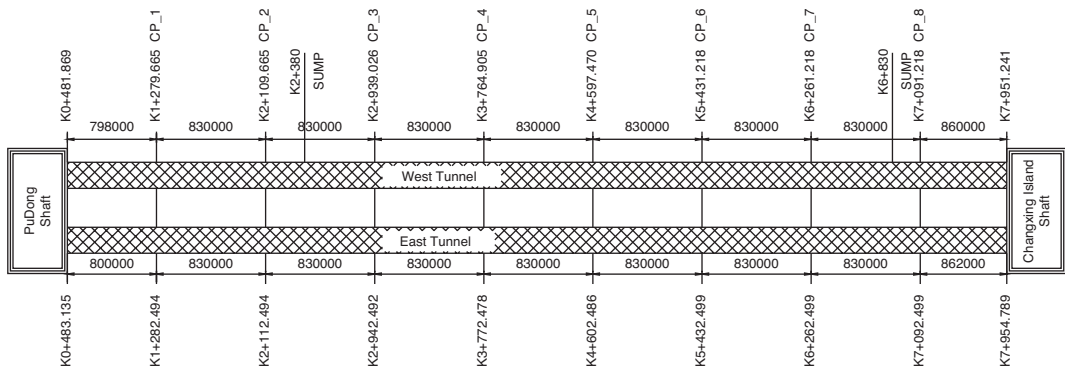
Figure 3. Schematic of original cross passage provisions.
