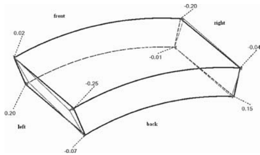
Figure 5. Mould correction.
