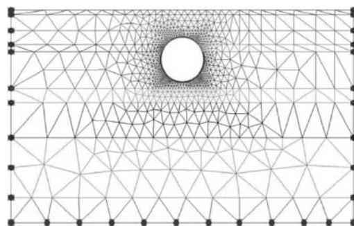
Figure 2. Mesh of the model.
