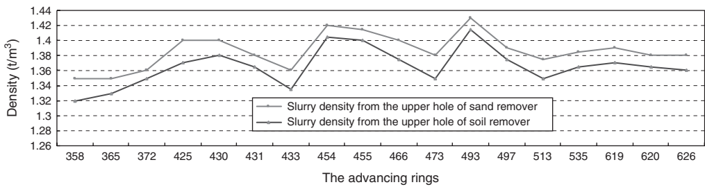
Figure 7. The trend of the density slurry coming out from the upper hole of sand remover and soil remover in the upline.
