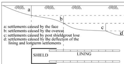
Figure 15. Settlement principle.
