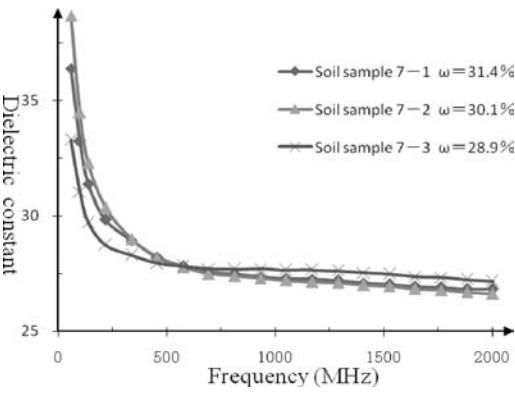
Figure 14. The curve of dielectric constant of the soil samples in the seventh soil layer (7-1, 7-2, 7-3) changing in frequency.
