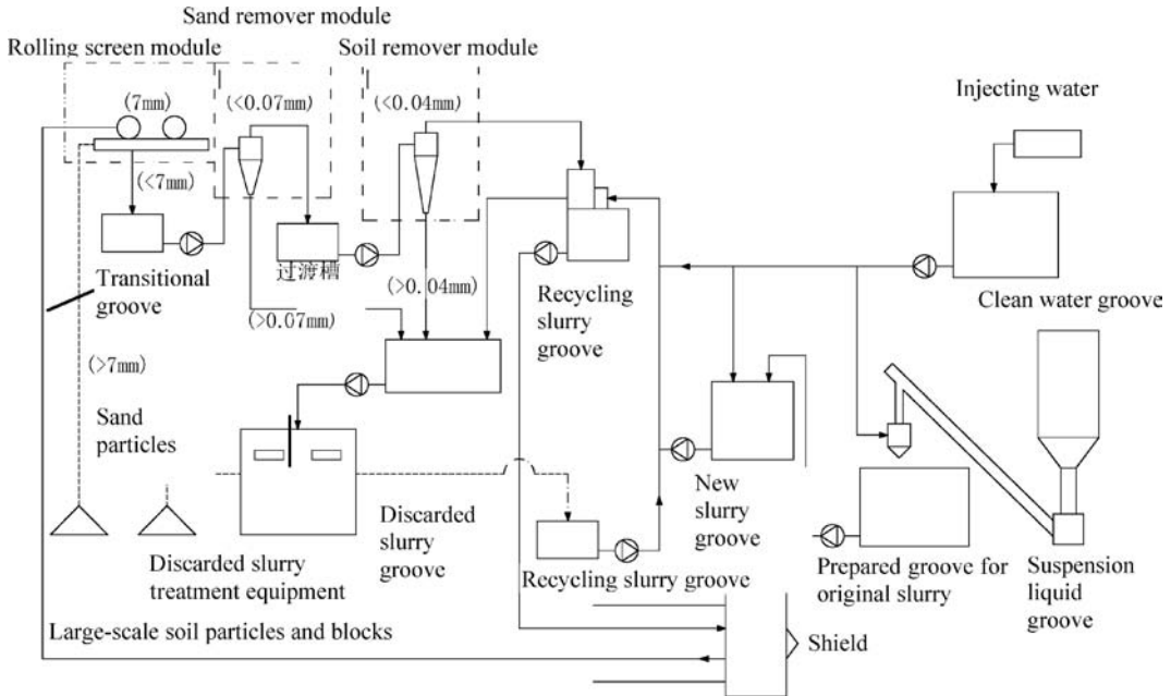
Figure 3. The integrated modules system in slurry treatment in Yangtze River Tunnel.
