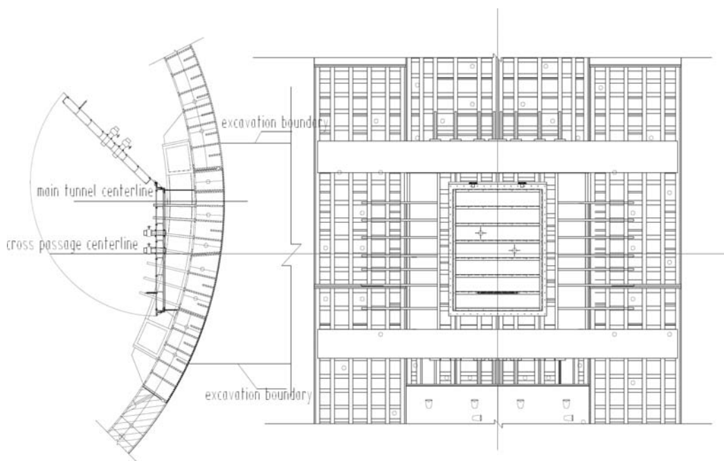
Figure 6. Protection device for segment.
