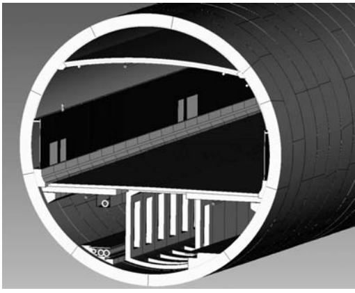
Figure 4. 3D model of a shield tunnel.
