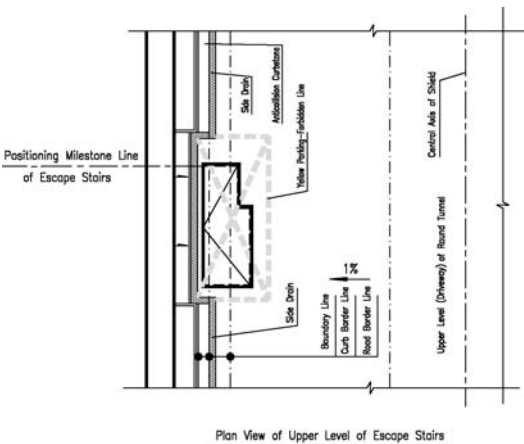
Figure 2. Escape stairs and safe exits.
