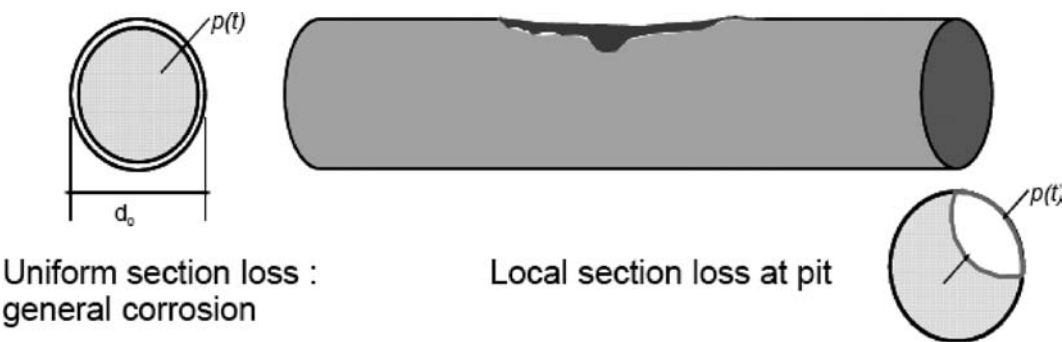
Figure 5. Section loss due to uniform and pitting corrosion.
