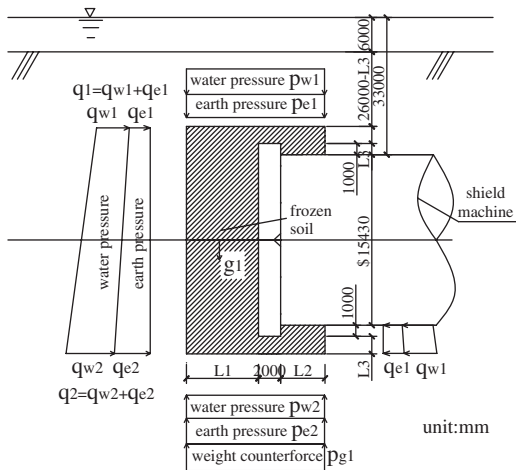
Figure 2. Force diagram of the frozen reinforced body.
