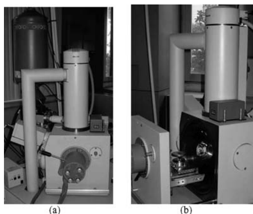
Figure 8. Set-up of ESEM apparatus.
