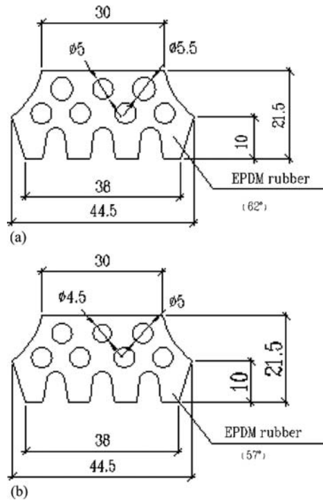
Figure 10. Gasket cross sections used in the project.
