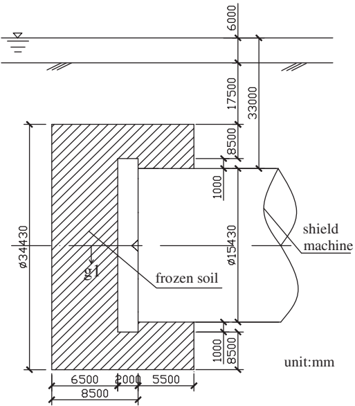
Figure 4. Frozen soil zone.
