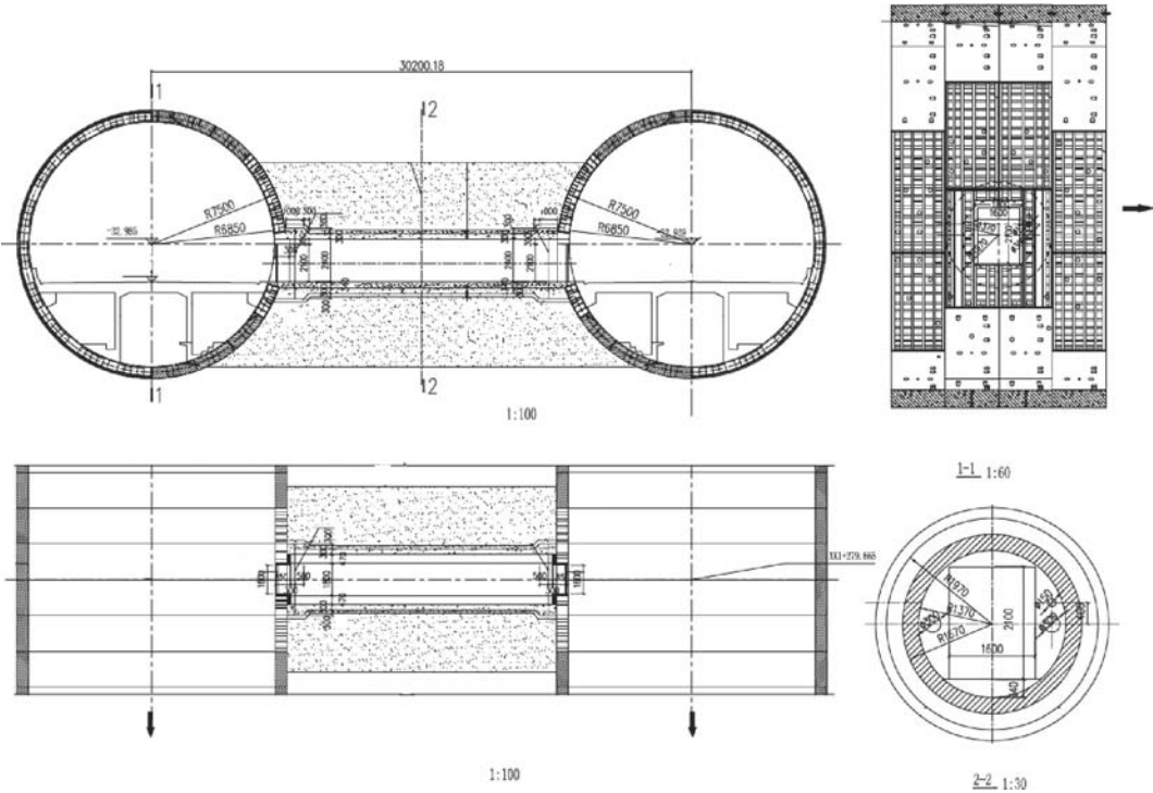
Figure 2. Cross passage structure sketch.
