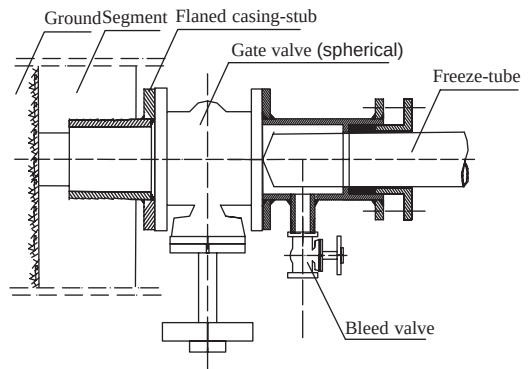
Figure 5. Blow-out preventer
