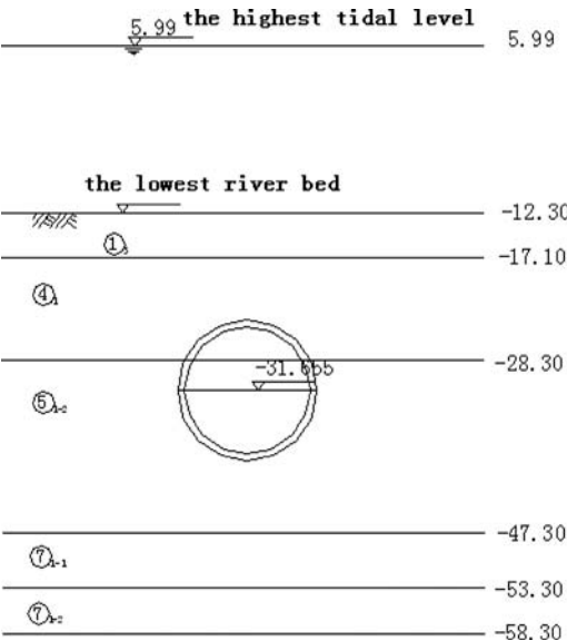
Figure 4. Cross-section of case 1.
