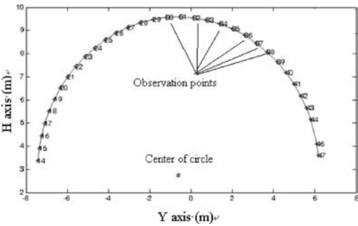
Figure 3. The distribution of the surveying points and the position of the centre of the circle.
