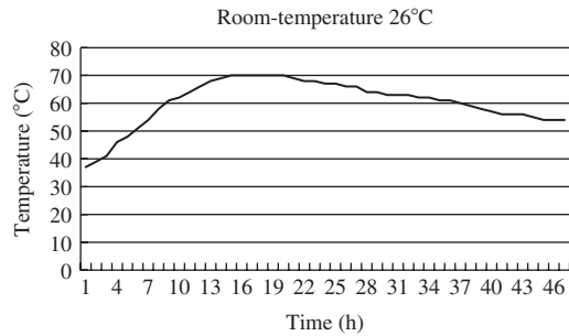
Figure 1. Segment inside temperature variation curve.
