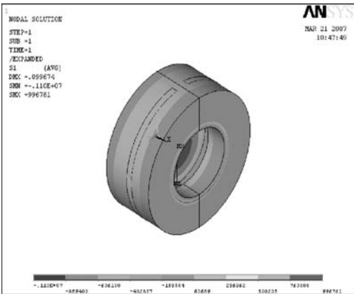
Figure 3. Distribution of the first principal stress.
