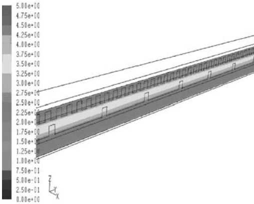
Figure 5. Velocity profile of flow field in streamline direction at z = -0.5 m.
