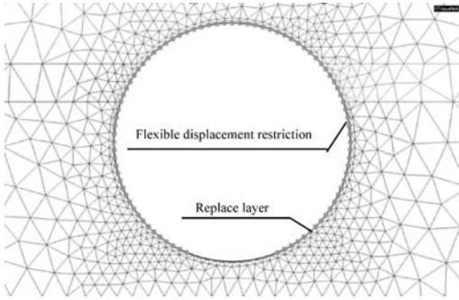
Figure 3. Flexible displacement limit around TBM and equivalent layer of surrounding ground.
