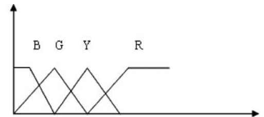
(c) Output membership function: degree of fault. where B-Normal; G-Early Fault; Y-Fault Warn; R-Fault Alarm.
