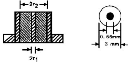
Figure 1. The sketch map of the coaxial probe.
