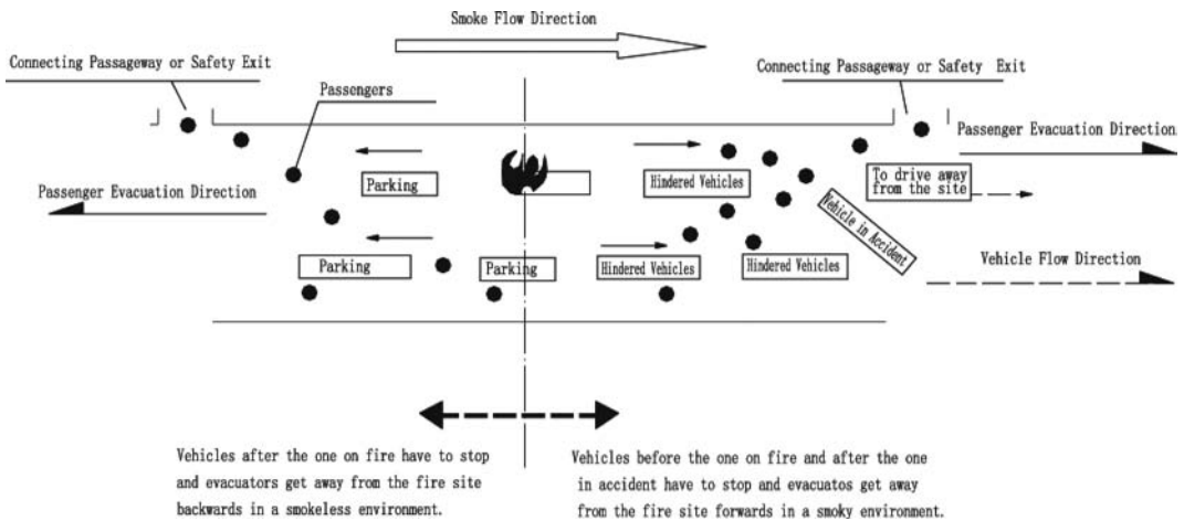
Figure 4. Passenger evacuation in a clogged operation condition.
