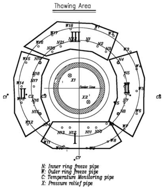
Figure 15. Divided thawing area of cross passage.
