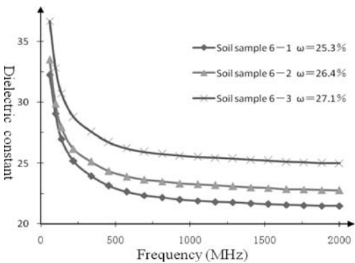
Figure 13. The curve of dielectric constant of the soil samples in the sixth soil layer (6-1, 6-2, 6-3) changing in frequency.
