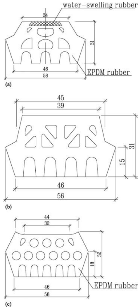
Figure 2. Cross-sections of three flexible rubber gaskets.
