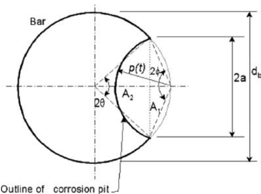
Figure 6. Calculation of residual area of an idealized pitted bar.
