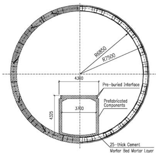
Figure 3. Cross section of road structure, phase I.
