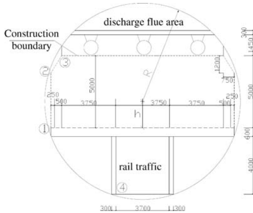
Figure 2. Sketch of tunnel section.
