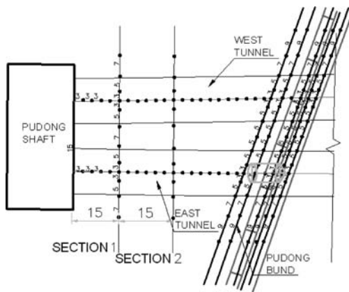
Figure 14. Monitoring point layout.
