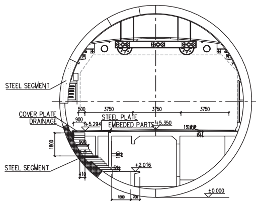
Figure 9. Cross section escape stairs.
