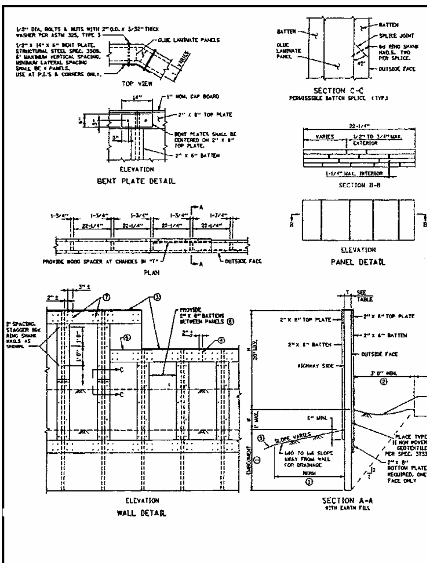
FIGURE 9.12 Typical design for noise wall using self-supporting, vertical wood glue-laminate panels: type II, aligned panels. (Adapted from Minnesota DOT design standards)
