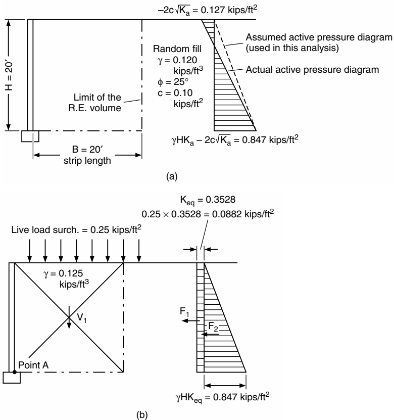
FIGURE 8.41 Design of Reinforced Earth retaining wall showing (a) active earth pressure, (b) addition of pressure from surcharge, (c) analysis at intermediate level, and (d) effective strip length. (From the Reinforced Earth Co., with permission)
