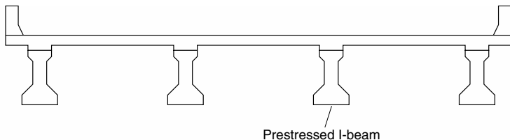
FIGURE 4.9 Cross section of prestressed-concrete I-beam bridge.
