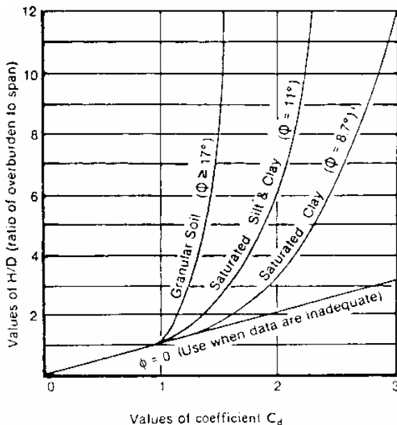
FIGURE 5.42 Diagram for coefficient C_d for load calculations for tunnels. \phi is soil friction angle. (From Standard Specifications for Highway Bridges , American Association of State Highway and Transportation Officials, Washington, D.C., 1992, with permission)
