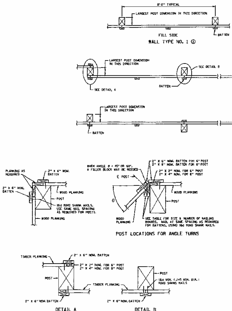
FIGURE 9.14 Typical design for noise wall using wood posts and horizontal tongue-and-groove timber panels. (Adapted from Minnesota DOT design standards)
