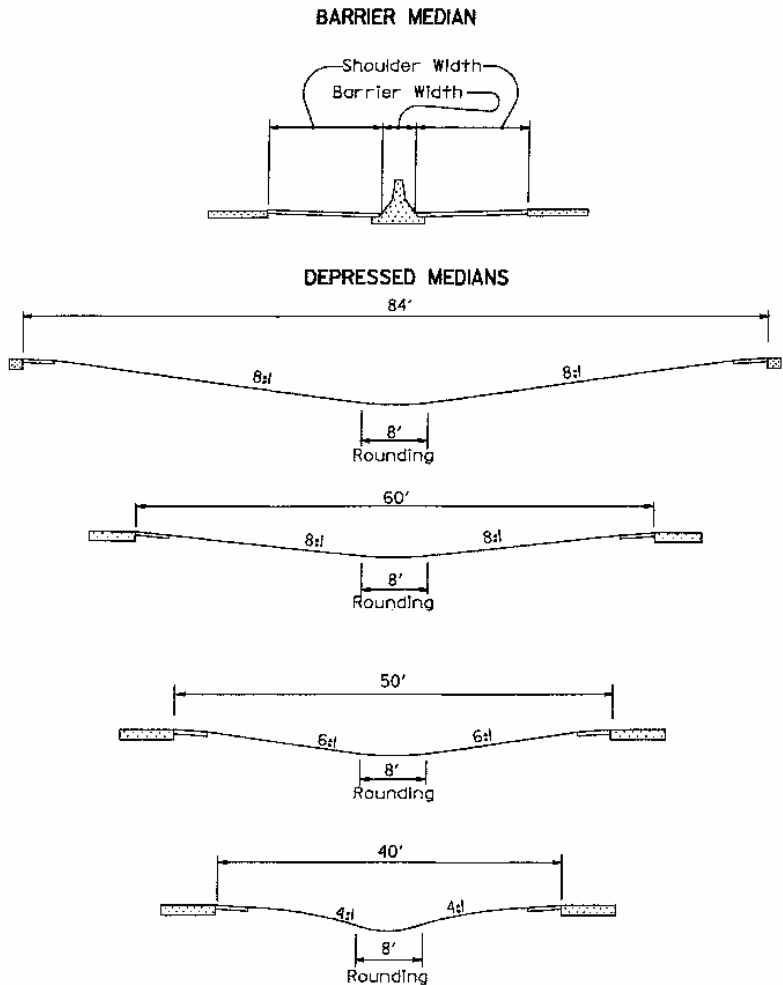
FIGURE 2.26 Typical designs for medians. (From Location and Design Manual, Vol. I, Roadway Design, Ohio Department of Transportation, with permission)
