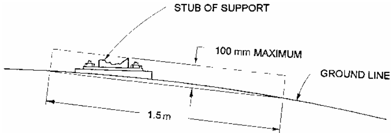
FIGURE 7.4 Breakaway support stub height measurement. Conversions: 100 mm = 4 in, 1.5 m = 5 ft.
