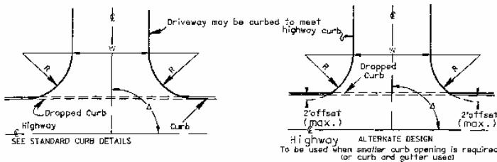
FIGURE 2.56 Designs for commercial drives. (From Location and Design Manual, Vol. 1, Roadway Design, Ohio Department of Transportation, with permission)
