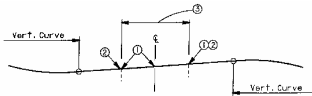
Example A - Crossroad Profile Tangent through Intersection
