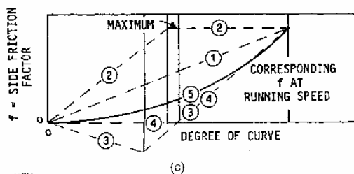
FIGURE 2.8 Methods of distributing superelevation and side friction. (a) Superelevation. (b) Corresponding friction factor at design speed. (c) Corresponding friction factor at running speed. (From A Policy on Geometric Design of Highways and Streets , American Association of State Highway and Transportation Officials, Washington, D.C., 1990, with permission)
