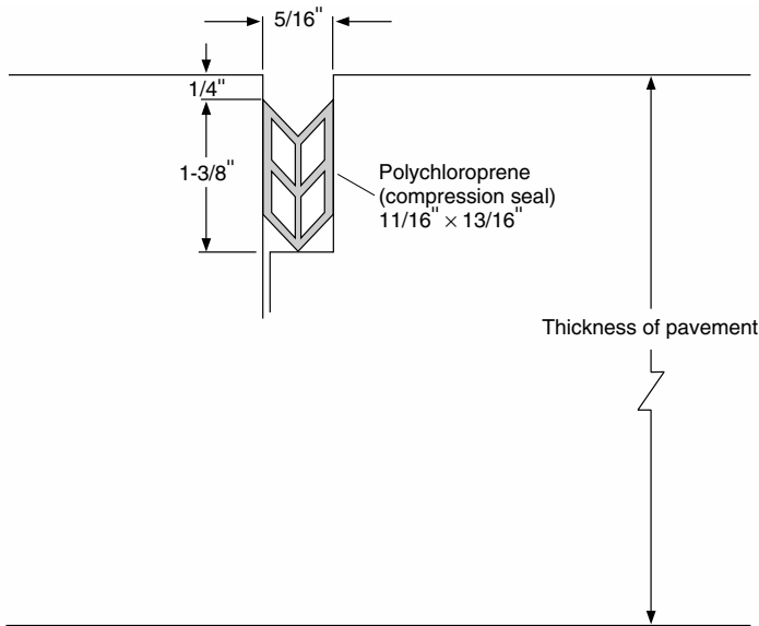
FIGURE 3.7 Typical preformed joint seal in rigid pavement.
