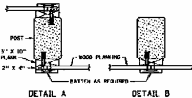
POST LOCATIONS FOR ANGLE TURNS
