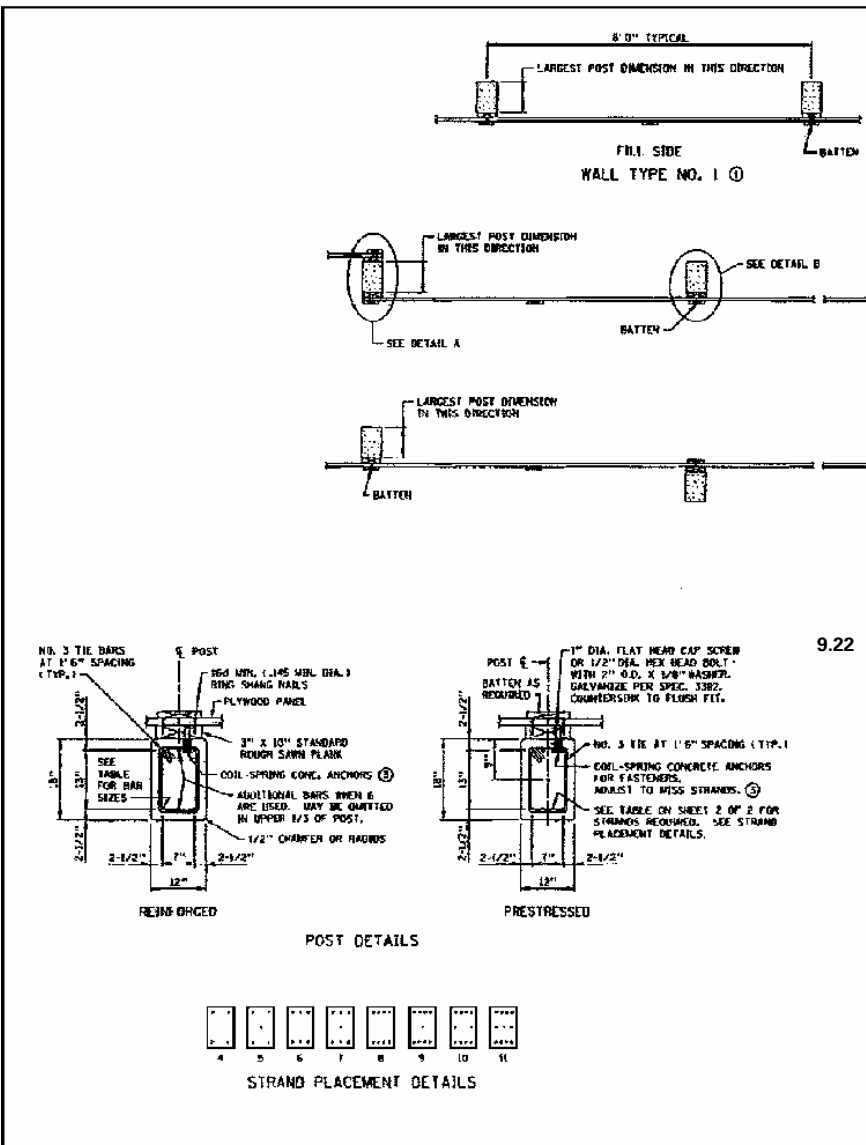
FIGURE 9.7 Typical design for noise wall using posts of reinforced or prestressed concrete and plywood panels. (Adapted from Minnesota DOT design standards)
