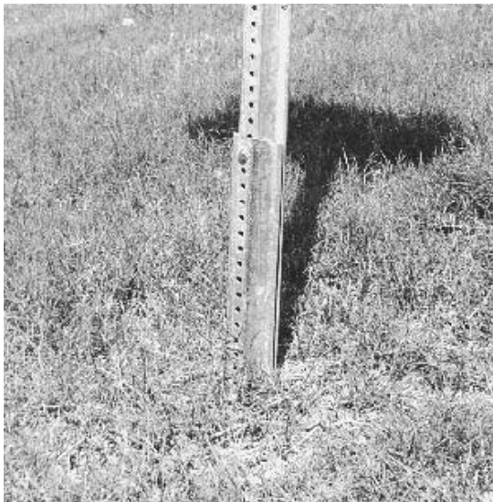
FIGURE 7.12 Improper splice of U-channel post system.
