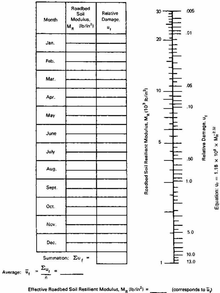
FIGURE 3.16 Chart for estimating effective roadbed soil resilient modulus for flexible pavements designed using the serviceability criteria. (From Guide for Design of Pavement Structures, American Association of State Highway and Transportation Officials, Washington, D.C., 1993, with permission)
