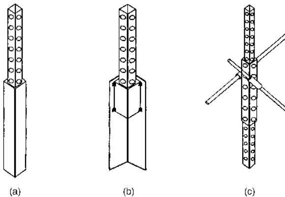
FIGURE 7.18 Anchor systems manufactured by Unistrut Corp. (a) Heavy-duty anchor. (b) Anchor post. (c) Stabilization anchor.
