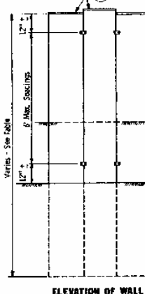
ELEVATION OF WALL
