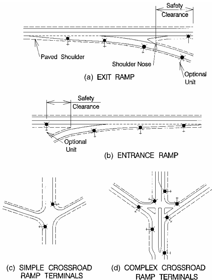
FIGURE 7.74 Typical luminaire locations for partial interchange lighting.
