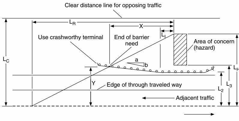
FIGURE 6.24 Layout of barrier approach. (From Roadside Design Guide, AASHTO, Washington, D.C., 2002, with permission)
