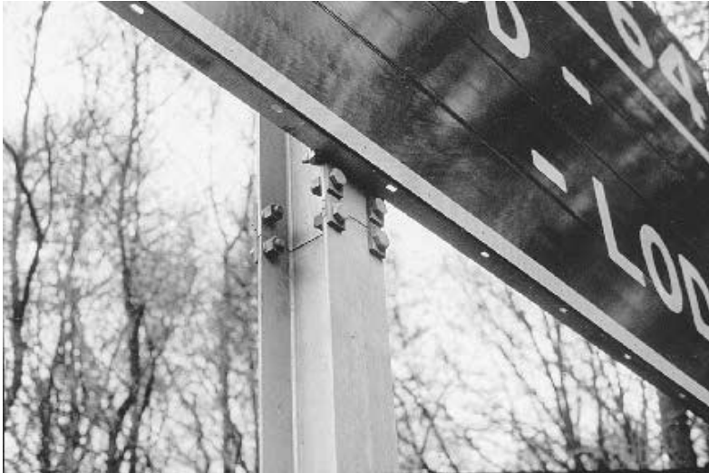
FIGURE 7.40 Commercially available hinge plates by Transpo Industries.
