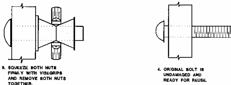
FIGURE 7.71 Vandalgard sign fastener.
