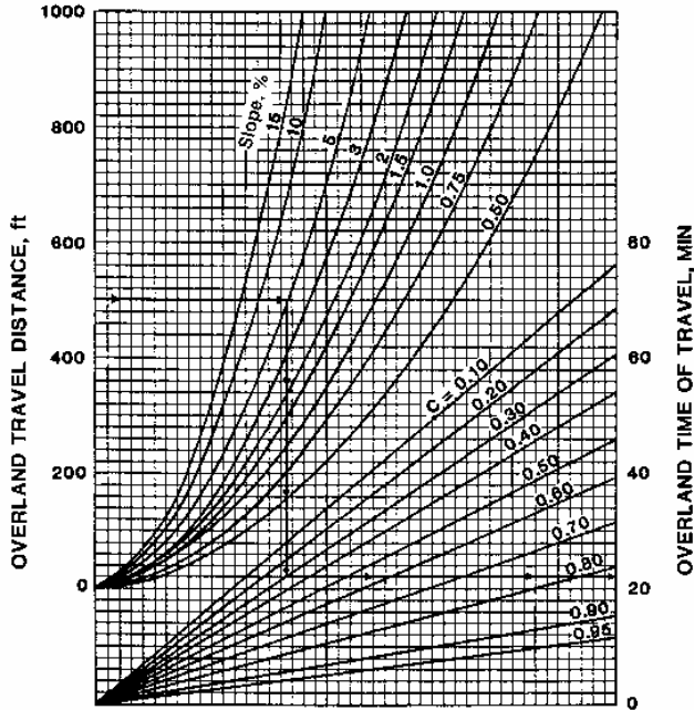
FIGURE 5.2 Overland time of concentration curves. (From Highway Design Manual, California Department of Transportation, with permission)
