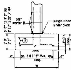
FOOTING DETAILS
