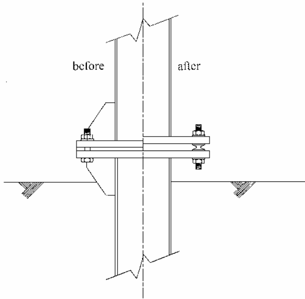
FIGURE 7.41 Typical before and after retrofit with Breaksafe.
