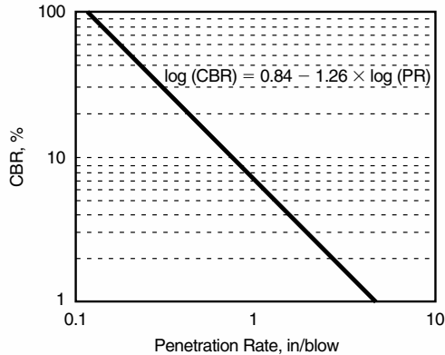
FIGURE 3.47 Correlation of California Bearing Ratio (CBR) and penetration rate. (From Pavement Technology Advisory 97-7 , Dynamic Cone Penetrometer, Illinois Department of Transportation, Bureau of Materials and Physical Research, 1997, with permission)
