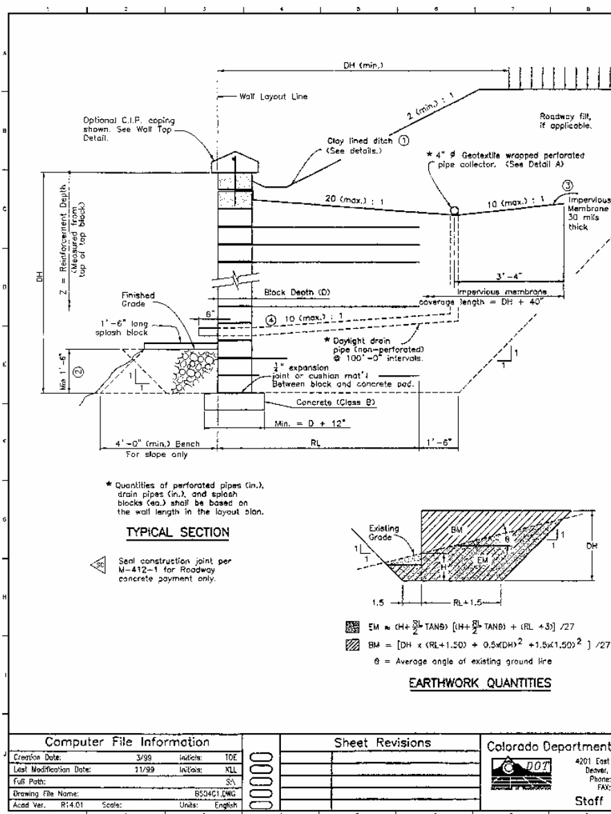
FIGURE 8.46a Worksheet for block facing MSE walls with 2-to-1 backslope, showing geometry and design assumptions. (From Bridge Design Work Sheets, Colorado Department of Transportation, Denver, Colo., with permission)
