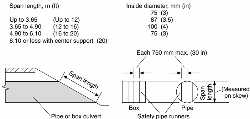
FIGURE 6.7 Safety treatment for ends of culverts showing diameters of grating (schedule 40 steel pipe) for various span lengths. (From Roadside Design Guide, AASHTO, Washington, D.C., 2002, with permission)
