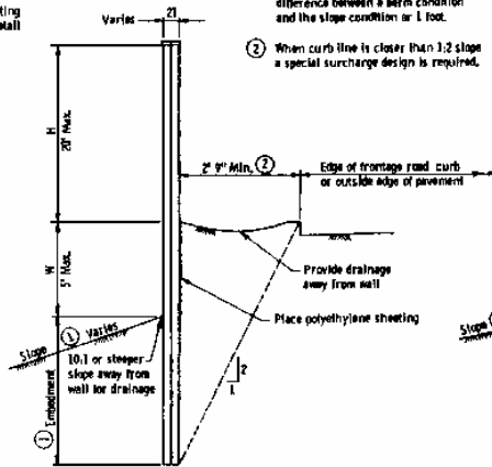
SECTION A-A WITH EARTH FILL
