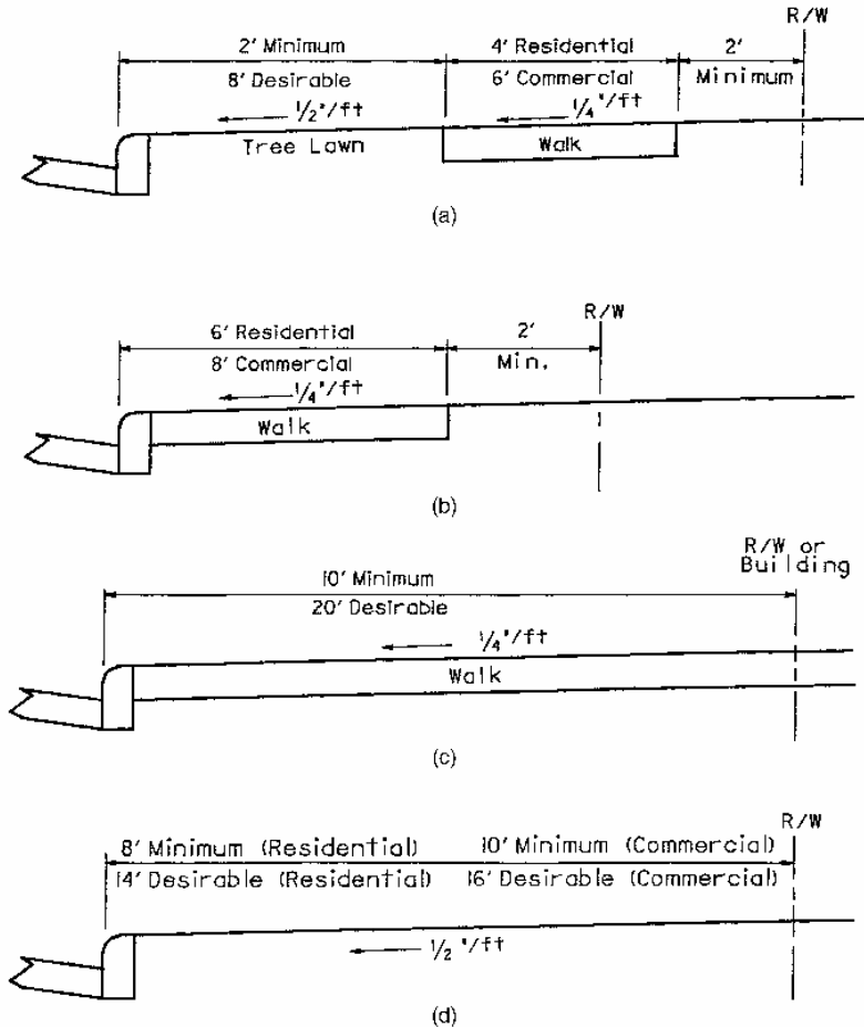
FIGURE 2.29 Examples of walk designs. (a) Walk with tree lawn. (b) Walk with no tree lawn. (c) Walk in downtown area. (d) Border area with no walk. (From Location and Design Manual, Vol. 1, Roadway Design, Ohio Department of Transportation, with permission)
