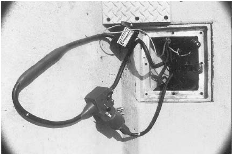
FIGURE 7.83 MG 2 /Duraline modular pole cable system.
