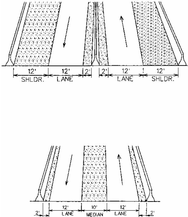
FIGURE 2.63 Cross sections for high-occupancy-vehicle two-way separated lanes on separated roadway. (From Guide for the Design of High Occupancy Vehicle Facilities, American Association of State Highway and Transportation Officials, Washington, D.C., 1992, with permission)
