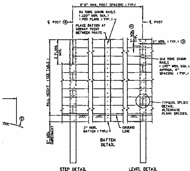
FRONT ELEVATION POST BATTENS NOT SHOWN
