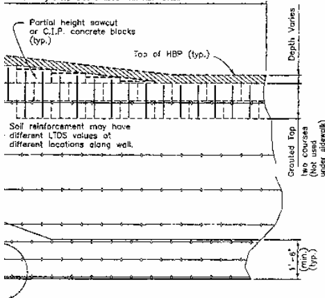
Partial Height top blocks used with HBP detail
