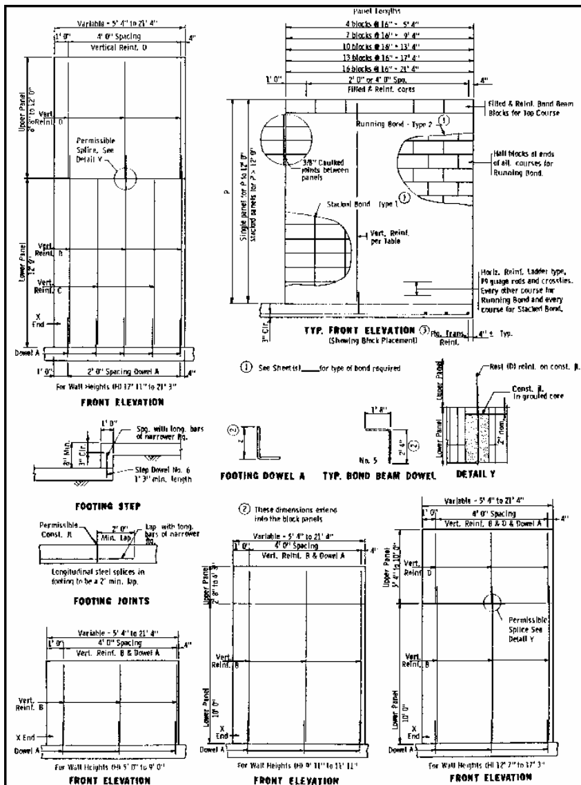
FIGURE 9.9 Typical design for noise wall using concrete block. (Adapted from Minnesota DOT design standards)
