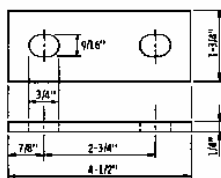
WASHER PLATE Structural Steel Spec. 3309
