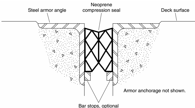
FIGURE 4.4 Cross section of compression seal.
