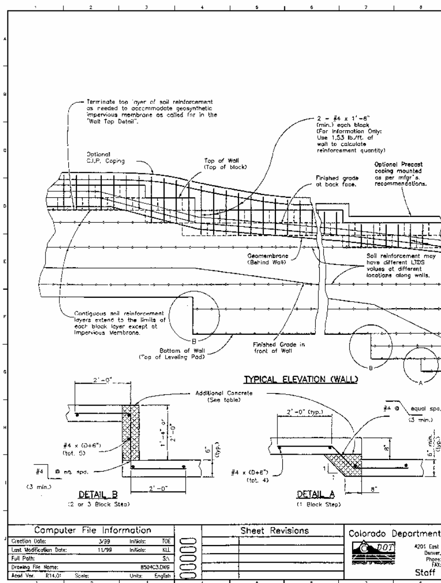
FIGURE 8.46c Worksheet for block facing MSE walls with 2-to-1 backslope, showing leveling pad, layout, and profile. (From Bridge Design Work Sheets, Colorado Department of Transportation, Denver, Colo., with permission)
