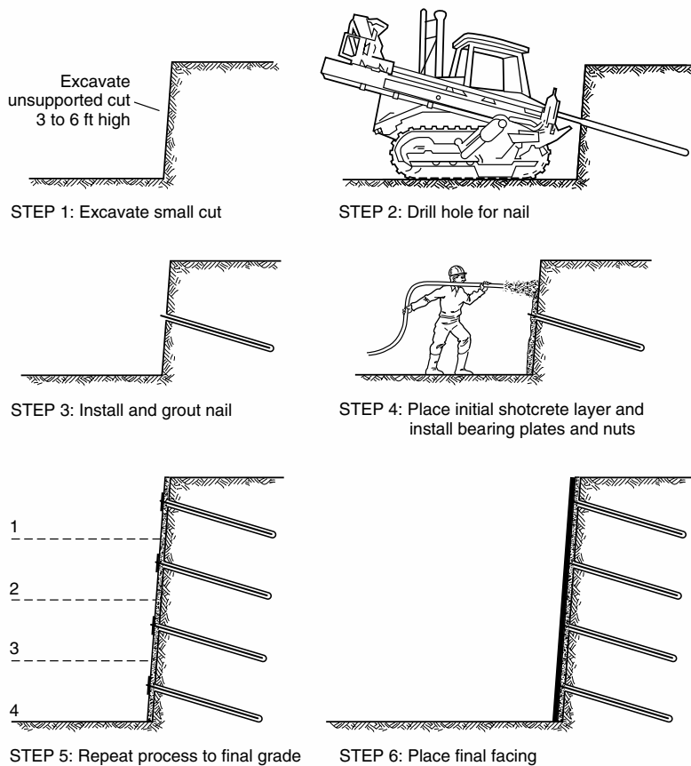
FIGURE 8.56 Typical construction sequence for soil nailed wall.
