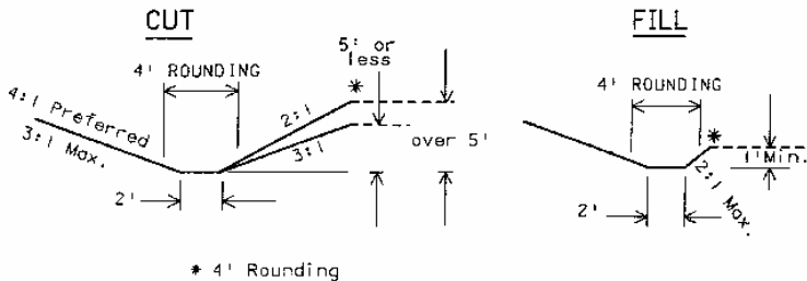
FIGURE 2.19 Examples of standard grading and normal ditches. (From Location and Design Manual, Vol. I, Roadway Design, Ohio Department of Transportation, with permission)
