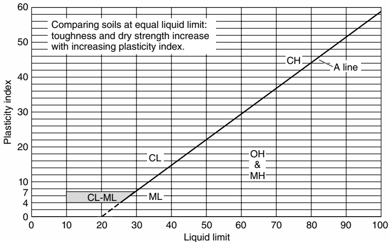
FIGURE 8.15 Plasticity chart for laboratory classification of fine-grained soils. (Adopted by U.S. Army Corps of Engineers and U.S. Bureau of Reclamation, January 1952)
