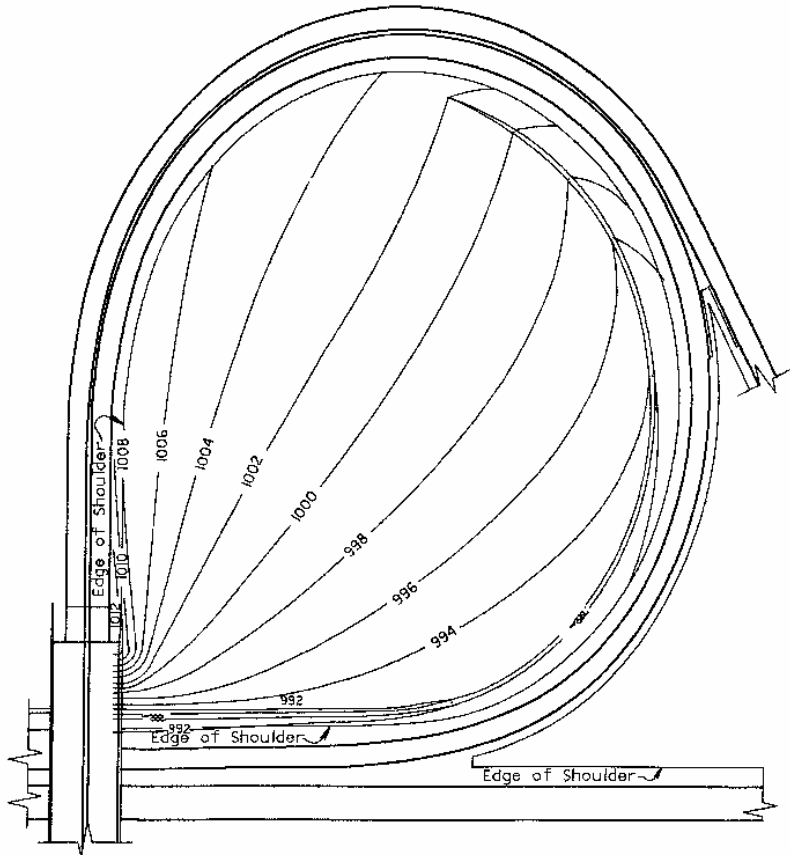
FIGURE 2.24 Contour grading of loop interior in cut section at interchange. (From Location and Design Manual, Vol. I, Roadway Design , Ohio Department of Transportation, with permission)
