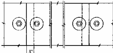
MOUNTING BRACKET DETAIL
