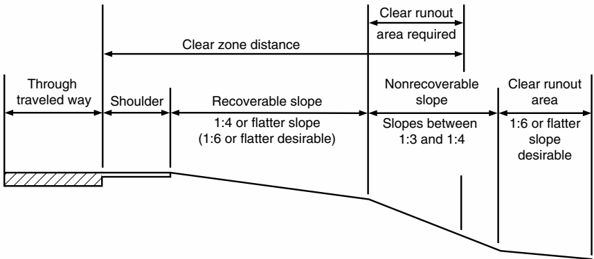
FIGURE 6.4 Example of “barn roof” section for parallel foreslope design; recoverable slope is followed by a nonrecoverable slope. (From Roadside Design Guide, AASHTO, Washington, D.C., 2002, with permission)
