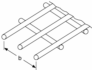
FIGURE 8.38 Metallic reinforcement for MSE walls showing correction for corrosion loss. (From the Reinforced Earth Co., with permission)
