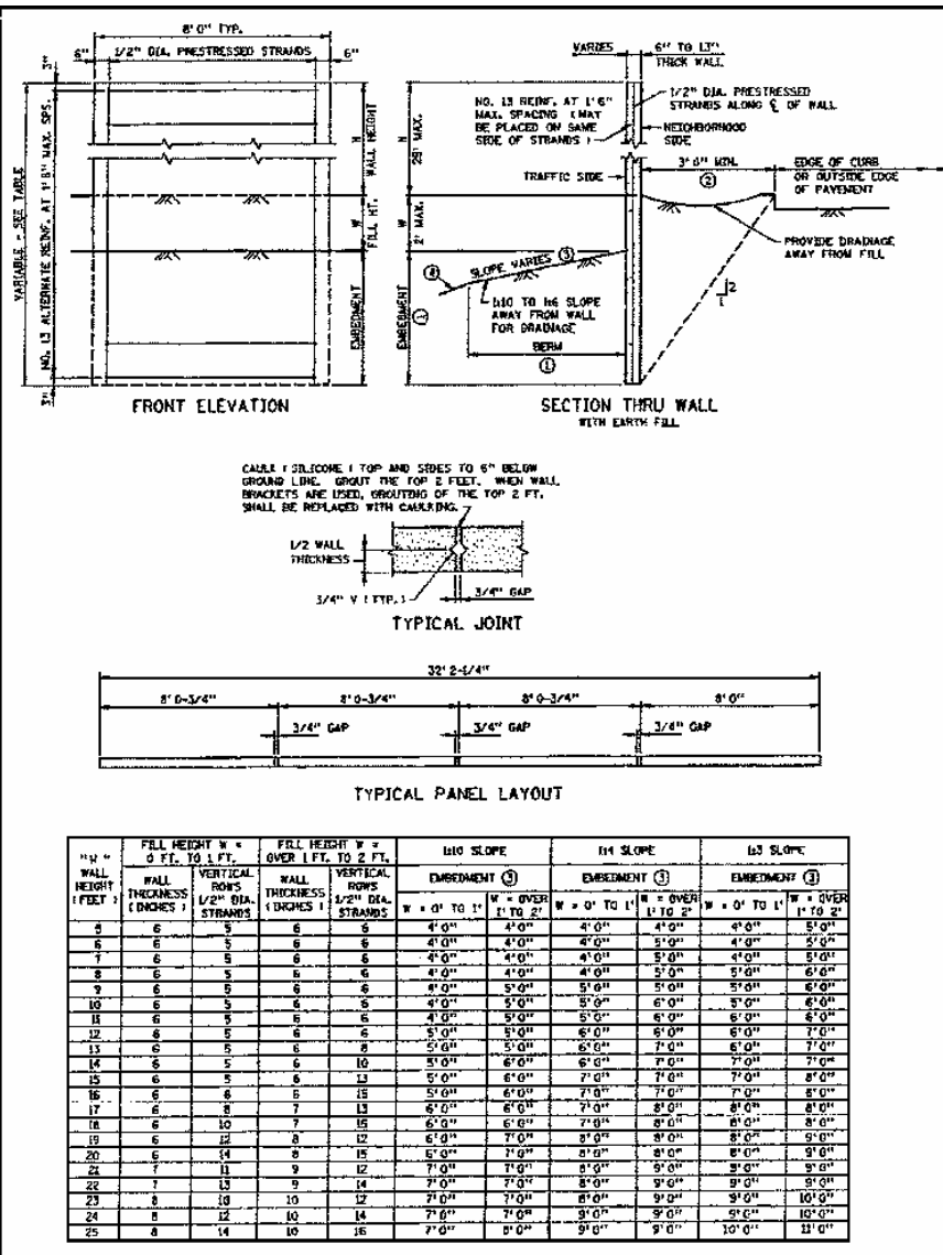
FIGURE 9.10 Typical design for noise wall using self-supporting, vertical prestressed concrete panels. (Adapted from Minnesota DOT design standards)
