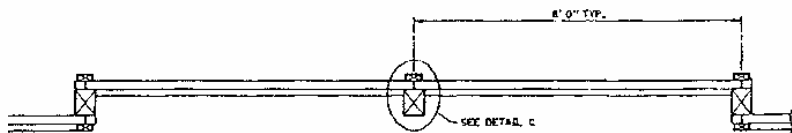
WALL TYPE NO. 2 ①②
