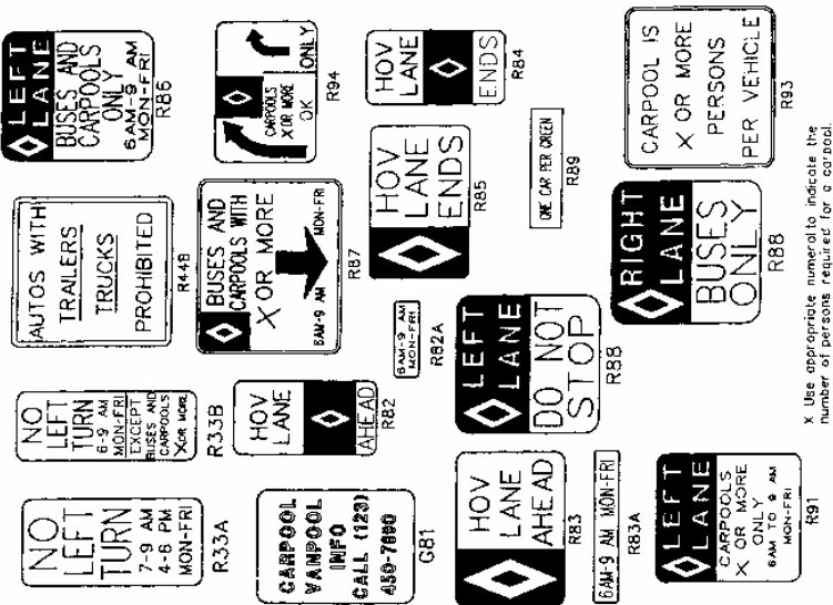
FIGURE 2.66 Sample signing and pavement markings for HOV lanes. (From Guide for the Design of High Occupancy Vehicle Facilities, American Association of State Highway and Transportation Officials, Washington, D.C., 1992, with permission)
