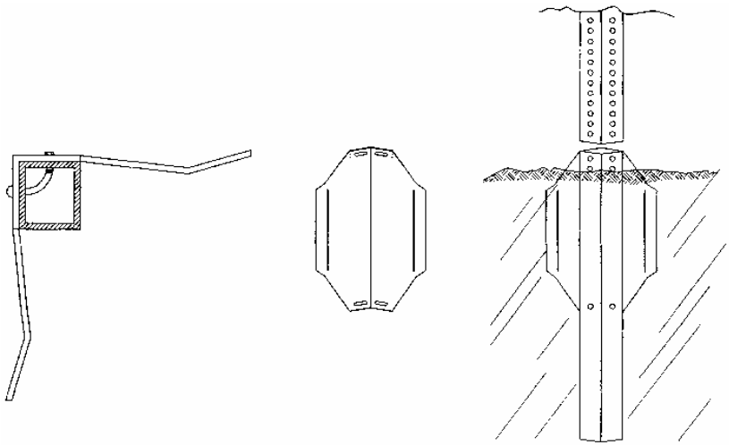
FIGURE 7.19 Anchor system manufactured by Xcessories Squared.
