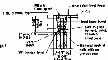
BOND BEAM CAP DETAIL
