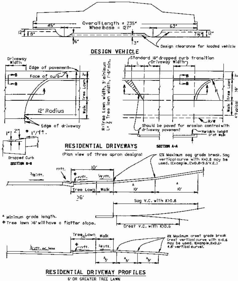
FIGURE 2.50 Details of driveway designs. (From Location and Design Manual, Vol. I, Roadway Design, Ohio Department of Transportation, with permission)
