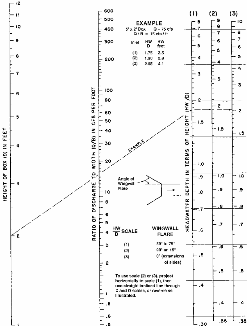
FIGURE 5.14 Flow nomograph for box culvert under inlet control. (From "Hydraulic Design of Highway Culverts," HDS 5, FHWA, with permission)
