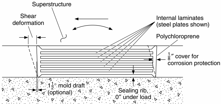
FIGURE 4.16 Elastomeric bearing for structural steel or concrete.
