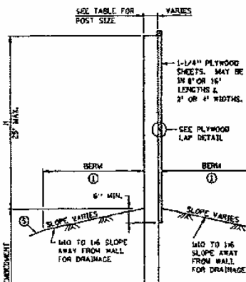
SECTION AT POST WITHOUT EARTH FILL
