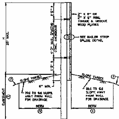
SECTION AT POST WITHOUT EARTH FILL
