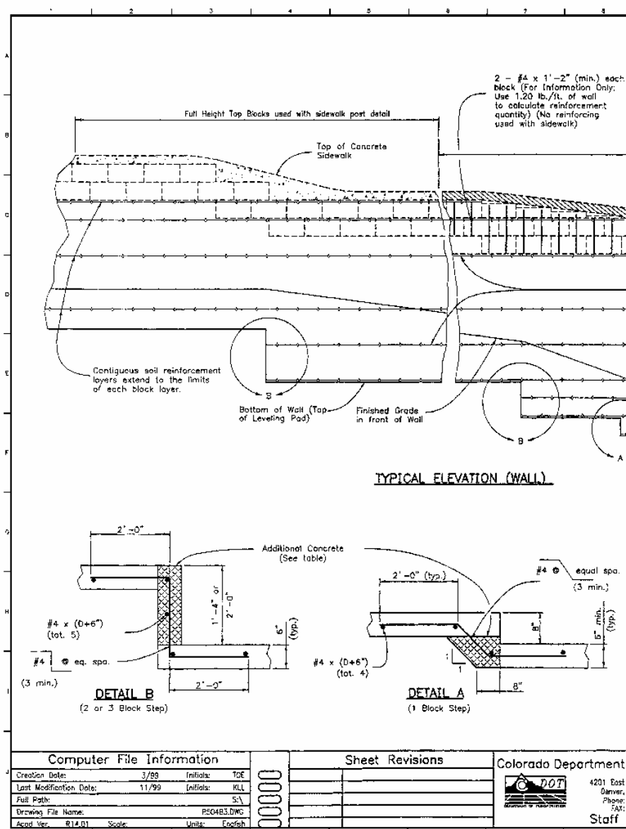
FIGURE 8.45c Worksheet for block facing MSE walls with post and W-beam barrier, showing leveling pad, layout, and profile. (From Bridge Design Work Sheets, Colorado Department of Transportation, Denver, Colo., with permission)
