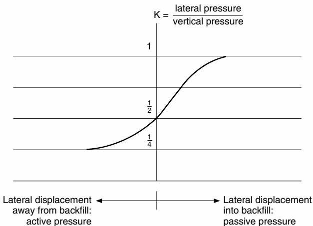
FIGURE 8.9 Active and passive pressures on restrained walls.
