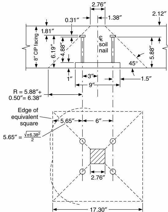
FIGURE 8.62 Bearing plate for soil nailed wall showing effective stress area for embedment design capacity. (From J. W. Keeley, Soil Nail Wall Facing: Sample Design Calculations, Federal Highway Administration, 1993, with permission)
