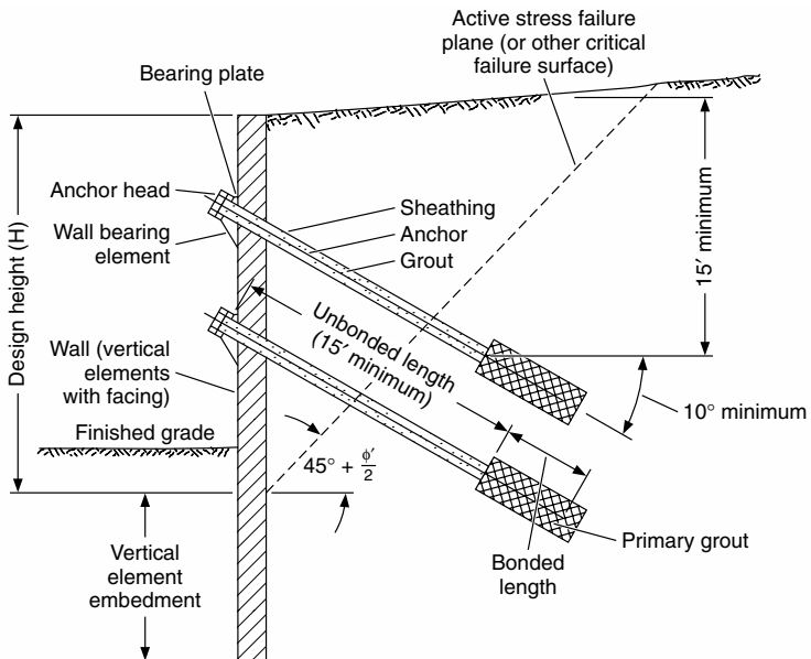
FIGURE 8.52 Terms used in flexible anchored wall design. (From Standard Specifications for Highway Bridges, 1996, and Interim Specifications, 1997–2000 , American Association of State Highway and Transportation Officials, Washington, D.C., with permission)
