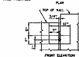
STRAIGHT JOINT USE WALL BRACKETS ON STRAIGHT PANEL JOINTS ONLY WHEN WALL RETAINS EARTH
