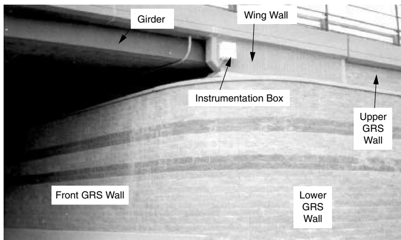
FIGURE 8.64 View of southeast side of the Founders/Meadows bridge abutment. (From Research Report, Colorado Department of Transportation, Denver, Colo., with permission)
