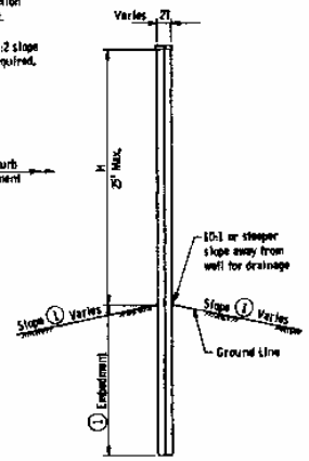
SECTION A-A WITHOUT EARTH FILL
