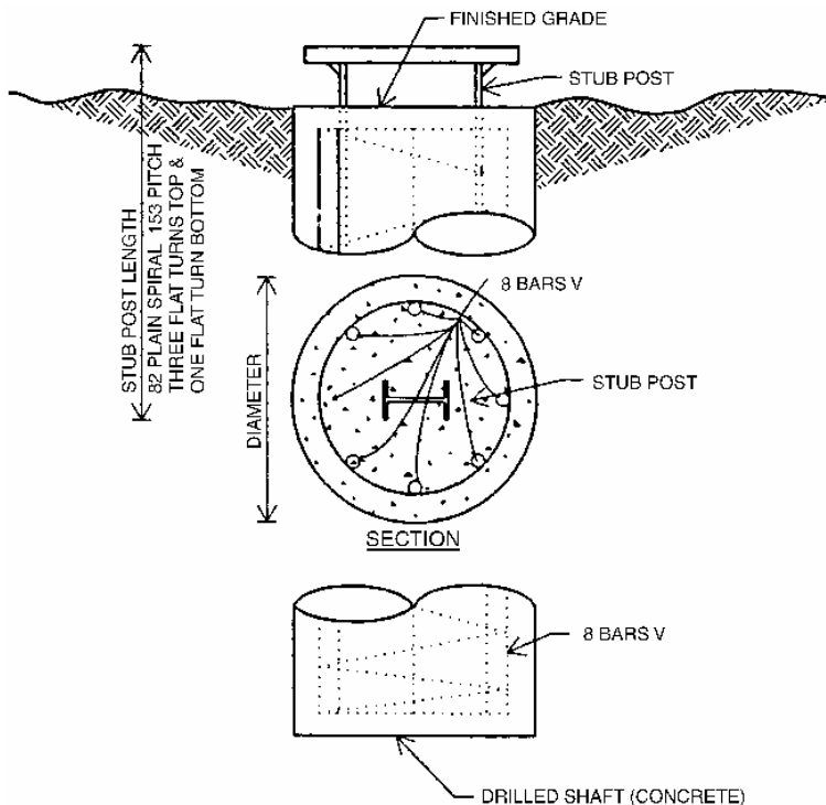
FIGURE 7.66 Horizontal base and concrete foundation detail.
