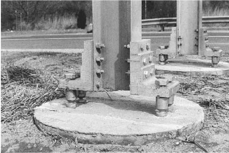
FIGURE 7.37 Base with load concentration couplers.
