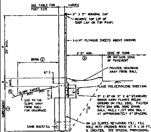
SECTION AT POST WITH EARTH FILL
