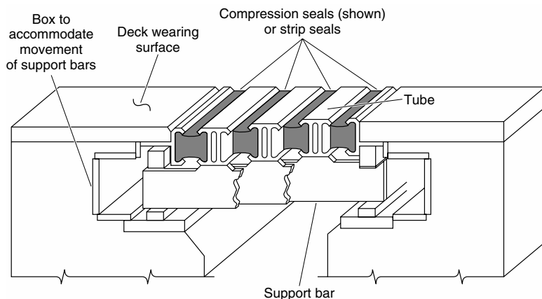
FIGURE 4.6 Cutaway view of modular expansion joint seal.
