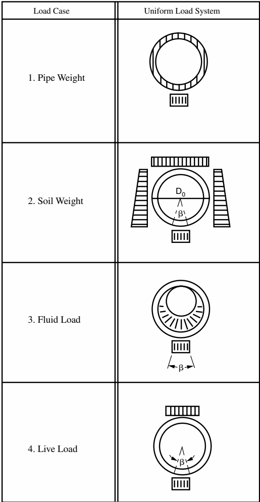
FIGURE 5.39 Pressure distributions for four load cases used in design of round concrete pipe. (From Concrete Pipe Technology Handbook, American Concrete Pipe Association, 1994, with permission)
