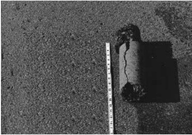
FIGURE 3.41 Pavement core taken at transverse joint in composite pavement.
