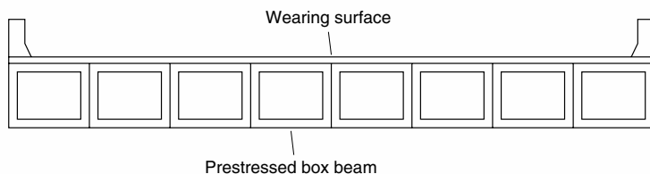
FIGURE 4.8 Cross section of prestressed-concrete box-beam bridge.
