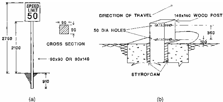
FIGURE 7.14 Typical installation of wooden sign supports. (a) Direct burial. (b) In concrete. Dimensions shown as mm. Conversions: 50 mm = 2 in, 100 mm = 4 in, 140 mm = 6 in, 360 mm = 14 in, 910 mm = 3 ft, 2100 mm = 7 ft, 2750 mm = 9 ft.
