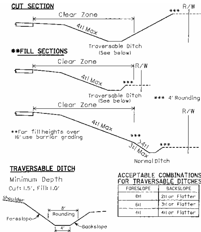
FIGURE 2.18 Examples of clear zone grading and traversable ditches. (From Location and Design Manual, Vol. 1, Roadway Design, Ohio Department of Transportation, with permission)
