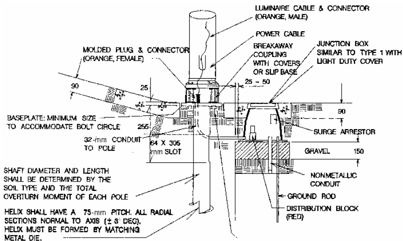
FIGURE 7.85 Auger base luminaire foundation system with underground modular cable distribution system. Dimensions shown as mm. Conversions: 25 mm = 1 in, 32 mm = 1.25 in, 50 mm = 2 in, 64 mm = 2.5 in, 75 mm = 3 in, 90 mm = 3.5 in, 150 mm = 6 in, 255 mm = 10 in, 305 mm = 12 in.
