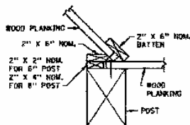
NAILING BOARDS AND CORNER BATTEN SELECTION TABLE FOR ANGLE TURNS TOWARD POST
