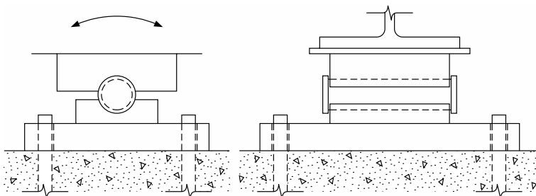
FIGURE 4.15 Fixed-pin bearing for structural steel.
