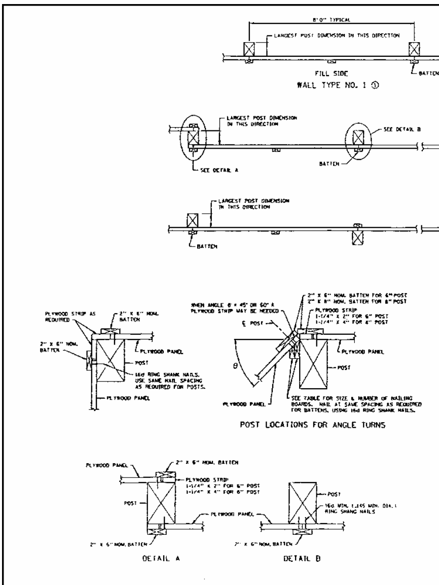
FIGURE 9.15 Typical design for noise walls using wood posts and horizontal tongue-and-groove plywood panels. (Adapted from Minnesota DOT design standards)
