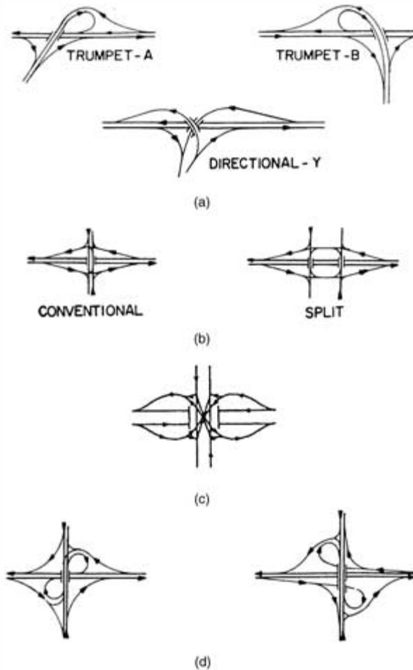
FIGURE 2.39 Common types of interchanges. (a) T and Y. (b) Diamond. (c) Single-point urban. (d) Partial cloverleaf. (From A Policy on Geometric Design of Highways and Streets , American Association of State Highway and Transportation Officials, 2001, with permission)
