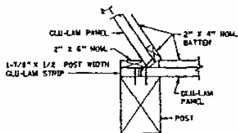
WALL TYPE NO. 3 ①②
