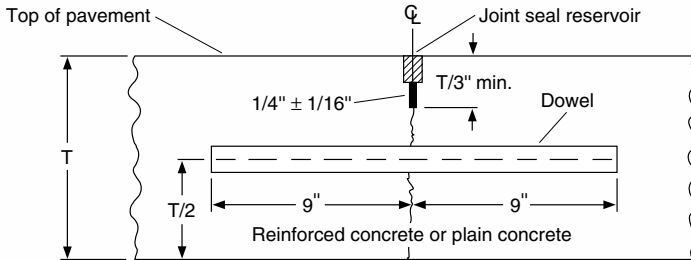
FIGURE 3.1 Typical contraction joint in rigid pavement with dowel for positive load transfer.
