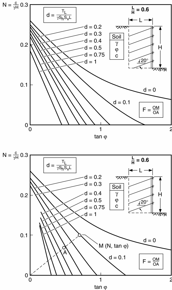
FIGURE 8.58 Preliminary design charts for soil nailed walls. (From Recommendations Clouterre, French National Research, 1991, translation by Federal Highway Administration, 1993, with permission)
