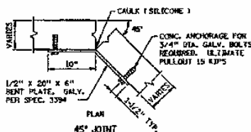
WALL BRACKET DETAILS
