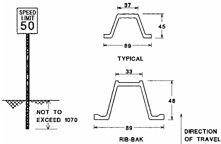
FIGURE 7.9 Installation and cross section of typical steel U-channel and RIB-BAK 3-lb/ft (4.5-kg/m) posts. Dimensions shown as mm. Conversions: 33 mm = 1 \frac{1}{8} in, 37 mm = 1 \frac{3}{8} in, 45 mm = 1 \frac{3}{4} in, 89 mm = 3 \frac{5}{8} in, 1070 mm = 42 in.
