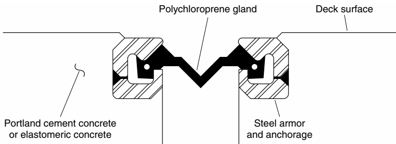
FIGURE 4.5 Cross section of strip seal.
