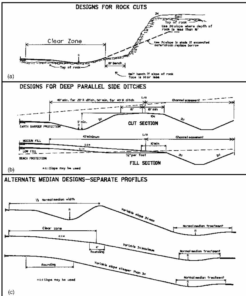
FIGURE 2.20 Examples of special designs for grading. (a) Designs for rock cuts. (b) Designs for deep, parallel side ditches. (c) Alternate median designs. (From Location and Design Manual, Vol. I, Roadway Design, Ohio Department of Transportation, with permission)
