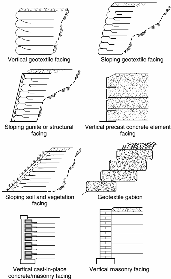
FIGURE 8.25 Facings for geotextile-reinforced walls.
