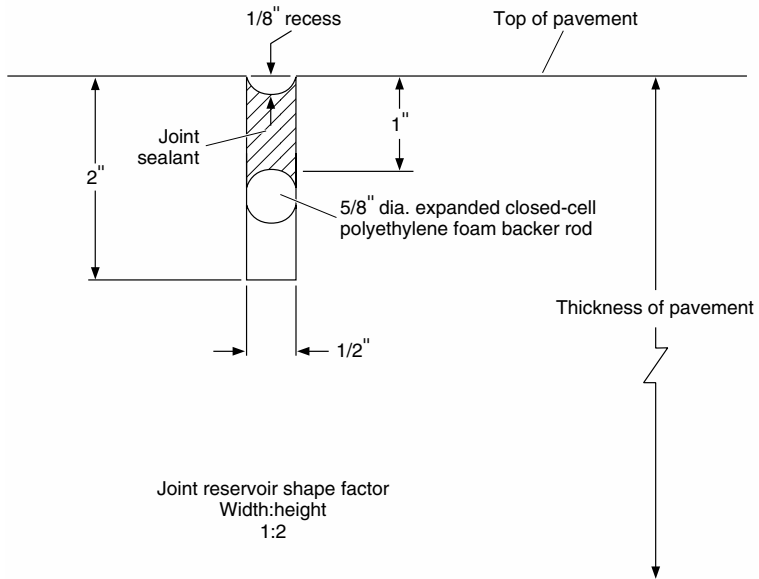
FIGURE 3.6 Typical field-formed joint seal in rigid pavement.
