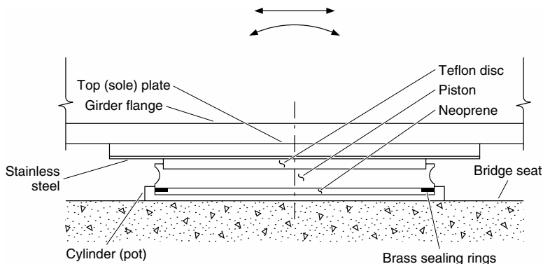
FIGURE 4.17 Pot bearing for structural steel or concrete.
