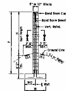
TYP. SECTION THRU WALL See tables for Additional Information
