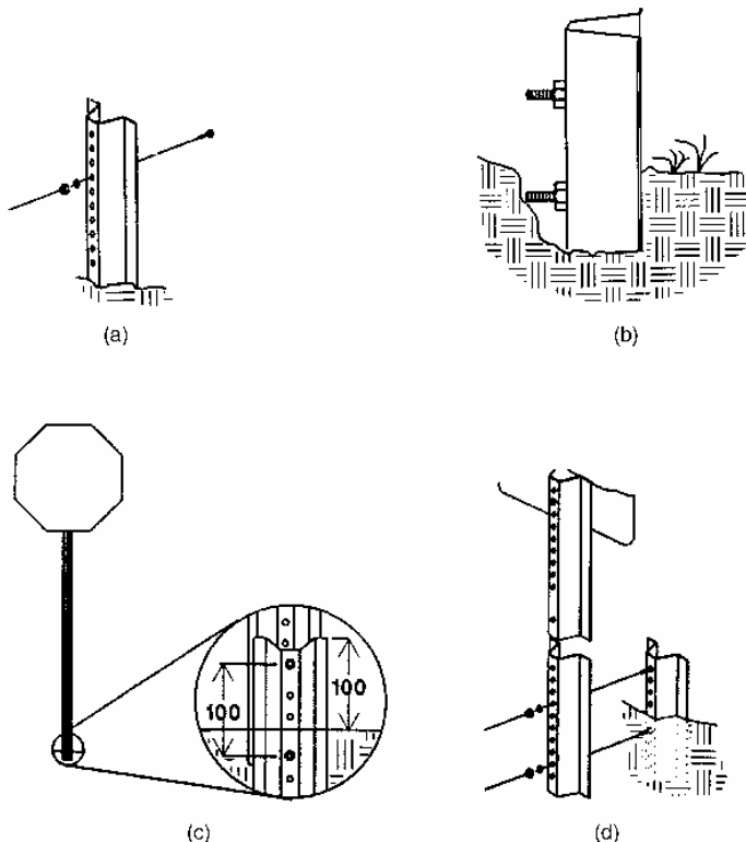
FIGURE 7.45 Generic method of splicing sign support to anchor piece. (a) Drive anchor post to within approximately 12 in (300 mm) from top of ground and install bolt with lock washer in fifth hole from top. (b) Drive post to 4 in (100 mm) or less from ground, and install bolt in first hole from back of post to allow room for sign post to be attached. (c) Install bolts 4 in (100 mm) apart with ground stub no higher than 4 in (100 mm) above ground. (d) Place signpost behind anchor stub, place bolts through first and fifth hole of sign post, use cut washers, and tighten securely.
