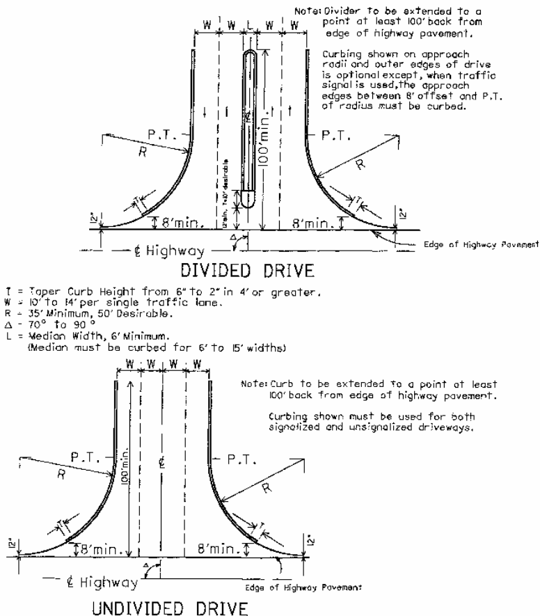
FIGURE 2.57 Designs for shopping center and industrial drives. (From Location and Design Manual, Vol. I, Roadway Design, Ohio Department of Transportation, with permission)
