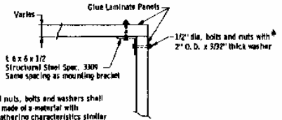
ANGLE TURN DETAILS
