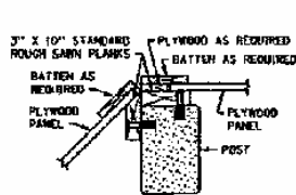
POST LOCATIONS FOR ANGLE TURNS
