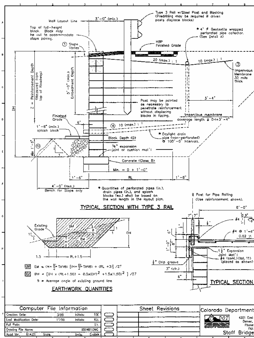
FIGURE 8.45a Worksheet for block facing MSE walls with post and W-beam barrier, showing geometry and design assumptions. (From Bridge Design Work Sheets, Colorado Department of Transportation, Denver, Colo., with permission)
