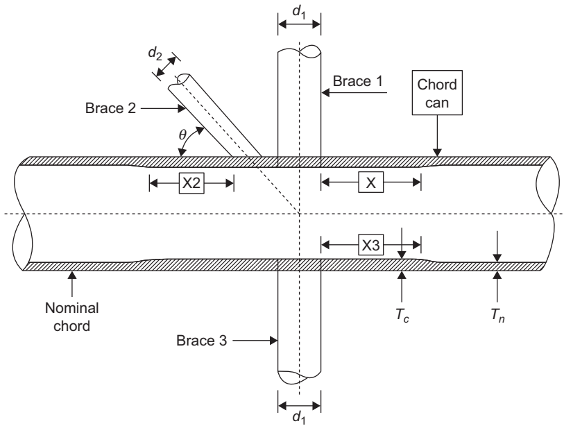
FIGURE 3.32 Chord length, L_{\text{ch}} .
