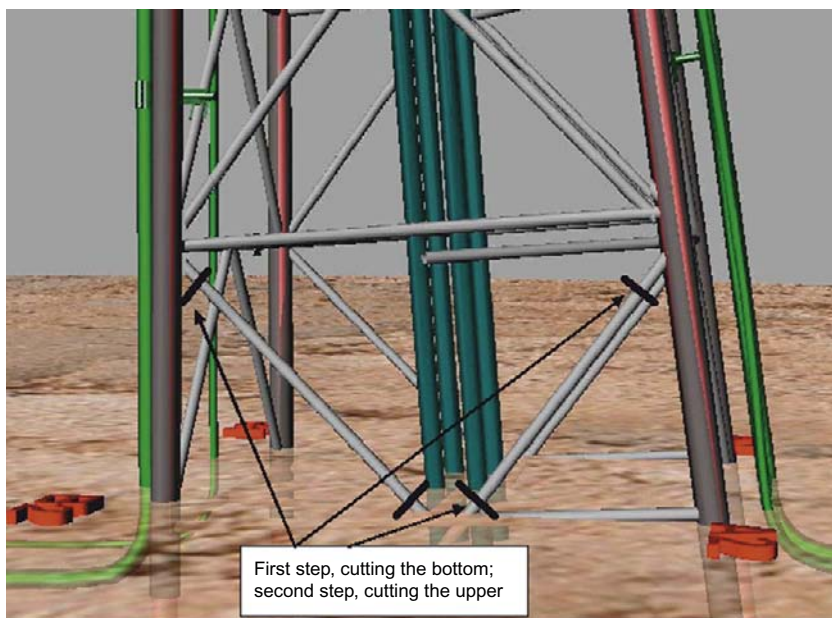
FIGURE 7.25 Locations for cutting the bracing.
