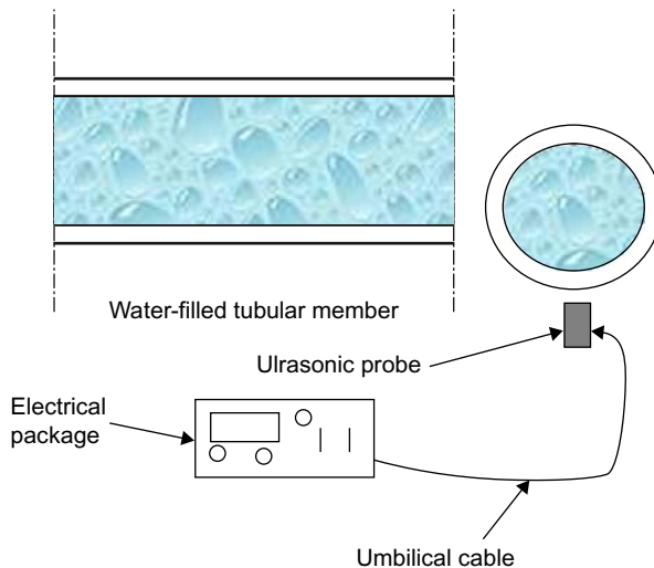
FIGURE 8.7 Typical arrangement of UT FMD equipment.
