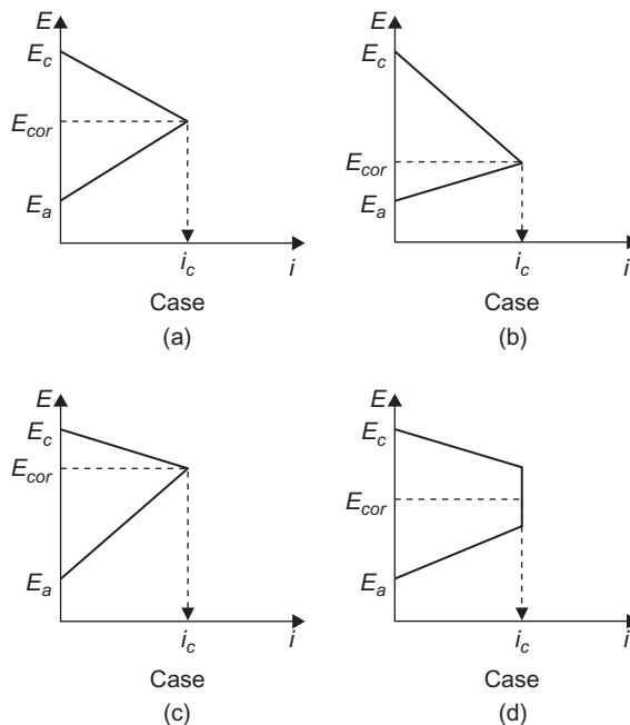
FIGURE 6.2 Evans diagrams.
