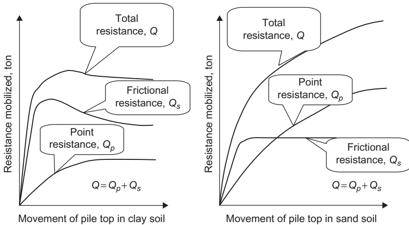
FIGURE 4.7 Typical load-movement characteristics of an axially loaded pile.
