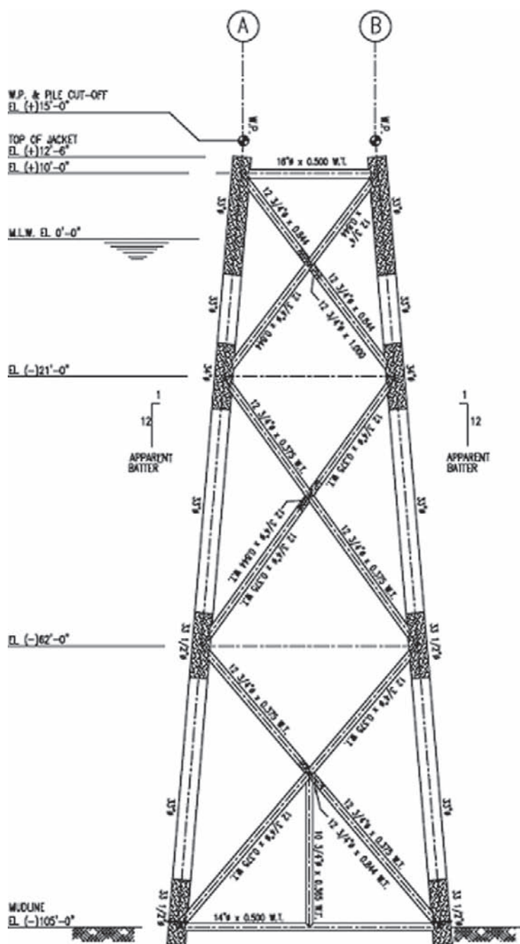
FIGURE 3.3 (a) Jacket view; (b) another view of the jacket.
