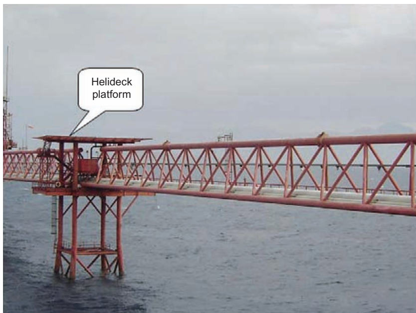
FIGURE 1.5 Bridges connecting a helideck platform.
