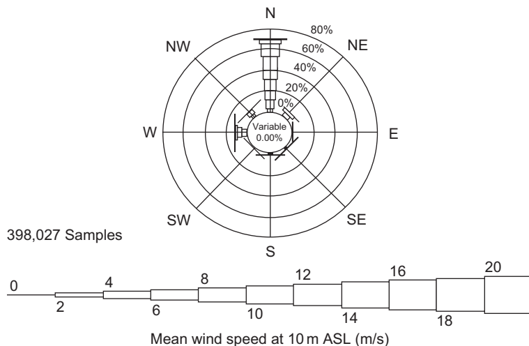
FIGURE 2.1 Example of wind at a location in the Gulf of Suez in the Red Sea (GoS).
