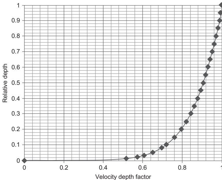
FIGURE 2.10 Current profile.
