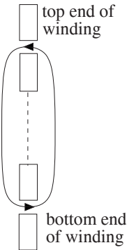
Figure 4.19 Axially placed parallel conductors in a winding.
