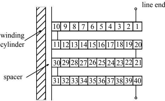
Figure 7.5 Continuous winding.
