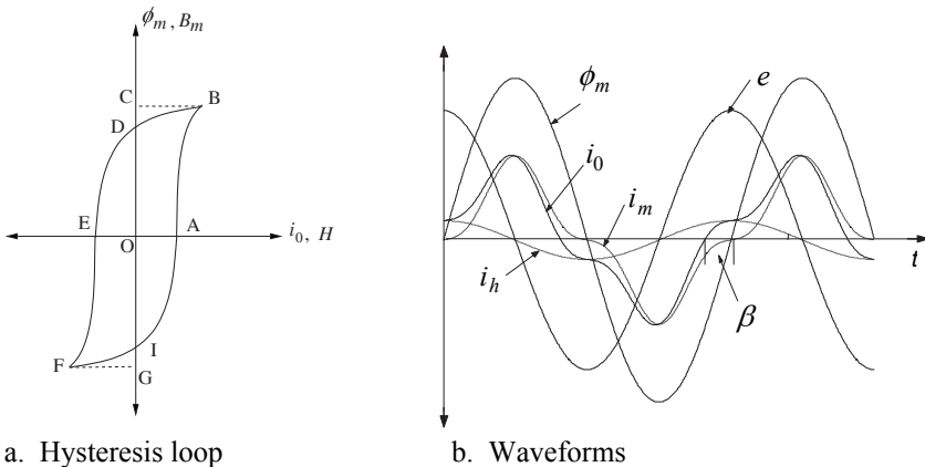
Figure 2.5 Hysteresis loss.
