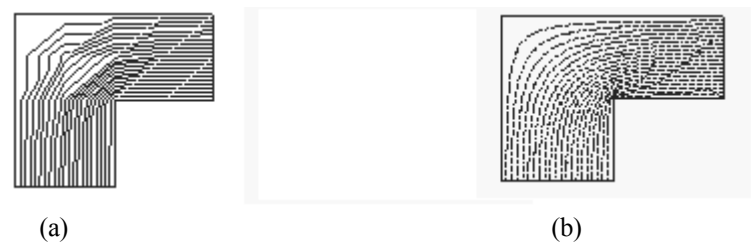
Figure 12.13 (a) Equipotential ( A ) lines for the coarse mesh of Figure 12.11. (b) Equipotential ( A ) lines for a dense mesh.
