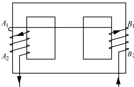
Figure 5.37 Compensating turns.
