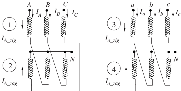
Figure 3.20 Zigzag/zigzag transformer.
