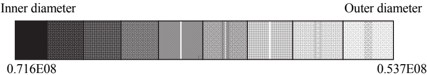
Figure 12.21 von-Mises stress distribution at 10.44 MPa pressure [50].
