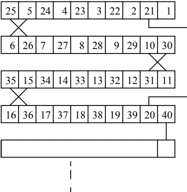
Figure 7.23 Four-disk interleaving.
