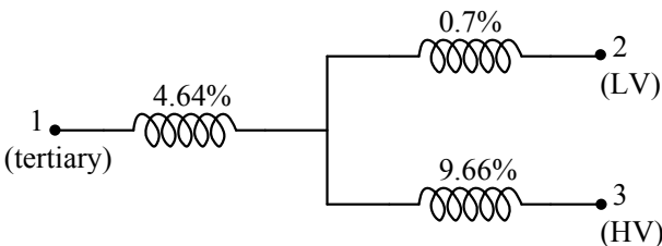
Figure 3.28 Zero-sequence star equivalent circuit.
