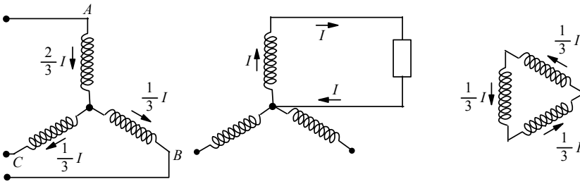
Figure 3.29 Unbalanced load.
