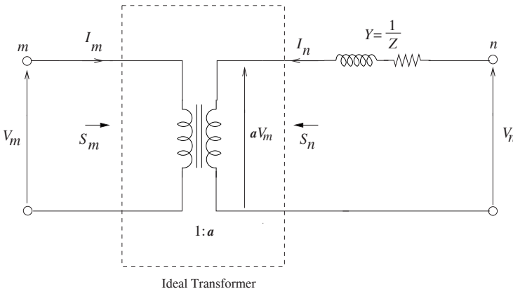
Figure 13.4 Regulating transformers.
