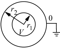
Figure 8.2 Concentric cylindrical electrodes.
