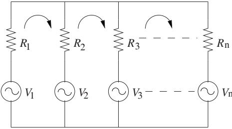
Figure 4.18 Equivalent circuit for calculation of circulating currents.
