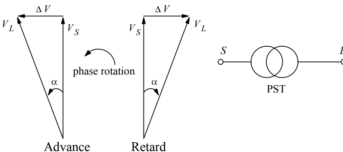
Figure 11.11 Advance mode and retard mode.
