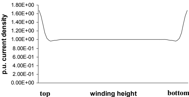
Figure 4.11 Eddy current distribution in a foil winding.
