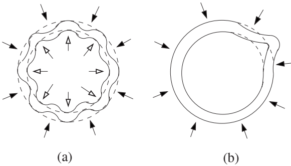
Figure 6.11 Buckling phenomena.
