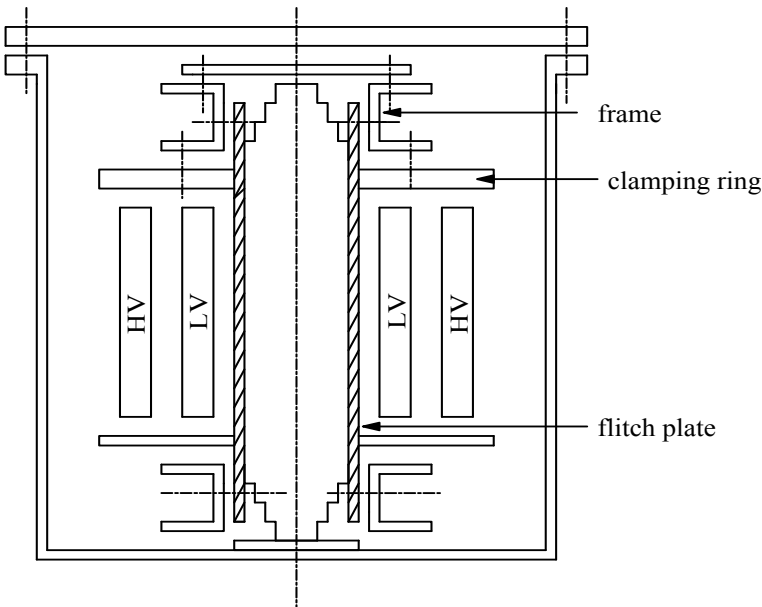
Figure 6.19 Clamping elements.
