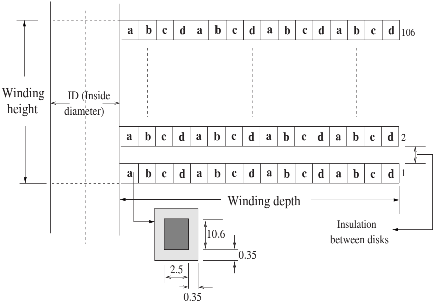
Figure A.1 LV winding details.
