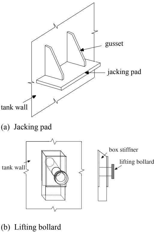
Figure 10.1 Jacking pad and lifting bollard.
