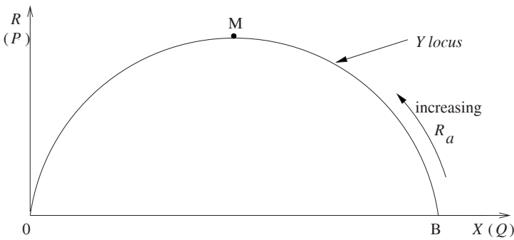
Figure 13.7 Circle diagram [18].
