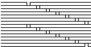
Step-lap joint
