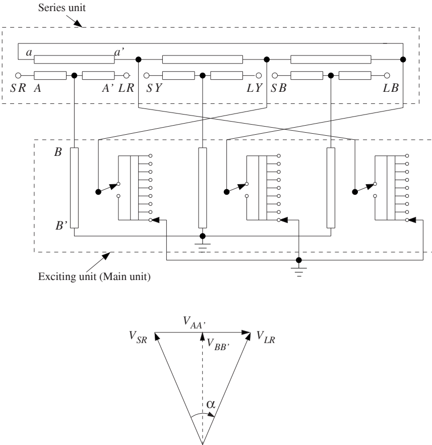
Figure 11.14 Commonly used configuration for two-core design PST.
