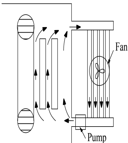
Figure 9.3 OFAF cooling.
