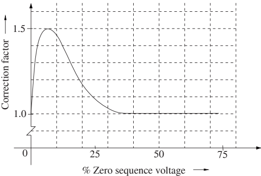
Figure 3.22 Correction factor for the zero-sequence reactance [16].
