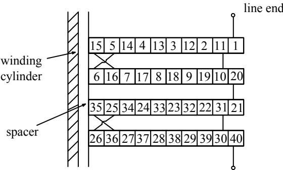
Figure 7.6 Interleaved winding.
