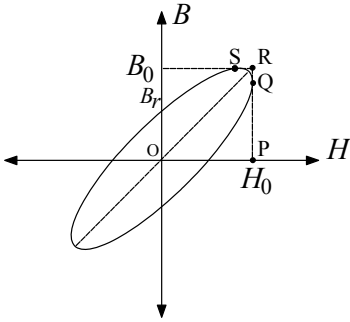
Figure 4.2 Elliptic hysteresis loop.
