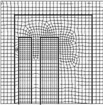
Figure 3.9 FEM mesh.
