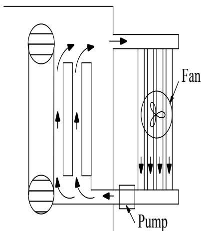
Figure 9.4 ODAF cooling.
