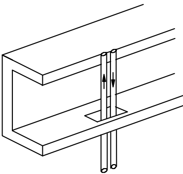
Figure 5.6 Go-and-return arrangement. Figure 5.7 Nonmagnetic insert.
