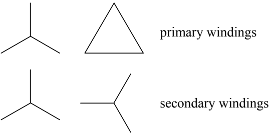
Figure 11.3 Twelve-pulse operation.
