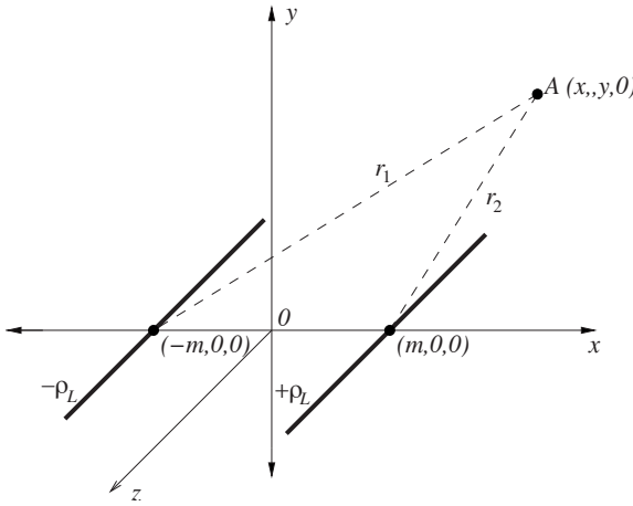
Figure D.1 Two line charges placed at x = -m and x = +m .
