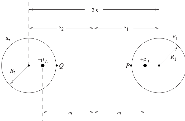
Figure D.2 Configuration of two parallel cylindrical conductors.
