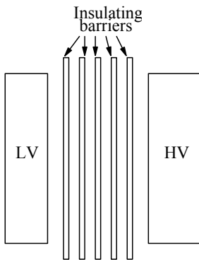
Figure 8.12 Subdivided duct between LV and HV windings.
