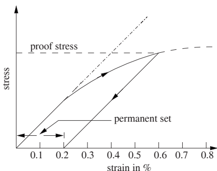
Figure 6.10 0.2% proof stress.
