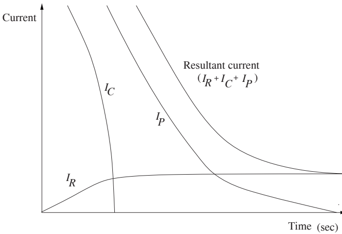
Figure 14.8 Currents components during PI test.
