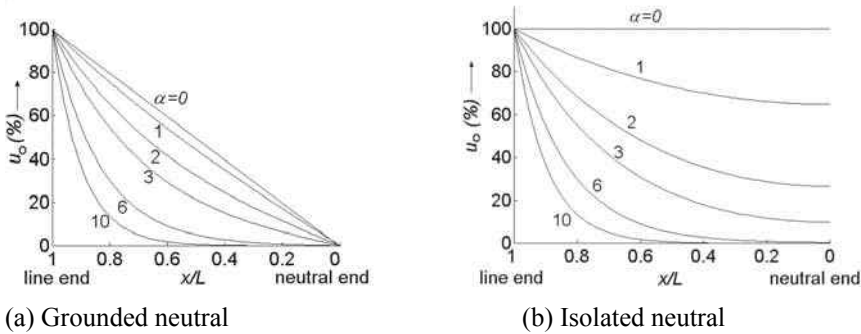
Figure 7.3 Initial voltage distribution.
