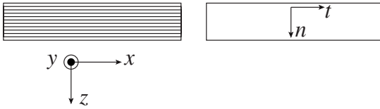
Figure 5.31 Anisotropic permeability.
