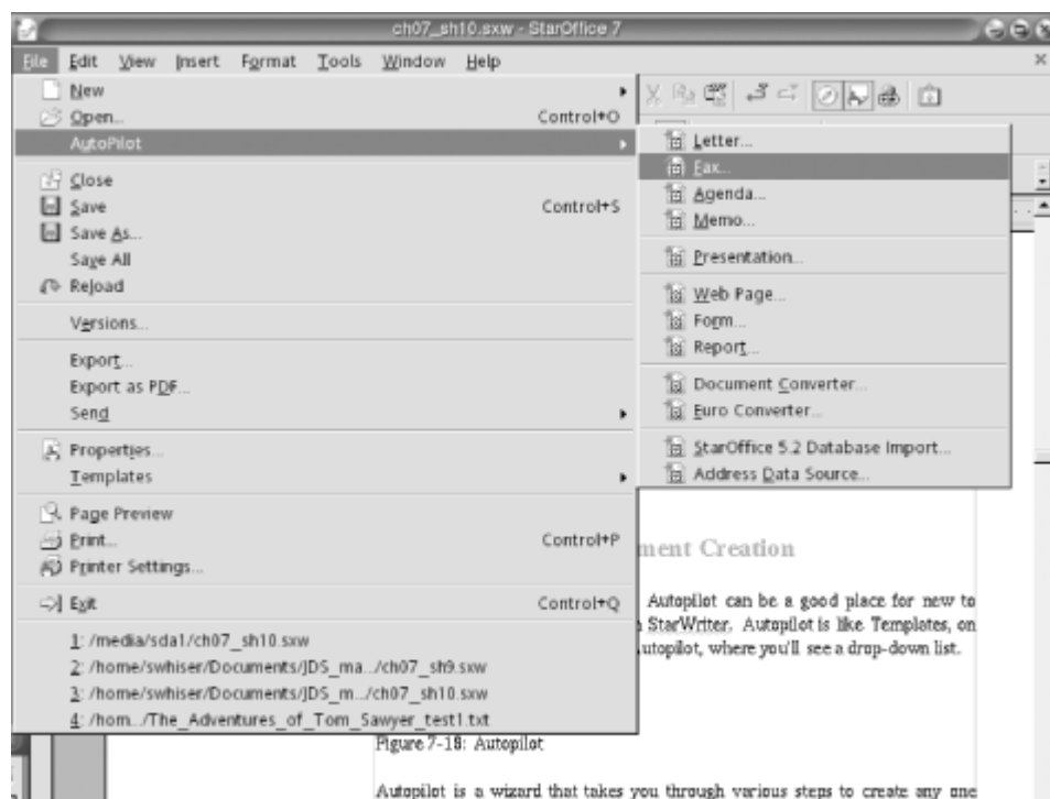
Figure 7-37. The Autopilot
