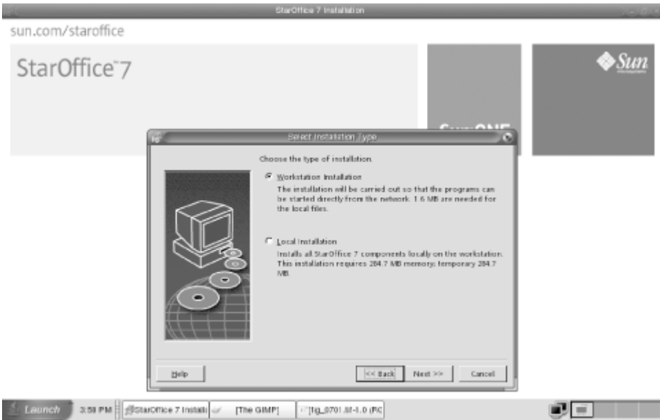
Figure 7-54. Installation type
