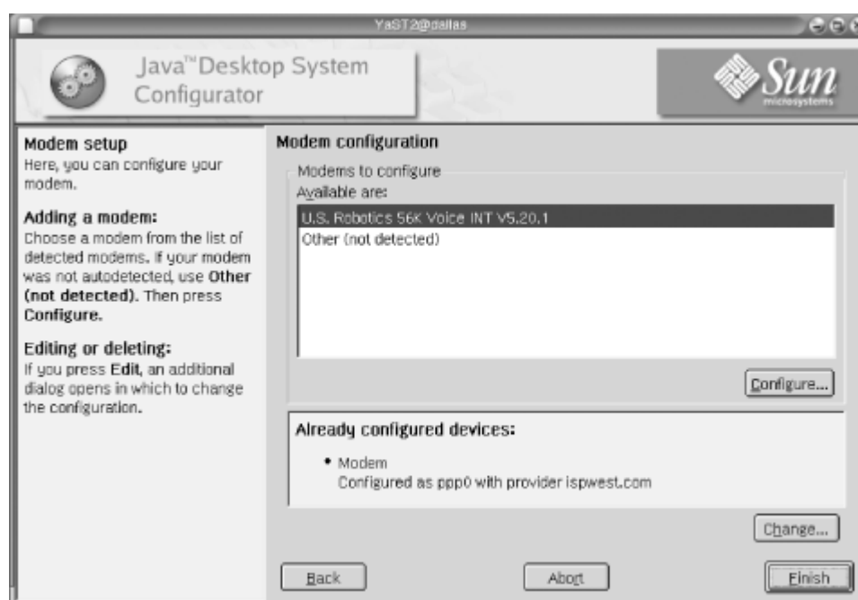
Figure 4-3. Modem autodetected
