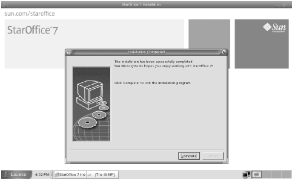
Figure 7-58. Installation completed
