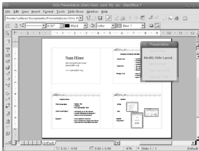
Figure 8-46. Handout View
