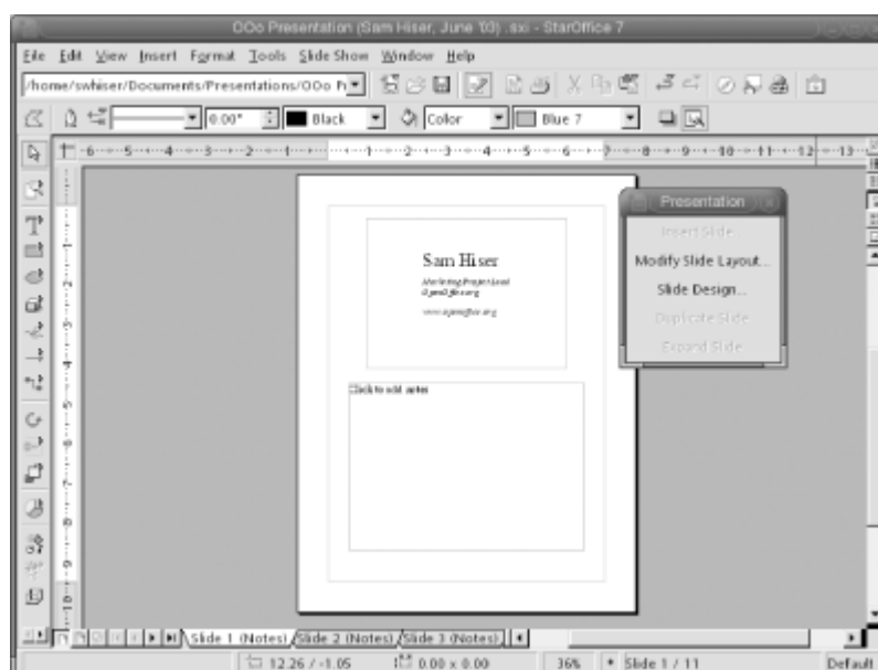
Figure 8-45. Notes View
