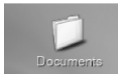
Figure 1-3. Documents icon
