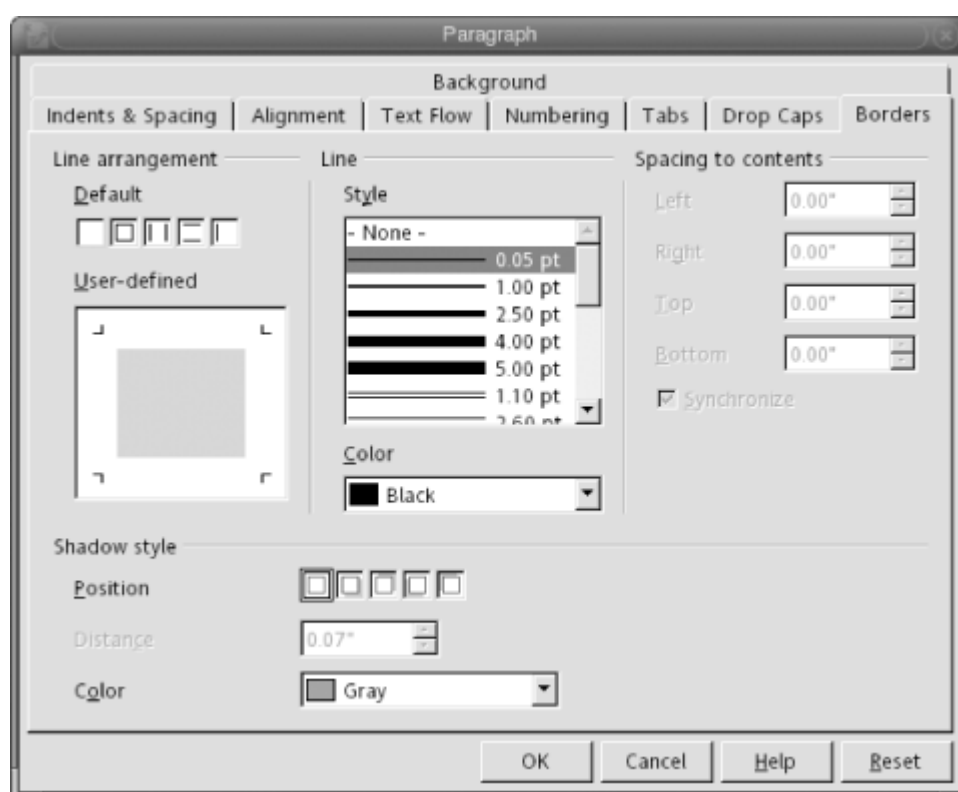
Figure 7-8. Paragraph window
