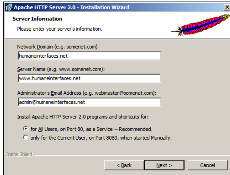
Figure A.1: Installing Apache 2.0
