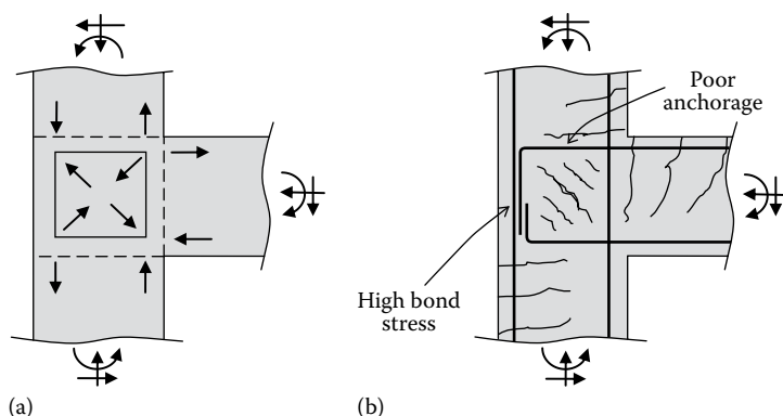
Figure 14.46 Three-member connection. (a) Internal forces. (b) Crack pattern.
