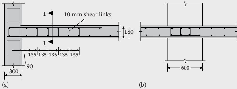
Figure 7.27 Sections through slab–column connection (Example 7.5). (a) Section perpendicular to slab edge. (b) Section I–I.
