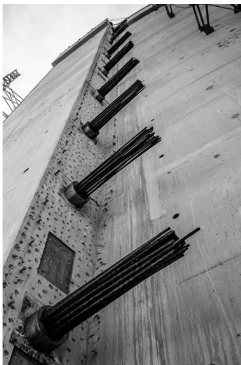
Figure 3.13 Prestressing anchorages at a buttress of a prestressed tank. (Courtesy of VSL International Limited, Hong Kong, China.)
