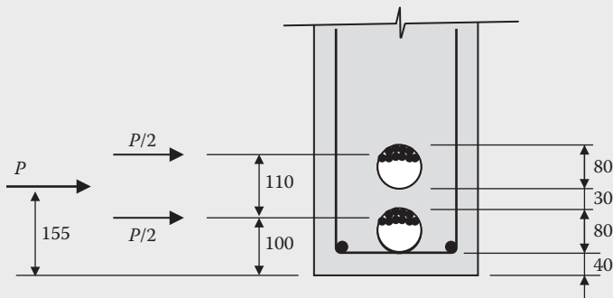
Figure 10.4 Cable locations and relevant dimensions at mid-span.
