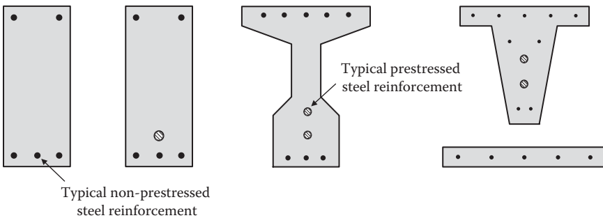
Figure 5.4 Typical reinforced and prestressed concrete sections.
