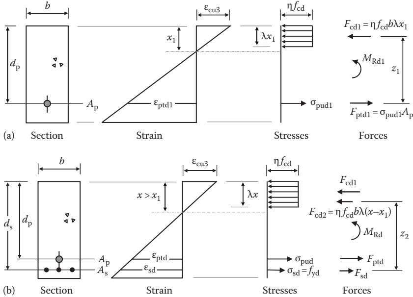
Figure 6.11 Cross-section containing tensile reinforcement – ultimate design condition. (a) Singly reinforced prestressed cross-section. (b) Cross-section containing both prestressed and non-prestressed tensile reinforcement.
