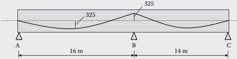
Figure 11.21 Two-span beam (Example 11.6).
