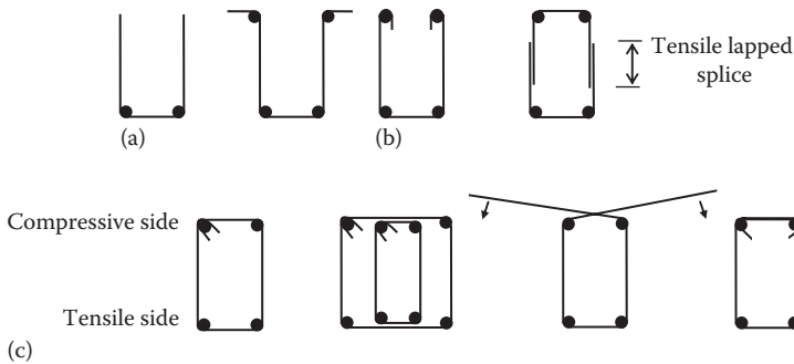
Figure 14.27 Stirrup shapes. (a) Incorrect. (b) Satisfactory in some situations. (c) Desirable.
