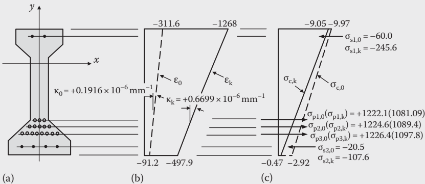
Figure 5.15 Strains and stresses at times t_0 and t_k (Example 5.6). (a) Cross-section. (b) Strain ( \times 10^{-6} ). (c) Stress (MPa).
