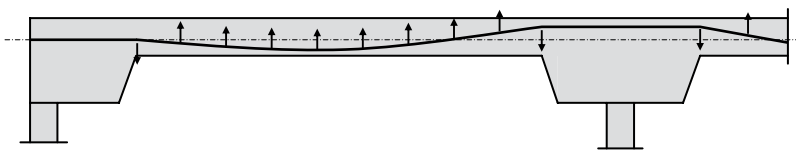
Figure 12.26 Band-beam and slab floor system.
