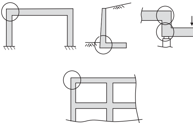
Figure 14.39 Two-member connections.
