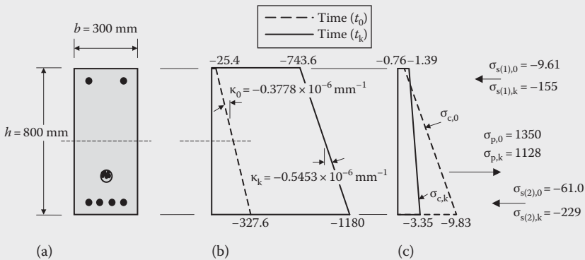
Figure 5.14 Strains and stresses at times t_0 and t_k (Example 5.5). (a) Section. (b) Strain ( \times 10^{-6} ). (c) Stress (MPa).
