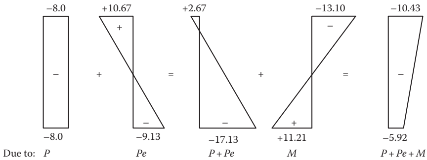
Figure 1.14 Component stress distributions in introductory example.
