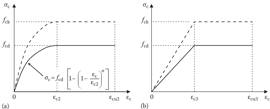
Figure 6.2 Idealised stress blocks for concrete in compression. (a) Parabola–rectangle diagram. (b) Bilinear diagram.
