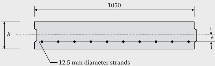
Figure 10.11 Cross-section of pretension plank (Example 10.2).
