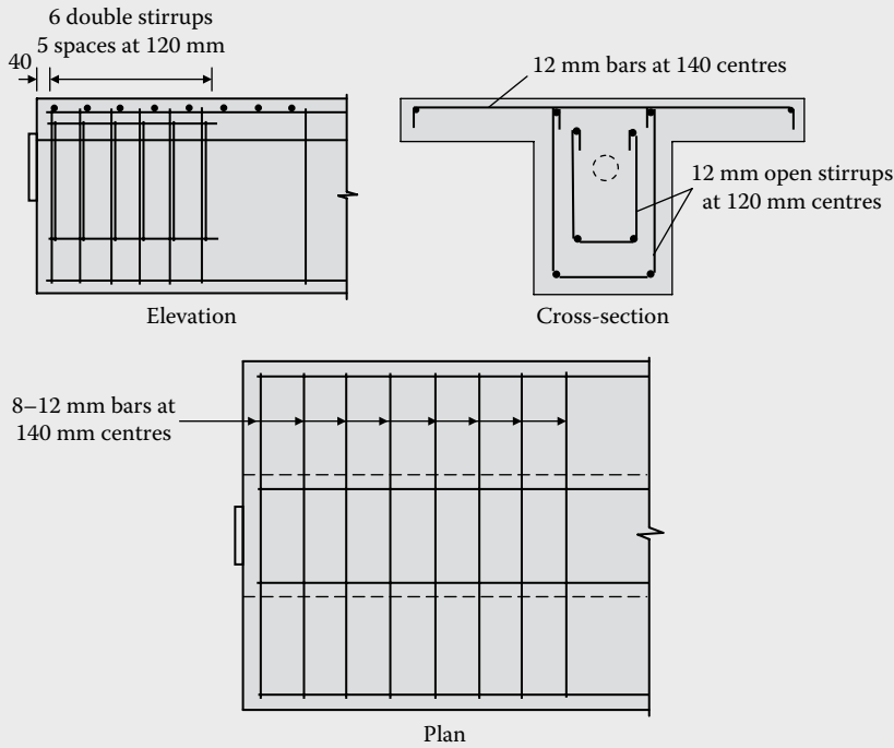
Figure 8.25 Reinforcement details for anchorage zone of T-beam (Example 8.3).
