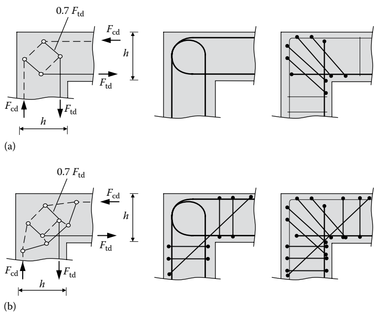
Figure 14.44 Strut-and-tie models and reinforcement details – opening bending [1]. (a) Moderate opening moment, A_s/bh \leq 0.02 . (b) Large opening moment, A_s/bh > 0.02 .
