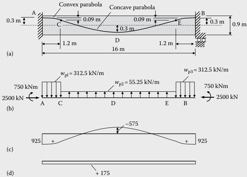
Figure 11.15 Fixed-end beam with curvilinear tendon profile (Example 11.3). (a) Elevation. (b) Equivalent loads. (c) Total moment diagram caused by prestress (kNm). (d) Secondary moment diagram (kNm).
