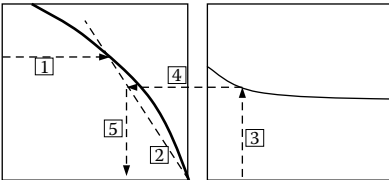
Figure 4.7 The final creep coefficient for concrete \varphi(\infty, t_0) under normal environmental conditions.
