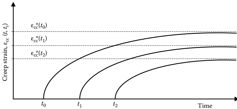
Figure 4.6 Effect of age at first loading on the creep coefficient.
