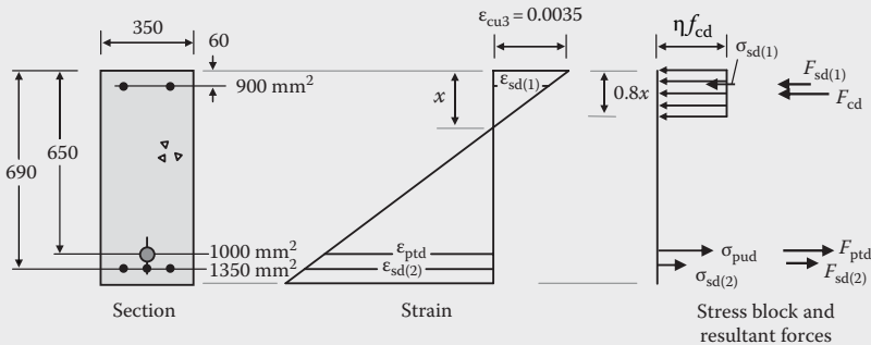
Figure 6.9 Section details and stress and strain distributions at the design ultimate moment condition (Example 6.3).
