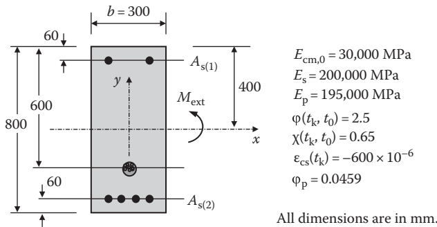
Figure 5.16 Post-tensioned cross section with tendon bonded after transfer.
