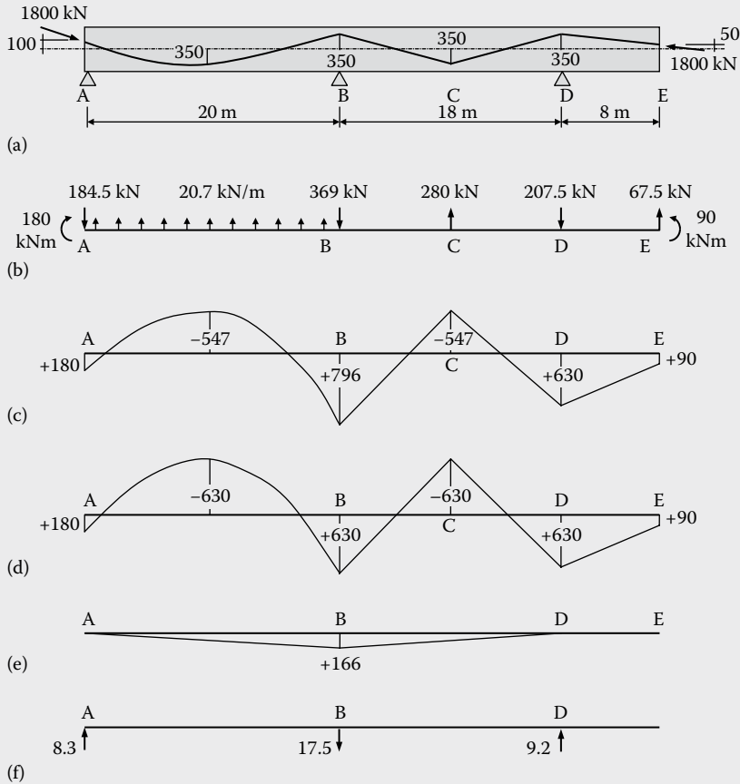
Figure 11.9 Equivalent loads and actions induced by prestress (Example 11.1).
