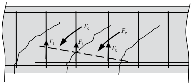
Figure 14.18 Anchorage of terminating bottom reinforcement.
