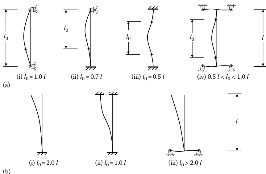
Figure 13.7 Effective lengths l_0 [2]. (a) Braced columns. (b) Unbraced columns.
