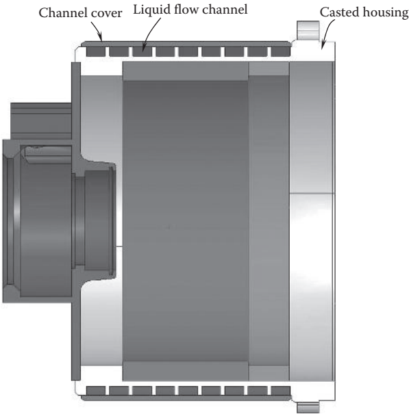
FIGURE 8.55 Liquid flow channels formed between the casted housing and the channel cover.
