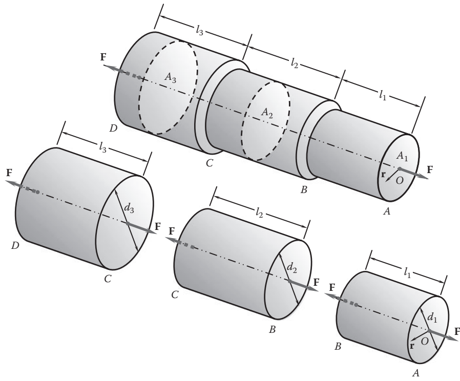
FIGURE 3.6 A stepped shaft subjected to an axial force.
