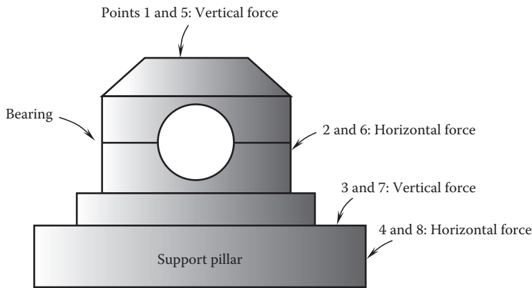
FIGURE 11.22 Using an instrumented hammer to excite the bearing support to obtain the natural frequency, damping, stiffness, and mass. Points 1 and 4 are taken on the south bearing, and points 5 and 8 are taken on the north bearing. Points 1, 3, 5, and 7 are vertical measurements, while points 2, 4, 6, and 8 are horizontal measurements.
