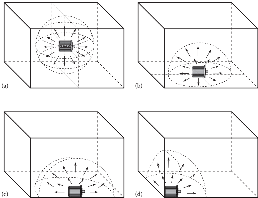
FIGURE 9.32 Directivity factor of the sound source for different source positions: (a) at room center, Q_0=1 ; (b) at the center of floor, Q_0=2 ; (c) at the center of floor edge, Q_0=4 ; and (d) at floor corner, Q_0=8 .
