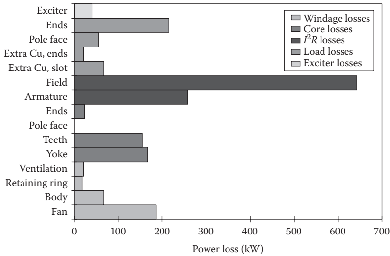
FIGURE 7.10 Various power losses for a high-power electric machine (machine A).
