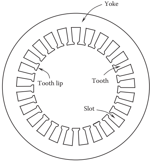
FIGURE 4.1 One-piece lamination is made by an undivided piece of steel sheet in full revolution. Stator slots are for receiving stator windings.
