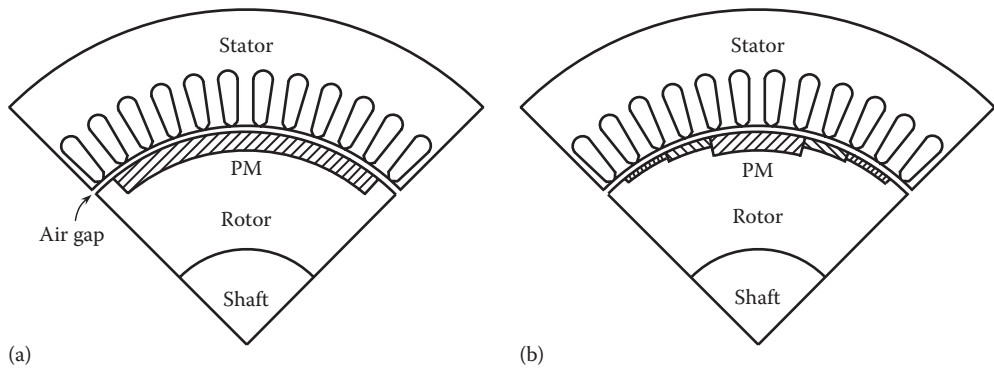
FIGURE 1.8 Rotors with surface-inset single PM (a) and stepped PMs (b).
