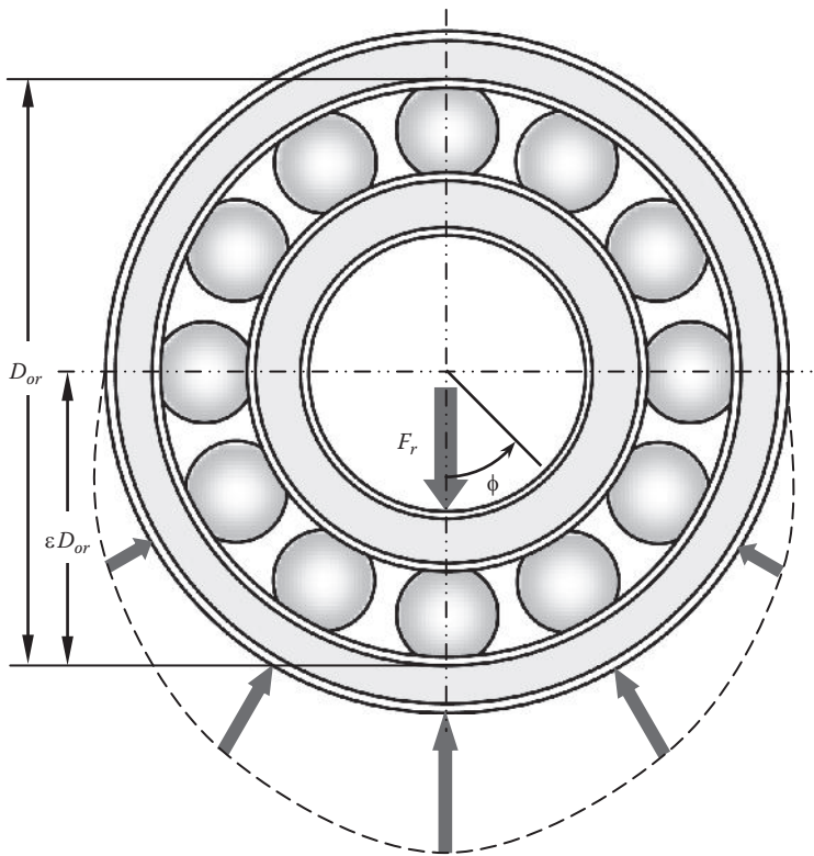
FIGURE 6.21 Load distribution of rolling bearing, \varepsilon = 0.5 in this case.
