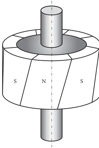
FIGURE 1.7 Skewed PMs on rotor core for reducing cogging torque.
