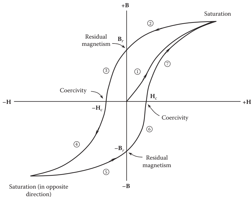
FIGURE 2.10 The magnetization hysteresis loop of a PM.
