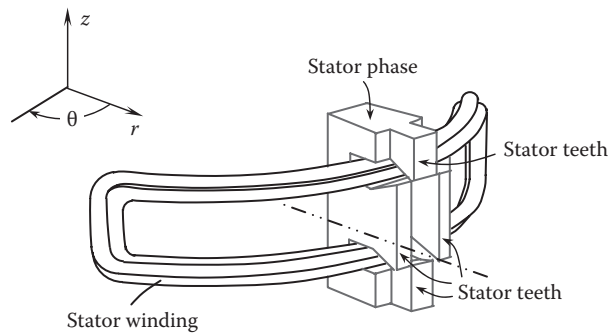
FIGURE 12.26 Single-stator winding and phase in an FC-TFM (European Patent 2,317,633) [12.31]. (Courtesy of the European Patent Office, Munich, Germany.)
