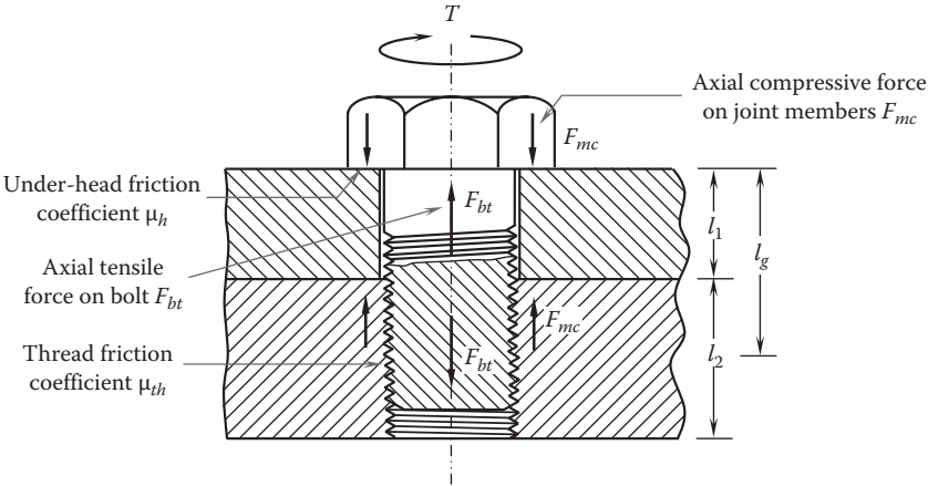
FIGURE 5.36 Screw-threaded member joint. Due to the elimination of a nut, the friction under nut-bearing surface no longer exists.
