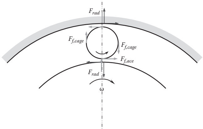
FIGURE 7.9 Bearing losses due to friction between balls and raceways, balls and the cage, and balls and the lubricant.
