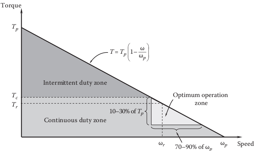
FIGURE 1.13 Torque–speed characteristics of a typical DC motor.
