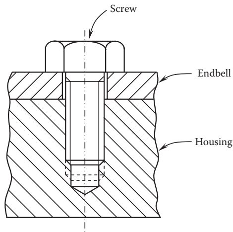
FIGURE 5.23 The motor housing is tapped for receiving short screws, which go through the endbell to complete the construct of the motor frame.
