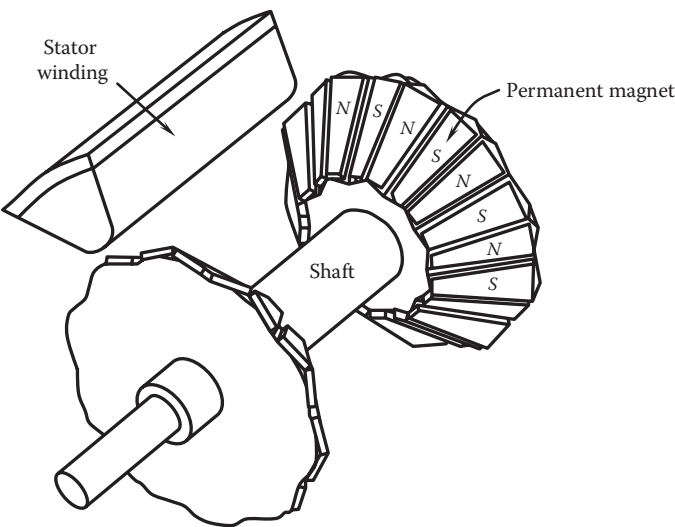
FIGURE 12.24 Conical rotor with PMs at two ends of the shaft and stator windings located between the PMs.
