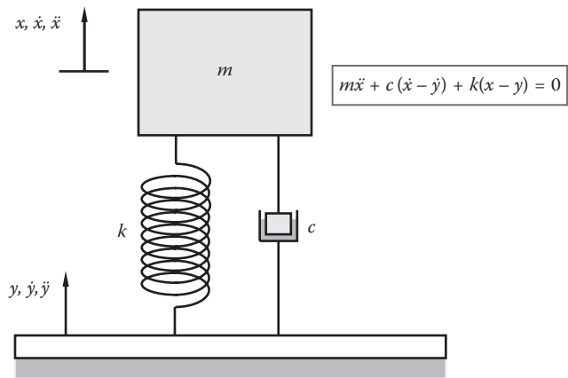
FIGURE 9.8 Vibration induced by support excitation in a two-degree-of-freedom mechanical system.
