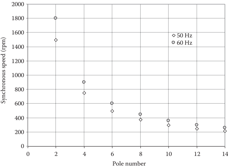
FIGURE 1.32 Synchronous speeds of 50 and 60 Hz machines under various pole numbers.
