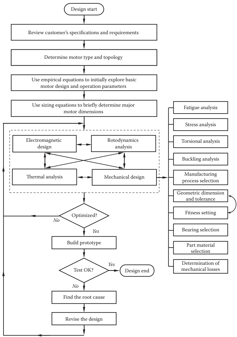
FIGURE 1.49 The flowchart of motor design.
