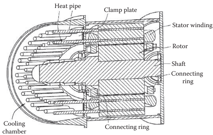
FIGURE 8.61 Cross-sectional view of motor cooling with heat pipes (U.S. Patent 7,569,955) [8.59]. (Courtesy of the U.S. Patent and Trademark Office, Alexandria, VA.)
