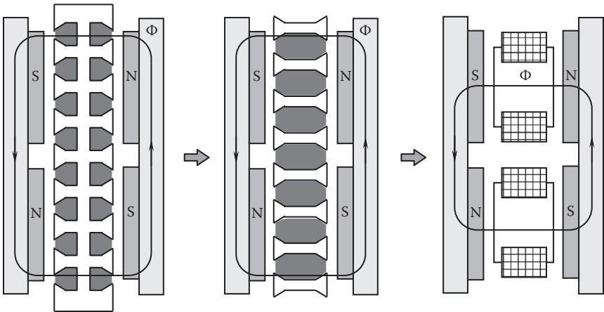
FIGURE 12.16 The topology of YASA motor, which combines two best-performing AF motors.
