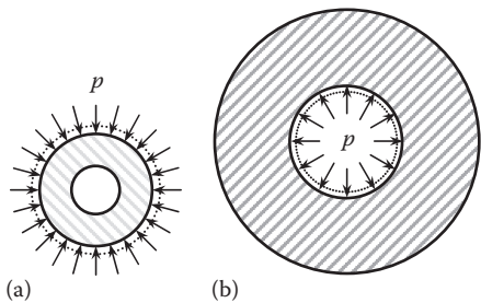
FIGURE 2.35 Contact pressure acting on (a) the hollow shaft and (b) the rotor core.
