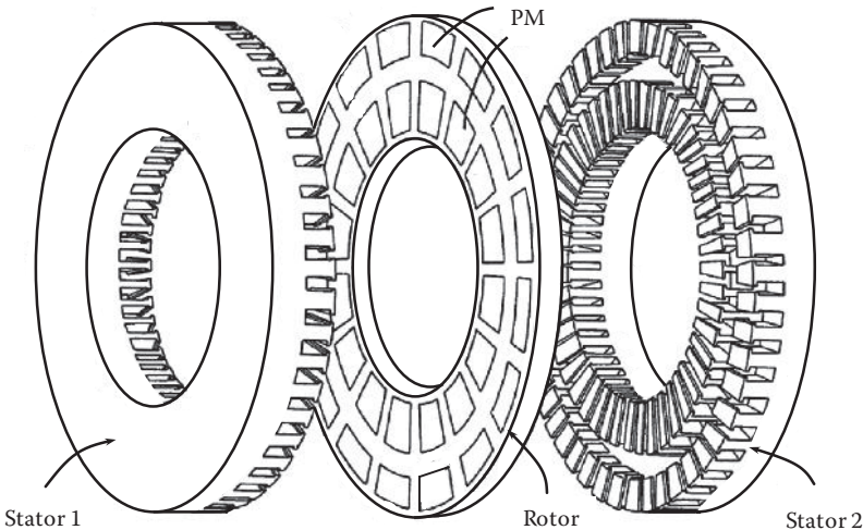
FIGURE 1.41 Brushless AF motor with the stator-rotor-stator structural topology, where PMs mounting on the rotor side surfaces and rotating with the rotor.
