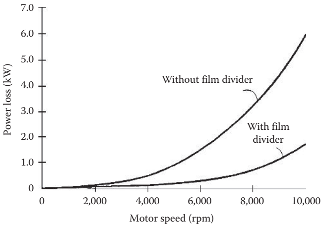
FIGURE 7.22 Comparison of windage power loss of motors with and without film divider in high-speed machine (U.S. Patent 5,828,148) [7.45]. (Courtesy of the U.S. Patent and Trademark Office, Alexandria, VA.)
