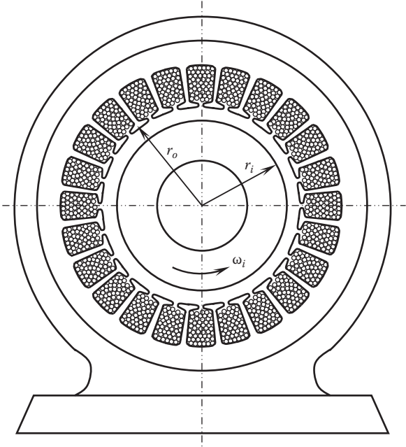
FIGURE 11.1 Schematic diagram of the formation of the air gap between the rotor and stator.
