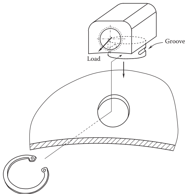
FIGURE 5.32 Cylinder-base faster, locked with a retaining ring at the grooves of the cylindrical base.
