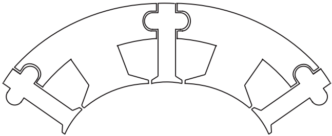
FIGURE 4.7 Alternative segmented stator laminations, showing each stator slot is formed between a large and a small segmented piece.
