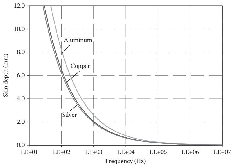
FIGURE 7.3 Variations of skin depth with frequency for different materials.
