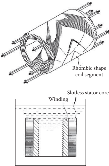
FIGURE 4.14 Fabrication of slotless stator (U.S. Patent 6,525,437) [4.12]. (Courtesy of the U.S. Patent and Trademark Office, Alexandria, VA.)
