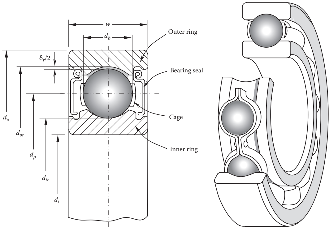
FIGURE 6.3 Deep-groove ball bearings (seals are removed from the right figure).
