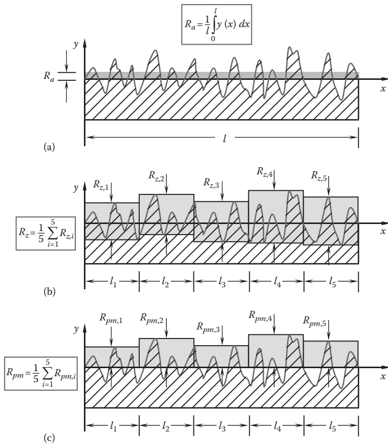
FIGURE 3.17 Three surface texture characteristic parameters: (a) average roughness R_a , (b) average peak-to-valley height R_z , and (c) average peak-to-mean R_{pm} .
