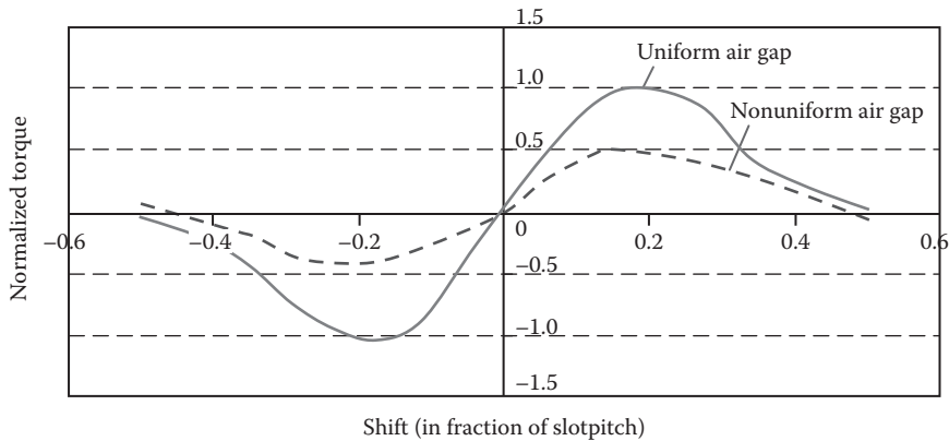
FIGURE 1.10 Comparison of cogging torque for uniform and nonuniform air gap (bread-loaf magnet shape).
