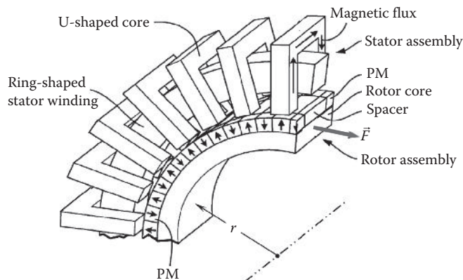
FIGURE 12.28 A partial perspective view of rotor and stator assembly of one-phase unit in a PM excited TF motor (U.S. Patent 8,299,669) [12.32]. (Courtesy of the U.S. Patent and Trademark Office, Alexandria, VA.)
