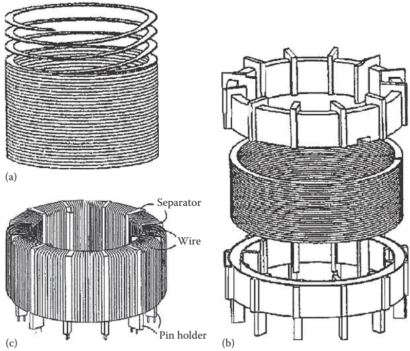
FIGURE 4.17 Using slinky method in designing slotless stator: (a) fabricating a helical stator core, (b) adding a molded plastic annular insulator at each end of the stator core, and (c) making the stator winding over the insulators (U.S. Patent Application 2005/0073210) [4.15]. (Courtesy of the U.S. Patent and Trademark Office, Alexandria, VA.)
