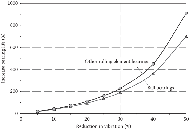
FIGURE 6.37 Impact of reduction in vibration level on bearing life.
