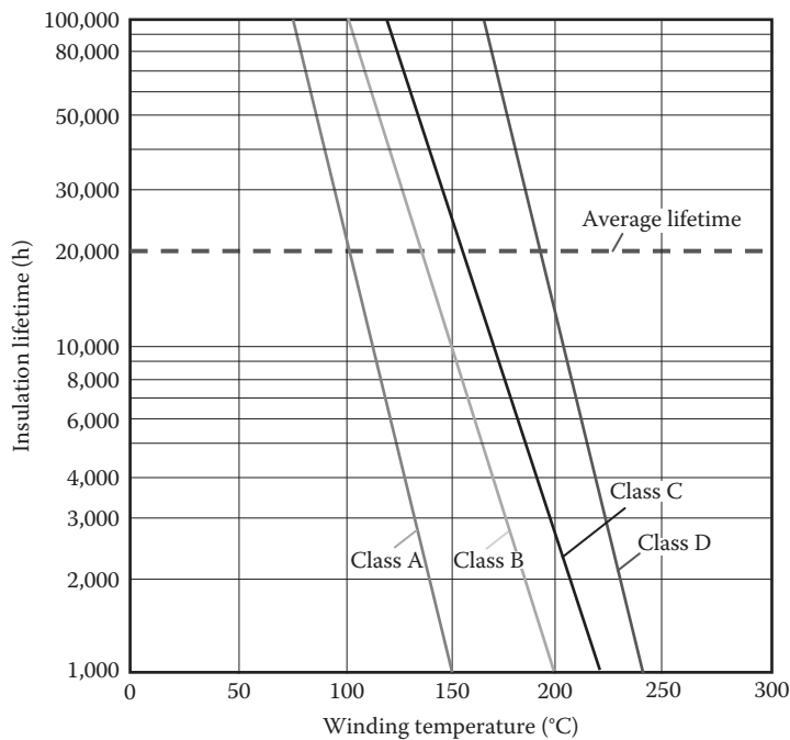
FIGURE 1.26 Thermal aging effect on lifetime of different insulation classes.
