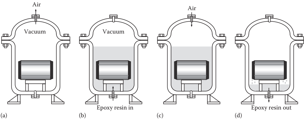
FIGURE 4.37 VPI process: (a) evacuating the container into deep vacuum, (b) introducing epoxy resin into the container until the stator is completely submerged, (c) releasing the vacuum of the container and applying pressure over the resin-covered stator to force resin completely into the stator, (d) draining epoxy resin out of the container, and (e) placing the stator into an oven and baking it for curing the epoxy resin (not shown).
