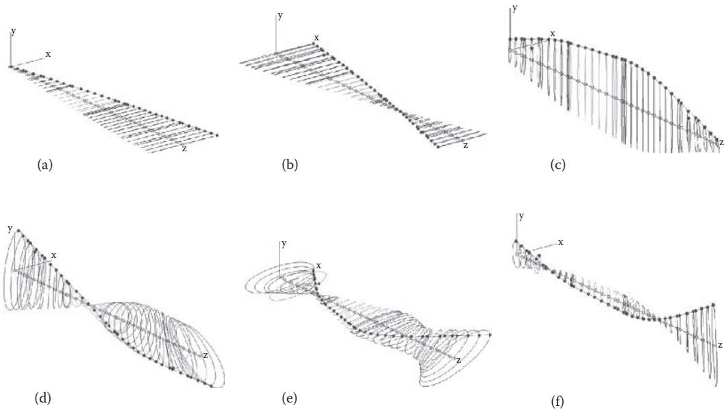
FIGURE 11.27 Damped critical-speed mode shapes: (a) mode 1 at 850 rpm; (b) mode 2 at 1527 rpm; (c) mode 3 at 2502 rpm; (d) mode 4 at 3915 rpm; (e) mode 5 at 4543 rpm; and (f) mode 6 at 5413 rpm.
