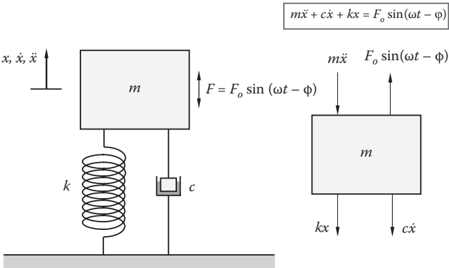
FIGURE 9.3 Forced vibration of single-degree-of-freedom system with damping.
