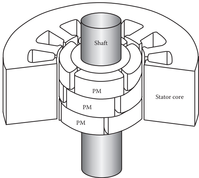
FIGURE 1.6 Step-skewed permanent magnets relative to stator teeth for reducing cogging torque.
