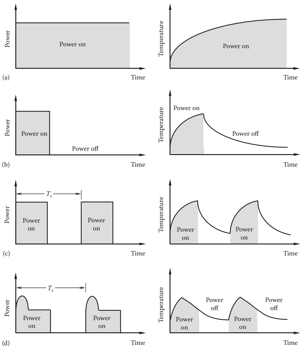
FIGURE 1.22 Temperature variations under different operation conditions: (a) S1—continuous operation; (b) S2—short time operation; (c) S3—intermittent periodic operation, where the start current has no impact on temperature rise; and (d) S4—intermittent periodic operation, where the start current has an impact on temperature rise.
