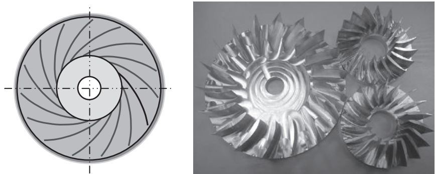
FIGURE 8.39 Helical impeller design in centrifugal fans.
