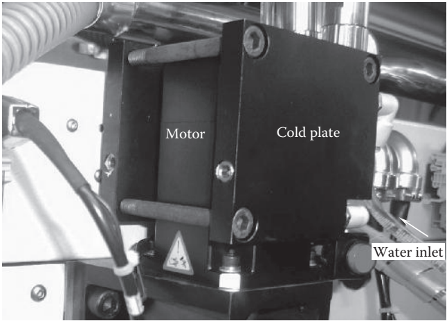
FIGURE 6.31 A motor is sandwiched by two water cold plates, causing a large temperature difference between the bearing outer ring and inner ring.
