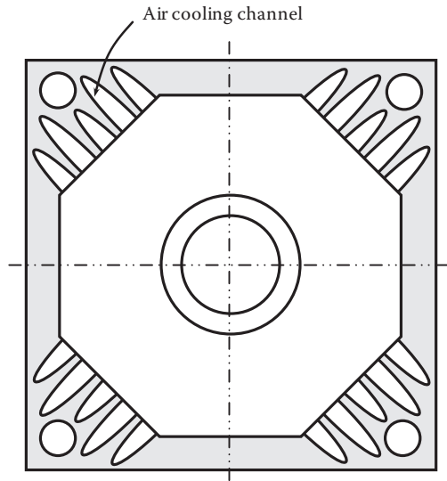
FIGURE 8.25 Air cooling channels through the motor housing.
