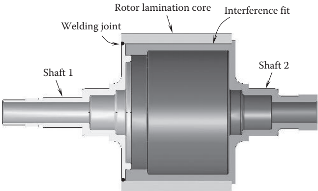
FIGURE 3.41 Alternative hollow shaft design: two shafts are integrated together with the rotor lamination core.
