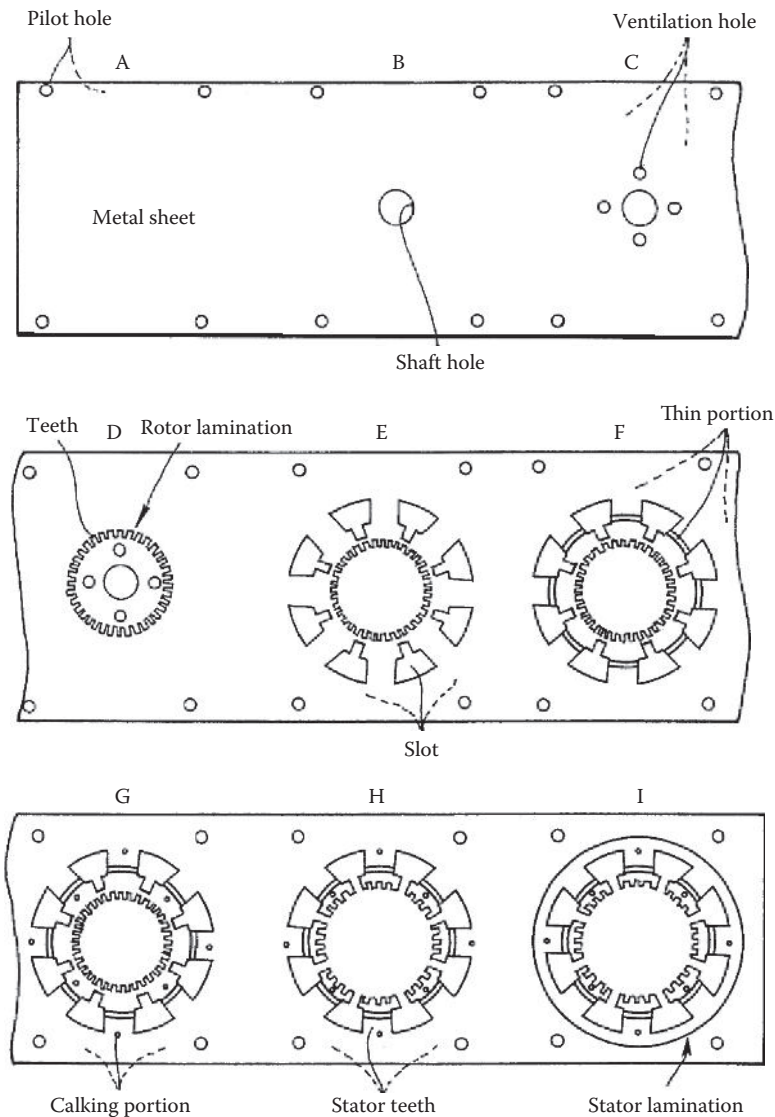
FIGURE 4.27 Rotor and stator laminations are made by a sequence of stamping operations (U.S. Patent 5,539,974) [4.21]. (Courtesy of the U.S. Patent and Trademark Office, Alexandria, VA.)
