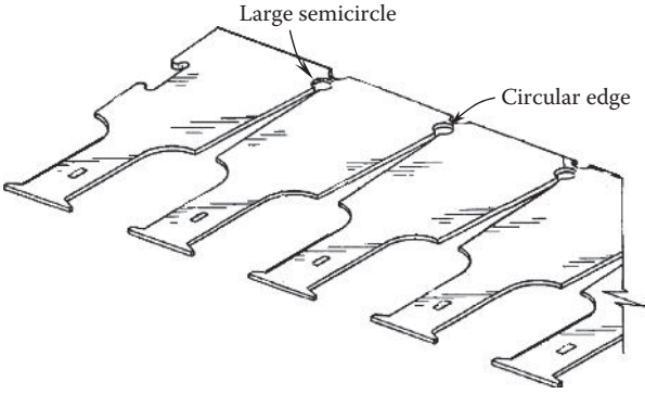
FIGURE 4.9 An alternative design of punched segmented laminations that connected together at the outer tips of the laminations (U.S. Patent 7,062,841) [4.9]. (Courtesy of the U.S. Patent and Trademark Office, Alexandria, VA.)
