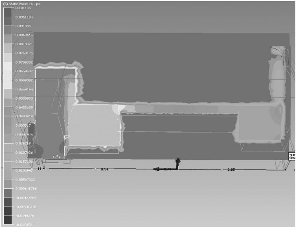
FIGURE 7.19 Pressure distribution inside the machine. The high-pressure zone is shown at the vicinity of the fan.
