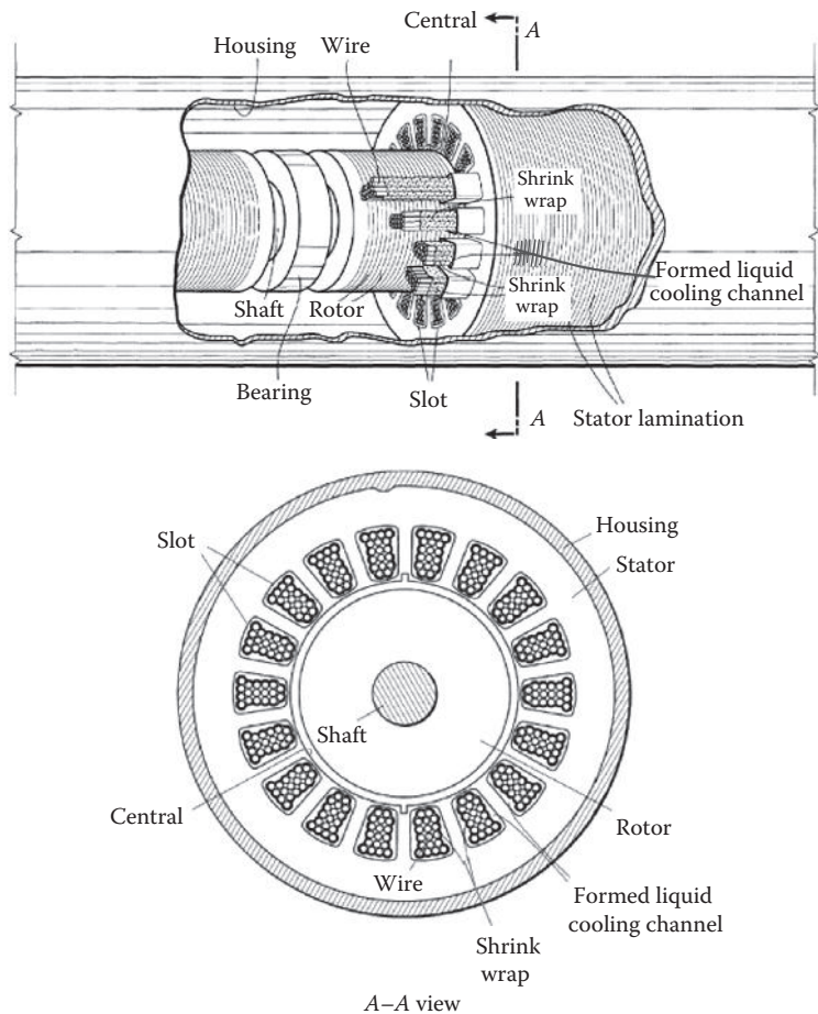
FIGURE 8.45 Enhanced heat transfer using shrink wrap surrounding magnet wires (U.S. Patent 7,679,242) [8.49]. (Courtesy of the U.S. Patent and Trademark Office, Alexandria, VA.)
