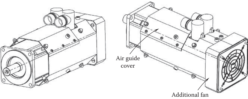
FIGURE 8.32 An additional cooling fan is mounted at the end of motor, blowing cooling air over the motor external surface. (Courtesy of Kollmorgen Corporation, Radford, VA.)
