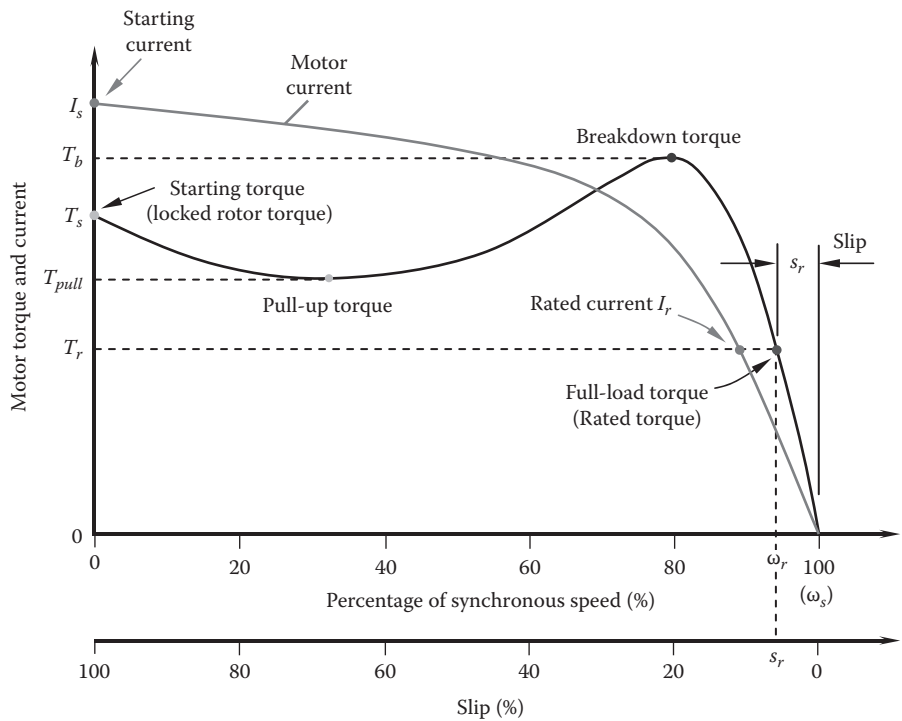
FIGURE 1.14 Torque–speed characteristics of a typical AC IM.
