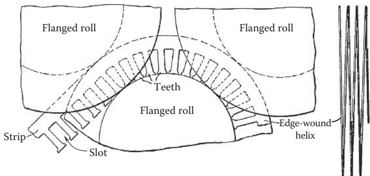
FIGURE 4.16 Fabrication of helical stator core with three flanged rolls (U.S. Patent 1,920,354) [4.11]. (Courtesy of the U.S. Patent and Trademark Office, Alexandria, VA.)
