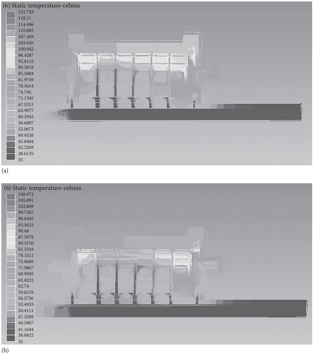
FIGURE 11.13 Temperature distributions inside the motor: (a) flowrate of 700 CFM and (b) flowrate of 900 CFM.
