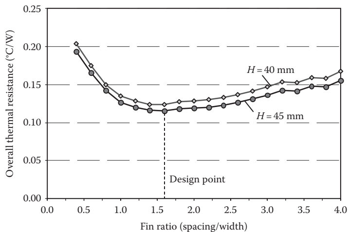
FIGURE 8.7 Effect of fin ratio on overall thermal resistance for a motor with finned housing.
