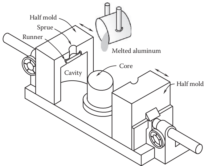
FIGURE 5.6 Permanent-mold casting for motor housing.
