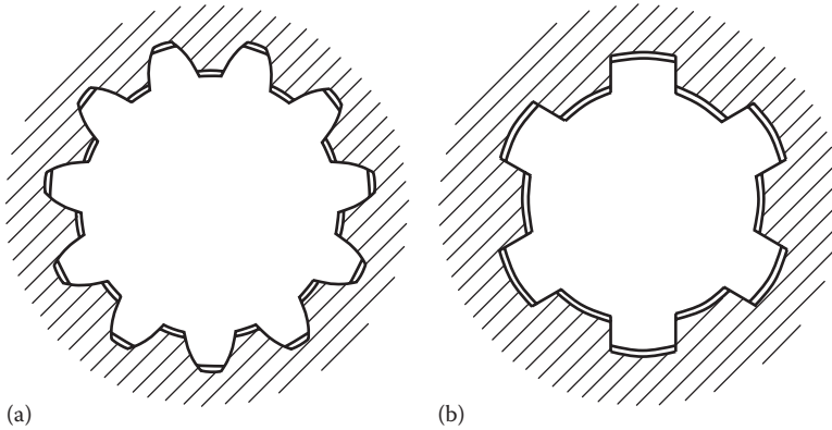
FIGURE 3.37 Spline types: (a) involute spline and (b) straight-sided spline.
