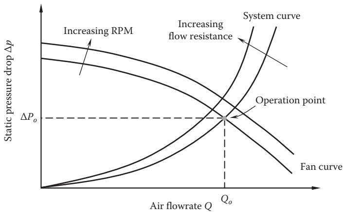
FIGURE 8.43 Fan performance characteristics.
