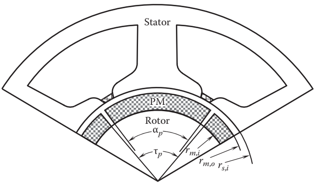
FIGURE 7.5 Eddy-current losses of PMs in PM motors having a fractional number of slots per pole.
