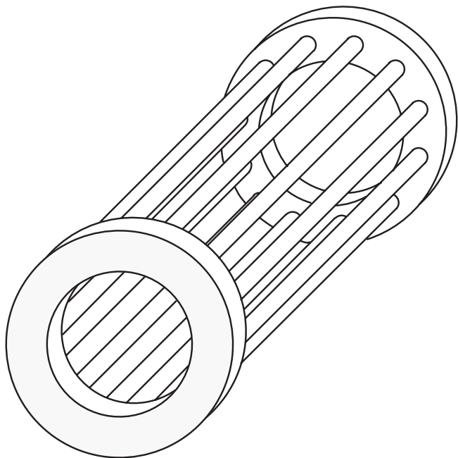
FIGURE 1.28 Conductive bars and end rings in a squirrel cage motor with closed slots.
