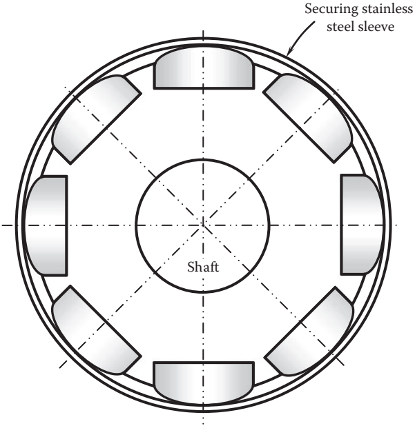
FIGURE 2.19 Using securing stainless steel sleeve for holding magnets on the rotor core.
