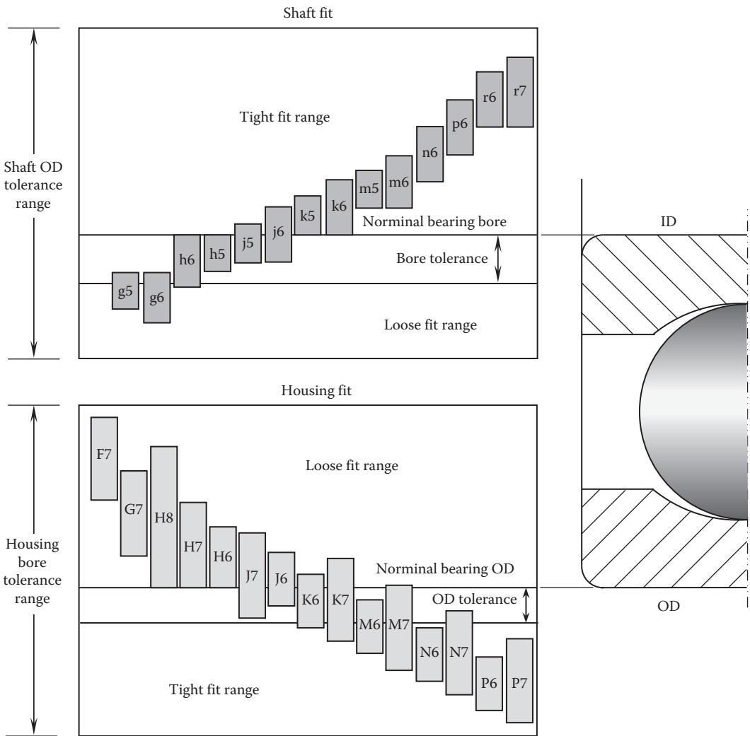
FIGURE 6.16 Fit section for bearings with shafts (top) and housings (bottom).
