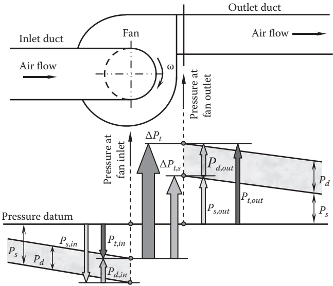
FIGURE 7.20 Relations of various pressures and pressure differentials at the inlet and outlet of a fan.
