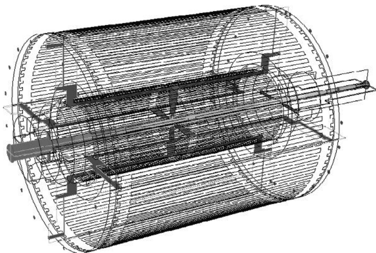
FIGURE 8.49 Cooling flow paths inside the rotor assembly.
