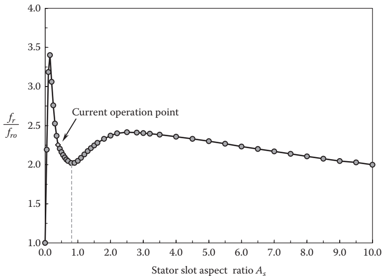
FIGURE 7.14 Effect of stator slot aspect ratio on rotor friction factor ratio.
