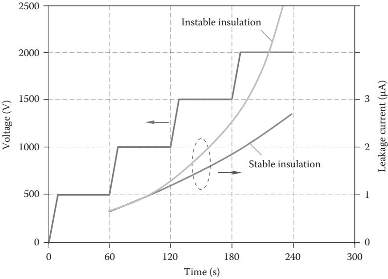
FIGURE 10.14 Step-voltage testing procedure.
