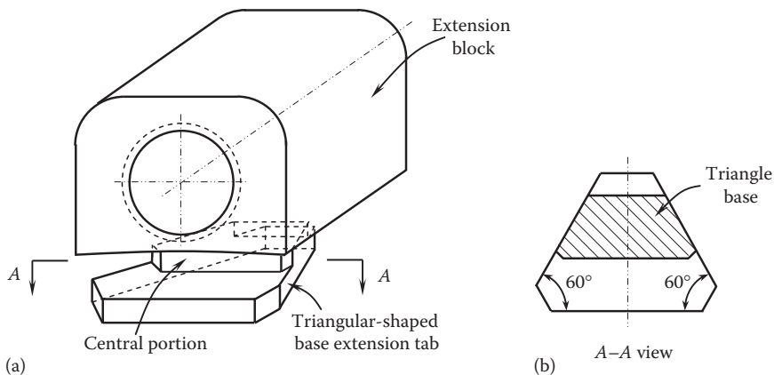
FIGURE 5.27 Triangle-base rotating fastener.
