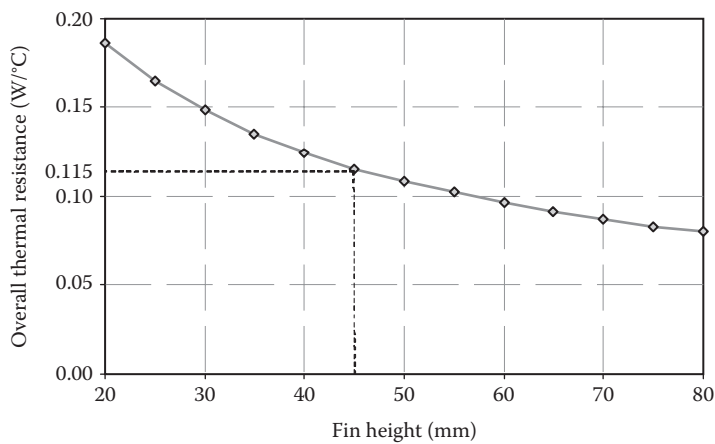
FIGURE 8.8 Effect of fin height on overall thermal resistance of a motor with finned housing.
