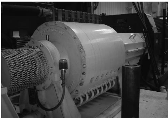
FIGURE 10.4 Water brake dynamometer for motor testing.
