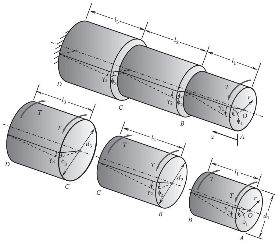
FIGURE 3.10 Torsional deflection of a stepped shaft subjected to a single torque and made from of single material.
