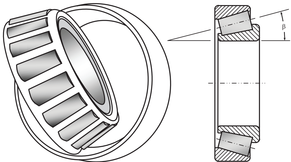
FIGURE 6.11 Tapered roller bearing, which can withstand both radial and axial loads. The cross-sectional view shows the specially designed tapered rollers and demonstrates their angular mounting, which gives their dual load ability.
