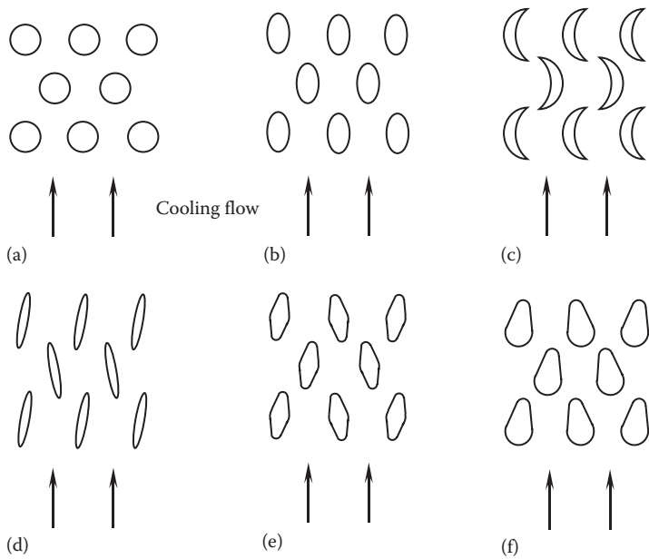
FIGURE 8.15 A variety of pin-fin shapes and arrangements: (a) round pin fins, (b) oval pin fins, (c) crescent pin fins, (d) tilted narrow oval pin fins, (e) tilted rhombic pin fins, and (f) tilted raindrop-shaped pin fins.
