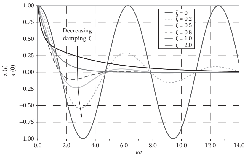
FIGURE 9.2 Comparison of damped and undamped harmonic oscillating systems with various damping ratios: (a) \zeta=1 , critical damping; (b) \zeta>1 , overdamped; (c) 0<\zeta<1 , underdamped; and (d) \zeta=0 , undamped.–
