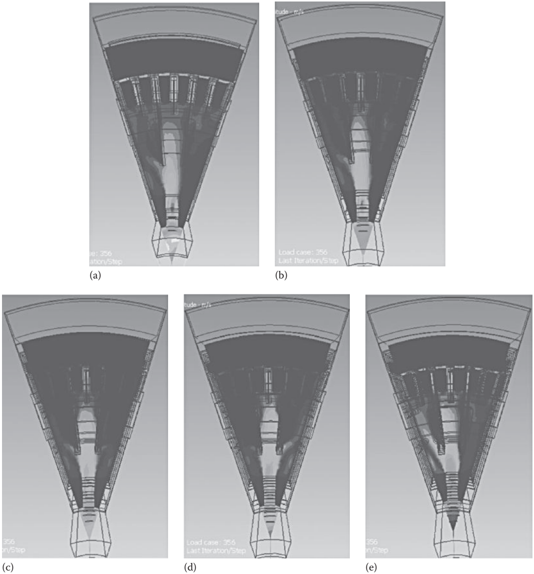
FIGURE 11.9 Velocity contours through the middle cooling channels: (a) channel 1, (b) channel 2, (c) channel 3, (d) channel 4, and (e) channel 5.
