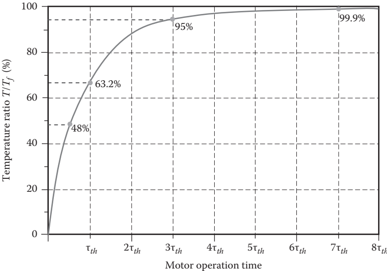
FIGURE 1.47 Variation of temperature ratio T/T_f as a function of motor operation time for a constant applied power.
