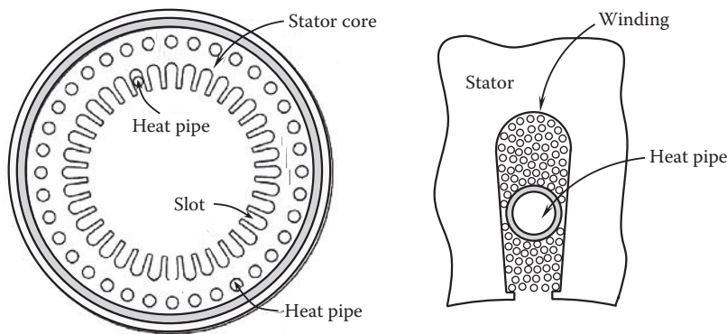
FIGURE 8.60 Heat pipes inserted in stator slots and stator core (U.S. Patent 7,569,955) [8.59]. (Courtesy of the U.S. Patent and Trademark Office, Alexandria, VA.)
