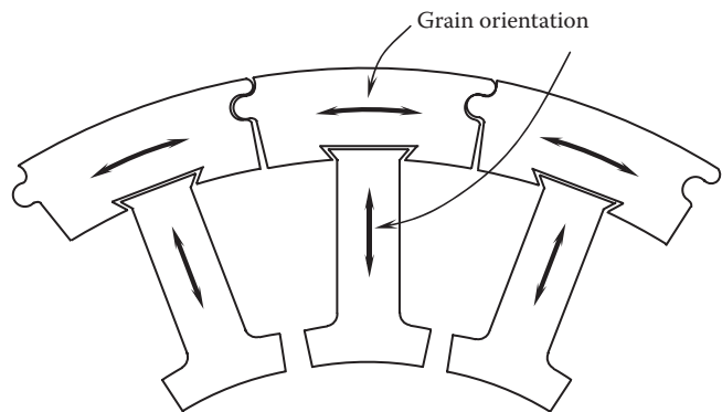
FIGURE 4.4 Grain-oriented segmented laminations.
