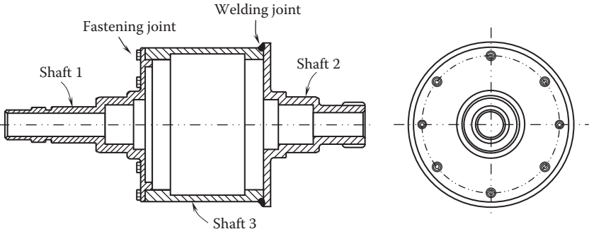
FIGURE 3.40 Three-piece hollow shaft design using fastening and welding joint methods.
