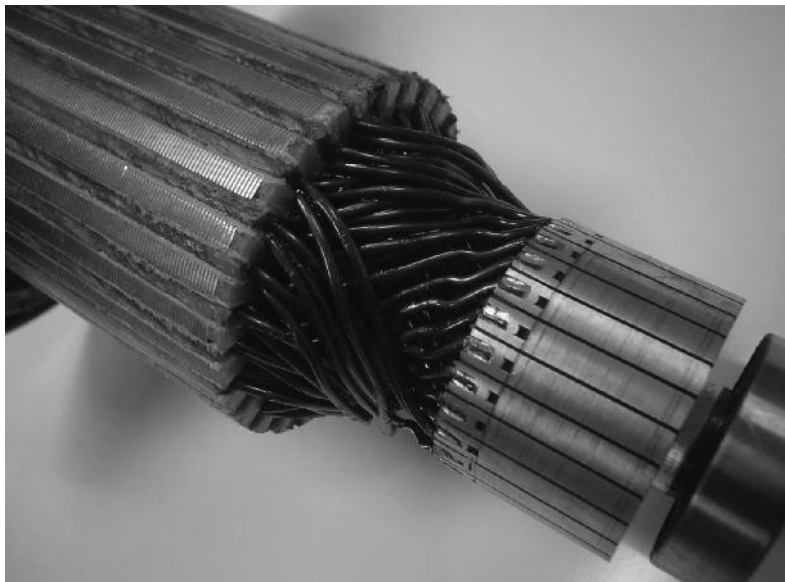
FIGURE 1.29 Rotor winding in a wound IM.
