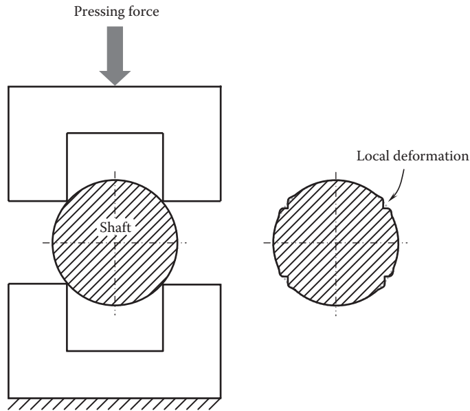
FIGURE 2.38 Fabrication of serrations on a shaft.
