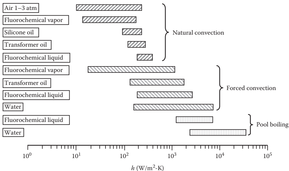
FIGURE 8.44 Relative magnitude of heat transfer coefficients for various coolants and modes of convection. (From Simons, R.E., Electron. Cool. , 2(2), 24, 1996.)
