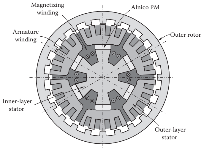
FIGURE 12.38 Topology of doubly salient PM memory motor.
