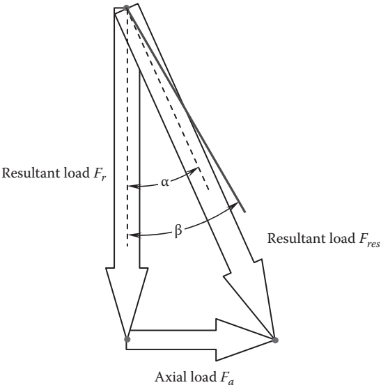
FIGURE 6.8 Loads acting on angular contact ball bearing. The load angle \alpha is determined from the radial and axial load.
