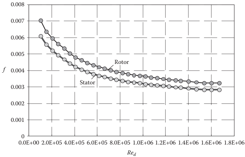
FIGURE 7.16 Comparison of friction factor on the smooth rotor and stator surfaces.
