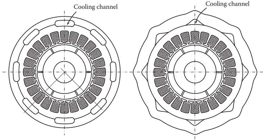
FIGURE 8.24 Arrangement of air cooling channels between the stator core and the motor housing.
