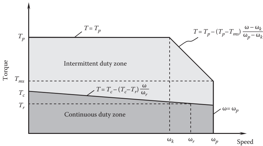
FIGURE 1.15 Torque–speed characteristics of a servomotor.
