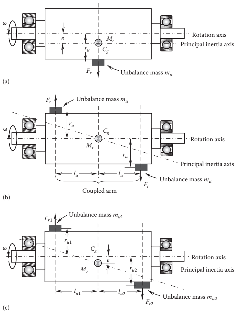
FIGURE 2.29 Three types of unbalance: (a) static unbalance, (b) coupled unbalance, and (c) dynamic unbalance. In all cases, the center of gravity is located on the principal inertia axis.
