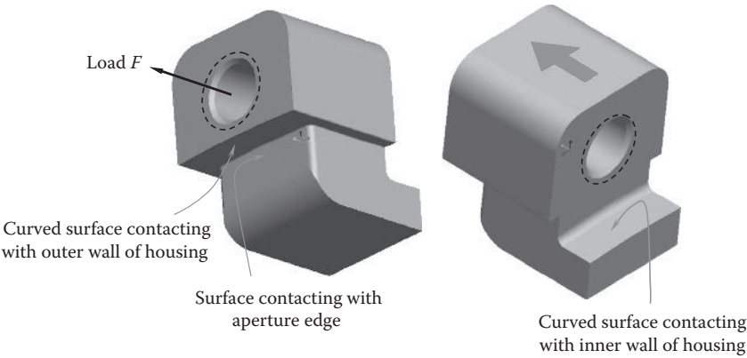
FIGURE 5.25 Contacting surfaces of Z-shaped fastener to housing.
