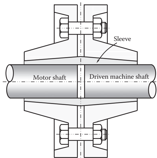
FIGURE 3.45 Flange rigid coupling. The sleeve is for aligning two shafts.
