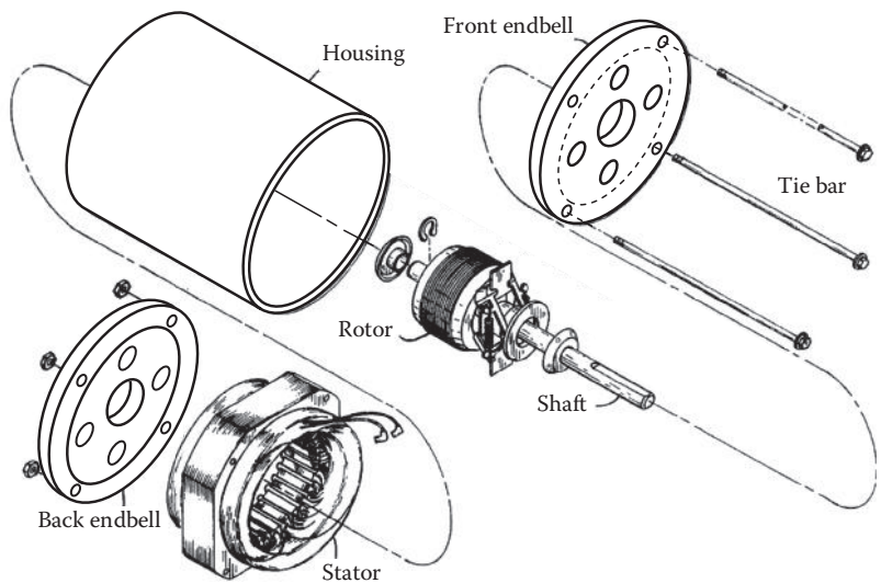
FIGURE 5.22 Motor assembly is secured by tie bars (U.S. Patent 5,412,270) [5.13]. (Courtesy of the U.S. Patent and Trademark Office, Alexandria, VA.)
