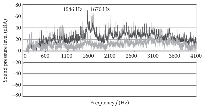
FIGURE 9.36 Comparison of SPLs for two PM servomotors with same brand and same model. Courtesy of Kollmorgen Corporation.
