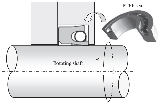
FIGURE 3.26 High-pressure, high-speed dynamic PTFE seal.
