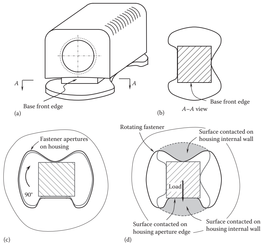
FIGURE 5.31 Installation of butterfly-base rotating fastener: (a) a perspective view of butterfly-base fastener, (b) a cross-sectional view of the butterfly-base extension tab, (c) inserting the fastener into an aperture on the housing, and (d) rotating 90° of the fastener and applying the load on the fastener.
