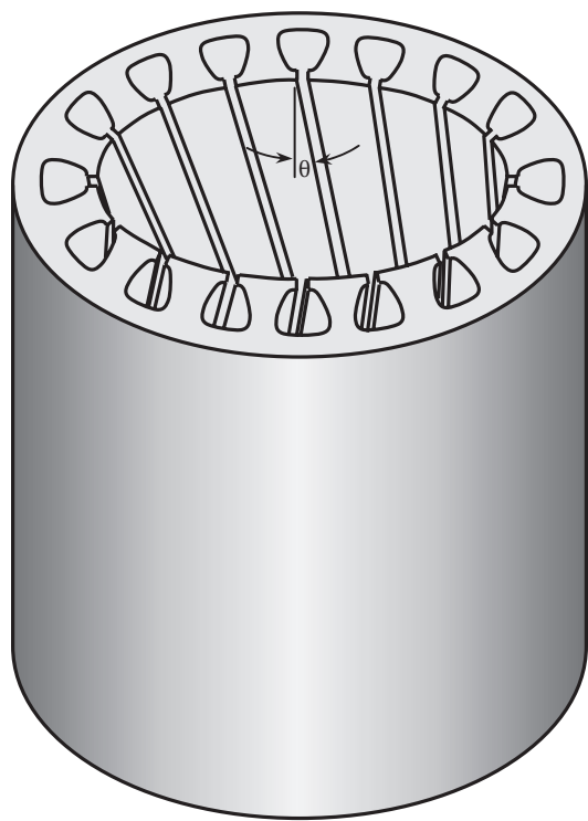
FIGURE 1.5 Skewed stator teeth with respect to its centerline for reducing cogging torque, where \theta is the skew angle.
