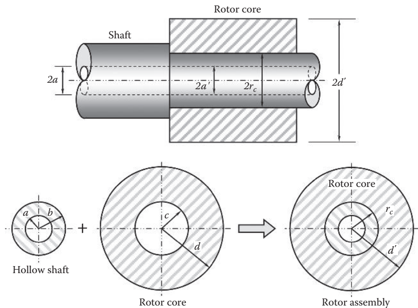
FIGURE 2.34 Dimensions of the hollow shaft and rotor core before and after assembly.
