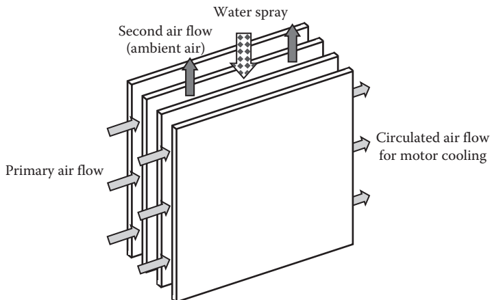
FIGURE 8.37 Forced air cooling with an indirect evaporation air cooler.
