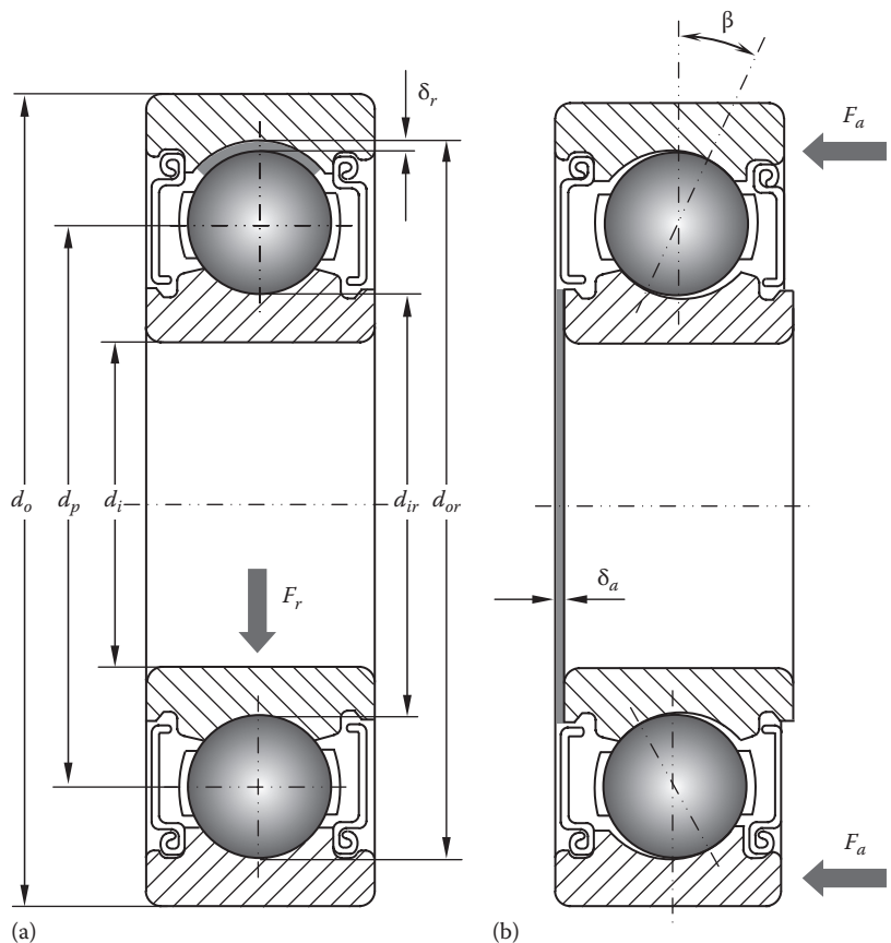
FIGURE 6.15 Bearing clearance: (a) when a bearing is subject to a radial load F_r , a radial clearance \delta_r is formed between the inner and outer ring; (b) when a bearing is subject to axial load F_a , the axial clearance \delta_a and contact angle \beta are formed, but the radial clearance disappears.
