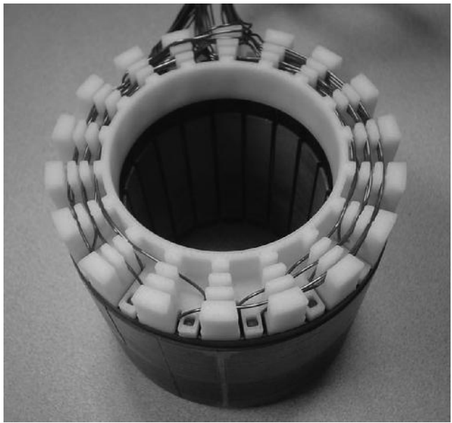
FIGURE 4.23 Specially designed molded plastic insulation part used at the motor ends for insulating the lead wires.
