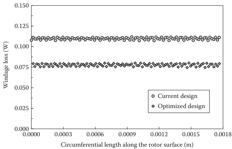
FIGURE 7.15 Comparison of rotor windage loss data between the current and optimized design.
