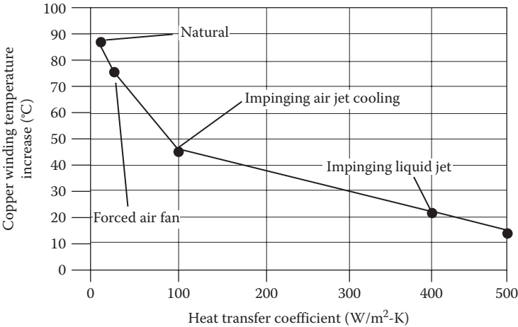
FIGURE 8.35 Temperature rise at end winding with different cooling methods (U.S. Patent 6,639,334) [8.36]. (Courtesy of the U.S. Patent and Trademark Office, Alexandria, VA.)
