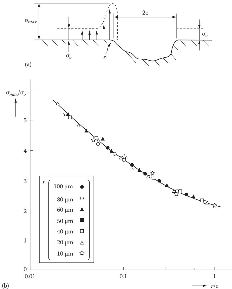
FIGURE 6.40 (a) Stress concentration around a surface dent and (b) the relationship between the stress ratio and the ratio of r/c (U.S. Patent 4,904,094) [6.52]. (Courtesy of the U.S. Patent and Trademark Office, Alexandria, VA.)
