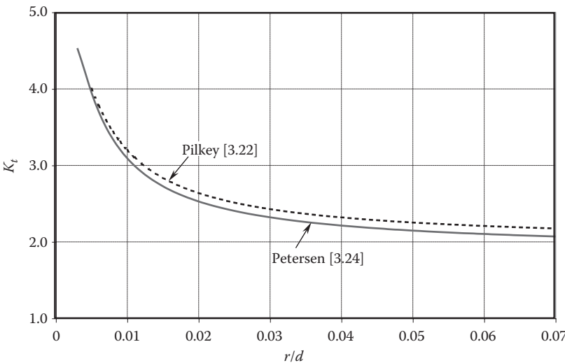
FIGURE 3.33 Comparison between two correlations of stress correlation of keyed shaft for the case of w/d = 1/4 and h/d = 1/8 .
