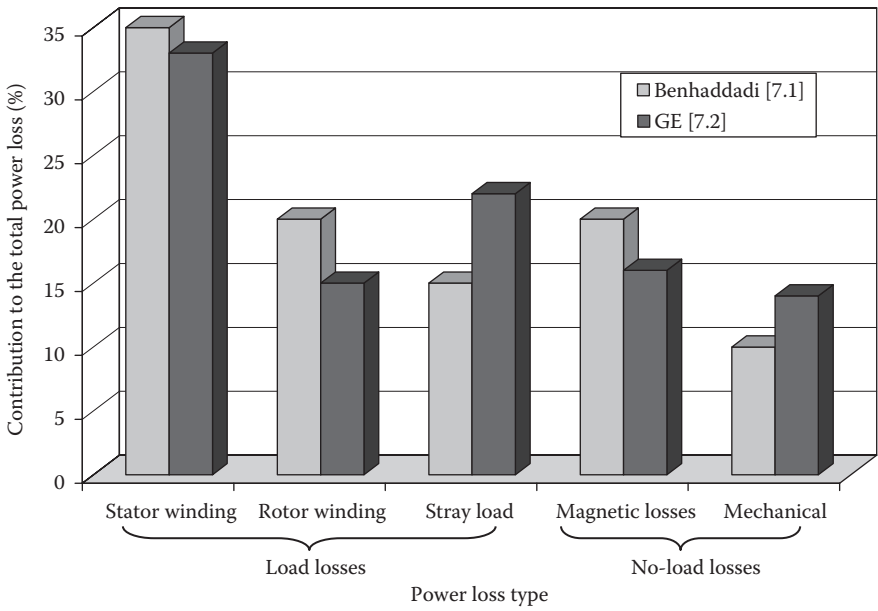
FIGURE 7.1 Comparison of power loss distributions in electric motors.
