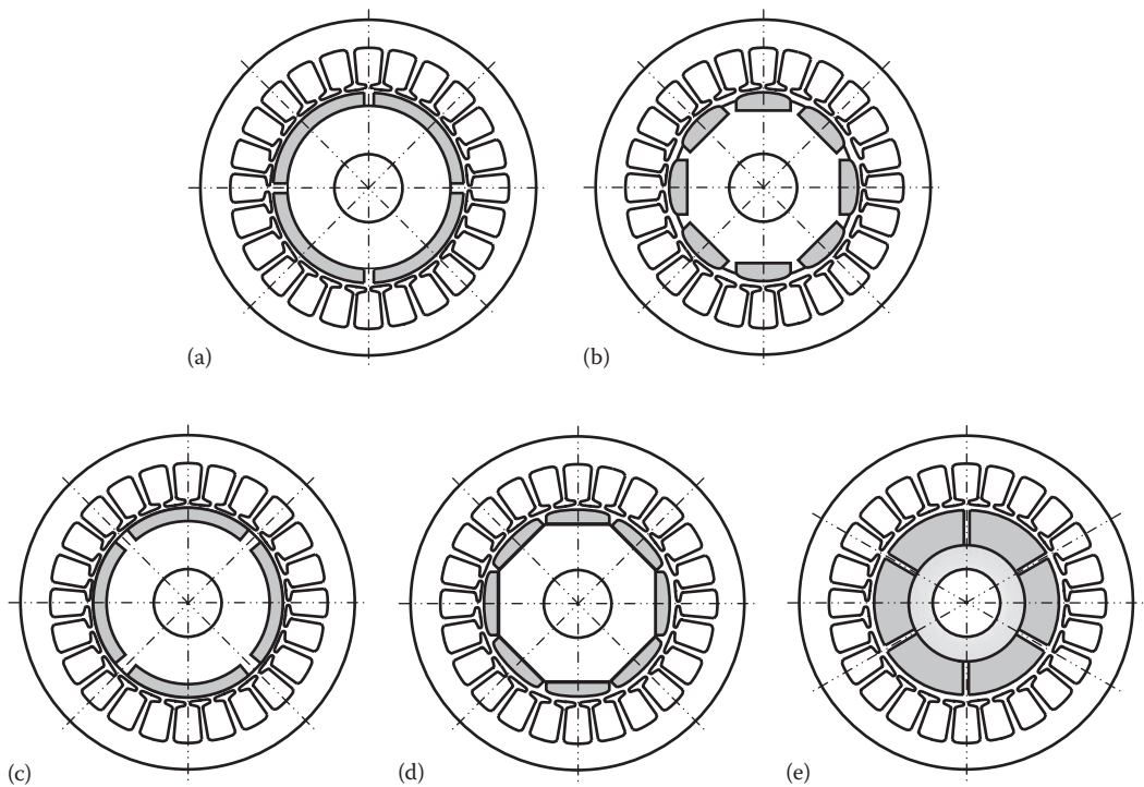
FIGURE 2.15 Various mounting methods on rotor surface: (a) tile-shaped magnets mounted on the rotor surface, (b) bread loaf magnets partially positioned in the sunken portions of the rotor, (c) tile-shaped magnets fully positioned in the sunken portions of the rotor, (d) bread loaf magnets mounted on the surface of an octagon rotor, and (e) thick magnets mounted on the thin rotor core, generating strong magnetic field.
