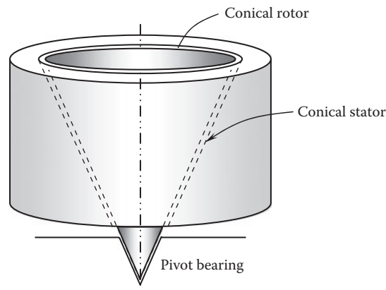
FIGURE 12.23 Conical rotor with a pivot bearing having a uniform air gap.
