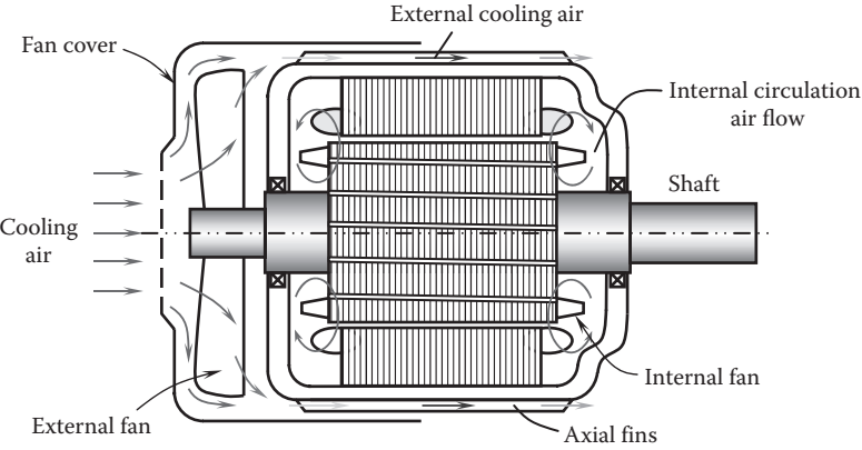
FIGURE 8.33 Motor is cooled by both external and internal air flows; the motor housing functions as a heat exchanger.
