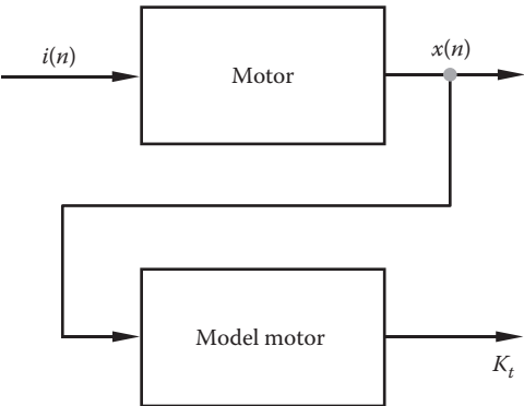
FIGURE 1.44 The block diagram of conventional circuit for estimating motor torque constant.
