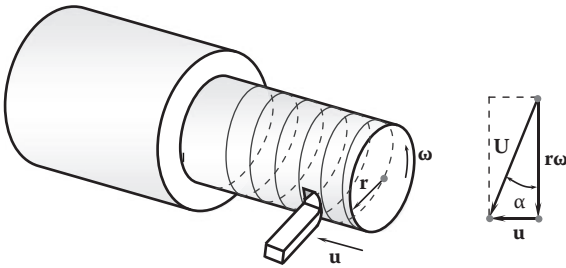
FIGURE 3.19 Formation of spiral grooves on shaft surface during shaft finishing machining.
