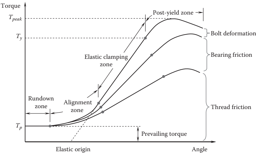
FIGURE 5.37 Four distinct zones in fastener-tightening process.
