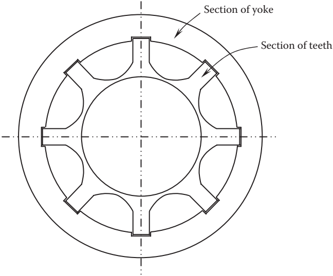
FIGURE 4.10 Integrated stator core with a section of teeth and a section of yoke; the section of teeth is positioned in the concave slots at the yoke inner surface.
