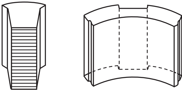
FIGURE 4.13 The sheets of teeth are held together as a subsection and then integrated with the yoke laminations.
