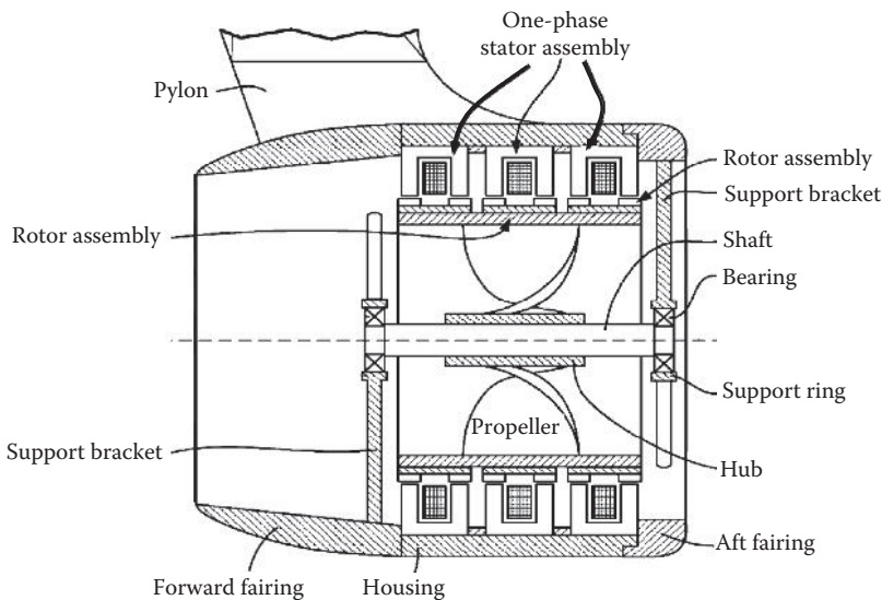
FIGURE 12.29 Structure of an RDT with a TF motor (U.S. Patent 8,299,669) [12.32]. (Courtesy of the U.S. Patent and Trademark Office, Alexandria, VA.)
