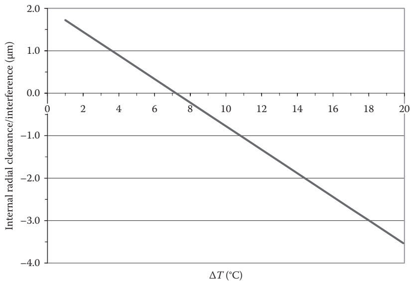
FIGURE 6.33 Effect of the temperature difference of the bearing inner and outer rings on the bearing radial clearance/interference for a specific bearing with the clearance class of CN.
