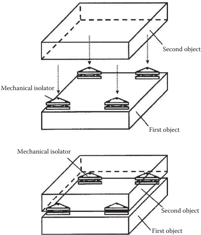
FIGURE 9.23 Mechanical isolation systems assembled into the multilayer magnetic system (U.S. Patent 8,279,031) [9.39]. (Courtesy of the U.S. Patent and Trademark Office, Alexandria, VA.)
