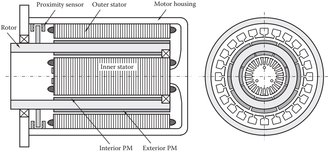
FIGURE 12.6 RF, dual-stator, PM motor with two bearings.
