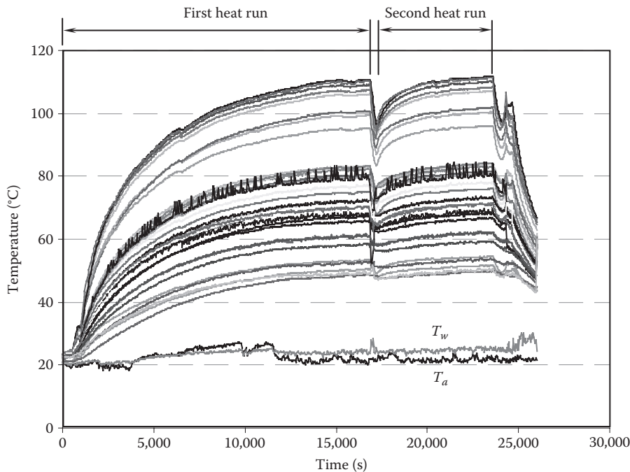
FIGURE 10.18 Thermal testing is performed at the rated speed and rated torque until thermal equilibrium is achieved. The testing data show that the successive test significantly reduces the motor heating time.
