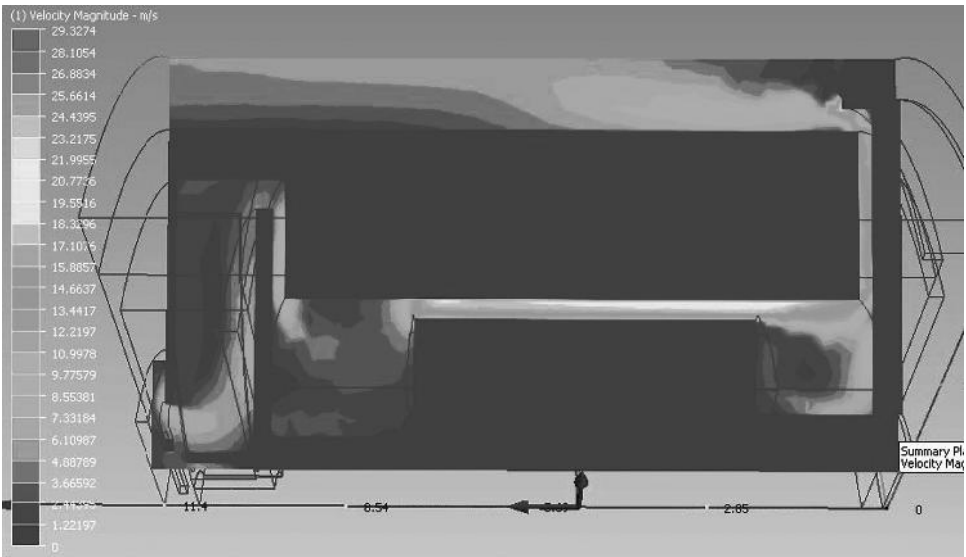
FIGURE 7.18 Velocity field through the internal cooling paths.
