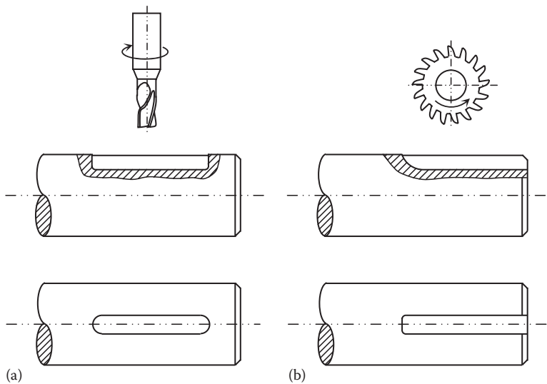
FIGURE 3.28 Keyseat types: (a) profile keyseat and (b) sled runner keyseat.
