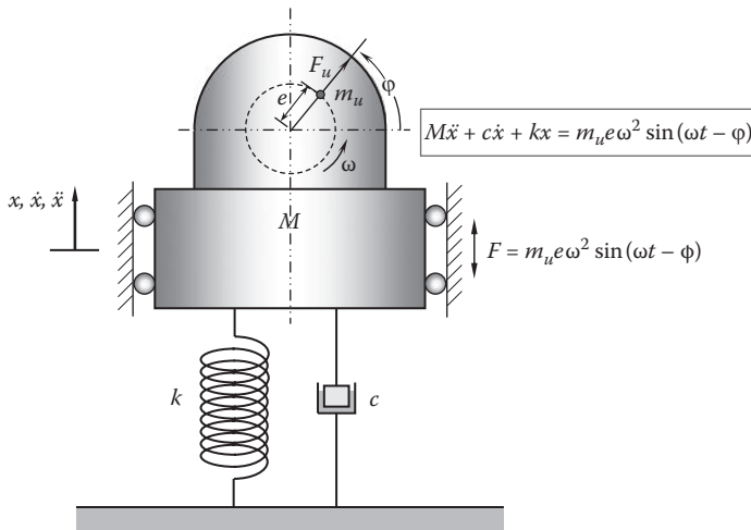
FIGURE 9.6 Forced vibration induced by unbalanced mass.
