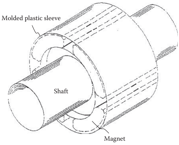
FIGURE 2.21 Retention of magnets with a molded plastic sleeve (U.S. Patent 4,973,872) [2.42]. (Courtesy of the U.S. Patent and Trademark Office, Alexandria, VA.)
