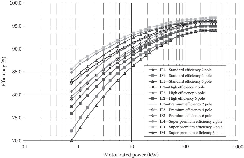
FIGURE 1.23 Comparison of four efficiency classes for electric AC motors with 50 Hz.
