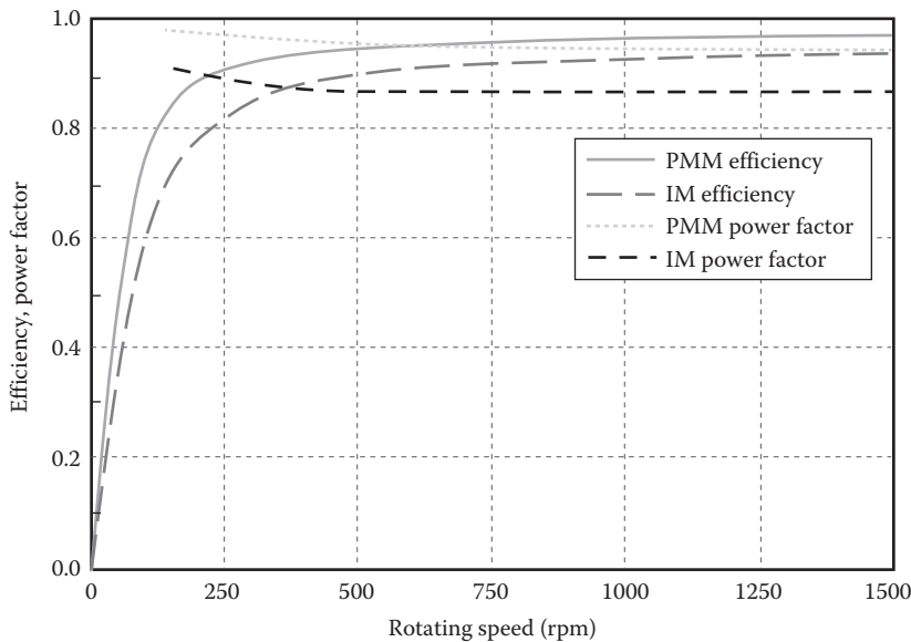
FIGURE 1.31 Comparison of calculated motor efficiency and power factor between a 55 kW, 1500 rpm IM and a PMM under an identical operation condition.
