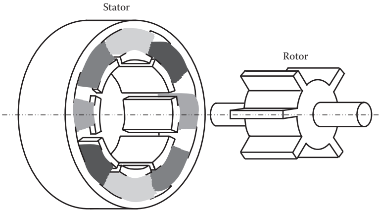
FIGURE 1.40 The salient rotor in an SRM.
