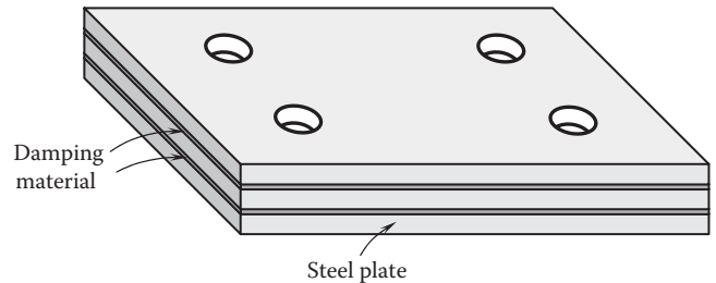
FIGURE 9.24 Laminated damping pad for providing effective damping of electric machine.
