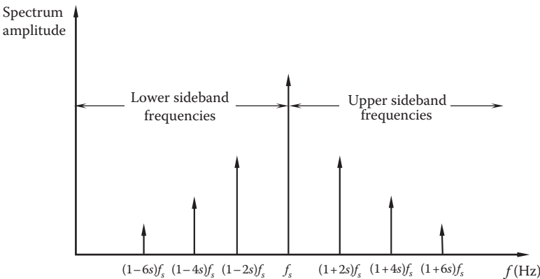
FIGURE 9.12 Sideband frequencies around the fundamental line frequency f_s .
