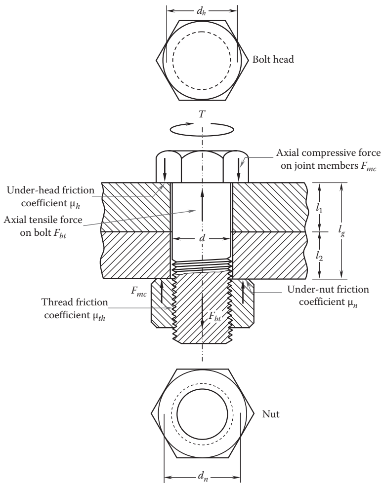
FIGURE 5.35 Bolt-nut fasteners with drilled holes through joint members.
