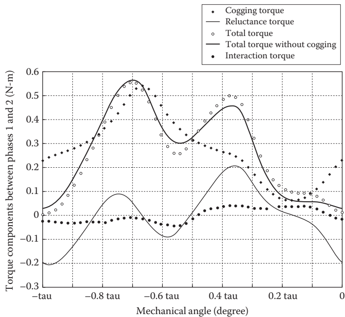
FIGURE 12.27 Torque component for the FC-TFM, obtained from simulations (European Patent 2,317,633) [12.31]. (Courtesy of the European Patent Office, Munich, Germany.)
