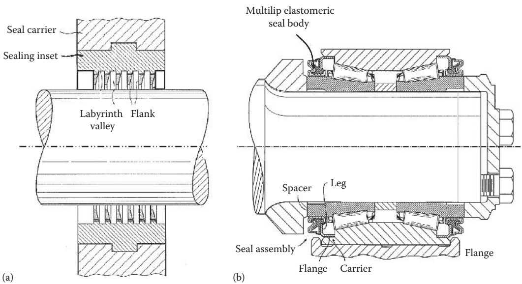
FIGURE 3.27 Noncontact labyrinth seals used in rotating machinery: (a) tooth-groove labyrinth seal (U.S. Patent Application 2012/0228830) [3.19] and (b) multilip labyrinth seal (U.S. Patent 8,342,535) [3.20]. (Courtesy of the U.S. Patent and Trademark Office, Alexandria, VA.)
