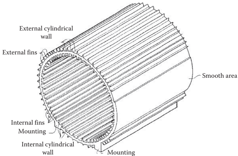
FIGURE 8.10 Outer and inner fins on the motor frame (U.S. Patent 4,839,547) [8.23]. (Courtesy of the U.S. Patent and Trademark Office, Alexandria, VA.)
