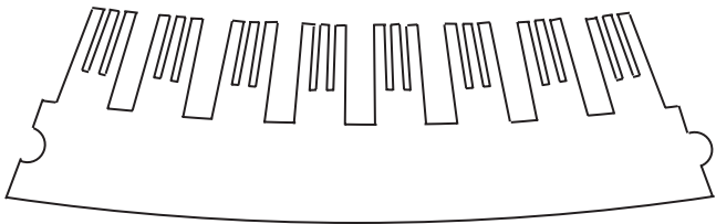
FIGURE 4.2 A segmented stator lamination containing a number of teeth for a large-size motor. The wide radial slots are used for receiving stator windings and the narrow radial slots for reducing eddy-current losses.
