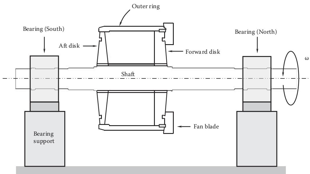
FIGURE 11.21 Configuration and components of the fan test system.
