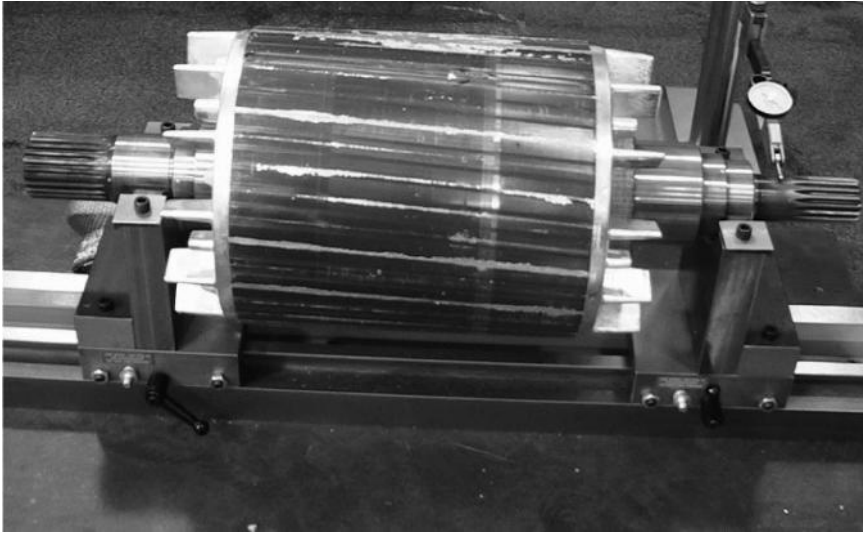
FIGURE 2.26 Measurement of shaft runout after rotor assembly but before rotor machining.
