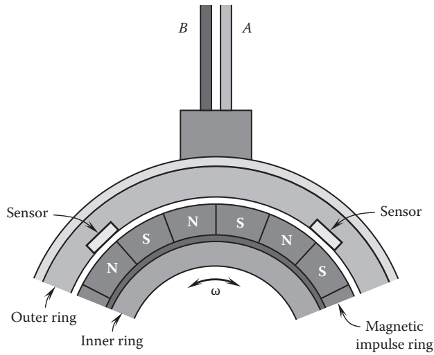
FIGURE 6.14 Operating principle of sensor bearing.
