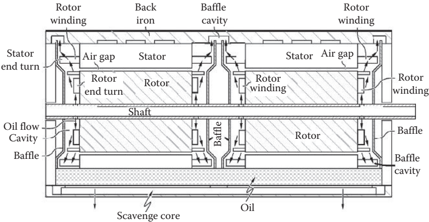
FIGURE 7.27 A liquid-cooled electric machine is cooled by injecting oil radially along a plurality of baffles via centrifugal force toward rotor and stator end windings [7.50]. (Courtesy of the U.S. Patent and Trademark Office, Alexandria, VA.)
