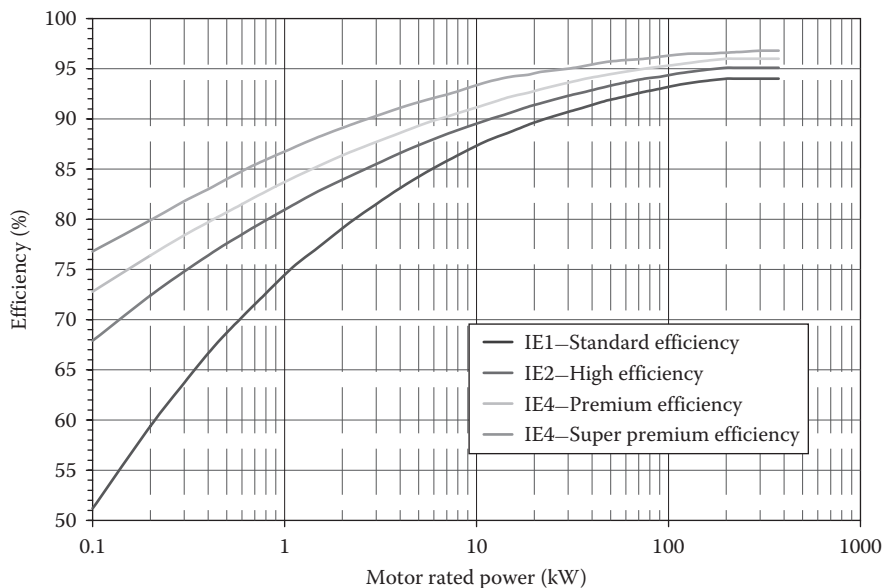
FIGURE 1.25 Comparison of four efficiency classes for 50 Hz, 4 pole electric motors.
