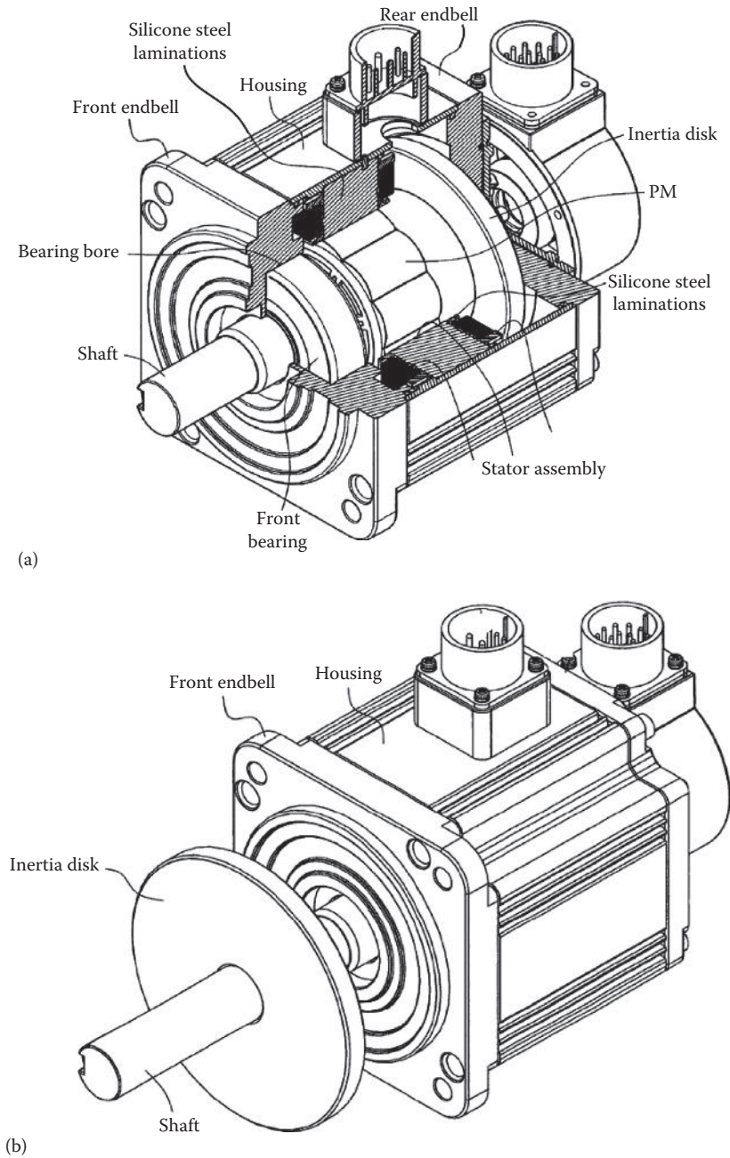
FIGURE 1.21 Addition of an inertia disk either inside (a) or outside (b) of a motor to increase the rotor inertia (U.S. Patent 7,911,095) [1.36]. (Courtesy of the U.S. Patent and Trademark Office, Alexandria, VA.)
