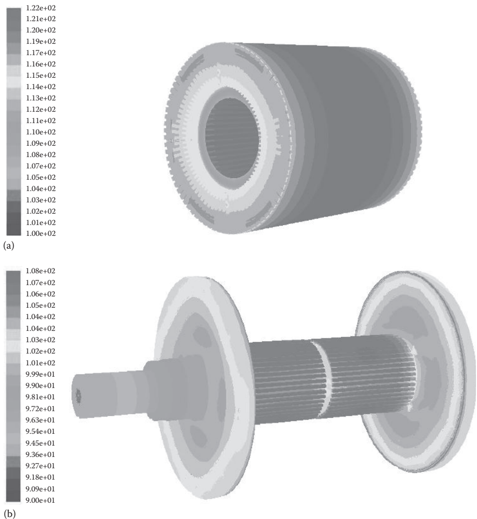
FIGURE 8.50 Temperature distributions in the rotor assembly: (a) rotor core and (b) shaft and end rings, showing the temperature generally decreasing from the center to the two rotor ends symmetrically.
