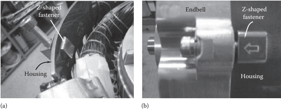
FIGURE 5.26 Configuration of Z-shaped fastener to housing (a) and housing endbell (b).
