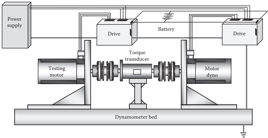
FIGURE 10.3 Motor testing system with the motor/generator dynamometer.
