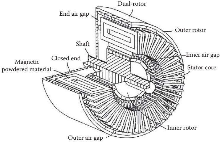
FIGURE 12.5 A cutaway perspective view of the motor assembly (U.S. Patent 6,924,574) [12.11]. (Courtesy of the U.S. Patent and Trademark Office, Alexandria, VA.)
