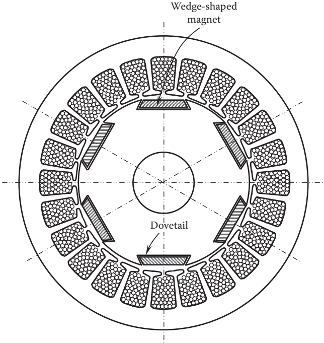
FIGURE 2.18 An innovative method for magnet retention by inserting wedge-shaped magnets into the dovetails on the rotor surface.
