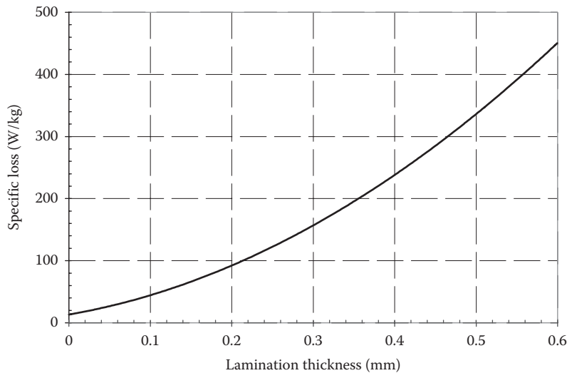
FIGURE 4.26 Specific iron loss in a PM motor versus lamination thickness at B=2T and f=1200 Hz, showing that the reduction in lamination thickness can significantly reduce stator power loss.
