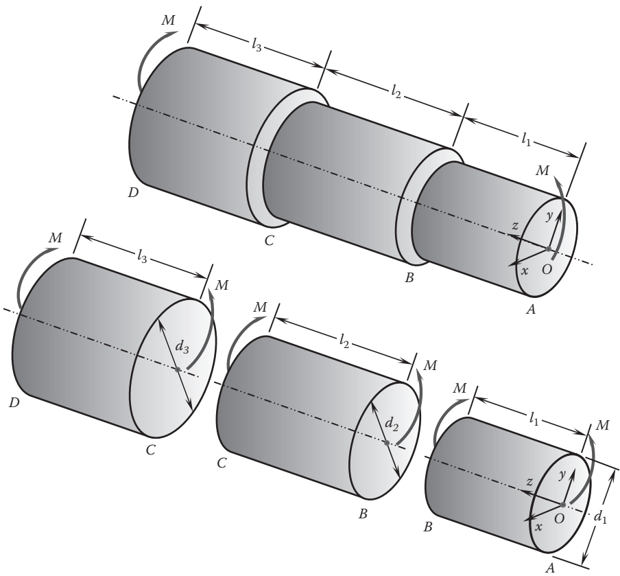
FIGURE 3.8 A stepped shaft subjected to pure bending moment.
