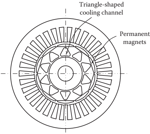
FIGURE 8.28 Triangle-shaped cooling channels through the rotor core.
