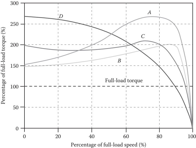
FIGURE 2.8 Torque-speed characteristics for design A, B, C, and D motors defined by NEMA.
