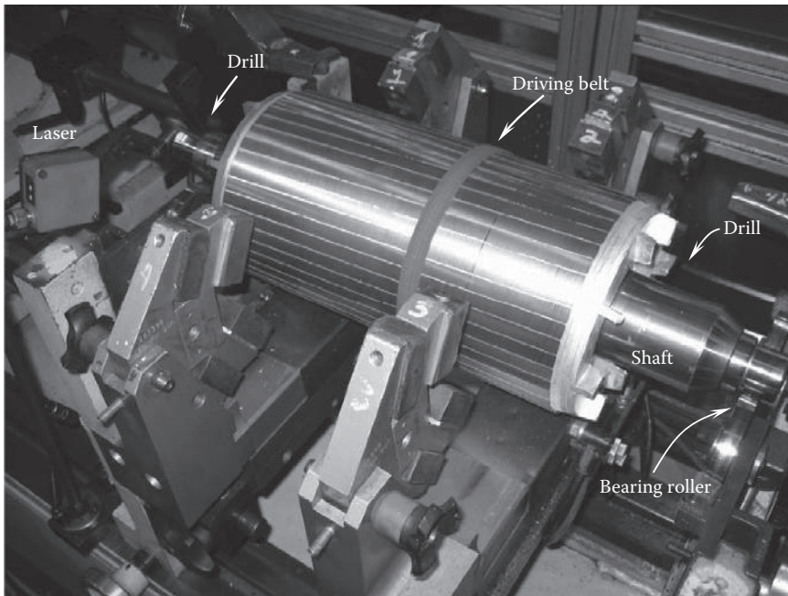
FIGURE 2.33 Automatically controlled rotor balancing process.
