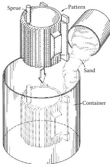
FIGURE 5.7 Making motor housing with lost-foam-casting process (U.S. Patent 6,109,333) [5.9]. (Courtesy of the U.S. Patent and Trademark Office, Alexandria, VA.)
