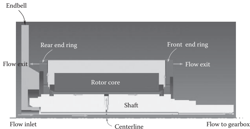
FIGURE 8.48 Cooling flow paths in the rotor assembly (only a half model shown here).
