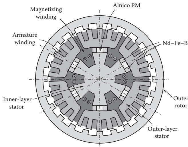
FIGURE 12.39 Doubly salient PM memory motor with dual magnet.
