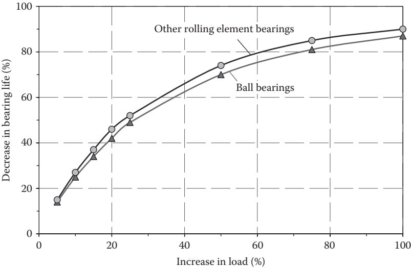
FIGURE 6.36 Impact of increased load on bearing life.
