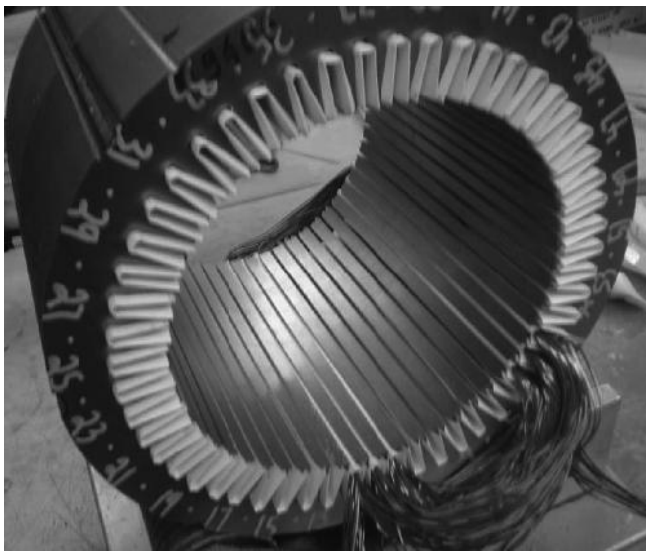
FIGURE 4.24 Insulation papers inserting in the stator slots for receiving winding coils.
