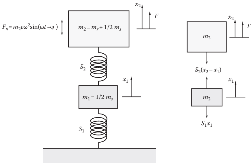
FIGURE 2.47 Reduced two-degree-of-freedom rotordynamic model for rotor assembly, where the exciting force is produced due to the rotor unbalance.
