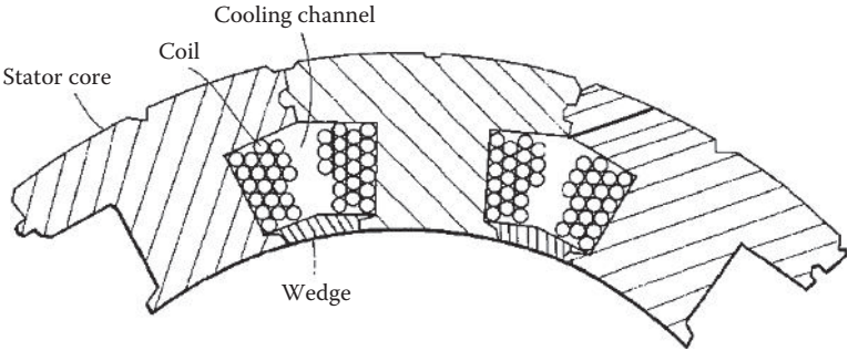
FIGURE 8.27 Cooling channels formed between stator winding coils (U.S. Patent 6,713,927) [8.34]. (Courtesy of the U.S. Patent and Trademark Office, Alexandria, VA.)
