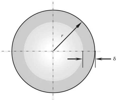
FIGURE 7.2 Skin depth of a conducting magnet wire, where \delta < r .
