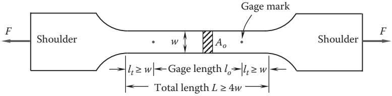
FIGURE 5.15 Typical tensile specimen, showing a reduced gage section at the middle and enlarged shoulders at the ends of the specimen.
