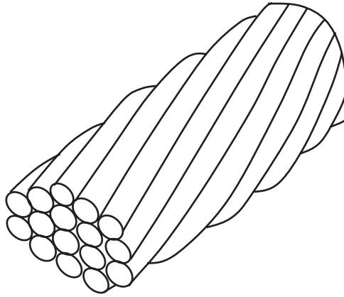
FIGURE 7.4 Litz wires used for motor windings for minimizing skin effect.
