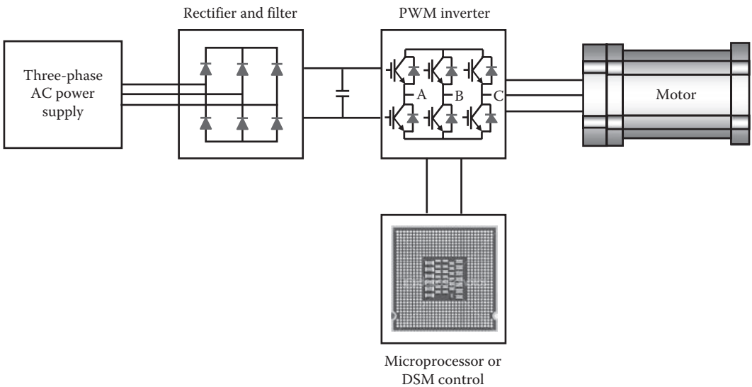
FIGURE 10.11 Block diagram of inverter-driven method.
