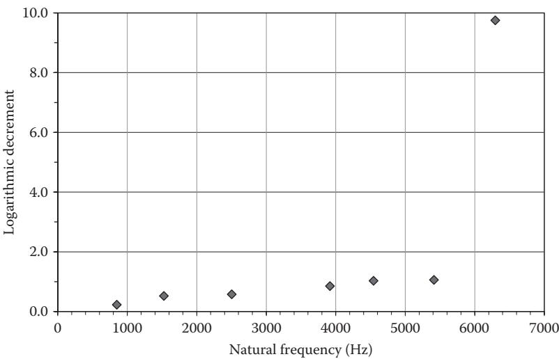
FIGURE 11.26 Damped natural frequencies versus damped ratios for determining the system stability.
