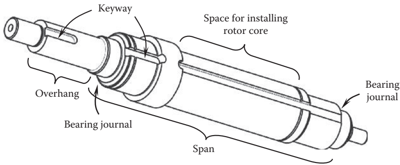
FIGURE 3.1 Structure of a motor shaft.
