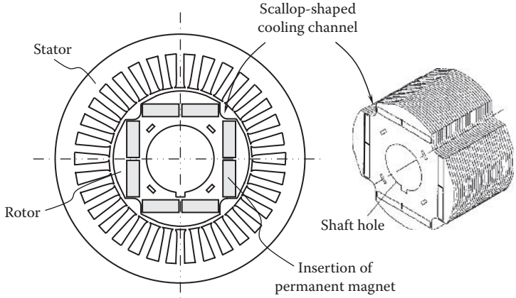
FIGURE 8.29 Scallop-shaped cooling channels between the rotor and stator (U.S. Patent 6,703,745) [8.35]. (Courtesy of the U.S. Patent and Trademark Office, Alexandria, VA.)
