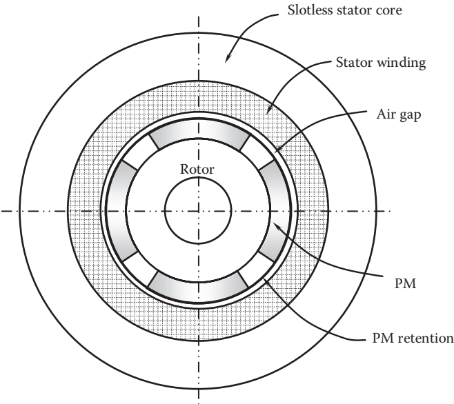
FIGURE 4.15 Structure of a four-pole slotless PM motor.
