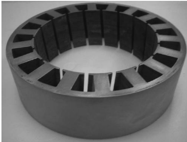
FIGURE 4.31 Stator core is secured with a thin sleeve at the outside of the core.
