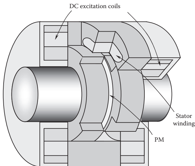
FIGURE 12.17 HESM with powdered iron core and global excitation coils.
