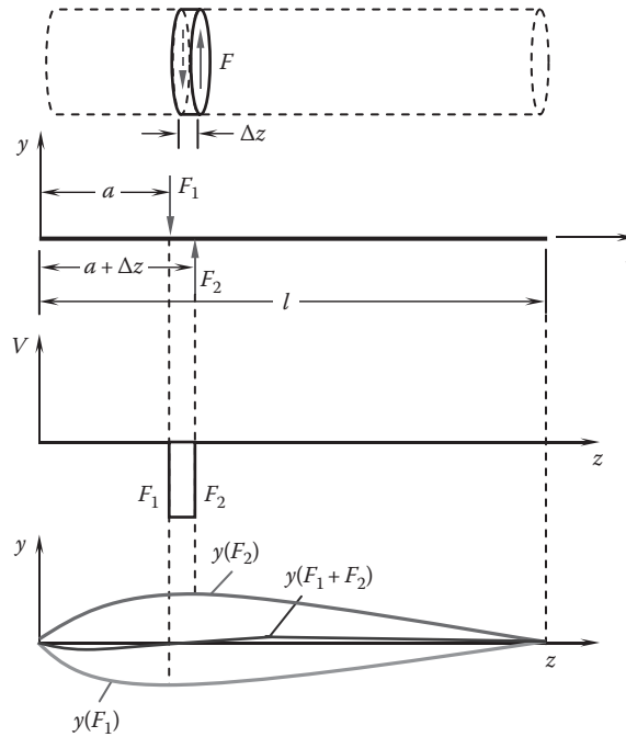
FIGURE 3.15 Deflection of a shaft subjected to shear load.
