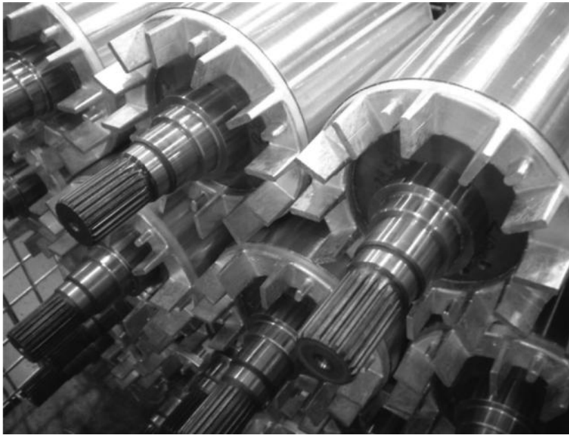
FIGURE 3.34 Spline shafts used in induction motors.
