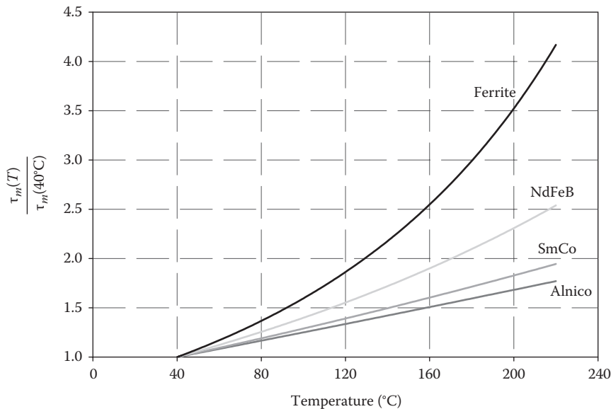
FIGURE 1.46 The temperature influence on mechanical time constant ratio for four types of PMs, with the ambient temperature of 40°C.
