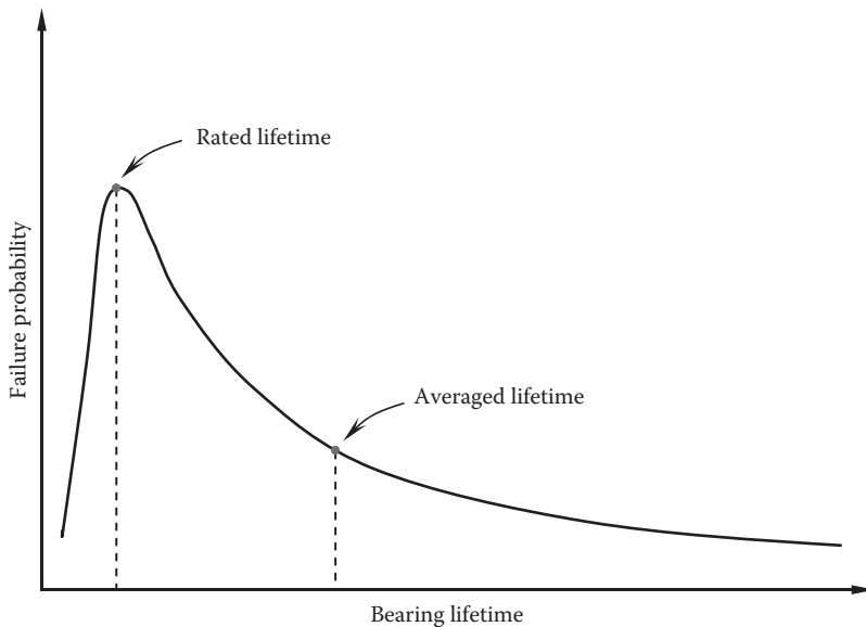
FIGURE 6.23 The bearing lifetime of motor as a function of bearing failure probability, suggested by NSK [6.29].
