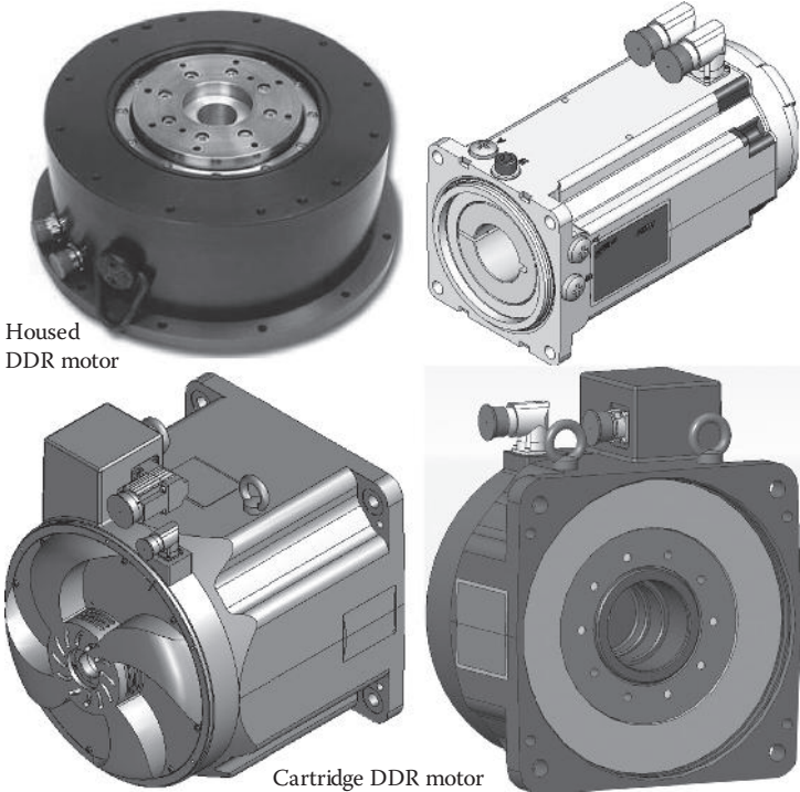
FIGURE 1.38 Various DDR motors. (Courtesy of Kollmorgen Corporation, Radford, VA.)
