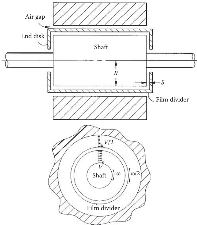
FIGURE 7.21 Using a film divider to lower windage loss in the air gap (U.S. Patent 5,828,148) [7.45]. (Courtesy of the U.S. Patent and Trademark Office, Alexandria, VA.)
