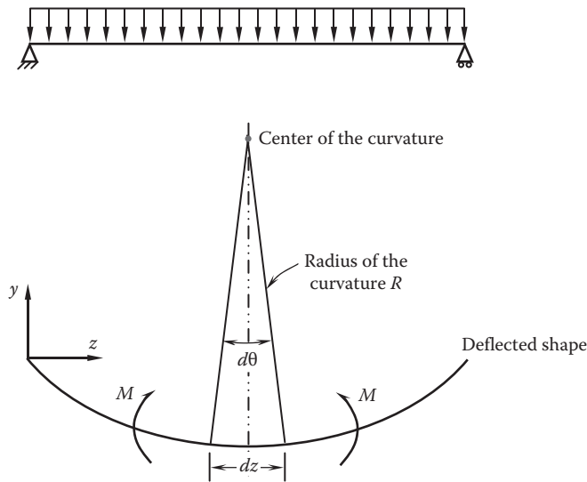
FIGURE 3.2 Beam deflection under uniformly distributed load.
