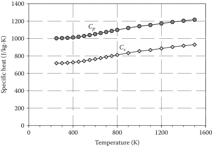
FIGURE 8.19 Specific heat of air as a function of temperature.
