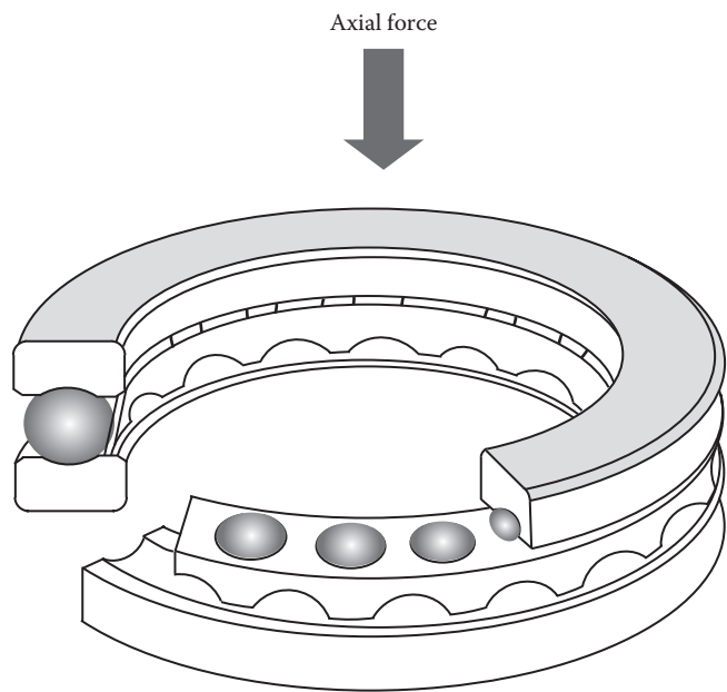
FIGURE 6.12 Thrust ball bearing designed for receiving thrust (axial) loads.
