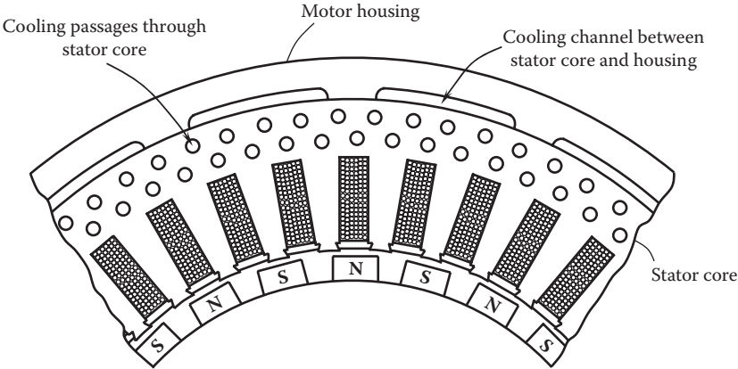
FIGURE 8.26 Cooling passages through the stator core and between the stator core and the housing (U.S. Patent 7,288,870) [8.33]. (Courtesy of the U.S. Patent and Trademark Office, Alexandria, VA.)
