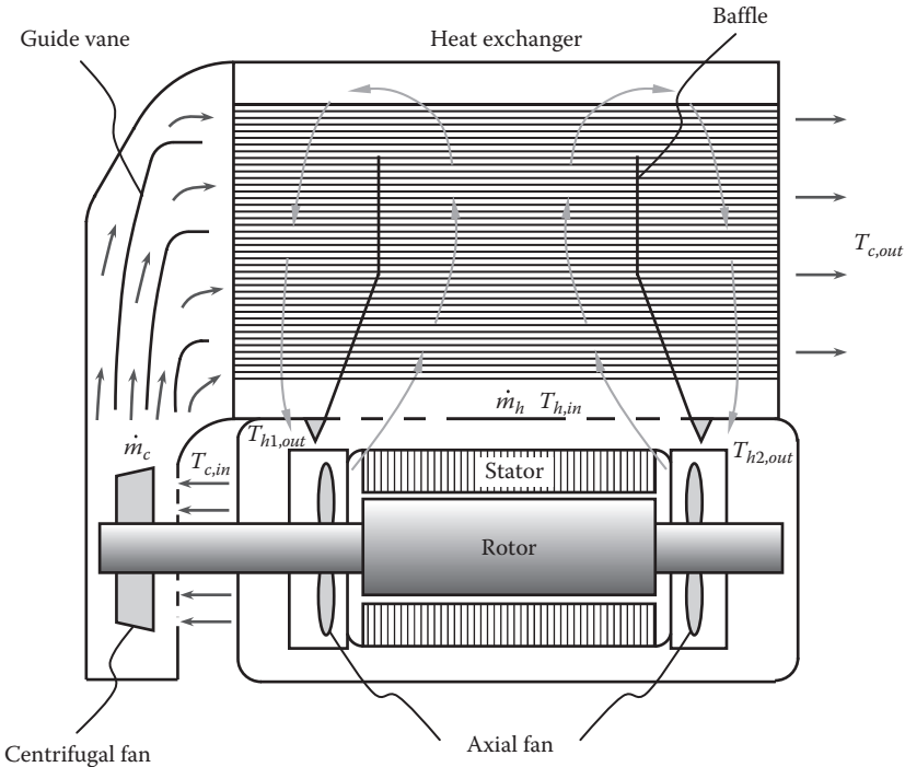
FIGURE 8.36 Forced air cooling with an air-to-air heat exchanger.
