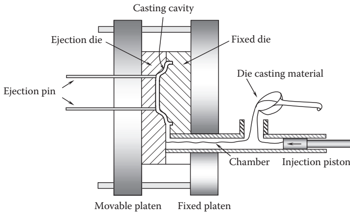
FIGURE 5.4 Illustration of die-casting process.
