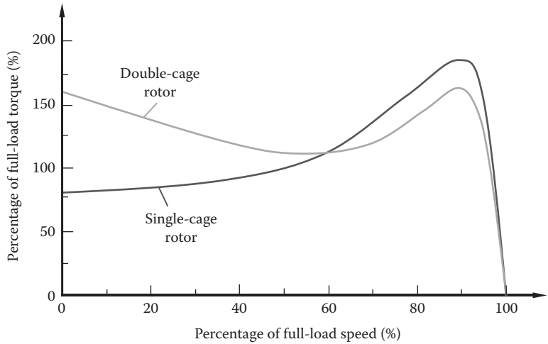
FIGURE 2.5 Comparison of torque–speed curves between double-cage and single-cage rotors.
