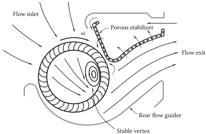
FIGURE 8.40 Cross section and flow pattern of a cross-flow fan.
