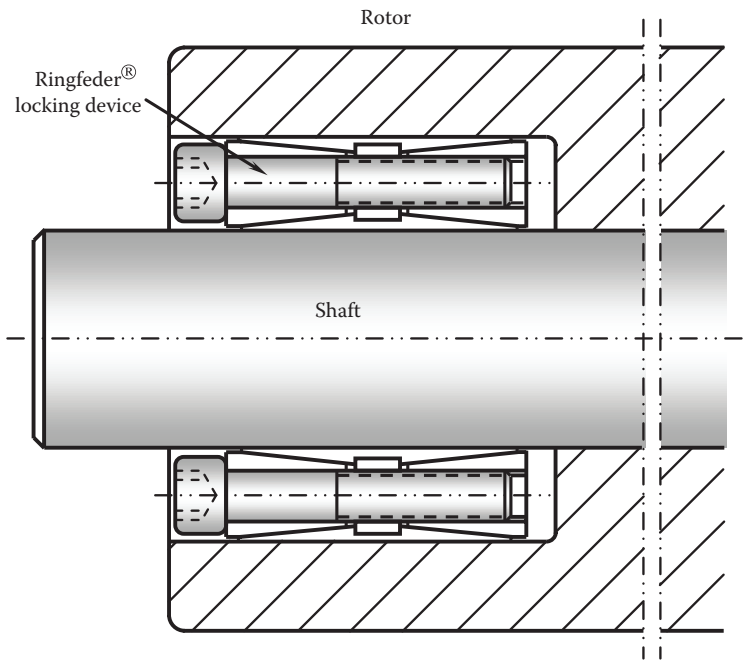
FIGURE 2.40 Keyless connection between shaft and rotor/hub using Ringfeder® locking device.
