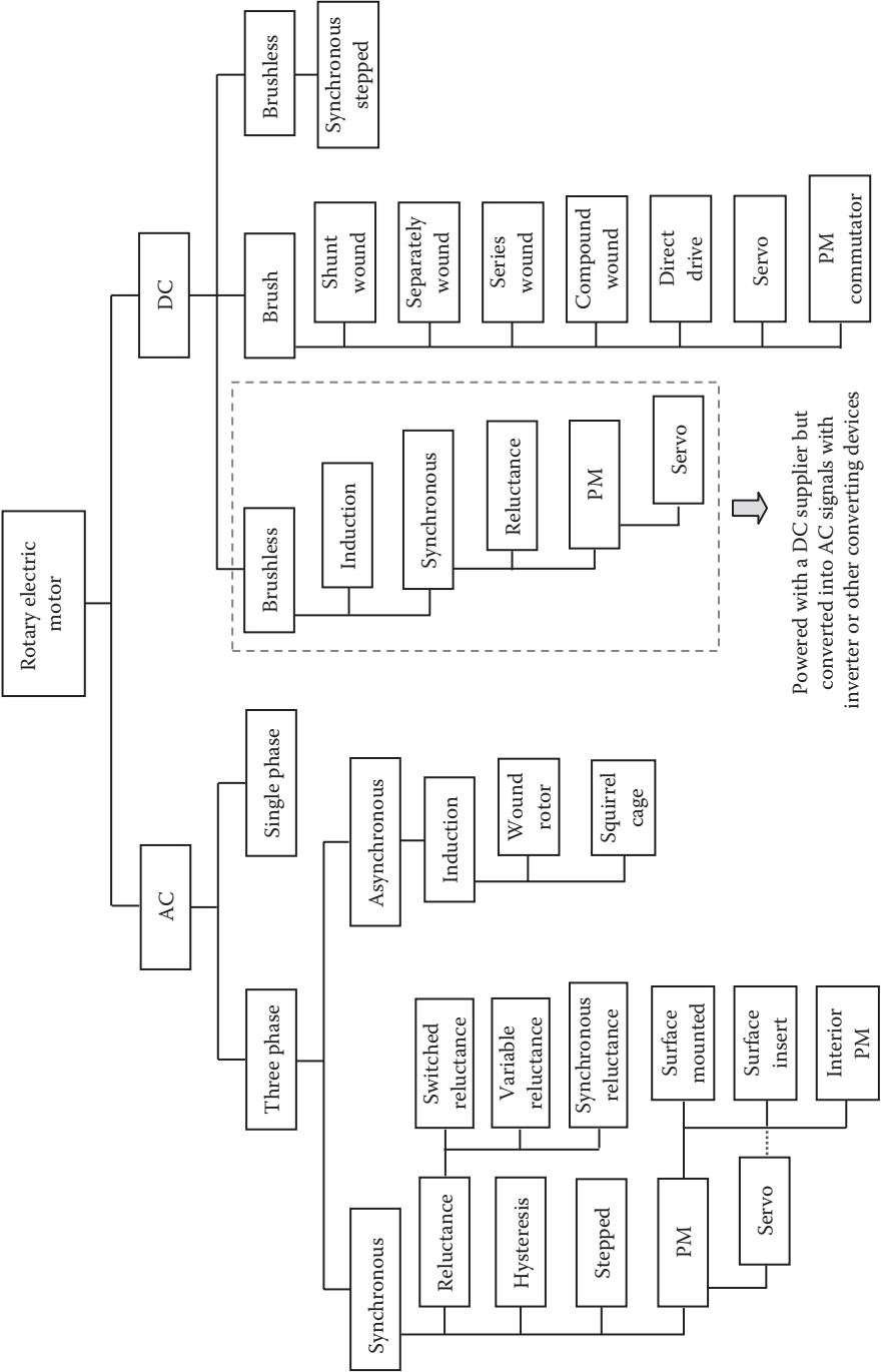
FIGURE 1.27 The classification of rotary electric motors.
