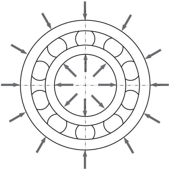
FIGURE 6.32 Due to the temperature difference on the bearing's outer and inner rings as a result of motor cooling, shrinkage occurs on the outer ring and expansion on the inner ring.
