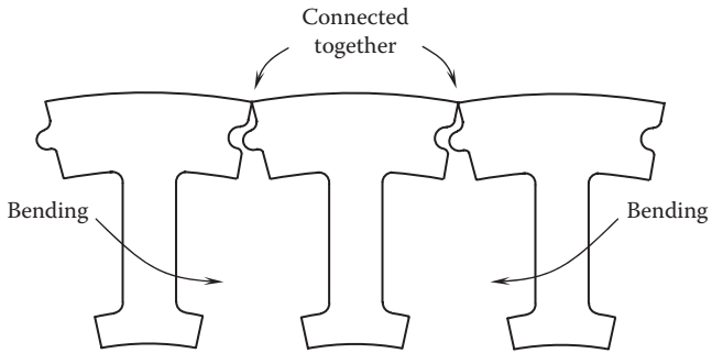
FIGURE 4.8 Punched segmented laminations are connected together at the outer tips of the laminations.
