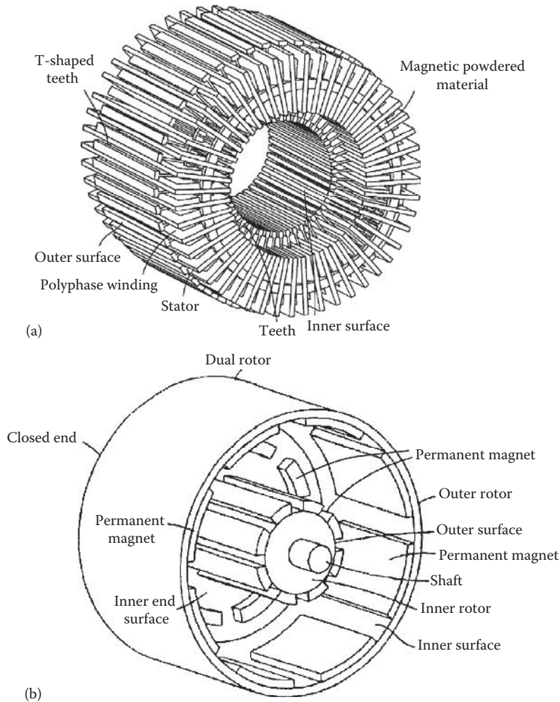
FIGURE 12.4 Dual-rotor, toroidally wound SPM motors: (a) stator and (b) dual rotor (U.S. Patent 6,924,574) [12.11]. (Courtesy of the U.S. Patent and Trademark Office, Alexandria, VA.)
