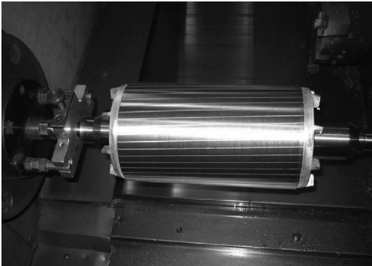
FIGURE 2.27 Machining the outer surface of a casted rotor with a CNC.
