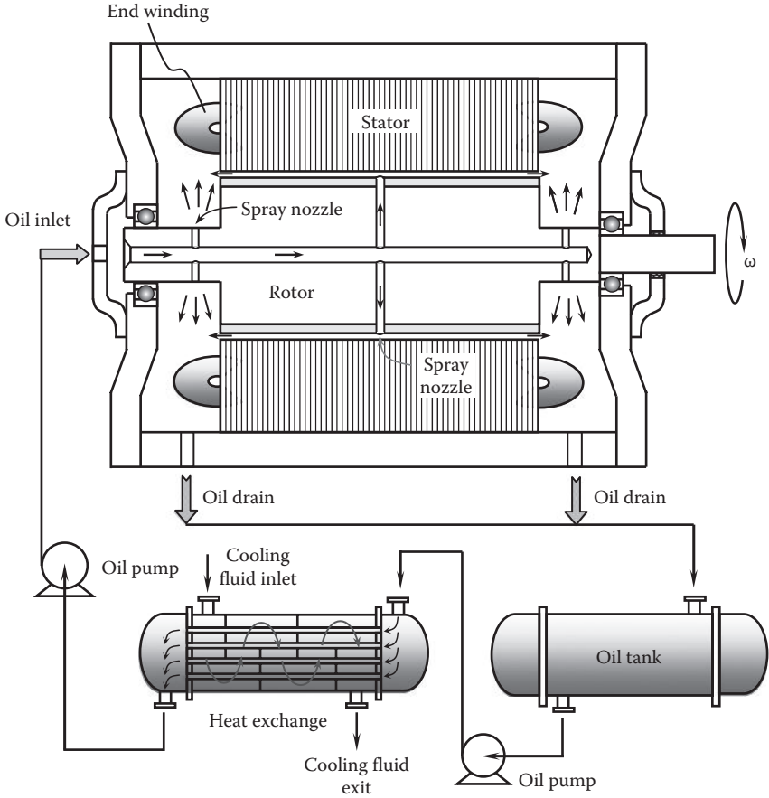
FIGURE 8.47 The internal spray cooling system by utilizing rotor centrifugal force.
