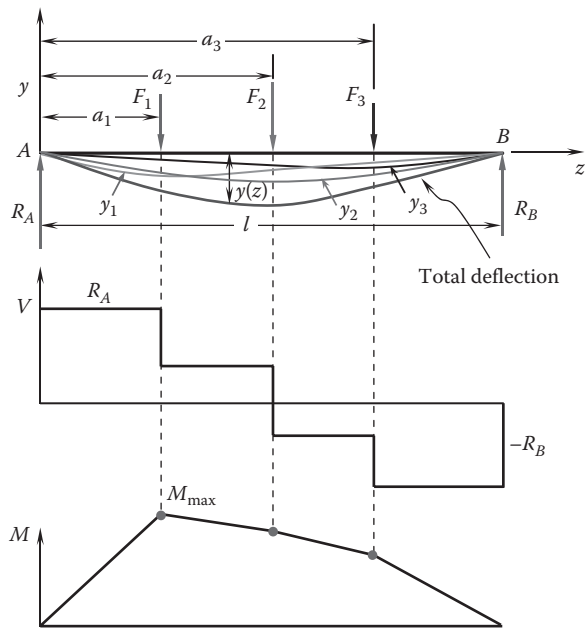
FIGURE 3.14 Deflection of a shaft subjected to multitransverse forces. The total deflection y(z) is the superposition of each deflection y_i(z) , corresponding to each transverse force.
