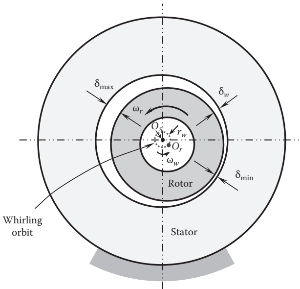
FIGURE 9.13 A general form of cylindrical circular rotor whirling.
