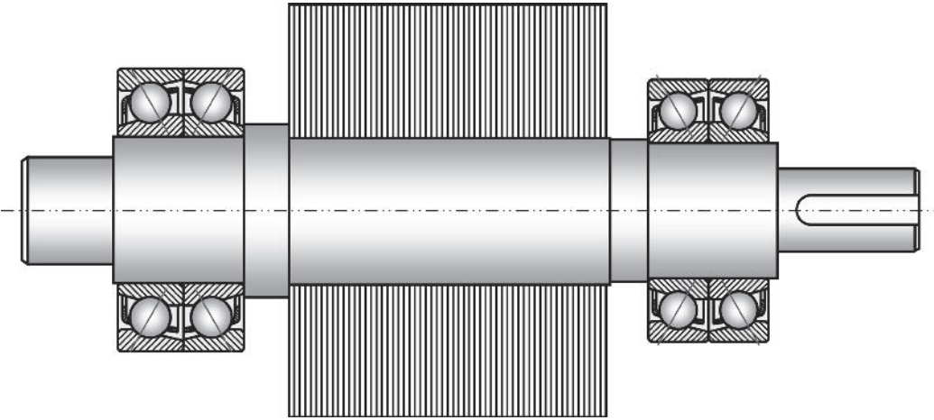
FIGURE 6.7 Matched angular contact ball bearings in a specific bearing arrangement for supporting heavy rotor.
