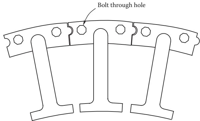
FIGURE 4.6 Patented segmented stator laminations in which both the tooth and yoke are segmented (U.S. Patent 7,816,830) [4.7]. (Courtesy of the U.S. Patent and Trademark Office, Alexandria, VA.)
