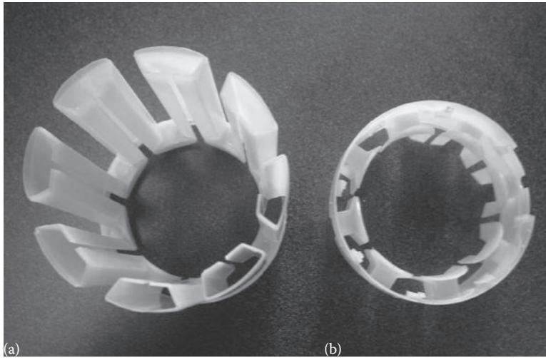
FIGURE 4.21 Molded plastic insulator: (a) main body; (b) end cap.
