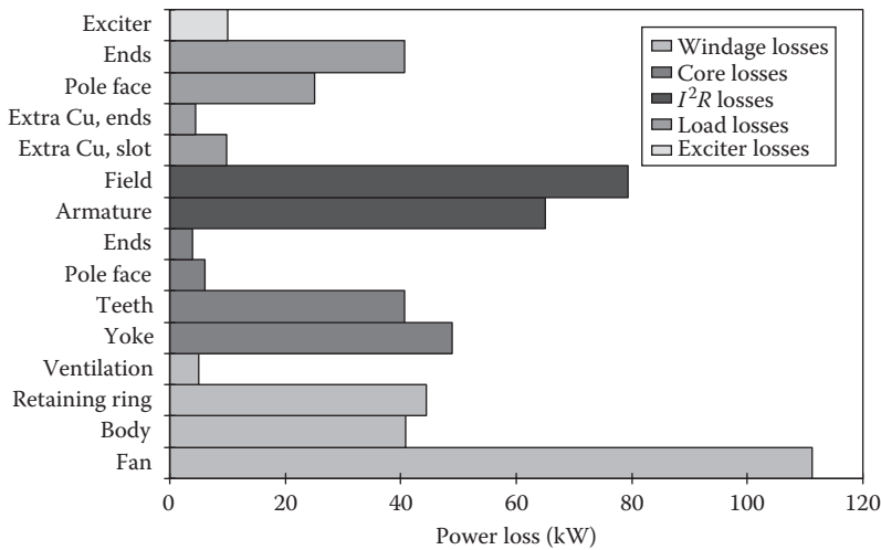
FIGURE 7.11 Various power losses for a high-power electric machine (machine B).
