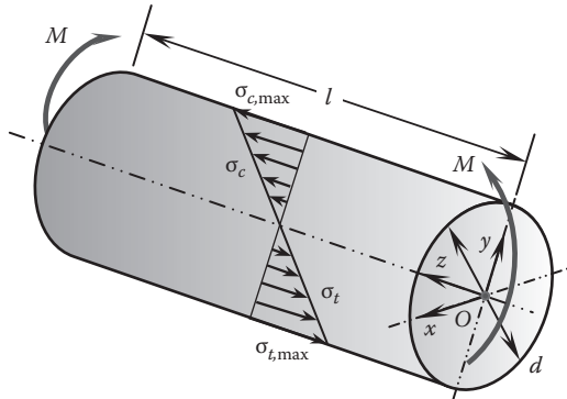
FIGURE 3.7 A single-section shaft subjected to pure bending moment.
