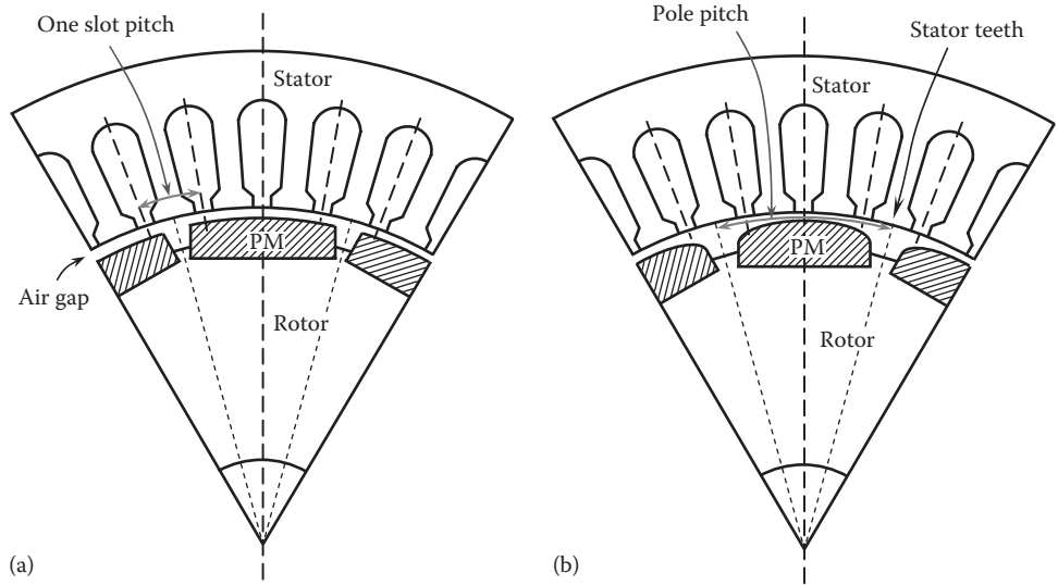
FIGURE 1.9 Surface-mounted PMs with different shapes for (a) uniform air gap and (b) nonuniform air gap.
