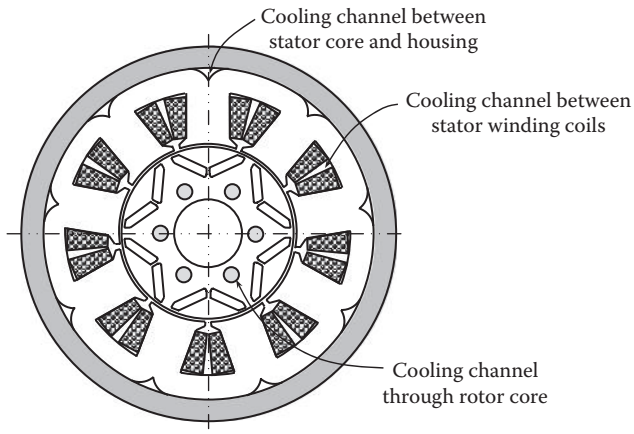
FIGURE 8.30 Combinations of different cooling channel arrangements.
