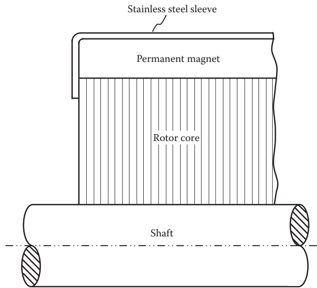
FIGURE 2.20 Bending of stainless steel sleeve at the end of rotor core for preventing magnets from shifting in the axial direction.
