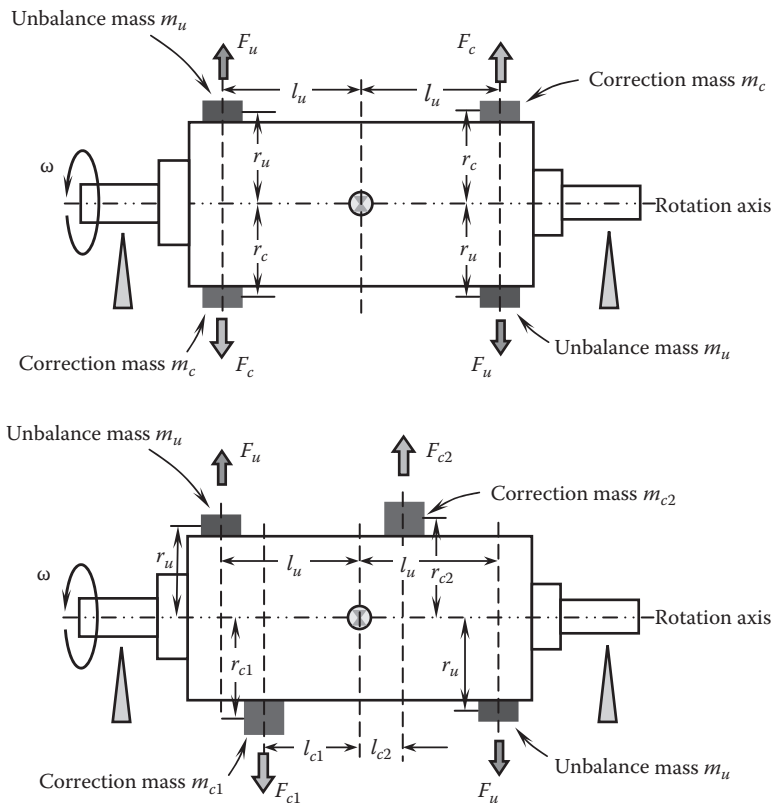
FIGURE 2.32 Balancing operation for coupled unbalance.
