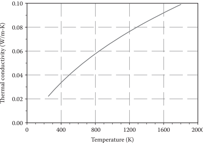
FIGURE 8.20 Thermal conductivity of air as a function of temperature.
