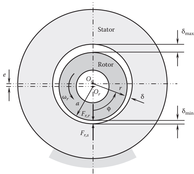
FIGURE 9.14 Asymmetrical air gap due to nonconcentric stator and rotor.
