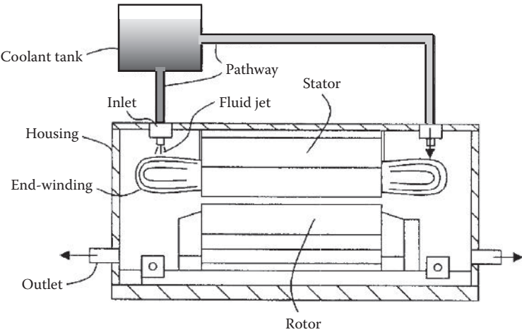
FIGURE 8.34 Cooling of end windings with an impinging jet cooling technique (U.S. Patent 6,639,334) [8.36]. (Courtesy of the U.S. Patent and Trademark Office, Alexandria, VA.)
