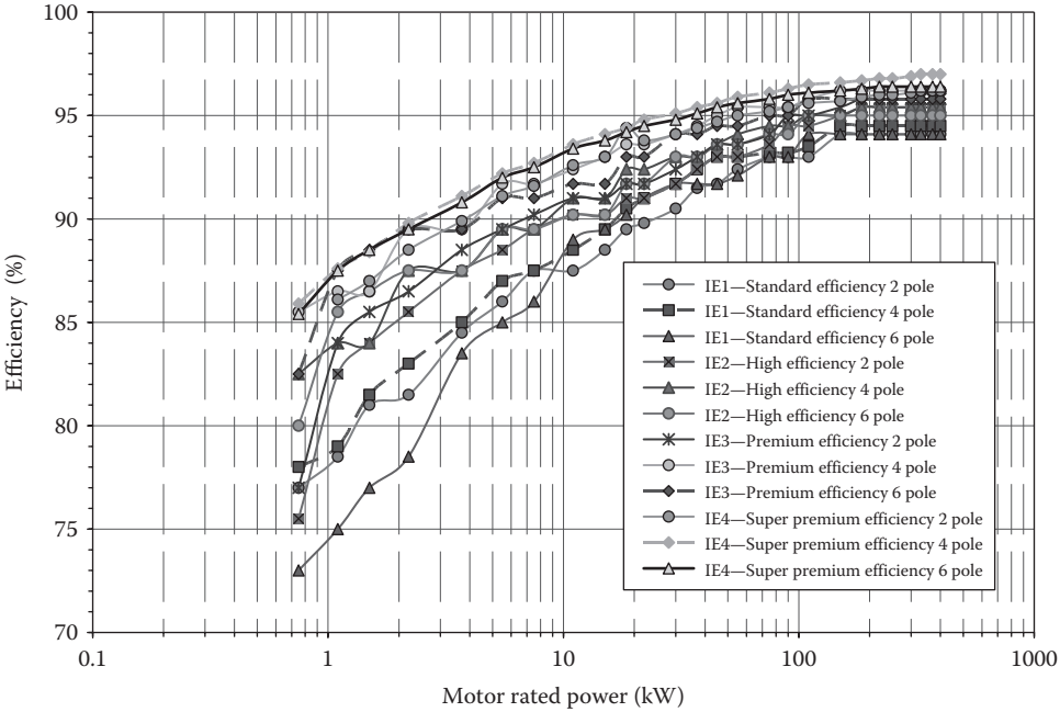
FIGURE 1.24 Comparison of four efficiency classes for electric AC motors with 60 Hz.
