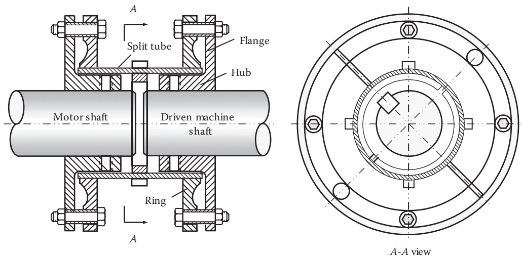
FIGURE 3.46 Semirigid coupling used in torque/power transmission. The motor shaft and driven machine shaft are indirectly connected together through two ring-shaped annular elements and split tubes for gaining a certain degree of flexibility.
