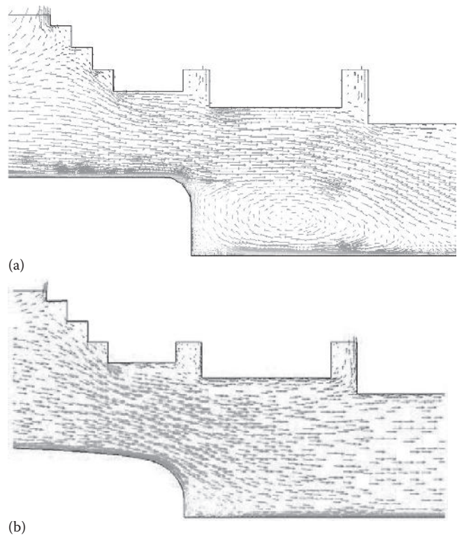
FIGURE 7.26 Reducing windage loss at the air-gap entrance by smoothing the cooling flow path: (a) original design with a large flow recirculation and (b) improved design with optimized flow path to eliminate the flow recirculation and thus reduce windage loss.
