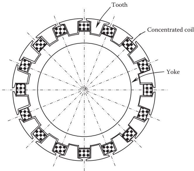
FIGURE 4.12 Integrated stator core with teeth and an internal yoke section; the teeth are positioned in the concave slots on the outer surface of the yoke, and the concentrated coils are inserted into the stator slots.
