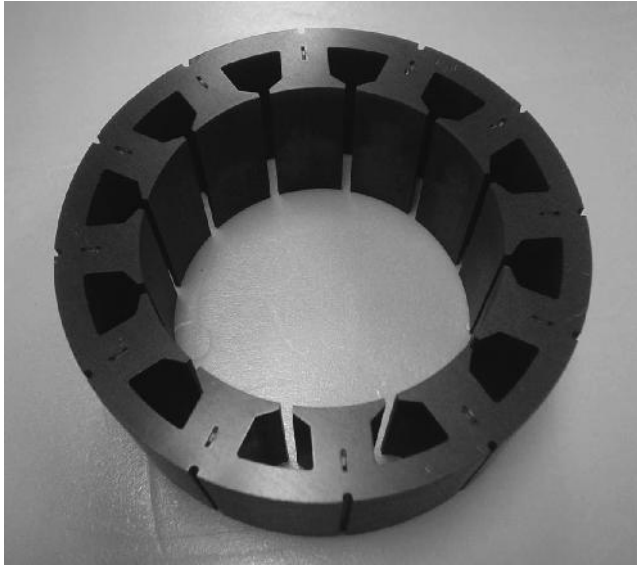
FIGURE 4.30 Stator core is made from dimpled laminations.
