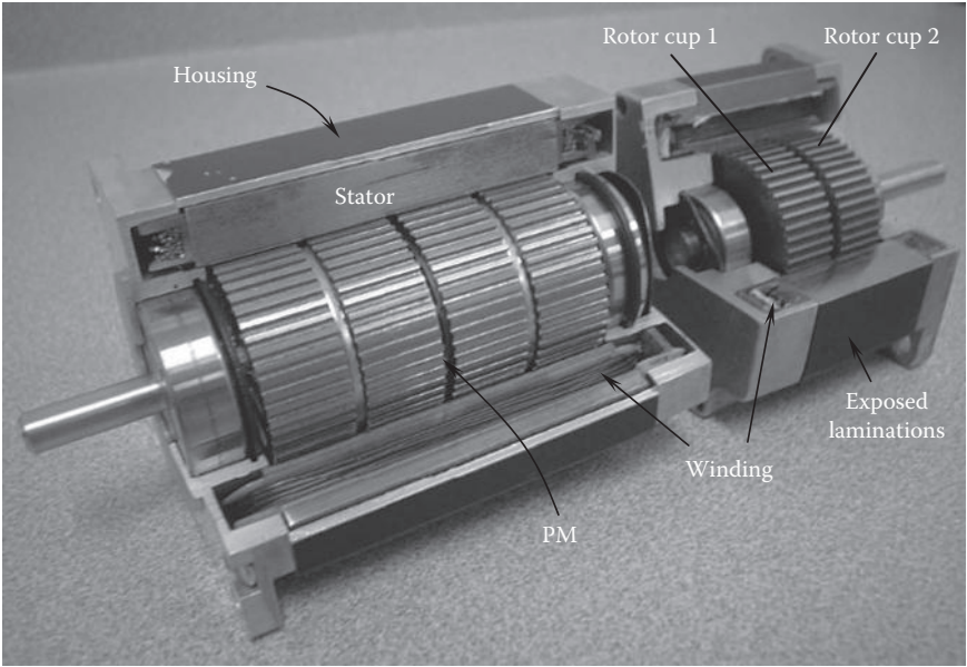
FIGURE 1.34 Structures of hybrid stepper motors, which combines features of the PM stepper and the variable reluctance stepper motors.
