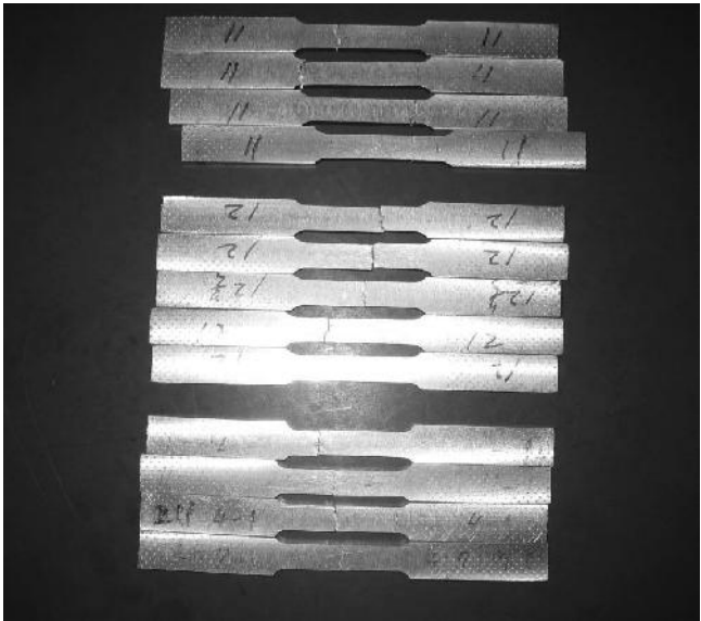
FIGURE 5.16 Testing specimens cutting from different locations of a casting housing.
