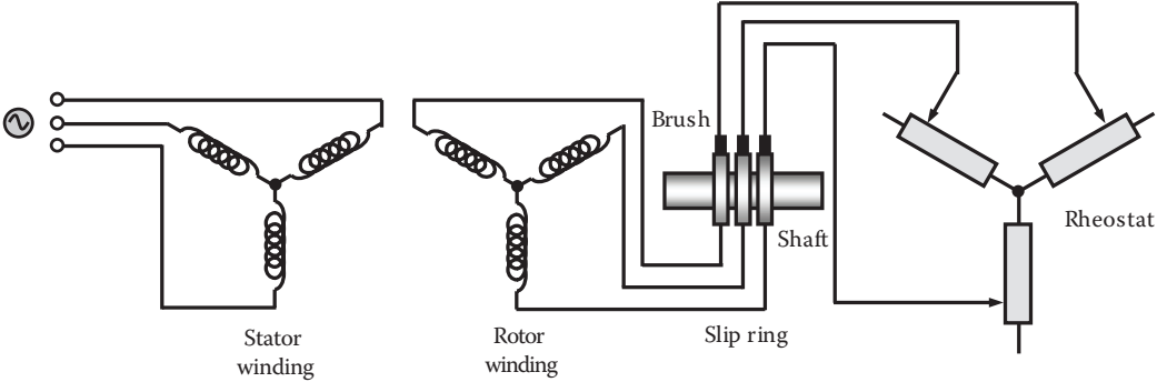
FIGURE 2.1 Wound rotor IM using slip rings and brushes to contact rotor winding and external resistances for improving motor start characteristics
