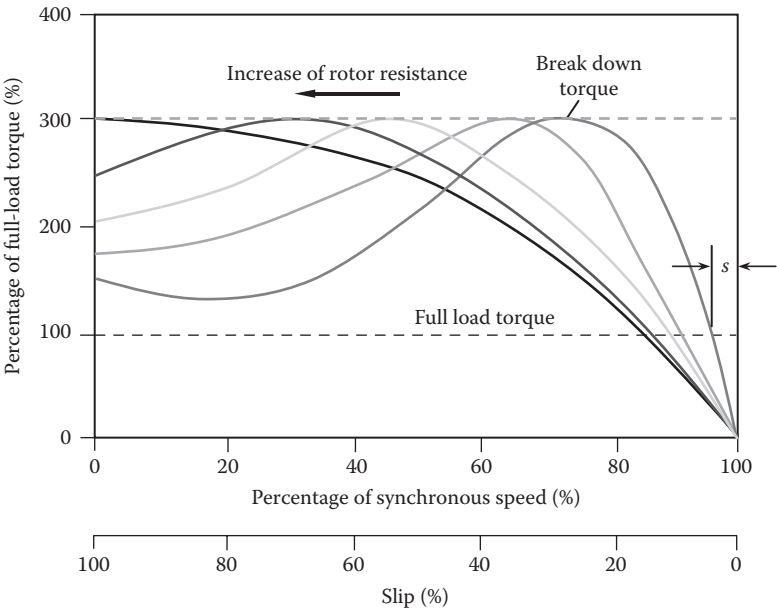
FIGURE 2.2 Variations of torque–speed characteristics of wound IMs as a function of rotor resistance. Increasing rotor resistance results in the shift of the breakdown torque toward zero speed, causing the increase of slip and starting torque and the decrease of full-load speed.
