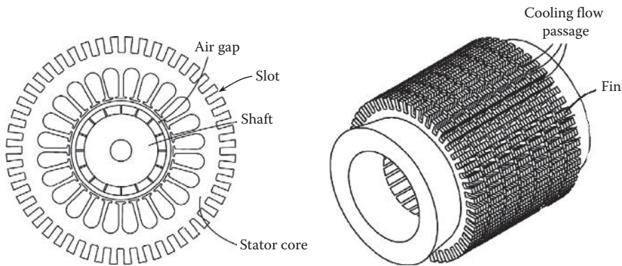
FIGURE 8.12 Stator laminations are stacked to form extending fins on the stator outer surface (U.S. Patent 8,053,938) [8.24]. (Courtesy of the U.S. Patent and Trademark Office, Alexandria, VA.)
