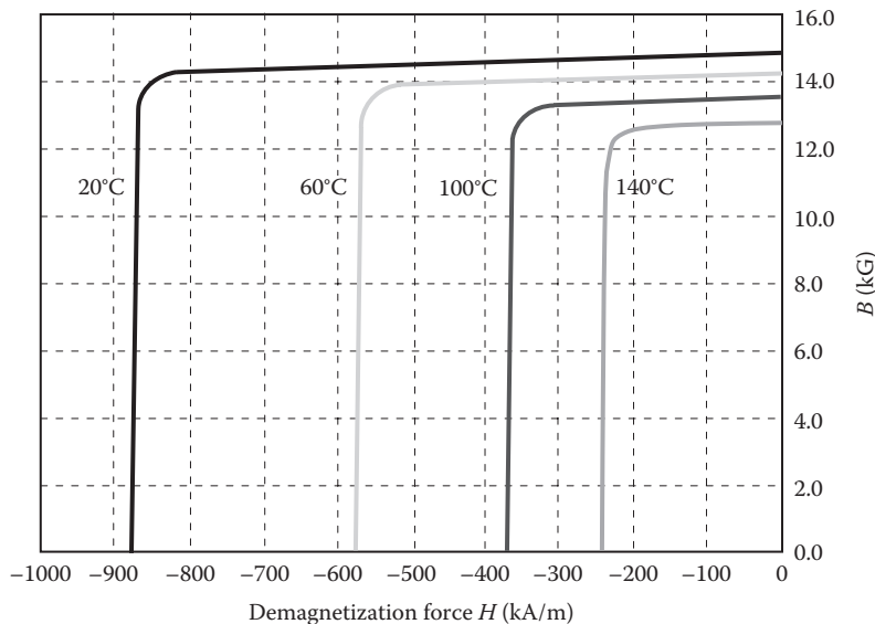
FIGURE 2.14 Impact of temperature on demagnetization characteristics of a typical Nd-Fe-B magnet.
