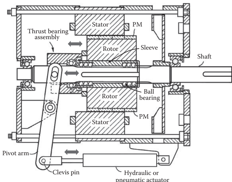
FIGURE 12.40 Structure of PM motor with adjustable axial rotor/stator alignment (U.S. Patent 6,555,941) [12.45]. (Courtesy of the U.S. Patent and Trademark Office, Alexandria, VA.)
