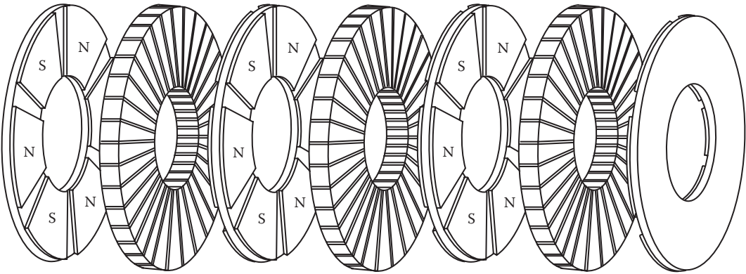
FIGURE 12.15 Perspective view of multistage of AF torus-type slotless PM motor.
