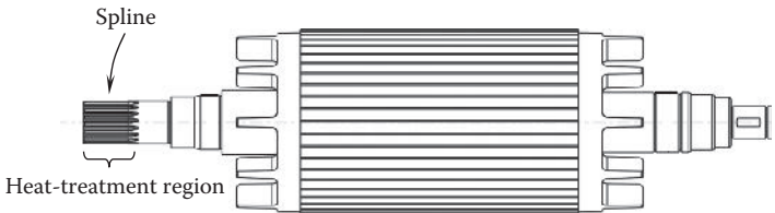
FIGURE 3.35 The spline is heat treated for increasing surface hardness, wear resistance and fatigue life.
