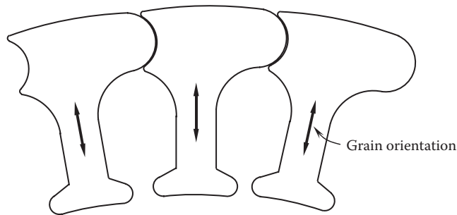
FIGURE 4.5 Patented segmented stator laminations with curved arc mating surfaces (U.S. Patent 5,212,419) [4.6]. (Courtesy of the U.S. Patent and Trademark Office, Alexandria, VA.)
