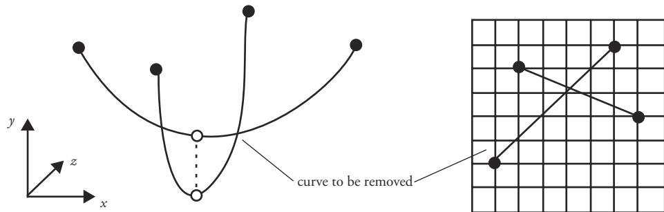
Figure 6.44 Two catenary curves supporting the same point
