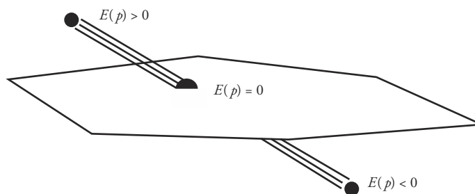
Figure 4.31 Point-plane collision
