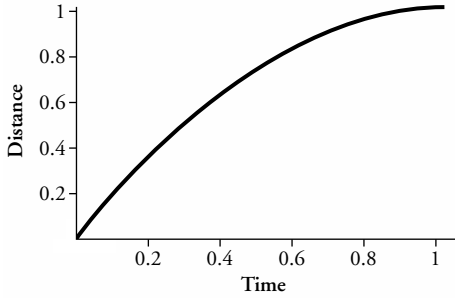
Figure 3.10 Graph of sample analytic distance-time function (2 - t)*t
