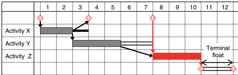
Figure 4.18 Terminal float.
