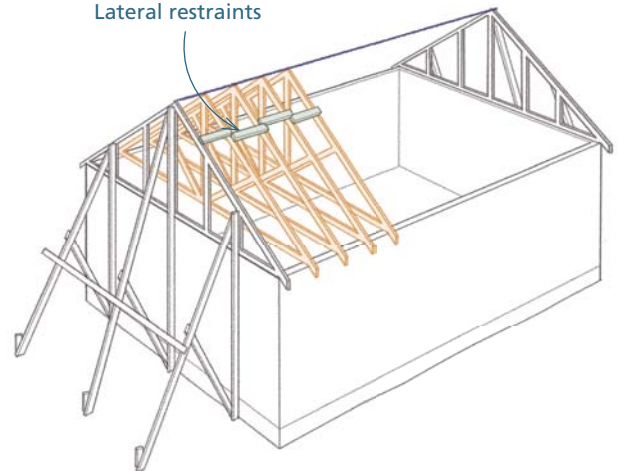
Lateral restraints
