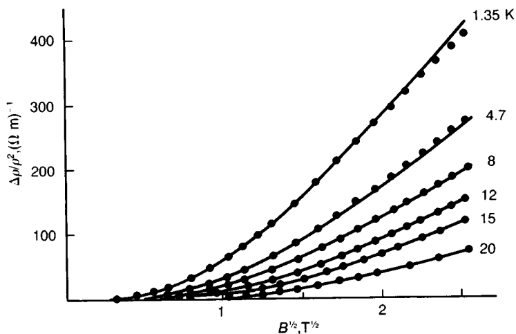
Fig. 16.7 Magnetoresistance of \text{Y}_{80}\text{Si}_{20} . The points are the experimental data and the continuous curves the theoretical fit. (After Bieri et al. 1986.)
