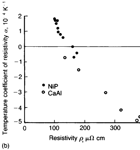
Fig. 11.2(a) The temperature coefficient of resistivity \alpha versus resistivity \rho for a range of metals and alloys to illustrate the Mooij correlation. (b) The same plot for two particular alloys. (After Howson and Gallagher 1988.)
