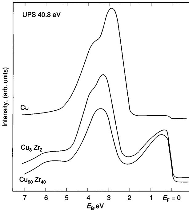
Fig. 8.5 Photoemission from crystalline Cu and Cu 3 Zr 2 and Cu 60 Zr 40 glass. (After Güntherodt et al. 1980.)
