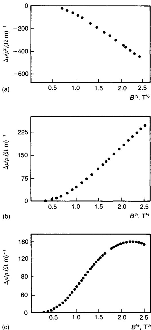
Fig. 11.10 Magnetoresistance versus B^{1/2} of (a) \text{Mg}_{80}\text{Cu}_{20} , which has only small spin-orbit scattering, so the magnetoresistance is negative at all appreciable fields; (b) \text{Cu}_{50}\text{Lu}_{50} , in which the spin-orbit scattering is strong enough to make the magnetoresistance positive throughout the field range; and (c) \text{Cu}_{50}\text{Y}_{50} , where the spin-orbit scattering is of moderate strength so that the magnetoresistance starts positive, reaches a maximum and would ultimately go negative at high enough fields. (The ordinates here are \Delta\rho/\rho^2 = -\Delta\sigma and so have the dimensions of conductivity.) (After Bieri et al. 1986.)
