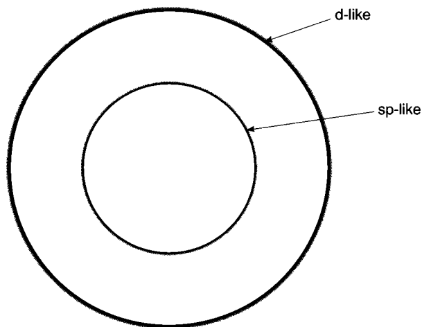
Fig. 8.6 Fermi surface of a disordered metal with s- and d-like electrons. All the states inside the d-like surface are occupied by d-like electrons and the s-like electrons are accommodated inside the s-like sphere. The surfaces will not be sharp because of the short mean free path of the electrons.
