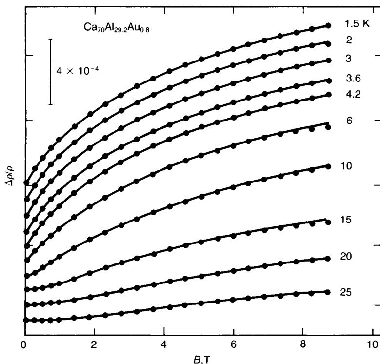
Fig. 16.12 Normalised magnetoresistance of \text{Ca}_{70}\text{Al}_{29.2}\text{Au}_{0.8} at different temperatures. Points are from experiment; curves from the theoretical fit. (After Sahnoun 1992.)
