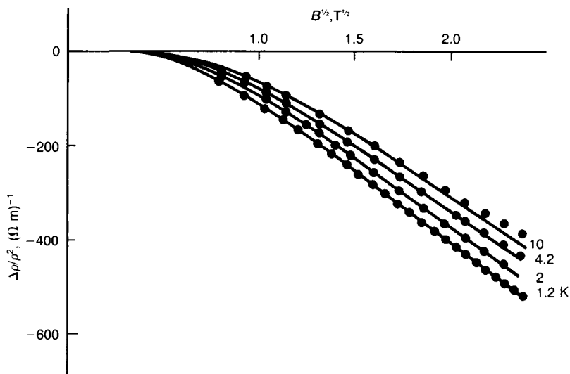
Fig. 16.3 Magnetoresistance of \text{Mg}_{80}\text{Cu}_{20} . The points are the experimental data and the continuous curves the theoretical fit. (After Bieri et al. 1986.)
