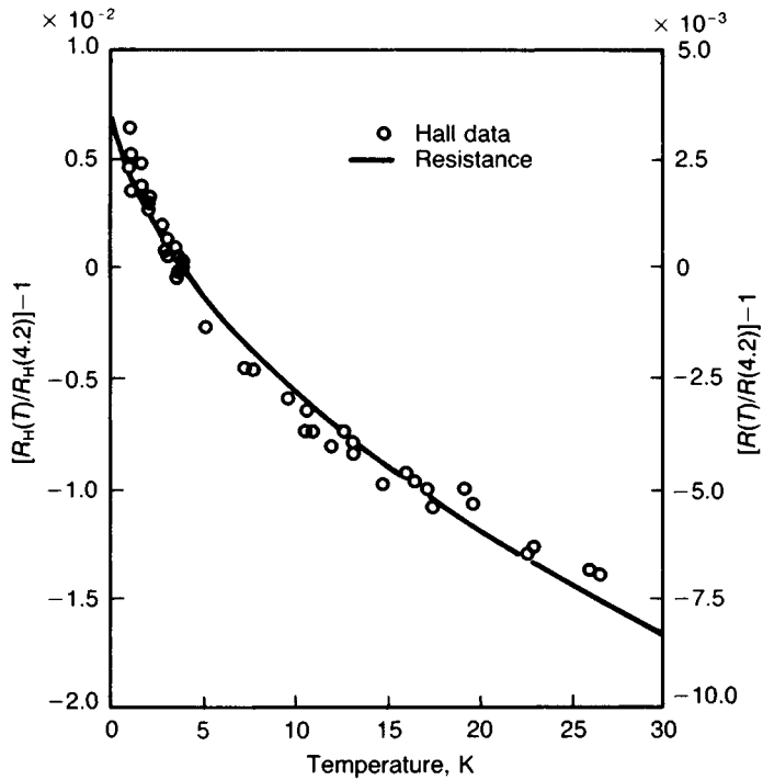
Fig. 14.3 The variation with temperature of the Hall coefficient of a Cu-Ti alloy compared with the variation to be expected from the resistivity due to the enhanced electron interaction. (After Drewery and Friend 1987.)
