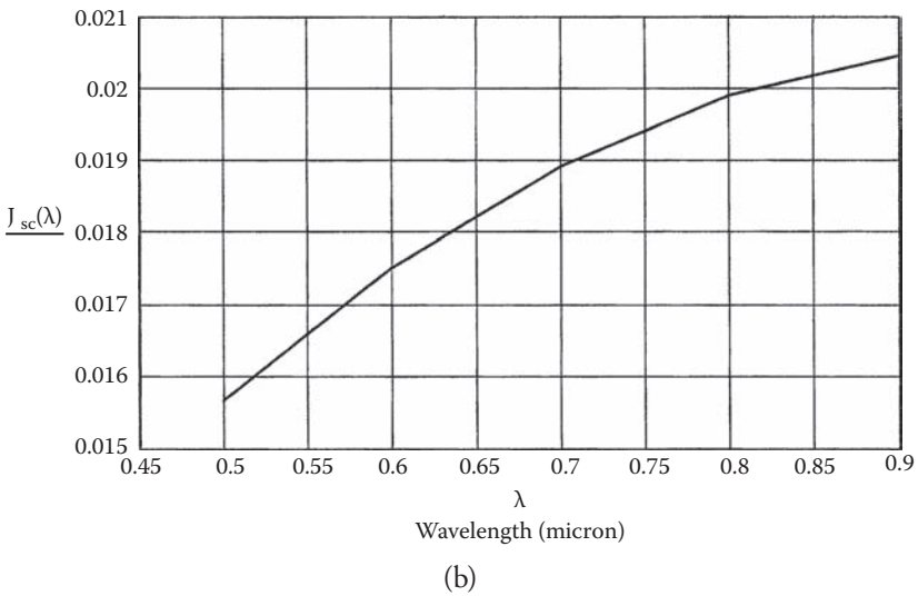
Figure 2.9 Short-circuit current as a function of wavelength for an absorption constant of 0.05 (a), 0.1 (b), and 0.2 (c). Continued
