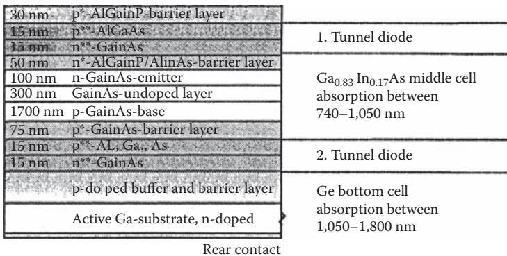
Figure 5.7 Architecture of a multijunction solar cell consisting of three photovoltaic layers, one stacked over the other, and each layer with different bandgap energy levels to absorb incident energy over various spectral regions.
