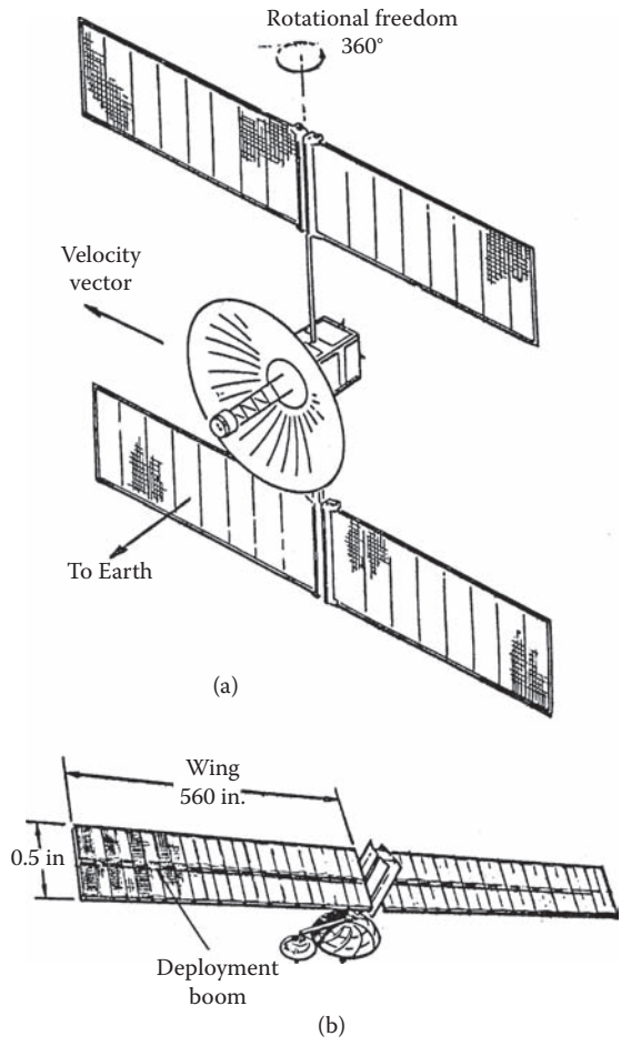
Figure 1.5 Design configurations for TV broadcast satellites consisting of (a) a 12-kW solar array and (b) a 5 kW solar array.
