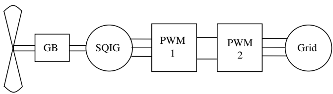
Figure 5.38 Variable-speed wind turbine with squirrel cage induction generator
