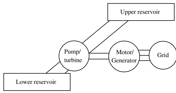
Figure 10.23 Pumped hydroelectric energy storage system
