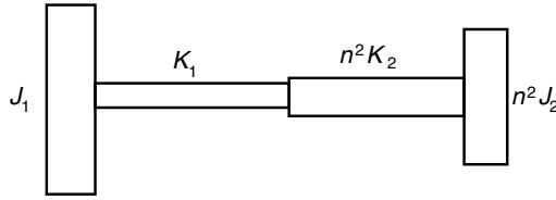
Figure 4.2 System equivalent to geared system; J , inertia; K , stiffness; n , speed ratio between the shafts; subscripts 1 and 2, gear 1 and 2
