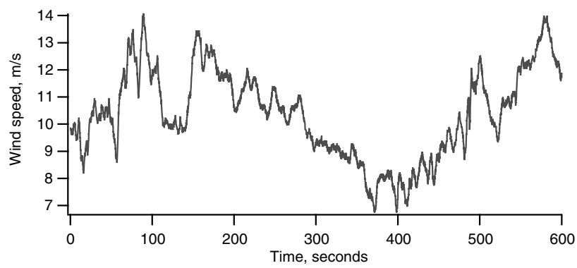
Figure 2.14 Sample wind data
