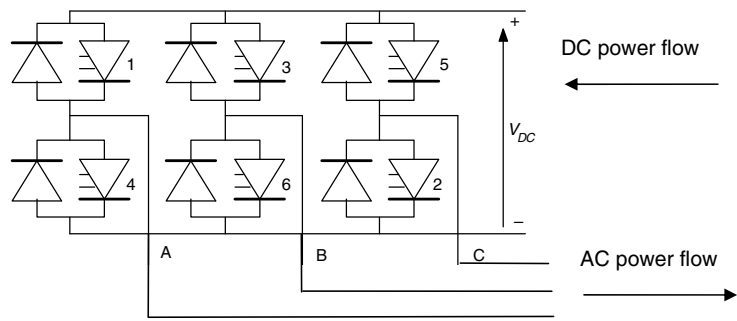
Figure 5.28 Voltage source inverter circuit
