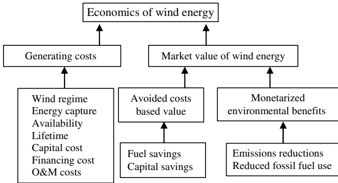
Figure 11.1 Components of wind system economics
