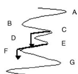
Figure 6.8 Rainflow cycle counting
