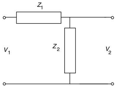
Figure 5.35 AC voltage filter; V_1 . AC voltage at filter input; V_2 . AC voltage at filter output; Z_1 resonant filter series impedance; Z_2 resonant filter parallel impedance
