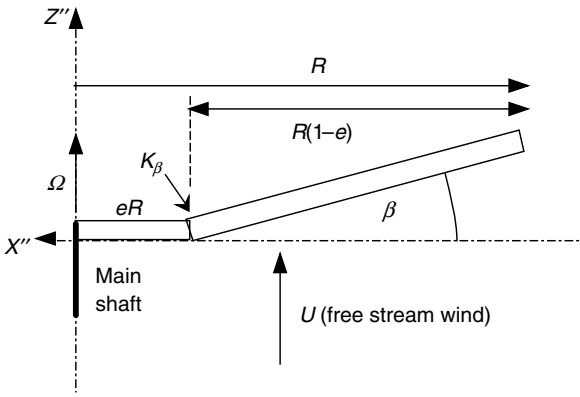
Figure 4.12 Hinge-spring model definitions
