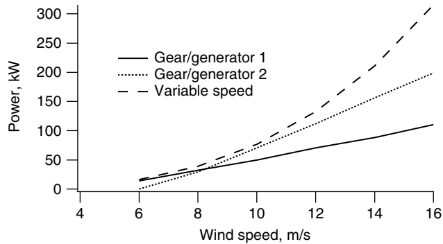
Figure 7.8 Power curves
