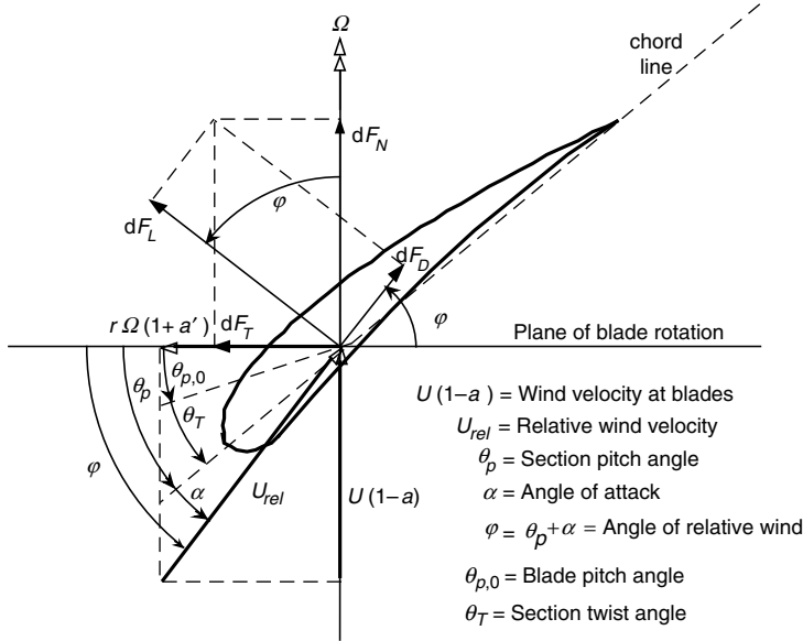
Figure 3.24 Blade geometry for analysis of a horizontal axis wind turbine. For definition of variables, see text
