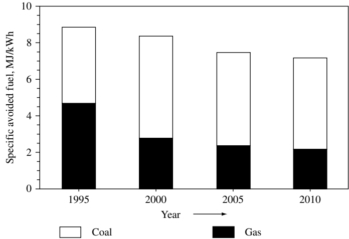
Figure 11.13 Specific avoided fuel consumption for the Netherlands (WEC, 1993) Reproduced by permission of the World Energy Council, London
