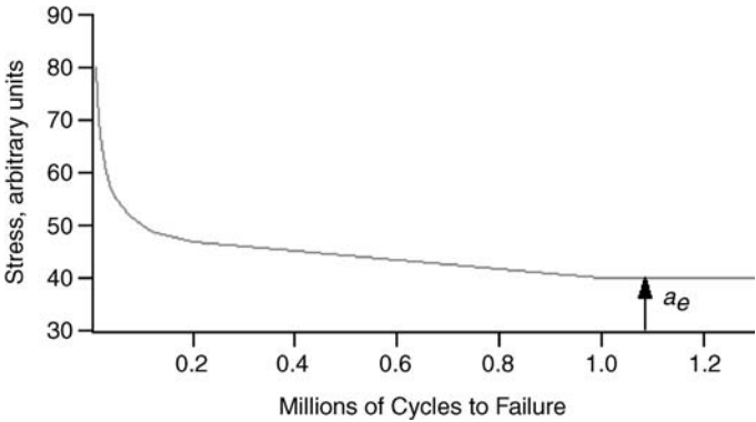
Figure 6.1 Typical S-N curve
