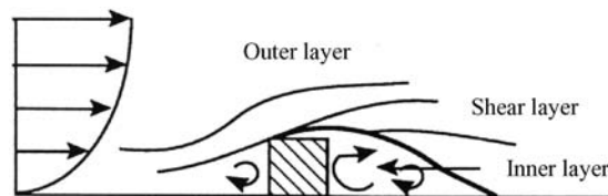
Figure 2.20 Schematic of a momentum wake (Rohatgi and Nelson, 1994). Reproduced by permission of Alternative Energy Institute
