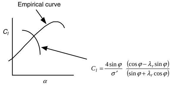
Figure 3.27 Angle of attack – graphical solution method; C_l , two-dimensional lift coefficient; \alpha , angle of attack; \lambda_r , local speed ratio; \phi , angle of relative wind; \sigma' , local rotor solidity
