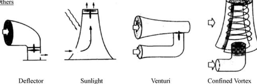
Figure 1.7 Various concepts for vertical axis turbines (Eldridge, 1980)
