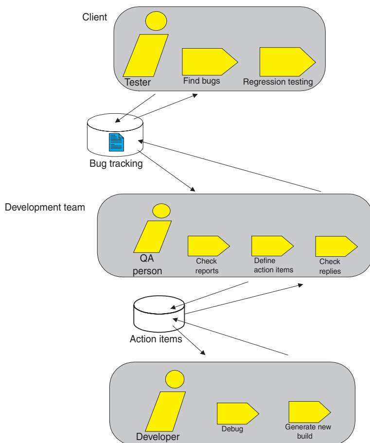
Figure 2.3 Checking error reports and developer feedback
