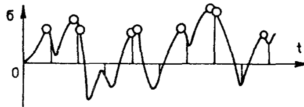
Fig. 11.4. Sampling method counting the maximum in every interval T , \circ – count.
