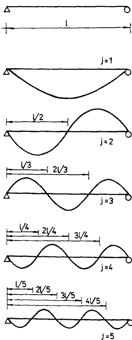
Fig. 4.1. Simply supported beam: modes of natural vibration.
