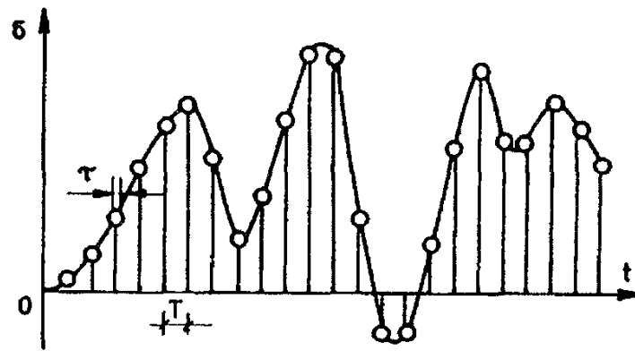
Fig. 11.3. Sampling method, T < 1/(2f) , \tau \leq T/50 , \circ – count.
