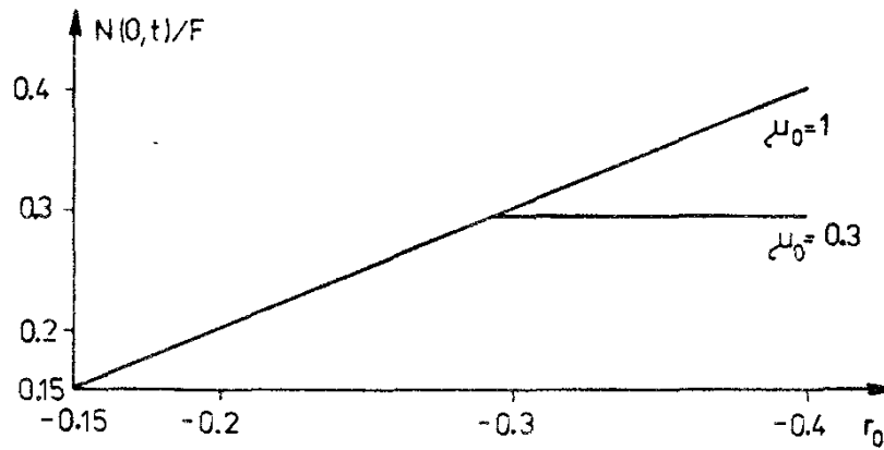
Fig. 8.11. Influence of the parameter of constant braking force r_0 for \mu_0 = 0.3 and \mu_0 = 1 on the horizontal force N(0, t) at the fixed bearing.
