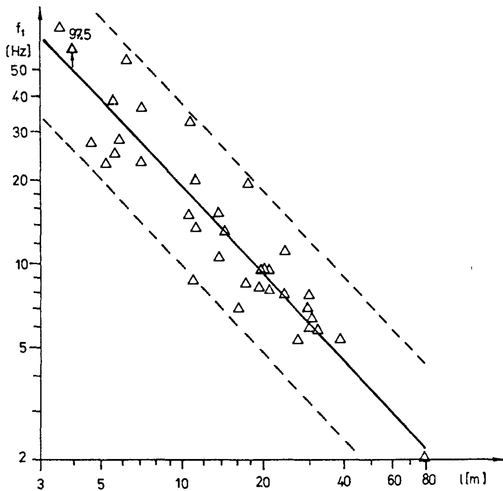
Fig. 4.23. First natural frequency f_1 plotted against span l for steel plate girder bridges without ballast (regression coefficients are in Table 4.7).
