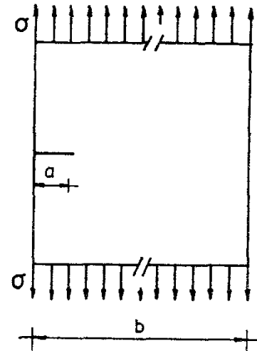
Fig. 13.7. Asymmetrical crack in a plate at normal stress, valid for a/b < 0.7 :
