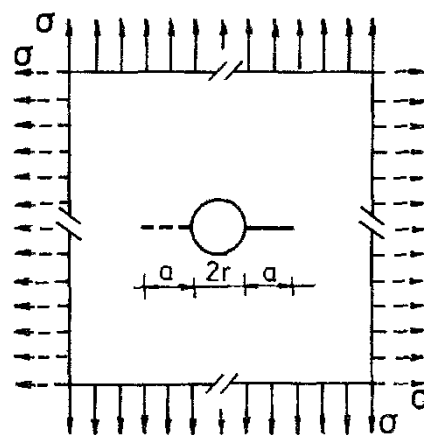
Fig. 13.9. Plate with a circular hole and with one or two cracks in uniaxial and biaxial stress state. Explanations, see the Table on page 255.
