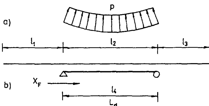
Fig. 14.21. Single-span bridge with long-welded rail, a) plan, b) elevation.
