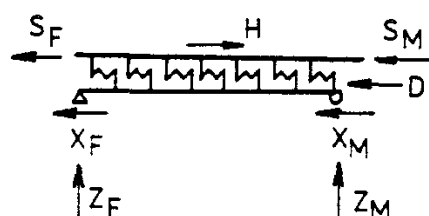
Fig. 8.17. Distribution of force H into rails S , bridge bearings X , gravel bed D . Vertical bridge reactions are Z . Indices: F – fixed bearing, M – movable bearing.
