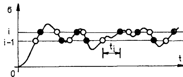
Fig. 11.5. Threshold method, \sum t_i , \circ – start of counting in the i -th class, \bullet – stop of counting in the i th class.
