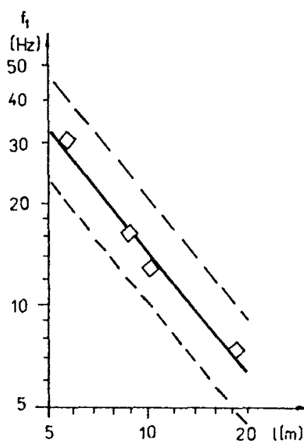
Fig. 4.25. First natural frequency f_1 plotted against span l for concrete bridges without ballast (regression coefficients are in Table 4.7).
