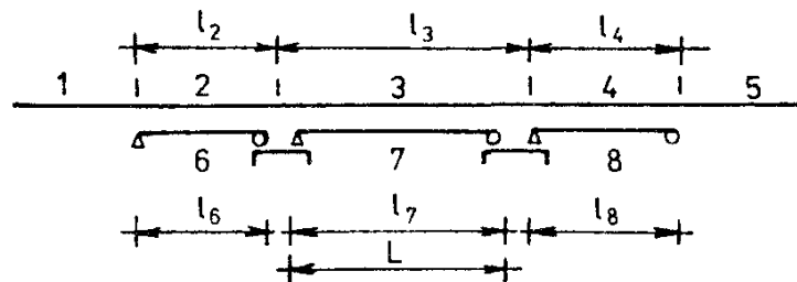
Fig. 14.7. Three-span bridge with alternate fixed and movable bearings on intermediate piers.
