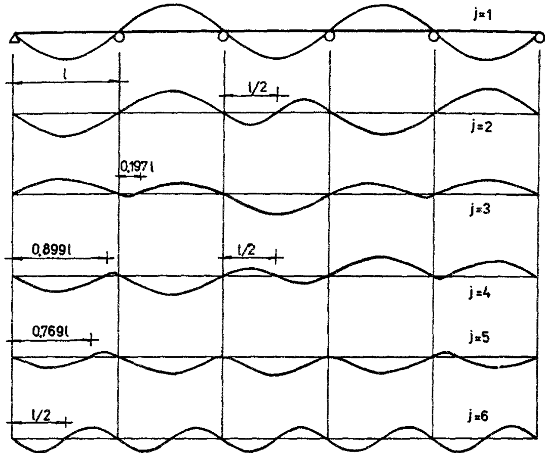
Fig. 4.12. Continuous beam of 5 equal spans: modes of natural vibration. The first dense region of natural frequencies j = 1 to 5.
