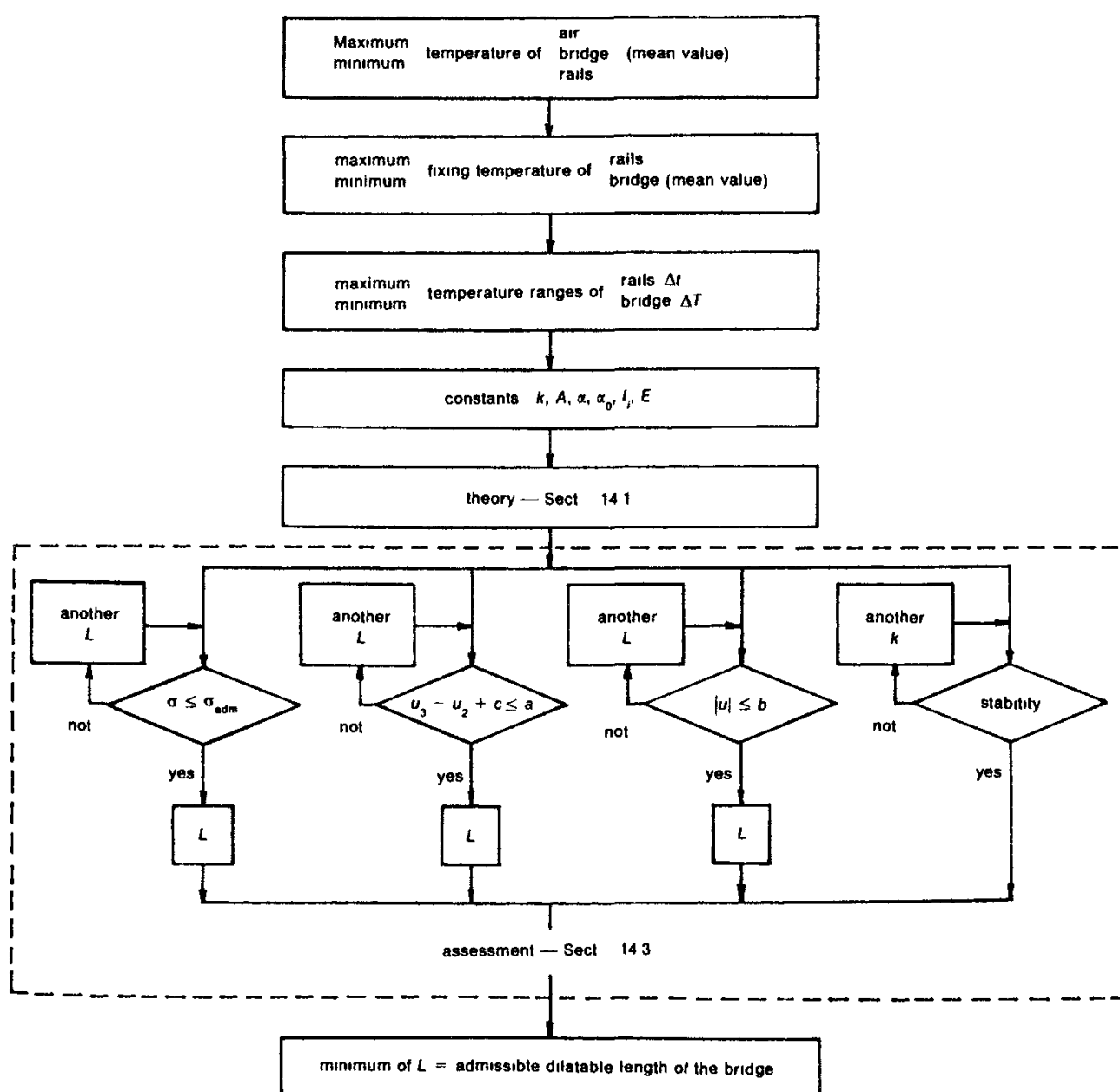
Fig. 14.16 Block diagram for the calculation of the admissible expansion length L of a bridge with long-welded rail.
