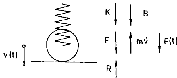
Fig. 3.7. Lumped mass and forces applied to it (positive force direction is downwards).
