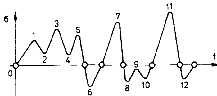
Fig. 11.6. Peak counting methods, \circ – transition of mean (basic) level.
