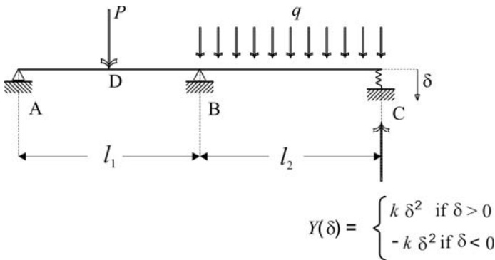
Fig. 5.15 Example 5.12: A two-span linearly elastic beam restrained by two rigid supports and a non-linear elastic spring
