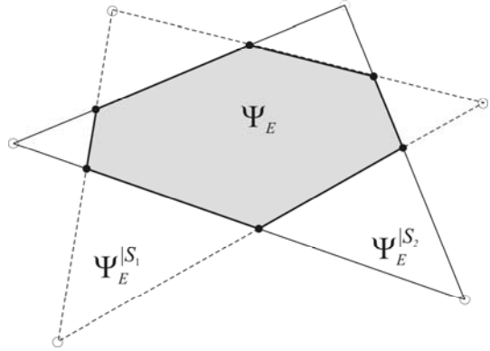
Fig. 4.10 Set of extreme points for the case of epistemic independence
