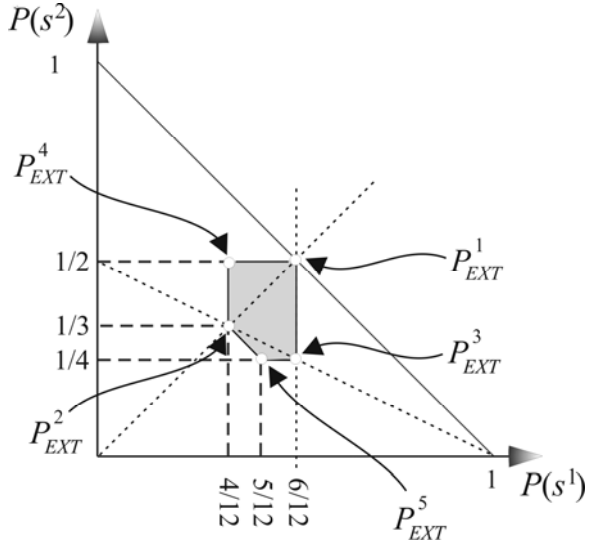
Fig. 3.20 Set \Psi^{EXT} = \Psi^E and extreme joint probability distributions in Example 3.14. Set \Psi is the triangle with extremes P_{EXT}^1, P_{EXT}^2, P_{EXT}^3
