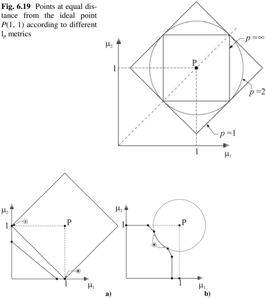
Fig. 6.20 Not unique decision with: a) p = 1 ; b) p = 2
