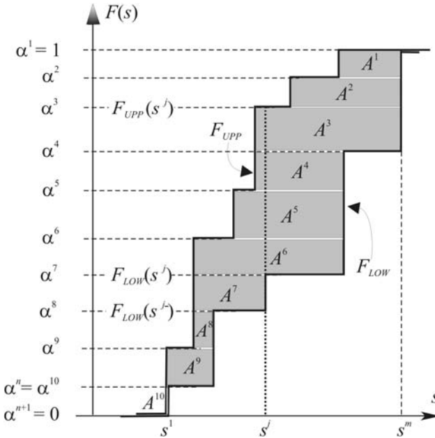
Fig. 3.25 Random set from a p-box
