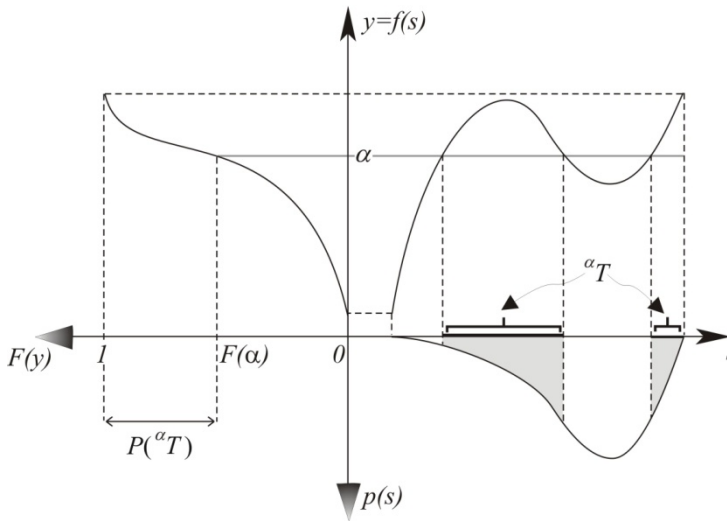
Fig. 3.21 \alpha -cuts {}^{\alpha}T of point-valued function f
