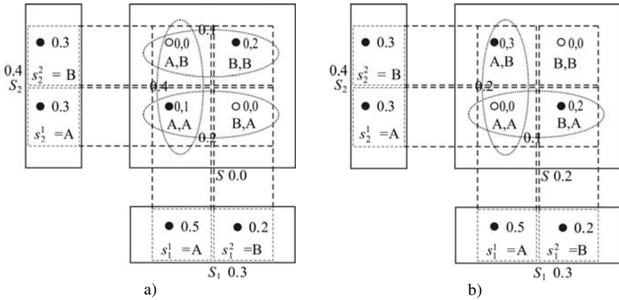
Fig. 4.12 Example 4.13: marginal random sets and random relations that: a) maximize the Plausibility; b) minimize the Belief. Numbers indicate values of probability assignment; dashed lines envelop focal elements for random relation
