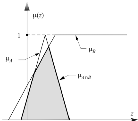
Fig. 6.13 Filtering the fuzzy measure A of the safety margin z through the fuzzy filter B (defining safety)
