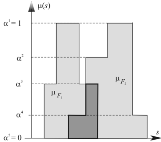
Fig. 6.10 Intersection of two normal fuzzy sets with a finite number of \alpha -cuts
