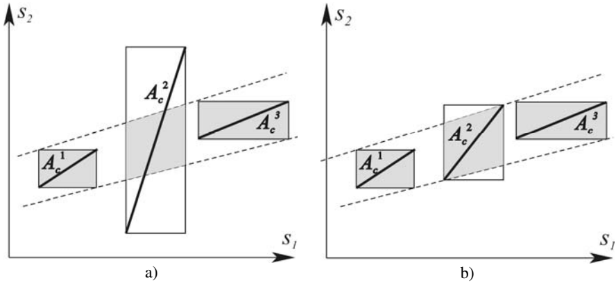
Fig. 4.17 a) Random relation made up of three focal sets for \rho_{x_1, x_2}^{(p)} = 1 ; light dashed lines indicate the widths of the marginals; b) Coherent focal sets
