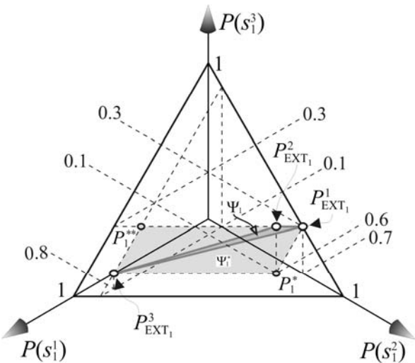
Fig. 4.7 Example 4.3: sets \Psi_1 and \Psi_1^*
