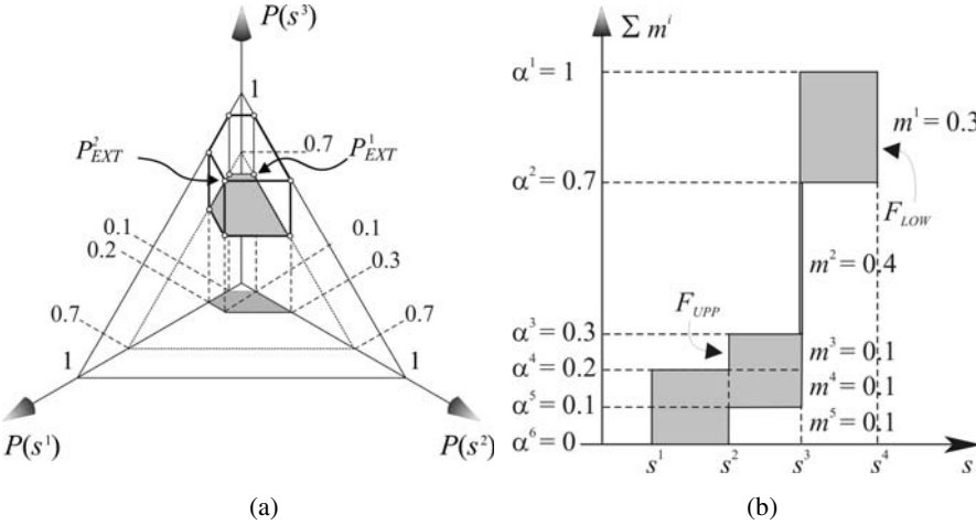
Fig. 3.26 Example 3.31: (a) extreme points in the 3-dimensional space; (b) equivalent random set
