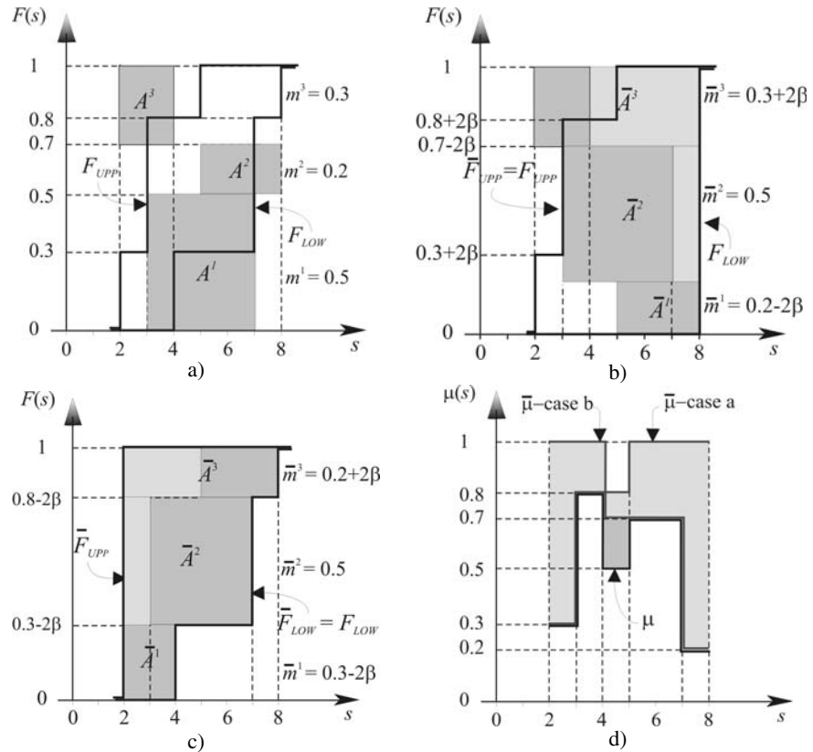
Fig. 5.9 Example 5.3: (a) Original focal elements and upper/lower CDFs; (b) consonant approximation, case (a); (c) consonant approximation, case (b); (d) contour functions of the original included random set ( \mu ) and of the inclusive consonant random sets for cases a) and b)
