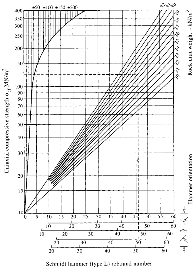
Fig. 1.2. Correlation between Schmidt hammer rebound number ( r ) and uniaxial compressive strength for different rock densities, (after Hudson and Harrison (1997), with permission)
