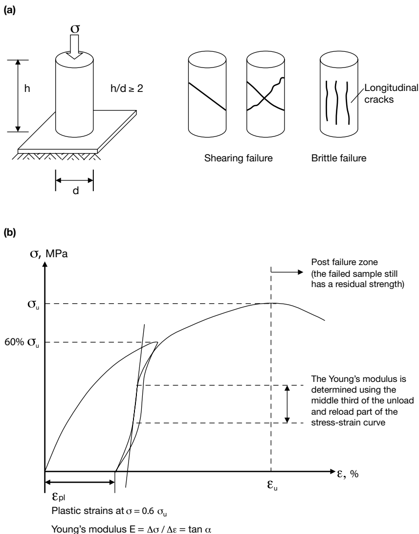
Figure 2.17 Uniaxial unconfined compression test.
