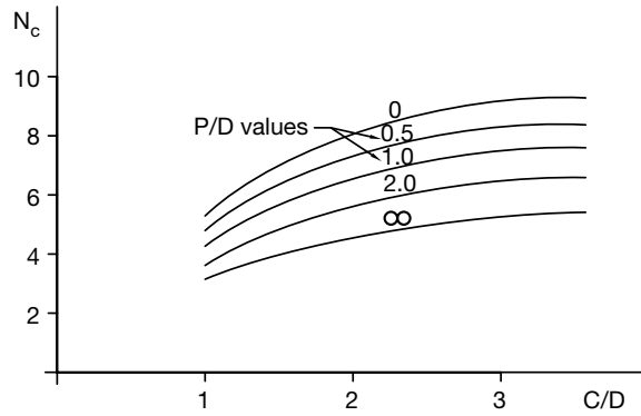
Figure 3.3 Critical stability ratio ( N_c ). (After Dimmock and Mair 2007b, used with permission from ICE Publishing and Professor Lord R.J. Mair.)
