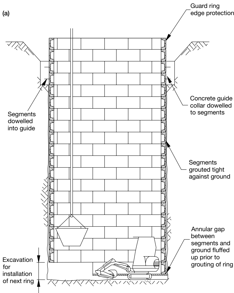
Figure 4.26 (a) ‘Underpinning’ technique for constructing shafts. (After BTS/ICE 2004, used with permission from ICE Publishing.) An example of the ‘underpinning’ technique used to construct a shaft. (Continued)
