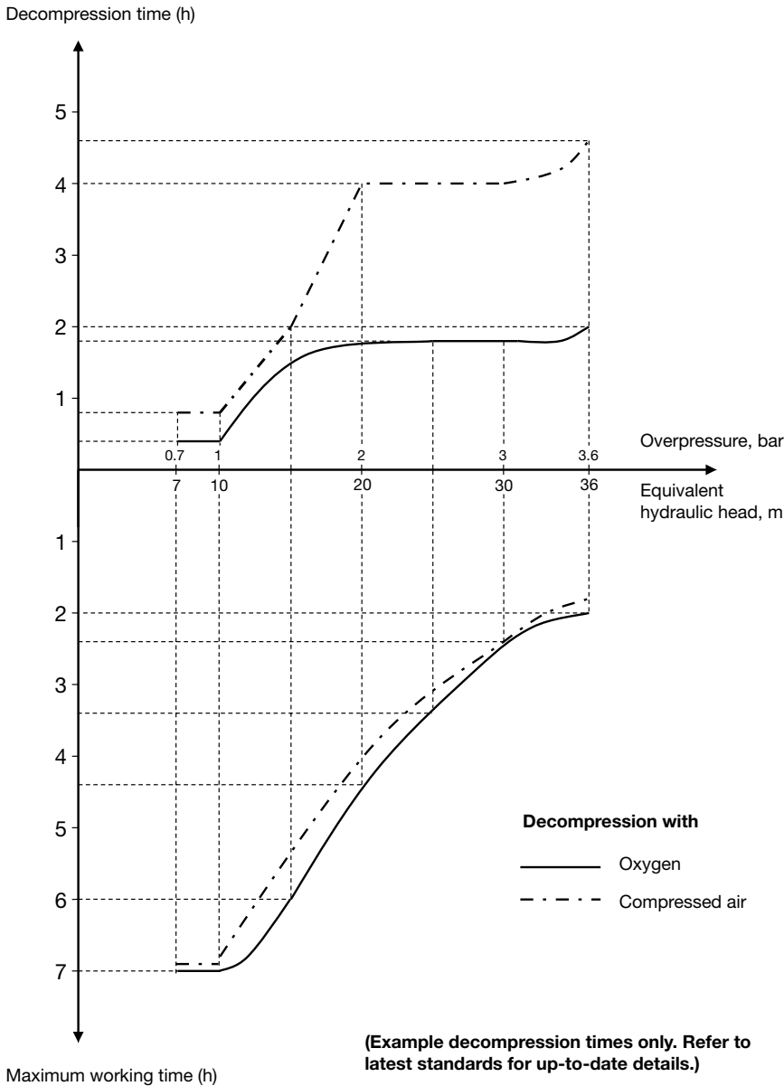
Figure 4.17 Simplified decompression times. (After Bundesgesetzblatt 2008.)
