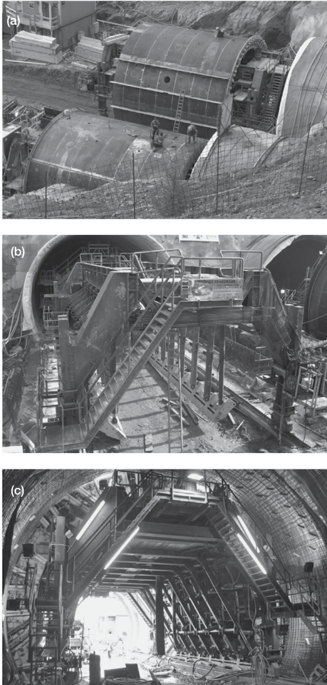
Figure 4.28 Construction of the inner lining, HKT, Germany: (a) and (b) Setting up the shuttering at the tunnel portal and (c) shuttering in the main tunnel.
