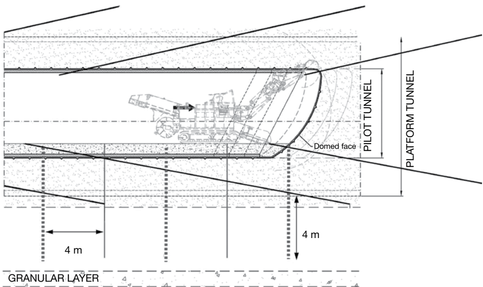
Figure 8.43 Phase 2 probing and depressurisation for the enlargement, in this case for the Platform tunnel, following the excavation of the Pilot tunnel. To confirm the existence of sufficient clay cover, the vertical probe holes extended 4 m below the invert of the Platform tunnel. The probe hole length was 8–9 m with 4 m spacing. (Graphic Credit: Crossrail Ltd., used with permission.)
