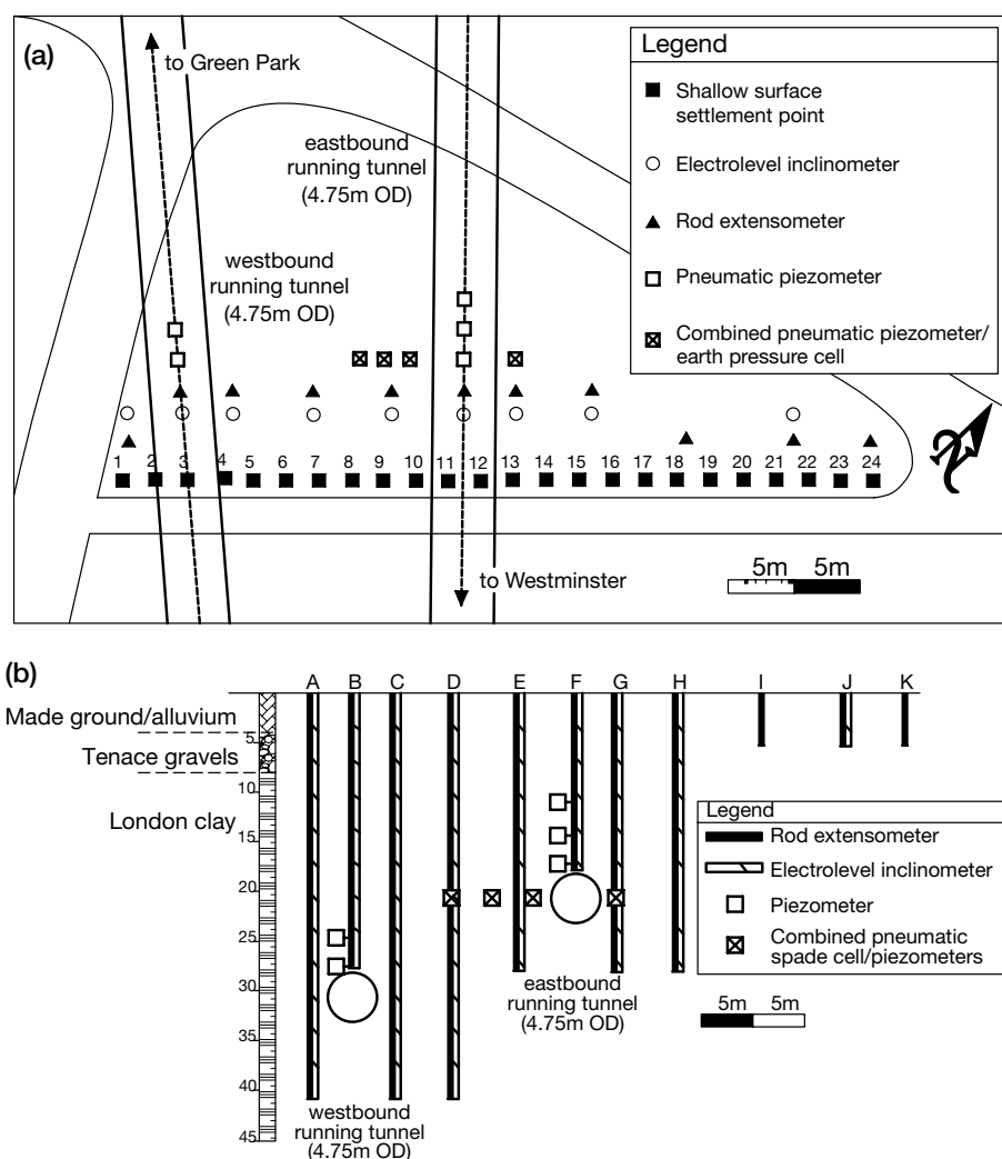
Figure 7.26 An example of the instrumentation used to monitor the ground behaviour resulting from a bored tunnel as part of the Jubilee Line Extension project on the London Underground, UK, (a) site plan and (b) instrumented cross section. (After Standing et al. 1996.)
