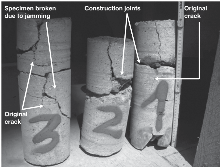
Figure 8.25 Cores, section W, Chainage 52–54.
