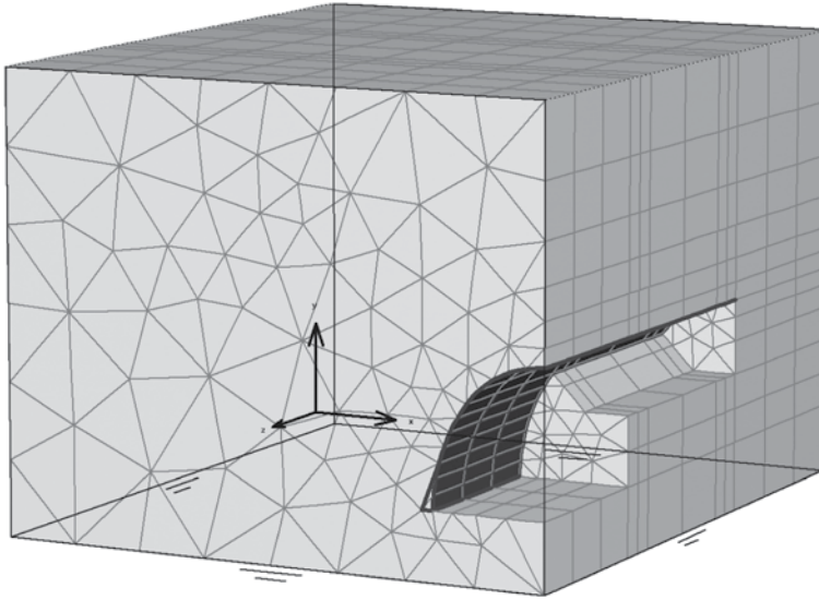
Figure 3.9 Example 3-D analysis of a tunnel being constructed using NATM, as produced using the PLAXIS 3-D® software. (Courtesy of Wilde Analysis Ltd.)
