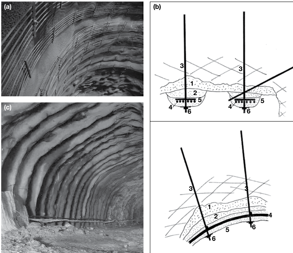
Figure 5.52 The rib reinforcement system (RRS), (a) the reinforcement bar-based ribs prior to spraying with concrete, (b) diagrams showing the RRS (see main text for description of the numbers) and (c) the final sprayed system, which can be covered with a final lining if required from an architectural point of view. (Used with permission of N. Barton.)
