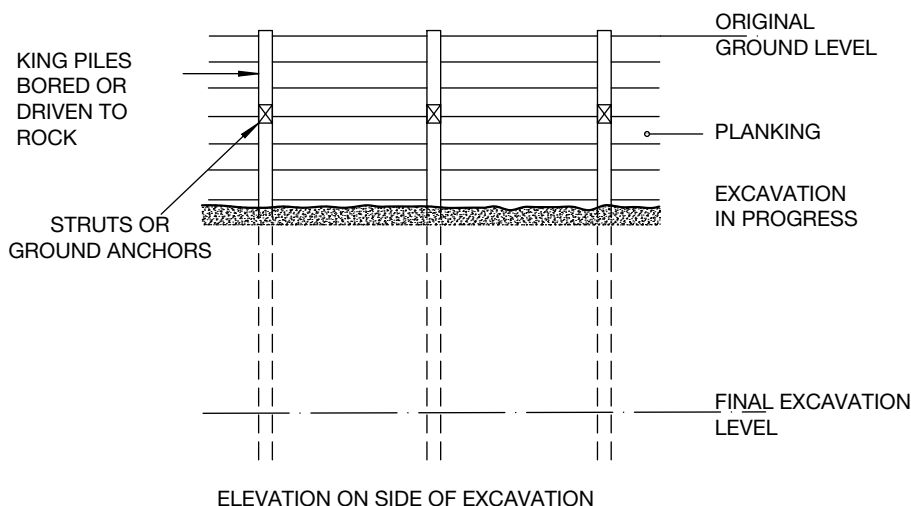
Figure 5.62 General arrangement of a king pile and poling board retaining wall. (After Megaw and Bartlett 1982, used with permission from John Bartlett.)
