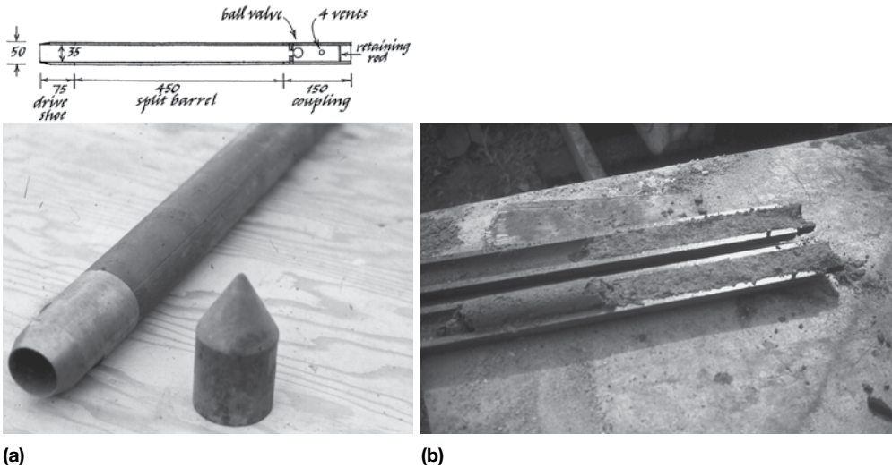
Figure 2.10 Split barrel sampler used for the SPT: (a) the open tube is used for fine-grained soils and the cone for coarse-grained soils and (b) in fine-grained soils, a sample can be obtained for visual inspection. (Courtesy of Dr. Ron Jones.)
