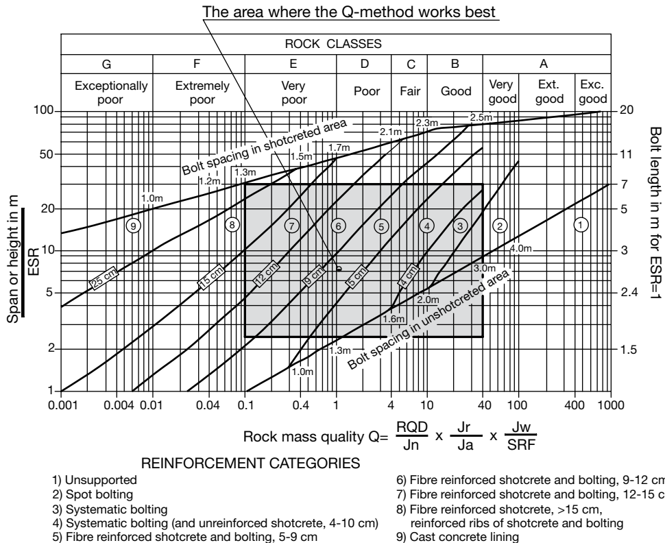
Figure 2.26 Limitations of the Q-method for rock support. Outside the shaded area supplementary methods/evaluations/calculations should be applied. (Reproduced from Palmström and Broch 2006.)
