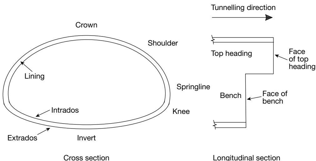
Figure 1.2 Terminology related to a tunnel cross section and longitudinal section.
