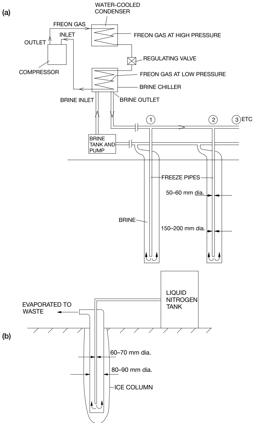
Figure 4.2 Ground freezing methods: (a) two-phase method and (b) direct process. (After Harris 1994.)
