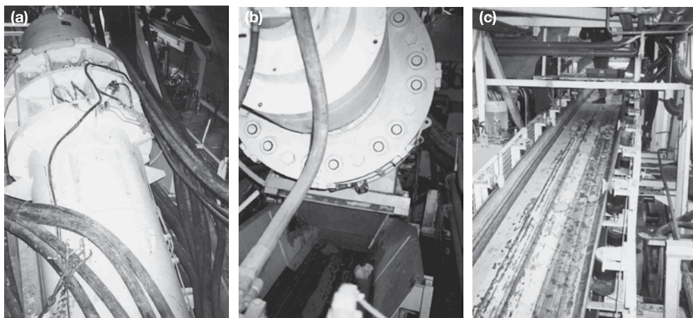
Figure 5.32 (a) and (b) The head of the Archimedeal screw and (c) conveyor system used in an EPBM on the Line B metro extension project in Toulouse, France (ground conditions: Toulouse Molasses, i.e. a hard sandy clay with pockets and lenses of very dense sand).
