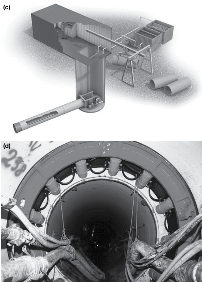
Figure 5.91 (Continued) (c) schematic representation of a microtunnelling operation (Courtesy of Herrenknecht.) and (d) an intermediate jacking station. (Courtesy of Herrenknecht AG/NoDig Media Services.)
