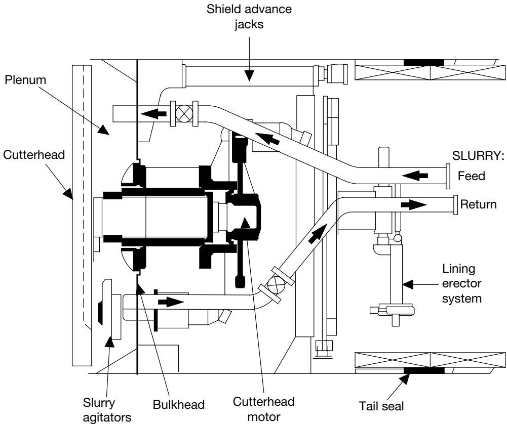
Figure 5.26 Longitudinal section through a slurry TBM. (After Jacob 1976).
