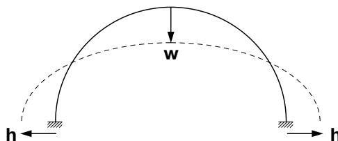
Figure 7.18 Divergence in combination with roof settlement. (Rokahr et al. 2002.)
