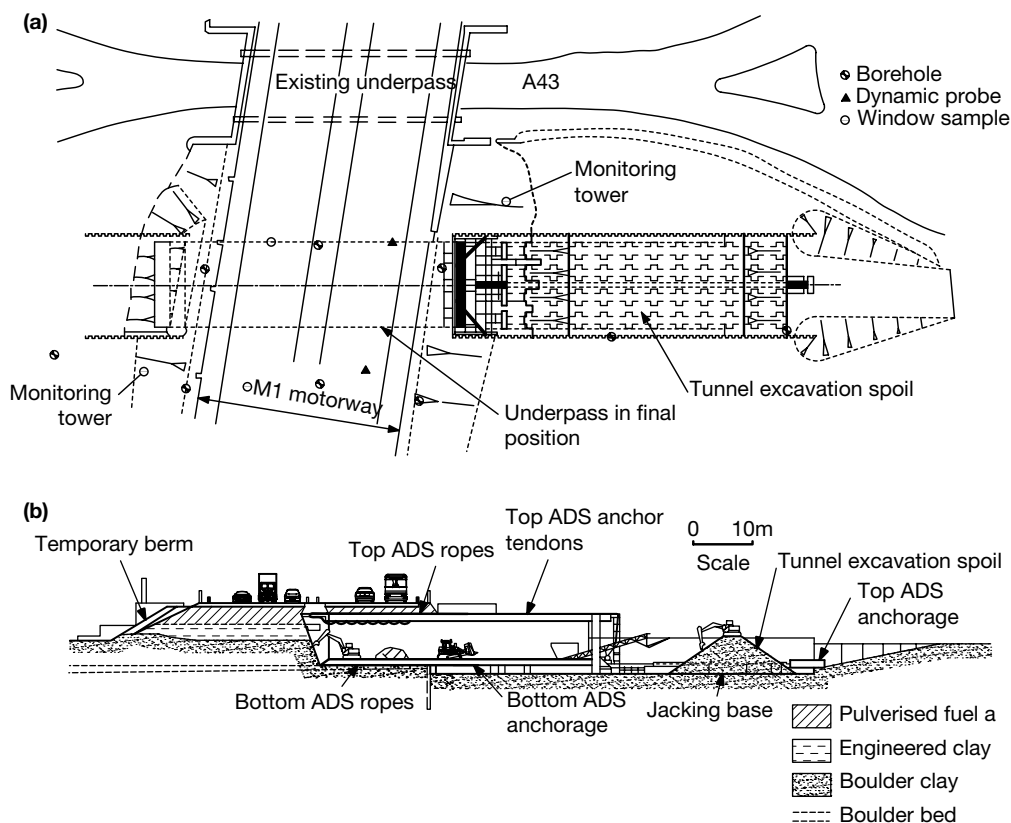
Figure 5.80 Details of the jacked box under-bridge at Junction 15A, M1 motorway, UK, (a) plan on completion of tunnelling and (b) longitudinal section during tunnelling. (Allenby and Ropkins 2004, courtesy of BAM Nuttall Ltd. and John Ropkins Ltd.)
