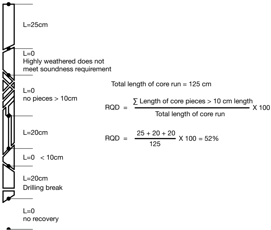
Figure 2.22 Procedure for measurement and calculation of RQD. (After Deere and Deere 1989, used with permission from Don Deere.)
