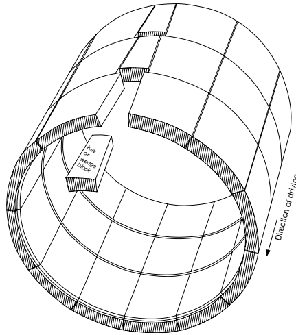
Figure 4.22 Principle of expanded wedge block segmental lining. (After Whittaker and Frith 1990 and Craig and Muir Wood 1978.)
