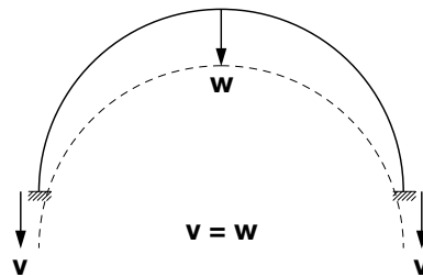
Figure 7.16 Rigid body displacement. (Rokahr et al. 2002.)
