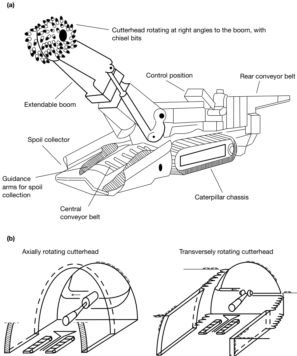
Figure 5.3 Partial face boring machine (roadheader), (a) schematic representation of a partial face boring machine and (b) advancement method of a partial face boring machine.
