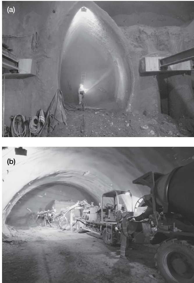
Figure 4.19 (a) Manual spraying and (b) spraying equipment used during the construction of the Lainzer Tunnel LT31 in Vienna, Austria.
