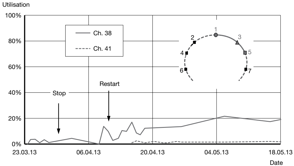
Figure 8.52 Utilisation versus time for section 1–3–5 at Ch. 38 and 41.
