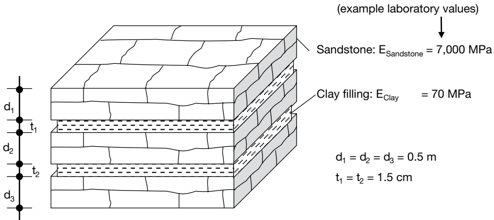
Figure 2.21 Example of how layering affects the E-modulus.
