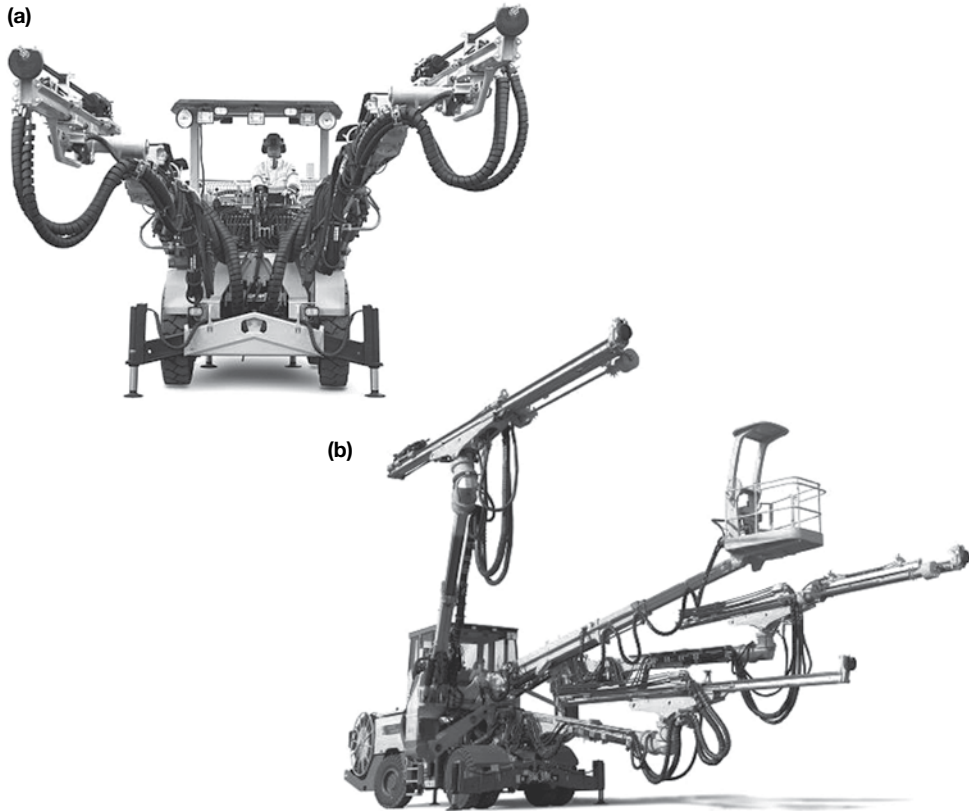
Figure 5.41 (a) Twin-boom hydraulic drill rig and (b) four-boom hydraulic drill rig. (Courtesy of Atlas Copco.)
