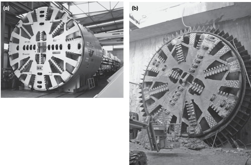
Figure 5.29 8.160 m diameter, 100 m long Herrenknecht S-192 Mixshield TBM used on the CTRL project in the United Kingdom, (a) before and (b) at breakthrough. This machine drove through alluvium, chalk and flints. (Courtesy of Herrenknecht.)
