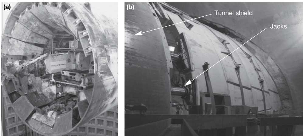
Figure 5.9 (a) The boom-in-shield tunnelling machine on removal after completion of the Heathrow Express Extension Tunnel at Terminal 5 in the United Kingdom (Manufacturer: Dosco) and (b) the same shield crossing an existing emergency exit where external strapping was required to support the erected lining.
