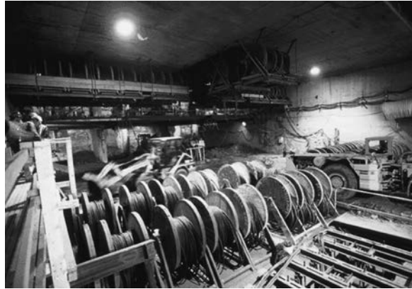
Figure 5.88 The inside of one of the tunnel box sections showing the proprietary ADS cable system. (Courtesy of Massachusetts Turnpike Authority.)
