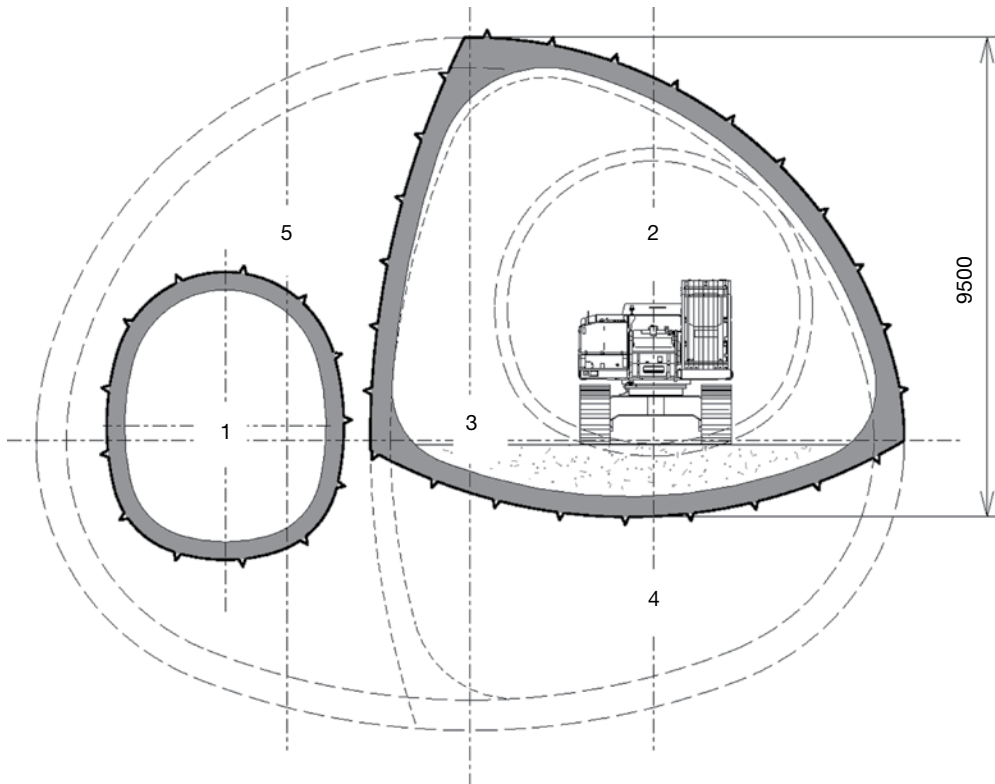
Figure 8.36 Whitechapel Station, Eastbound Cavern, excavation stages: 1 = Crossover tunnel; 2 = Eastbound Running tunnel; 3 = Eastbound Cavern, Top Heading; 4 = Eastbound Cavern, Invert; 5 = Eastbound Cavern, Single Side Wall Drift (line of sight is west). The graphic shows the completed stage 3. The Crossover tunnel (stage 1) will be demolished during stage 5. (Graphic Credit: Crossrail Ltd., used with permission.)
