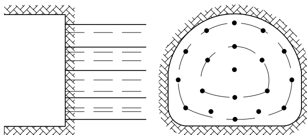
Figure 4.12 Schematic representation showing a typical arrangement of dowels used in the tunnel face. (After ITA/AITES 2007.)
