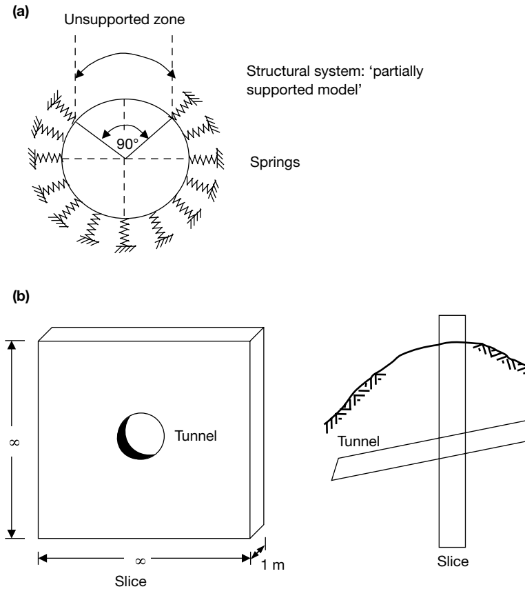
Figure 3.6 Calculation models for tunnels in soft ground. (a) Springmodel and (b) continuum model.
