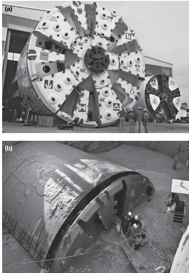
Figure 5.30 14.2 m diameter Herrenknecht S-108 Mixshield TBM used to construct the 4th Elbe Tunnel in Hamburg, Germany, (a) before and (b) at breakthrough (length of drive 2.56 km, through sand, glacial drift, silt, gravel and boulders). (Courtesy of Herrenknecht.)
