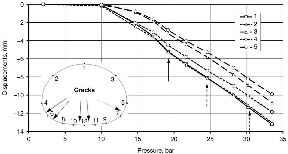
Figure 8.4 Vertical displacements at the crown and corresponding cracks.
