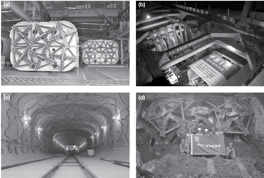
Figure 5.39 (a) Non-circular jacked box EPBMs used on the Zhongzhou Avenue Undercrossing Tunnel in China, (a) in the factory, (b) being launched, (c) during construction showing the bentonite lubrication injection system and (d) at breakthrough. (Courtesy of the China Railway Engineering Equipment Group Co.)
