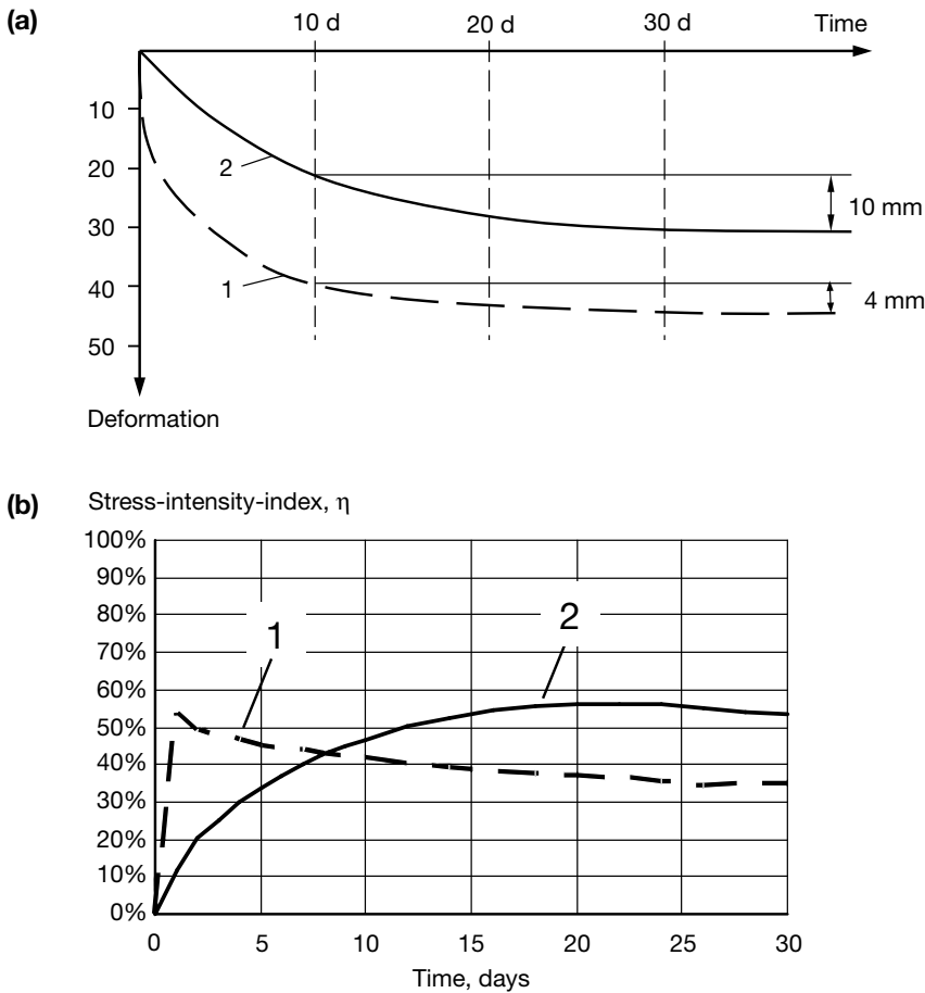
Figure 7.23 (a) Example deformations of the crown depending on time ( d = time in days) and (b) corresponding stress-intensity-index.
