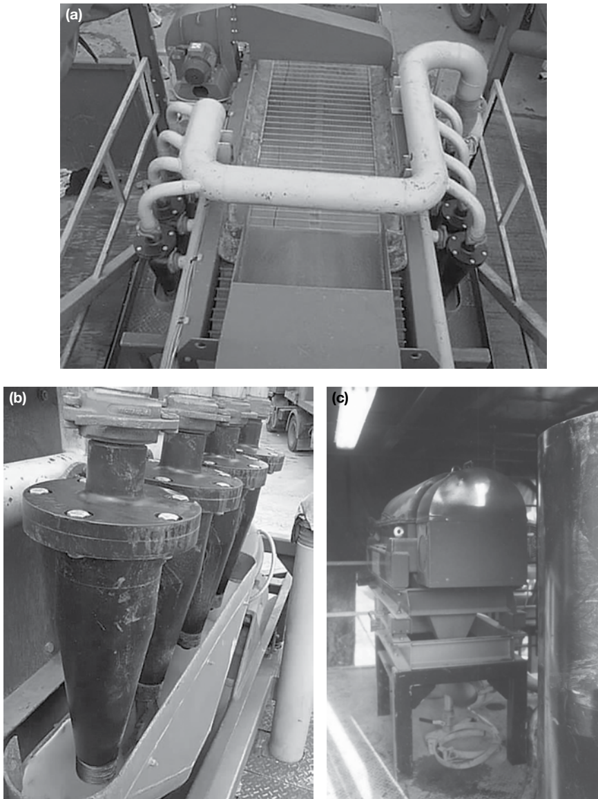
Figure 5.93 Equipment used to separate the excavated material from the slurry, (a) primary screen, (b) hydro-cyclones and (c) centrifuge. (Courtesy of Herrenknecht/the Pipe Jacking Association.)
