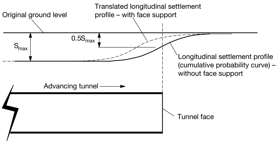
Figure 7.3 Longitudinal settlement profile above tunnels in soft ground, showing the difference in distribution for open-face tunnelling and where there is significant face support. (After Mair and Taylor 1997.)
