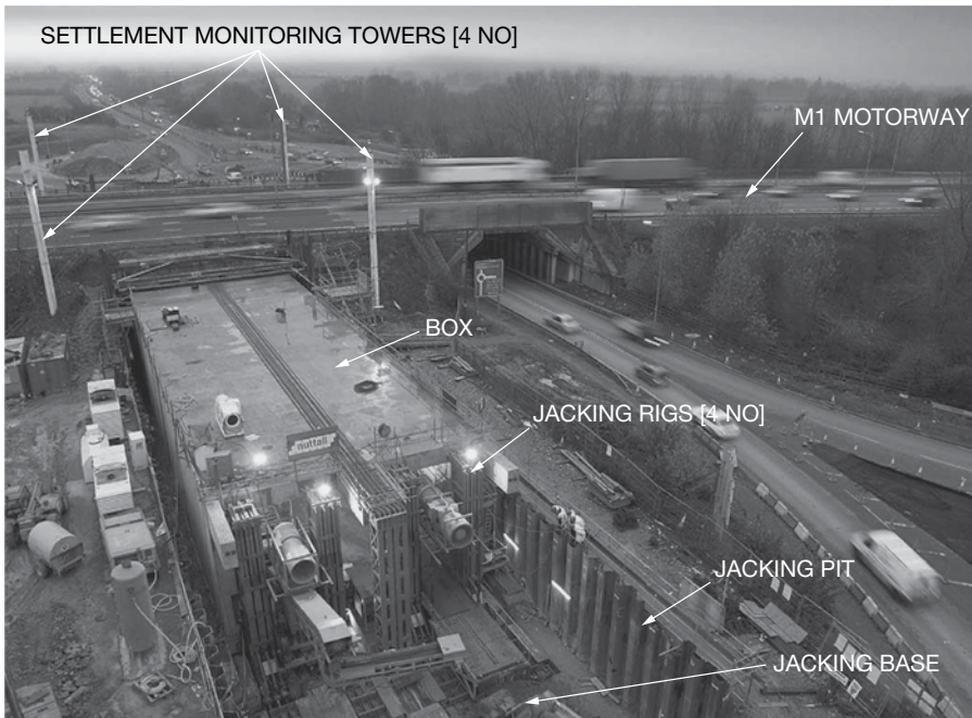
Figure 5.82 Rear view of the box during the jacking operation. (Allenby and Ropkins 2004, courtesy of BAM Nuttall Ltd. and John Ropkins Ltd.)
