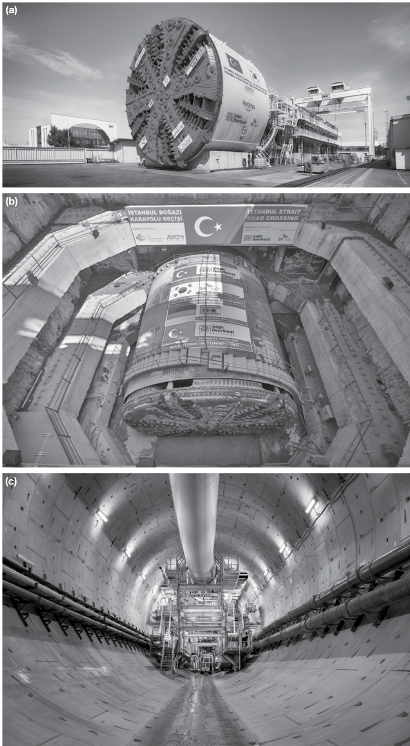
Figure 8.56 The Bosphorus Strait Mixshield TBM (13.66 m diameter) (a) in the factory, (b) at the reception shaft and (c) a view towards the rear of the TBM. (Courtesy of Herrenknecht.)
