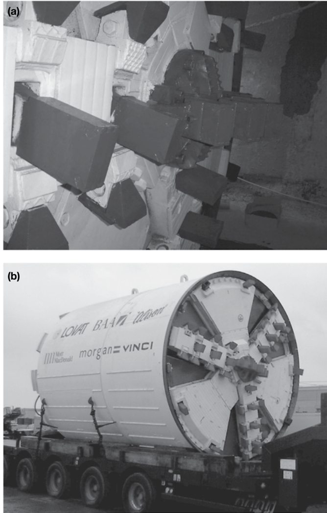
Figure 5.24 (a) The cutter dressing used in soft ground (London Clay), and (b) the fully refurbished Lovat TBM (SWOT at Heathrow Airport Terminal 5, UK). (Note: Lovat is now known as the Caterpillar Tunneling Canada Corporation.)
