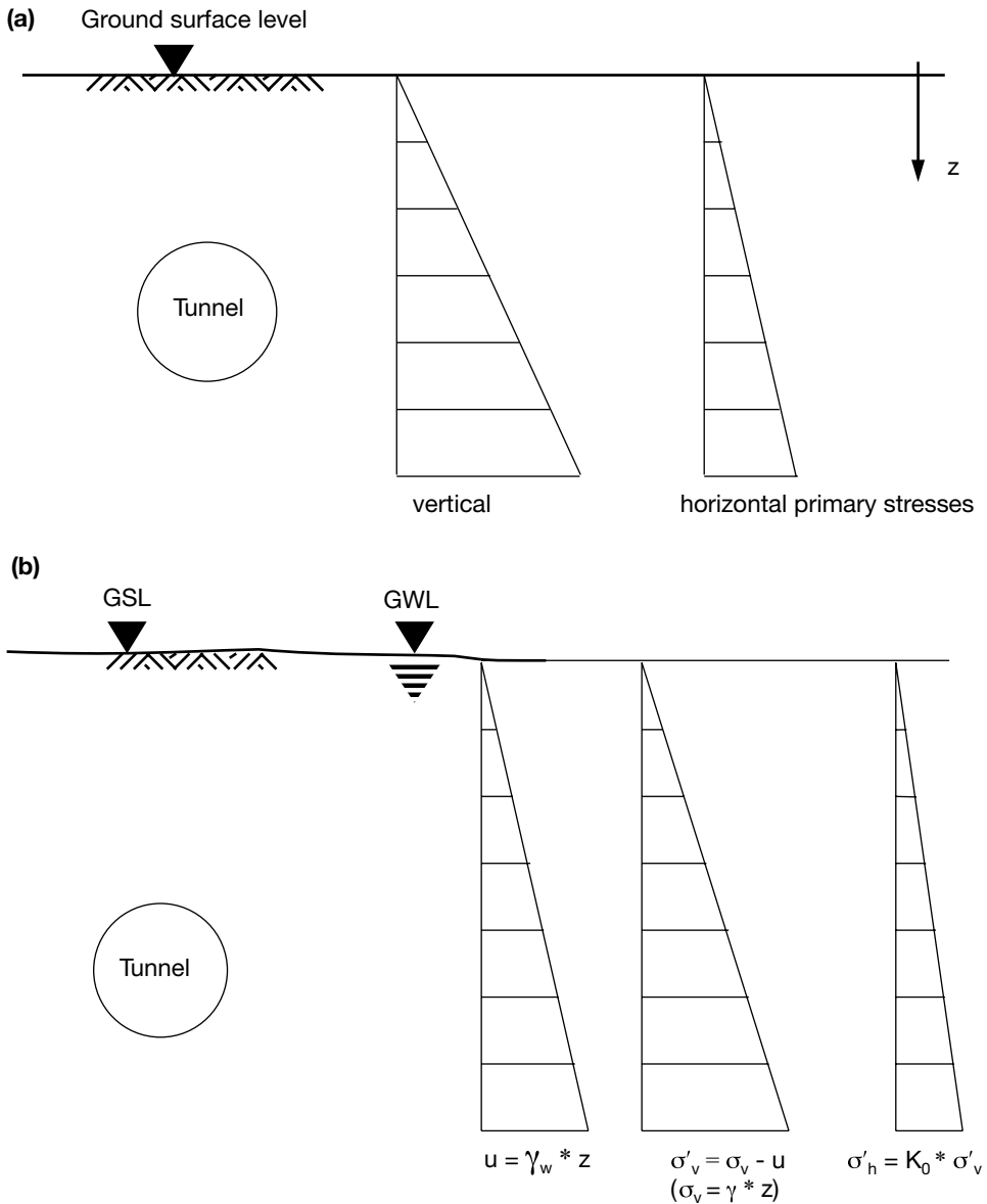
Figure 3.1 Primary stress distribution (a) above the groundwater table and (b) below the groundwater table (GWL).
