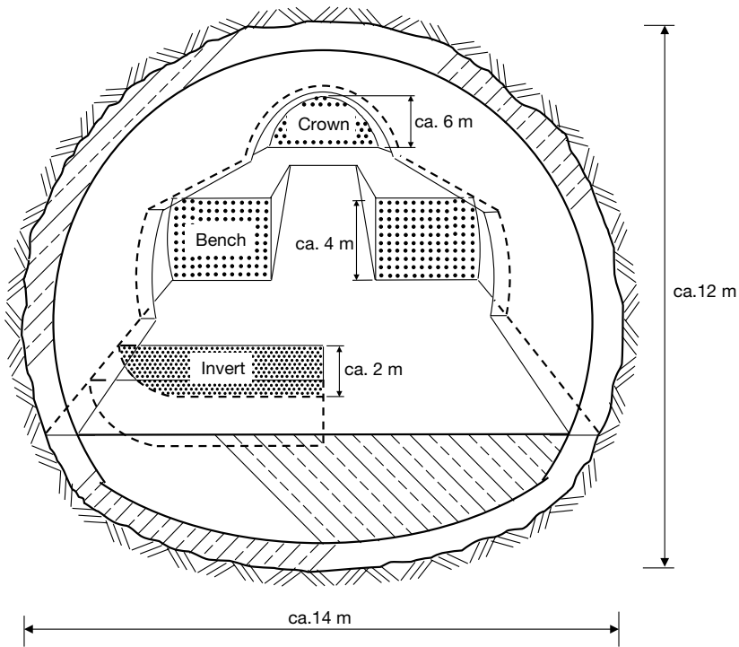
Figure 5.53 Example cross section through a tunnel constructed using NATM.
