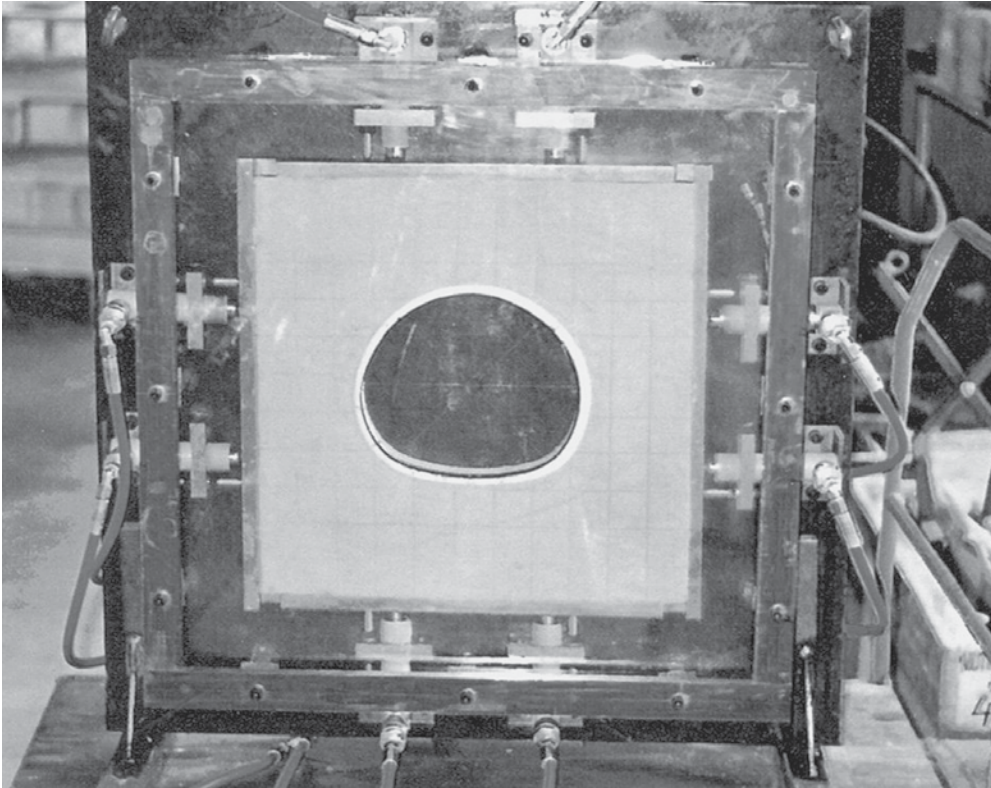
Figure 8.3 Model testing.
