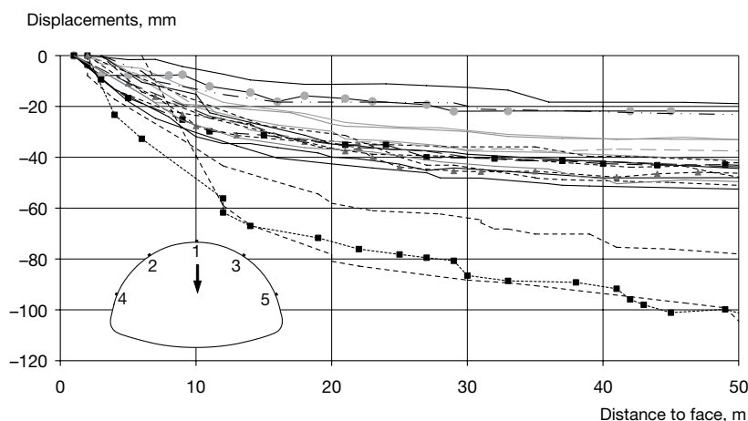
Figure 7.15 Vertical displacements for point 1 at different cross sections in the Eggetunnel for Chainage 482–684 in similar geological conditions.
