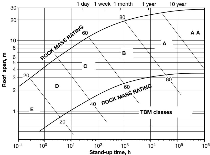
Figure 2.24 Boundaries of rock mass classes for TBM applications. (After Bieniawski 1989, modified from a plot by Lauffer 1988, used with permission from VGT Verlag GmbH and taken from Felsbau.)
