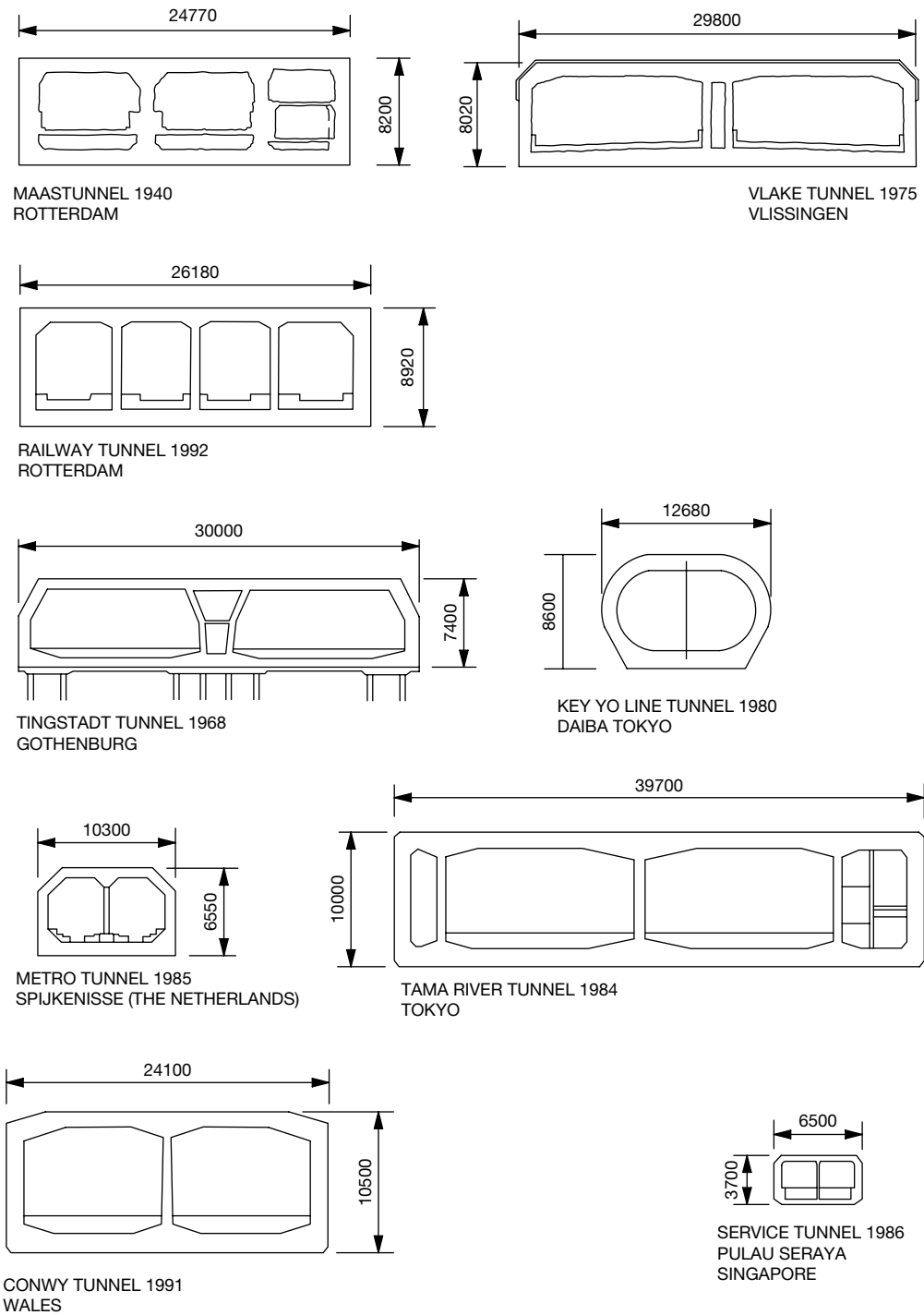
Figure 5.69 Typical cross sections for concrete immersed tube tunnels (all dimensions in mm). (After ITA 1997)
