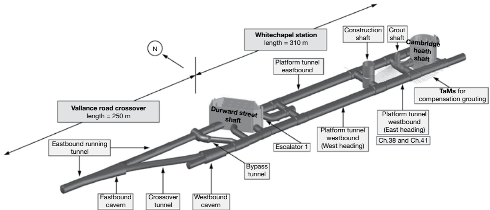
Figure 8.31 Whitechapel Station Layout. (Graphic Credit: Crossrail Ltd., used with permission.)
