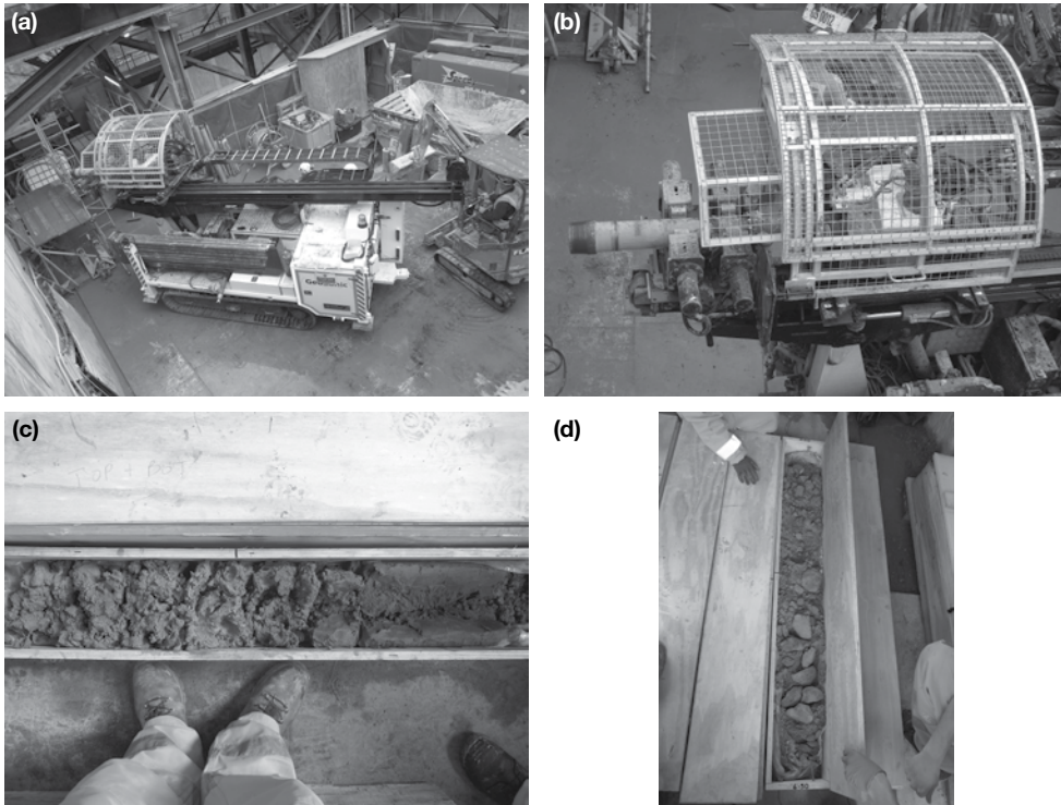
Figure 2.7 (a) and (b) Sonic drilling rig and (c) and (d) example core samples collected using a sonic drilling rig.
