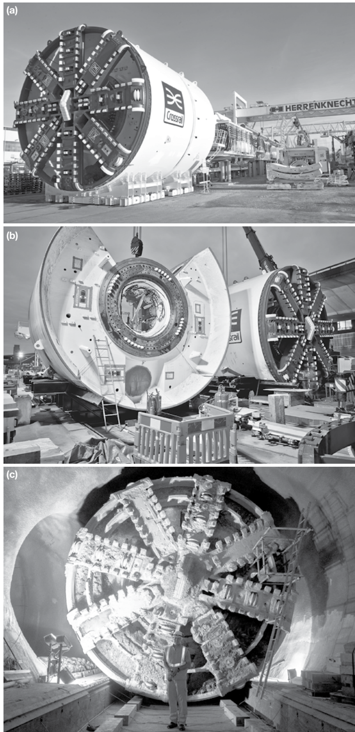
Figure 8.59 (a) and (b) 7.08 m diameter EPBMs (S705 and S706) used on Crossrail's project in London, UK (between Royal Oak and Farringdon) (Courtesy of Herrenknecht) and (c) breakout of another of the EPBMs at Liverpool Street Station, with Dr. Stärk standing in front of it. (Courtesy of Crossrail Ltd.)
