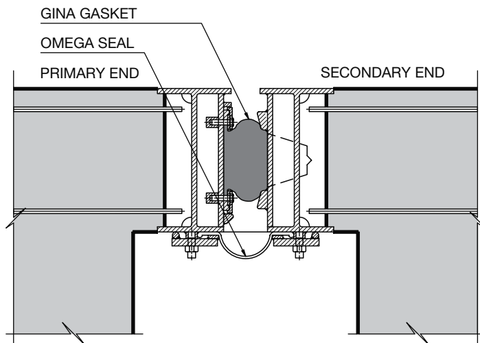
Figure 5.70 Example of rubber gasket joint. (Courtesy of COWI A/S.)
