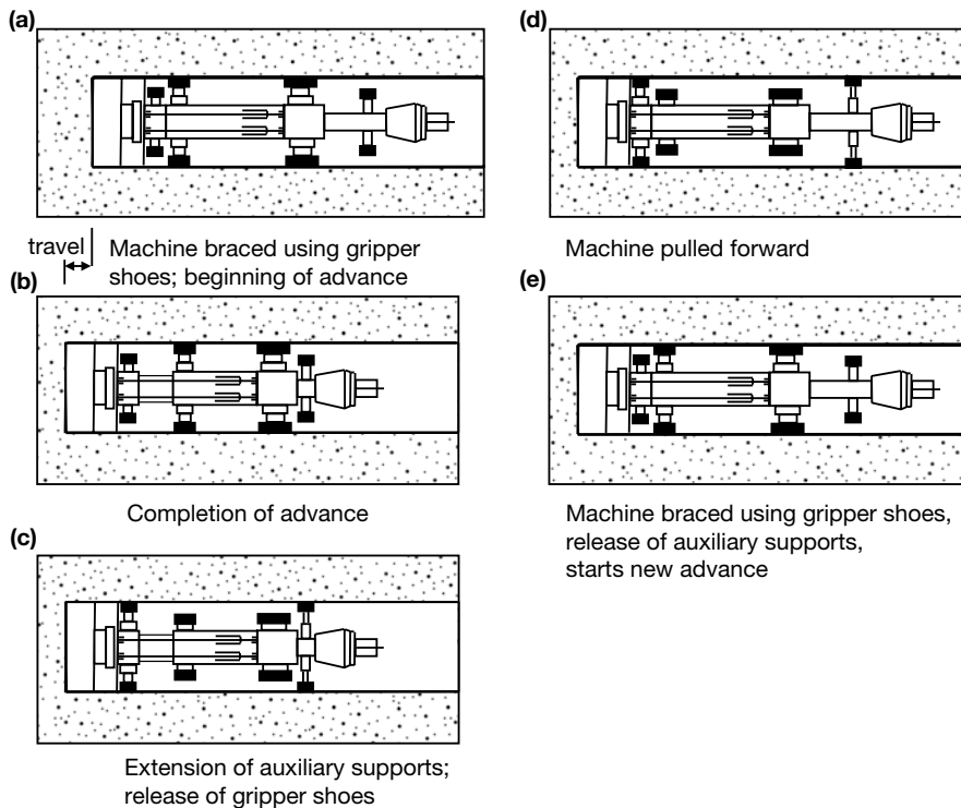
Figure 5.14 Principle of the 'gripper' TBM technique. (Courtesy of Aker Wirth.)
