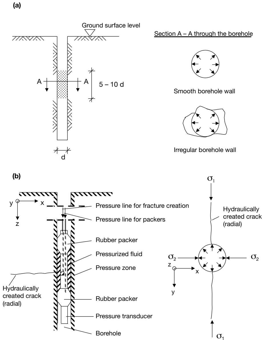
Figure 2.14 Schematic representation of the (a) dilatometer and (b) hydraulic fracturing tests.
