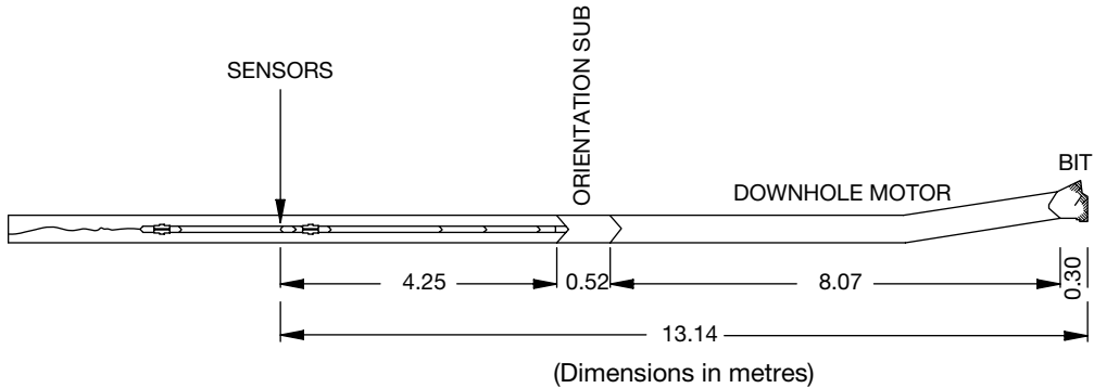
Figure 5.97 Schematic view of a typical bent-subassembly. The sensors for locating the drill head are spaced behind the motor to reduce magnetic interference. (After Riggall 2008.)
