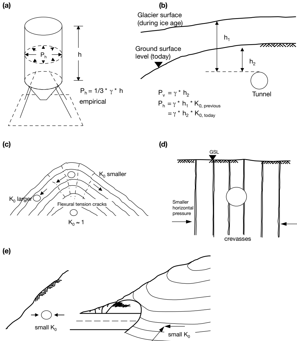
Figure 3.5 Coefficient of lateral earth pressure. (a) Horizontal pressure in a silo, (b) ice age pre-loading, (c) horizontal pressure for strata in connection with a saddle, (d) horizontal pressure with crevasses and (e) horizontal pressure near a portal.
