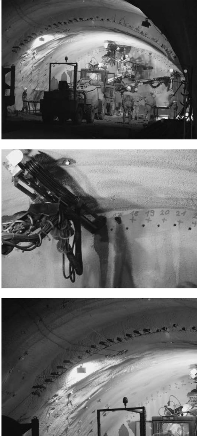
Figure 4.14 Forepoling using dowels as a roof pipe umbrella on the Lainzer Tunnel LT3I in Vienna, Austria.
