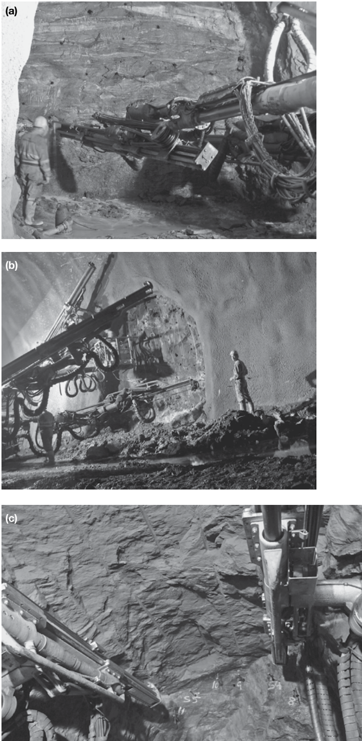
Figure 5.42 Examples of drilling blasting holes, (a) and (b) for an emergency cross-passage, Katschberg Tunnel, Austria and (c) for the Spillvatten Tunnel, Goeteborg, Sweden (an 8 km sewer tunnel, cross-sectional area 11 m 2 , ground included granitic gneiss).
