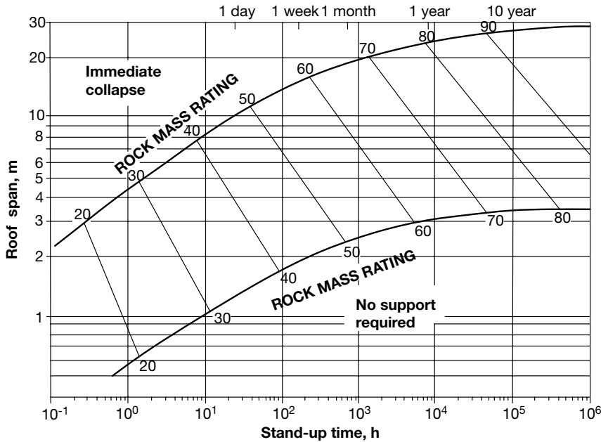
Figure 2.23 Relationship between the stand-up time and roof span for various rock mass classes. (After Bieniawski 1989.)
