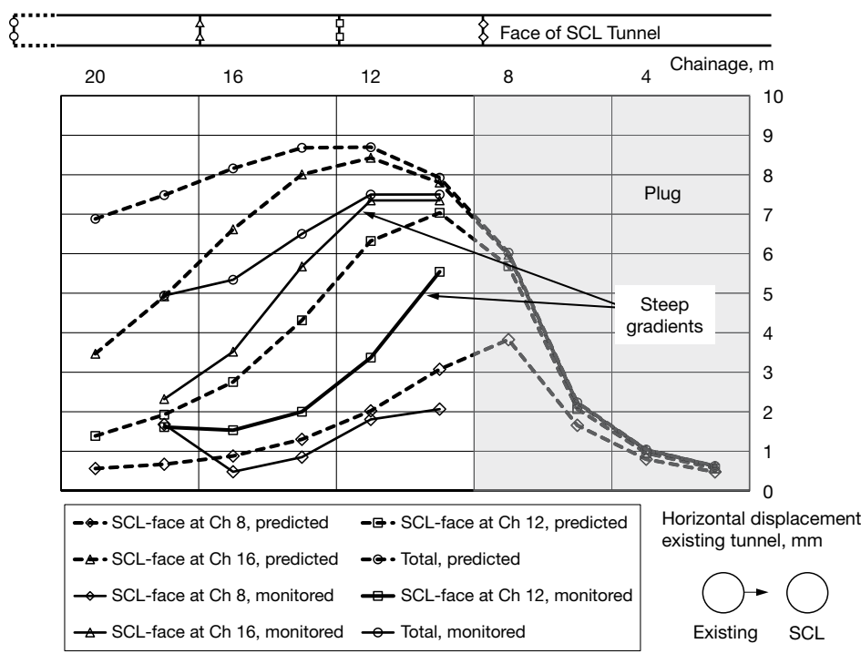
Figure 8.15 Predicted and measured horizontal displacements in the existing Piccadilly Line Eastbound Tunnel.
