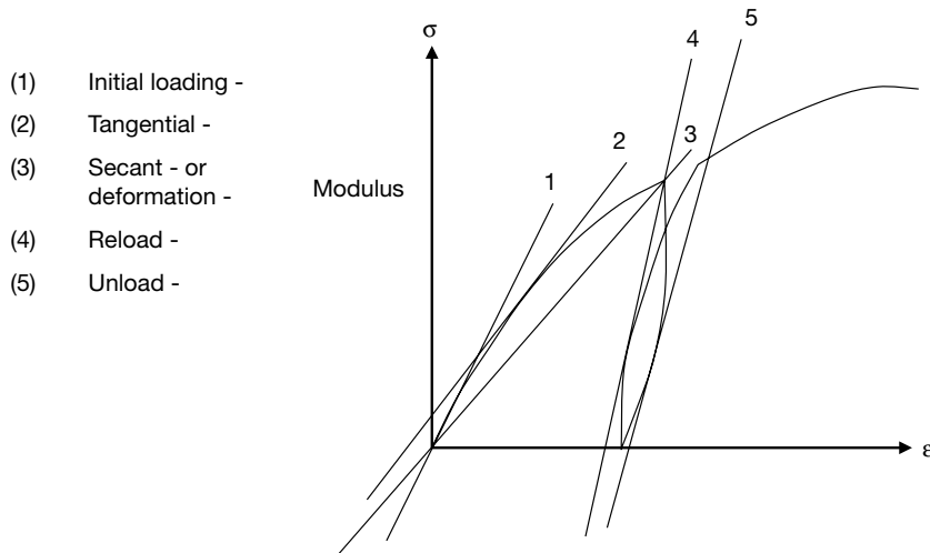
Figure 2.18 Definitions of different modulus values.
