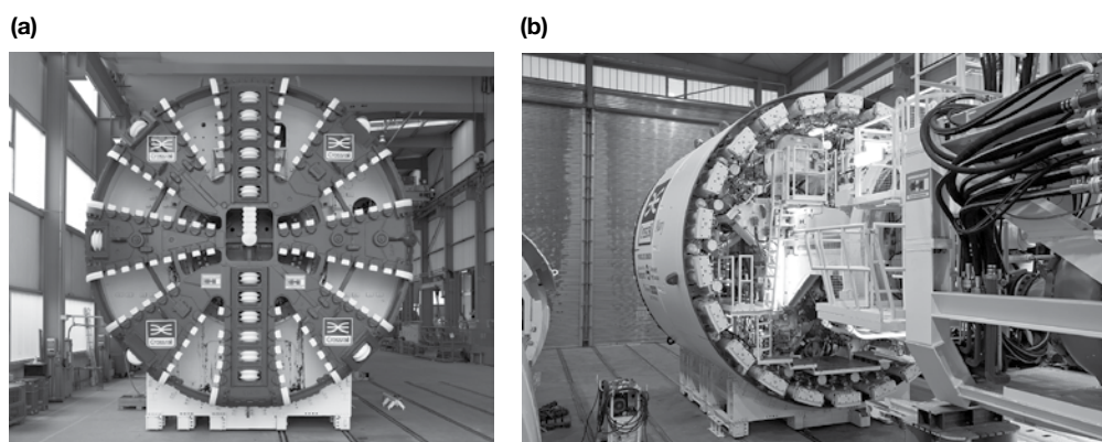
Figure 5.36 (a) and (b) 7.08 m diameter Mixshield TBMs (S731 and S732, respectively) used on the Crossrail project to tunnel under the River Thames in London, UK. (Courtesy of Herrenknecht.)
