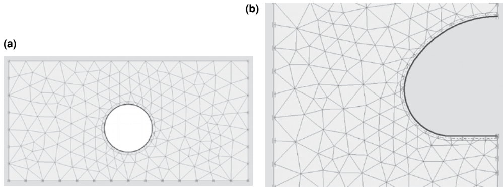
Figure 3.8 Example 2-D meshes using FEs, (a) 2-D plain strain analysis of a bored tunnel construction and (b) 2-D plain strain analysis (with symmetry associated with the tunnel centre line) of a tunnel being constructed using NATM, as produced using the PLAXIS® software. (Courtesy of Wilde Analysis Ltd.)
