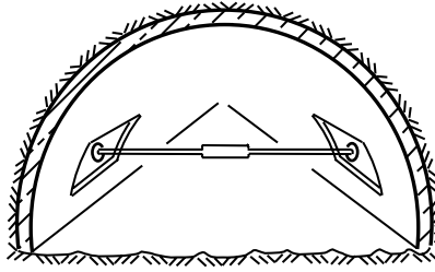
Figure 2.15 Diagram showing one method of conducting the double load plate test.
