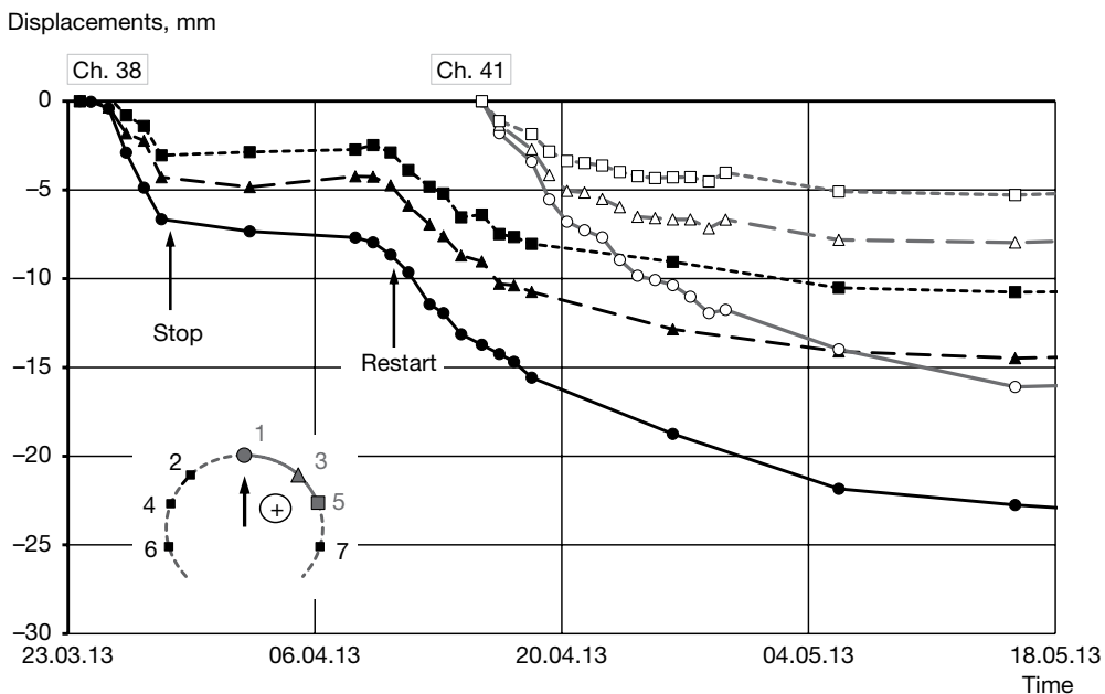
Figure 8.51 Ch. 38 and Ch. 41: Vertical displacement for points 1, 3, 5. Negative displacements = settlement. Points 2, 4, 6 and 7 are not shown for clarity.
