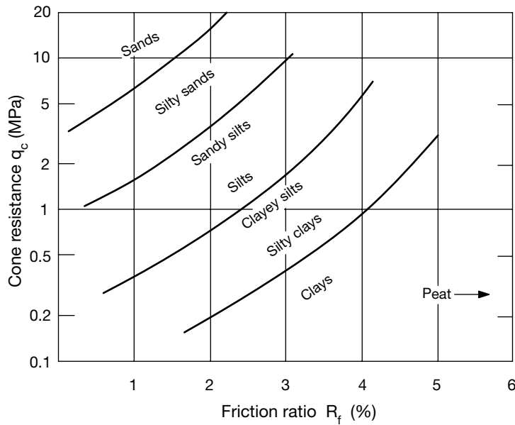
Figure 2.13 Simplified version of a friction ratio cone resistance plot used to obtain an approximate description of the ground.
