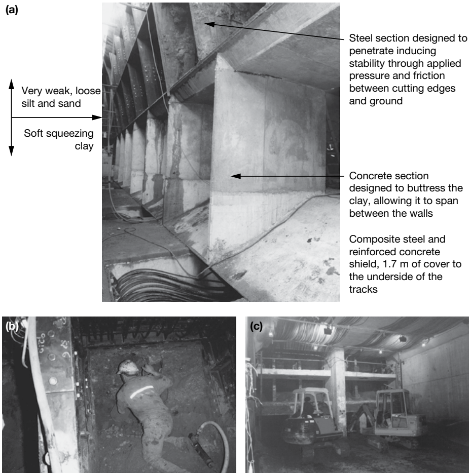
Figure 5.77 Example shield as used on a jacked box tunnel as part of the Docklands Light Railway, Lewisham, London, UK (box size 17 m wide, 6.2 m high and 48 m long), (a) composite steel and reinforced concrete shield, (b) hand mining in a top compartment through very weak, loose sand and silt and (c) rear view of the face during excavation. (Courtesy of BAM Nuttall Ltd. and John Ropkins Ltd.)
