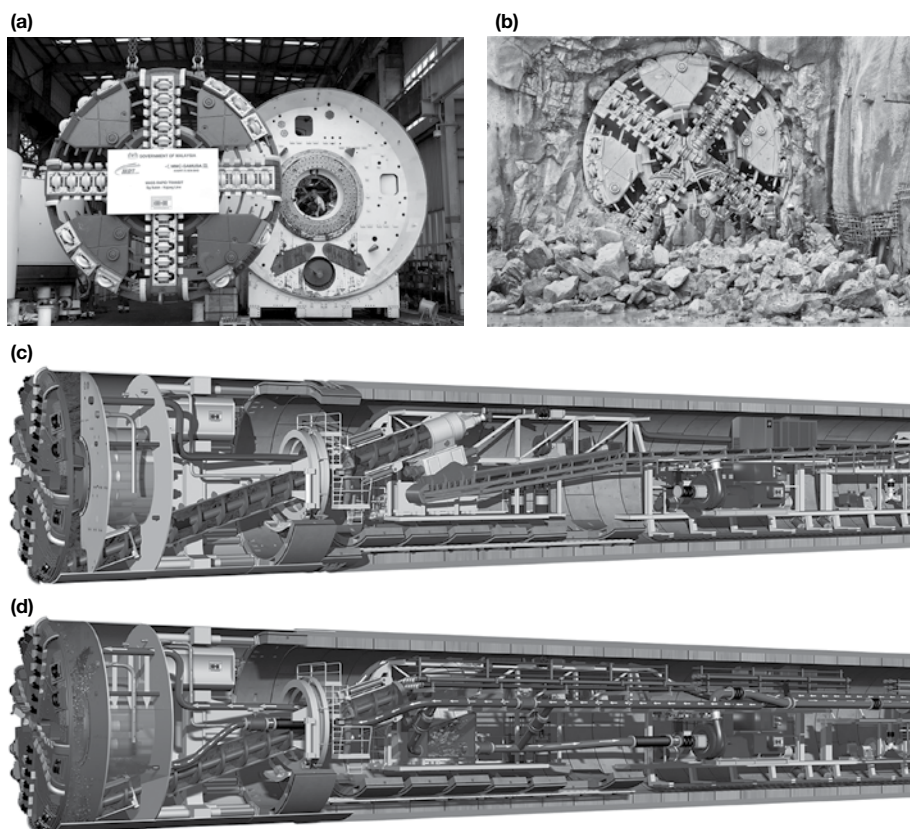
Figure 5.37 Klang Valley multimode 6.62 m diameter TBM, (a) the TBM cutterhead in the factory, the excavation chamber (plenum) is also shown together with the end of the screw conveyor, (b) the TBM completing a drive, note the ground it is driving through, (c) the TBM working in EBM mode and (d) the TBM working in slurry mode showing the slurry line connections. (Courtesy of Herrenknecht.)
