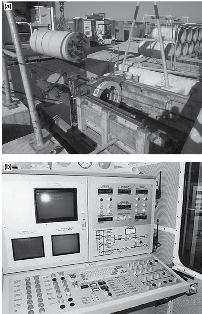
Figure 5.92 (a) A typical pipe jacking site arrangement and (b) a control panel for a pipe jacking or microtunnelling machine. (Courtesy of Herrenknecht and the Pipe Jacking Association.)
