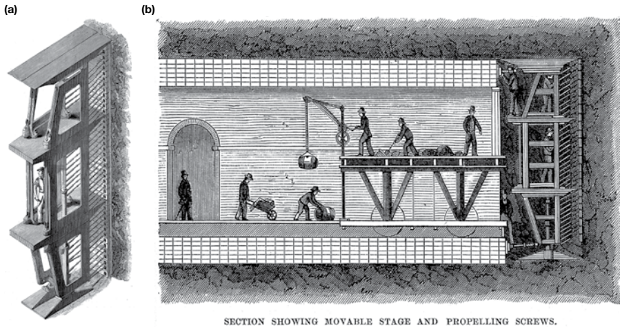
Figure 1.1 'Brunel's shield' used for the first Thames Tunnel. (a) One of the 12 frames making up the shield and (b) a long section through this tunnel during construction. (After Beamish 1862.)
