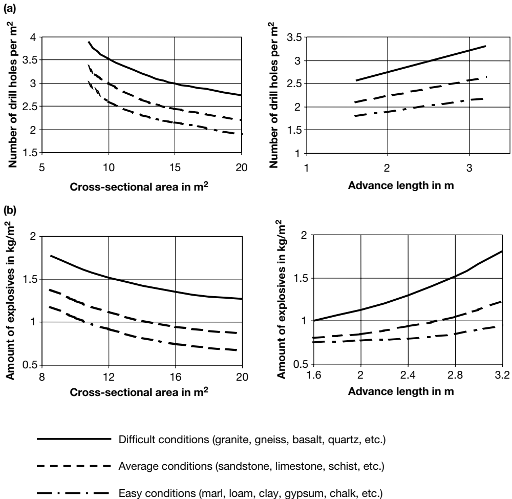
Figure 5.51 Number of drill holes and amount of explosive as a function of cross-sectional area and advance length, respectively, (a) number of drill holes and (b) amount of explosive. (After Müller, 1978.).
