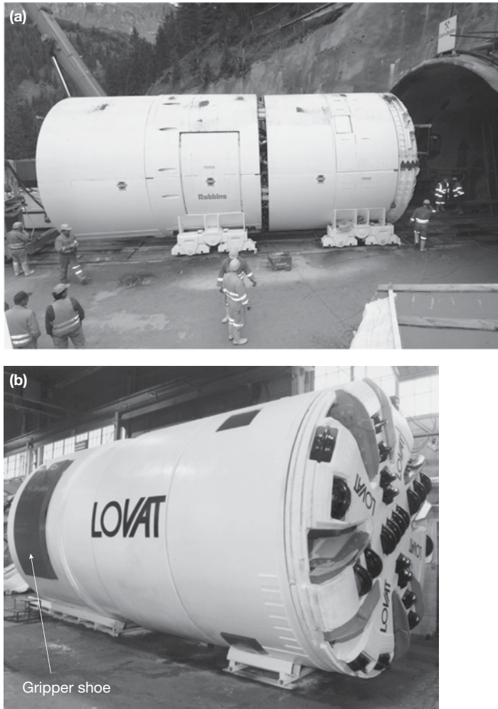
Figure 5.21 (a) Double-shield TBM used in Austria (5.5 m diameter, ground conditions gneiss and amphibolites (Courtesy of The Robbins Company.) and (b) double-shield TBM used in Seoul, Korea (3.48 m diameter, 2.75 km length). (Courtesy of Lovat, now known as the Caterpillar Tunneling Canada Corporation.)
