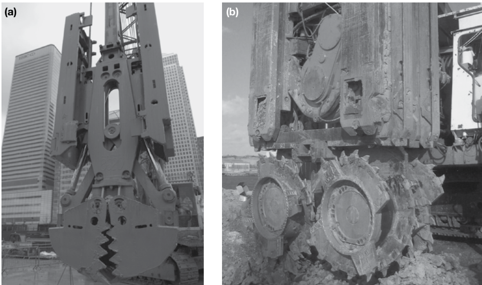
Figure 5.64 (a) Grab or clam bucket excavator and (b) hydrofraise used for diaphragm wall construction. (Courtesy of Bachy Soletanche Ltd.)
