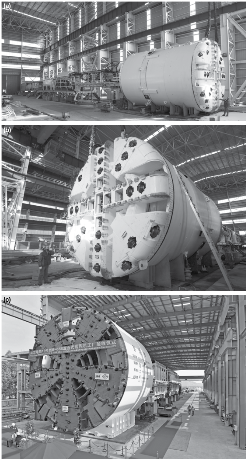
Figure 8.58 (a) and (b) A 6.5 m diameter EPBM used on the Nanjing Metro in China (Courtesy of The Robbins Company) and (c) an 11.61 m diameter Mixshield TBM used on the Nanjing Metro in China. (Courtesy of Herrenknecht.)
