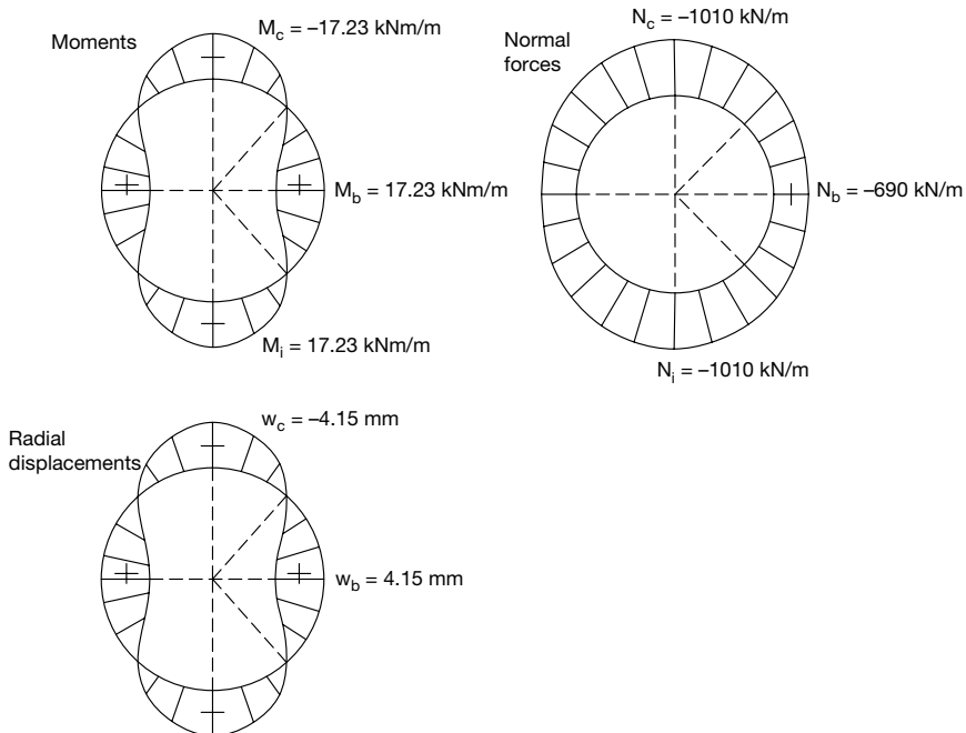
Figure B.4 Moments, normal forces and radial displacements.
