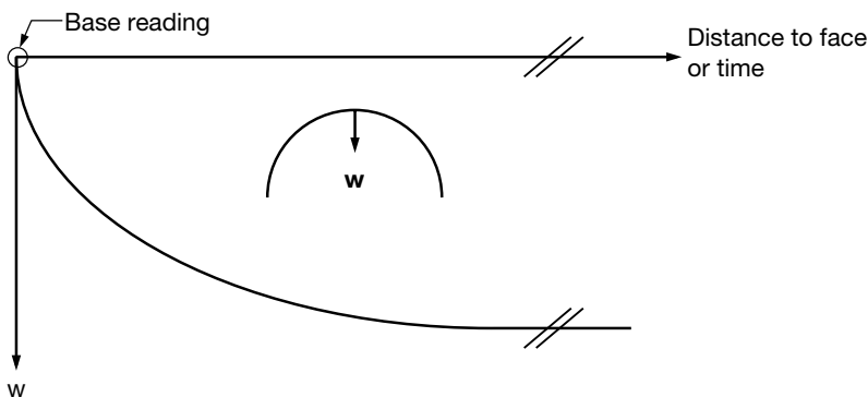
Figure 7.12 Vertical displacement at the crown of a tunnel (idealised example).
