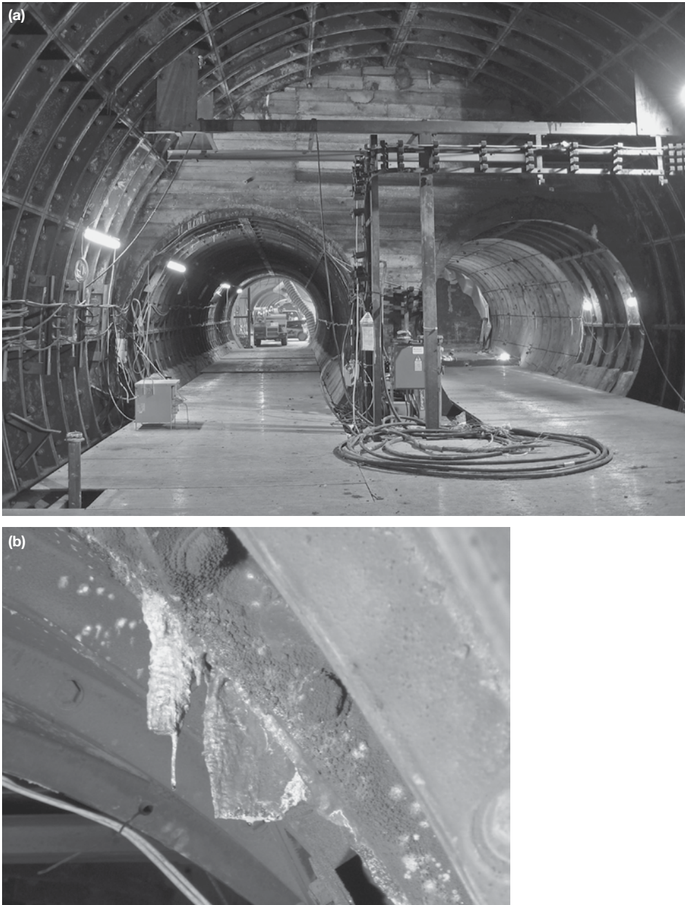
Figure 8.13 (a) Existing Piccadilly Line tunnels, SGI-Segments (LHS), Concrete Segments (RHS) and (b) existing Piccadilly Line Eastbound Tunnel, stalactites on the SGI-Segments.
