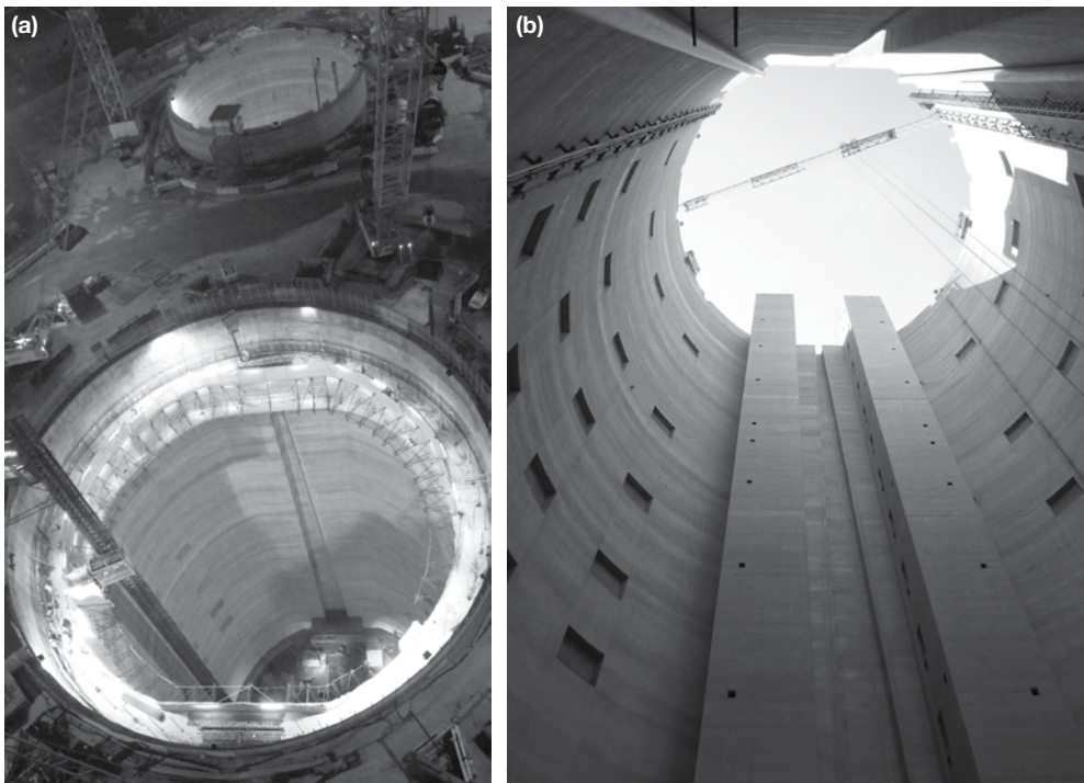
Figure 8.62 (a) One of the shafts during the slip lining process and (b) the completed shaft. (Courtesy of Underground Professional Services and Morgan Sindall.)
