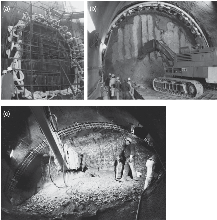
Figure 4.3 Examples of ground freezing used in tunnelling: (a) horizontal freezing to rescue a broken down TBM in Cairo, (b) freezing at the portal of a 13 m diameter road tunnel in Du Toitskloof, South Africa, through decomposed granite and (c) excavation of the tunnel crown through frozen sand and gravel in Dusseldorf. (Courtesy of British Drilling & Freezing Co. Ltd.)
