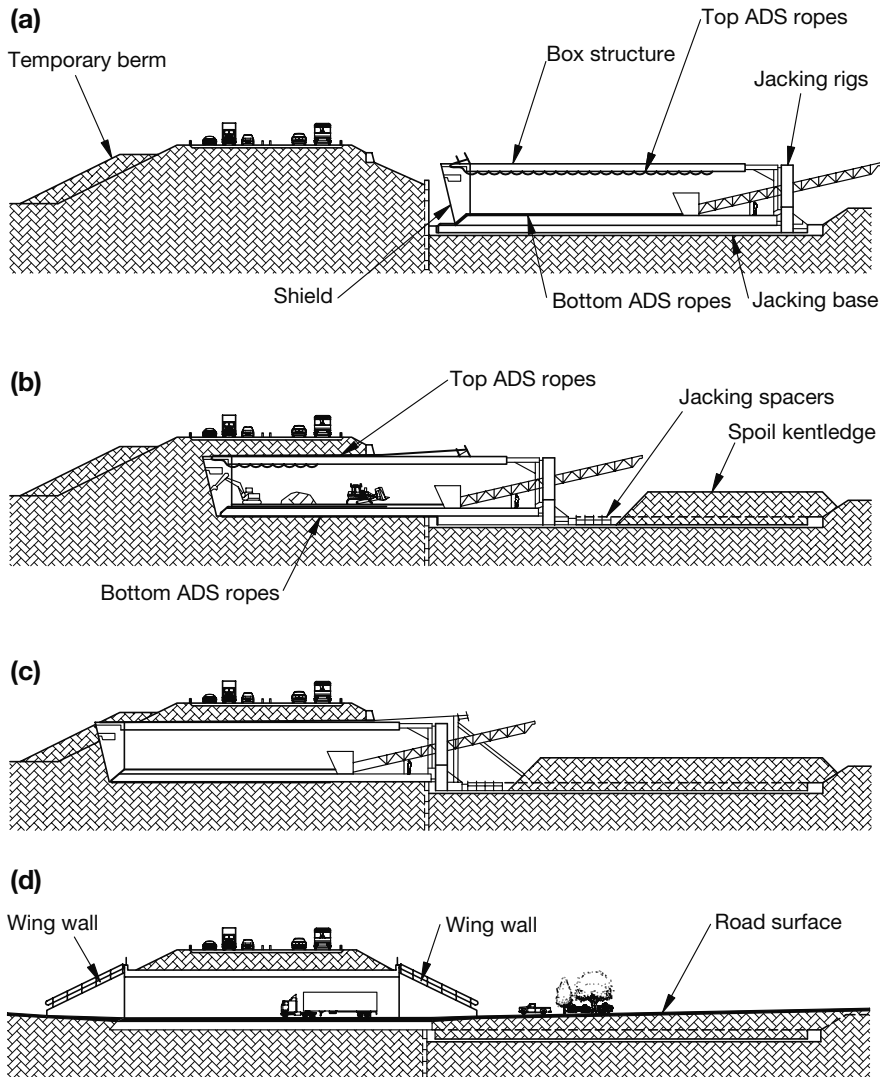
Figure 5.76 Jacked box tunnel installation, (a) box ready for installation, (b) box partially installed, (c) box fully installed and (d) completed structure. (Allenby and Ropkins 2007, courtesy of BAM Nuttall Ltd. and John Ropkins Ltd.)
