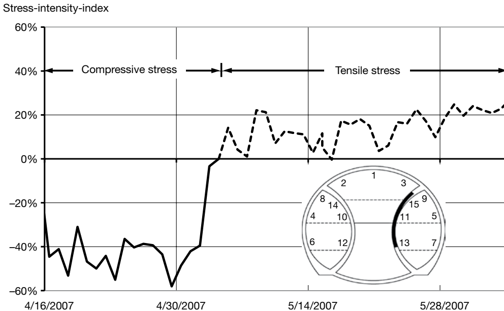
Figure 8.28 Stress-intensity-index, section W, Chainage 60.
