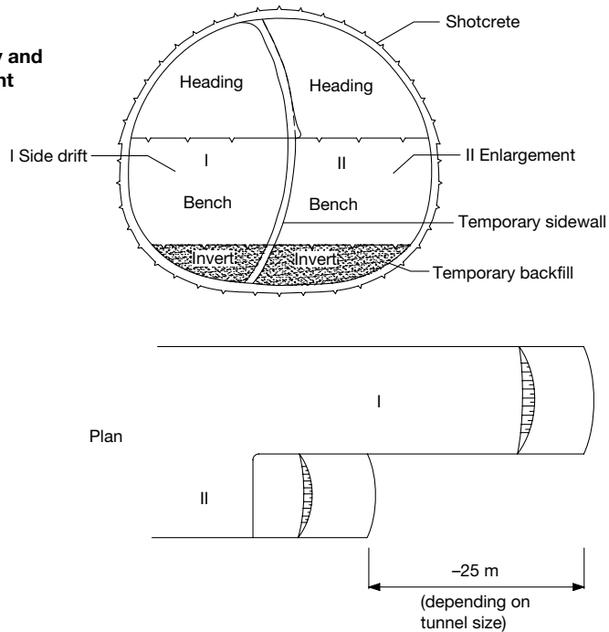
Figure 5.57 Possible excavation sequences for SCL (and NATM). (After ICE 1996, used with permission from ICE Publishing.) (Continued)
