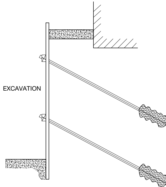
Figure 5.61 General arrangement of an anchored retaining wall. (After Megaw and Bartlett 1982, used with permission from John Bartlett.)
