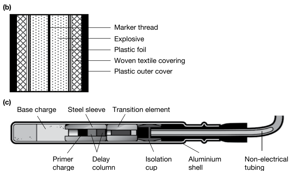
Figure 5.45 Details of detonators, (a) cross section of an electric detonator timer, (b) cross section of a detonator cord and (c) non-electrical detonator.
