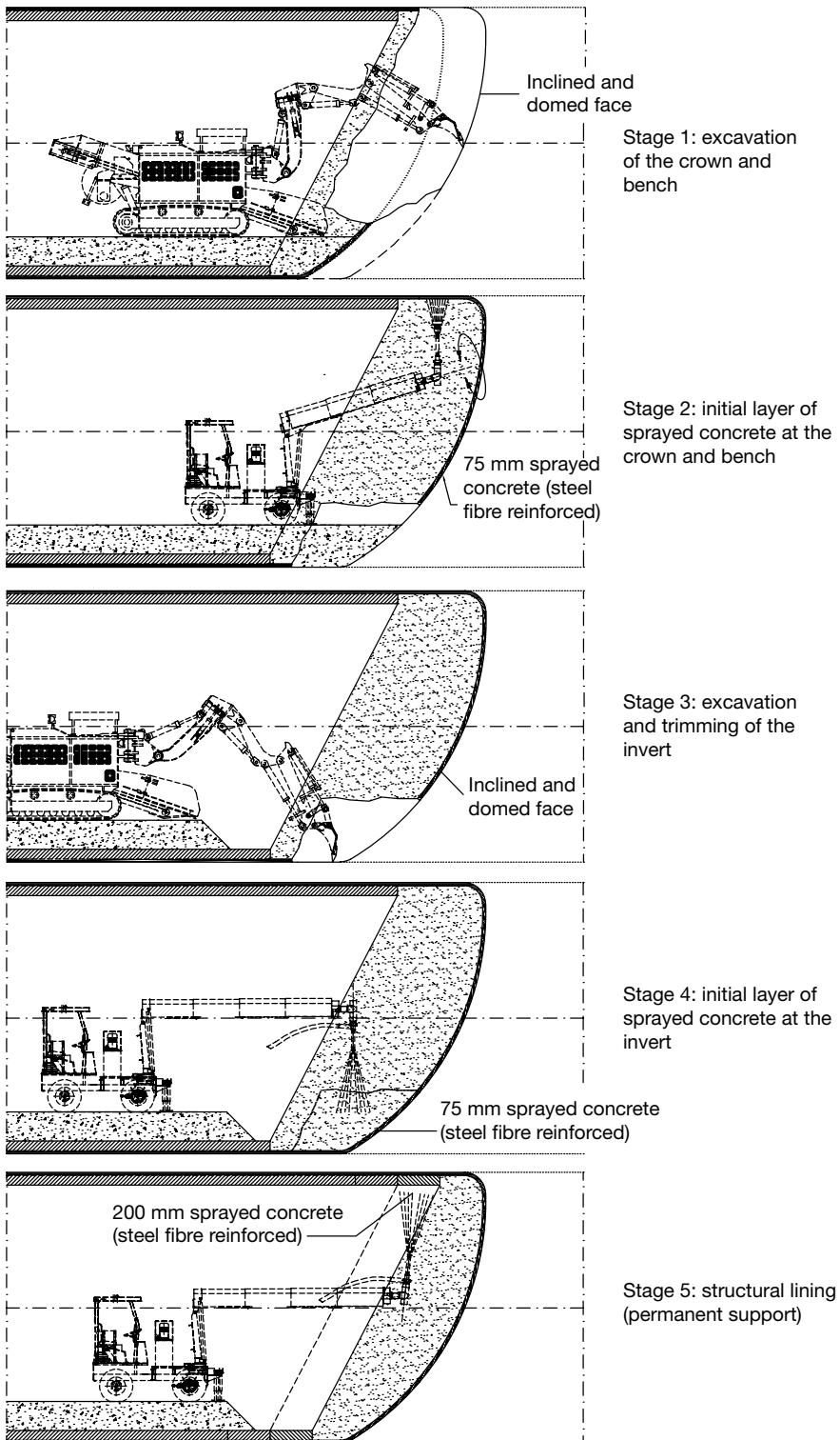
Figure 8.11 Construction sequence for the LaserShell™ method. (Courtesy of BeMo Tunnelling GmbH Innsbruck.)
