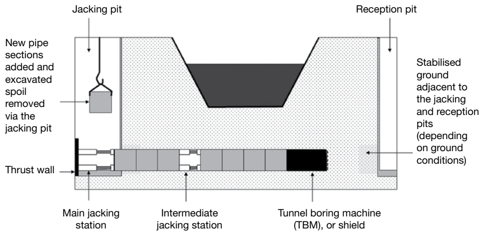
Figure 5.89 Illustration of a pipe jack under a canal. (Courtesy of A. Royal.)
