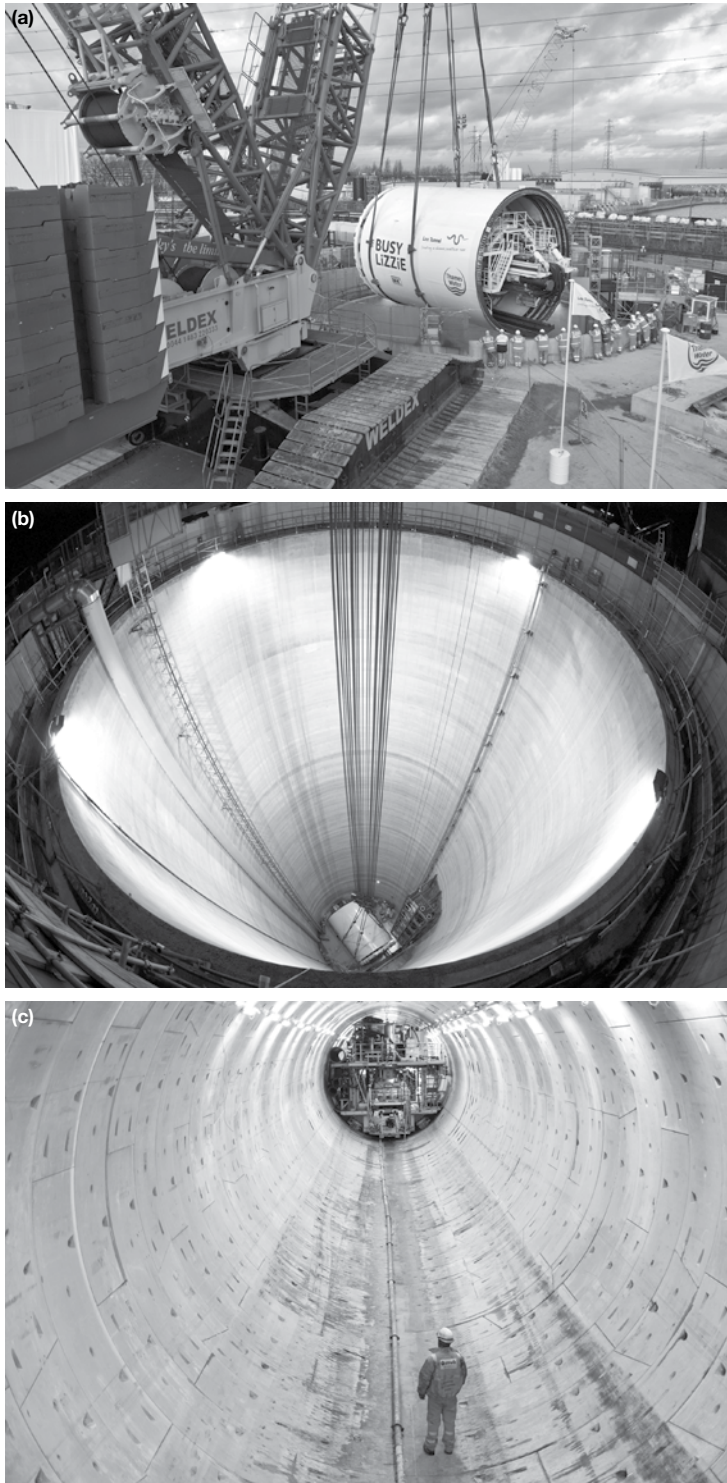
Figure 8.63 (a) and (b) An 8.8 m diameter slurry TBM (named 'Buzy Lizzie') being installed in the shaft and (c) the steel fibre-reinforced segmental lining. (Courtesy of Underground Professional Services and Morgan Sindall.)
