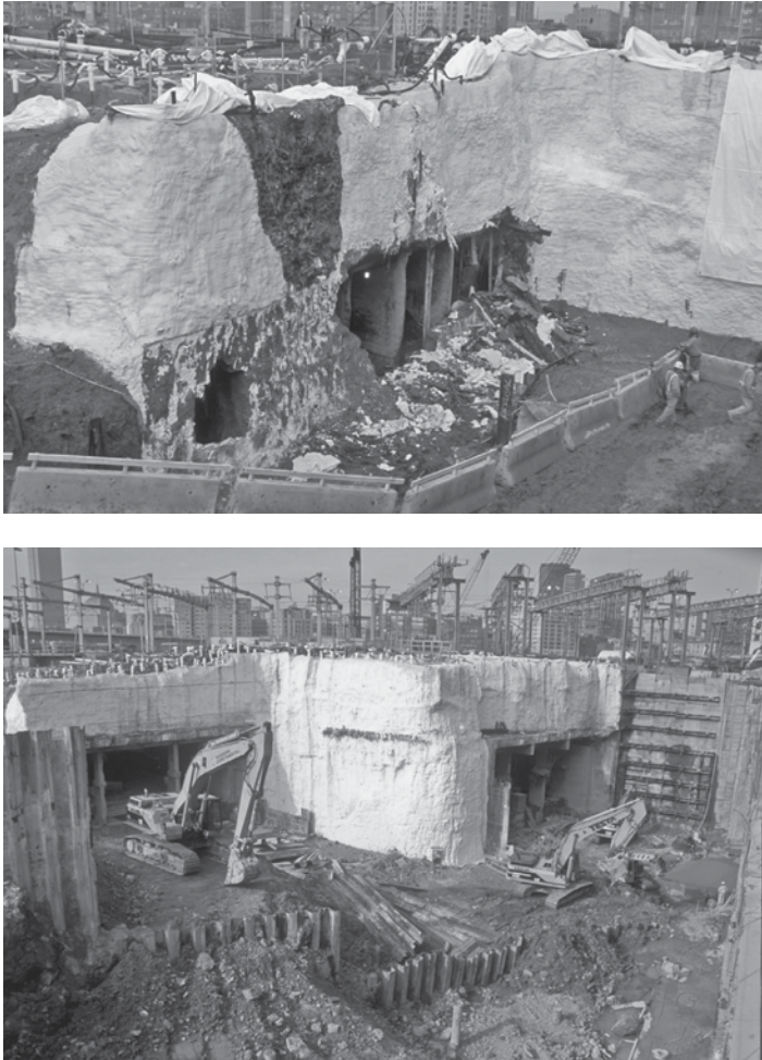
Figure 5.86 Breakthrough of two of the jacked tunnels, showing the freezing operation at the ground surface. (Courtesy of Massachusetts Turnpike Authority.)
