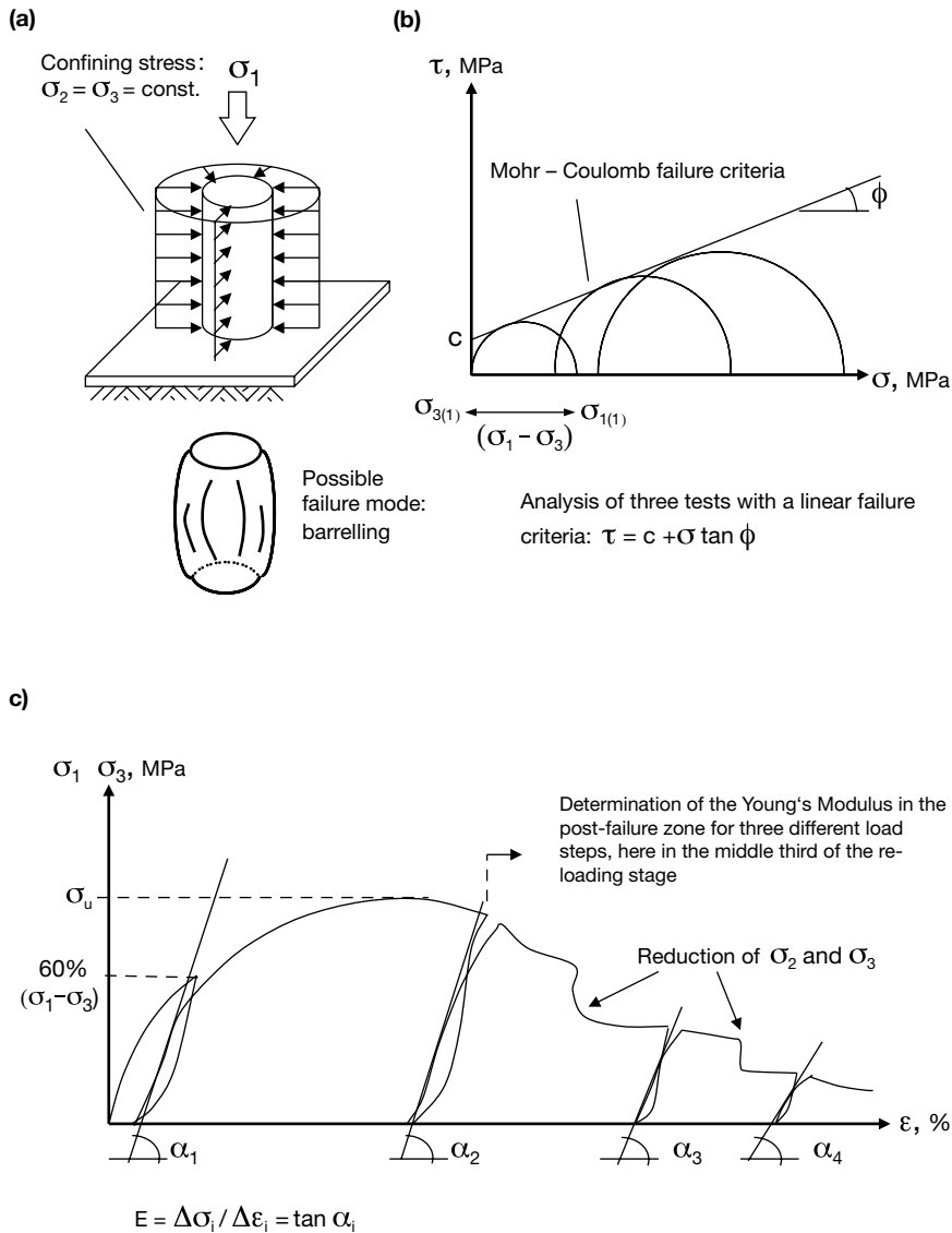
Figure 2.19 Triaxial test (a) sample and failure mode, (b) \tau - \sigma -diagram and (c) \sigma - \epsilon -diagram.
