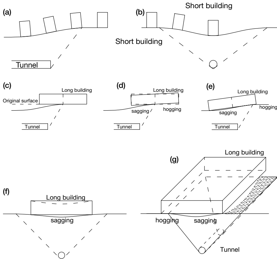
Figure 7.6 Some idealised modes of behaviour for short buildings and long buildings due to a tunnel construction below. (a) and (b) Behaviour of a short building with respect to its position in relation to the longitudinal and transverse ground displacements; (c), (d) and (e) behaviour of a long building with respect to its position in relation to the longitudinal ground displacements; (f) and (g) behaviour of a long building with respect to its position in relation to the transverse ground displacements. (Attewell 1995, after Attewell et al. 1986.)
