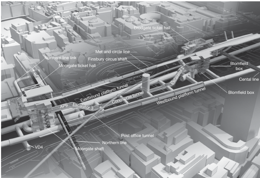
Figure 8.46 The new Liverpool Street Station and existing underground structures. Not shown for clarity are the Geotechnical Adits above the new Concourse tunnel and the Goswell Sewer above the Northern Line. (Graphic Credit: Crossrail Ltd., used with permission.)
