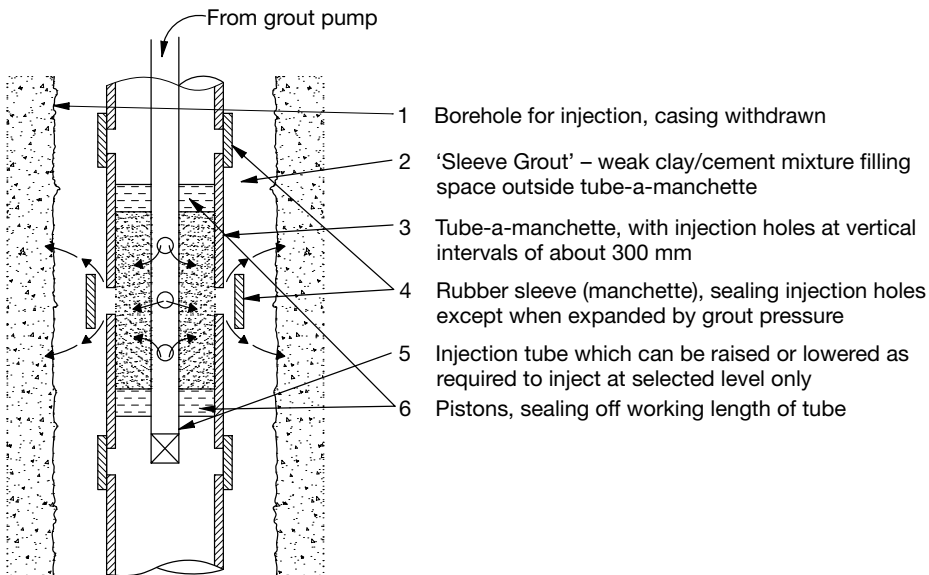
Figure 4.6 General arrangement of a TAM. (After Megaw and Bartlett 1982, used with permission from John Bartlett.)
