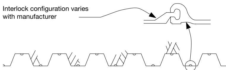
Figure 5.60 Sheet pile excavation support. (After Kuesel and King 1996.)
