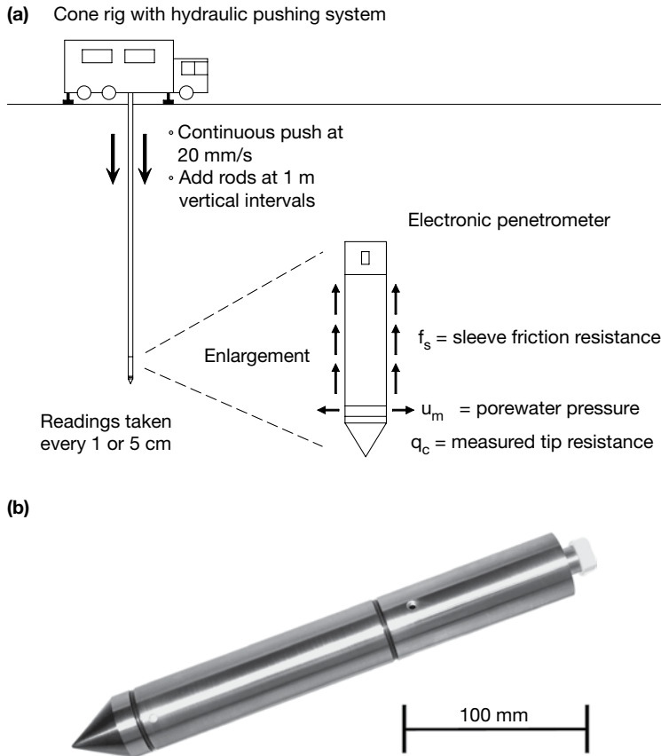
Figure 2.11 Cone penetration testing: (a) Test arrangement (After Mayne 2007.) (b) Example of an electric penetrometer cone. (Courtesy of Geopoint Systems BV.).
