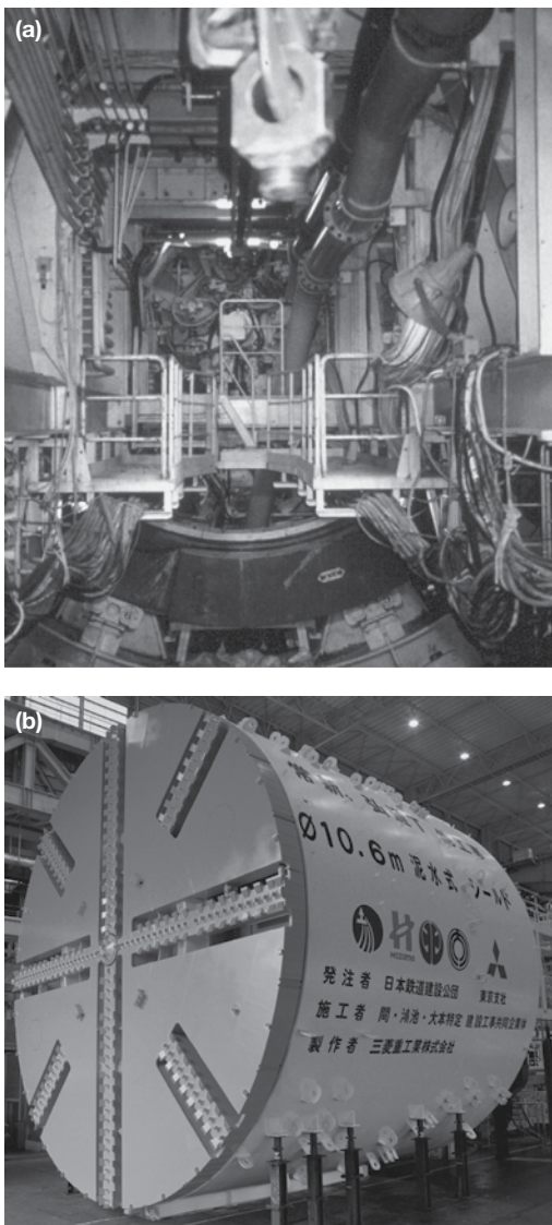
Figure 5.27 (a) View taken towards the rear of a Mitsubishi 10.6 m diameter slurry machine used in Japan (note the two slurry pipes at the top right, one for passing the slurry into the machine, which enters at the top of the shield, and one for removing the slurry and excavated material, which comes from the bottom of the shield) and (b) the full STBM in the factory showing the cutterhead. (Courtesy of Mitsubishi Heavy Industries Mechatronics Systems Ltd.)
