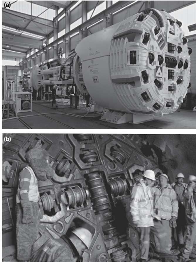
Figure 5.19 (a) and (b) 5.03 m diameter Herrenknecht S-351 gripper TBM used at Glendoe, UK. (Courtesy of Herrenknecht.)
