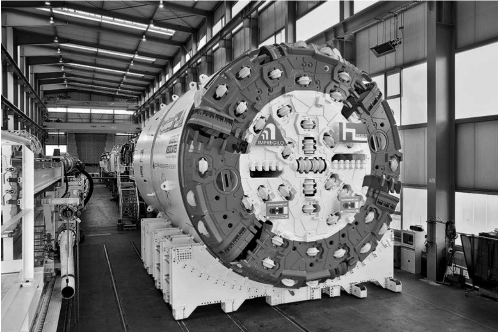
Figure 8.61 A 7.18 m diameter Herrenknecht multimode TBM used to construct the Lake Mead Intake No. 3, Las Vegas, USA. (Courtesy of Herrenknecht.)
