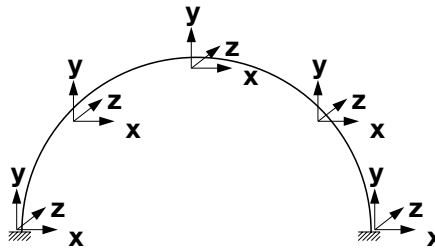
Figure 7.21 Minimum required monitoring points to create a deflected shape.
