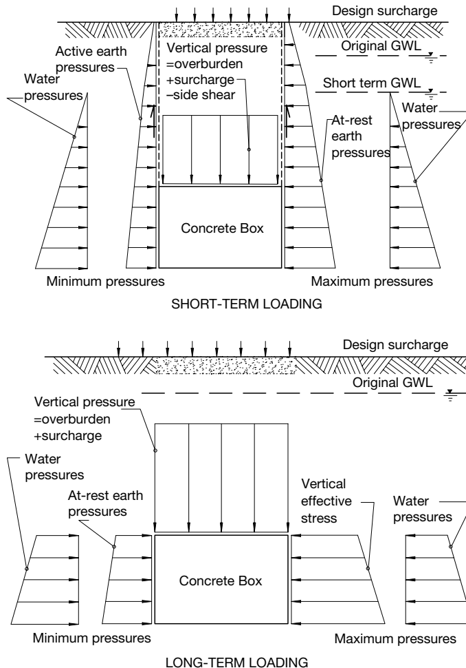
Figure 5.59 Example of design loadings in the short- and long-term for a concrete box structure. (After Kuesel and King 1996.)
