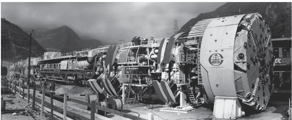
Figure 5.18 Gripper machine with multiple 'X' formation gripper shoes (diameter 8.8 m, length 5.7 km, through Gneiss in Quinling China). (Courtesy of Aker Wirth.)
