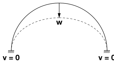
Figure 7.17 Roof settlement. (Rokahr et al. 2002.)
