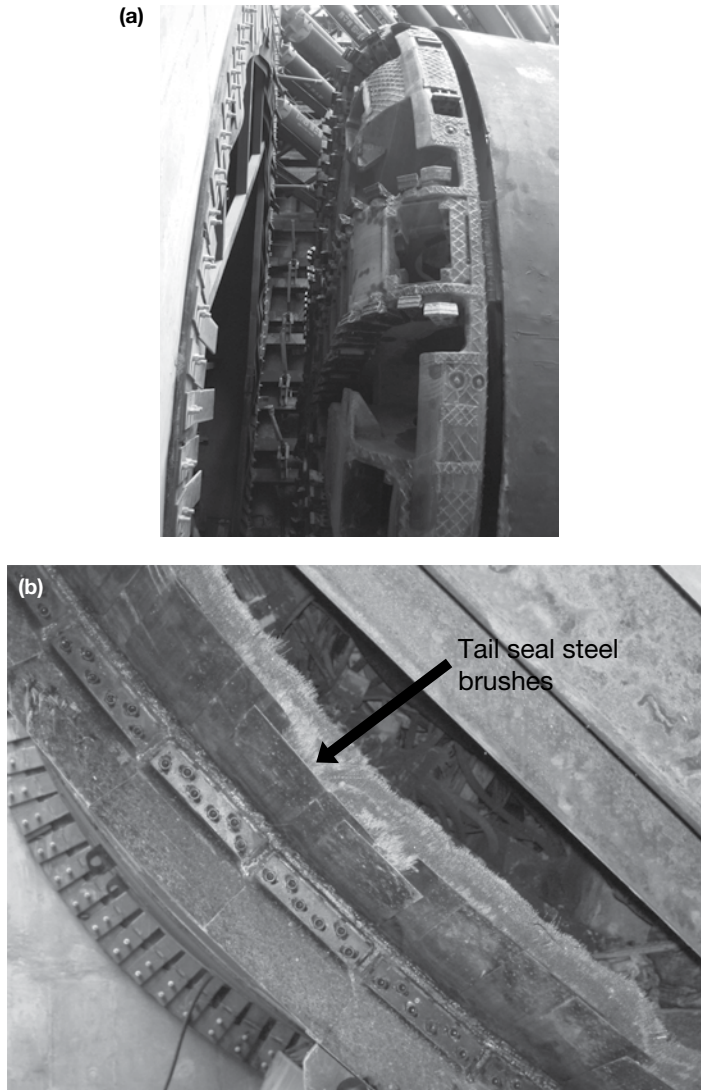
Figure 5.13 (a) 7.590 m diameter EPBM just before it started excavating the second of two drives on the Seoul Subway Line 9 and (b) the rear of the same TBM showing a close-up of the tail seal steel brushes.
