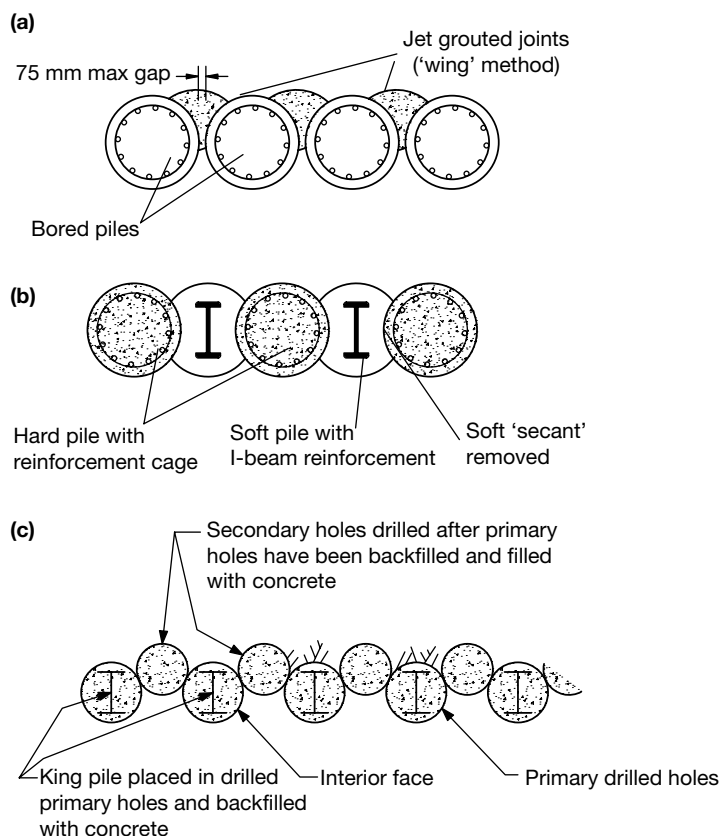
Figure 5.65 General arrangements for bored pile retaining walls, (a) contiguous pile wall and (b) secant pile wall (After Woodward 2005.) and (c) off-set bored pile wall. (After Kuesel and King 1996.)
