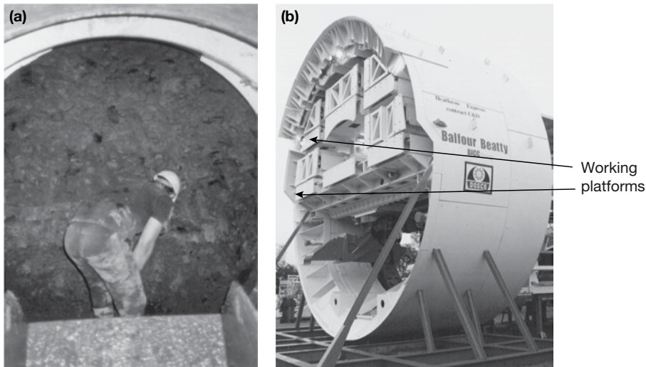
Figure 5.6 (a) Manual shield tunnelling as part of a pipe jacking operation and (b) a 9.17 m diameter open shield. (Courtesy of Dosco Overseas Engineering Ltd.)
