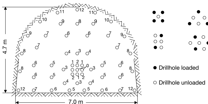
Figure 5.50 Example of the burn cut positioned close to the centre of the face showing examples of the loaded and unloaded drill hole pattern.
