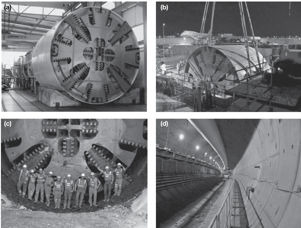
Figure 5.33 Heathrow Airside Road Tunnel, UK, (a) 9.16 m diameter Herrenknecht S-185 EPBM, (b) lowering the EPBM into the starting shaft, (c) breakthrough and (d) the completed concrete segmental lined tunnel. (Courtesy of Herrenknecht.)
