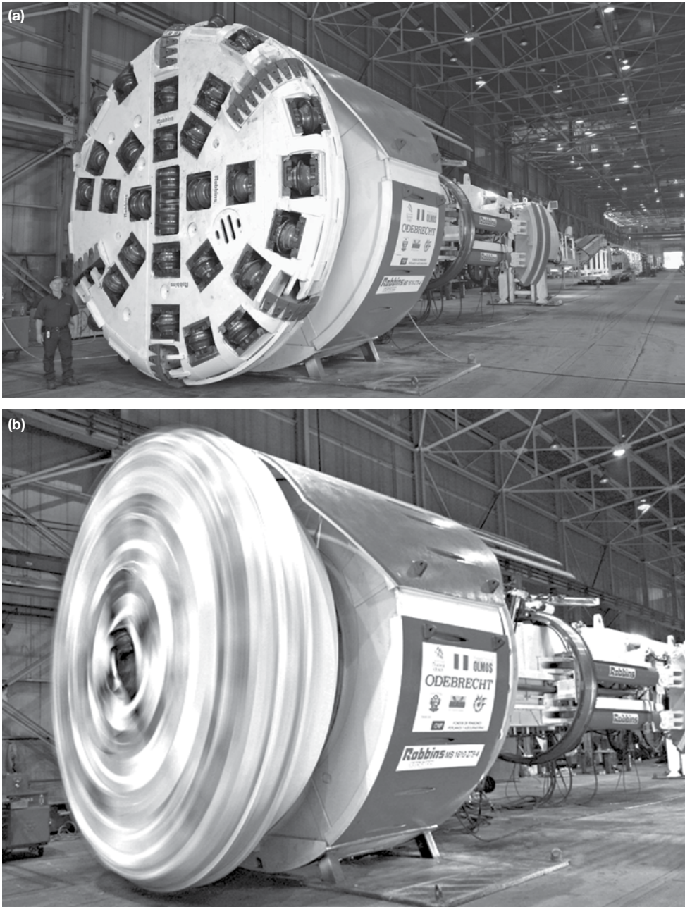
Figure 8.53 (a) and (b) a 5.30 m diameter Robbins Main Beam TBM used on the Olmos Trans-Andean Water Transfer Tunnel, Peru. (Courtesy of The Robbins Company.)
