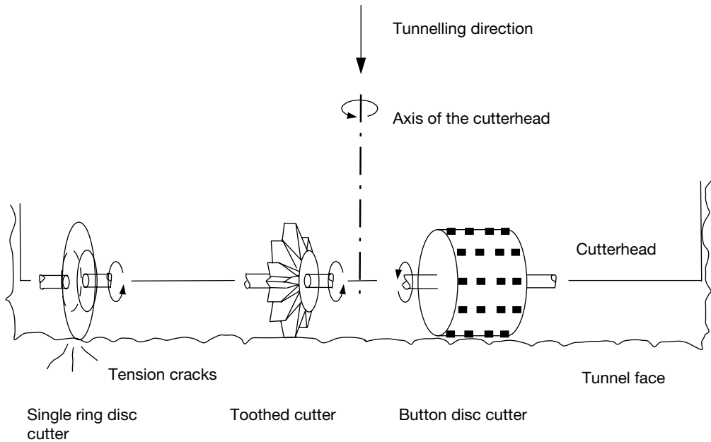
Figure 5.22 Different types of rotating excavation tools for hard rock (disc cutter, toothed cutter and button disc cutter).
