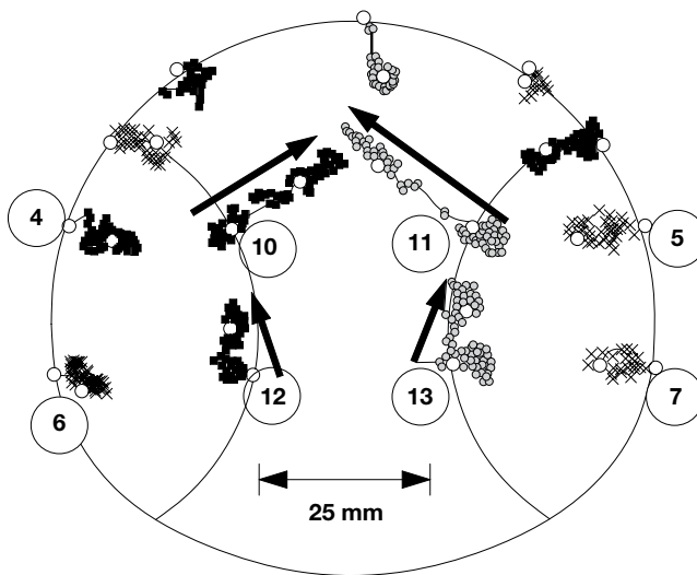
Figure 8.27 Displacements of the sidewall drift during excavation of Centre Drift I, section W, Chainage 60.
