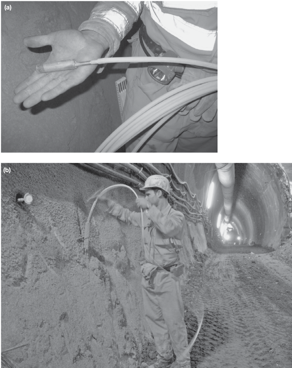
Figure 8.1 (a) 'Eggemouse' and (b) invert control with the 'Eggemouse' at the Lainzer Tunnel LT31, Vienna, Austria.
