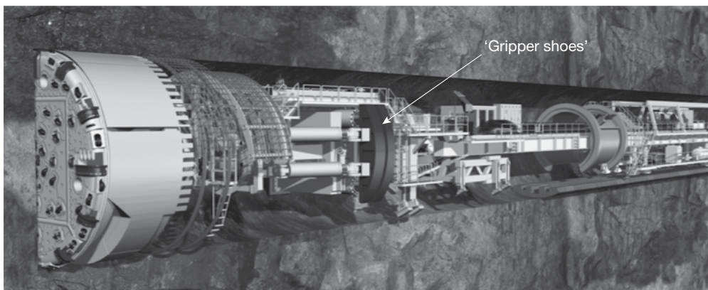
Figure 5.15 Gripper TBM. (Courtesy of Herrenknecht.)
