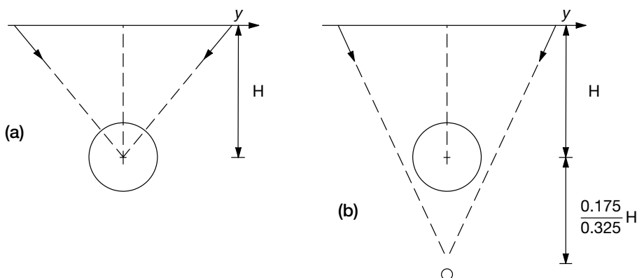
Figure 7.5 Direction of the ground displacement vectors above tunnels in clay (After Mair and Taylor 1997), (a) vectors directed towards axis (Attewell 1978, O'Reilly and New 1982.) and (b) vectors directed towards point O. (Taylor 1995b.)
