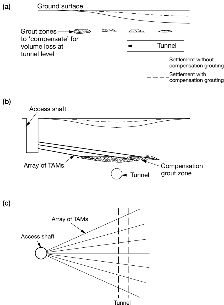
Figure 4.15 Compensation grouting for tunnel construction. (a) longitudinal section, (b) cross section and (c) plan. (After Woodward 2005 and Burland et al. 2001a.)
