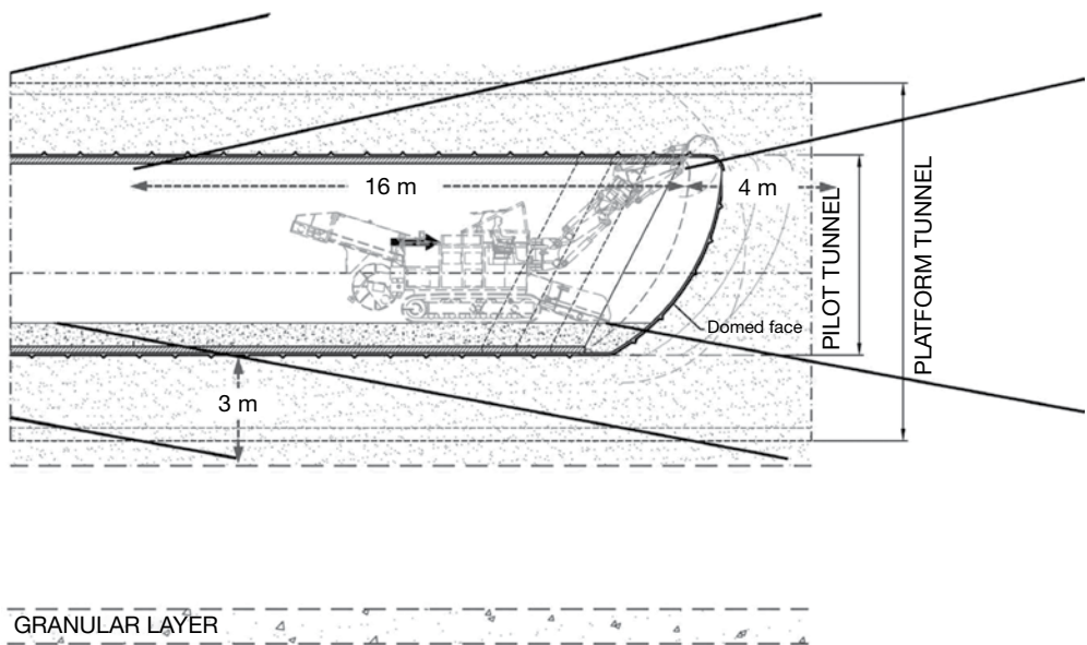
Figure 8.42 Phase 1 probing ahead of the Pilot tunnel. (Graphic Credit: Crossrail Ltd., used with permission.)
