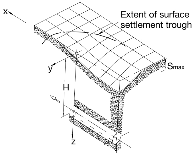
Figure 7.4 3D representation of the surface settlement as a tunnel is constructed in soft ground. (Attewell 1995, after Yeates 1985.)
