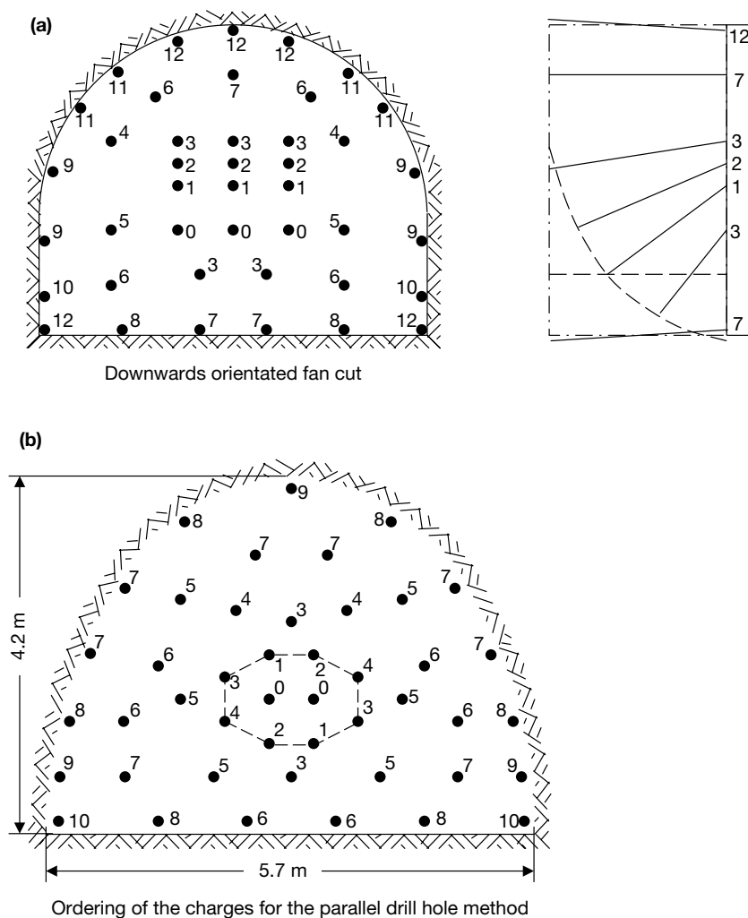
Figure 5.49 (a) Fan cut and (b) parallel drill hole method (the numbers against the drill holes indicate the order of blasting).
