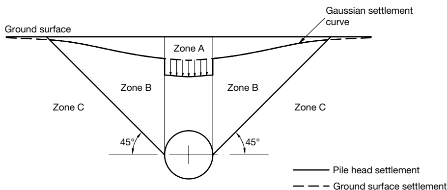
Figure 7.7 Zones of influence of pile settlement due to EPB shield tunnelling in London Clay. (After Selemetas et al. 2006.)
