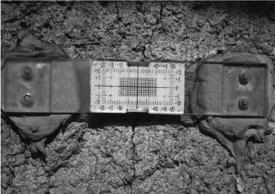
Figure 7.24 Tell Tale™ placed over a crack in sprayed concrete lining.
