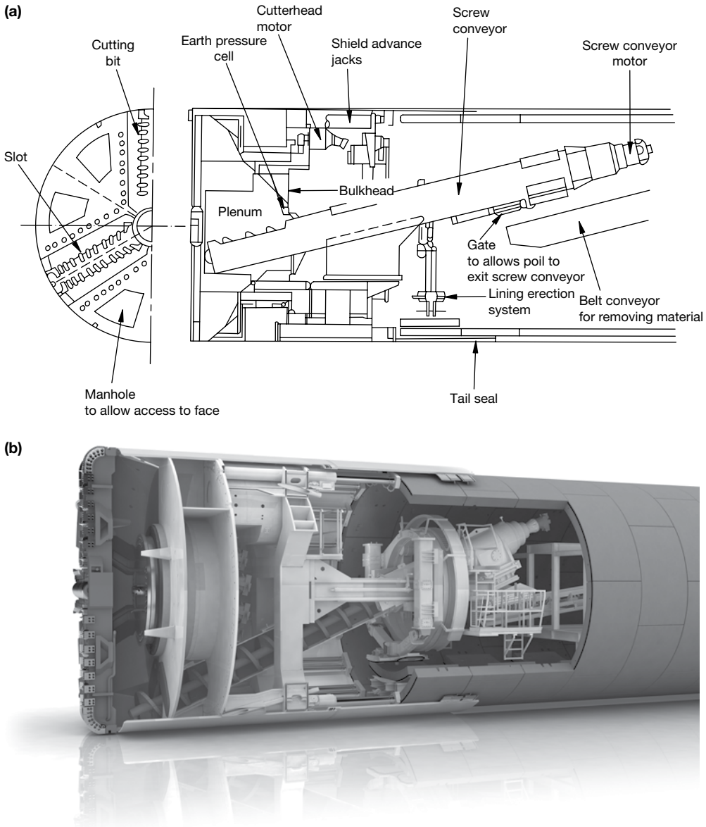
Figure 5.31 (a) Longitudinal section through an EPBM. (After Clough, 1983.) and (b) 3D schematic representation of an EPBM. (Courtesy of Herrenknecht.)
