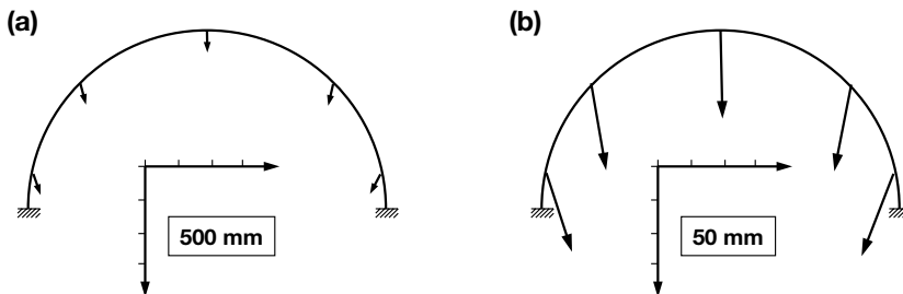
Figure 7.22 (a) and (b) Vertical and horizontal displacements plotted as x - y -vectors using different scales. (Rokahr et al. 2002.)
