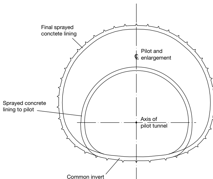
Figure 5.57 (Continued) Possible excavation sequences for SCL (and NATM). (After ICE 1996, used with permission from ICE Publishing.)
