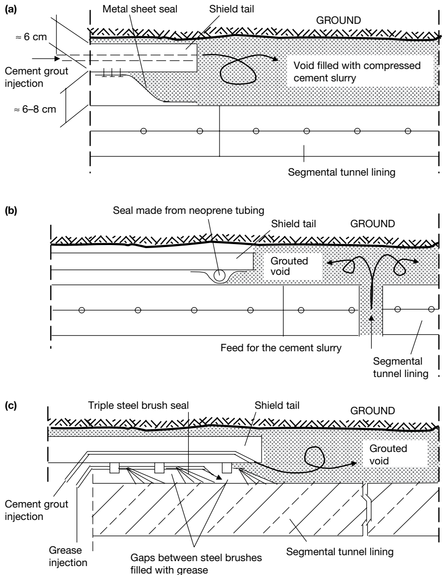
Figure 5.12 Different shield tail sealing systems, (a) metal sheet (b) neoprene tube and (c) steel brushes.
