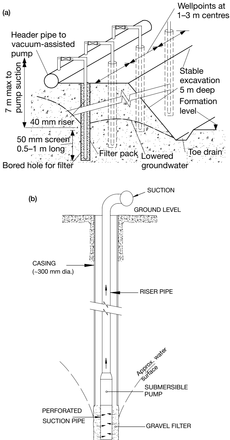
Figure 4.4 (a) Typical wellpoint arrangement. (After Woodward 2005.) (b) Details of a deep well arrangement. (After Megaw and Bartlett 1982, used with permission from John Bartlett.)
