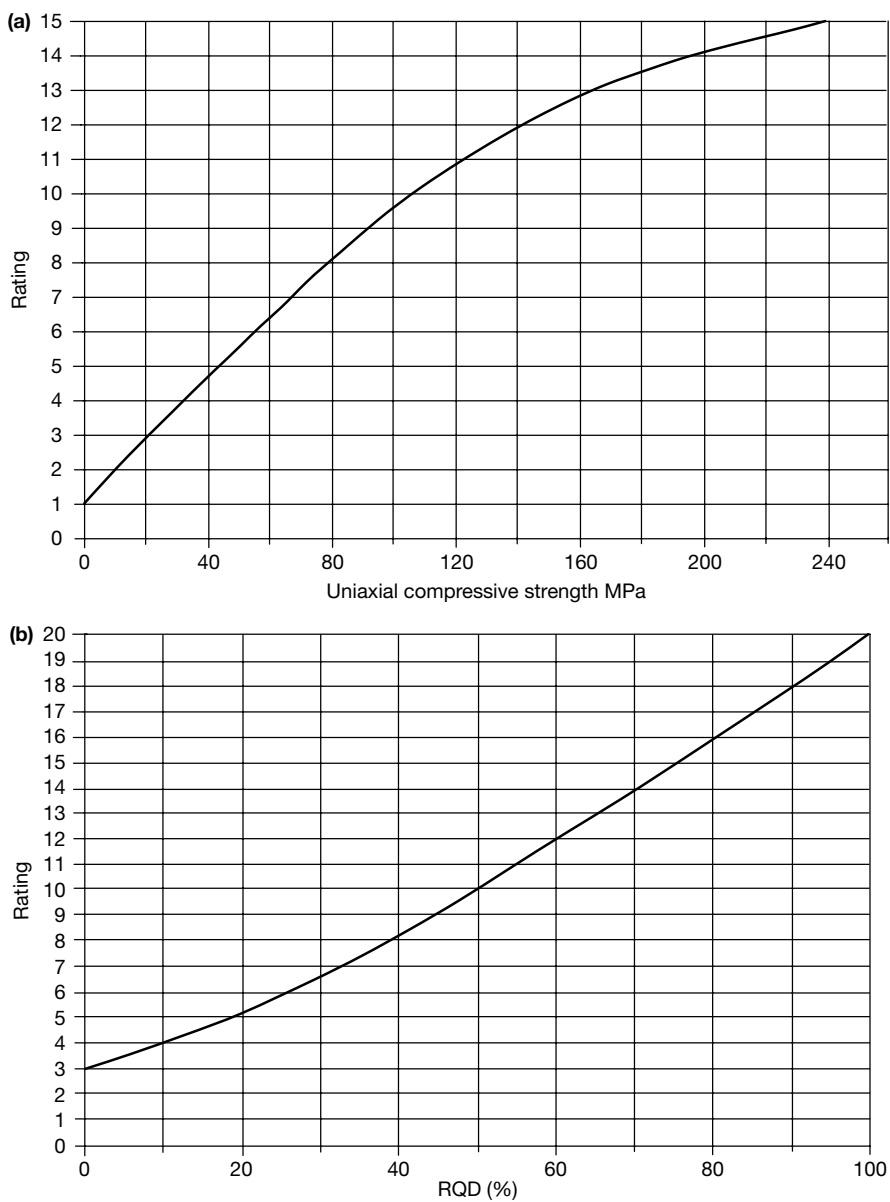
Figure A.1 Charts for various RMR ratings. (a) Chart A ratings for strength of intact rock, (b) Chart B ratings for RQD. (Continued)
