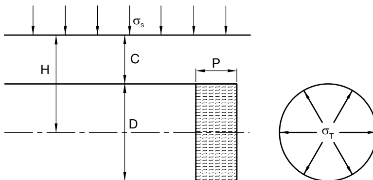
Figure 3.2 Stability parameters. (After ITA/AITES 2007.)
