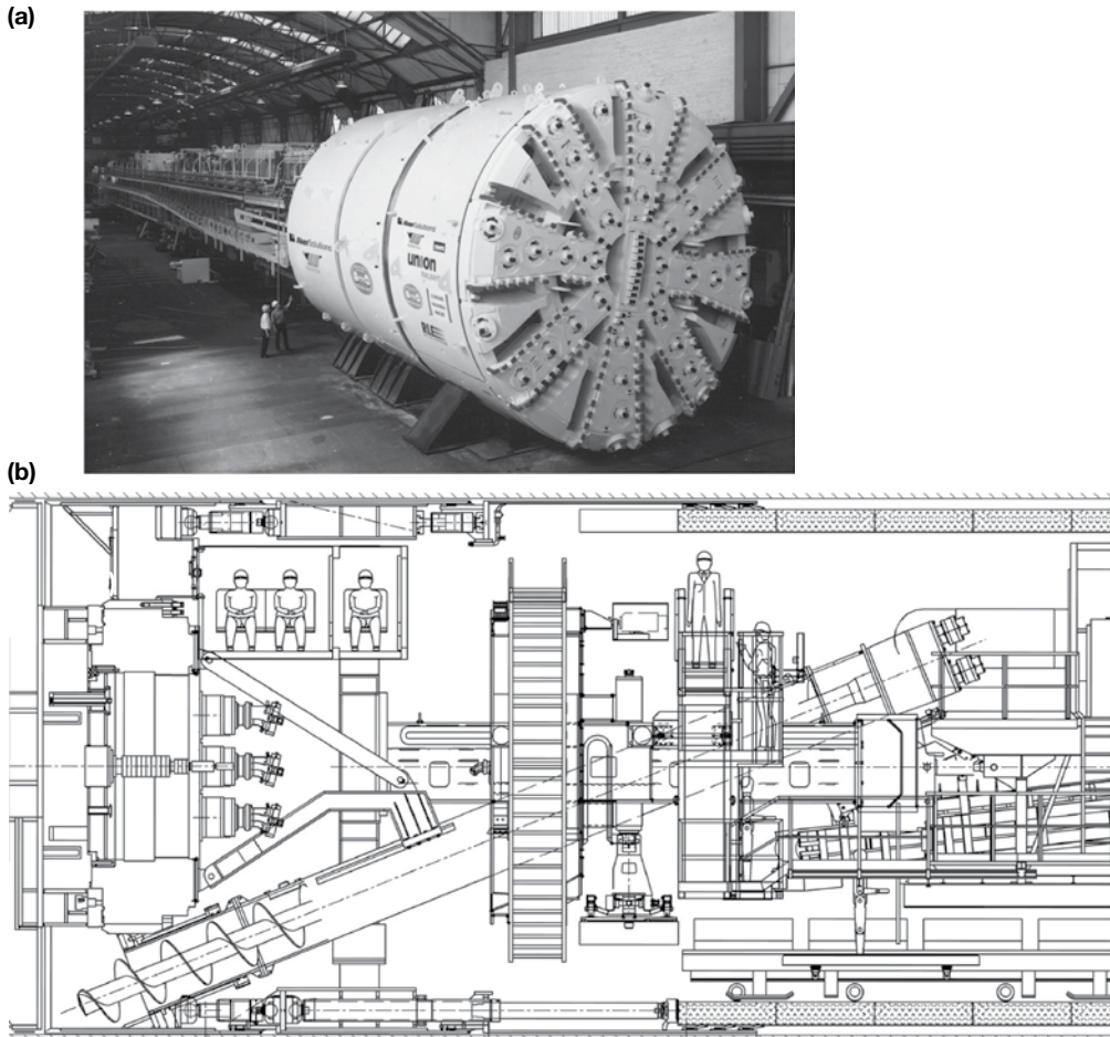
Figure 5.34 (a) 8.16 m diameter EPB machine used on the CTRL project in the United Kingdom and (b) schematic longitudinal section through this machine. (Courtesy of Aker Wirth.)
