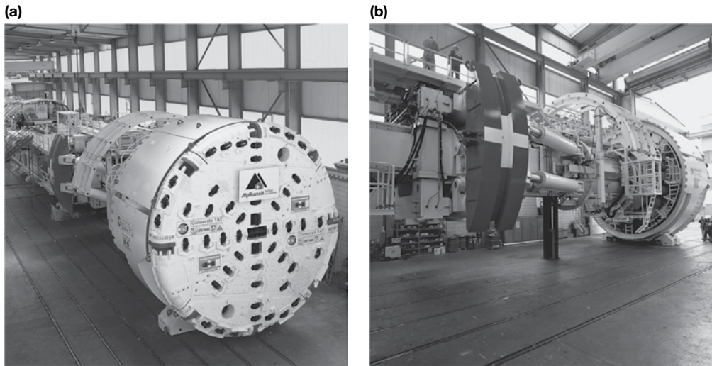
Figure 5.17 8.83 m diameter Herrenknecht S-210 gripper TBM used on the Gotthard Base Tunnel in Switzerland, (a) cutter head and (b) rear view showing gripper shoe. (Courtesy of Herrenknecht.)
