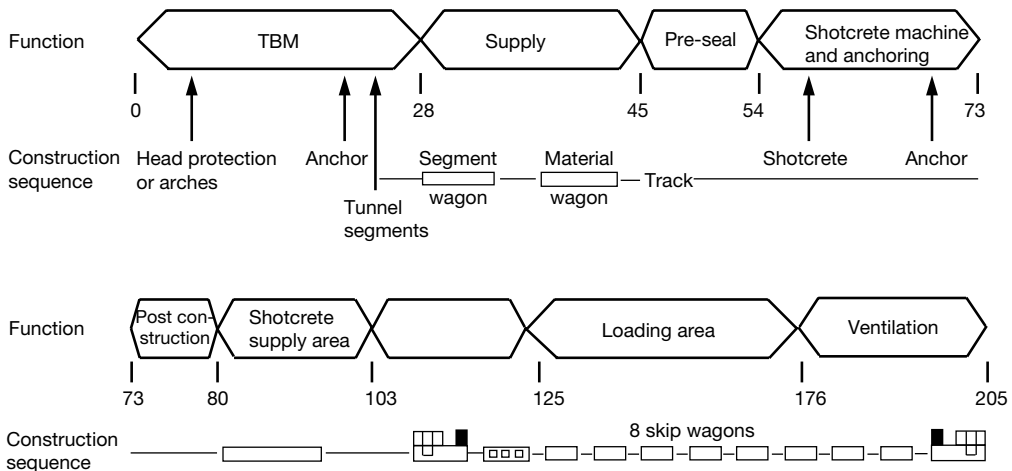
Figure 5.16 Example of the functions associated with a gripper TBM and typical lengths in metres, with tunnel support using a combination of invert segments and sprayed concrete. (After BetonKalender. 2005. Fertigteile und Tunnelbauwerke , Vols 1 and 2. Ernst & Sohn, Berlin, used with permission from Rowa Tunnelling Logistics.)
