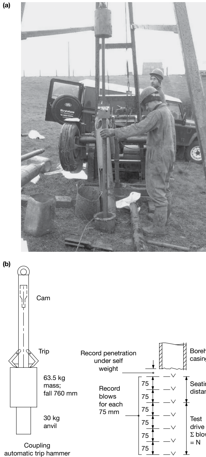
Figure 2.9 (a) SPT carried out using a cable percussion rig (shell and auger) (Courtesy of Soil Mechanics.). (b) Schematic representation of the SPT automatic trip hammer arrangement and procedure. (Courtesy of Dr. J. Billam.).
