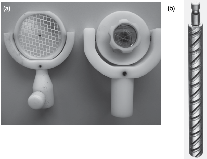
Figure 7.9 (a) Monitoring targets: Bireflex target (LHS), prism target (RHS) and (b) bolt on which the monitoring targets are mounted.
