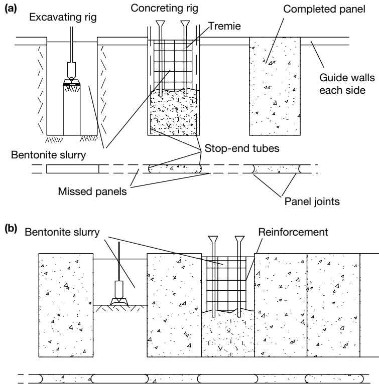
Figure 5.63 Typical construction process for a cast in situ diaphragm wall, (a) primary panels and (b) secondary panels. (After Woodward 2005.)
