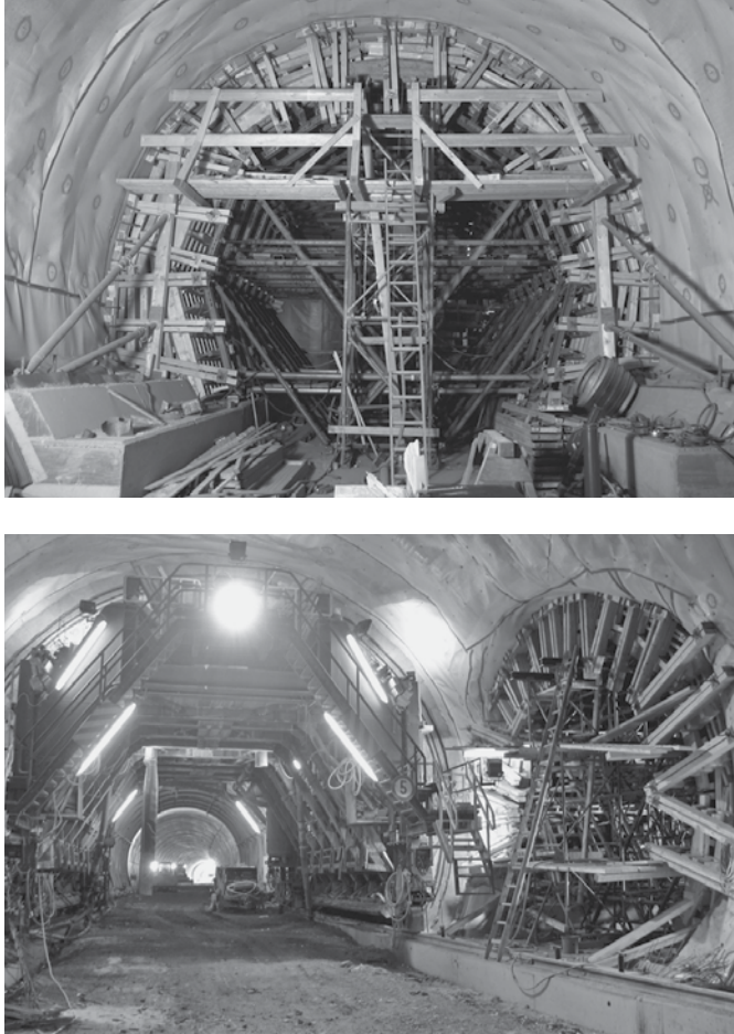
Figure 4.29 Inner lining construction, including waterproofing as used for the emergency cross-passage, HKT, Germany. (Courtesy of BeMo Tunnelling GmbH Innsbruck.)
