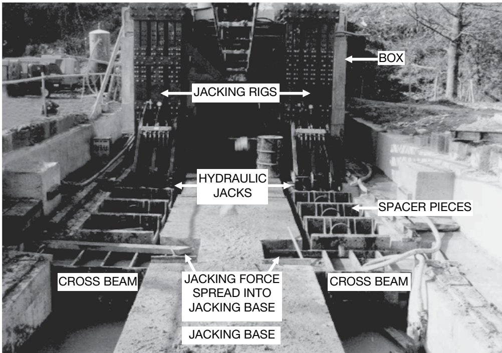
Figure 5.78 Example of jacking equipment and how the reaction forces are passed into the jacking base. (Allenby and Ropkins 2007, courtesy of BAM Nuttall Ltd. and John Ropkins Ltd.)
