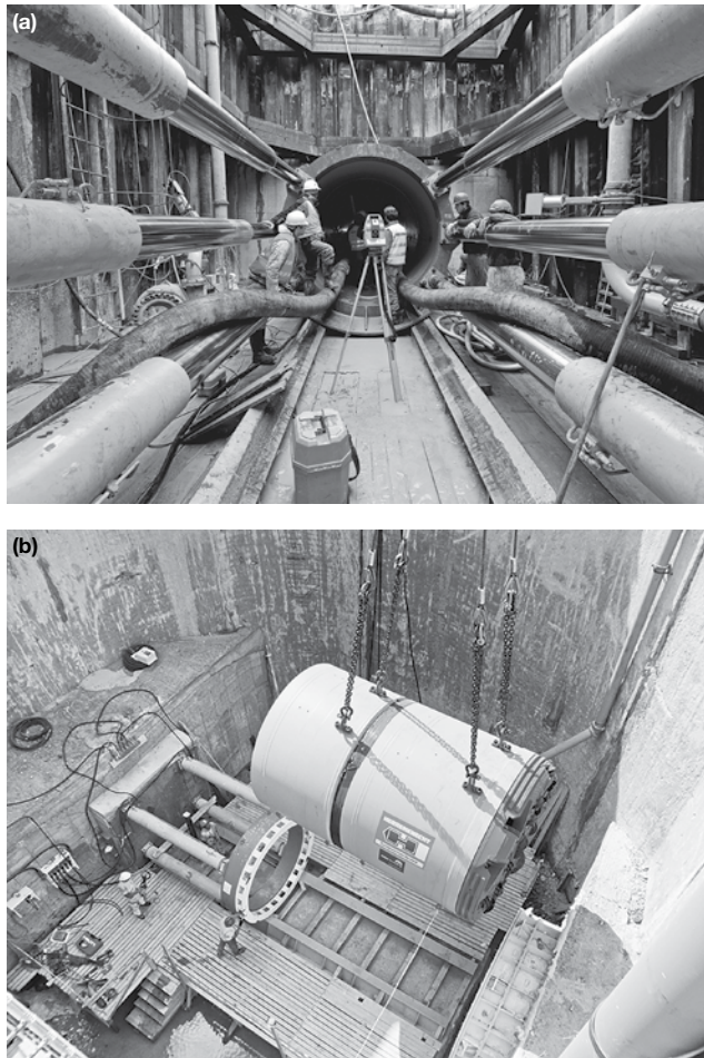
Figure 5.90 (a) View from the bottom of the jacking pit, (b) a microtunnelling machine being lowered in the jacking pit (Continued)
