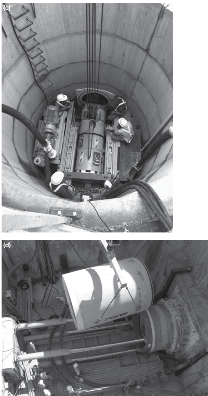
Figure 5.90 (Continued) (c) a microtunnelling machine set up at the bottom of the jacking pit and (d) a concrete jacking pipe being lowered into the jacking pit. (All photographs courtesy of Herrenknecht or the Pipe Jacking Association.)
