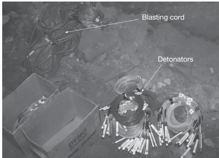
Figure 5.46 Detonators and blasting cord as used on the Katschberg Tunnel, Austria.
