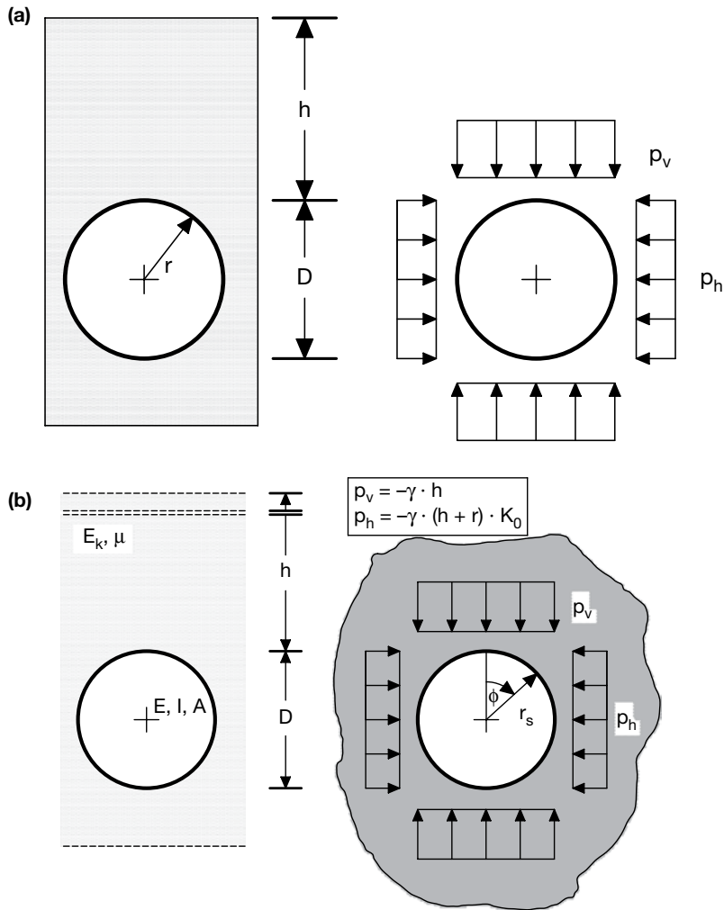
Figure B.1 (a) Analytical model for deep tunnels and (b) primary loads. (Ahrens et al. 1982.)
