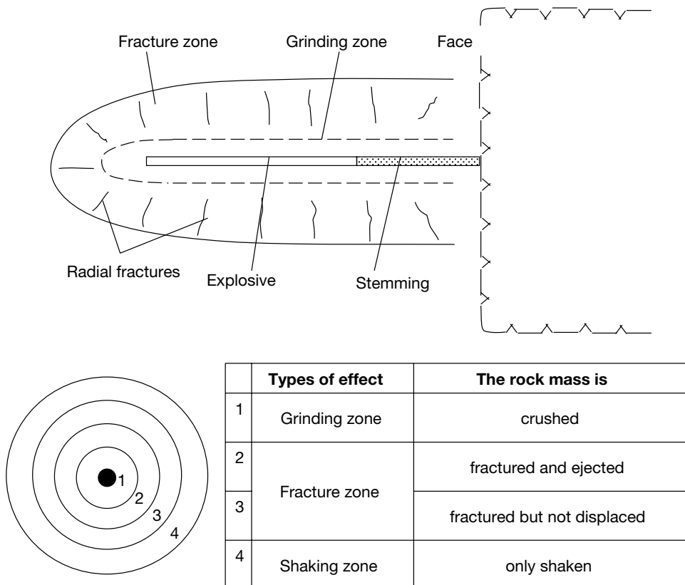
Figure 5.44 Affected zones around an explosion at the tunnel face.
