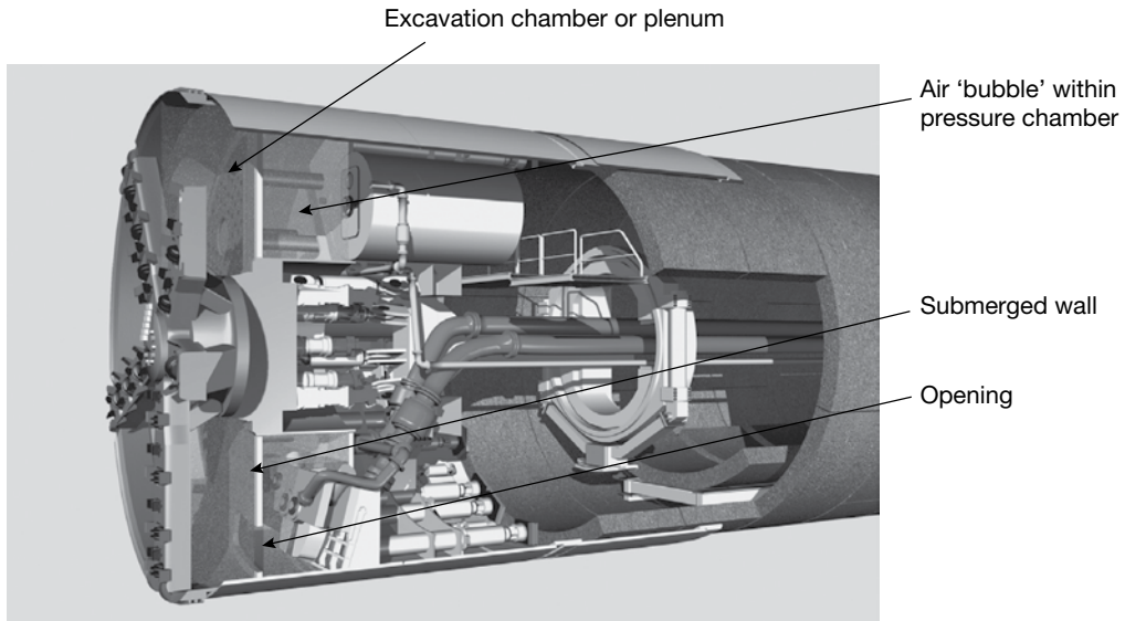
Figure 5.28 Mixshield TBM. (Courtesy of Herrenknecht.)
