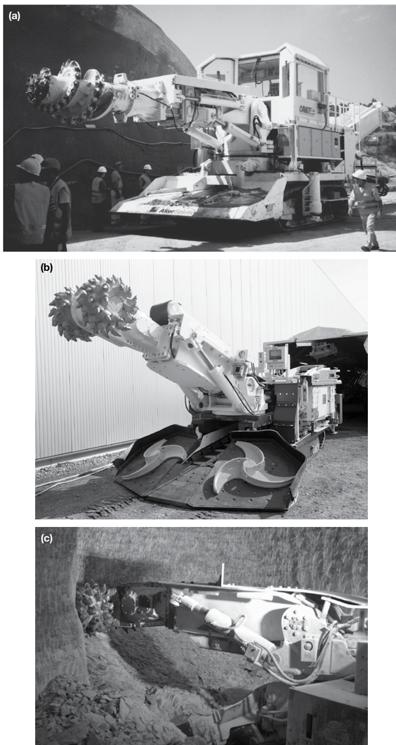
Figure 5.4 Example partial face boring machines (roadheaders), (a) with an axial cutterhead (Courtesy of Aker Wirth.) and (b) and (c) with a transverse cutterhead. (Courtesy of IBS Industriemaschinen-Bergbau-Service GmbH.)
