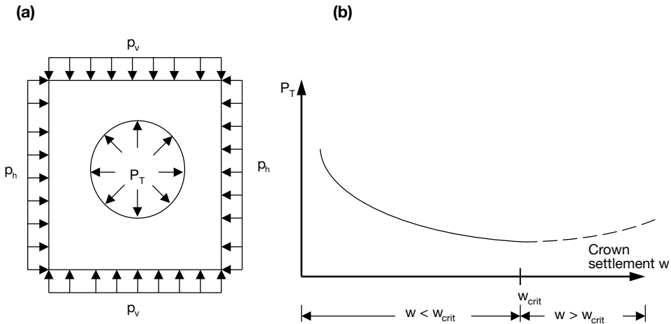
Figure 3.7 Tunnel support resistance method. (a) Structural system and (b) Fenner–Pacher curve.
