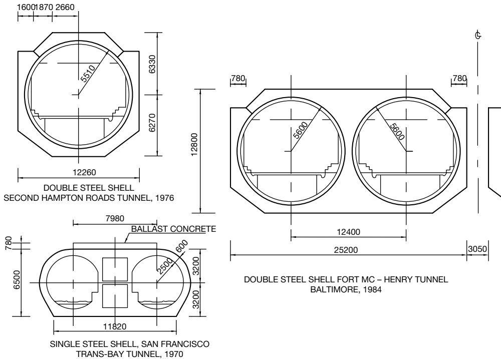
Figure 5.68 Typical cross sections for steel shell immersed tube tunnels (all dimensions in mm). (After ITA 1997.)
