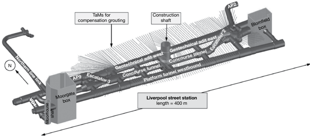
Figure 8.40 Liverpool Street Station layout. (Note: the Broadgate Ticket Hall at the end of AP2, to the north of the Blomfield Box, is not shown for clarity.) (Graphic Credit: Crossrail Ltd., used with permission.)
