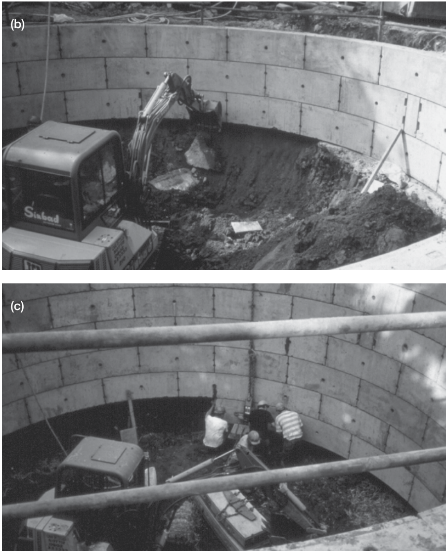
Figure 4.26 (Continued) (b) shows the excavation process and (c) shows the installation of the concrete segments.
