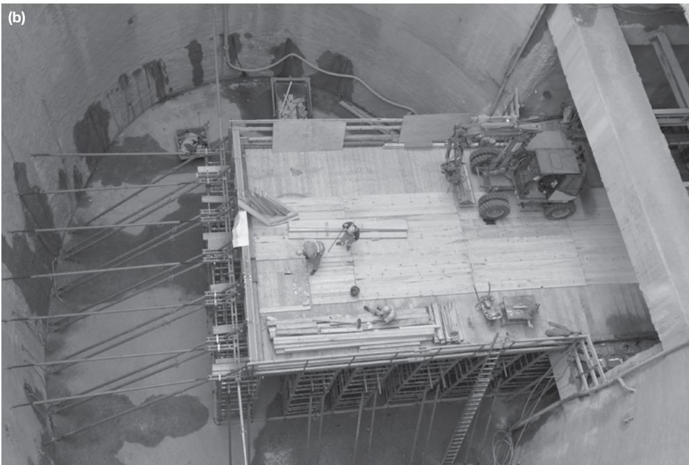
Figure 8.18 (a) Shaft 'Klimtgasse'. Excavation platform with planking nearly finished. Shaft walls appear curved due to wide angle of photo. (b) Excavation platform. Shoring towers in place, web girders are laid close together and covered in planking.
