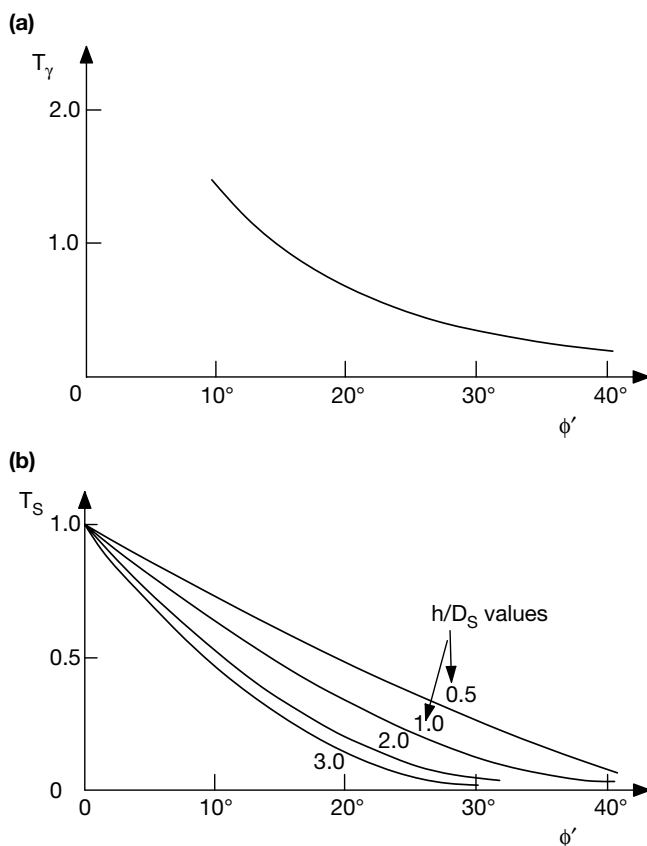
Figure 3.4 (a) Determination of the tunnel stability number in coarse-grained soils for the soil load and (b) determination of the tunnel stability number in coarse-grained soil for the surface surcharge. (After Thomson 1995, from Atkinson and Mair 1981, reproduced with permission from Emap Ltd and Springer.)
