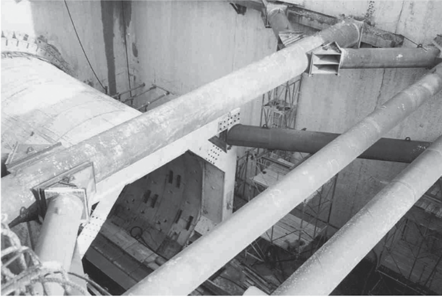
Figure 5.11 Example of a reaction frame used to start off a TBM.
