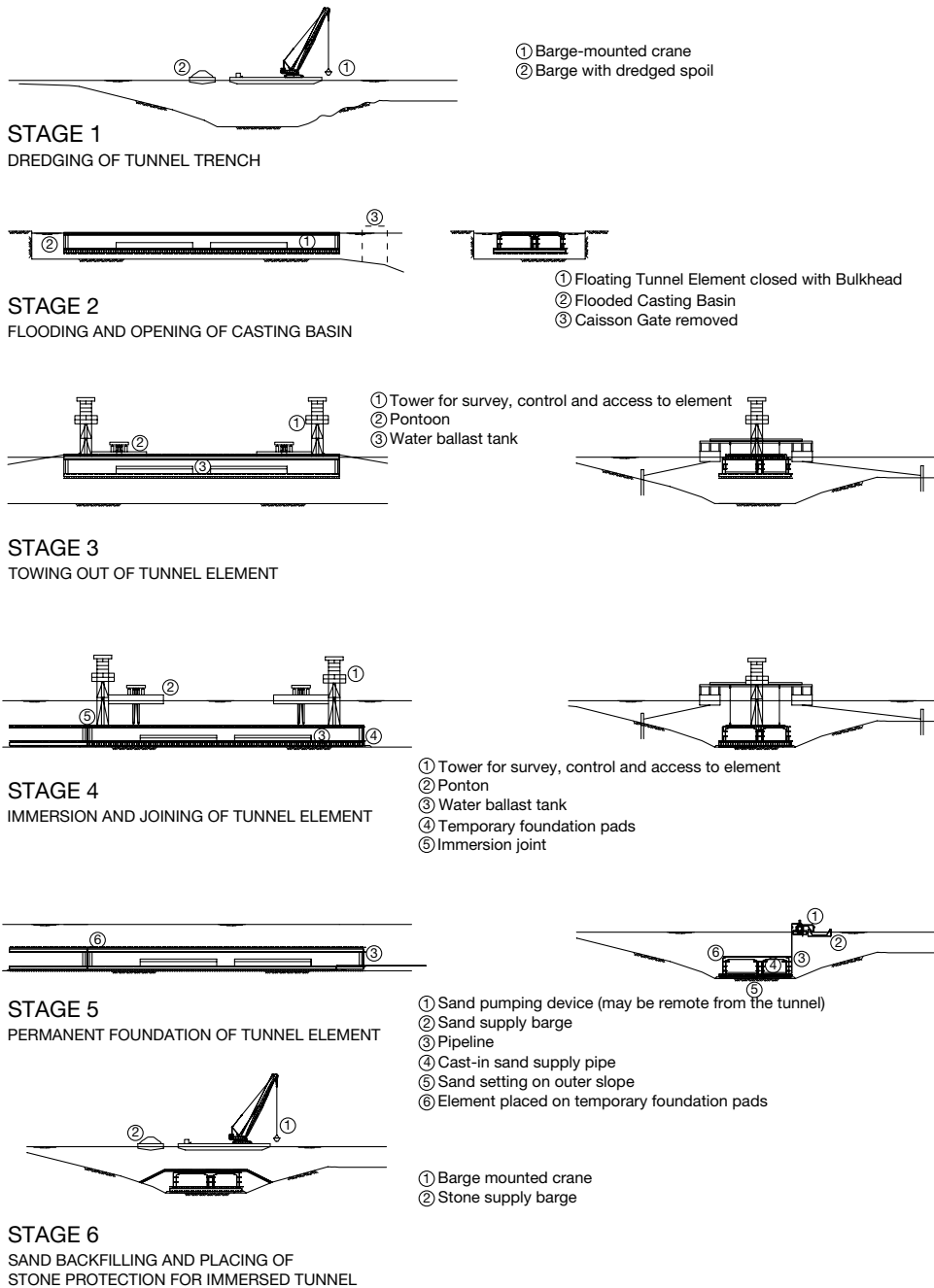
Figure 5.67 Typical sequence for the construction of an immersed tube tunnel. (Courtesy of COWI A/S.)
