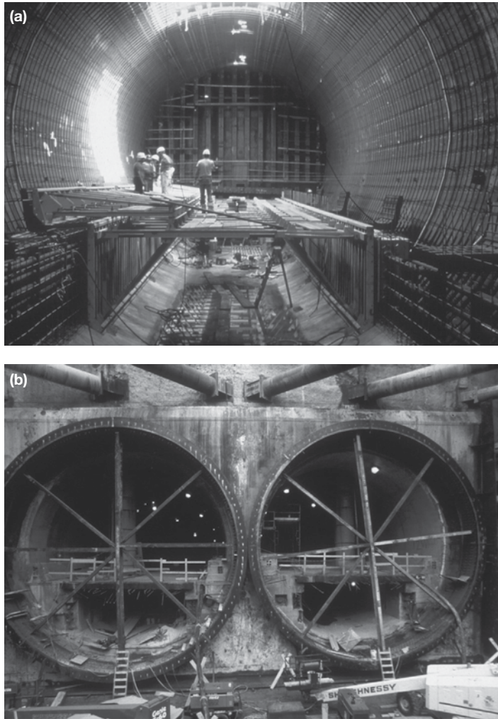
Figure 5.75 (a) Internal fitting out of one of the tunnel elements (a reinforced concrete lining was placed inside the steel shell) and (b) the binocular immersed tube emerging into the cut-and-cover section of the Ted Williams Tunnel. (Courtesy of Massachusetts Turnpike Authority.)
