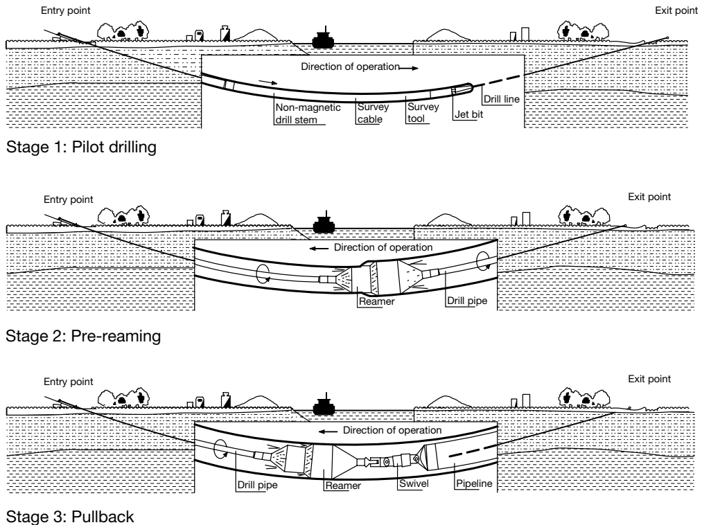
Figure 5.94 Typical HDD installation, including pilot drilling, pre-reaming and pullback operations (the central section of each stage is enlarged for clarity). (Courtesy of Herrenknecht.)
