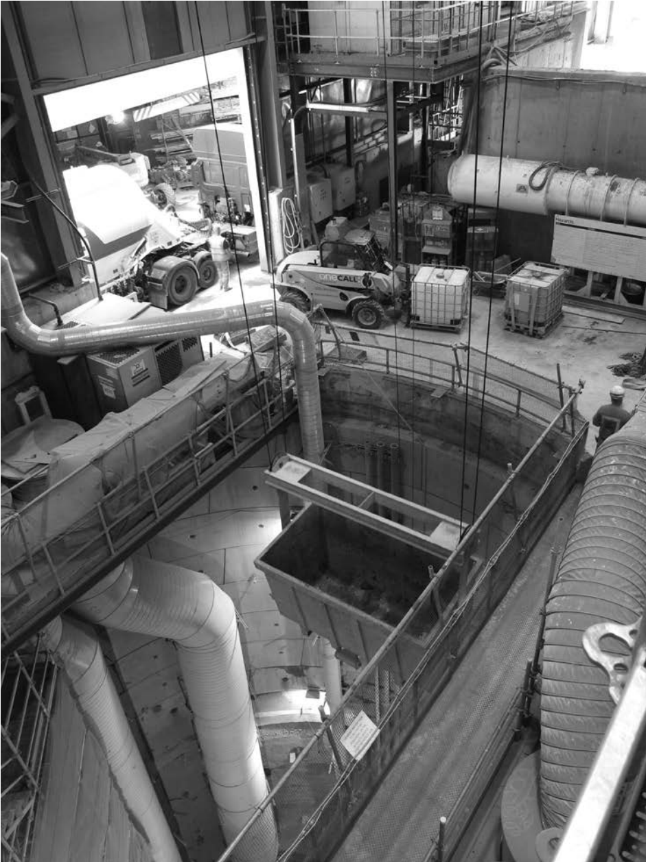
Figure 8.33 Whitechapel Station, acoustic shed. The muck bin is lowered into the construction shaft. To the left of the muck bin, two of the four ventilation ducts are visible. Further to the left, in the bottom corner is the stair tower for pedestrian access. (Photo Credit: Crossrail Ltd., used with permission.)
