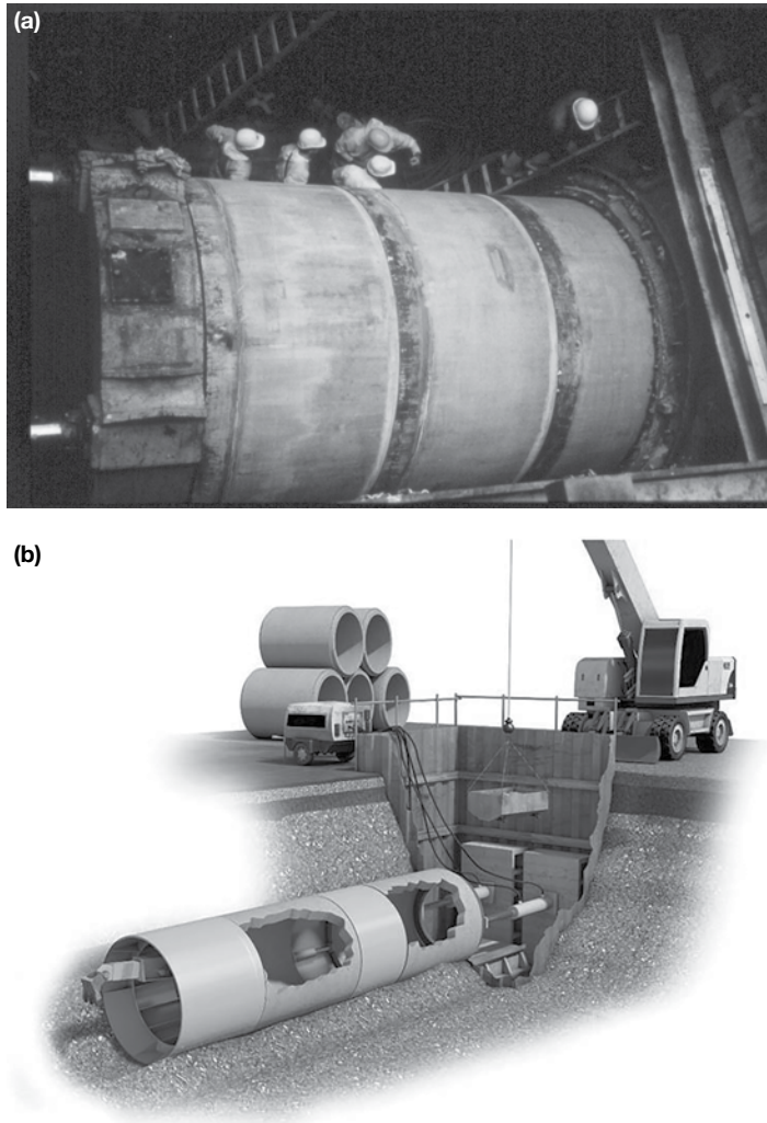
Figure 5.91 (a) Concrete pipes being jacked forwards, (b) a schematic representation of a pipe jacking operation (Courtesy of Herrenknecht.) (Continued)
