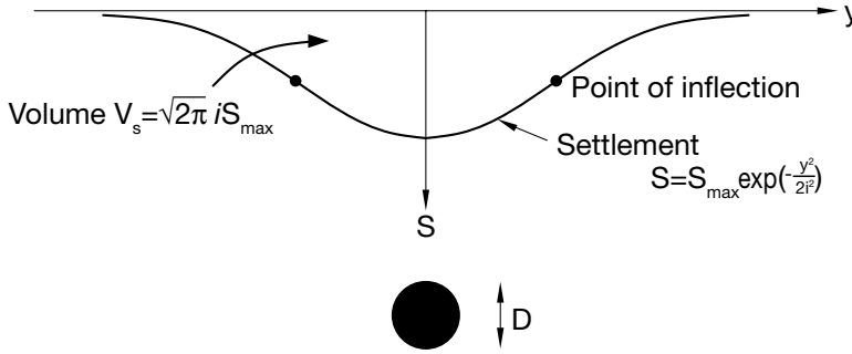
Figure 7.2 Gaussian curve for representing the transverse settlements above a tunnel in soft ground. (After Dimmock and Mair 2007a, used with permission from ICE Publishing and Professor Lord R.J. Mair.)
