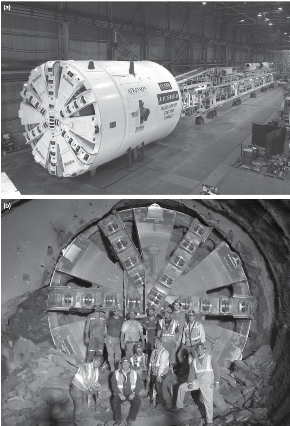
Figure 8.54 A 6.4 m diameter single-shield TBM used at Dulles Airport, Washington, USA, (a) in the factory and (b) at breakthrough. (Courtesy of The Robbins Company.)
