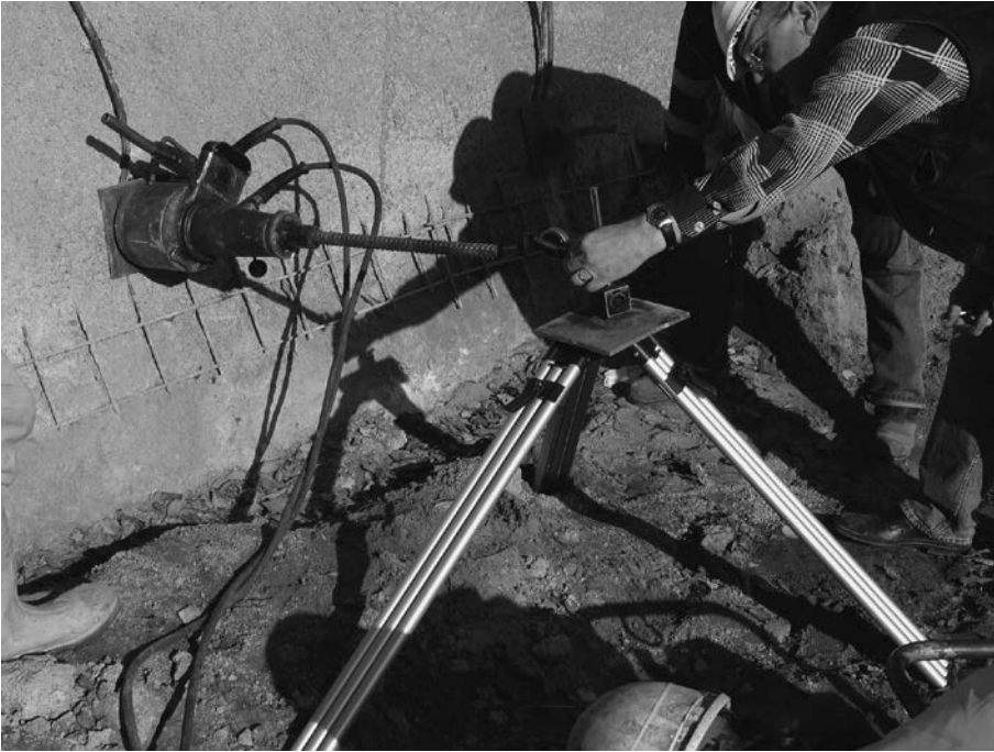
Figure 4.10 Load testing of an anchor, Lainzer Tunnel LT3I, Vienna, Austria.
