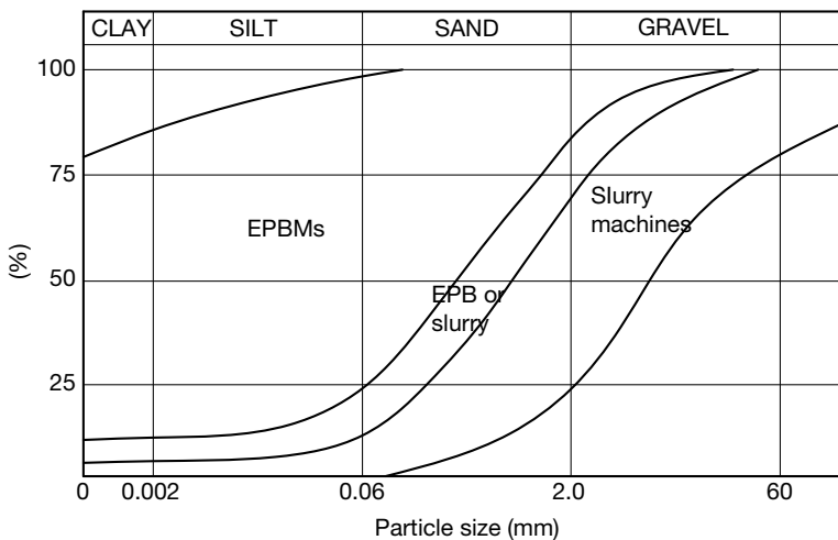
Figure 5.35 Graph of soil particle distribution curves related to the choice of EPB and slurry machines (STBM). (After BTS/ICE 2005, used with permission from ICE Publishing.)
