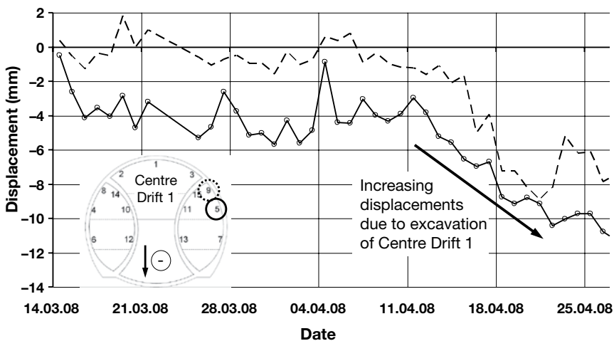
Figure 7.14 Displacement versus time graph showing the development of new displacements in the right-hand side wall drift following excavation of Centre Drift I (LT31, Vienna, Section W, Chainage 650).
