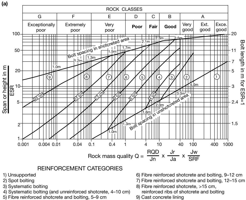
Figure 2.25 (a) Estimated support categories based on the Q-system. (After Grimstad and Barton 1993, reproduced from Palmström and Broch 2006.) (Continued)
