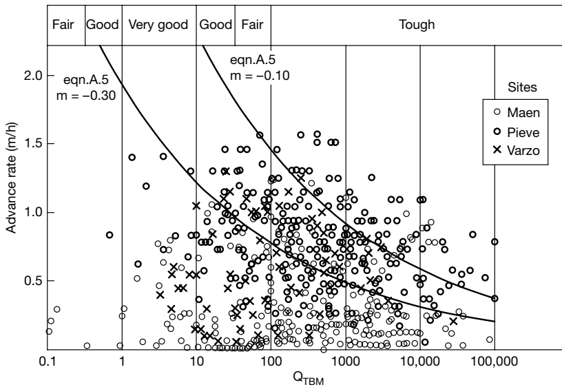
Figure A.2 AR for three TBM tunnels plotted against Q_{TBM} . (Sapigni et al. 2002, reproduced from Palmström and Broch 2006.)
