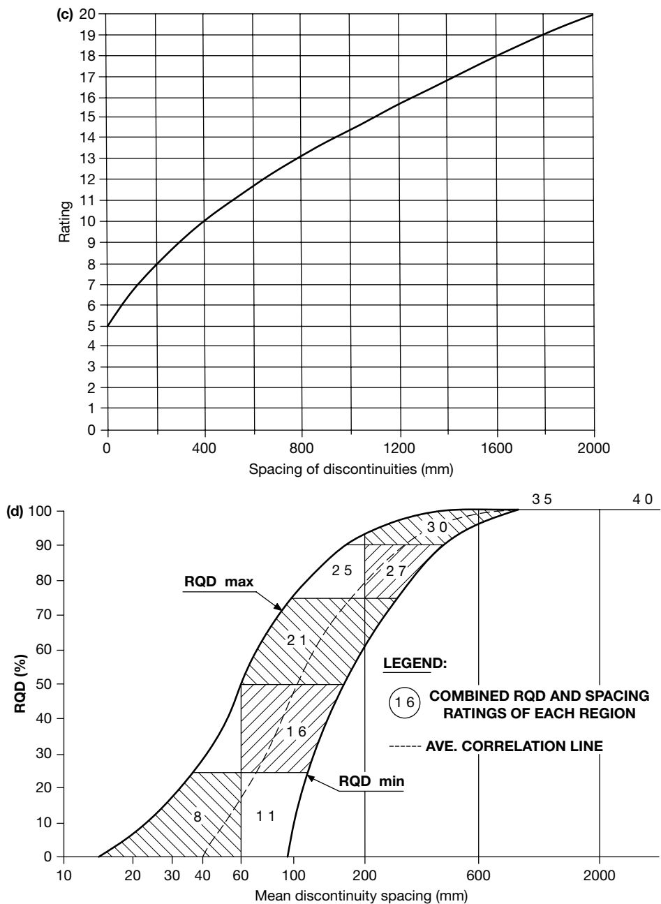
Figure A.1 (Continued) Charts for various RMR ratings. (c) Chart C ratings for discontinuity spacing and (d) Chart D correlation between RQD and discontinuity spacing. (After Bieniawski 1989.)
