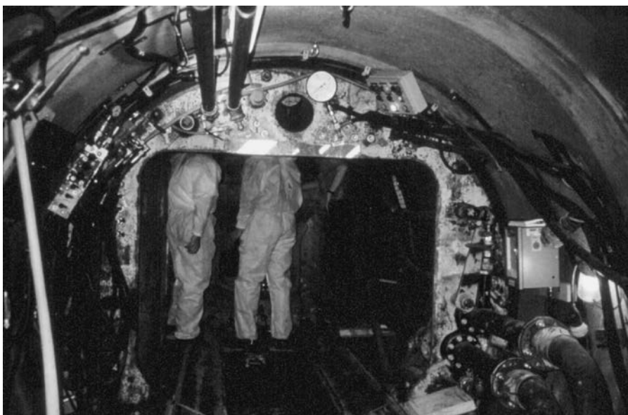
Figure 4.16 Airlock arrangement on a pipe jacking project for a new sewer in Germany (see Section 5.11 for a description of pipe jacking).
