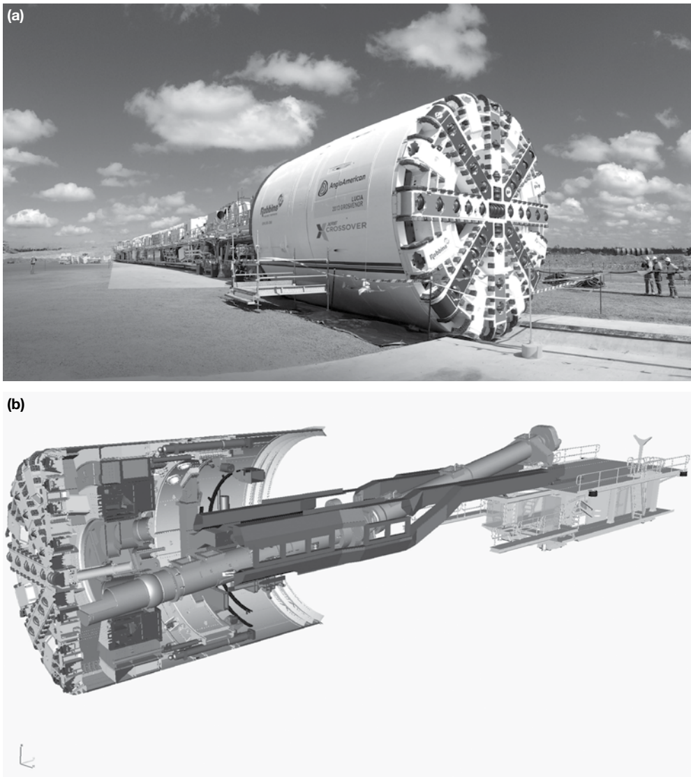
Figure 8.60 (a) and (b) An 8 m diameter Robbins XRE TBM used in the Grosvenor Coal Mine, Queensland, Australia. (Courtesy of The Robbins Company.)
