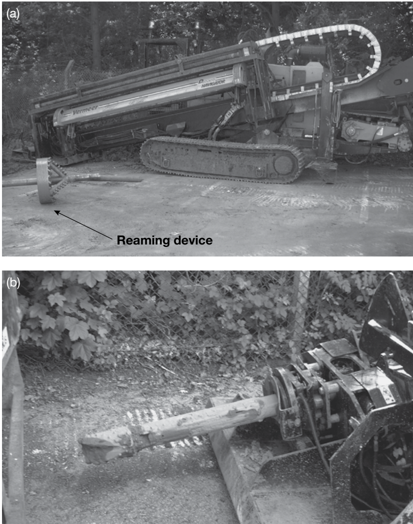
Figure 5.95 (a) An example of an HDD rig (note an example of a 'reaming' device beside the rig on the left) and (b) a close-up of the pilot drill head (note the 'chisel' type drill head with an angled face).
