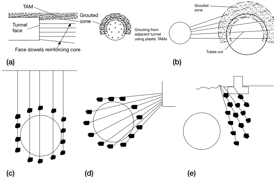
Figure 4.5 Examples of grouting tunnels during construction: (a) from within a tunnel, (b) using an adjacent tunnel (After Woodward 2005.), (c) from the ground surface, (d) from an adjacent shaft, or (e) as protection to adjacent structures. (After Baker 1982, used with permission from ASCE.)
