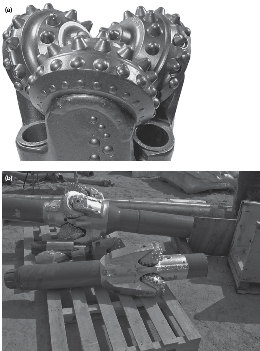
Figure 5.96 (a) Rock drill bit and (b) rock pre-reamer. (Courtesy of Prime Drilling HDD-Technology.)
