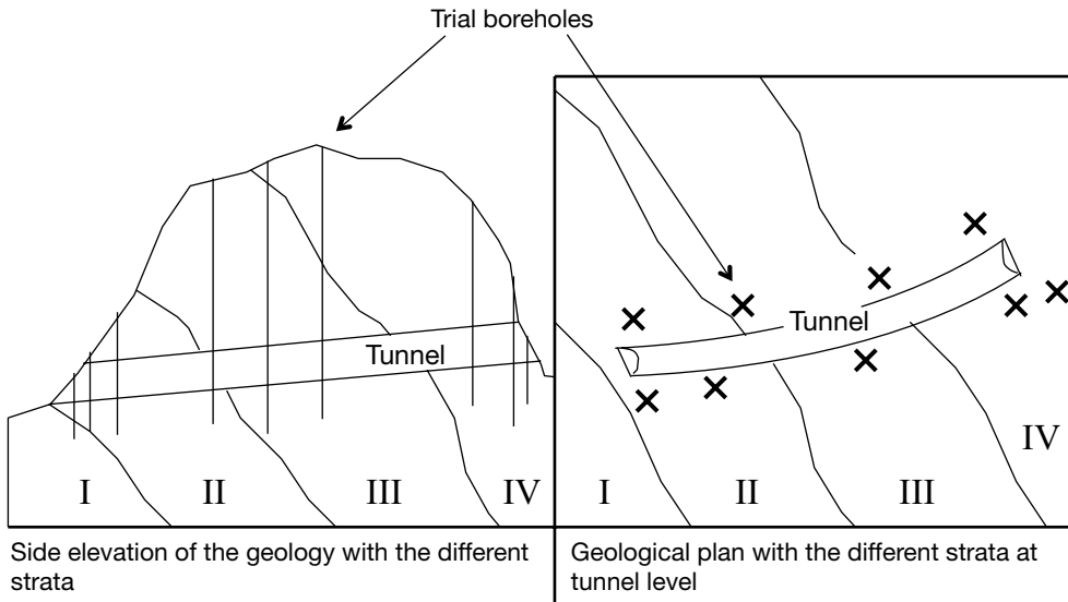
Figure 2.8 Possible borehole locations for a mountain tunnel. (Note: exaggerated vertical scale.)
