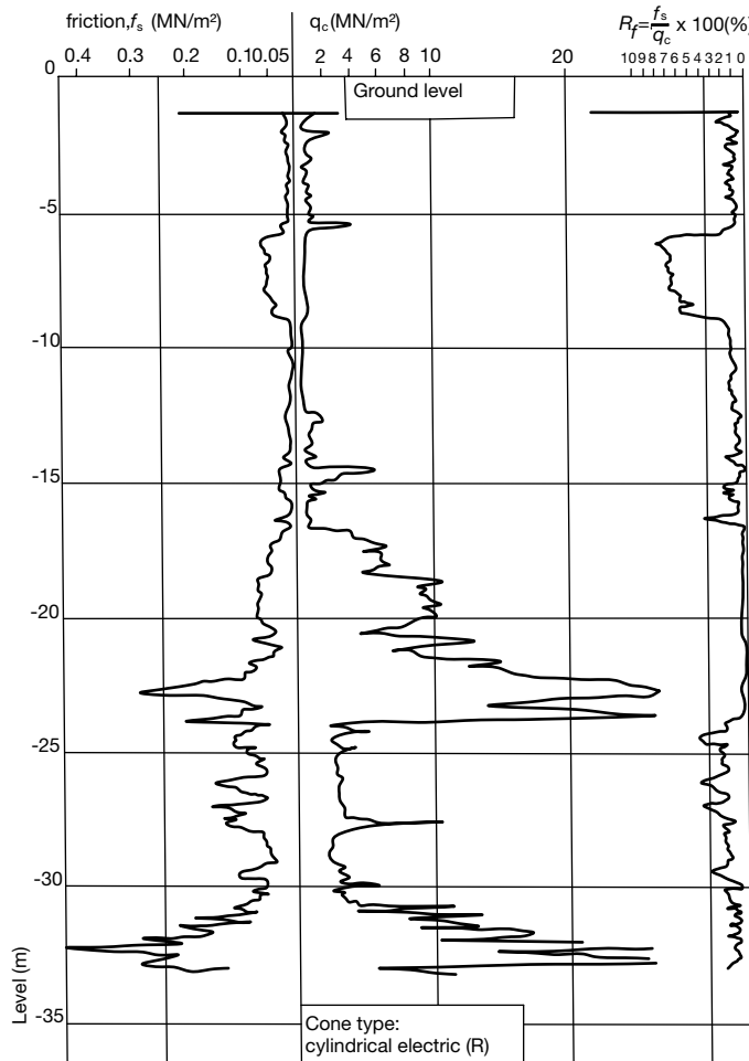
Figure 2.12 Typical plot from a CPT. (After Meigh 1987.)
