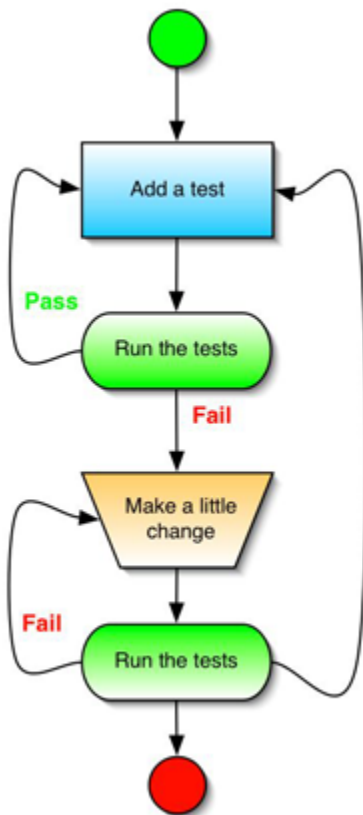
Figure 8.1: Model of test-first development
