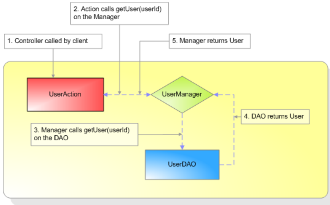
Figure 9.1: MyUsers application flow
