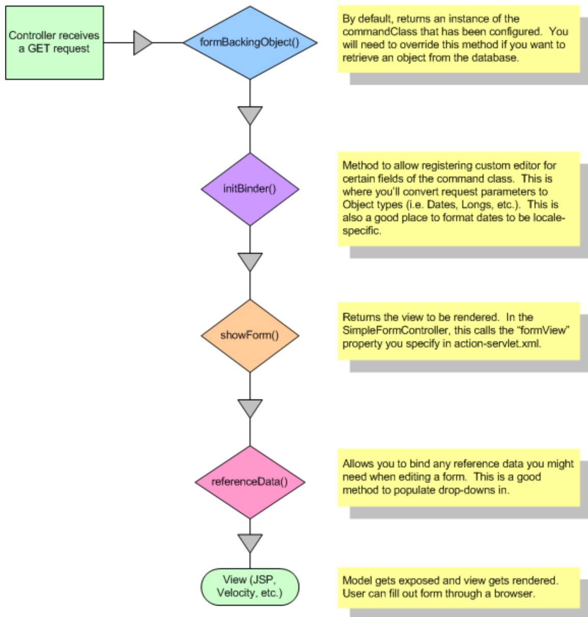
Figure 9.1: GET request lifecycle
