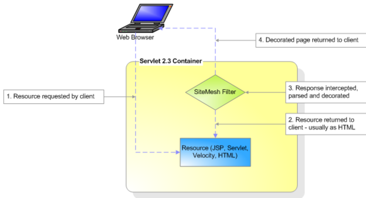
Figure 9.1: The SiteMesh process
