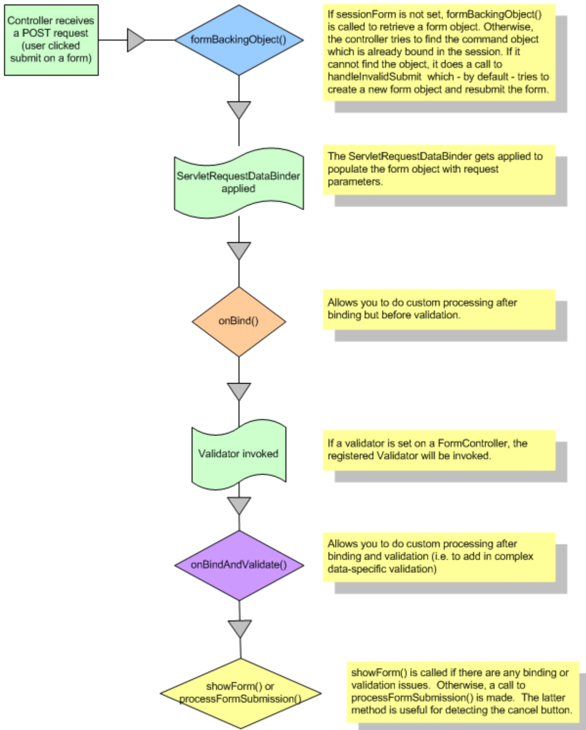
Figure 9.1: POST request lifecycle
