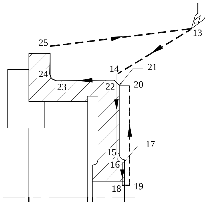
Fig. 12.70 Finishing
