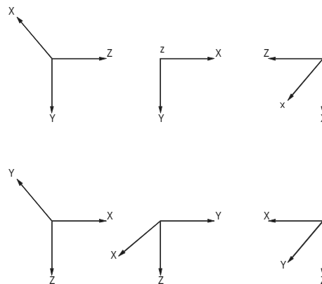
Fig. 12.31 Co-ordinate System
