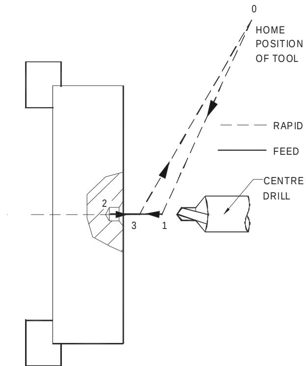
Fig. 12.53 The Central Drilling
