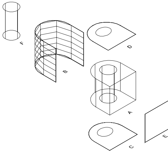
Fig. 6.6 B-Rep Model
