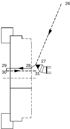
Fig. 12.57 Rough Boring
