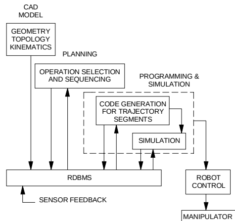
Fig. 13.9 Structure of an Off-line Programming System
