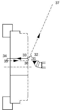
Fig. 12.58 Finish Boring
