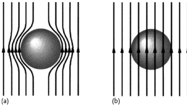
Figure 7.2 The Meissner effect. (a) A superconductor repels a weak magnetic field from its body below the transition temperature ( T < T_c ) while (b) at a temperature above the transition temperature ( T > T_c ) the magnetic field penetrates its body.
