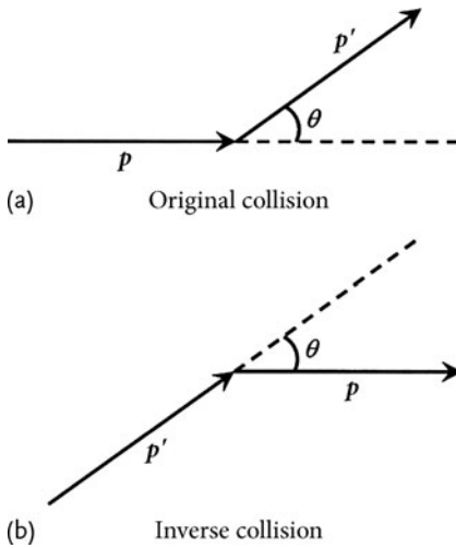
Figure 2.4 In (a), the electron suffers a change in momentum from \mathbf{p} to \mathbf{p}' after scattering. The inverse collision is shown in (b).
