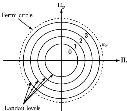
Figure 10.9 The circulation part of the Landau states is represented by the circular shell in \Pi_x \Pi_y -space.
