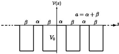
Figure 3.3 A Kronig–Penney potential has a square-well with depth V_0 and width \beta periodically arranged with period a = \alpha + \beta .
