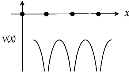
Figure 3.1 A periodic potential in one dimension. The blackened circles (●) indicate lattice ions.
