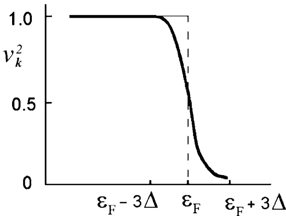
Figure 7.22 The behavior of v_k^2 near the Fermi surface.
