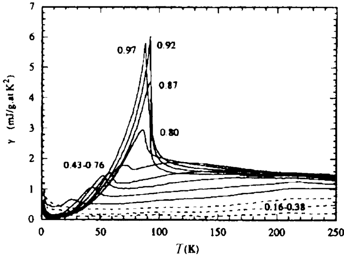
Figure 7.12 Electronic heat capacity C_{el}/T over temperature T , that is \gamma(x, T) \equiv C_{el}/T is plotted against T for \text{YBa}_2\text{Cu}_3\text{O}_{6+x} relative to \text{YBa}_2\text{Cu}_3\text{O}_6 . Values of x are 0.16, 0.29, 0.38, 0.43, 0.48, 0.57, 0.67, 0.76, 0.80, 0.87, 0.92, and 0.97, after Loram et al. [14].
