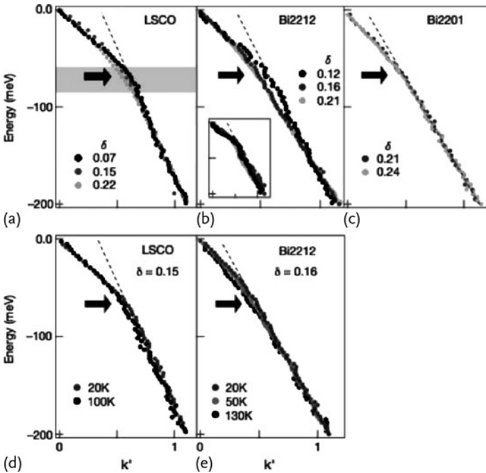
Figure 7.24 The quasiparticle dispersion relations derived from the momentum distribution curves along (0, 0) - (\pi, \pi) for (a) LSCO at 20 K, (b) Bi2212 at 20 K. Both materials are in superconducting states with the doping \delta indicated. (c) The dispersion relation for Bi2201
