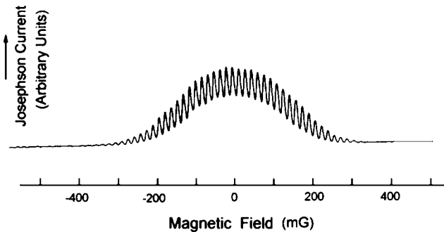
Figure 7.9 Current versus magnetic field, after Jaklevic et al. [8].
