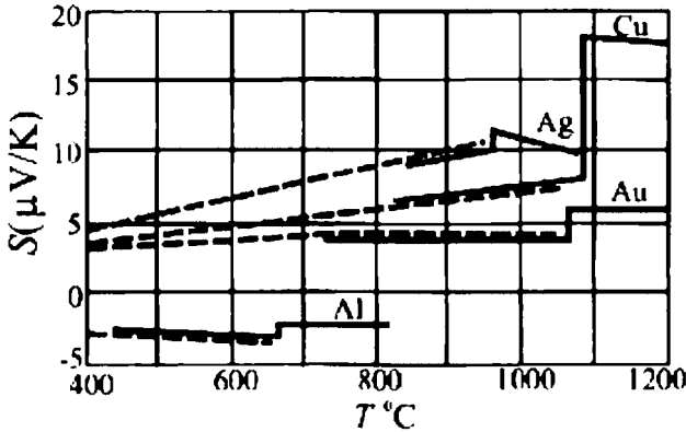
Figure 13.3 High-temperature Seebeck coefficients above 400 °C for Ag, Al, Au, and Cu. The solid and dashed lines represent two experimental data sets. Taken from [3]. The discontinuities arise from melting.
