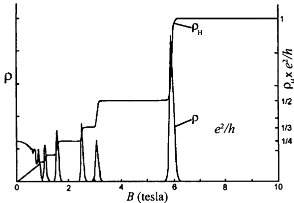
Figure 11.3 Observed QHE in the GaAs/AlGaAs heterojunction at 60 mK, after Tsui [3]. The Hall resistivity \rho_H and the resistance \rho are shown as a function of the magnetic field B in tesla.
