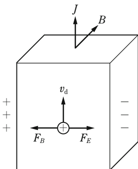
Figure 2.3 Schematic view of Hall’s experiment. The magnetic and electric forces ( \mathbf{F}_B , \mathbf{F}_E ) are balanced to zero in the Hall effect measurement.
