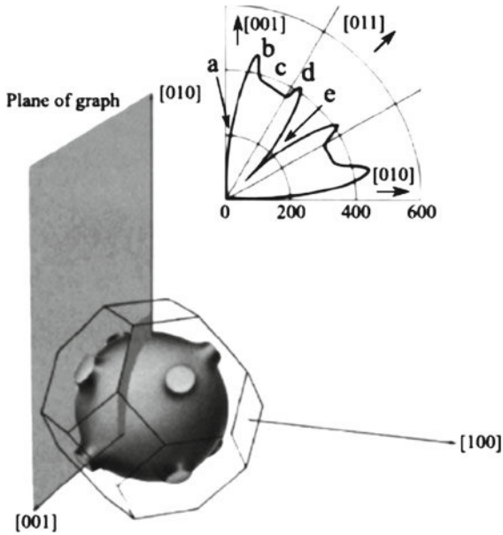
Figure 10.7 The striking anisotropy of the MR in Cu after Klauder and Kunzler [11]. The [001] and [010] directions of the Cu crystal are shown. The current flows in the [100] direc-
