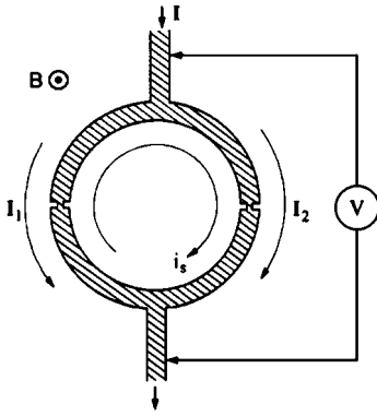
Figure 7.8 Superconducting quantum interference device (SQUID).
