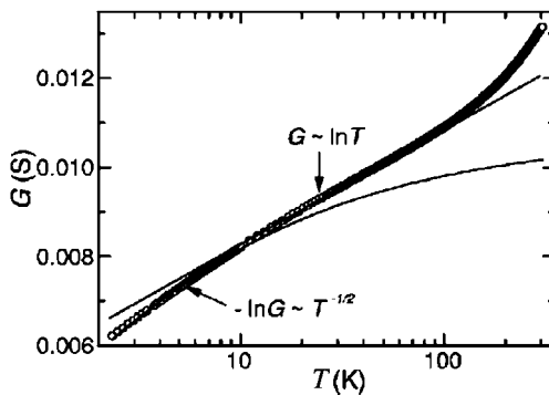
Figure 13.9 The conductance G of the multiwalled carbon nanotube samples as a function of temperature (after [1, Figure 3]).
