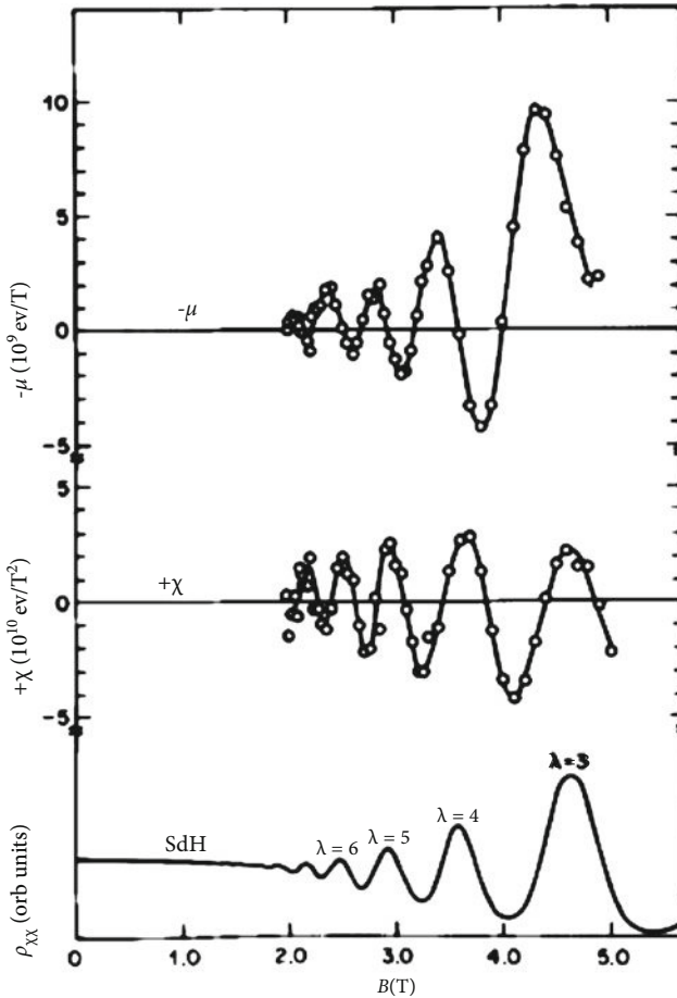
Figure 10.5 Experimental results on a stack of 4000 layers of 2D electron systems equivalent to an area of 240 \text{ cm}^2 after Störmer et al. [9]. \mu is the magnetic moment, and \chi is the suscep-
