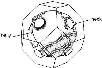
Figure 13.7 The Fermi surface of silver (fcc) has “necks,” with the axes in the \langle 111 \rangle direction, located near the Brillouin boundary, reproduced after [6–8].
