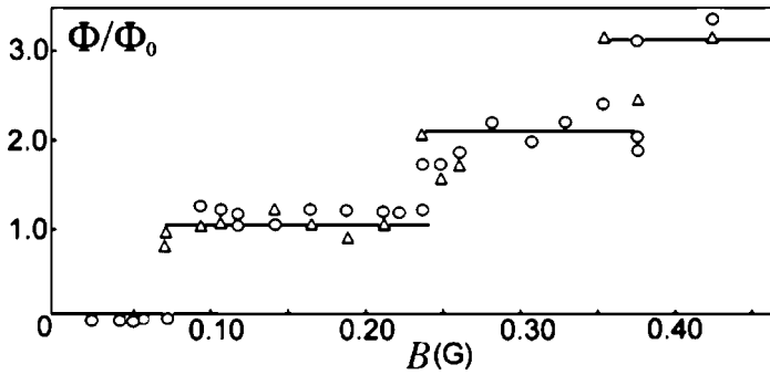
Figure 7.6 The magnetic flux quantization, after Deaver and Fairbank [4]. The two sets of data are shown as \Delta and \circ .
