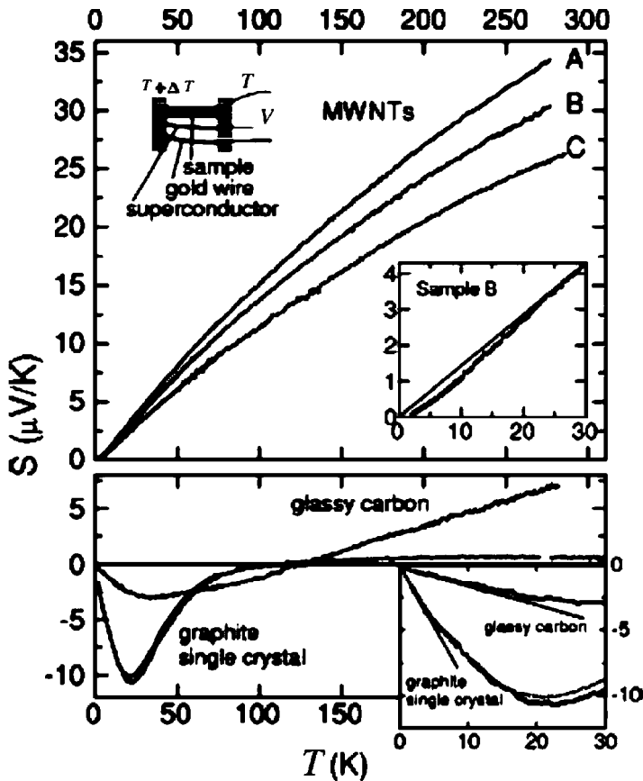
Figure 13.2 (a) The temperature dependence of thermoelectric power of MWNTs at several doping levels. The suppression of TEP from linearity at low temperatures is clearly shown in the lower-right inset (the line represents a
