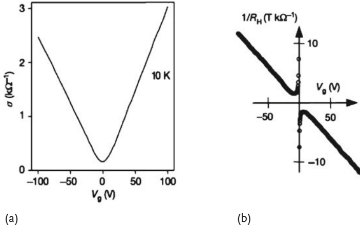
Figure 12.1 The gate field effects in graphene. Graphene’s conductivity in (a) \sigma (a) and Hall coefficient R_H (b) as a function of gate voltage V_g . R_H was measured in magnetic fields B of 2 T. R_H = 1/ne is inverted to emphasize the linear dependence n \propto V_g . The Hall coefficient changes its sign near V_g = 0 . After [1, Figure 1].
