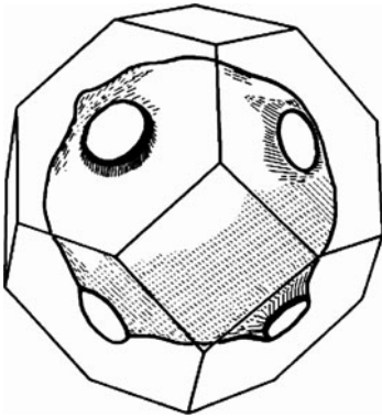
Figure 3.7 The Fermi surface of Cu (fcc) bulges out in the \langle 111 \rangle direction to make contact with the hexagonal zone faces.
