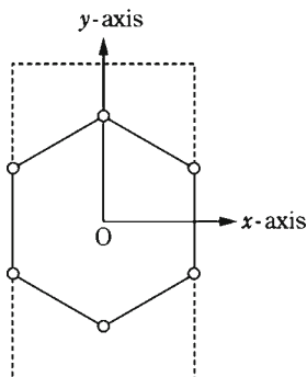
Figure 13.8 A honeycomb lattice and the Cartesian (rectangular) unit cell (dotted line) of graphene. The rectangular unit cell contains four \text{C}^+ ions represented by open circles (o).
