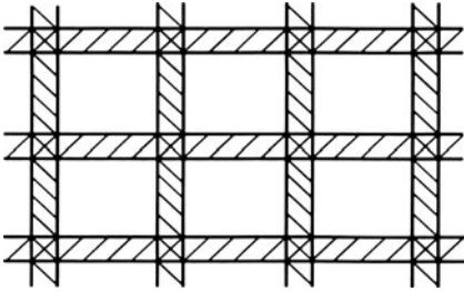
Figure 3.5 A 2D model potential. Each singly shaded stripe has a potential energy (depth) V_0 . Each cross-shaded square has a potential energy 2V_0 .
