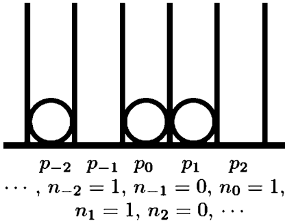
Figure A.2 A many-fermion state is represented by the set of fermion numbers \{n_j\} occupying the state p_j \equiv 2\pi\hbar j/L . Each n_j is restricted to 0 or 1.
