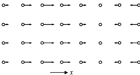
Figure 4.3 Longitudinal waves proceeding in the x -direction: \lambda = 12a_0 . Circle (o) indicates a lattice ion.
