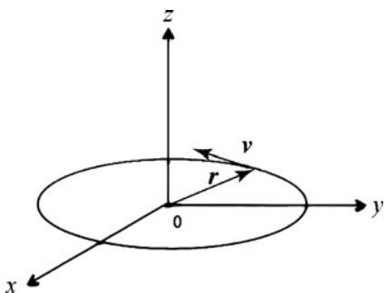
Figure 9.1 An electron with a circular motion generates a magnetic moment \boldsymbol{\mu} proportional to its angular momentum \mathbf{l} = m\mathbf{r} \times \mathbf{v} .
