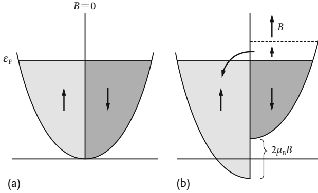
Figure 9.3 The density of states \mathcal{D}_+ and \mathcal{D}_- , for the free electrons with up ( \uparrow ) and down ( \downarrow ) spins, are drawn against the energy \epsilon , which is measured upwards. (a) When B = 0 the two halves of the Fermi–Dirac distribution are equal, and thus M = 0 ; (b) when a field B is applied, the antiparallel half flip into the parallel half, resulting in a net parallel magnetization.
