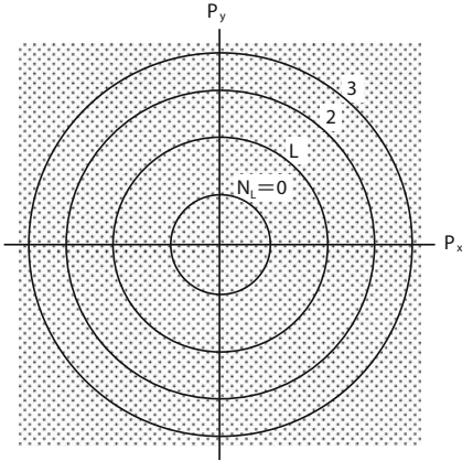
Figure 10.4 Quantization scheme for free electrons: without magnetic field (dots) and in a magnetic field (circles) perpendicular to the paper.
