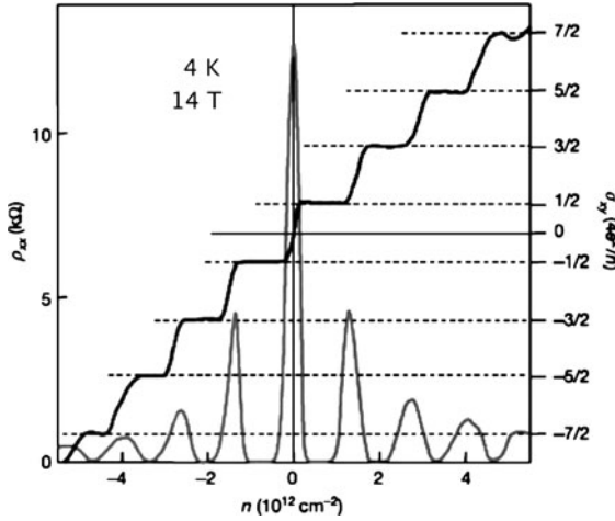
Figure 12.3 QHE in graphene. After Novoselov et al. [1].
