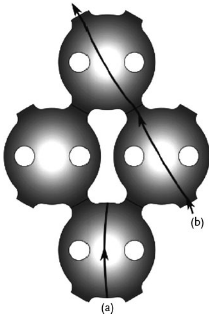
Figure 10.6 The figure shows a closed orbit “a” in k -space that can be traced by the electron, and an open orbit “b” that extends over the two Brillouin zones and that cannot be traveled by an electron.
