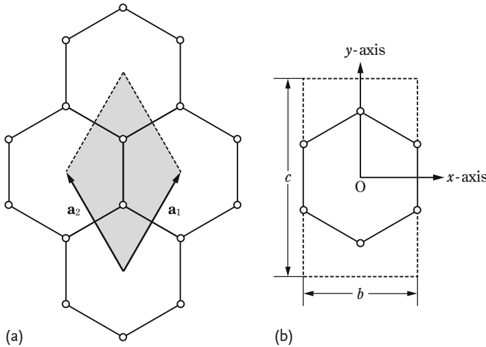
Figure 5.1 (a) The WS unit cell, a rhombus (shaded area) for graphene. (b) The orthogonal unit cell, a rectangle (dotted lines) with side lengths (b, c) . Open circles (o) indicate the C^+ ions and the lines between open circles indicate the chemical bonds.
