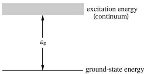
Figure 7.10 Excitation energy spectrum with a gap.
