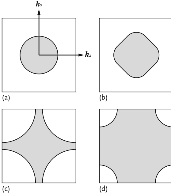
Figure 4.2 2D intersections at k_z = 0 of the constant frequency planes for a simple cubic lattice in the \omega -increasing order: (a–d). The shaded areas correspond to the lowest-frequency (energy) sides. There is a singular point between (b,c) where the curvature sign changes. After [6].
