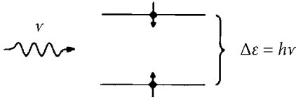
Figure 9.2 Electron spin resonance (ESR). An electron with the up-spin may absorb a photon of the energy h\nu and jump to the upper energy level by flipping its spin if \Delta\varepsilon = h\nu .
