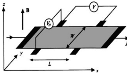
Figure 11.2 Hall effect measurements. The Hall voltage V_H is generated perpendicular to the current J and the magnetic field B .
