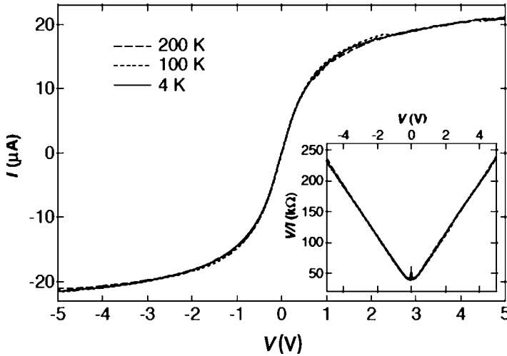
Figure 8.8 Large-bias I - V characteristics at different temperatures using low-resistance contacts for a sample with an electrode spacing of 1 \mu\text{m} . The inset plots R = V/I vs. V . After Yao, et al. [31].
