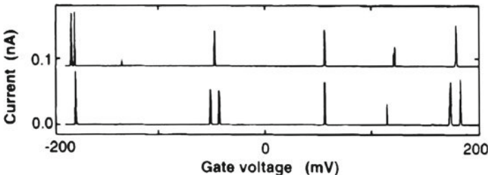
Figure 8.2 Current vs. gate voltage at V_{\text{bias}} = 30 \mu\text{V} . (After Tans et al. in [5, Figure 2].)
