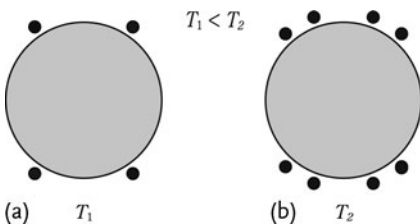
Figure 13.4 (a,b) More “electrons” (dots) are excited above the Fermi surface (solid line) at the high-temperature end: T_2 (> T_1) . The shaded area denotes the electron-filled states. “Electrons” diffuse from (b) to (a).
