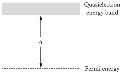
Figure 7.20 Quasielectrons have an energy gap \Delta relative to the Fermi energy.
