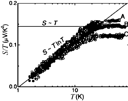
Figure 13.1 Low-temperature Seebeck coefficient S of MWNTs plotted as S/T on a logarithmic temperature scale (reproduced from [1, Figure 2]).
