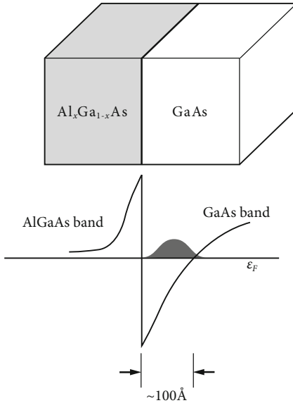
Figure 11.1 The GaAs/AlGaAs heterojunction. The electrons are localized within less than 100 Å of the interface. The shaded area represents the electron distribution.
