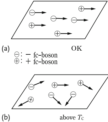
Figure 11.7 \pm fc-bosons at 0K (or below T_c ) (a) and noncondensed fc-bosons above T_c (b).
