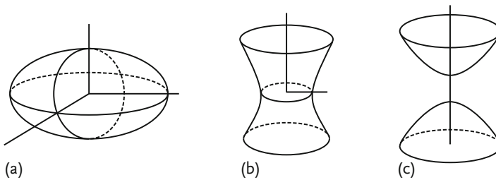
Figure 3.12 (a) Ellipsoid, (b) hyperboloid of one sheet (neck), (c) hyperboloid of two sheets (inverted double caps).
