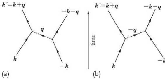
Figure 7.16 (a,b) Two Feynman diagrams representing a phonon exchange between two electrons.
