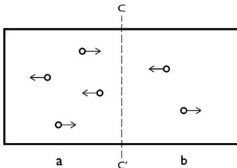
Figure 2.1 If the particles flow out in all directions with no preference, there will be more particles crossing the imaginary boundary CC' in the a to b direction than in the opposite direction.
