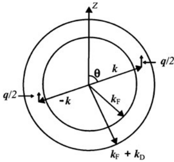
Figure 8.5 The range of the interaction variables (k, \theta) is limited to a circular shell of thickness k_D .
