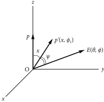
Figure 2.5 A new frame of reference in which the positive z-axis points in the direction of the fixed vector p . In this frame, the direction of the electric field E is specified by (\theta, \phi) and that of the momentum p' by (\chi, \phi_1) .
