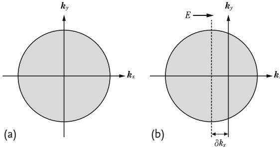
Figure 13.6 As the electric field E points in the positive x -direction, the steady-state electron distribution in (b) is generated by a translation of the equilibrium distribution in (a) by the amount \delta \mathbf{k} = -eE\tau/\hbar .
