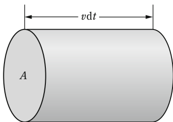
Figure 2.2 A particle moving with a speed v sweeps the volume (vdt)A during the time dt , where A represents the cross section.
