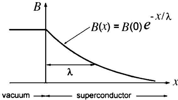
Figure 7.4 Penetration of the magnetic field into a superconductor slab. The penetration depth \lambda is of the order of 500 Å near 0 K.
