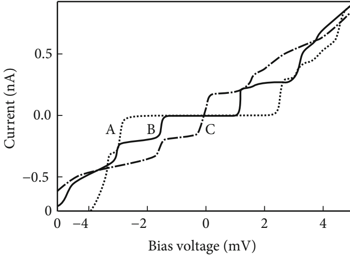
Figure 8.1 Current–voltage curves for nanotubes at gate voltages of 88.2 mV (trace A), 104.1 mV (trace B) and 120.0 mV (trace C) at T = 5 mK. (After Tans et al. in [5, Figure 2].)
