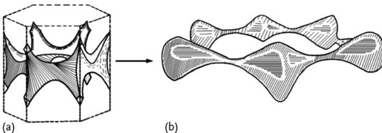
Figure 3.8 The Fermi surfaces in the second zone for Be. (a) NFEM "monster," (b) measured "coronet." The coronet encloses unoccupied states.
