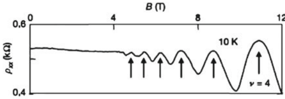
Figure 12.2 The SdH oscillations in graphene at gate voltage V_g = -60 V, temperature T = 10 K. The longitudinal resistivity \rho_{xx} (k \Omega ) is plotted as a function of magnetic field B (T). After [1, Figure 2].
