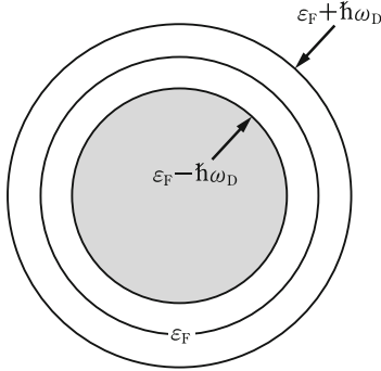
Figure 7.19 The k -space shell in 2D where pairons of both charge types are generated and intercorrelated.
