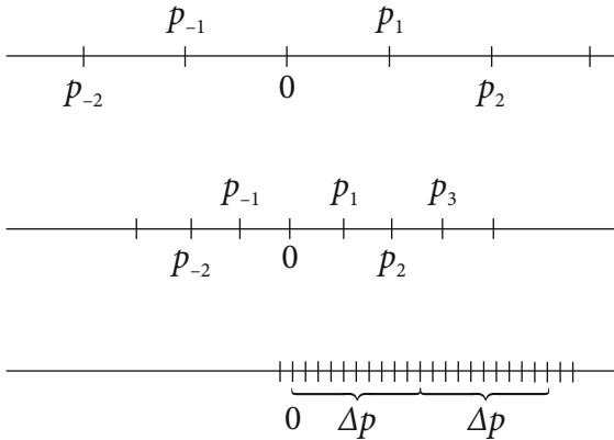
Figure 3.11 The linear momentum states are represented by short bars forming a linear lattice with unit spacing equal to 2\pi\hbar/L . As the normalization length L is made greater, the spacing becomes smaller.
