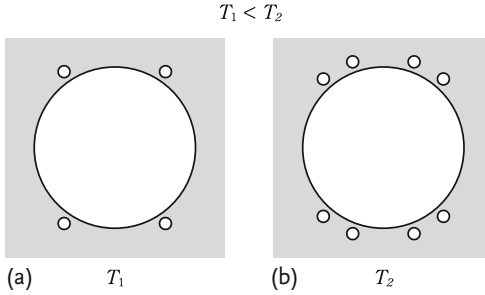
Figure 13.5 (a,b) More “holes” (open circles) are excited below the Fermi surface at the high-temperature end: T_2 (> T_1) . “Holes” diffuse from (b) to (a).
