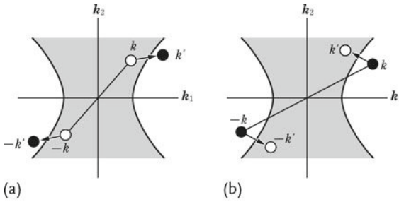
Figure 7.17 k -space diagrams representing (a) pair creation of ground pairons and (b) pair annihilation.
