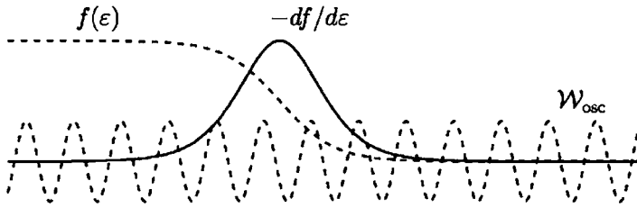
Figure 10.3 Numerous oscillations in W_{osc} within the width of -df/d\varepsilon cancel out the contribution to the free energy F .
