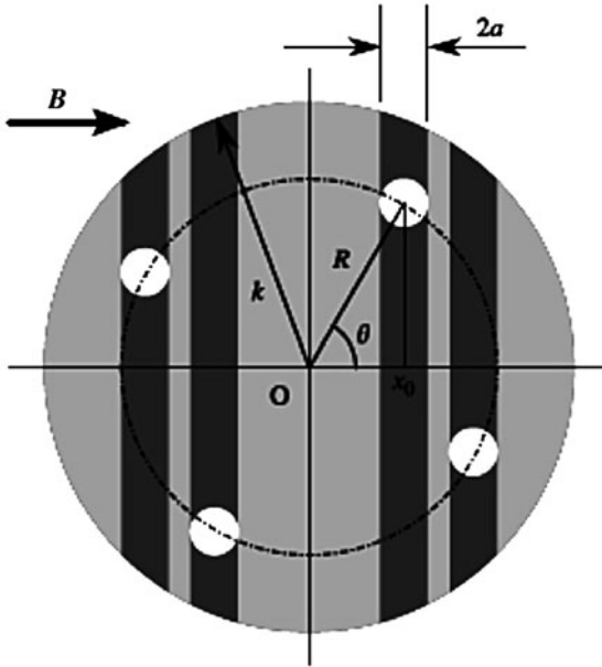
Figure 10.8 The electron circulates perpendicular to the magnetic field B in the k -space. If the electron hits the bad ball of radius a , it will not complete circulation, and it does not
