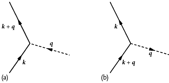
Figure 4.4 Feynman diagrams representing (a) absorption and (b) emission of a phonon (indicated by the dashed line) by an electron. They correspond to the interaction terms in (4.94).
