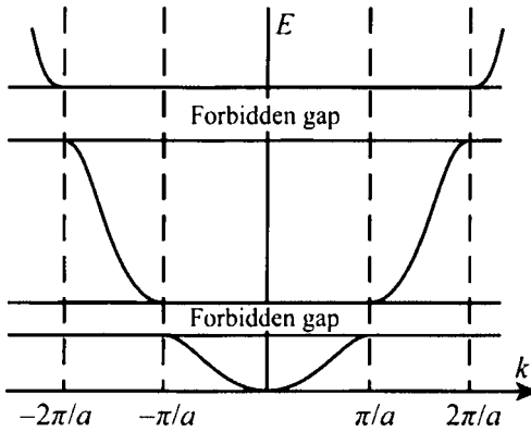
Figure 3.4 E - k diagram showing energy bands and forbidden gaps.
