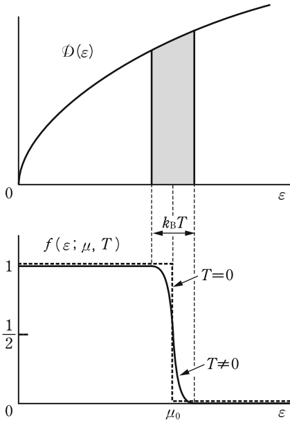
Figure 3.10 The density of states in energy, D(\epsilon) , and the Fermi distribution function f(\epsilon) are drawn as a function of the kinetic energy \epsilon . The change in f is appreciable only
