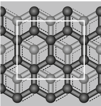
Figure 14.1 The Cartesian unit cell (white solid lines) viewed from the top for graphite. The unit cell of graphite has two layers of graphene. The carbons (circles) in the A (B) planes are shown in black (gray).
