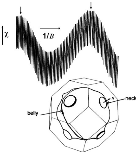
Figure 10.2 The dHvA oscillations in silver with the magnetic field along a \langle 111 \rangle direction, after Schönberg and Gold [4, 5]. The two distinct periods are due to the neck and belly orbits indicated in the inset.
