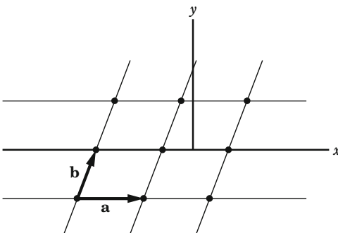
Figure 5.2 An oblique net with base vectors (\mathbf{a}, \mathbf{b}) .
