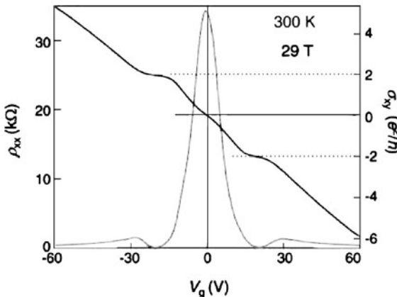
Figure 12.4 Room-temperature QHE in graphene after Novoselov et al. [7]. Hall conductivity \sigma_{xy} (e^2/h) (dark) and resistance \rho_{xx} (light) as a function of gate voltage ( V_g ) at
