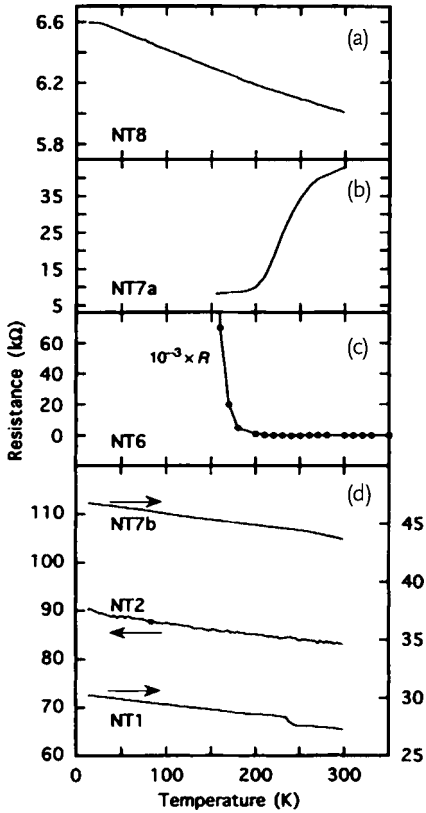
Figure 5.3 Temperature dependence of the resistance of different NTs after Ebbesen et al. [2]. (a) Nanotube NT8, (b) NT7a, (c) NT6, (d) NT1, NT2, NT7b.
