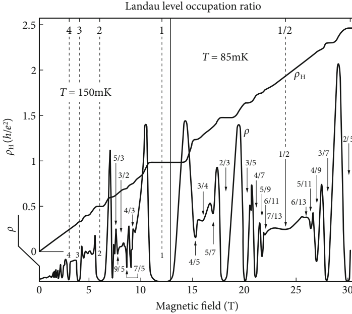
Figure 11.4 The Hall resistivity \rho_H (\equiv \rho_{xy}) in h/e^2 and the resistivity \rho (\equiv \rho_{xx}) in GaAs/AlGaAs at 85, 150 mK are plotted as a function of the magnetic field B in tesla, reproduced after Willett et al. [10]. The high-field \rho trace is reduced in amplitude by a factor of 2.5. The upper numbers indicate the Landau-level occupation ratio \nu .
