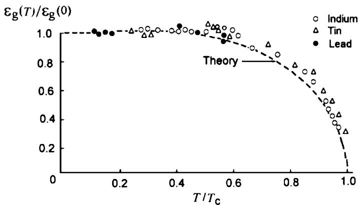
Figure 7.11 The energy gap \varepsilon_g(T) versus temperature, as determined by tunneling experiments, after Giaever and Megerle [13].
