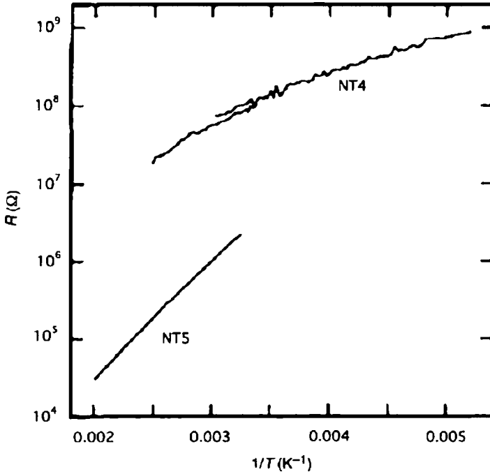
Figure 5.4 Semilogarithmic plot of the resistance R of NT4 and NT5 versus the inverse of the temperature after Ebbesen et al. [2].
