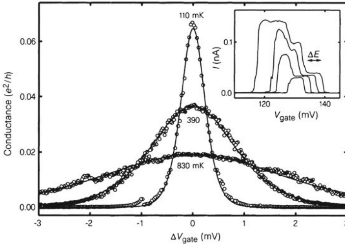
Figure 8.3 Conductance G = I/V_{\text{bias}} versus \Delta V_{\text{gate}} at low bias voltage V_{\text{bias}} = 10 \mu\text{V} and different temperatures. Solid lines are fits of G \propto \cosh^{-2}(e\Delta V_{\text{gate}}/(\alpha 2k_{\text{B}}T)) , where
