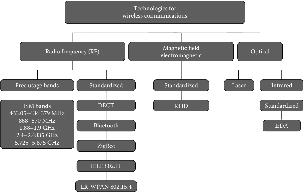
FIGURE 85.8 Currently available frequencies for wireless applications.
