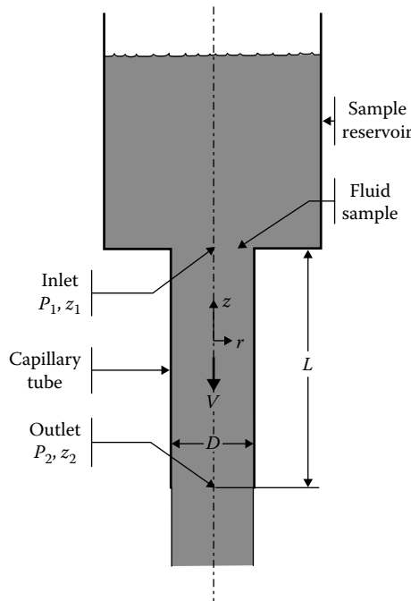
FIGURE 46.6 Capillary viscometer geometry.
