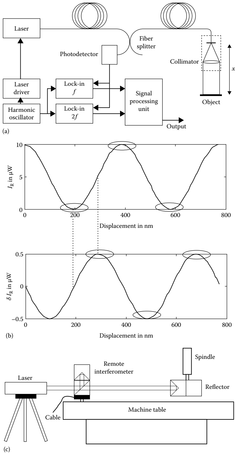
FIGURE 27.7 Displacement sensor based on a Fabry-Pérot interferometer: (a) a Fabry-Pérot-type sensor, (b) change in intensity as a function of distance, and (c) an experimental set up.
