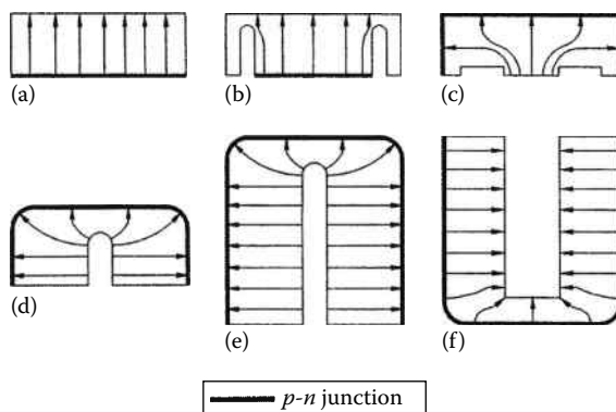
FIGURE 81.10 Schematic cross section and electrostatic field distribution in HPGe detectors. The dark line represents the p - n junction: (a) true planar, (b) grooved planar, (c) low-capacity planar, (d) truncated coaxial, (e) closed-end coaxial, and (f) well geometry.
