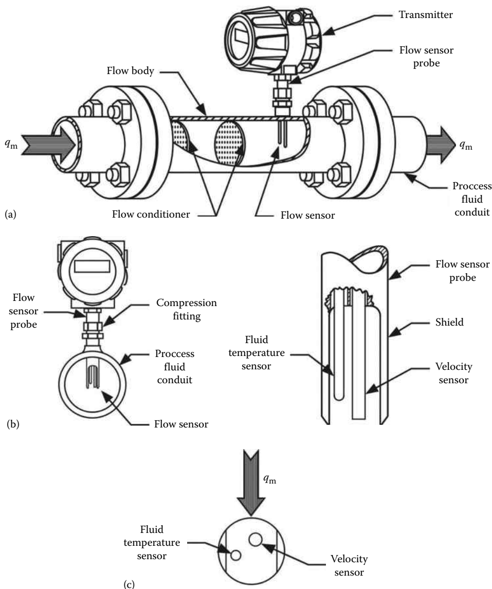
FIGURE 63.1 In-line and insertion meter configurations of thermal dispersion mass flow meters. (a) In-line configuration, (b) insertion configuration, installed, and (c) detail of flow sensor, insertion meter shown. (Adapted from Olin, J.G., Advances in thermal dispersion mass flow meters—Part 1: Principle of operation , Sierra Instruments Technical Report No. SI-JGO-2010-1, 2010. With permission from Sierra Instruments, Inc.)
