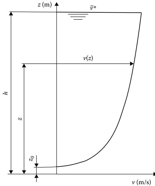
FIGURE 57.11 Logarithmic law describing open-channel velocity profile.
