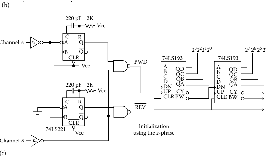
FIGURE 30.7 Circuit producing a direction and a count signal. (From Conner, D., EDN , 35(9), 57, 1990.) (a) Caution must be exercised when using this circuit for counting purposes since multiple counts are possible when the encoder oscillates around the A = 0 and B = 0 and the A = 0 and B = 1 states. (From Kuzdrall, J.A., Electron. Des. , 17, 81, 1992.) (b) Counts up and down at the same states transition but depending on the direction of movement.
