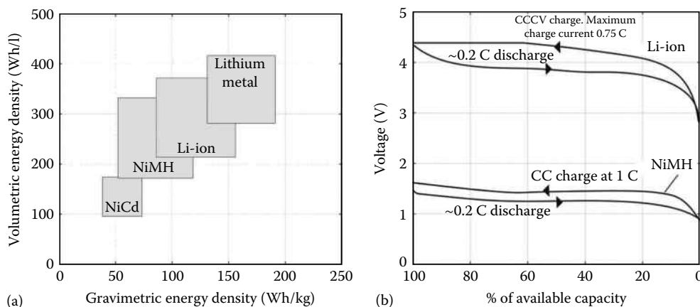
FIGURE 88.4 (a) Volumetric energy density plotted against gravimetric energy density for common secondary battery types. (Adapted from Linden, D. and Reddy, T.B., Handbook of Batteries , 3rd edn., McGraw-Hill, New York, 2001.) (b) Charge (at 1 C and 0.75 C) and discharge (at 0.2 C) curves for Li-ion and NiMH batteries.
