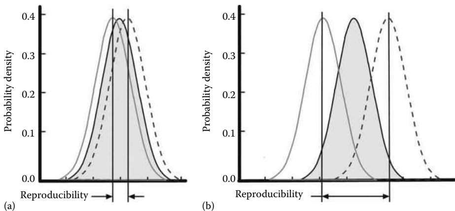
FIGURE 28.16 Reproducibility demonstration based on the results of measurements: (a) High reproducibility, and (b) low reproducibility.
