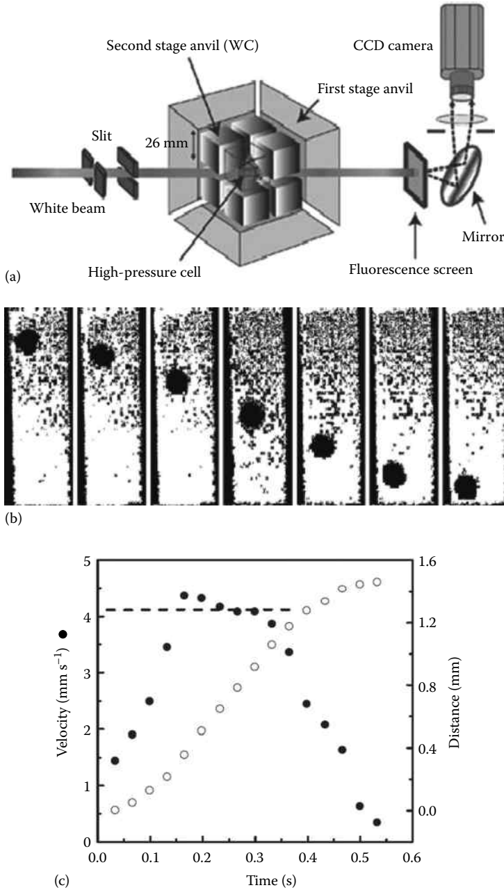
FIGURE 46.14 (a) Synchrotron x-ray radiography setup for a high-pressure Stokesian viscometry measurement [51]. (b) Synchrotron radiographic images of a Pt core—ruby mantle composite sphere falling in liquid Fe–29 wt% S at 2.6 GPa and 1373 K. Images are separated in time by 62 ms [52]. (c) Distance and velocity of falling composite sphere versus time in Fe–29 wt% S liquid, at 2.6 GPa and 1373 K. Dashed line is terminal velocity [52].
