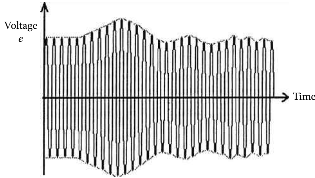
FIGURE 25.14 An amplitude-modulated signal. It is possible to configure some sensors to give amplitude-modulated signals, as in the case of capacitive vibration displacement sensors. When rectified, the average value of this wave gives the mean separation of the plates. The vibration amplitude around this mean position can be extracted by a demodulator and low-pass filter circuit. The output of the low-pass filter is a direct indication of the vibrations.
