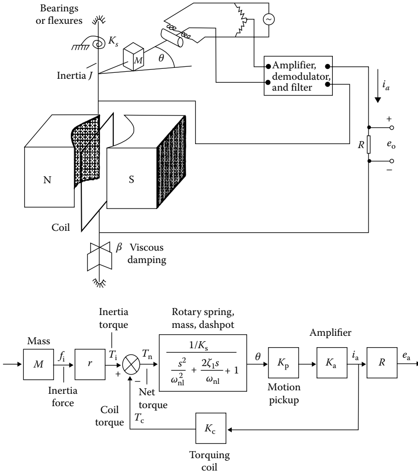
FIGURE 36.7 A simplified version of a rotational-type servo accelerometer. Acceleration of the instrument case causes an inertial force on the sensitive mass, tending to make it pivot in its bearings or flexure mounts. The rotation from neutral is sensed by inductive sensing and amplified, demodulated, and filtered to produce an electric current that is directly proportional to the motion from the null. The block diagram representation is useful in analysis.
