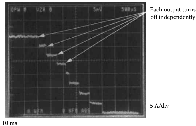
FIGURE 71.14 Independent thermal shutdown of an eight-output power IC. (Courtesy of Motorola, Inc., Schaumburg, IL.)
