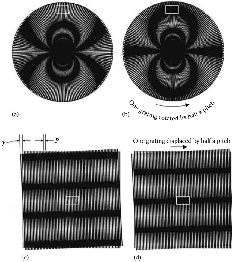
FIGURE 30.12 Moiré fringes produced when two gratings of equal pitch are overlaid. In (a), two radial gratings with 180 cycles have their centers displaced horizontally by approximately half of the grating pitch (as measured on the perimeter). This could be due to encoder-assembly errors. The fringes are always circular and pass by the two centers. In (b), the same displacement was followed by a rotation of half a pitch as a result of the normal movement of the encoder disk. This causes a phase change of 180^\circ of the fringe pattern at any fixed observation point, as represented by the rectangular observation region. The width of the fringes depends on the offset displacement between the two grating centers. If they coincide, the whole pattern changes from a dark to a relatively bright fringe. In (c), two linear gratings are rotated by one-tenth (in radian) of their grating pitch. This could be due to encoder assembly or mounting errors. As a result, Moiré fringes occur at 90^\circ to the grating and with a period 10 times larger. The normal displacement of one grating by half of the grating pitch causes a phase change of 180^\circ of the Moiré fringe pattern at any fixed observation point, as represented by the rectangular observation region. (From Ditchburn, R.W., Light , Vol. 1, Academic Press, New York, 1976.)
