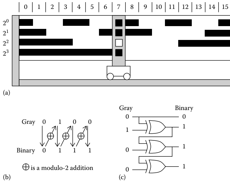
FIGURE 30.4 (a) Gray code allows a transition on only one track between each successive position so that no ambiguity arises. A scheme based on modulo-2 additions converts the Gray code to natural binary code in (b). Exclusive ORs implement the conversion in (c).
