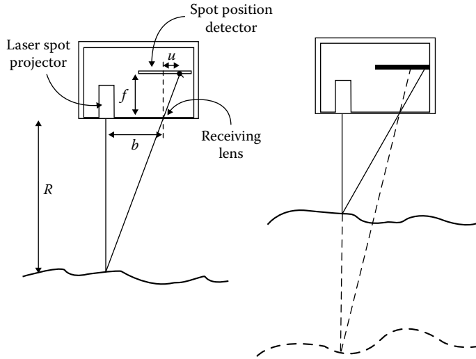
FIGURE 14.5 A simple pinhole camera model illustrates the basic active triangulation principle. As the distance R to the target surface changes, the spot position u on the detector changes, maintaining similarity between the large triangle outside the camera and the small triangle inside. There is an inverse relationship between R and u .
