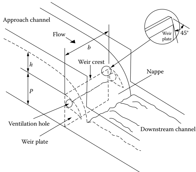
FIGURE 52.5 Full-width thin-plate weir. Flow rate \dot{Q} varies with water level h above the weir crest ( \dot{Q} \propto h^{3/2} ) and with a flow-dependent discharge coefficient C_d .
