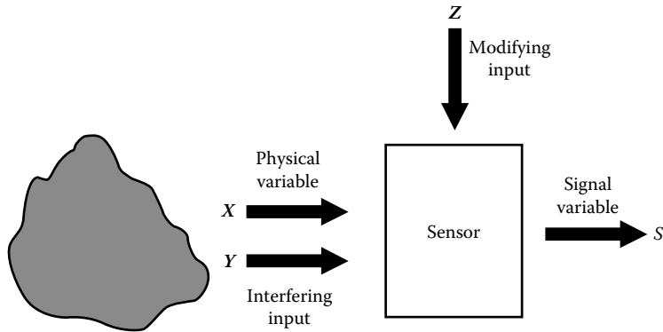
FIGURE 2.4 Interfering inputs.
