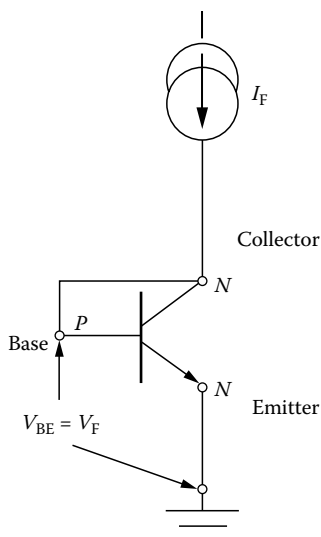
FIGURE 71.1 Bipolar transistor configured as a temperature sensor. The base of the transistor is shorted to the collector. A constant current flowing in the remaining pn (base to emitter) junction produces a forward voltage drop V_F proportional to temperature.
