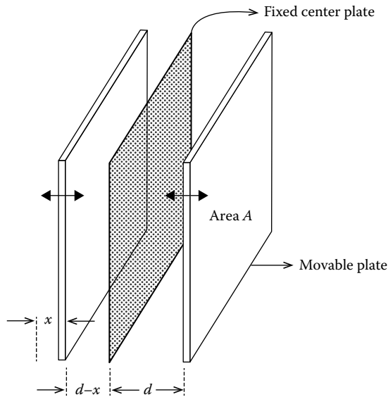
FIGURE 25.4 A differential capacitive sensor. They are essentially three-terminal capacitors with one fixed center plate and two outer plates. The response to physical variables is linear. In some versions, the central plate moves in response to physical variable with respect to two outer plates, and in others, the central plate is fixed and the outer plates are allowed to move.
