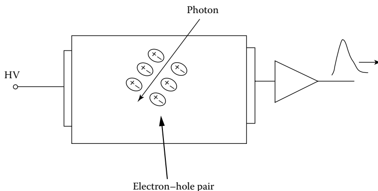
FIGURE 81.18 Schematic illustration of charge generation in a planar detector.
