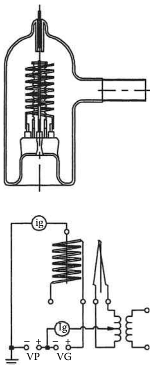
FIGURE 40.16 Bayard–Alpert hot cathode ionization gage.
