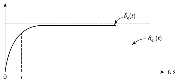
FIGURE 93.3 Time response of an actuator.
