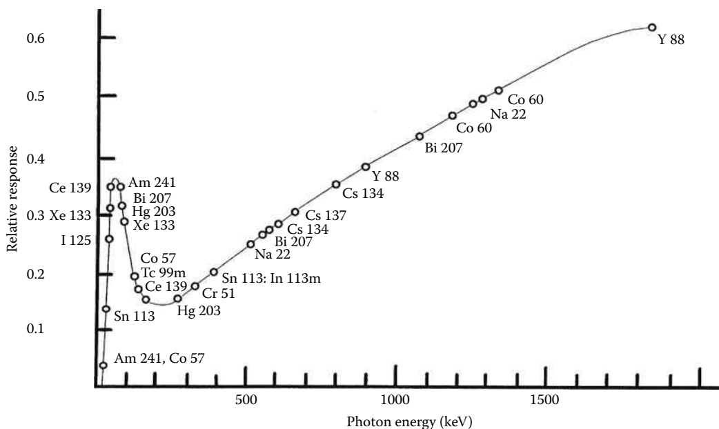
FIGURE 80.17 Photon response as a function of energy for a pressurized reentrant ionization chamber. (From Dell, M.A., Capintec, instruments, private communication, 1997.)
