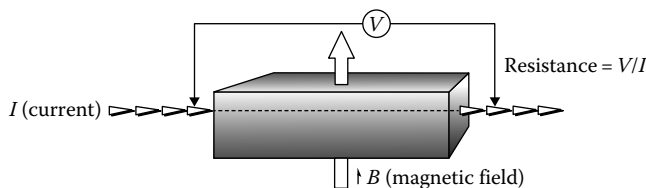
FIGURE 31.7 Magnetoresistance.
