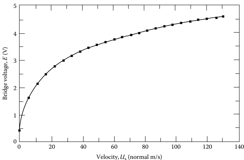
FIGURE 59.7 Typical flow-calibration curve for an industrial thermal anemometer. The electronics drive is that shown in Figure 59.6. The constant-temperature differential ( T_v - T_T ) is 50.0 °C. The cold resistances R_{v0} and R_{T0} of the velocity and temperature sensors at 20 °C are approximately 20 and 200 W, respectively. (With permission of Sierra Instruments, Inc., Monterey, CA.)
