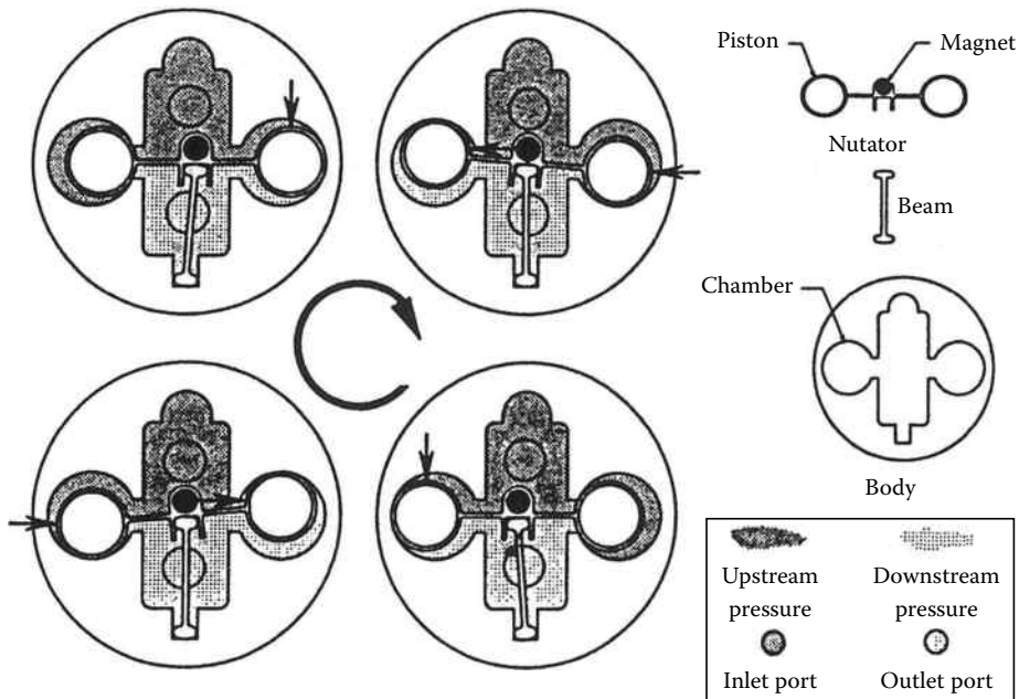
FIGURE 53.6 Nutating-disk-type PD meter. (Courtesy of DEA Engineering Company, Mission Viejo, CA.)
