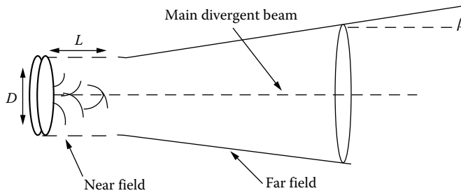
FIGURE 29.3 Illustration of the ultrasound beam in the near field and the far field of the transducer.
