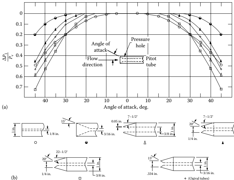
FIGURE 62.8 (a) Variation of total pressure indication with angle of attack and (b) geometry for Pitot tubes. (From ASME/ANSI PTC 19.2-2010, Instruments and Apparatus, Part 2, Pressure Measurements , ASME, Washington, DC, 2010. With permission.)
