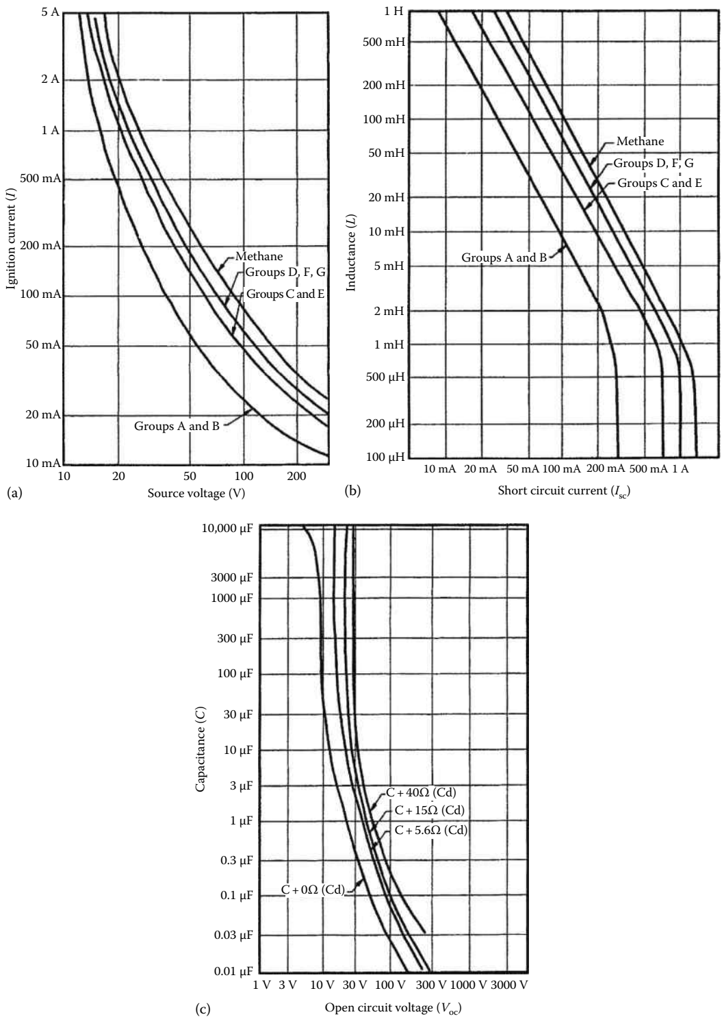
FIGURE 94.2 (a) Resistance circuit ignition curves for all circuit metals, (b) inductance circuit ignition curves at 24 V for all circuit metals, and (c) capacitance circuit ignition curves for Groups A and B for all circuit metals.
