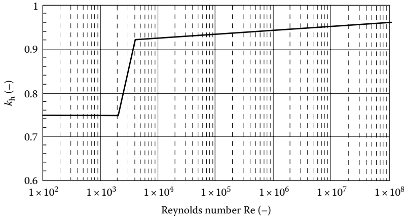
FIGURE 57.8 Dependence of the k_h factor for single-path measurement on the Reynolds number. Between a Reynolds number of 2000 and 4000, the transitional flow regime occurs.
