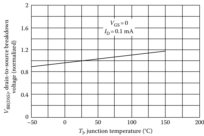
FIGURE 71.11 Power MOSFET’s breakdown voltage variation versus temperature.
