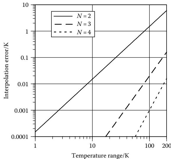
FIGURE 69.4 The typical standard deviation of interpolation errors versus the number of terms used in the calibration equation. The lines are indicative only: the errors tend to be greater for temperatures below 0^{\circ}\text{C} , and for thermistors with a high \beta value.
