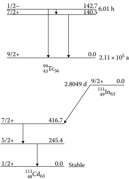
FIGURE 80.5 Simplified nuclear decay schemes for the radionuclides ^{99\text{m}}\text{Tc} and ^{111}\text{In} . The vertical arrows indicate transitions between nuclear excited states. Gamma-ray emission competes with internal conversion processes for each transition. (From Leo, W.R., Techniques for Nuclear and Particle Physics Experiments , Springer-Verlag, Berlin, Germany, 1992.)
