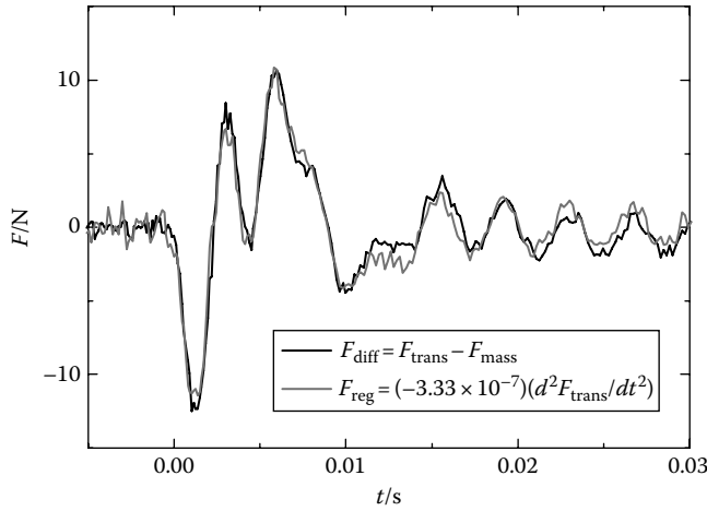
FIGURE 12.5 Changes in F_{\text{diff}} and F_{\text{reg}} against time.
