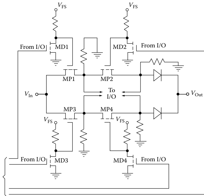
FIGURE 11.6 Solid-state fail-safe relay.
