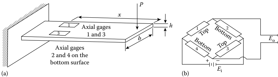
FIGURE 41.6 Beam-type load cells: (a) a selection of beam-type load cells (elastic element with strain gages) and (b) gage positions in the Wheatstone bridge. (From Dally, J.W. et al., Instrumentation for Engineering Measurements , John Wiley & Sons, New York, 1984.)
