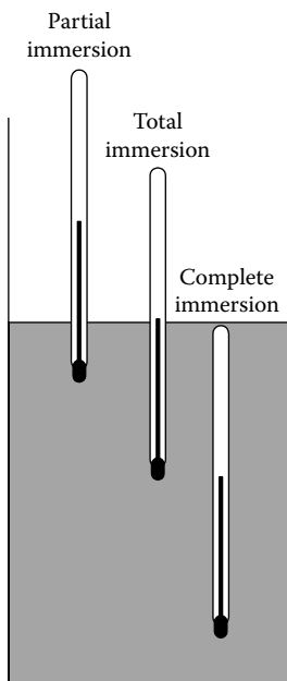
FIGURE 74.3 Immersion conditions used for LIG thermometers.
