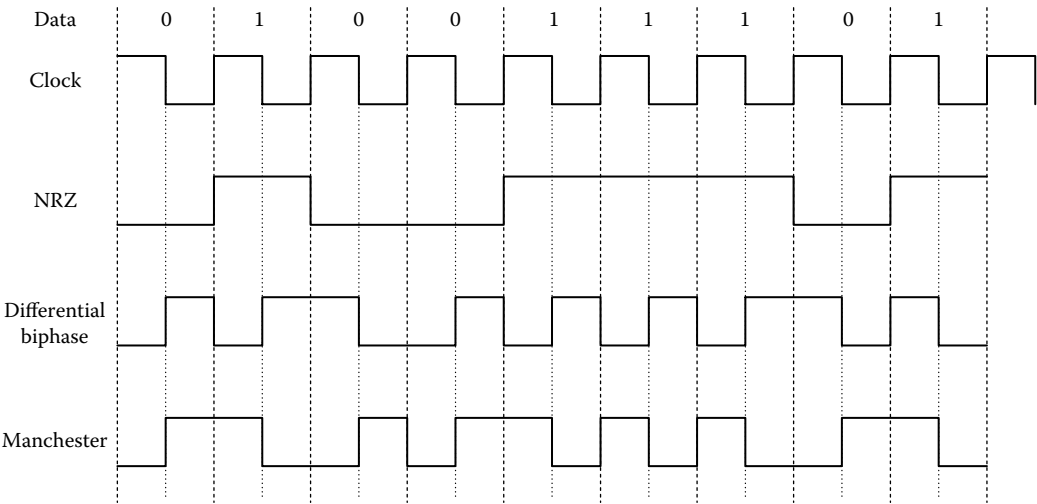
FIGURE 90.9 IRIG standards. NRZ (nonreturn to zero): “1” represented by a high logic level and “0” represented by a low logic level. Differential biphase: “1” represented by a change in level at the start of the clock period and “0” represented by no change of level at the start of the clock period. There is always a change of level at the middle of the clock period. Manchester: “1” represented by a high-to-low transition at the middle of the clock period and “0” represented by a low-to-high transition at the middle of the clock period.
