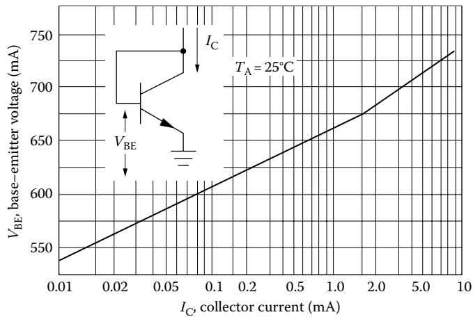
FIGURE 71.4 Base-emitter voltage versus collector-emitter current.
