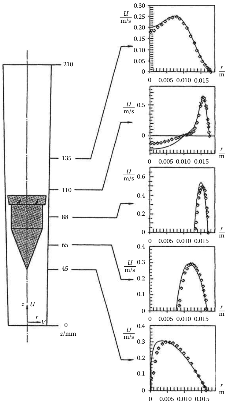
FIGURE 52.14 Comparison of measured and computed velocity profiles for laminar flow through a rotameter (Reynolds number 220). U = axial component (m/s), z = axial position (mm), and r = radial position (m).
