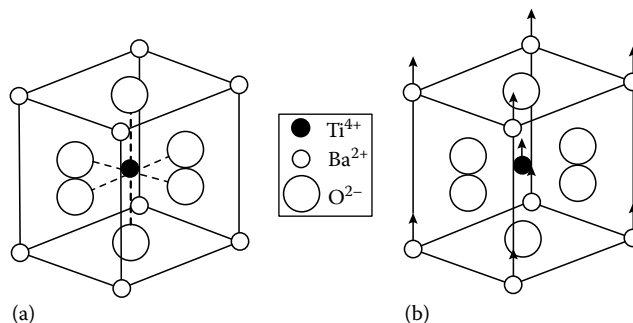
FIGURE 26.3 Crystal structure of BaTiO_3 : (a) Above the Curie point, the cell is cubic; (b) below the Curie point, the cell is tetragonal with Ba^{2+} and Ti^{4+} ions displaced relative to O^{2-} ions.
