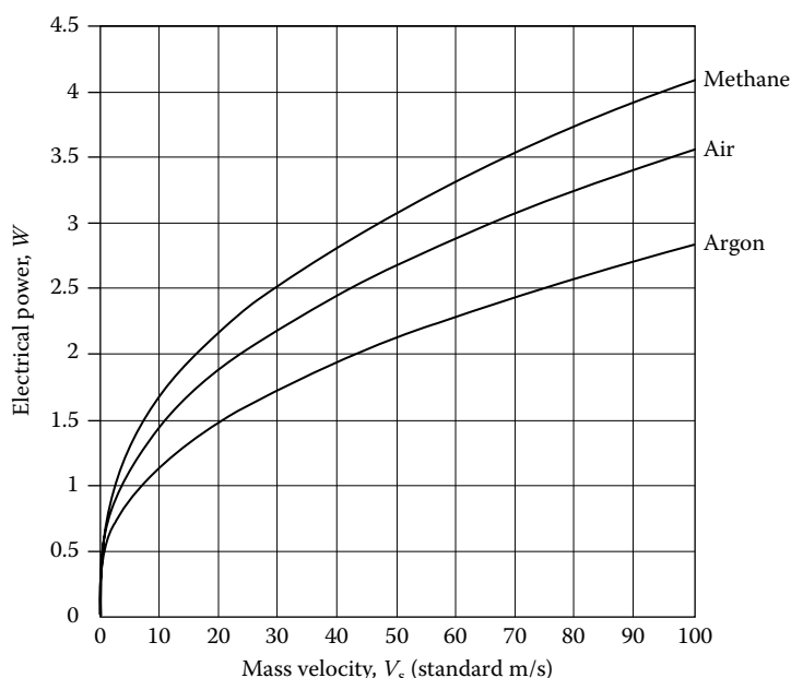
FIGURE 63.5 Typical outputs of the dry-sensor microprocessor-based system for three different gases. T = 300 K; P = 1 bara; \Delta T = 50 K. The “standard” conditions for V_s (standard m/s) are 70 °F and 1 atm. (Adapted from Olin, J.G., Advances in thermal dispersion mass flow meters—Part 1: Principle of operation, Sierra Instruments Technical Report No. SI-JGO-2010-1, 2010. With permission from Sierra Instruments, Inc.)
