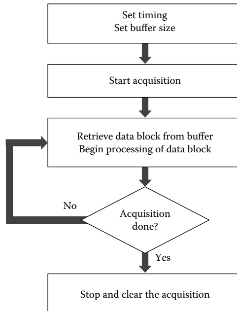
FIGURE 10.5 Flowchart for program for a continuous buffered acquisition.
