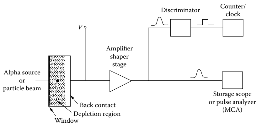
FIGURE 82.8 Using a pulse counter, this simple setup is used to measure the activity of a radioactive sample or the intensity of an accelerator beam. With the addition of a storage oscilloscope or an MCA, the energy deposited in the detector by each incoming charged particle may be measured.
