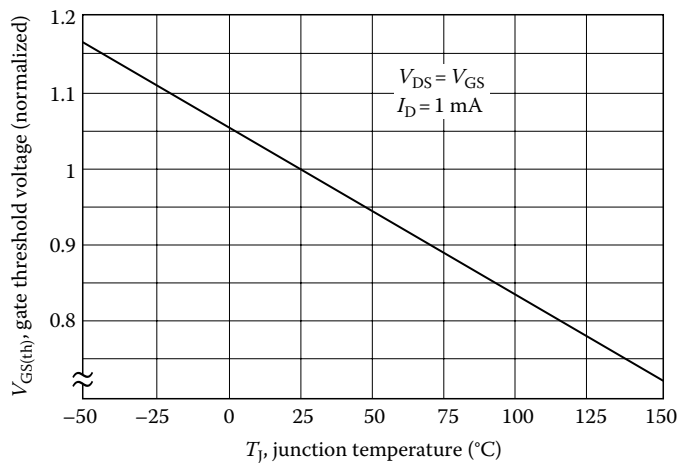
FIGURE 71.10 Power MOSFET's gate threshold variation versus temperature.
