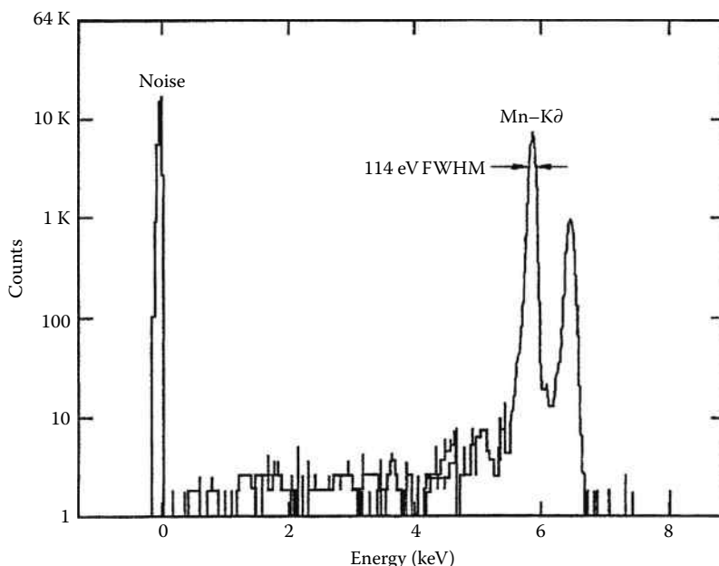
FIGURE 81.14 Manganese x-ray spectrum from ^{55}\text{Fe} source collected with an HPGe detector. (From Darken, L. S. and Cox, C. E., in Semiconductors for Room-Temperature Nuclear Detector Applications , Academic Press, New York, 1995, reprinted with permission of Oxford Instruments, Inc.)
