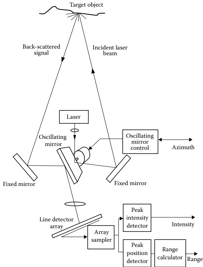
FIGURE 14.6 The Hymarc laser triangulation line scanner uses the synchronized scanning principle. Both sides of an oscillating mirror are used to sweep both the projected beam and the axis of detection over the target. The detector array is tilted to the lens plane to maximize the depth of focus.
