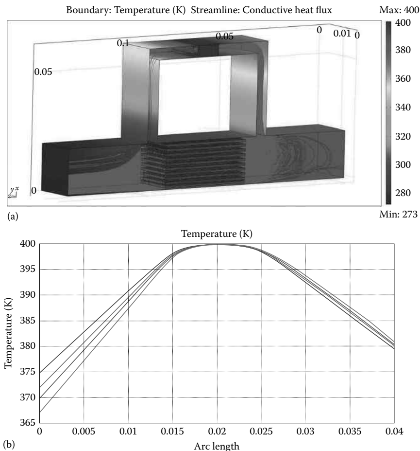
FIGURE 50.7 (a) Simulation result of temperature distribution over capillary zone in the sensor. (b) Simulated profile temperature for capillary-type thermal mass flow meter.
