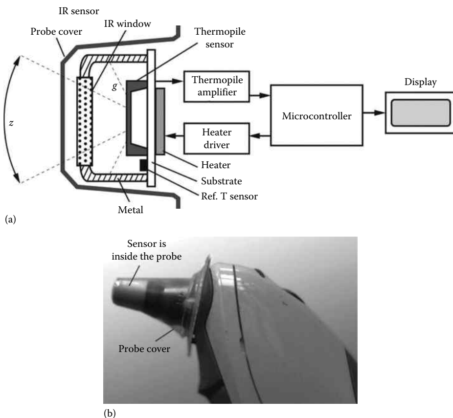
FIGURE 72.14 (a) Heated IR sensor in a medical ear thermometer and (b) the front end of Braun-Thermoscan ear thermometer.
