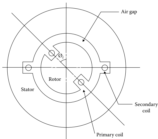
FIGURE 24.10 An induction potentiometer is a linear-variable inductor with two concentrated windings wound on the stator and on the rotor. The rotor winding is excited with ac, inducing voltage in the stator windings. The amplitude of the output voltage is dependent on the relative positions of the coils, as determined by the angle of rotation. For concentrated coils, the variation of the amplitude is sinusoidal, but linearity is restricted in the region of the null position. Different variations of induction potentiometers are available with distributed coils that give linear voltages over an angle of 180° of rotation.
