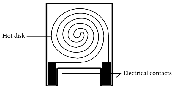
FIGURE 66.4 Schematic diagram of a transient hot-disk instrument.
