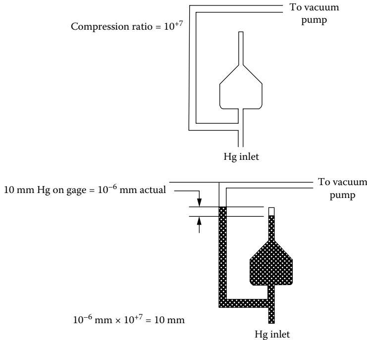
FIGURE 40.4 McLeod gage. (From Hoffman, D.M. et al., The Handbook of Vacuum Science and Technology , Academic Press, Orlando, FL, 1998. With permission.)
