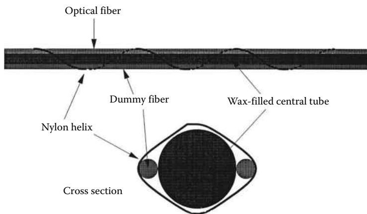
FIGURE 77.9 Fiber-optic distributed heat (fire) alarm.
