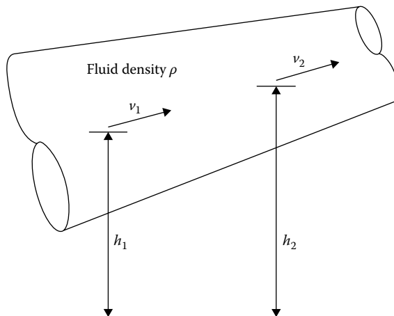
FIGURE 51.2 Flow through an inclined, tapered pipe.
