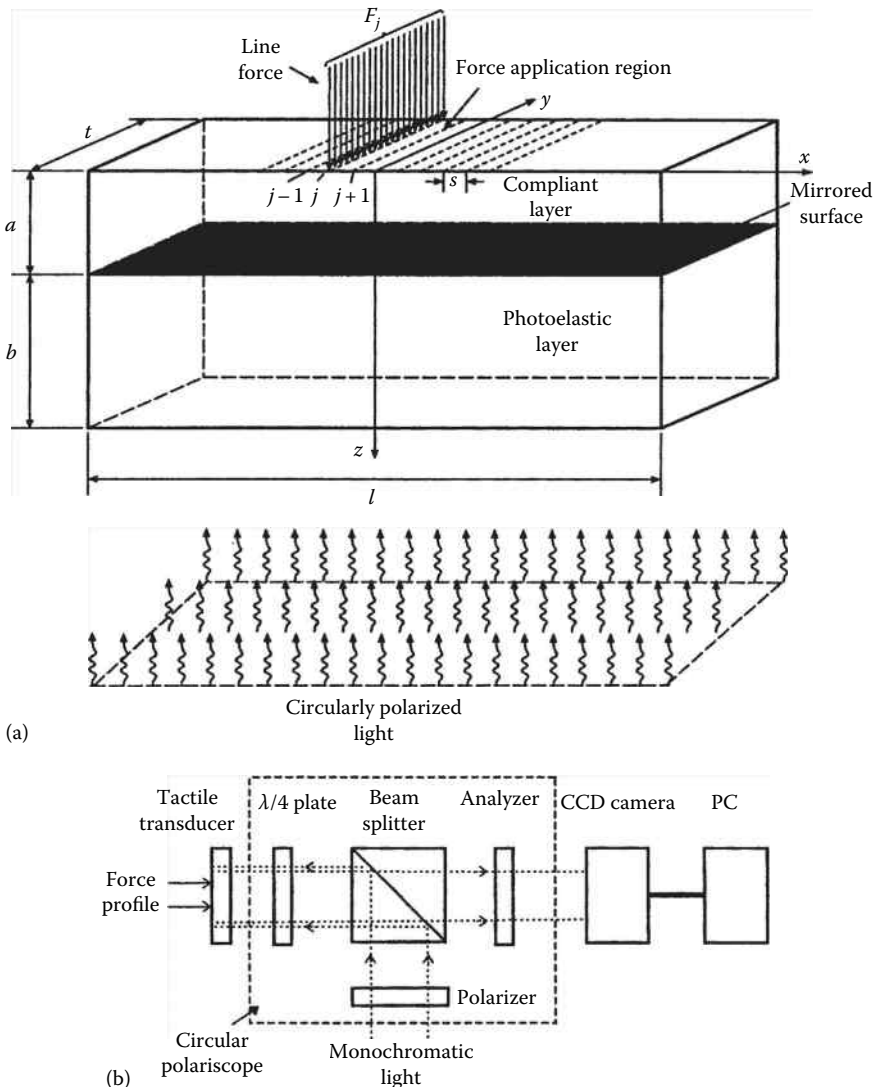
FIGURE 38.12 (a) Photoelastic transducer. (b) Circular reflective polariscope.
