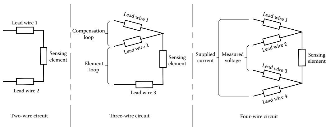
FIGURE 68.15 Temperature sensor lead wire configurations.
