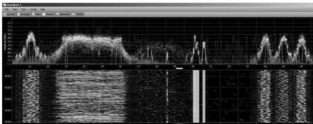
FIGURE 86.5 Density graph and waterfall trace of the 2.4 GHz band.
