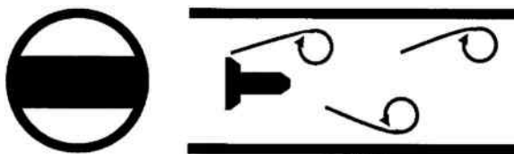
FIGURE 58.2 Vortex shedding in a pipe.
