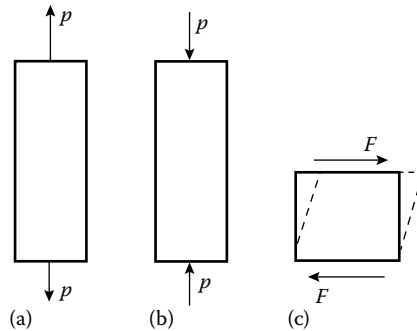
FIGURE 41.1 When a metal is loaded in uniaxial tension (a), uniaxial compression (b), or simple shear (c), it will behave elastically until a critical value of normal stress or shear stress is reached.
