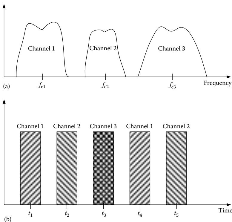
FIGURE 90.2 Basic characteristics of (a) FDM and (b) TDM signals. In FDM different channels are allocated at different subcarrier frequencies ( f_{c1}, f_{c2}, \dots ) while in TDM, only one channel is transmitted at a given time. The remaining channels are transmitted sequentially.
