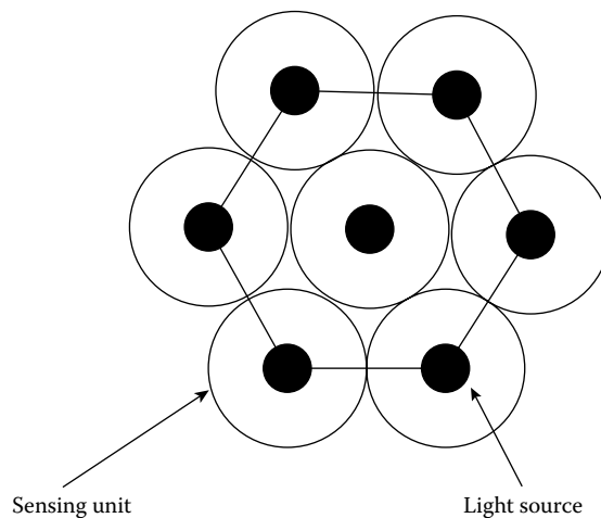
FIGURE 22.15 Configuration of HexEye (top view).
