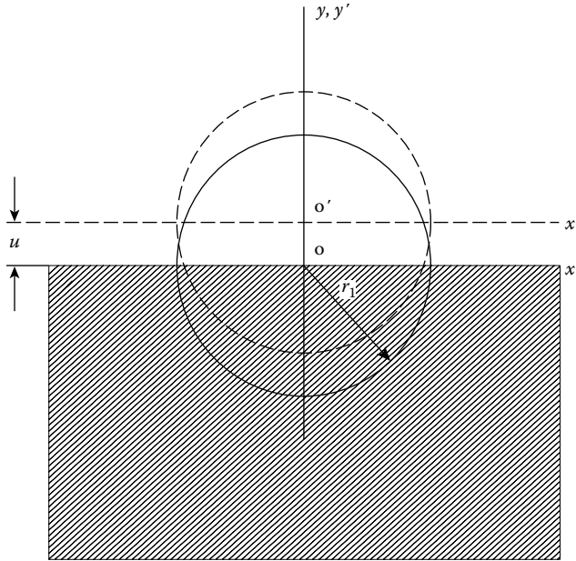
FIGURE 34.2 Essential features of a position-sending detector (PSD), as represented by a photodetector shadowed by a semi-infinite knife edge.
