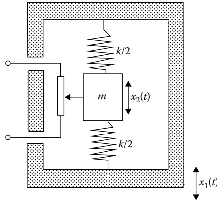
FIGURE 36.14 A potentiometer accelerometer. The relative displacement of the seismic mass is sensed by a potentiometer arrangement. The potentiometer adds extra weight, making these accelerometers relatively heavier. Suitable liquids filling the frame can be used as damping elements. These accelerometers are mainly used in low-frequency applications.
