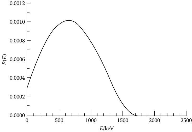
FIGURE 80.3 Theoretical distribution of beta particles as a function of energy for ^{32}\text{P} . (From Collé, R., NIST, private communication, 1997.)
