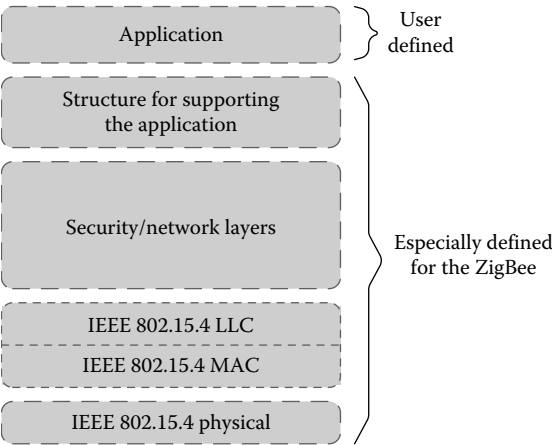
FIGURE 85.17 Adopted layers from the OSI model for use by ZigBee.
