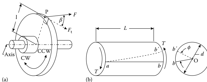
FIGURE 44.1 (a) Off-axis force F at P produces a torque T = (F \cos \beta) l tending to rotate the body in the CW direction. (b) Transmitting torque T over length L twists the shaft through angle \phi .
