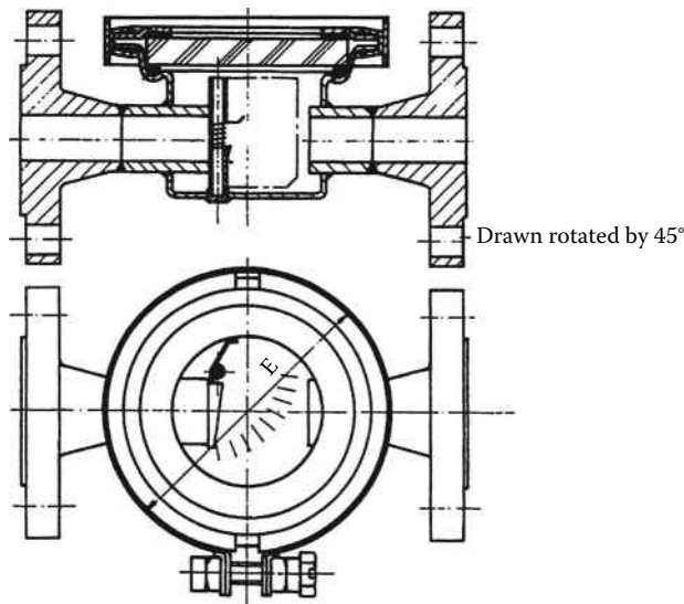
FIGURE 52.4 Flow indicator. The angle of the vane provides a measure of the flow rate.
