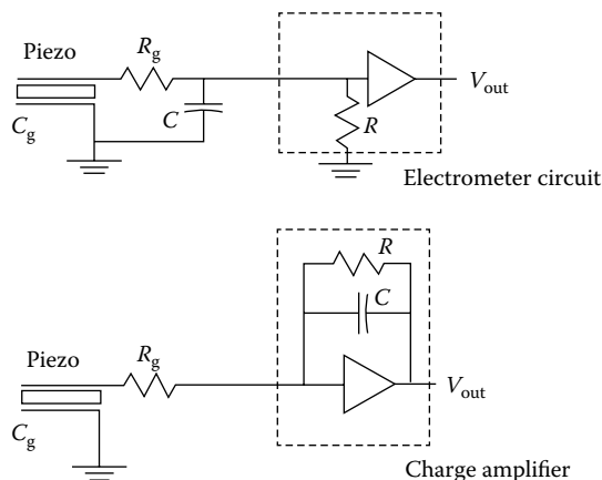
FIGURE 37.11 The electrometer and charge amplifier are the most common circuits used to measure charge from piezoelectric transducers.
