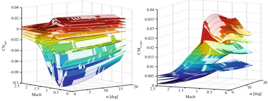
Fig. 7.27 Identified aerodynamic coefficients C_{n_{wfl}} (left) and C_{n_{wfl}} (right) superimposed with their database
