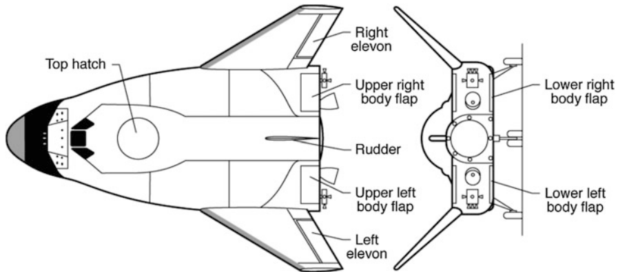
Fig. 7.18 The HL-20 vehicle
