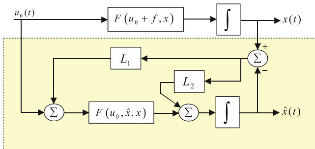
Fig. 3.12 Bloc diagram of the nonlinear residual generator
