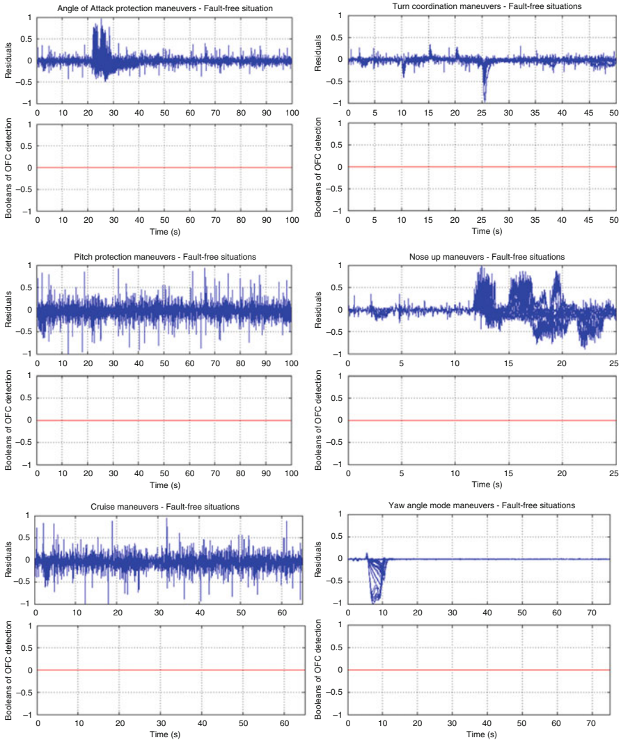
Fig. 3.22 Normalized residuals in fault-free situations with parametric variations: Fault reconstruction via sliding-mode differentiation
