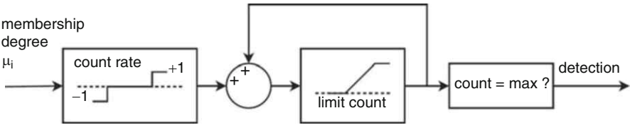
Fig. 5.8 Soft monitor
