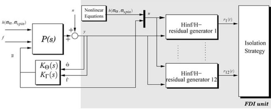
Fig. 7.5 FDI system
