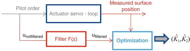
Fig. 4.5 Optimization of detection filter parameters
