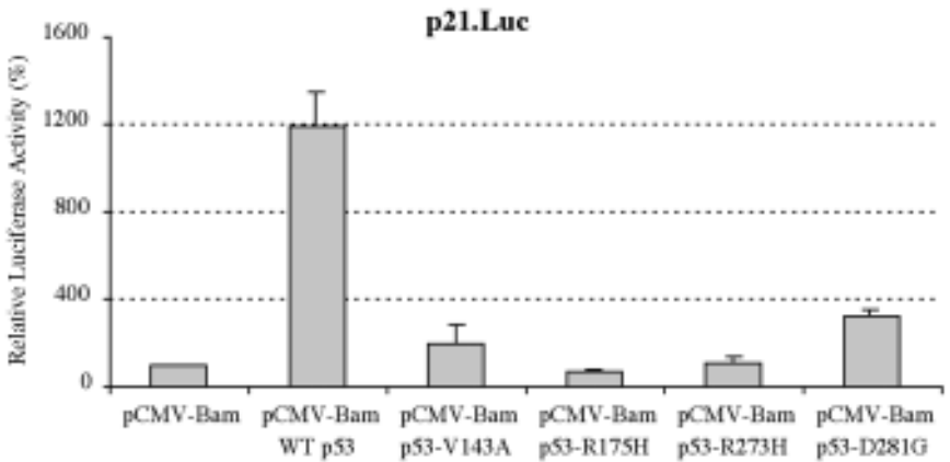
Fig. 3. Human Saos-2 cells were transfected with the expression plasmid for WT p53, p53-V143A, p53-R175H, p53-R273H, p53-D281G, or vector alone (pCMV-Bam) and p21.Luc using the LIPOFECTAMINE 2000 reagent as described in Table 4 . The cells were harvested 48 h after transfection using Reporter lysis buffer, and luciferase activity was measured. The vector reading was set to 100.
