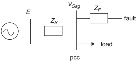
FIGURE 31.4 Voltage divider model for a voltage sag.
