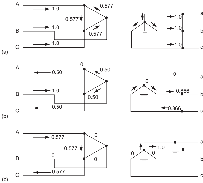
FIGURE 23.12 \Delta -Y transformer banks.
