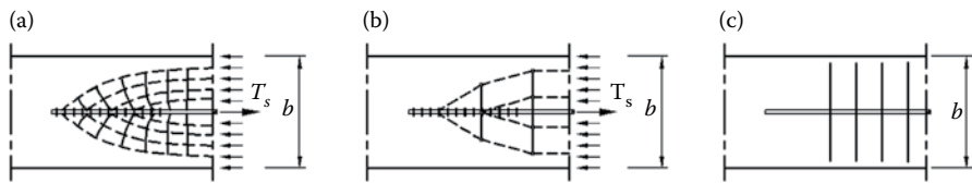
FIGURE 3.14 Symmetrical anchorage of a reinforcing bar in a concrete body: (a) stress trajectories, (b) plane STM , and (c) associated transverse reinforcement. (From Schlaich, J., and Schäfer K., IABSE Workshop , New Delhi, 1993.)
