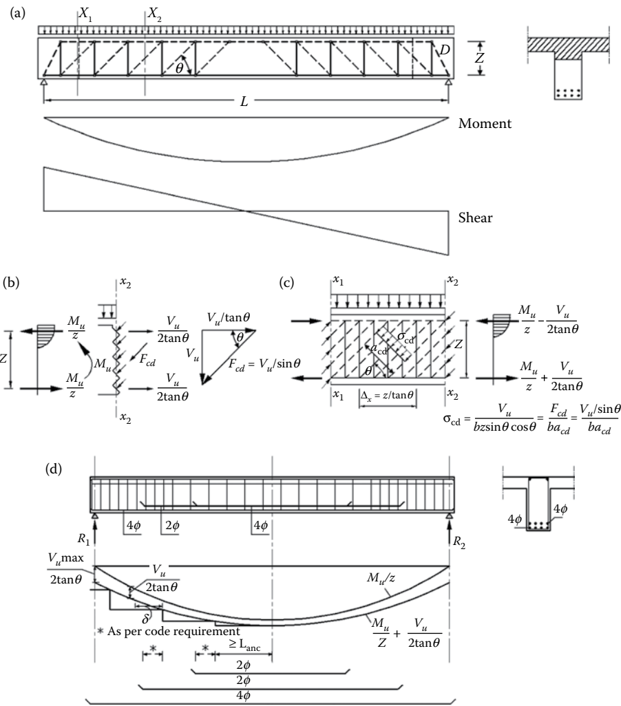
FIGURE 2.24 STM of a beam under uniform load: (a) the STM (truss model), moment and shear of the beam, (b) force transfer within section x_2 of the segment, (c) force equilibrium of the segment between sections x_1 and x_2 , and (d) tension and shifted tension diagrams of the bottom chord.
