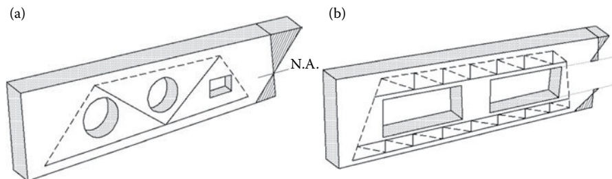
FIGURE 6.1 Definition of small and large openings. (Schlaich and Schäfer, 1993): (a) beam with small openings and (b) beam with large openings.
