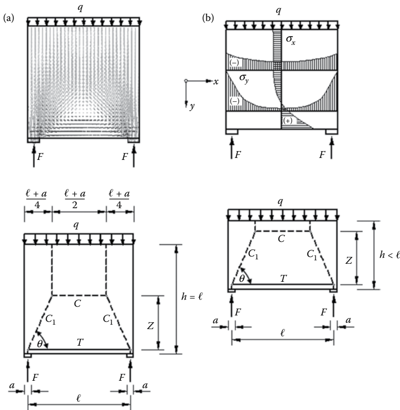
FIGURE 2.12 Region D_5 (Schlaich and Schäfer, 1991, 1993): (a) principal stress pattern from a linear-elastic analysis, (b) corresponding stress diagrams, and (c, d) STMs .
