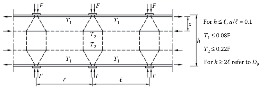
FIGURE 2.17 Region D_{10} (Schlaich and Schäfer, 1991, 1993)— STM .
