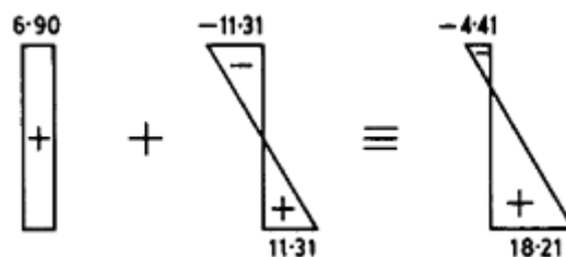
Figure 1.21 Stresses at the supports of beam in Example 1.1 (N/mm 2 ).
