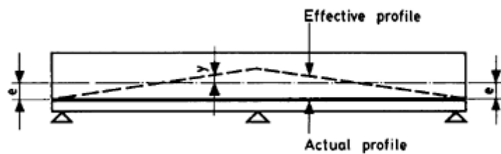
Figure 11.3 Effective tendon profile.
