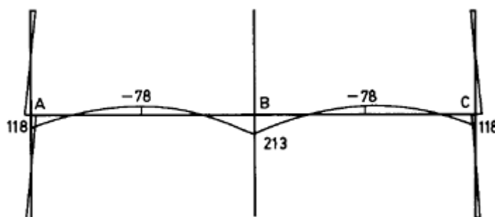
Figure 12.15 Bending and prestress moments at transfer (kNm).
