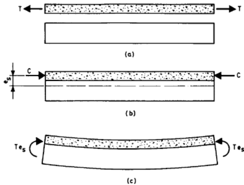
Figure 10.14 Internal stress resultants due to differential movements.
