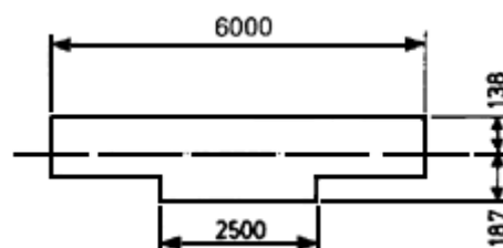
Figure 12.12 Equivalent slab section at drop panel.
