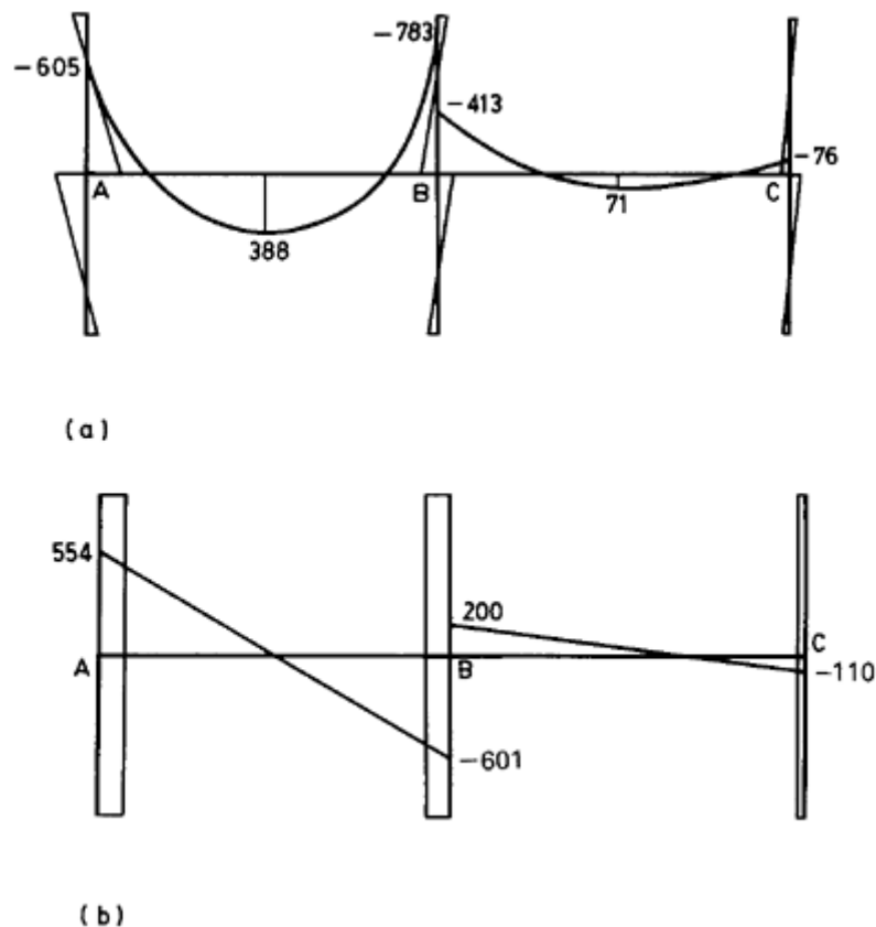
Figure 12.21 Ultimate (a) bending moment (kNm) and shear force (kN) diagrams.
