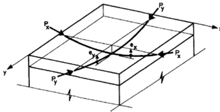
Figure 12.1 Two-way prestressed concrete slab.
