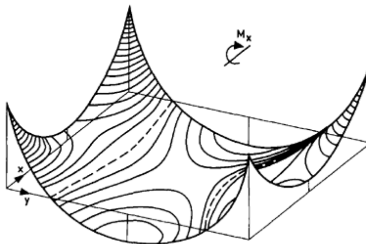
Figure 12.4 Bending moment distribution in flat slab panel due to applied loads.
