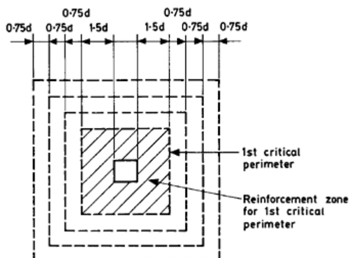
Figure 12.19 Failure zones.
