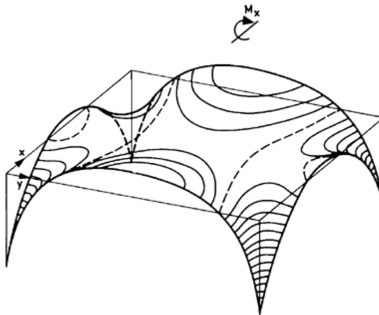
Figure 12.5 Prestress moment distribution in flat slab panel.
