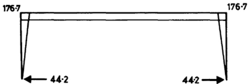
(b) Secondary moments and reactions (kNm, kN)
