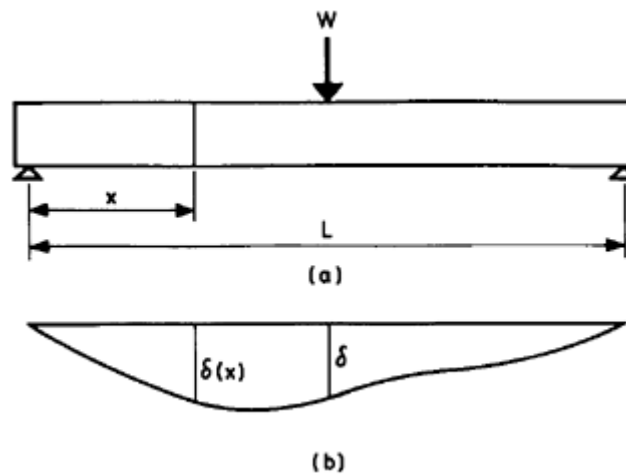
Figure 6.1 The virtual work principle.
