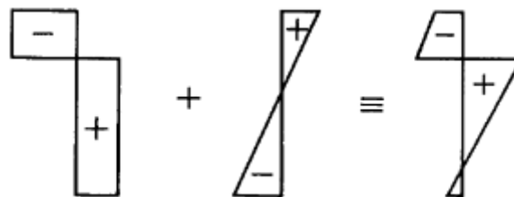
Figure 10.15 Stresses due to differential movements.
