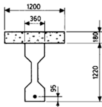
Figure 10.6 Composite section in Example 10.2.
