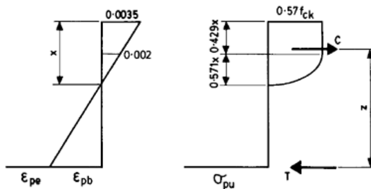
Figure 5.13 Strain and stress distributions from Fig. 5.12 .
