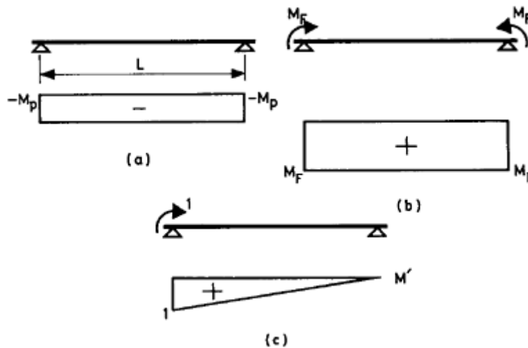
Figure 11.6 Primary moment as distributed applied moment.
