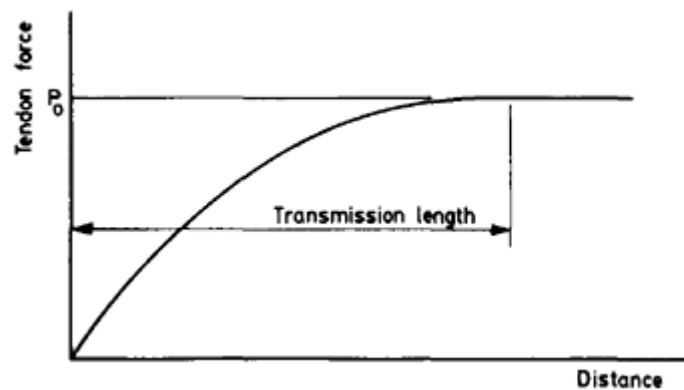
Figure 8.14 Transmission length.
