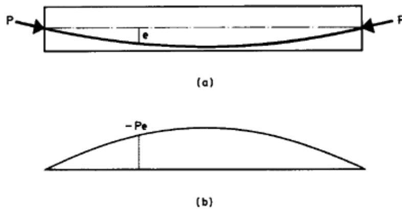
Figure 6.2 Relationship between (a) tendon eccentricity and (b) prestress moment diagram.
