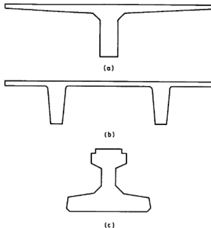
Figure 9.9 T-sections: (a) single; (b) double; (c) inverted.
