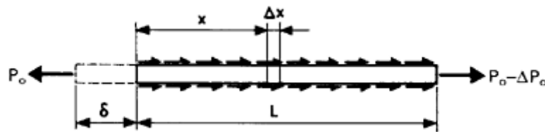
Figure 4.11 Tendon elongation.
