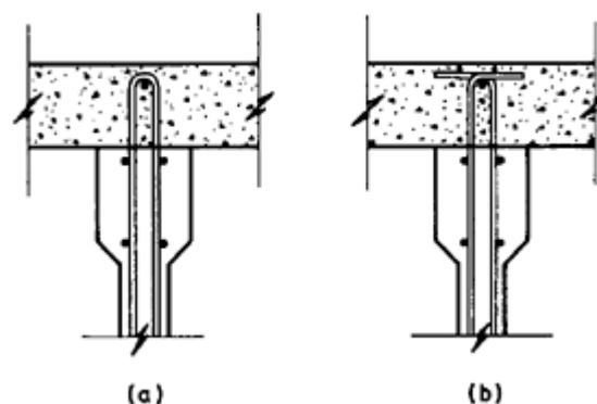
Figure 10.9 Horizontal shear connection alternatives.
