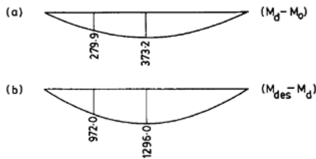
Figure 10.11 Bending moment diagrams for composite section in Example 10.4 (kNm): (a) weight of slab; (b) imposed load.
