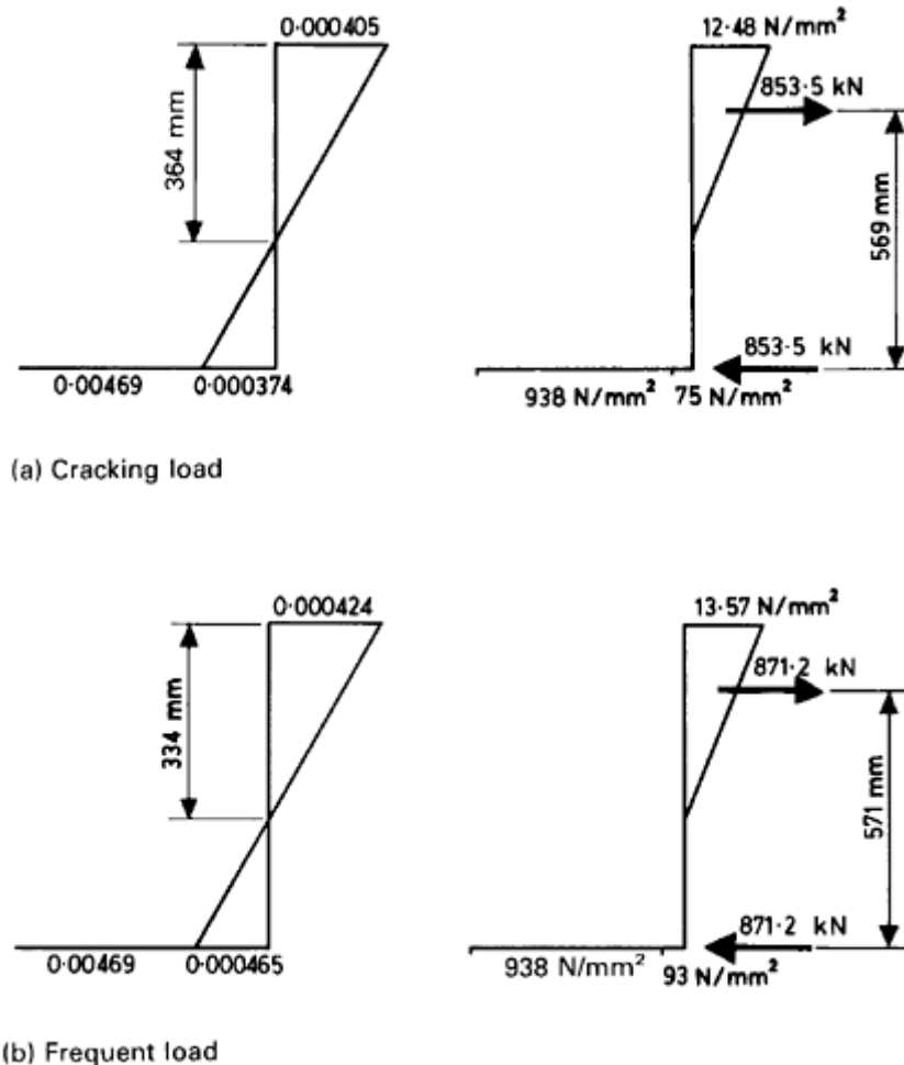
Figure 5.18 Cracked section strain and stress distributions for (a) cracking and (b) frequent loads.
