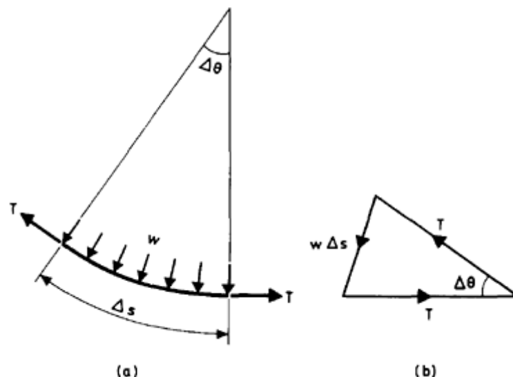
Figure 1.29 Small length of tendon.
