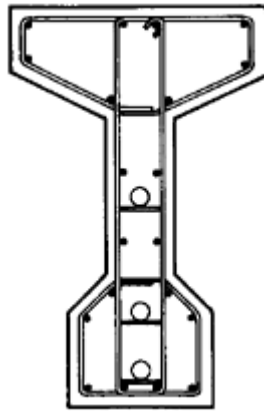
Figure 9.12 Reinforcement cage in a post-tensioned beam.
