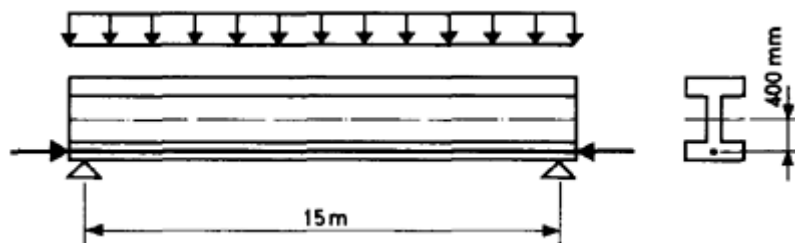
Figure 1.18 Internal equilibrium.
