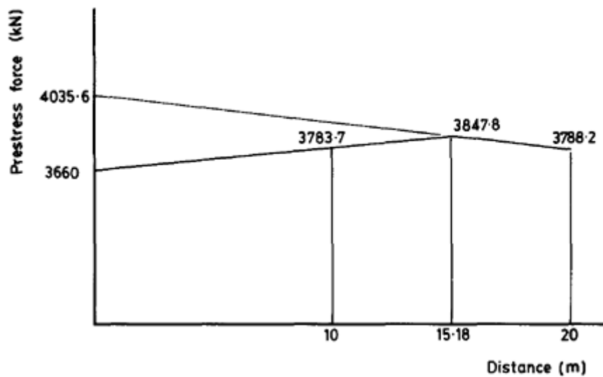
Figure 4.12 Initial overtensioning for beam in Example 4.1.
