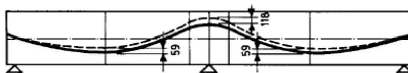
Figure 11.15 Effective tendon profile for beam in Example 11.2.
