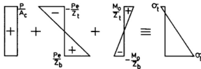
Figure 1.17 Stresses due to prestress and self weight.
