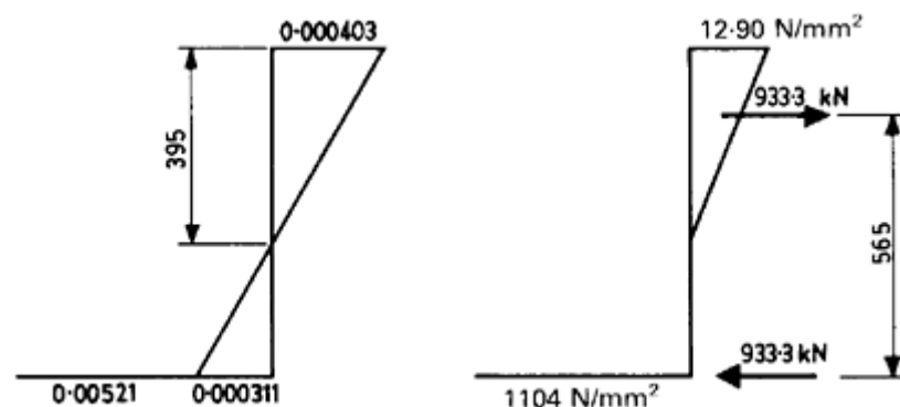
Figure 5.6 Strain and stress distributions for Example 5.3.
