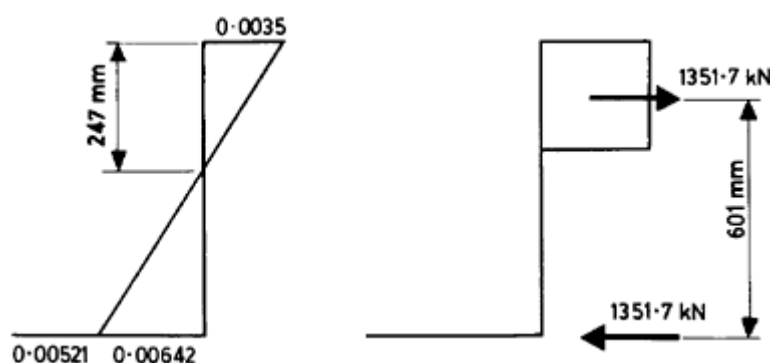
Figure 5.17 Strain and stress distributions for beam in Example 5.8.
