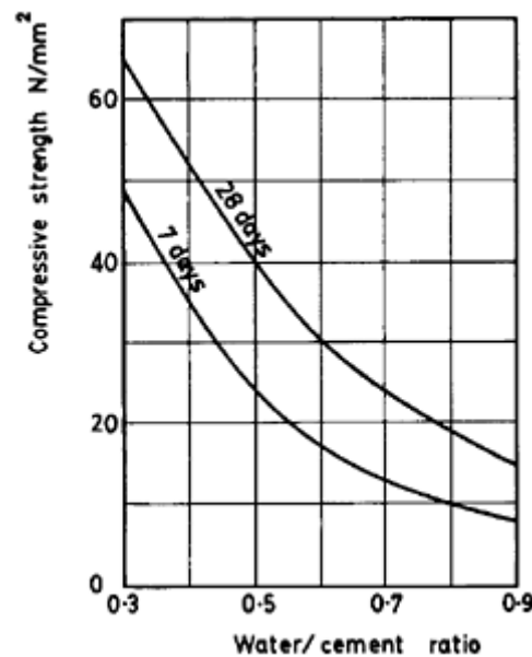
Figure 2.1 Strength of OPC concrete.
