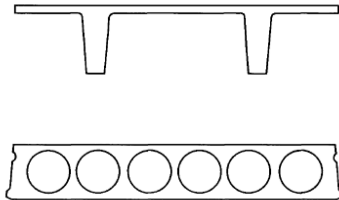
Figure 1.3 Examples of precast beams.
