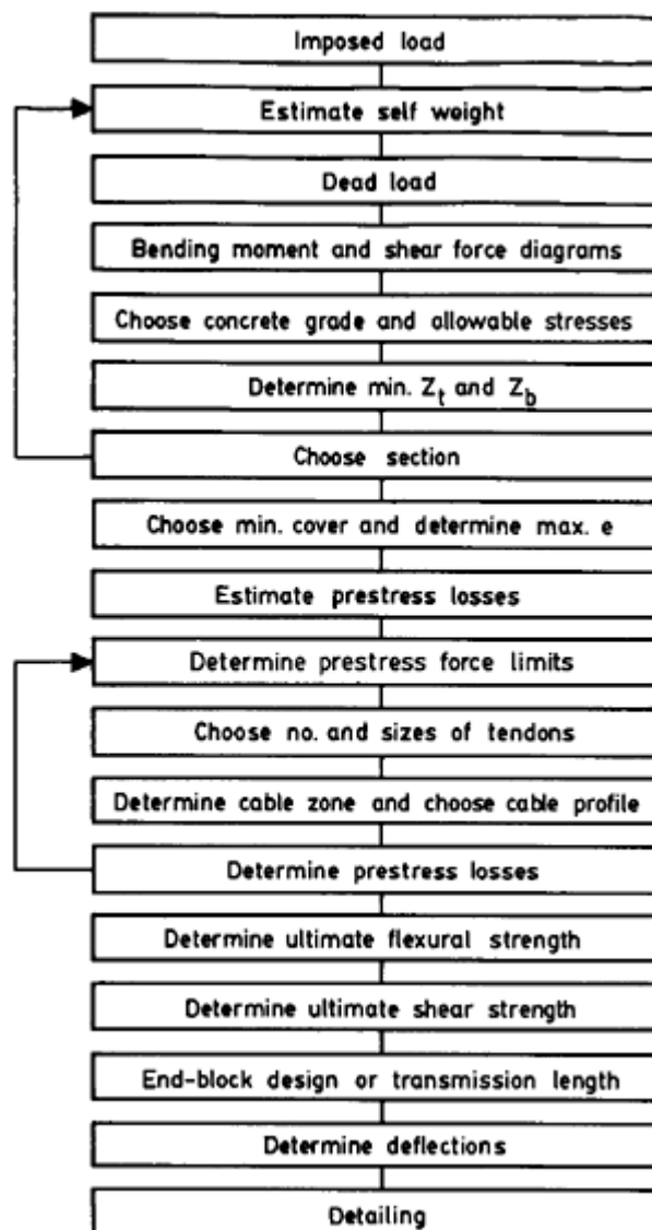
Figure 9.10 Flow chart for uncracked members.
