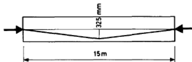
Figure 4.12 Initial overtensioning for beam in Example 4.1.
