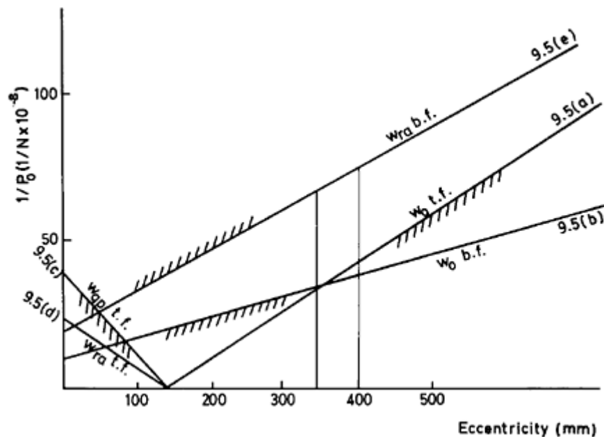
Figure 9.3 Magnel diagram.
