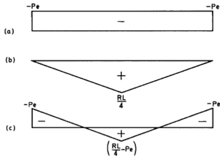
Figure 11.2 Secondary moments.
