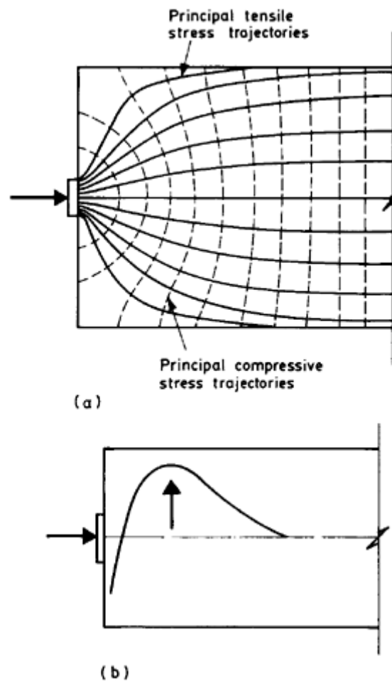
Figure 8.9 End-block (a) stress distribution and (b) bursting forces.
