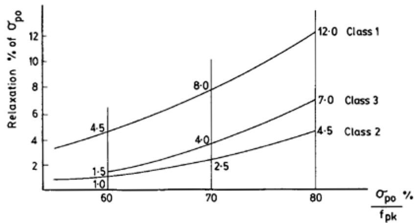
Figure 2.7 Relaxation of steel at 20 °C after 1000 h.
