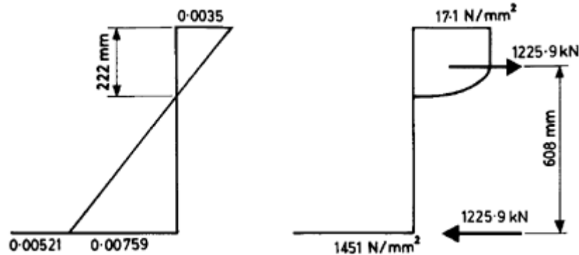
Figure 5.14 Strain and stress distributions for Example 5.5.
