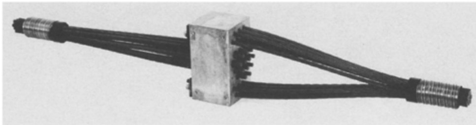
Figure 8.6 Coupler ( courtesy Bureau BBR Ltd ).
