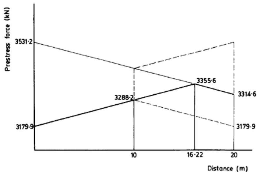
Figure 4.10 Prestress force distribution for beam in Example 4.1.
