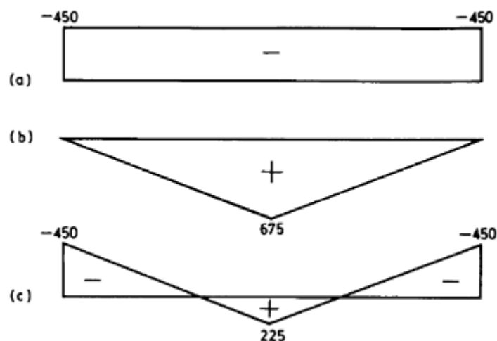
Figure 11.4 Prestress moments for beam in Example 11.1 (kNm).
