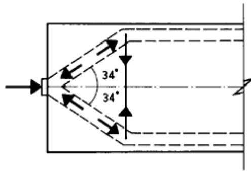
Figure 8.10 Strut-and-tie model of end-block.
