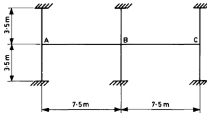
Figure 12.11 Equivalent frame.
