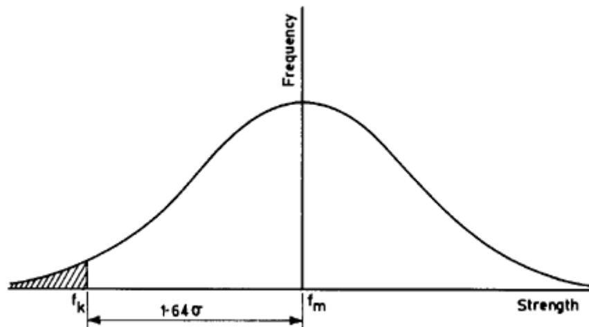
Figure 3.1 Concrete strength distribution.
