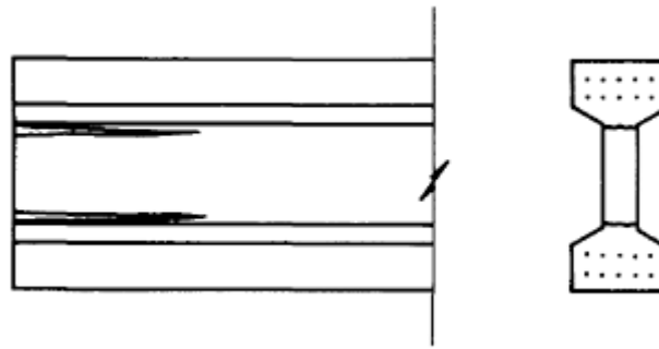
Figure 8.15 Cracking in a pretensioned member.
