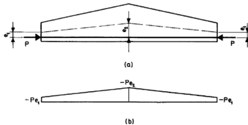
Figure 1.33 Member with varying section.
