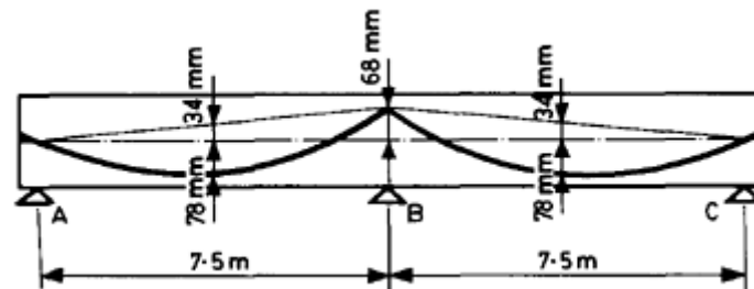
Figure 12.10 Idealized tendon profile.
