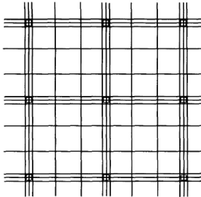
Figure 12.3 Tendon layout for square column grid.
