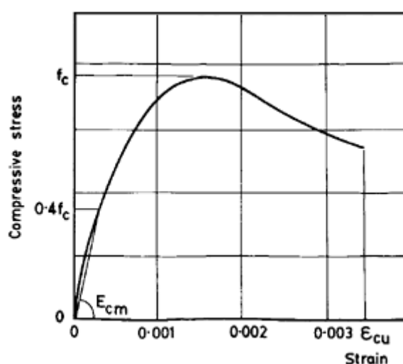
Figure 2.2 Stress-strain curve for concrete.
