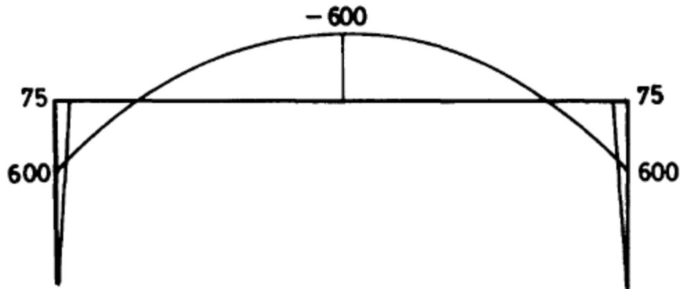
(a) Primary moments (kNm)
