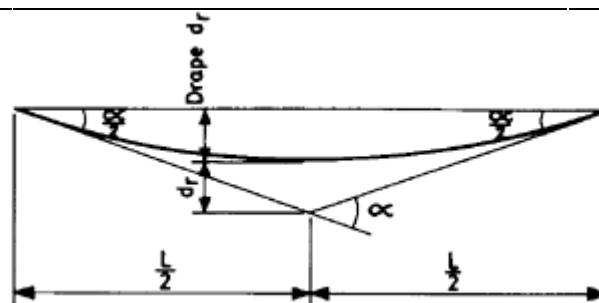
Figure 4.6 Properties of parabolic profiles.
