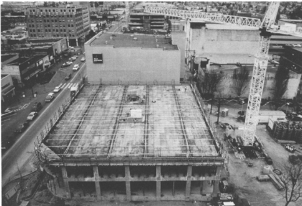
Figure 1.6 Prestressed flat slab construction ( courtesy VSL International ).
