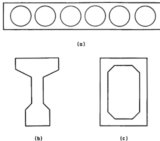
Figure 9.8 Sections: (a) hollow-core slab; (b) I-section; (c) box-section.
