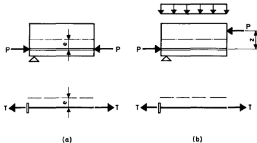
Figure 1.18 Internal equilibrium.
