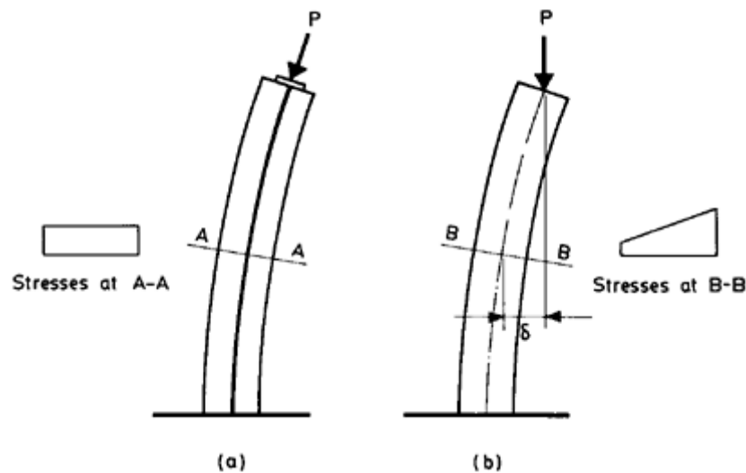
Figure 1.26 (a) Prestressed and (b) axially loaded vertical members.
