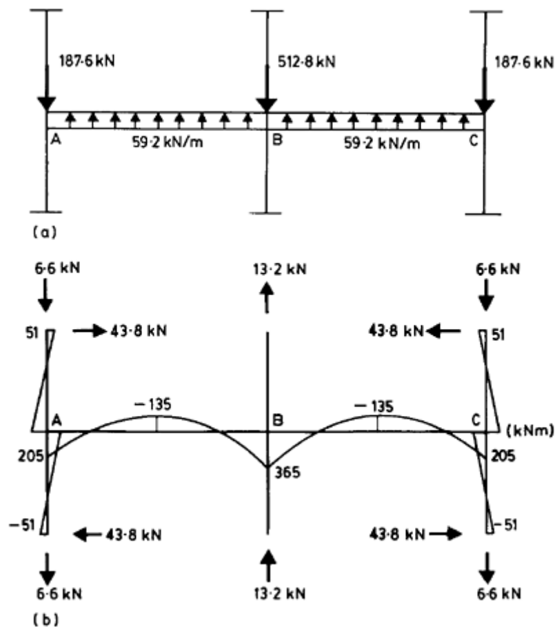
Figure 12.14 (a) Equivalent loads and (b) total prestress moments.
