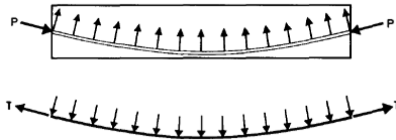
Figure 1.28 Free bodies of concrete and curved tendon.
