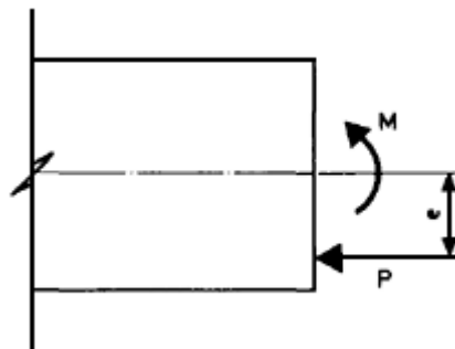
Figure 5.1 Prestress moment and applied moment at a section.
