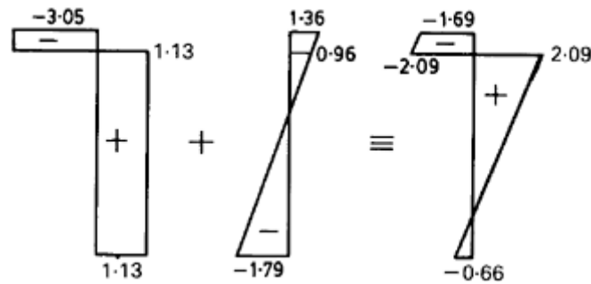
Figure 10.16 Stress distribution for composite section in Example 10.5 ( \text{N/mm}^2 ).
