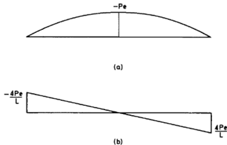
Figure 1.32 (a) Prestress moment and (b) shear force diagrams.
