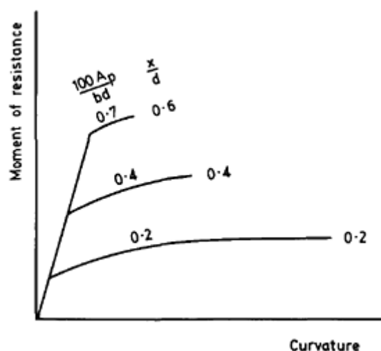
Figure 11.24 Moment-curvature relationships.
