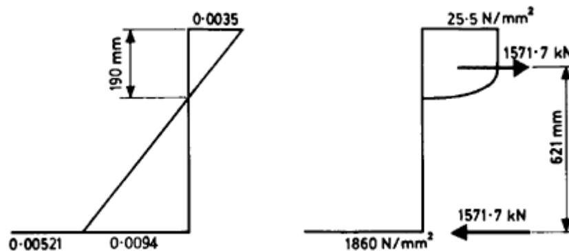
Figure 5.9 Strain and stress distributions for Example 5.4.
