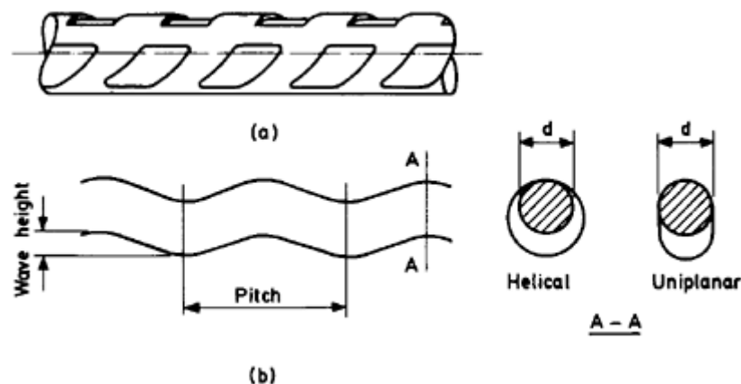
Figure 2.5 Wire for prestressing: (a) indentations; (b) crimps.
