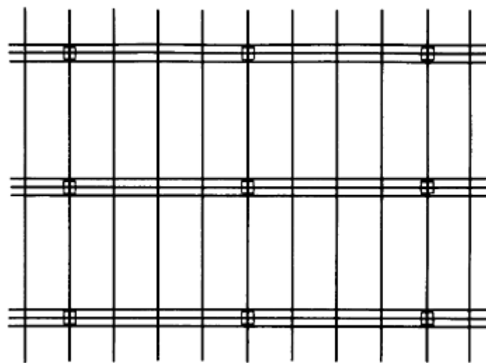
Figure 12.6 Tendon layout for rectangular column grid.
