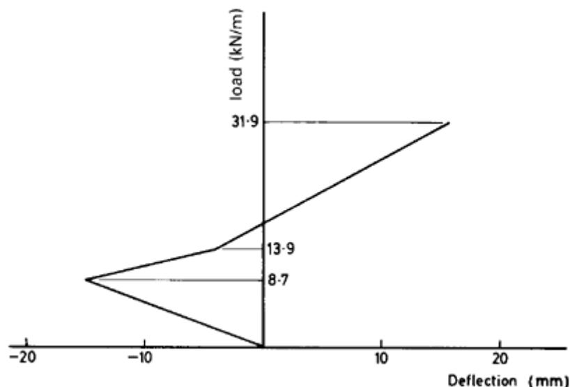
Figure 10.12 Load-deflection curve for composite section in Example 10.4.
