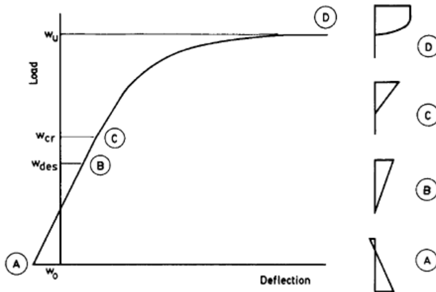
Figure 5.11 A typical load-deflection curve for a prestressed concrete member.
