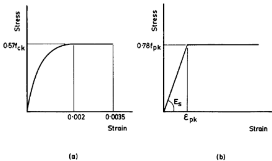
Figure 5.12 Design stress-strain curves for (a) concrete and (b) steel.
