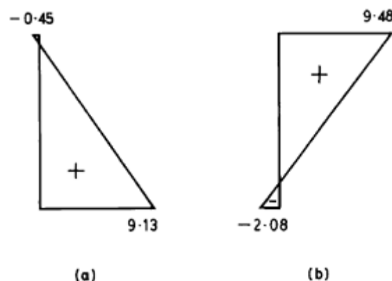
Figure 5.3 Stress distribution for beam in Example 5.1 (N/mm 2 ) (a) at transfer and (b) under the total design load.
