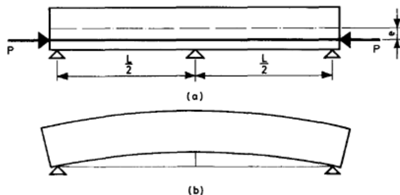
Figure 11.1 Continuous prestressed concrete beam.
