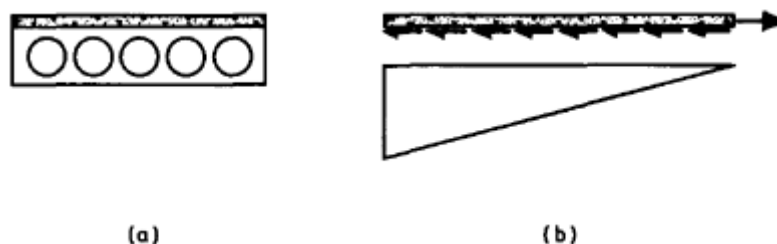
Figure 10.8 Horizontal shear: (a) composite section; (b) free-body diagram for in situ slab.
