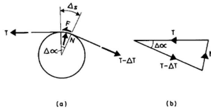
Figure 4.3 Friction in a cable.
