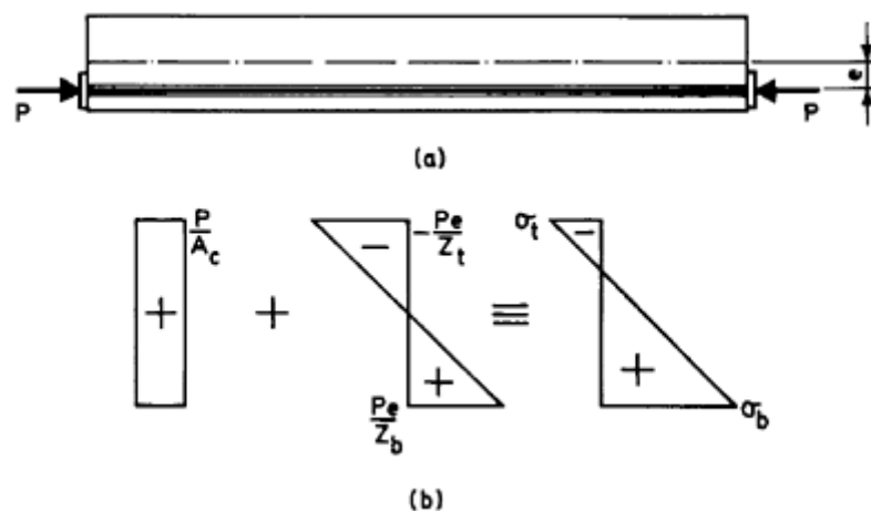
Figure 1.15 Eccentrically prestressed member.
