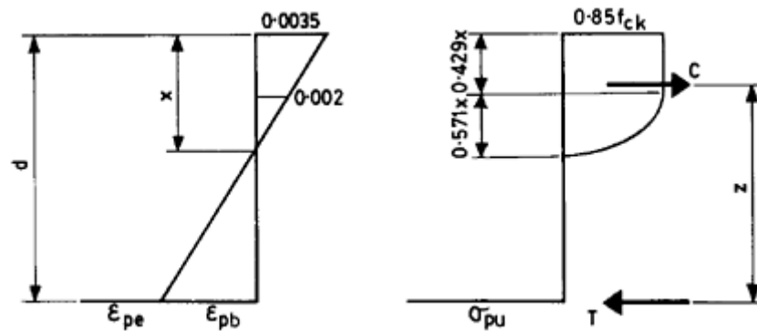
Figure 5.8 Strain and stress distributions from Fig. 5.7 .
