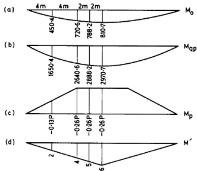
Figure 6.4 Bending moments for beam in Example 6.1 (kNm).
