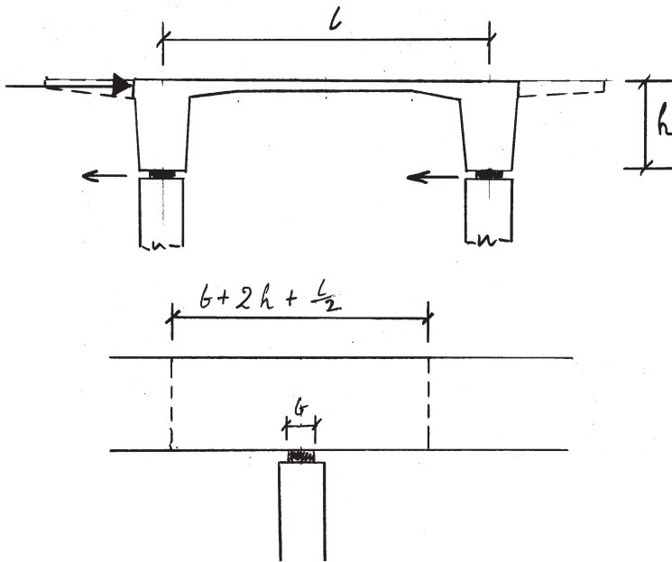
Figure 12.7 Portal resisting horizontal loads
