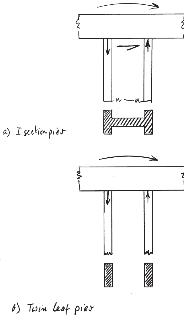
Figure 7.19 Development of twin leaf piers
