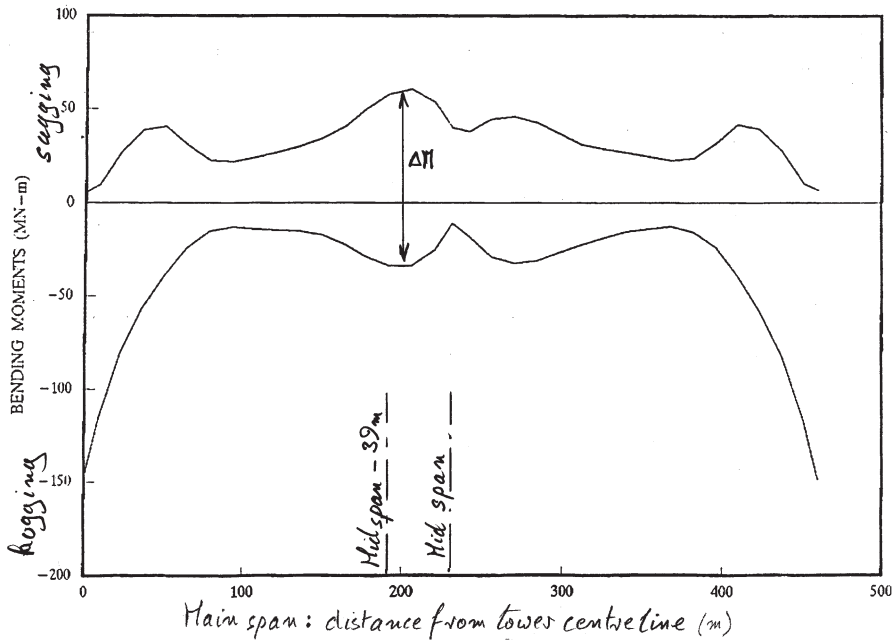
c) Live load bending moment envelope for one box
