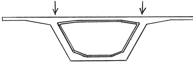
b) Narrow bottom slab with concrete cast down webs
