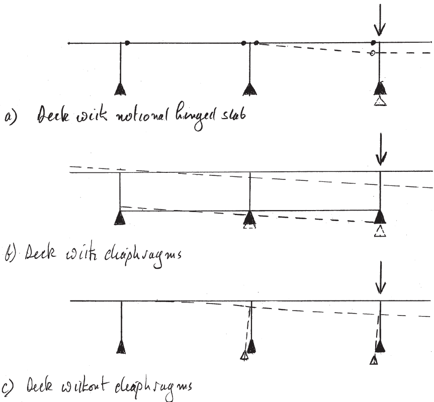
Figure 8.5 Transverse distribution of loads on beam type decks
