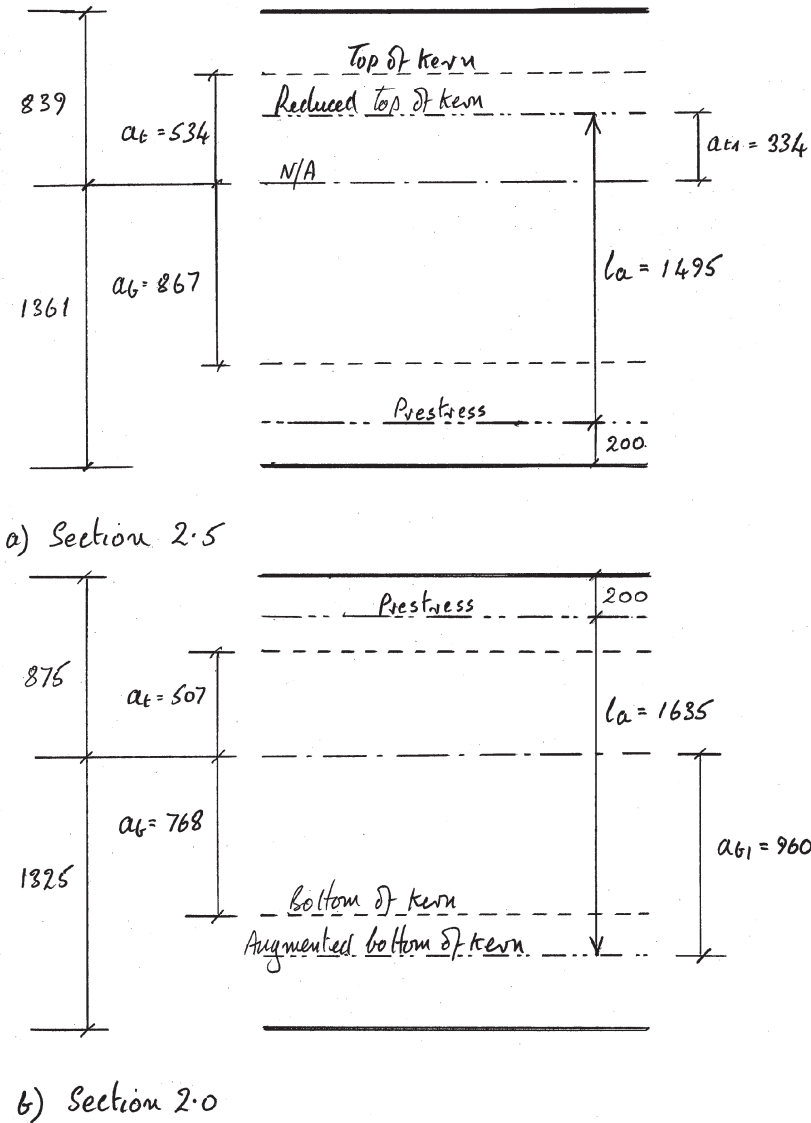
Figure 6.22 Non-zero stress limits
