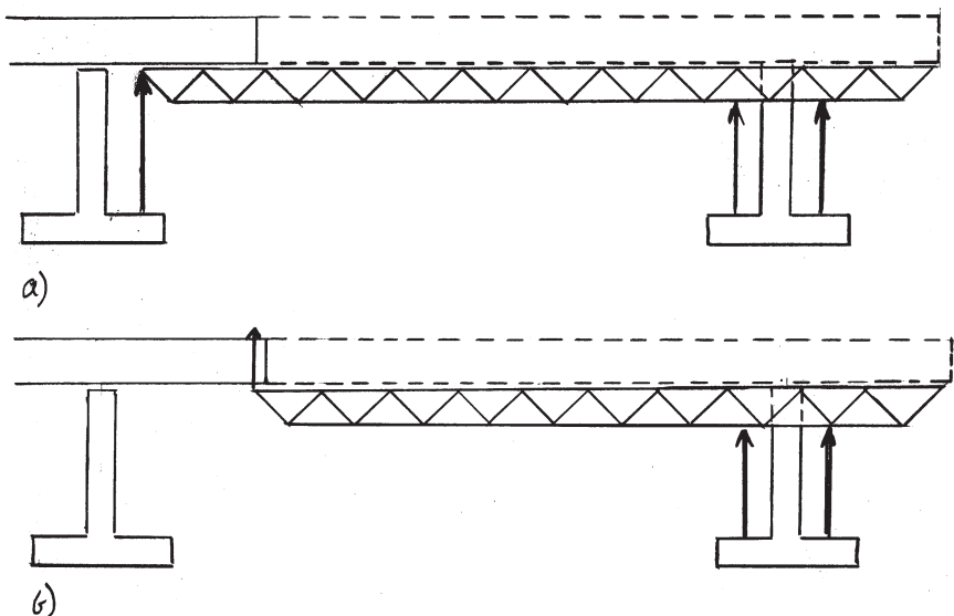
Figure 15.4 Support of falsework truss for span-by-span construction
