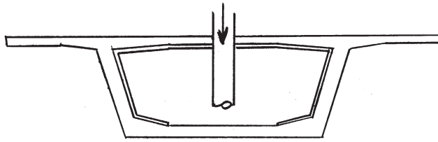
a) Wide bottom slab cast through trunking
