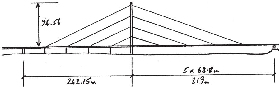
b) Knie Bridge; Düsseldorf (Adapted from Walther, R., Houniet, B., Isler, M. and Moia, P., Cable stayed Bridges, Thomas Telford 1999 London)
