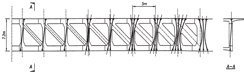
b) Prestress of truss members
