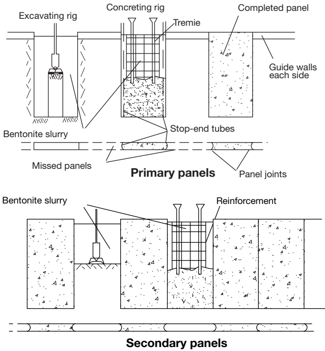
Figure 5.56 Typical construction process for a cast in situ diaphragm wall (after Woodward 2005)
