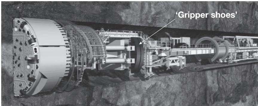
Figure 5.14 Gripper TBM (courtesy of Herrenknecht)
