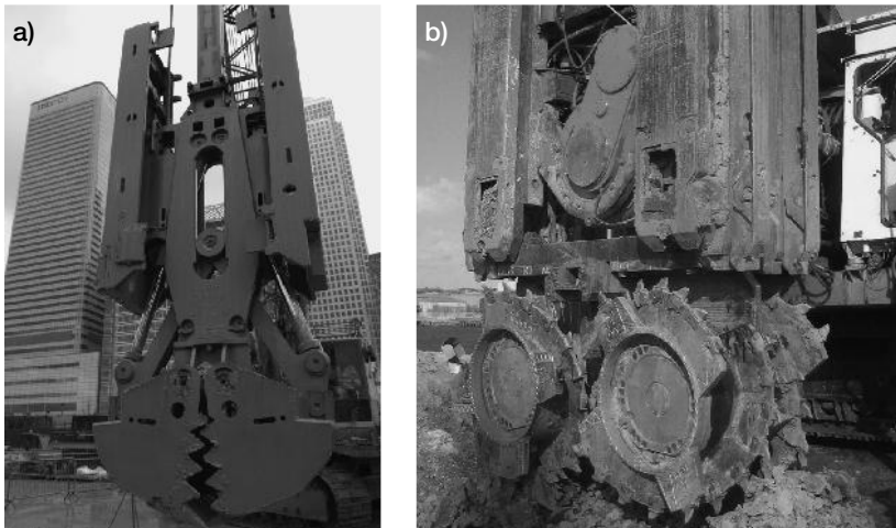
Figure 5.57 a) Grab or clam bucket excavator, and b) hydrofraise used for diaphragm wall construction (courtesy of Bachy Soletanche Ltd)
