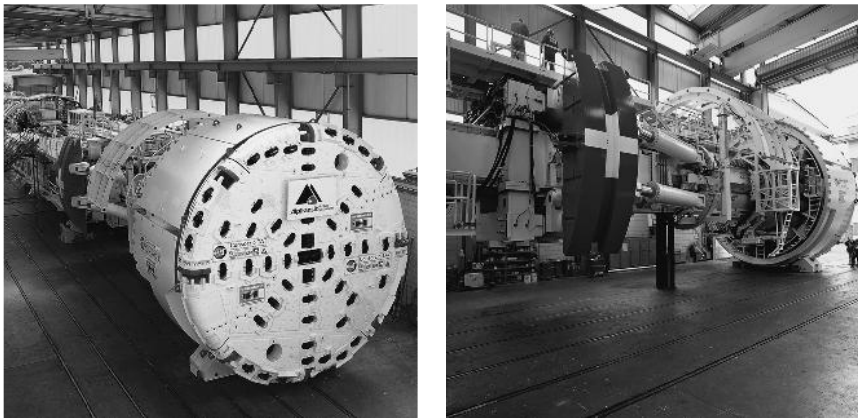
Figure 5.16 8.83 m diameter Herrenknecht S-210 Gripper TBM used on the Gotthard Base Tunnel in Switzerland, a) Cutterhead, b) Rear view showing gripper shoe (courtesy of Herrenknecht)
