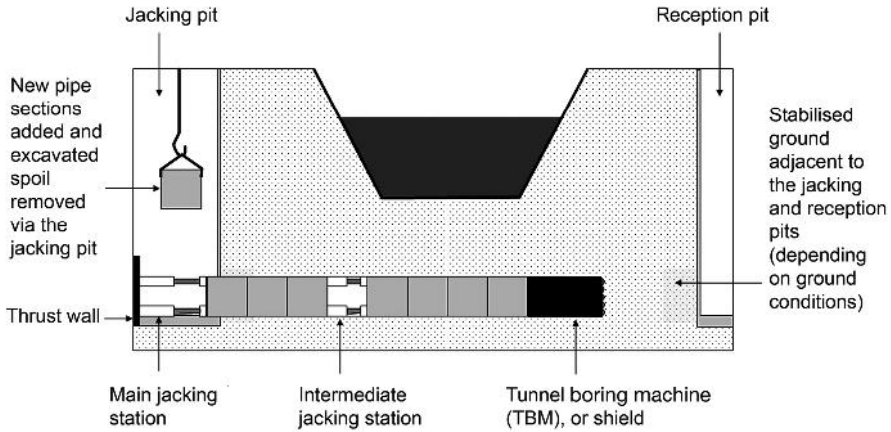
Figure 5.82 Illustration of a pipe jack under a canal (courtesy of A. Royal)
