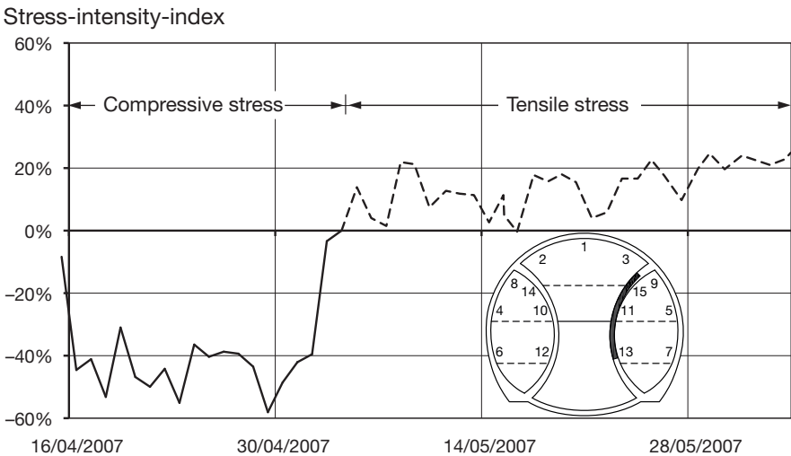
Figure 8.28 Stress-intensity-index, section W, Chainage 60
