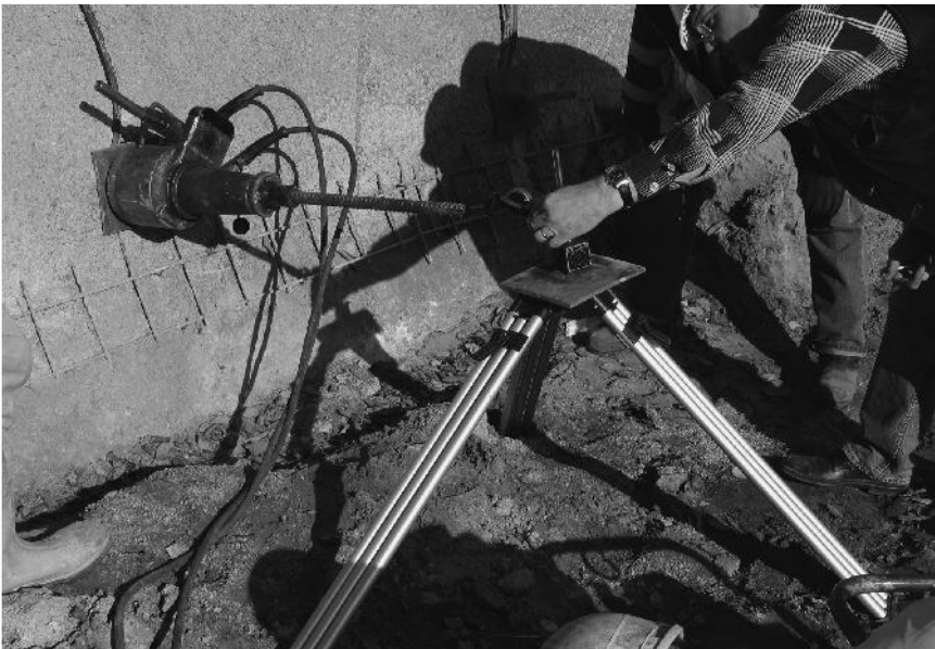
Figure 4.10 Load testing of an anchor, Lainzer Tunnel LT31, Vienna, Austria
