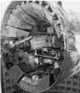
Figure 5.9 a) The boom-in-shield tunnelling machine on removal after completion of the Heathrow Express Extension Tunnel at Terminal 5 in the UK (Manufacturer: Dosco), b) the same shield crossing an existing emergency exit where external strapping was required to support the erected lining
