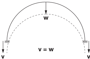
Figure 7.16 Rigid body displacement
