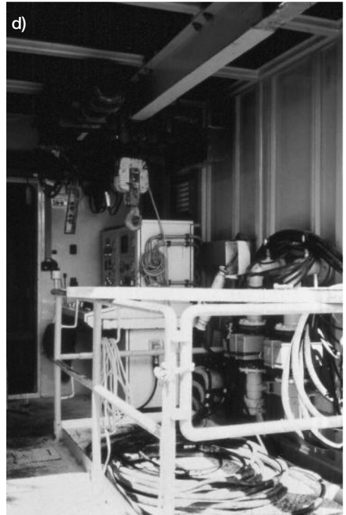
Figure 5.83 a) Jacking forward the tunnel sections from the jacking pit, b) intermediate jacking station (courtesy of Herrenknecht AG/NoDig Media Services), c) jacking arrangement and thrust wall, d) microtunnelling control centre placed over the jacking pit
