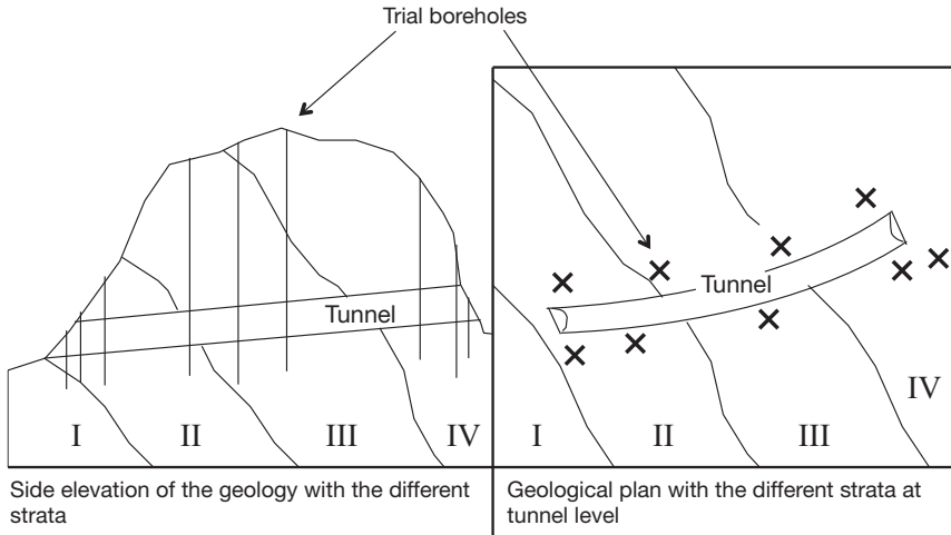
Figure 2.7 Possible borehole locations for a mountain tunnel (Note: exaggerated vertical scale)
