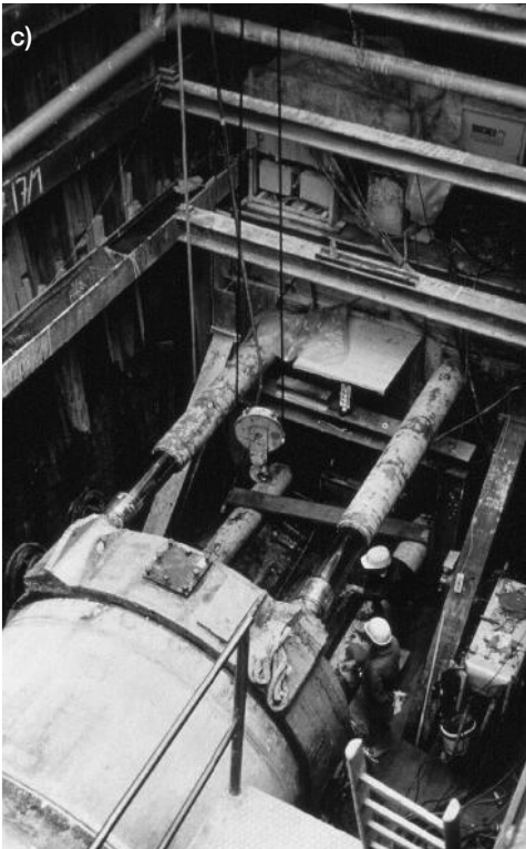
Figure 5.83 a) Jacking forward the tunnel sections from the jacking pit, b) intermediate jacking station (courtesy of Herrenknecht AG/NoDig Media Services), c) jacking arrangement and thrust wall, d) microtunnelling control centre placed over the jacking pit
