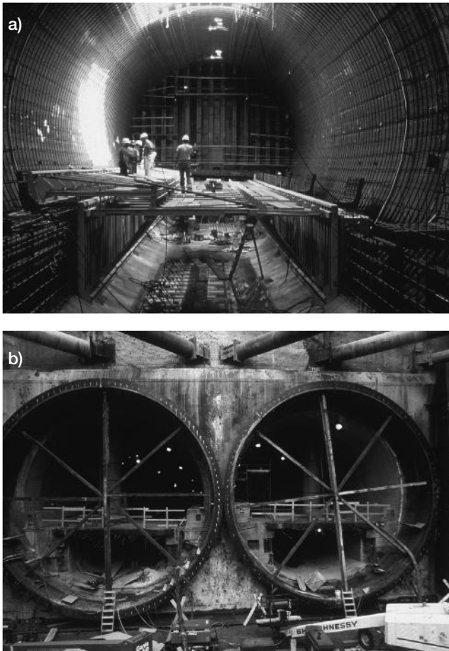
Figure 5.68 a) Internal fitting out of one of the tunnel elements (a reinforced concrete lining was placed inside the steel shell), b) the binocular immersed tube emerging into the cut-and-cover section of the Ted Williams Tunnel (courtesy of Massachusetts Turnpike Authority)
