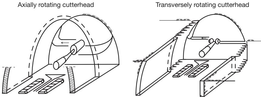
Figure 5.3 Partial face boring machine (roadheader)
