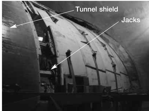
Figure 5.9 a) The boom-in-shield tunnelling machine on removal after completion of the Heathrow Express Extension Tunnel at Terminal 5 in the UK (Manufacturer: Dosco), b) the same shield crossing an existing emergency exit where external strapping was required to support the erected lining
