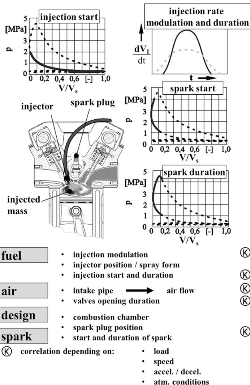
Fig. 2.40 Correlation of parameters for optimization of internal mixture formation in an SI engine. Variable parameters are indicated by K
