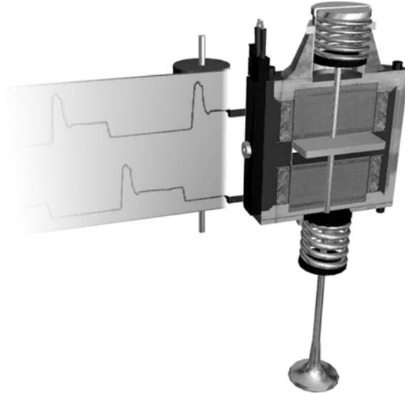
Fig. 2.33 Electromagnetic valve control
