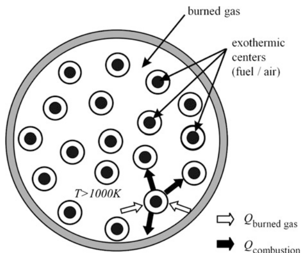
Fig. 2.66 Control of combustion by self-ignition in exothermic centers distributed isotropically within a burned gas volume
