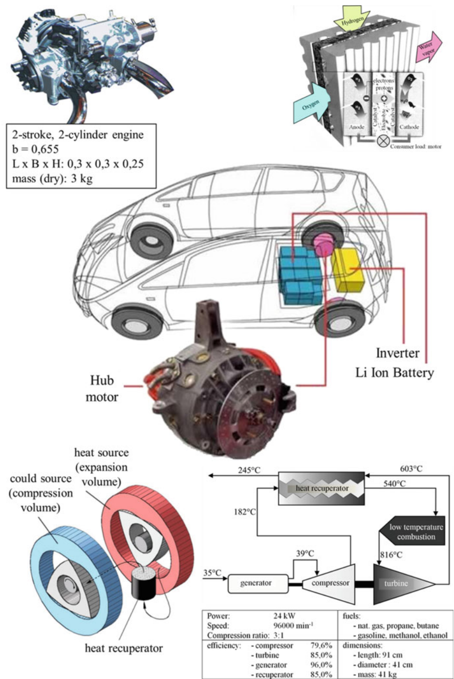
Fig. 6.5 City car with range extender. Propulsion is by motors, and electric power is generated by means of a fuel cell or by combustion (piston engine, Wankel, Stirling, or gas turbine)
