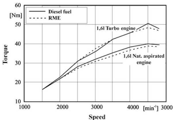
Fig. 3.40 Comparison of torque obtained for a CI engine using diesel fuel or RME
