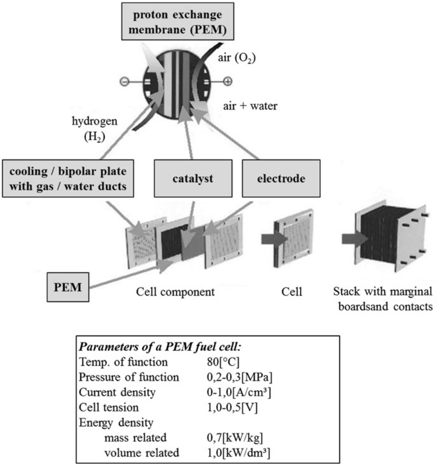
Fig. 4.19 Stack of a fuel cell
