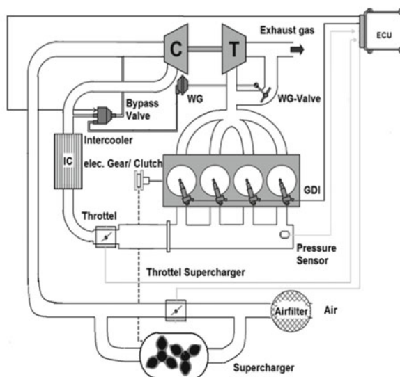
Fig. 2.13 Down-sizing compact engines with super- or turbocharging
