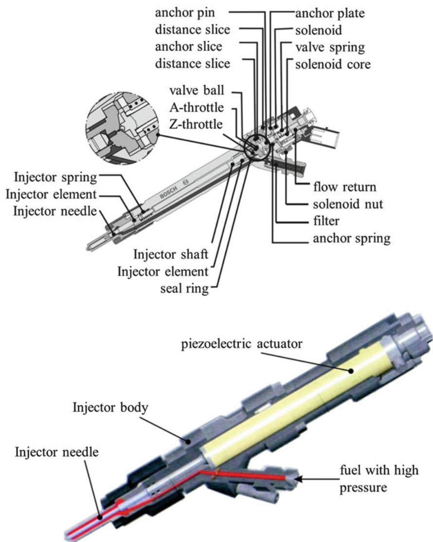
Fig. 2.60 Injectors with electromagnetic and piezoelectric/hydraulic actuation for direct injection systems in CI engines
