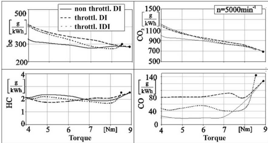
Fig. 2.74 bsfc, \text{CO}_2 , CO, and HC for constant speed and different loads in SI engines with compression ratios of 15.4:1 (direct injection, DI) and 11.5:1 (intake duct injection, IDI)
