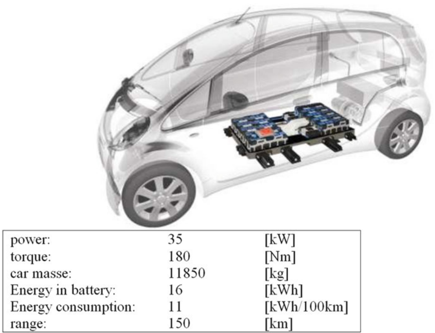
Fig. 4.37 Electric car: Mitsubishi i-MiEV (Source: Mitsubishi)
