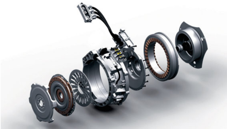
Fig. 5.38 Hybrid module with motor and clutch (Source: Porsche)
