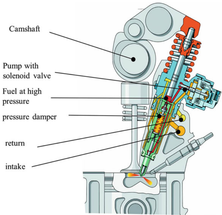
Fig. 2.63 Pump-injector unit
