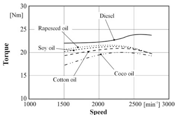
Fig. 3.38 Comparison of maximum torque obtained using different fuels
