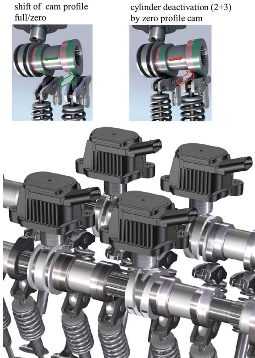
Fig. 2.27 System for shifting of cam profiles (Source: Volkswagen)
