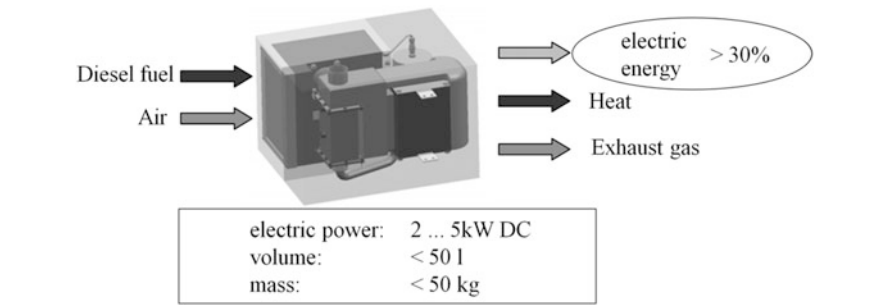
Fig. 4.31 Fuel cell using diesel fuel, with fuel dosage as shown in Fig. 4.29 [21]
