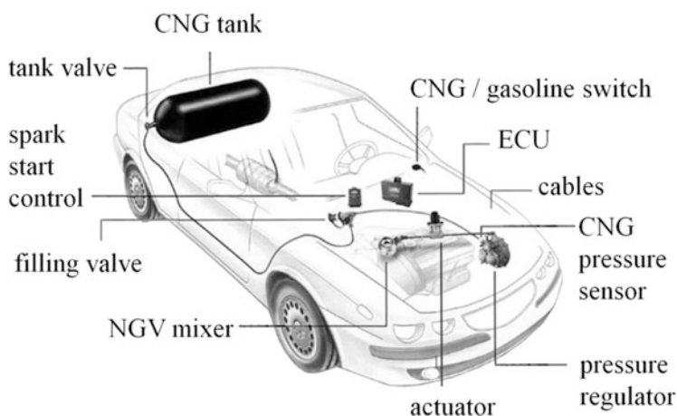
Fig. 3.13 Example of a bivalent car: Skoda Octavia (Source: Skoda)
