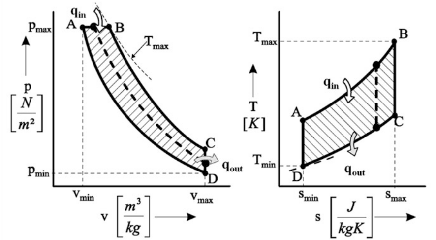
Fig. 2.4 Diesel cycle
