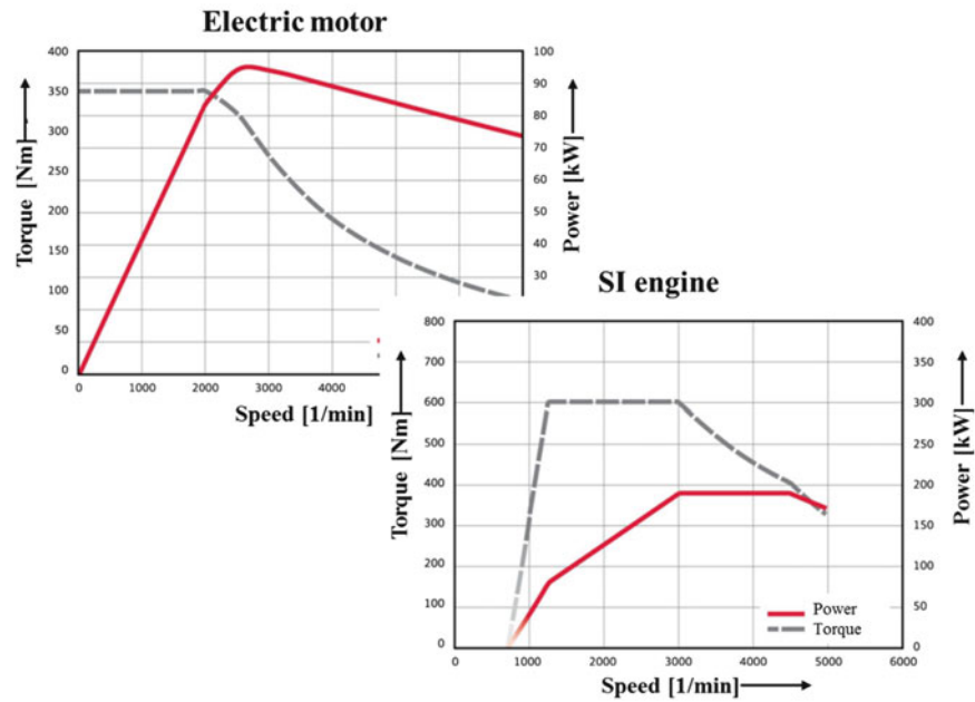
Fig. 1.21 Typical torque/power history in electric motor and spark-injection engine
