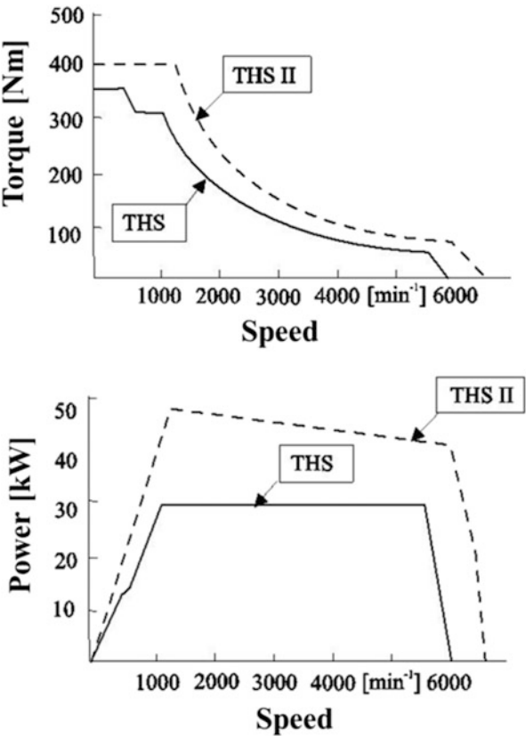
Fig. 5.30 Torque and power characteristics of the motor in the hybrid propulsion system (gasoline engine plus motor) of the Toyota Prius, 1st and 2nd generation; THS Toyota hybrid system (Source: Toyota)
