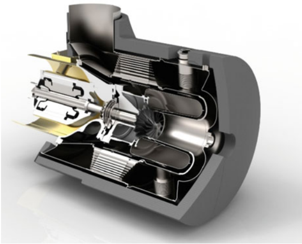
Fig. 2.92 Gas turbine as a current generator (Source: Capstone)
