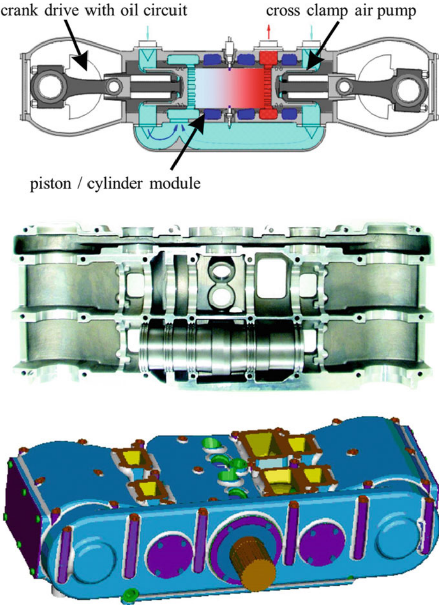
Fig. 2.84 Two-stroke engine with opposite pistons (Golde method)
