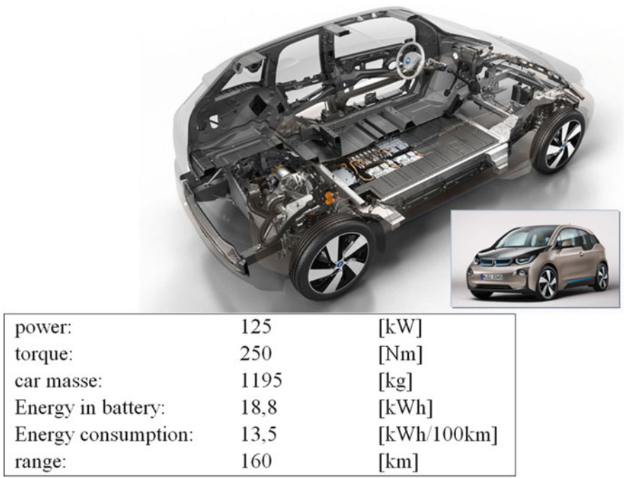
Fig. 4.35 Electric car: BMW i3 (Source: BMW)
