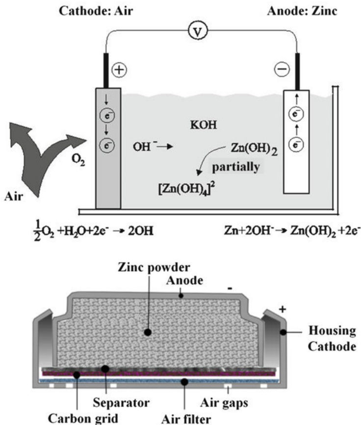
Fig. 4.11 Zinc-air battery: principle of function
