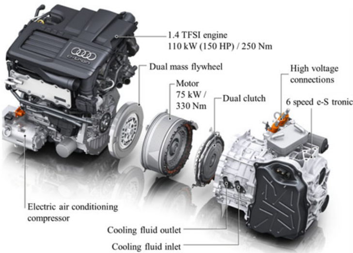
Fig. 5.40 Audi A3 e-tron (Source: Audi)
