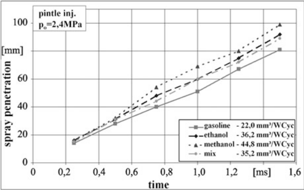
Fig. 3.28 Time-related spray penetration length for gasoline, ethanol, methanol, and a mix of all three, using a pintle injector and stoichiometric fuel/air ratio
