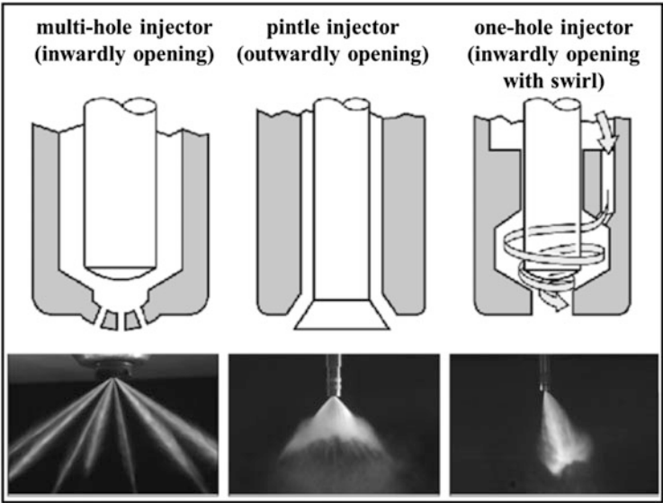
Fig. 2.47 Injectors for gasoline direct injection
