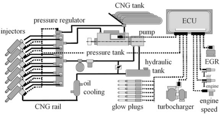
Fig. 3.10 CNG direct injection
