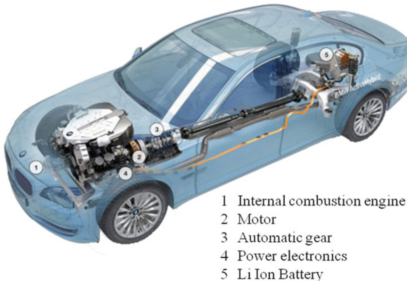
Fig. 6.2 Upper class/SUV full hybrid: BMW Active Hybrid 7
