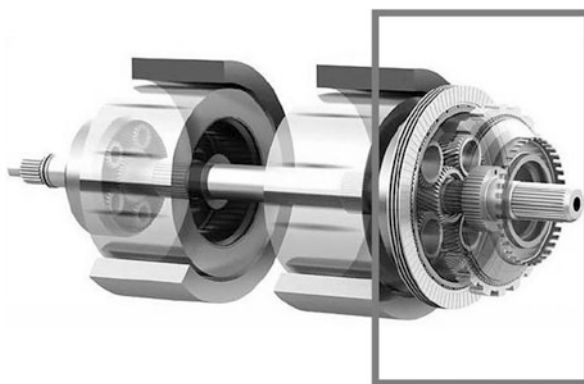
Fig. 5.46 Main components of the electrically supported, continuously variable gear with two-stage gear
