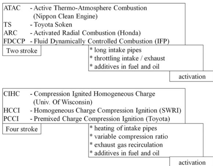
Fig. 2.64 Controlled self-ignition: most frequent methods
