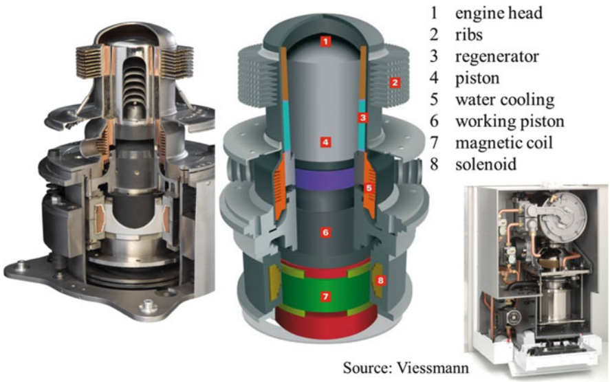
Fig. 2.98 Micro power station for heat and current (Viessmann) (Source: Viessmann)
