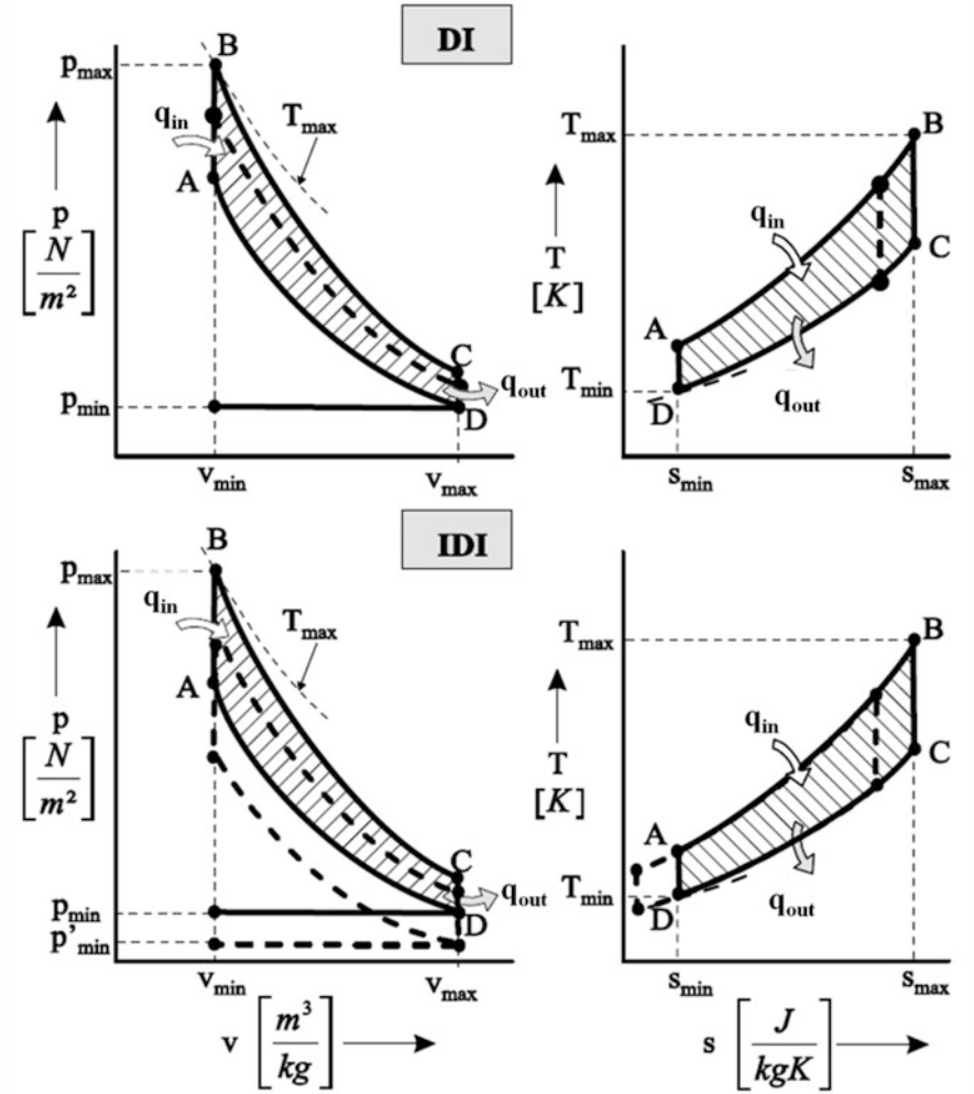
Fig. 2.3 Otto cycle
