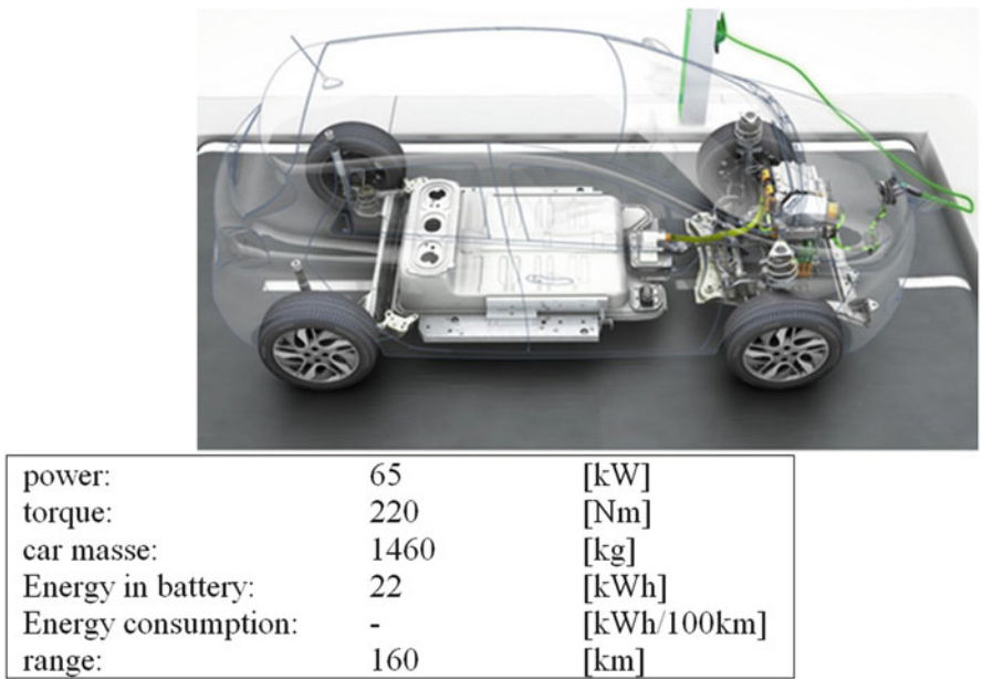
Fig. 4.36 Electric car: Renault Zoe (Source: Renault)
