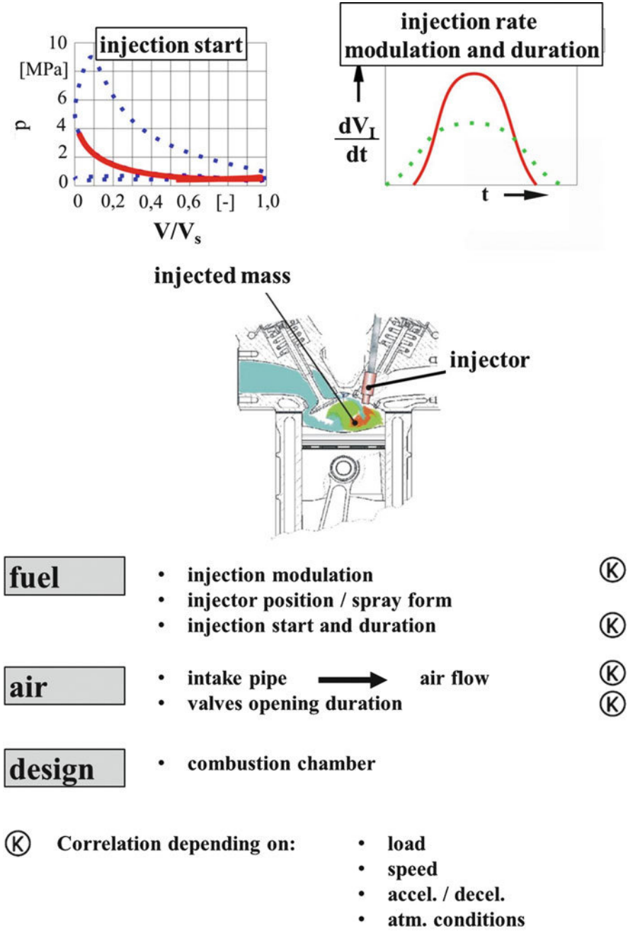
Fig. 2.58 Correlation of parameters for optimization of internal mixture formation in a CI engine
