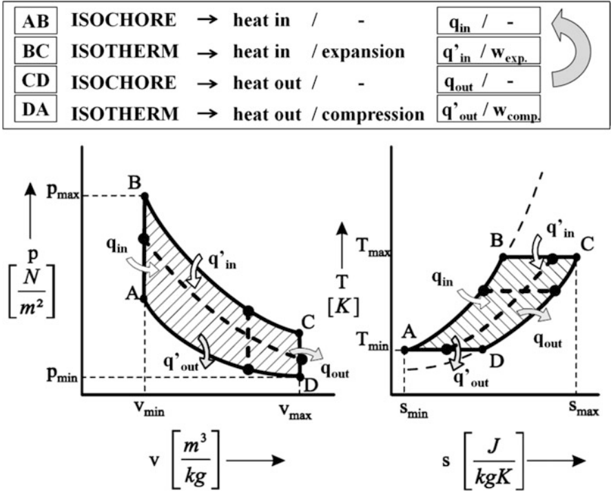
Fig. 2.2 Stirling cycle
