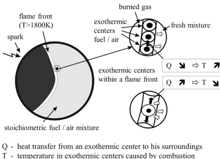
Fig. 2.65 Flame propagation into an isotropic, stoichiometric fuel–air mixture
