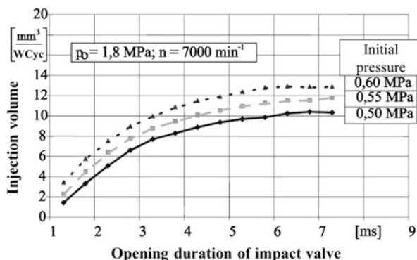
Fig. 5.14 Injection volume as a function of the opening duration of the impact valve and the initial pressure in a direct injection system with high-pressure modulation
