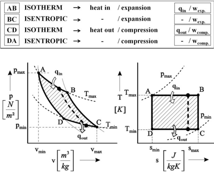
Fig. 2.1 Carnot cycle
