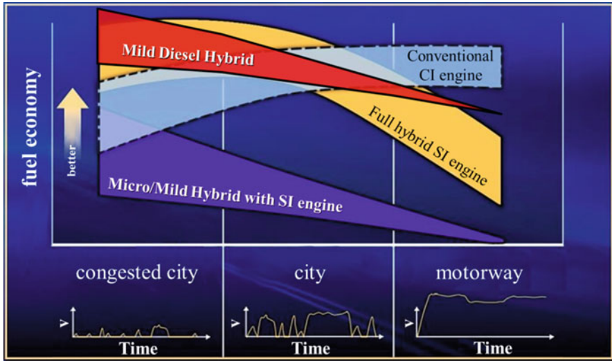
Fig. 5.25 Influence of driving cycle on fuel economy when using micro-, mild and full hybrids, in comparison with a conventional diesel engine
