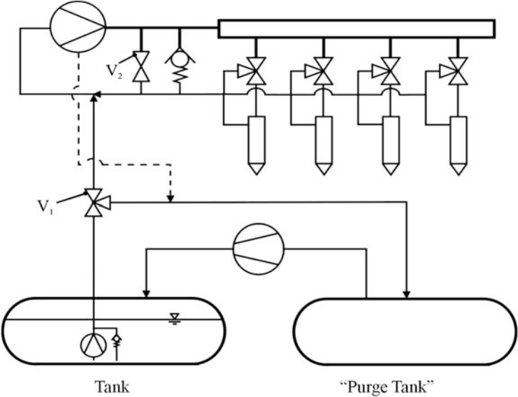
Fig. 3.41 Direct injection system for liquefied gases
