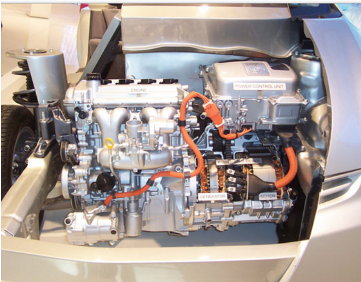
Fig. 5.33 Toyota Prius HSD (Hybrid Synergy Drive)
