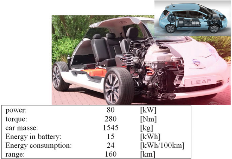
Fig. 4.34 Electric car: Nissan Leaf (Source: Nissan)
