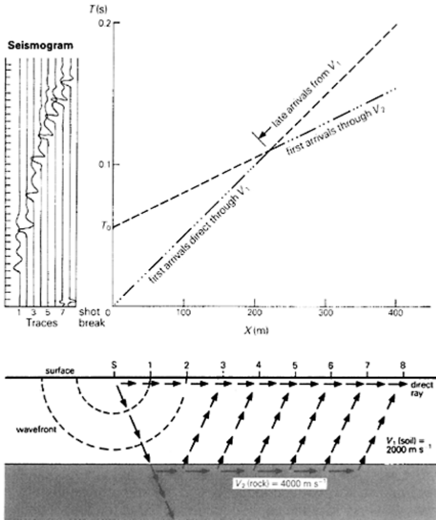
Figure 6.9 An explosive charge, fired at the shot point S , generates body and surface waves which propagate in all directions from S . Only the rays and wavefronts of the longitudinal ( P ) waves are represented, since with their higher velocity relative to the other types of wave they arrive first at the detectors laid out along the spread (traverse) being surveyed. The times of first arrivals (see text) at detectors 1 to 8 can be read from the corresponding trace on the seismogram. The first seismic pulse at each detector produces a sudden sharp deflection of the trace. The time can be read from timer lines on the seismogram, numbered relative to zero time at the shot break. The corresponding time-distance ( T - X ) graph is a plot of these first-arrival times against
