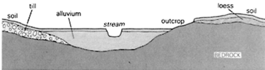
Figure 3.2 Thin (<1 m) soils developed on top of transported deposits, which include alluvium, glacial drift or till, and wind-deposited loess. Bedrock crops out on hillside. Even in this situation, residual deposits could be found occurring immediately above the bedrock and below the transported deposits.
