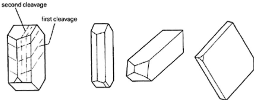
Figure 2.9 Various types of feldspar crystal, showing the two feldspar cleavages.
