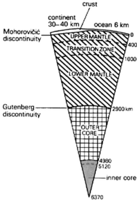
Figure 4.29 Layers of the Earth and major discontinuities.
