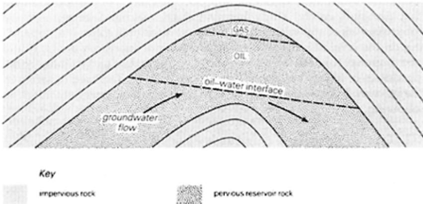
Figure 5.13 A thick pervious layer (the reservoir rock) and an overlying impervious layer (the roof rock) has been folded to form an anticline. This has trapped petroleum which has moved through the reservoir rock under the action of buoyancy and the hydraulic gradient, but cannot move further under the same forces. The less dense gas fraction has risen to the top, and the oil is concentrated below it. The voids in the rock below the oil/water interface are filled with groundwater, which is flowing from left to right. The hydraulic gradient which produces this flow has also caused a tilt of the gas/oil and the oil/water interfaces in the direction of flow. If there were no flow the interfaces would be horizontal.
