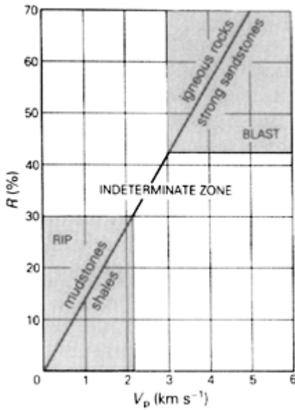
Figure 7.4 Laboratory-determined seismic velocity ( V_p ) plotted against in situ rebound number ( R ) for various rock types.
