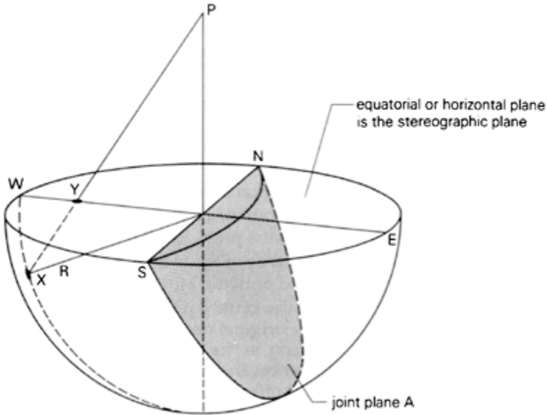
Figure H.3 Polar projection (Y), of pole (R) to joint plane (A) (see exact location of Y on Fig. H.4).
