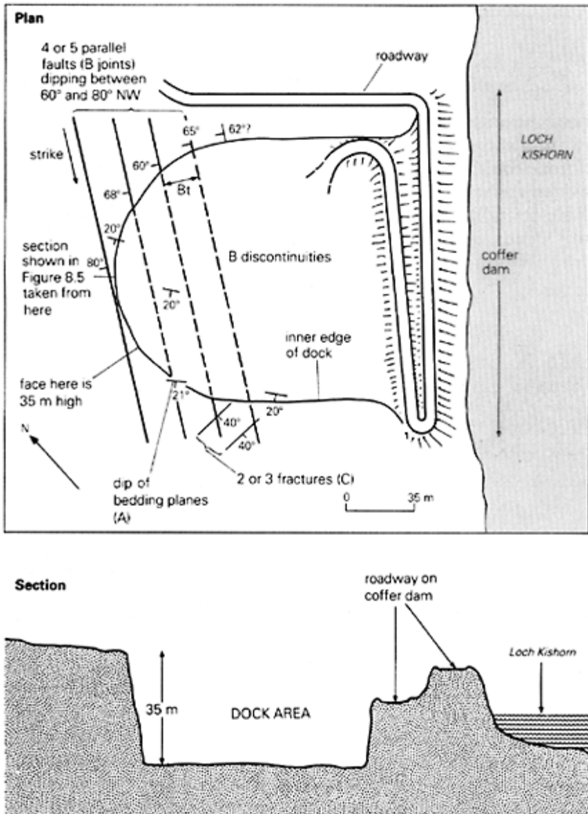
Figure 8.6 Plan and section of the Kishorn Dock excavation showing the main discontinuities, and also the bedding planes of the rocks.
