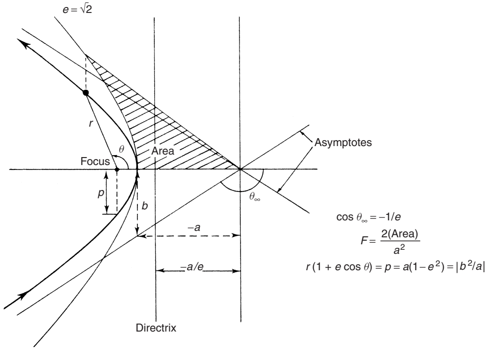
Figure 4.8 Hyperbola ( e > 1 )
