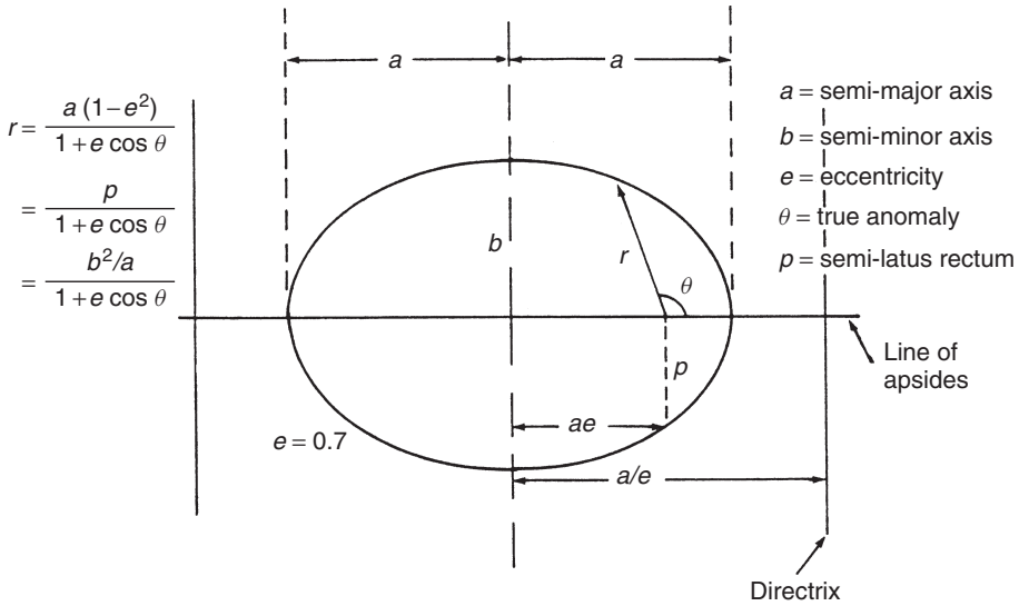
Figure 4.5 Ellipses
