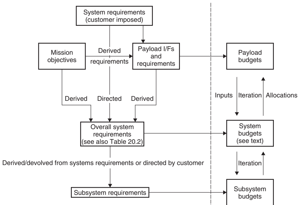
Figure 20.3 Expansion/translation of top-level requirements to system and subsystem level
