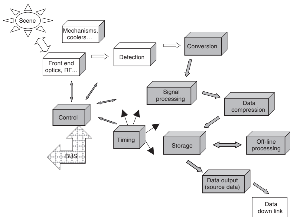
Figure 13.7 Generalized instrument
