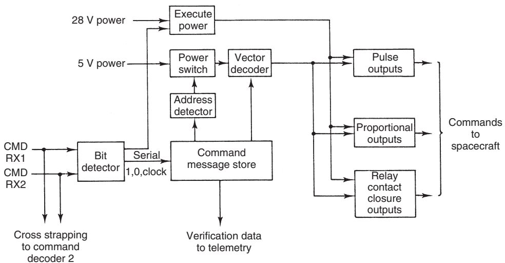
Figure 13.4 Telecommand decoder
