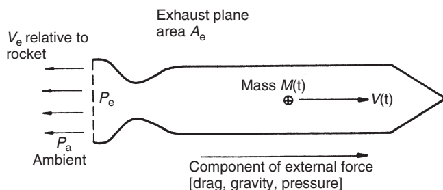
Figure 6.3 Schematic rocket
