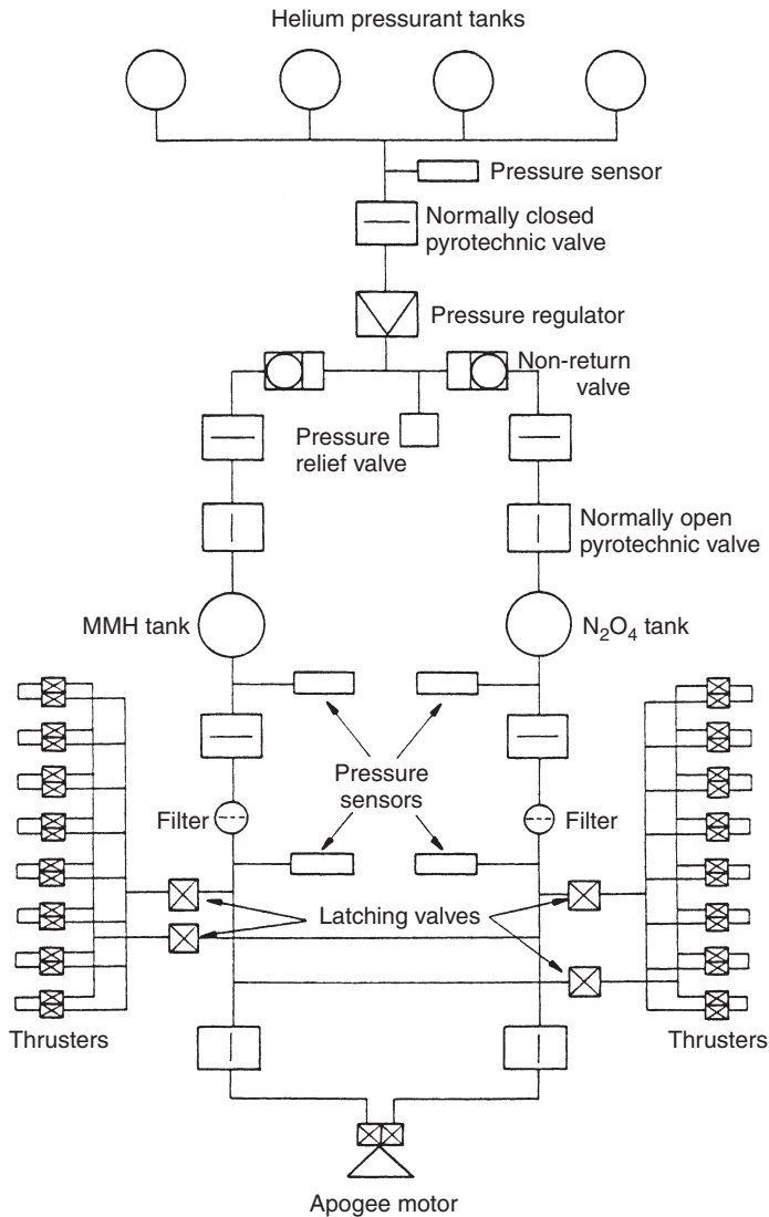
Figure 6.21 Schematic of a typical bi-propellant propulsion system
