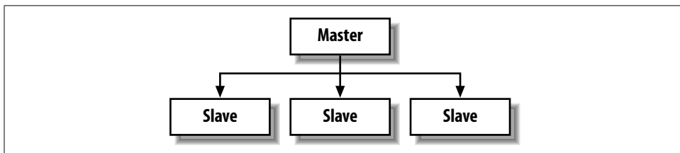
Figure 13-4. Database replication
