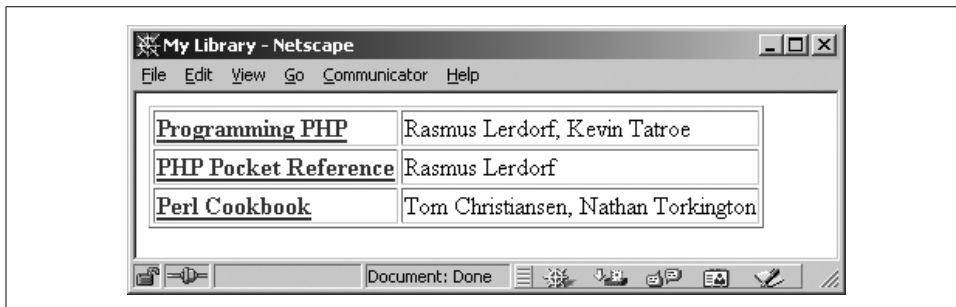
Figure 11-1. Book menu
