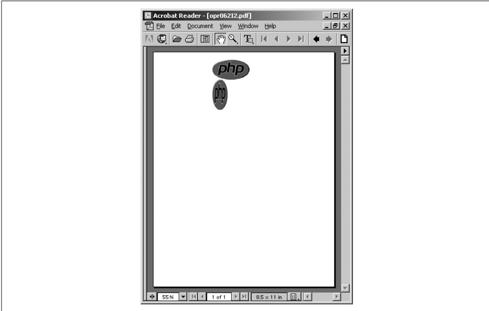
Figure 10-8. Nonproportional scaling
