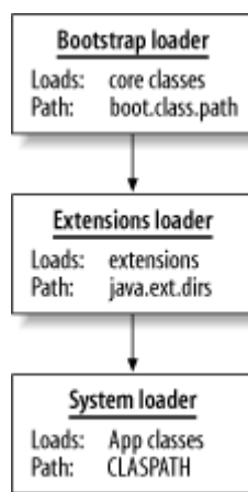
Figure 6-6. The Java 2 class loader has three major loaders
