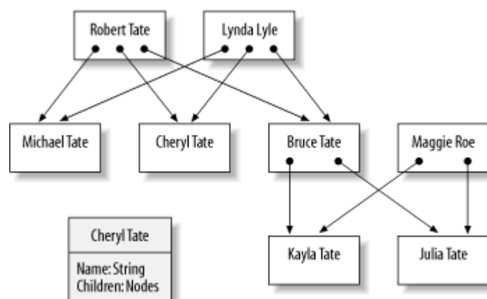
Figure 1-3. A simple node class, a string, and a collection form the foundation of a family tree
