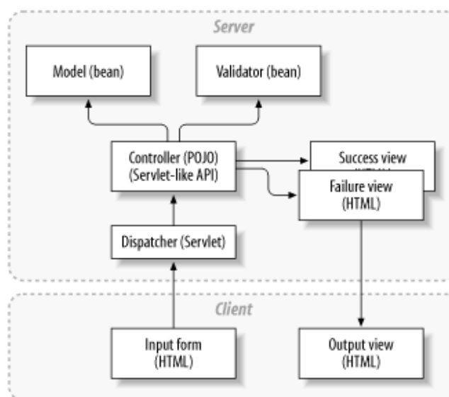
Figure 8-4. The MVC Web framework works much like Struts
