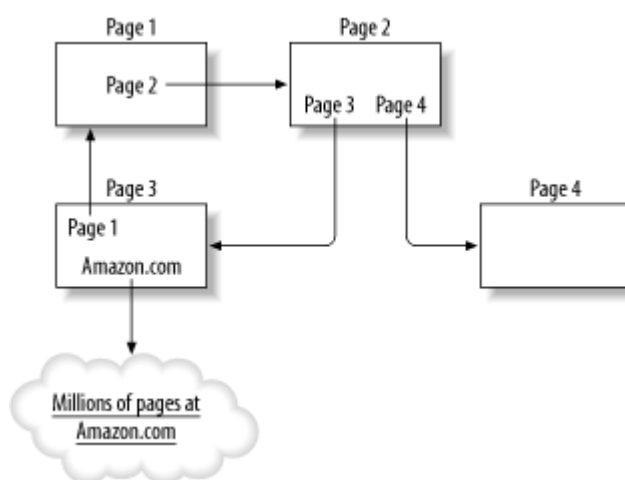
Figure 9-1. A simple, four-page web site that breaks any naïve crawler
