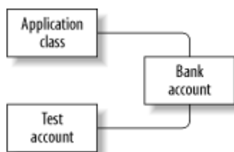
Figure 2-6. Testing improves the design of your application by reducing coupling
