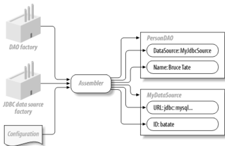
Figure 6-8. Lightweight inversion of control containers relieve applications of creation and assembly of objects.
