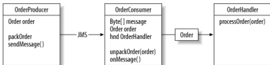
Figure 2-7. Testability improves a design with only a single producer and consumer to a design that breaks out an order and handler
