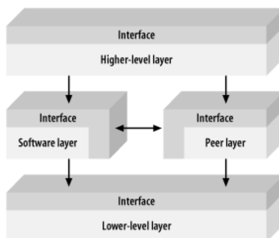
Figure 3-3. A typical intermediate software layer has layers above and below
