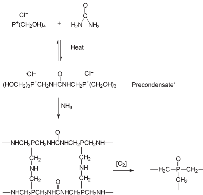
8.13 THPC-urea-ammonia reaction.
