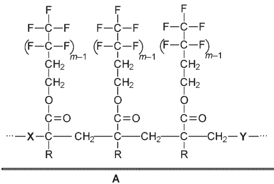
6.9 Fluorocarbon repellent on fibre surface. m = 8-10 . X and Y are comonomers, mainly stearylacrylates. R = H or CH_3 (polyacrylic or polymethacrylic acid esters). A is the fibre surface.
