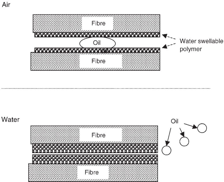
7.5 Mechanism of soil release with acrylic copolymers.
