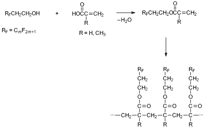
6.7 Preparation of perfluoro containing acrylic polymers.
