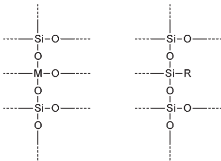
18.2 Schematic representation of the chemical modifications of the silicon oxide network. Inorganic modification with M = Al, Ti, Zr and others, organic modification with R = alkyl, aryl, both without and with additional functional groups, for example fluoroalkyl, or R = bioactive or dyestuff group.
