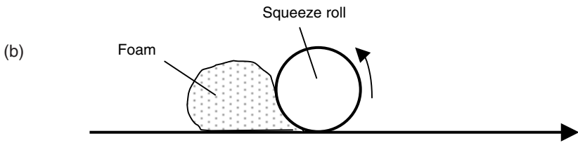
Roller coater
