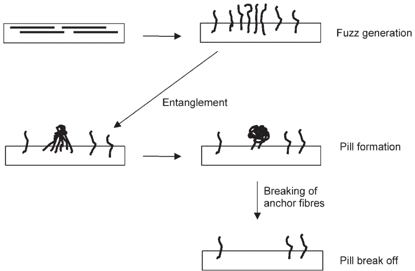
11.1 Pilling mechanism.
