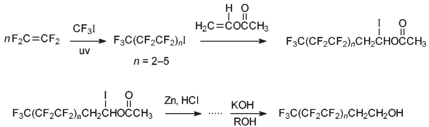
6.8 Telomerisation process for preparing fluoroalkyls.
