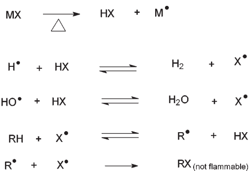
8.8 Competing free radical reactions during combustion of halogen (X)-containing material (M). R is the organic residue.
