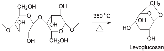
8.7 Thermal degradation of cellulose.
