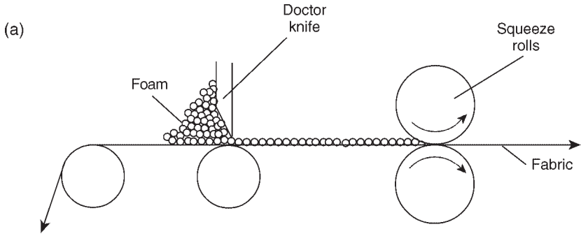
Doctor blade coater
