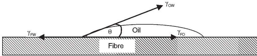
7.3 Fibre-oil-water interface.
