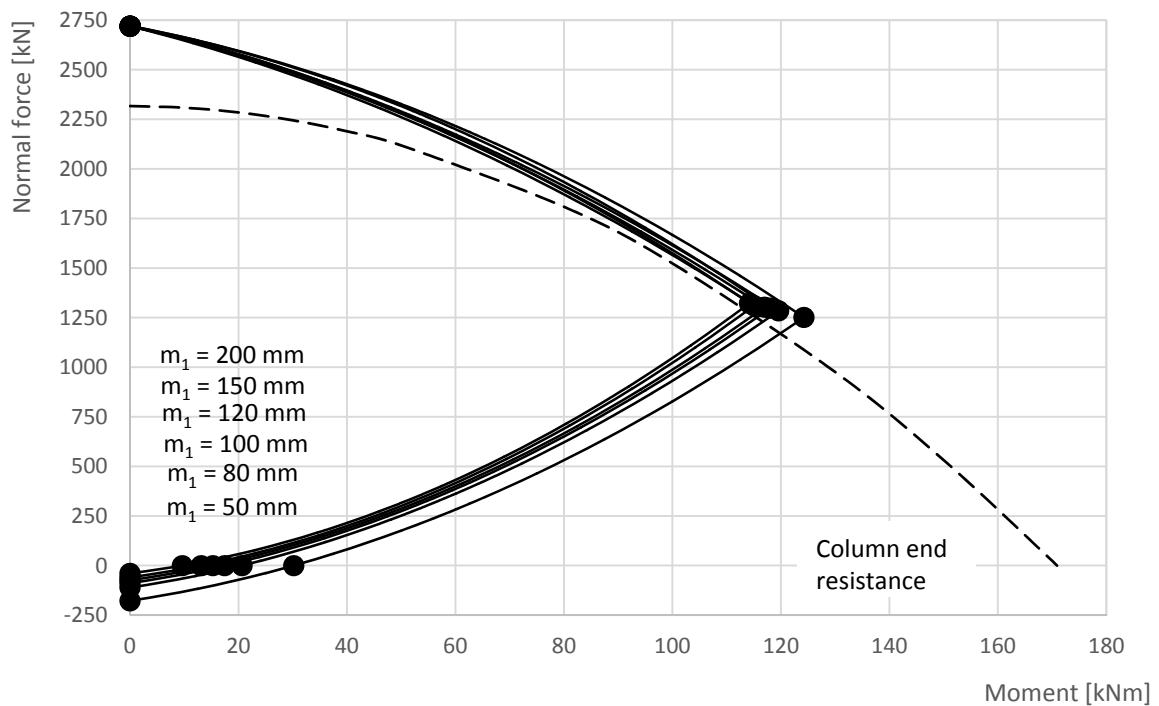
Fig. 4.39: Moment - normal force interaction diagram for different distances between the headed and threaded studs m_1 , for the anchor plate steel S355
