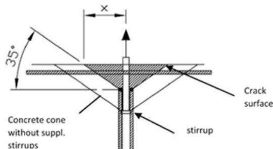
Fig. 2.6: Definition of distance x
