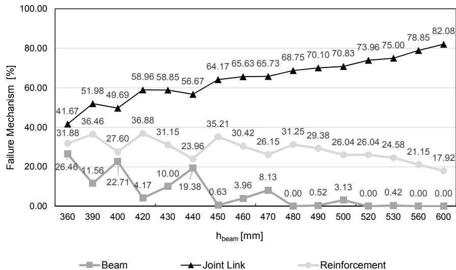
Fig. 4.53: Influence of total height
