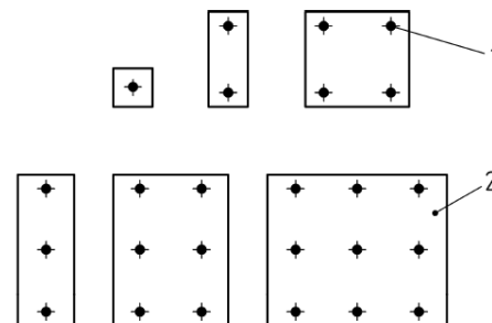
Fig. 4.23: Number of headed studs according to CEN/TS 1992-4-1 [1]
