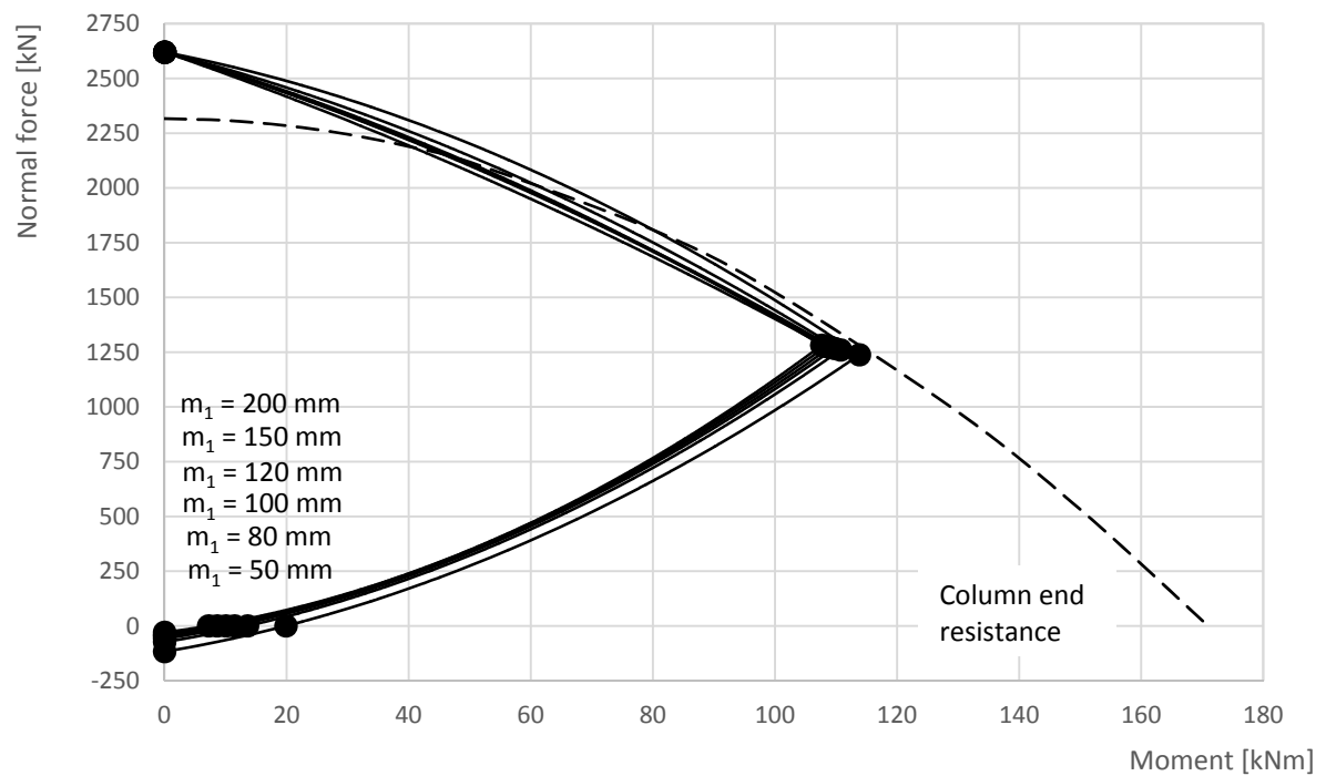
Fig. 4.40: Moment – normal force interaction diagram for different distances between the headed and threaded studs m_1 , for the anchor plate steel S235
