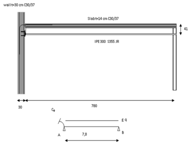
Fig. 3.1: Structural system
