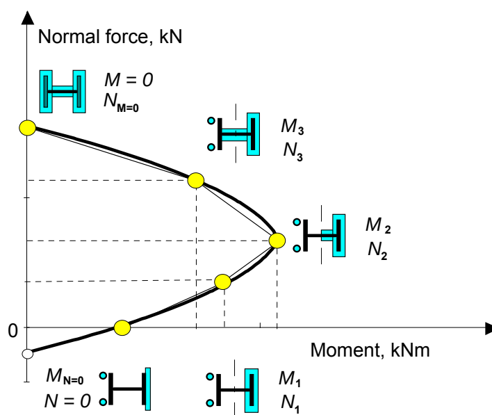
Fig. 4.44: Tabulated points at the moment –normal force interaction diagram in Tab. 4.10. to Tab. 4.15
