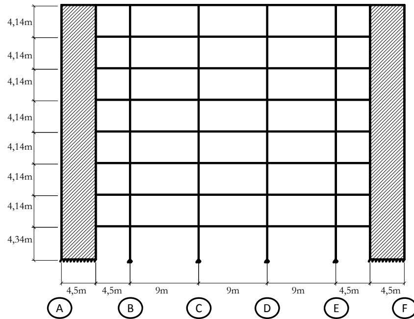
Fig. 7.6b Geometry of sub-structure II, Office building alignment 3
