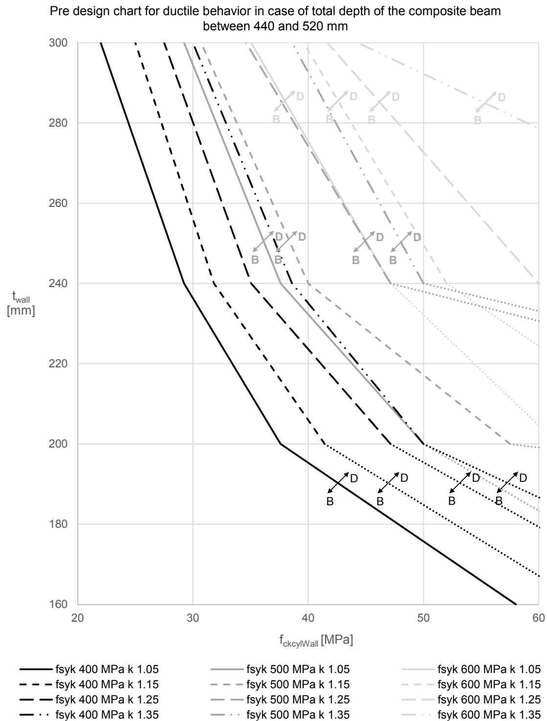
Fig. 4.60: Pre design chart for ductile behaviour in case of total depth of the composite beam between 440 and 520 mm
