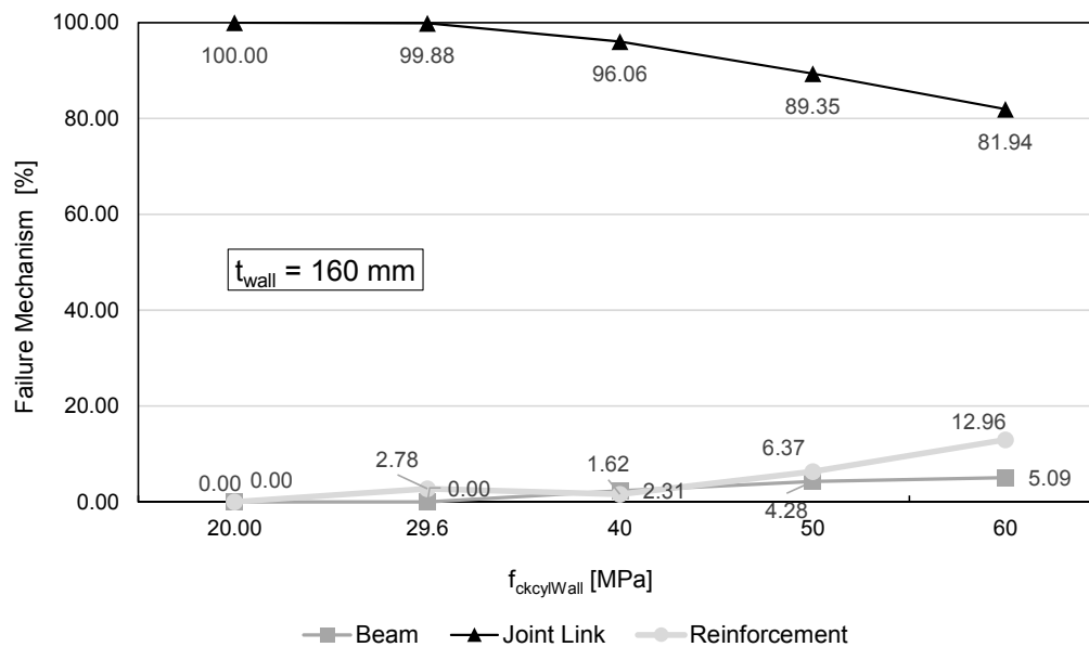
Fig. 4.55: Influence of wall concrete grade for t_{\text{wall}} = 160 mm
