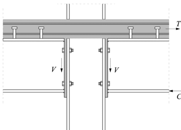
Fig. 2.8 Composite joint
