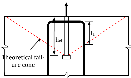
Fig. 4.4: Definition of effective bond length, l_1 of stirrups and its dependence on the effective embedment depth, h_{ef}
