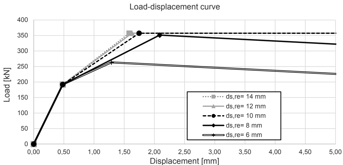
Fig. 4.19: Load-displacement curve for variation of the diameter of the supplementary reinforcement
