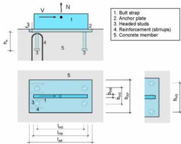
Fig. 2.20: Geometry of the joint with rigid anchor plate
