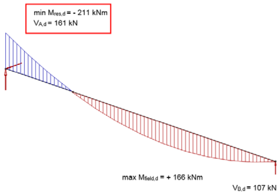
Fig. 3.8: Internal forces by taking into account the secant stiffness C_\varphi at the support A
