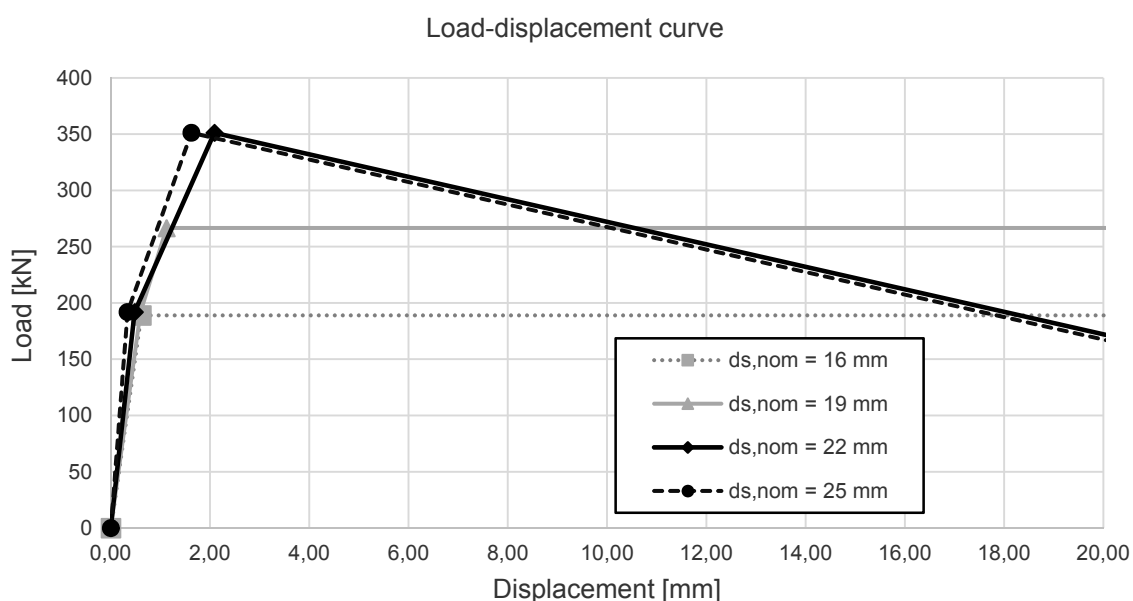
Fig. 4.16: Load-displacement curve of the tensional component for variation of the diameter of the headed studs
