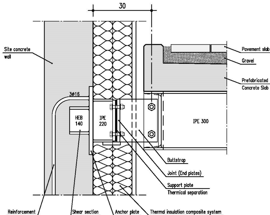
Fig. 3.18: Conventional joint solution of the balcony construction
