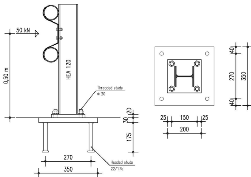
Fig. 3.10: Conventional joint solution of the safety fence
