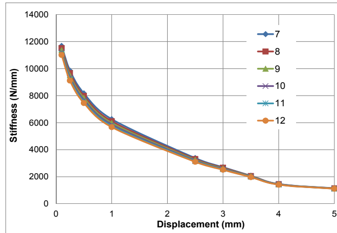
Fig. 4.7: Influence of pressing relation, m on stiffness of anchorage
