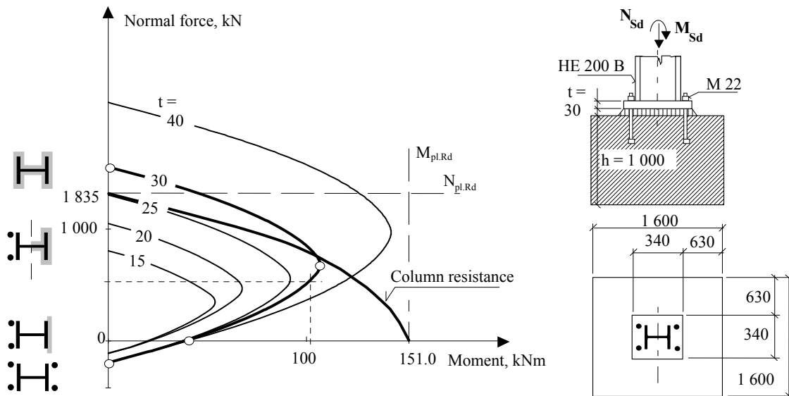
Fig. 9.155a The column base resistance is compared to the column resistance for different base plate thickness
