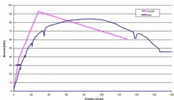
Moment-rotation-curve for test B2-C-R
