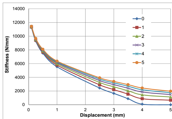
Fig. 4.8: Influence of design bond strength, f_{bd} on stiffness of anchorage
