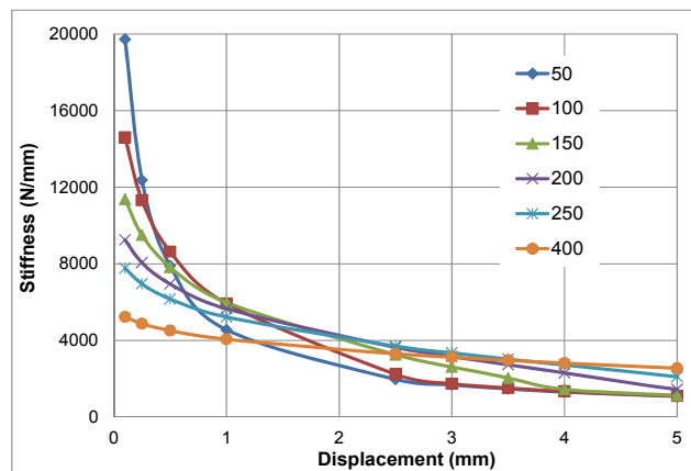
Fig. 4.5: Influence of effective embedment depth, h_{ef} on stiffness of anchorage
