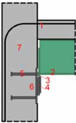
Fig. 2.5: Components for joints with negative bending moment
