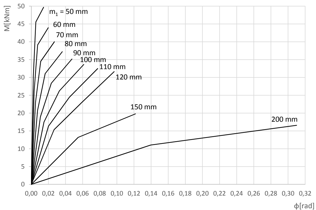
Fig. 4.41: Moment – rotation diagram for different distances between the headed and threaded studs m_1 , for the anchor plate steel S355
