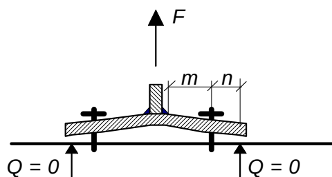
Fig. 4.4 T-stub separated from the concrete block with no prying force
