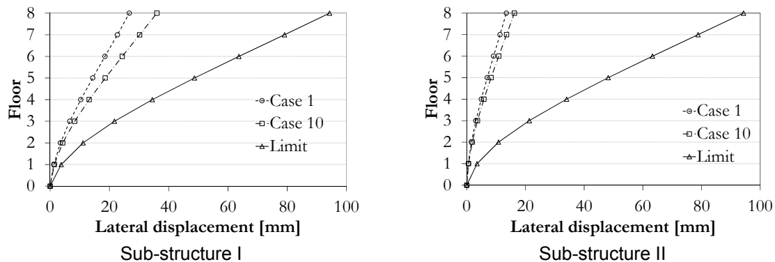
Fig. 7.11 Lateral displacements envelops
