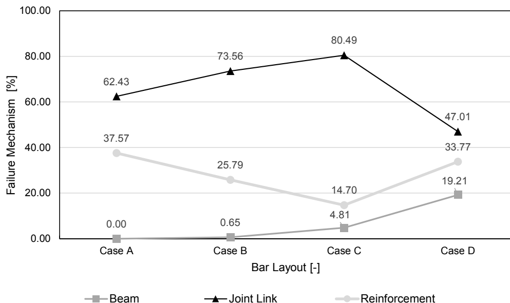
Fig. 4.46: Influence of rebar layout
