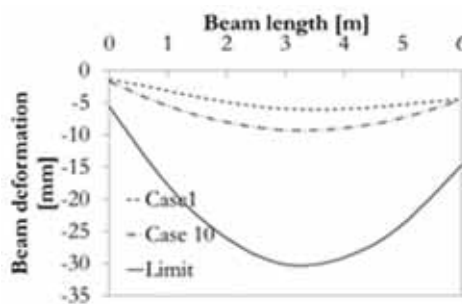
a) Sub-structure I
