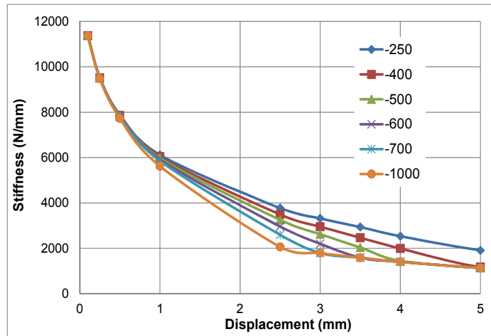
Fig. 4.3: Influence of parameter, \alpha_c on stiffness of anchorage
