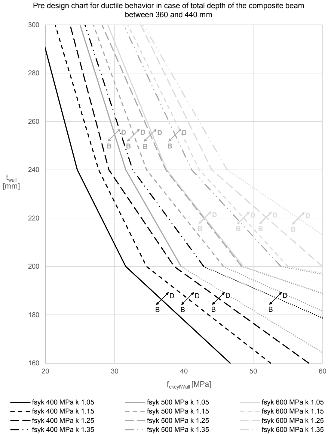
Fig. 4.59: Pre design chart for ductile behaviour in case of total depth of the composite beam between 360 and 440 mm
