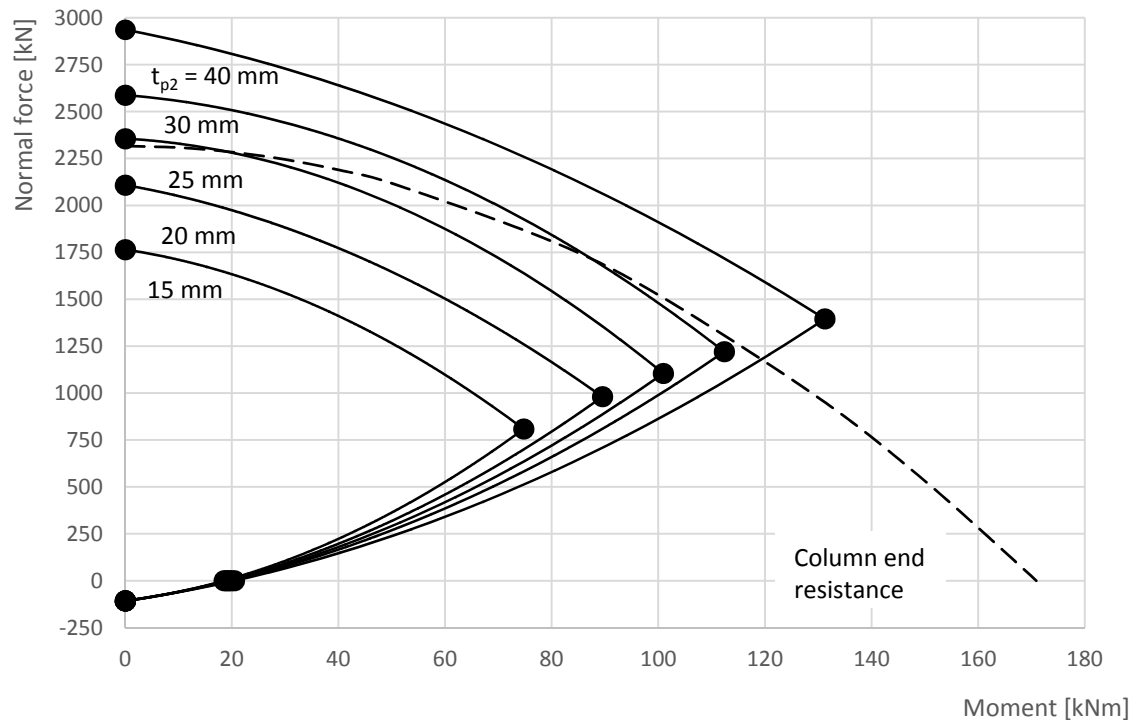
Fig. 4.32: Moment - normal force interaction diagram for different base plate thickness t_{p2} and steel S235
