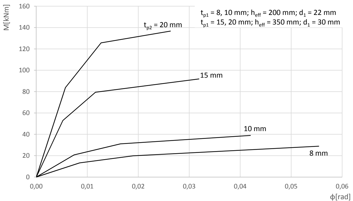
Fig. 4.35: Moment - rotation diagram for different anchor plate thickness t_{p1} , for the anchor plate steel S355, and the headed stud lengths h_{\text{eff}} = 200 \text{ mm} and 350 \text{ mm}
