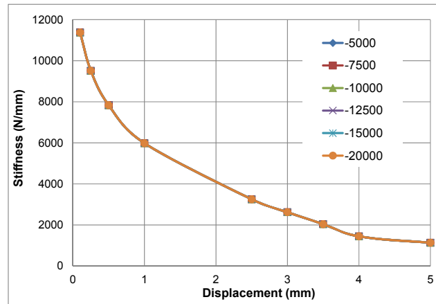
Fig. 4.10: Influence of descending anchor stiffness due to concrete, k_{c,de} on stiffness of anchorage
