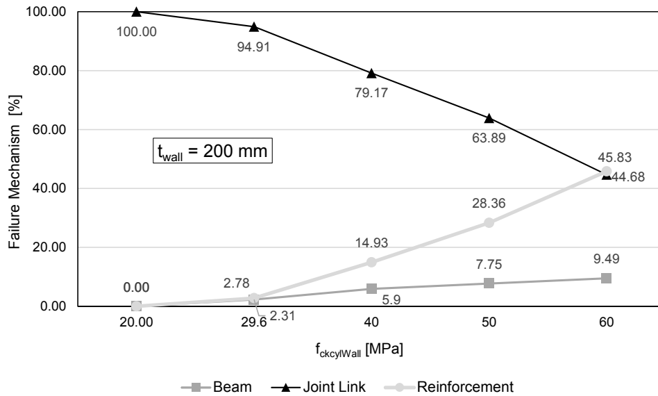
Fig. 4.56: Influence of wall concrete grade for t_{wall} = 200 mm
