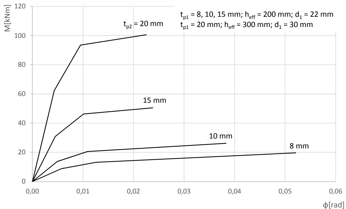
Fig. 4.36: Moment – rotation interaction diagram for different anchor plate thickness t_{p1} , for the anchor plate steel S235, and the headed stud lengths h_{eff} = 200 mm and 300 mm
