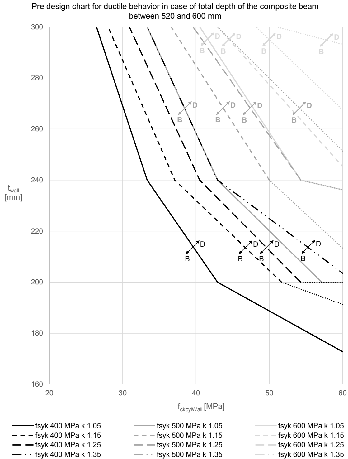
Fig. 4.61: Pre design chart for ductile behaviour in case of total depth of the composite beam between 520 and 600 mm
