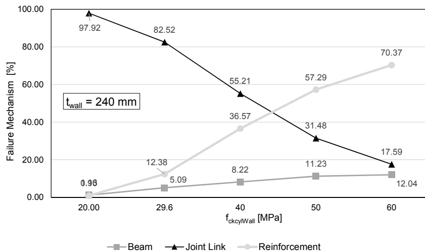
Fig. 4.57: Influence of wall concrete grade for t_{wall} = 240 mm
