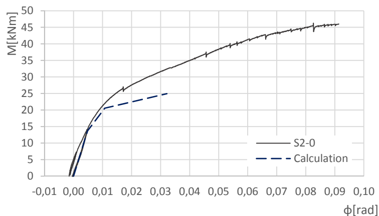
Fig. 4.28: Comparison of predicted and measured moment rotational relation for experiment S2-0, eccentricity 495 mm
