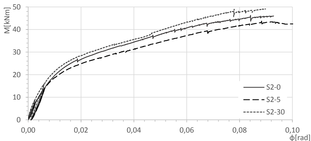
Fig. 4.26: Moment-rotation curves of three experiments with different position of headed and threaded studs
