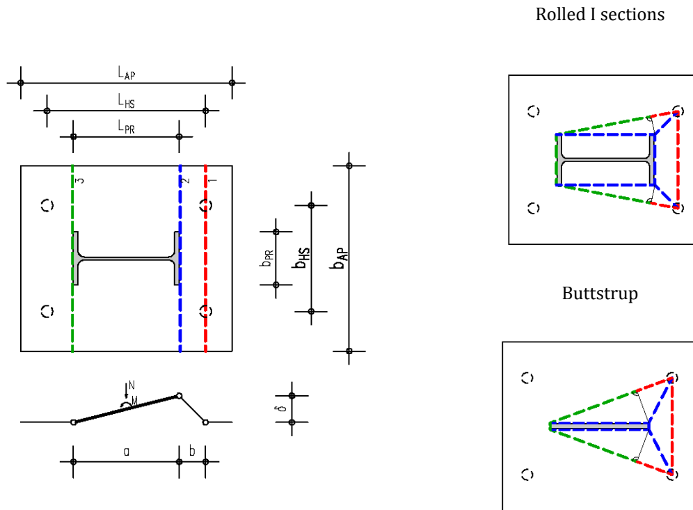
Fig. 2.12: Static model of the anchor plate yielding lines with yielding lines over the whole width
