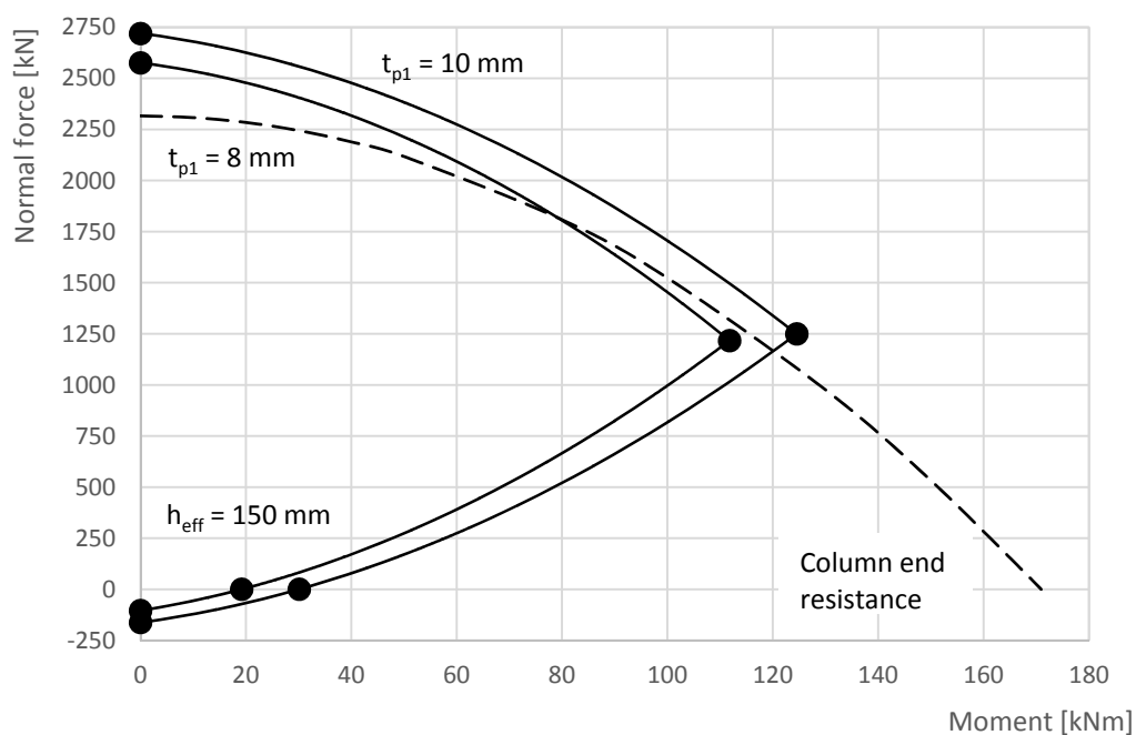
Fig. 4.33: Moment - normal force interaction diagram for different anchor plate thickness t_{p1} , for the anchor plate steel S355, and the headed stud length h_{eff} = 150 mm
