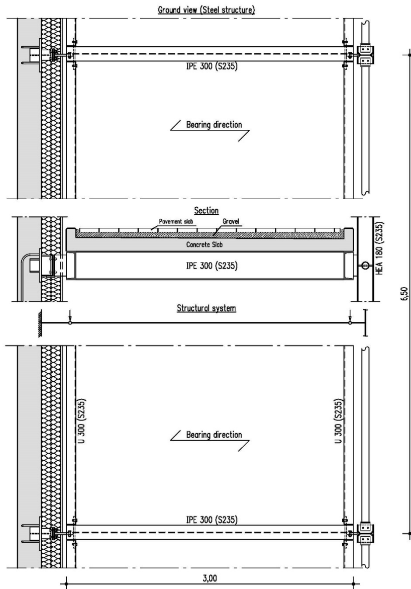
Fig. 3.17: Conventional solution and structural system
