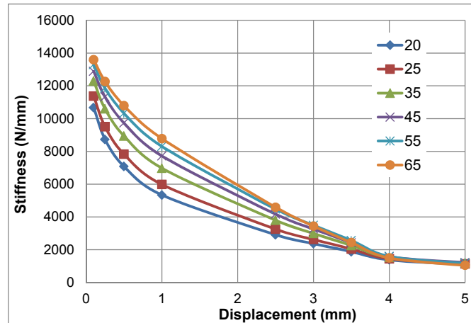
Fig. 4.2: Influence of Concrete Strength, f_{ck} on stiffness of anchorage with supplementary reinforcement
