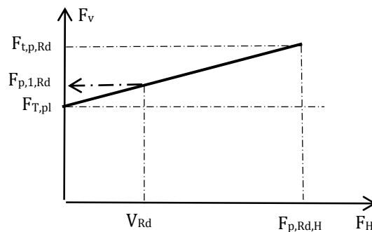
Fig. 9.22 Acting vertical F_v and horizontal F_H forces to the anchor plate
