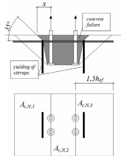
Fig. 4.24: Design approach for more than one headed stud under tension
