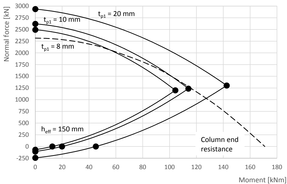
Fig. 4.34: Moment - normal force interaction diagram for different anchor plate thickness t_{p1} , for the anchor plate steel S235, and the headed stud length h_{\text{eff}} = 150 \text{ mm}
