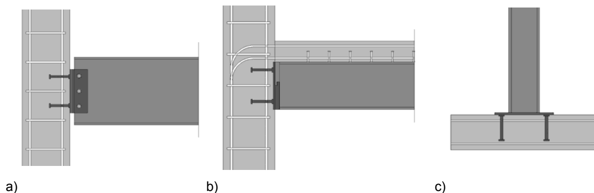
Fig. 1.1 Examples for steel-to-concrete joints, a) simple joint, b) composite joint, c) column bases
