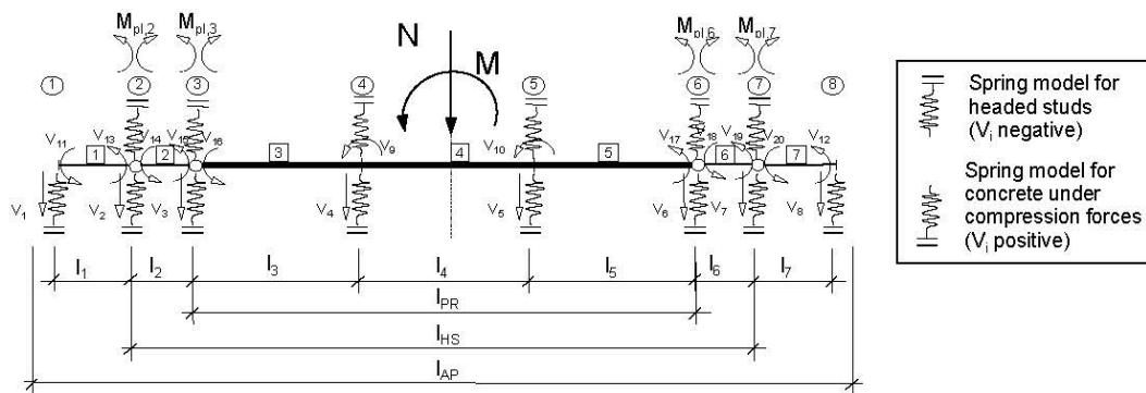
Fig. 2.9: Design model for vertical loads and bending moments
