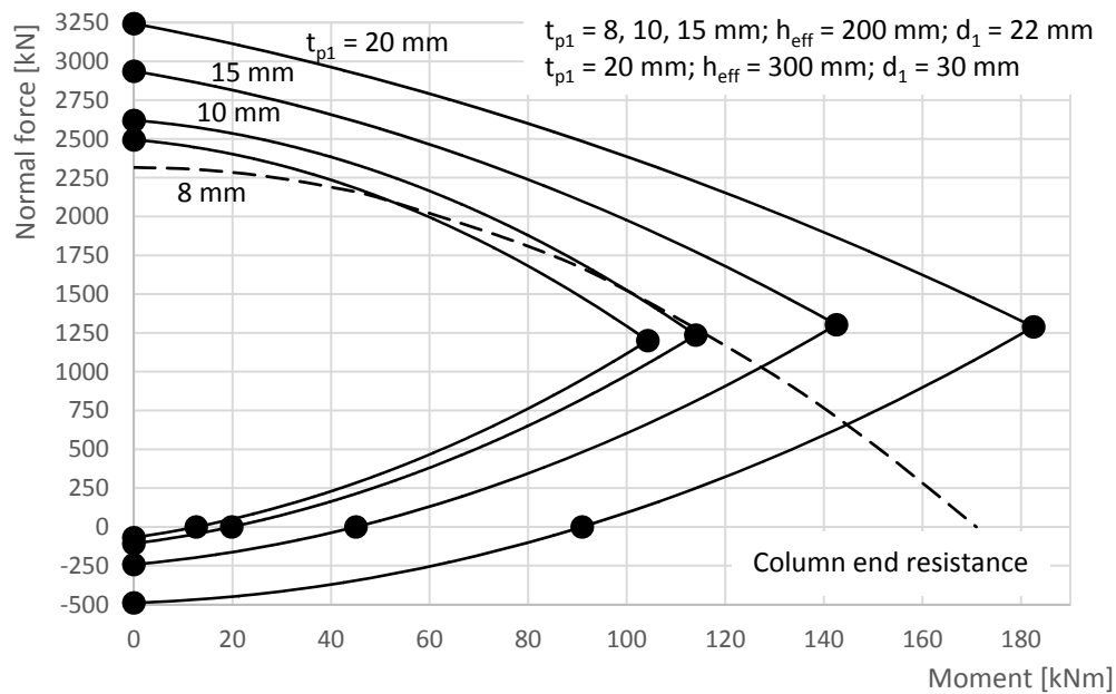
Fig. 4.38: Moment - normal force interaction diagram for different anchor plate thickness t_{p1} , for the anchor plate steel S235, and the headed stud lengths h_{eff} = 200 mm and 300 mm
