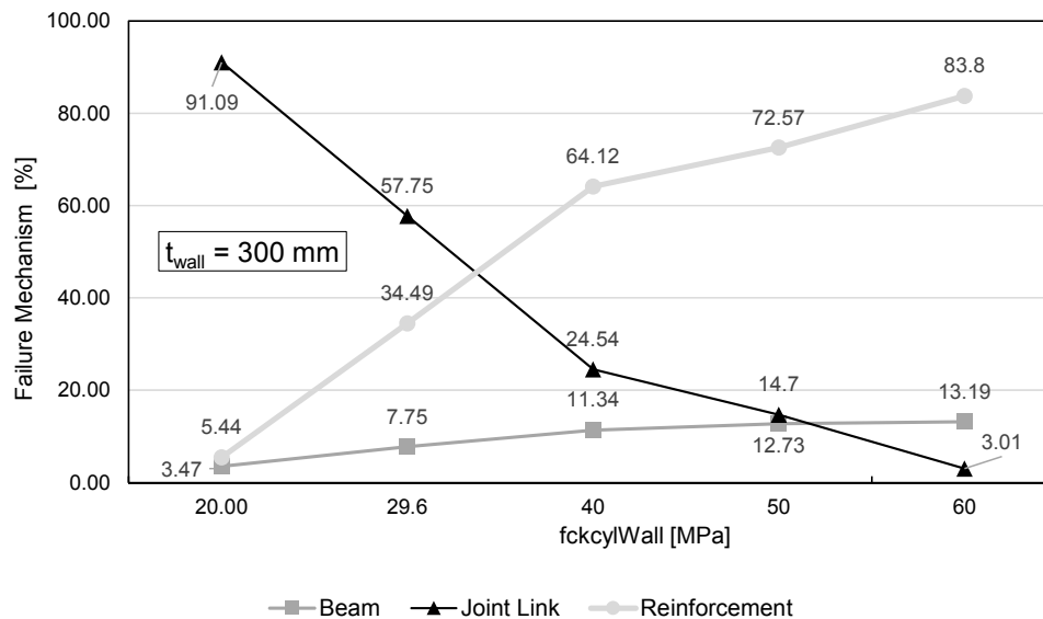
Fig. 4.58: Influence of wall concrete grade for t_{wall} = 300 mm
