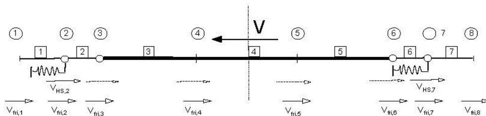
Fig. 2.11: Design model for horizontal (shear) loads
