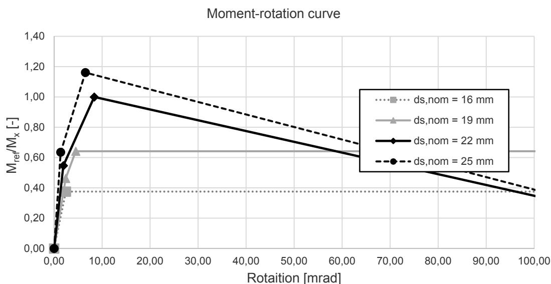
Fig. 4.17: Moment-rotation curve of the simple steel-to-concrete joint for variation of the diameter of the headed studs
