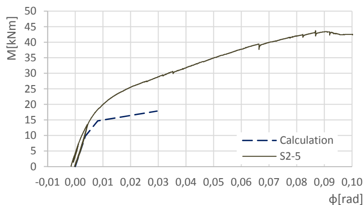
Fig. 4.29: Comparison of predicted and measured moment rotational relation for experiment S2-5, eccentricity 354 mm
