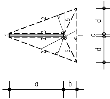
Fig. 2.14: Geometry for local rotating yielding lines
