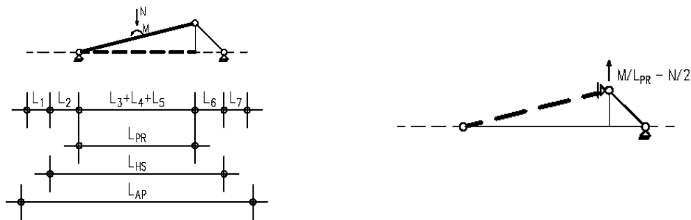
Fig. 2.10: Model of the baseplate under tension and simplified calculation model
