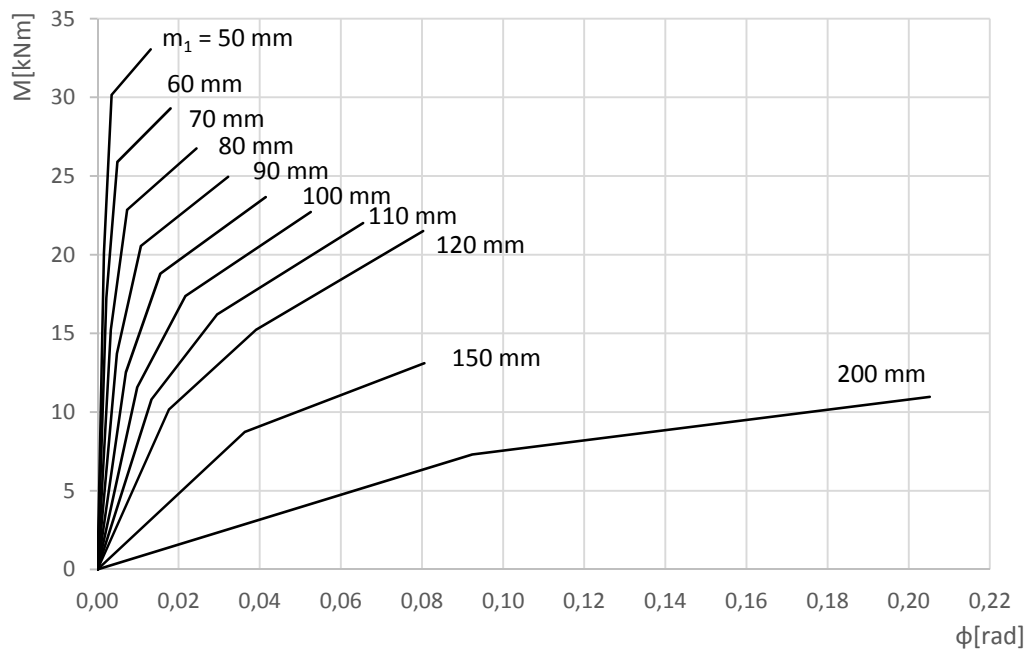
Fig. 4.42: Moment – rotation diagram for different distances between the headed and threaded studs m_1 , for the anchor plate steel S235
