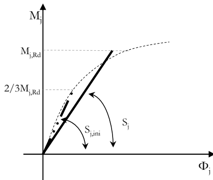
Fig. 7.2a Linear elastic M- \Phi curve idealized for the joint behaviour
