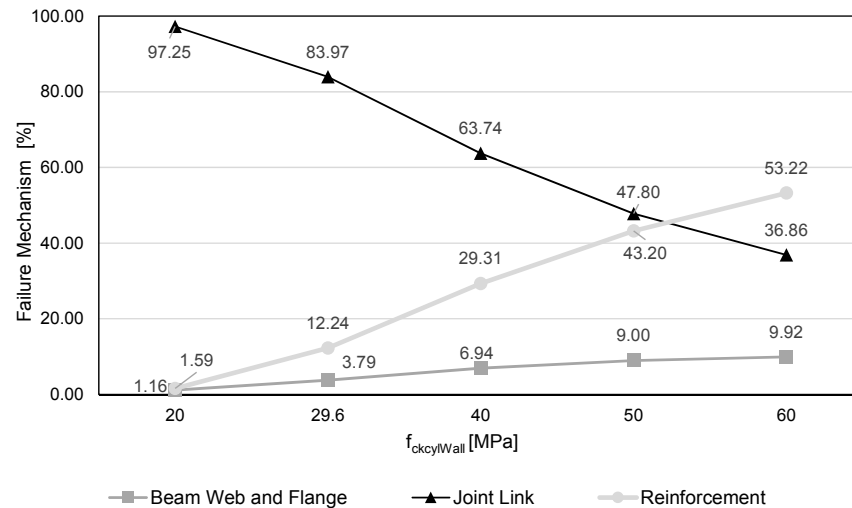
Fig. 4.54: Influence of wall concrete grade
