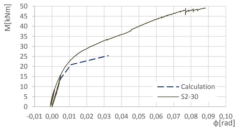
Fig. 4.30: Comparison of predicted and measured moment rotational relation for experiment S2-30, eccentricity 504 mm
