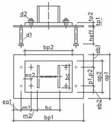
Fig. 4.43: Scheme of base plate with anchor plate
