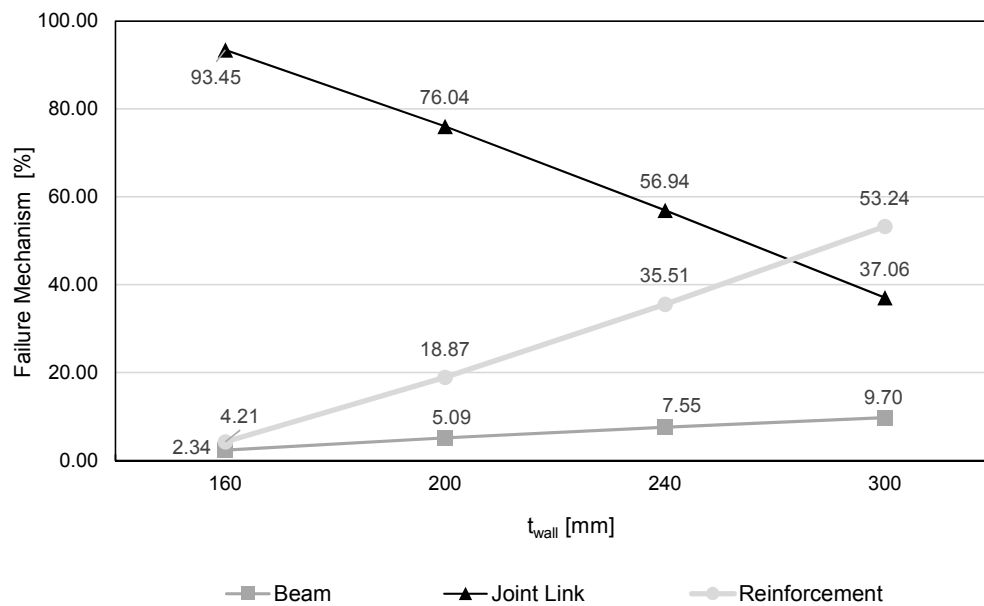
Fig. 4.50: Influence of t_{wall}
