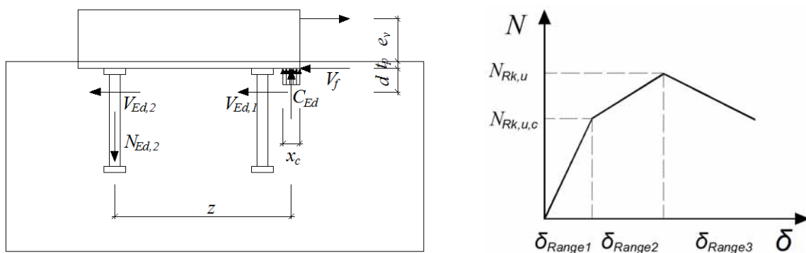
Fig. 4.11: Analytic model of the simple steel-to-concrete joint (left), load-deformation of the tensional component if supplementary reinforcement can be activated in best case (right)
