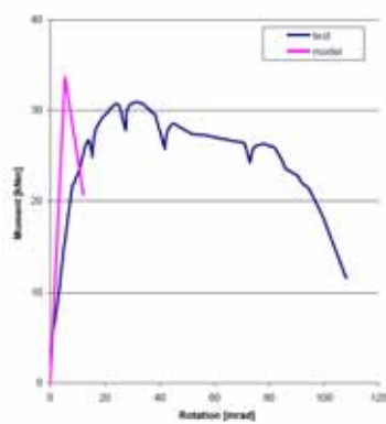
Moment-rotation-curve for test B1-BS
