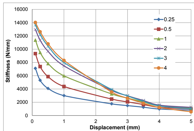
Fig. 4.6: Influence of shoulder width, a , on stiffness of anchorage
