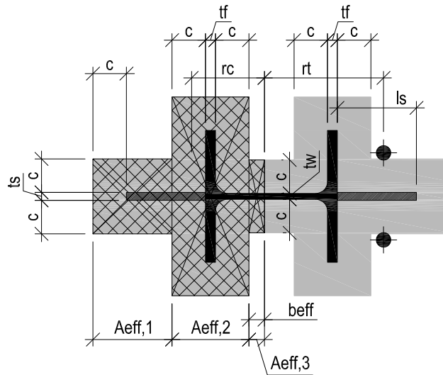
Fig. 9.18 The effective area under the base plate
