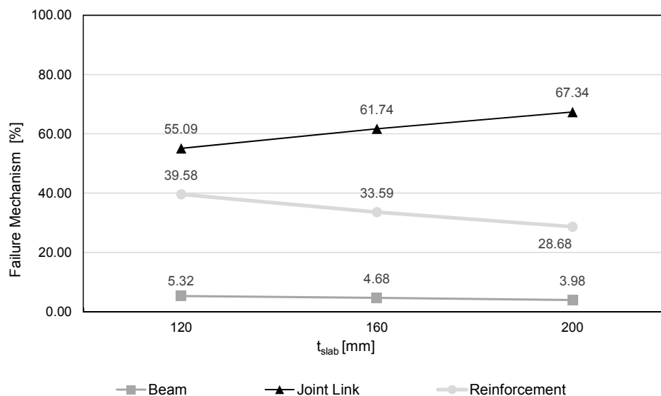
Fig. 4.51: Influence of t_{slab}
