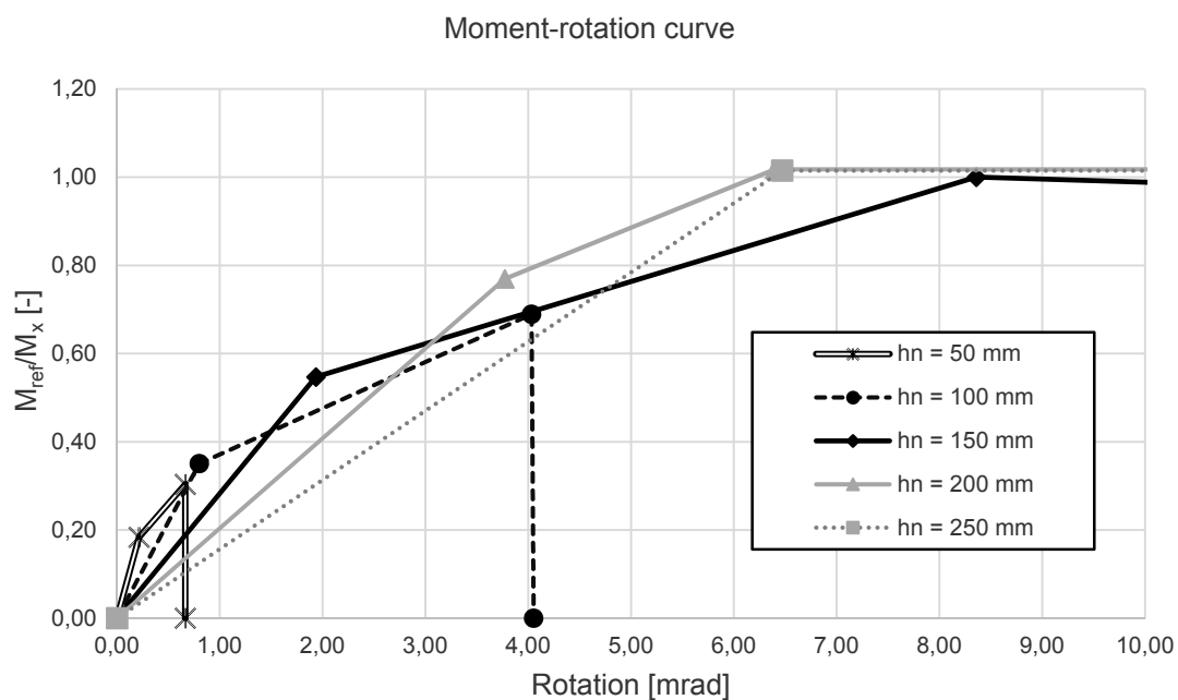
Fig. 4.15: Moment-rotation curve for variation of the effective height
