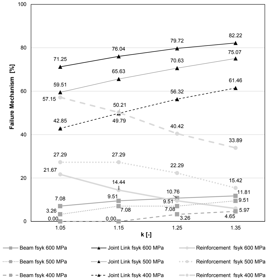
Fig. 4.49: Interaction between yield and ultimate strength
