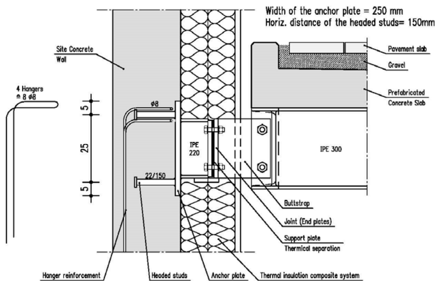
Fig. 3.19: Improved joint solution of the balcony construction
