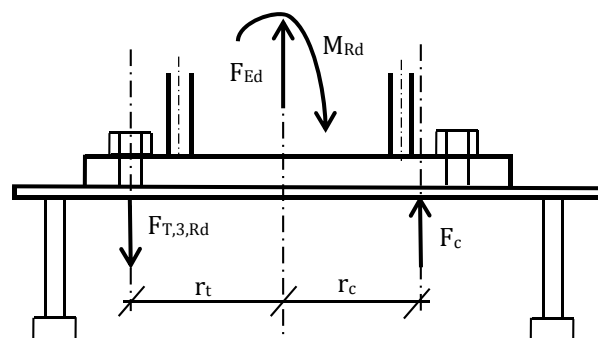
Fig. 9.23b The lever arm of concrete and threaded stud to the column axes
