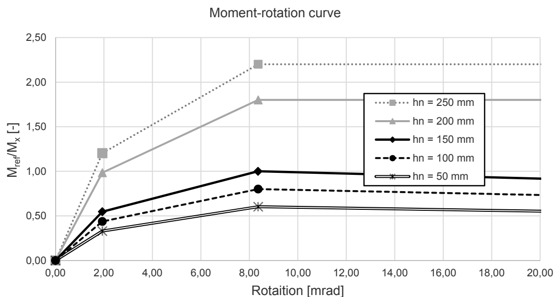
Fig. 4.18: Moment-rotation curve for variation of the eccentricity
