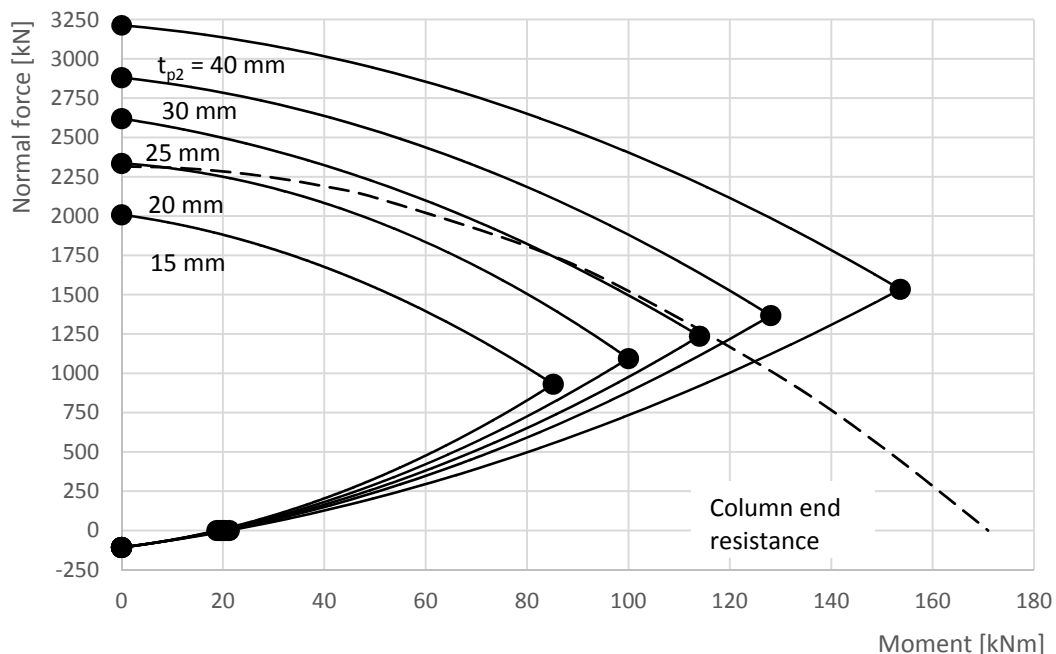
Fig. 4.31: Moment - normal force interaction diagram for different base plate thickness t_{p2} and steel S355
