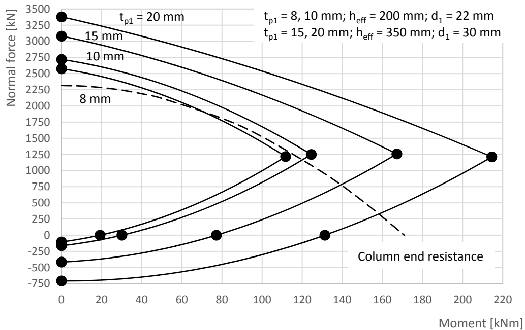
Fig. 4.37: Moment – normal force interaction diagram for different anchor plate thickness t_{p1} , for the anchor plate steel S355, and the headed stud lengths h_{eff} = 200 mm and 350 mm
