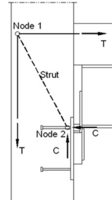
Fig. 2.7: Strut and tie model
