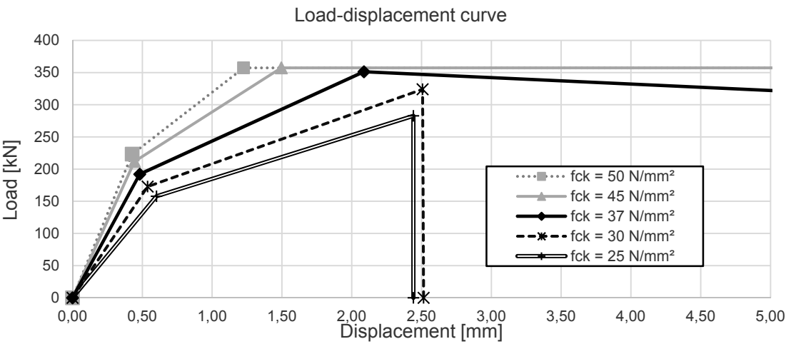
Fig. 4.21: Load-displacement curve for variation of the concrete strength
