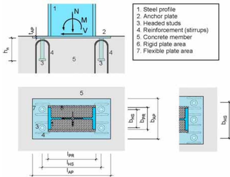
Fig. 2.8: Geometry of the joint with slim anchor plate
