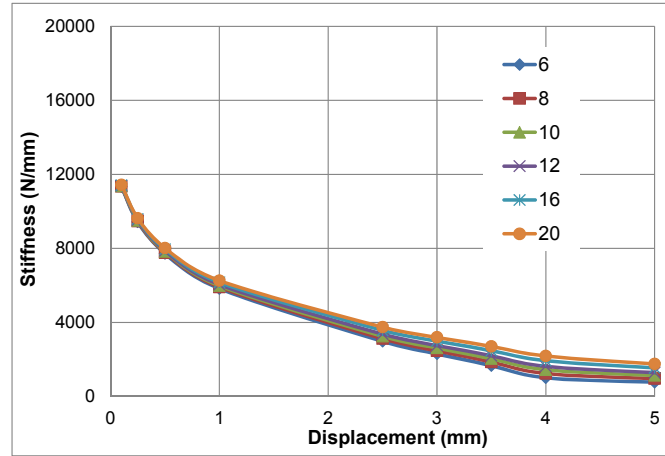
Fig. 4.9: Influence of diameter of supplementary reinforcement, d_{s,re} on stiffness of anchorage
