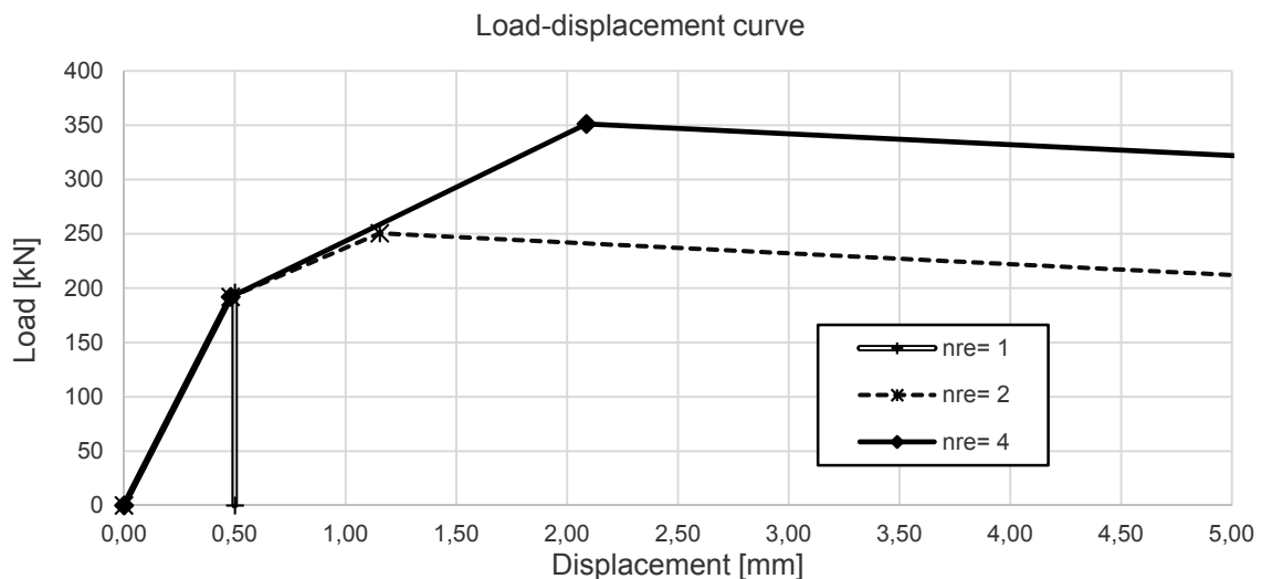
Fig. 4.20: Load-displacement curve for variation of the number of stirrups
