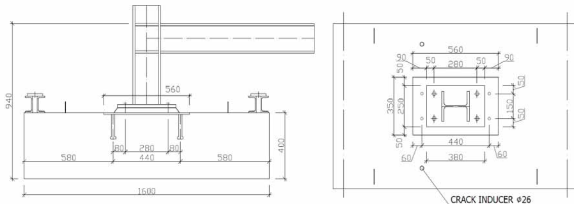
Fig. 4.25: Geometry of tests with column base with anchor plate
