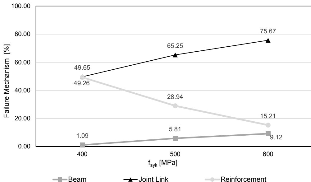
Fig. 4.47: Influence of yield strength of slab reinforcement
