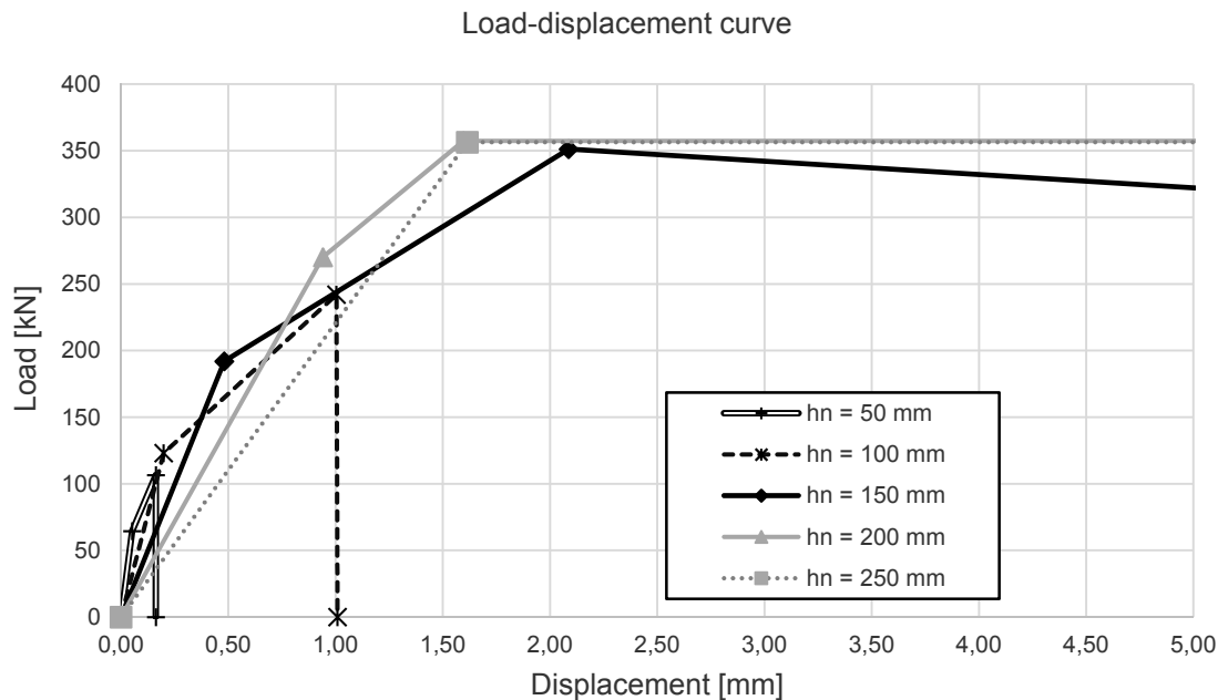
Fig. 4.14: Load-displacement curve of the tensional component for variation of the effective height
