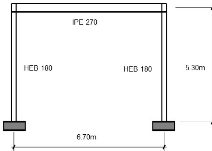
Fig. 9.33 Designed portal frame
