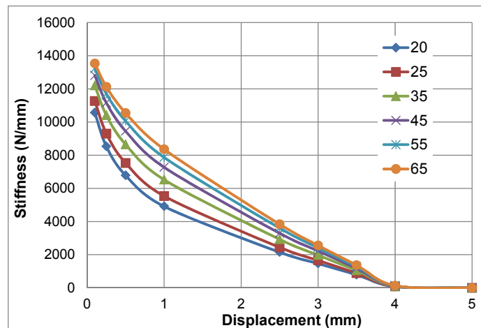
Fig. 4.1: Influence of Concrete Strength f_{ck} on stiffness of anchorage without supplementary reinforcement
