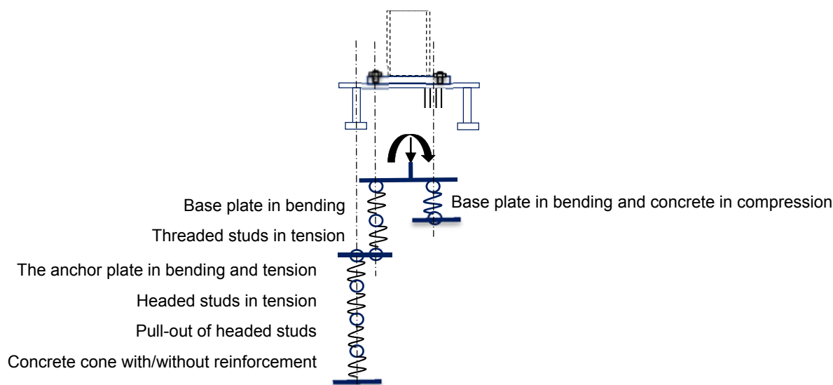
Fig. 6.5 Deformational springs representing in the model the components
