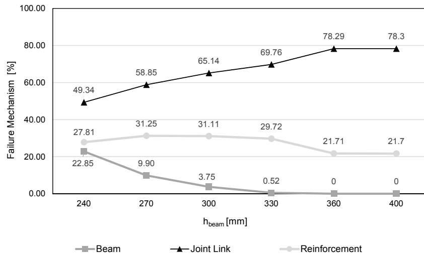
Fig. 4.52: Influence of h_{beam}
