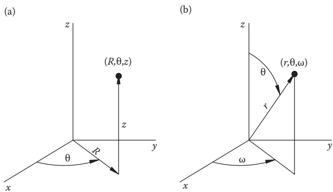
FIGURE A.1 Relationship between Cartesian coordinates and (a) cylindrical coordinates and (b) spherical coordinates.
