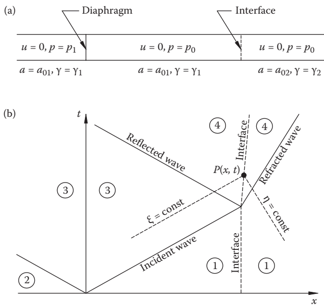
FIGURE 12.4 Shock tube with gas interface and xt diagram subsequent to bursting the diaphragm.
