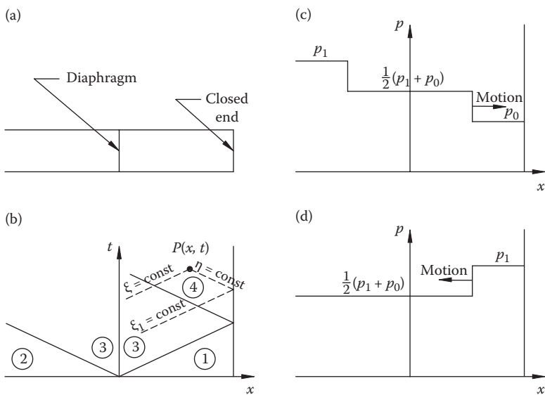
FIGURE 12.3 (a) Shock tube, (b) xt diagram; (c) pressure distribution at some time and (d) at a later time.
