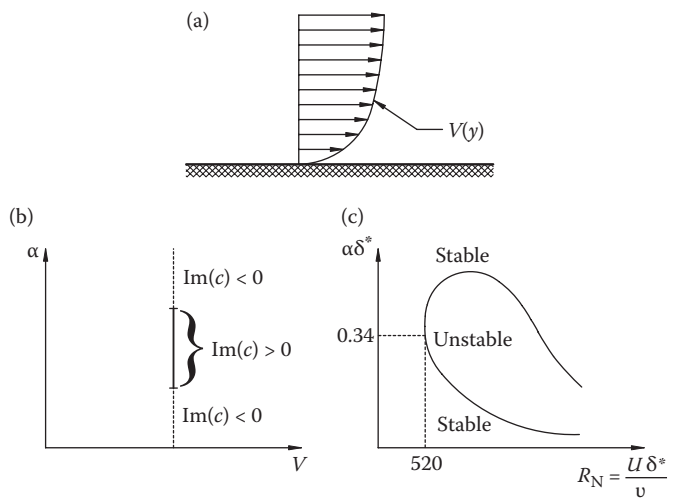
FIGURE 9.9 (a) Undisturbed boundary-layer velocity profile, (b) stability calculation results for fixed V , and (c) stability diagram.
