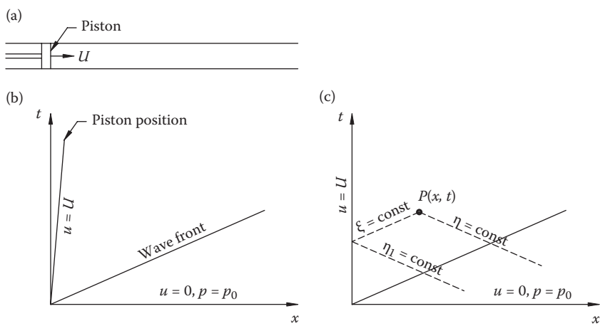
FIGURE 12.5 (a) Piston and cylinder, (b) actual xt diagram, and (c) linearized xt diagram.
