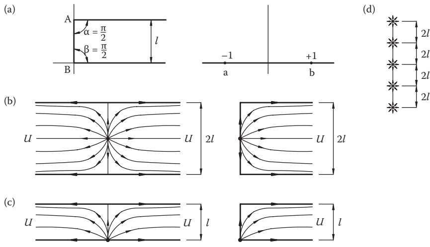
FIGURE 4.20 (a) Mapping planes for a source in a channel, (b) flow field for a full or semi-infinite channel, (c) flow field for the source at the wall, and (d) infinite array of sources.
