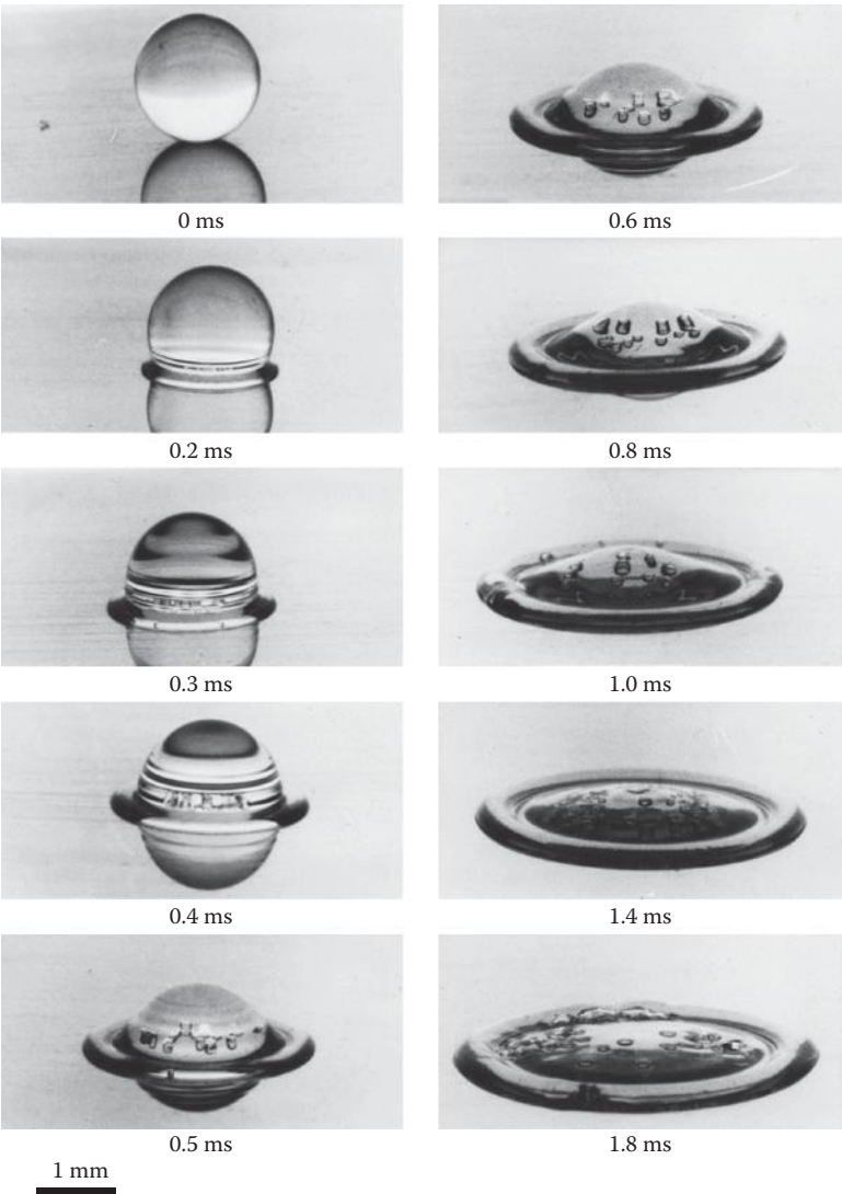
FIGURE 8.3 Heptane droplet striking a stainless steel surface at a temperature of 160°C. (Courtesy of Professor Sanjeev Chandra, University of Toronto, Toronto, Canada.)
