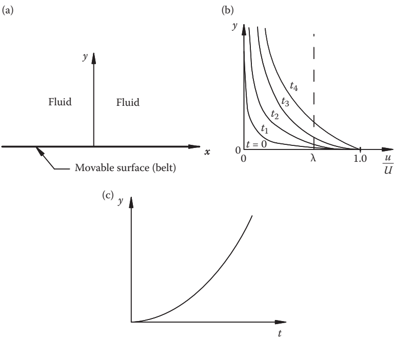
FIGURE 14.5 (a) Definition sketch for an impulsively moving surface, (b) expected form of the solution curves, and (c) typical curve that represents u/U = \text{constant} .
