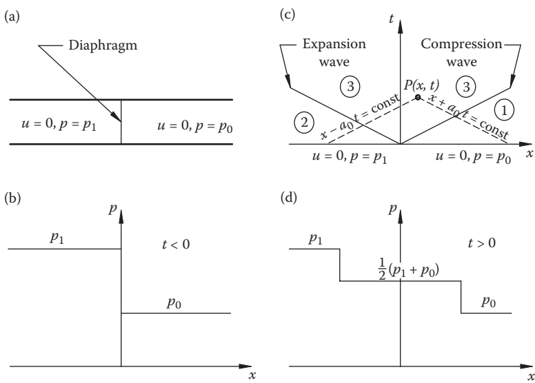
FIGURE 12.2 (a) Shock tube, (b) initial pressure distribution, (c) xt diagram, and (d) typical pressure distribution for t > 0 .
