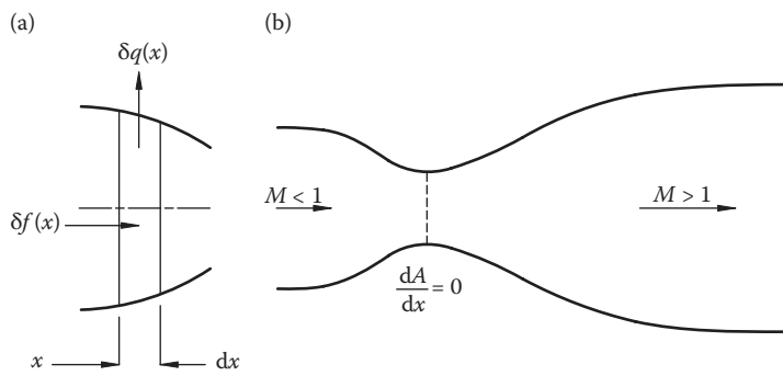
FIGURE 12.7 (a) Element of one-dimensional flow field and (b) flow through a typical nozzle.
