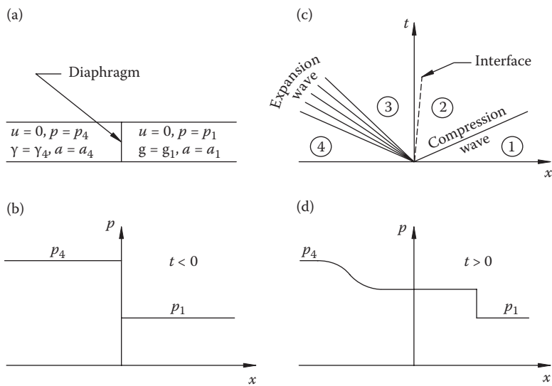
FIGURE 12.6 (a) Shock tube configuration, (b) initial pressure distribution, (c) xt diagram, and (d) typical pressure distribution for t > 0 .
