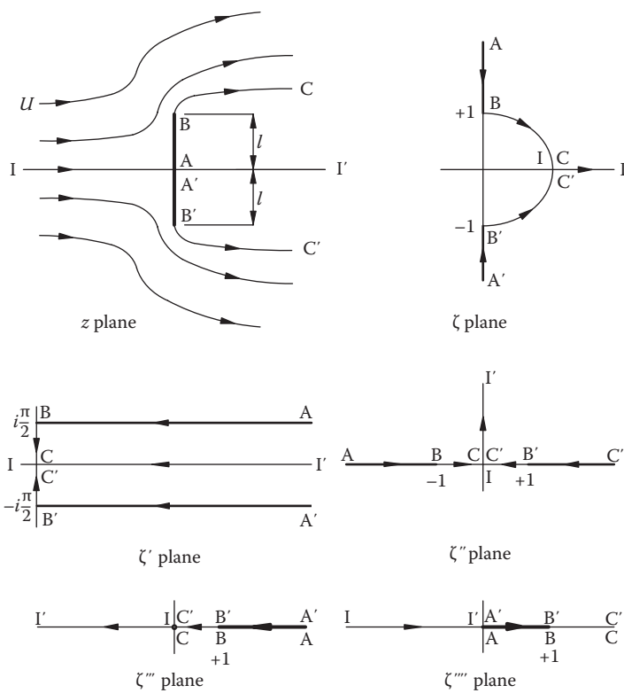
FIGURE 4.22 Mapping planes for flow over a flat plate that is oriented perpendicular to a uniform flow.
