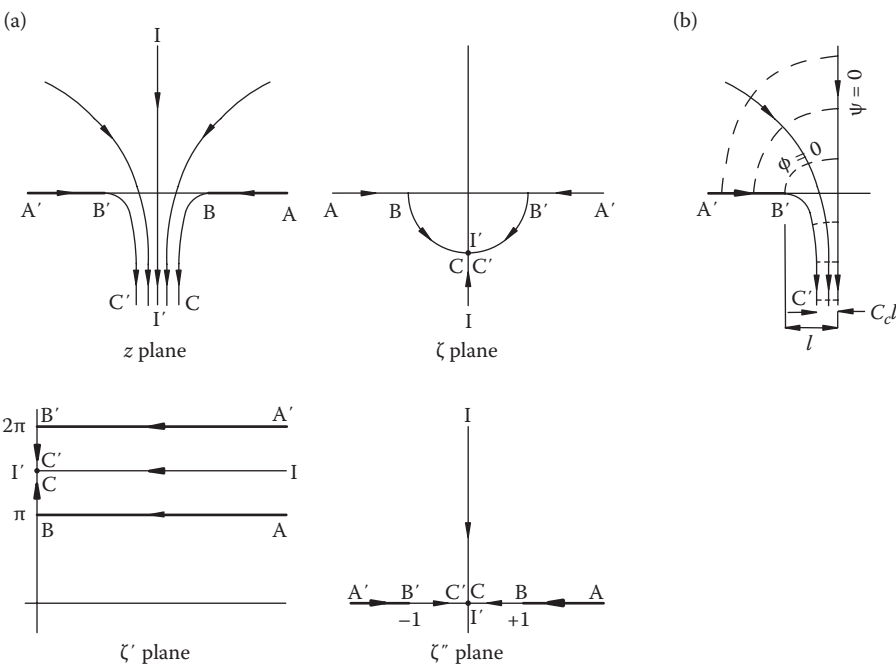
FIGURE 4.21 (a) Mapping planes for flow through a slit and (b) geometry of one of the free bounding streamlines.
