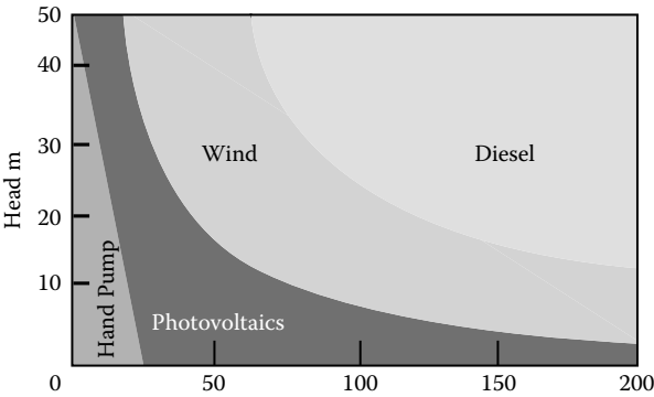
FIGURE 6.20 Competitive ranges for water-pumping systems in terms of hydraulic power (m 4 /day).
