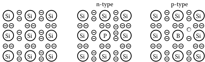
FIGURE 6.2 Semiconductors doped with phosphorus and boron. Electrons are - , and holes are \bigcirc , which are treated as a positive charge with a mass essentially the same as the electron mass.
