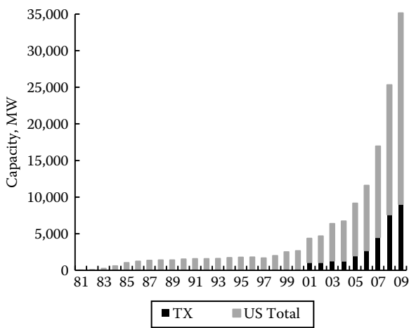
FIGURE 9.13 Wind power installed in the United States, primarily wind farms.
