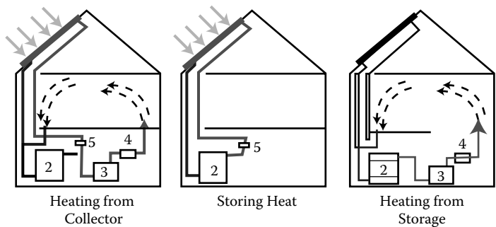
FIGURE 5.13 Active solar heating system using air for heat transport.
