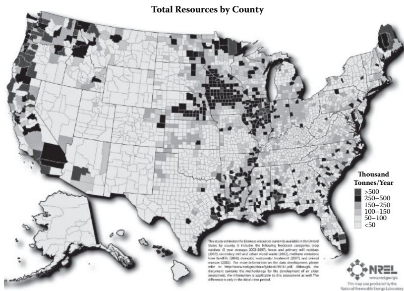
FIGURE 10.3 Biomass resource by county for the United States. (Map from NREL, http://www.nrel.gov/biomass .)
