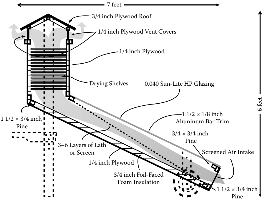
FIGURE 5.22 Diagram of indirect solar food dryer, based on design, Appalachian State University, 1997.
