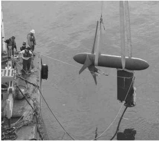
FIGURE 12.15 Tidal turbine, 35 kW, being installed in East River, New York City. (Courtesy of Verdant Power.)
