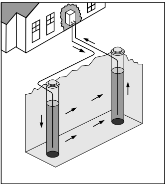
FIGURE 11.10 Geothermal heat pump, open-loop system.
