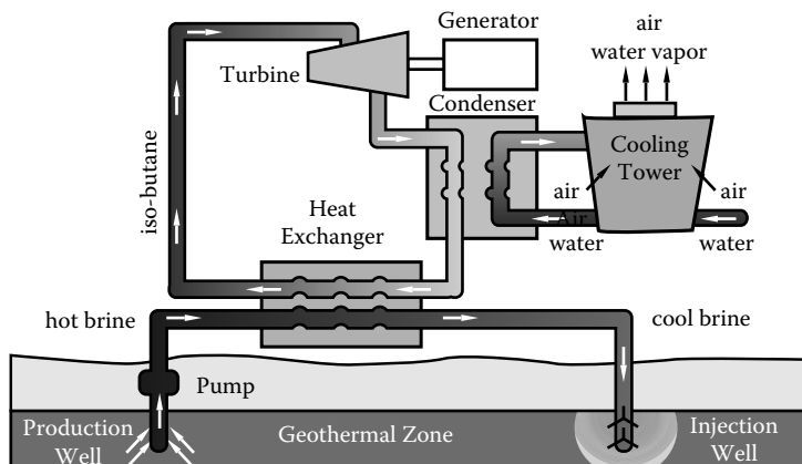
FIGURE 11.19 Diagram of a binary geothermal system.
