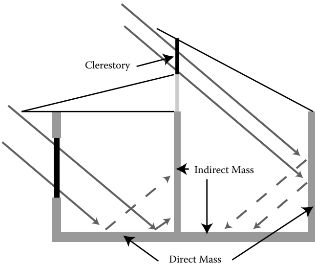
FIGURE 5.6 Direct gain through south-facing windows and clerestory. Clerestory gives direct gain into rooms that are not on the south side of the house. Overhangs shade windows in the summer.
