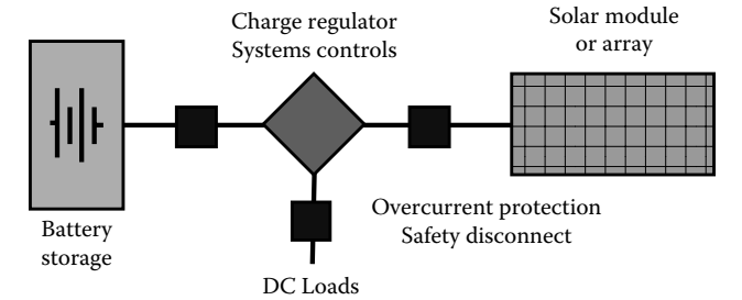
FIGURE 6.18 Diagram of simple PV system for lights, radio, and television.
