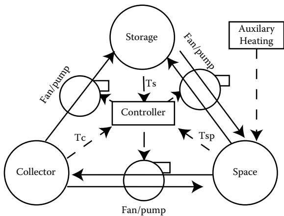
FIGURE 5.11 Diagram of an active solar heating system.
