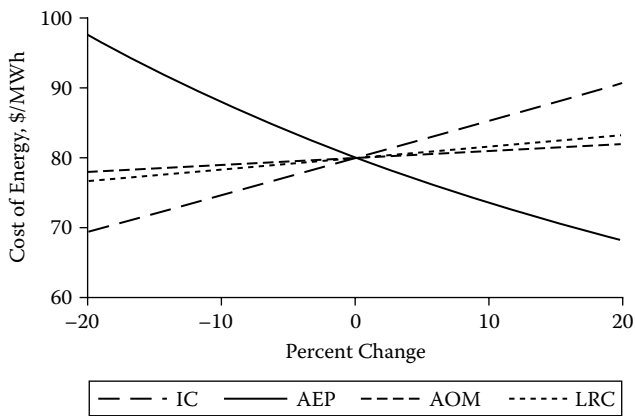
FIGURE 15.1 Sensitivity analysis for the example COE (COE = $93/MWh).
